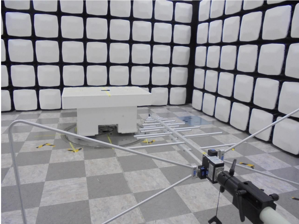
NFC Radiated Test Setup Photo(30 MHz ~ 1 GHz)
