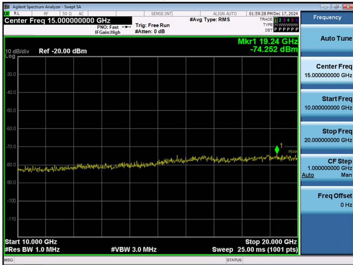
LTE B2_15 M_Conducted Spurious(Above10 G)_Mid_QPSK_1RB
