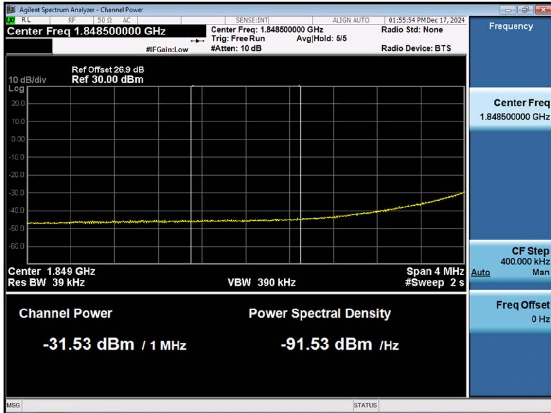
LTE B2_15 M_Extended Band Edge_Low_QPSK_FullRB
