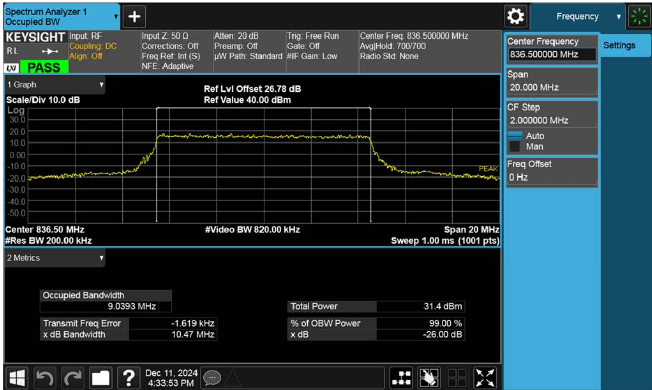
BAND 26. Occupied Bandwidth Plot (10 M BW Ch.26915 QPSK_RB50_0)
