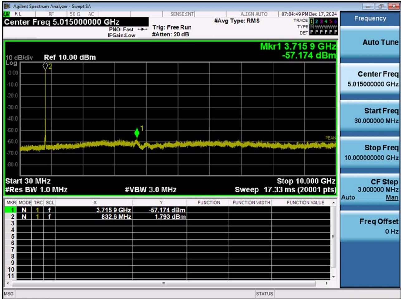
BAND 26. Conducted Spurious Plot (26915ch_10 MHz_QPSK_RB 1_0)
