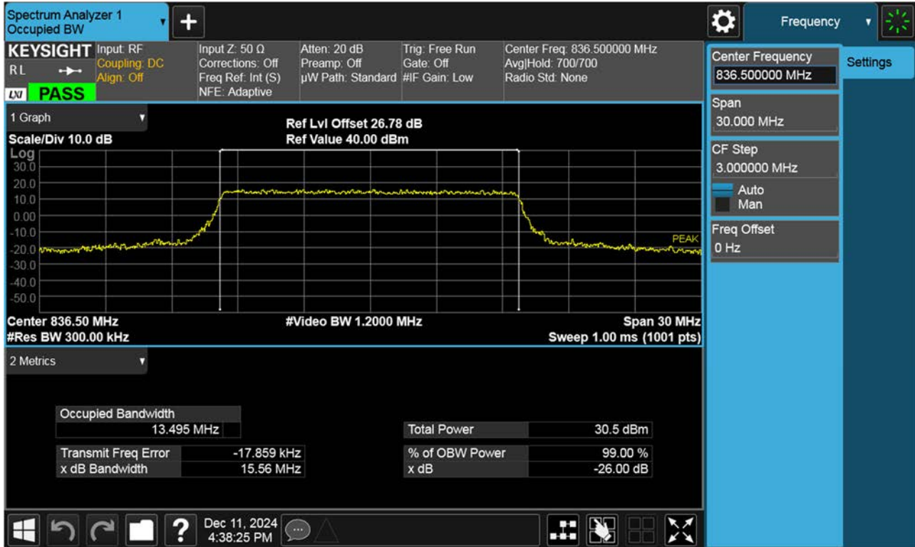
BAND 26. Occupied Bandwidth Plot (15 M BW Ch.26915 16QAM RB 75_0)
