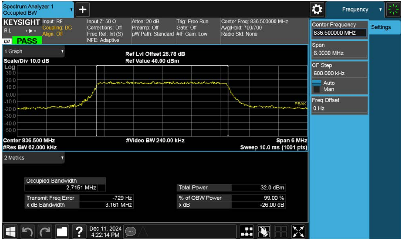
BAND 26. Occupied Bandwidth Plot (3 M BW Ch.26915 QPSK_RB15_0)
