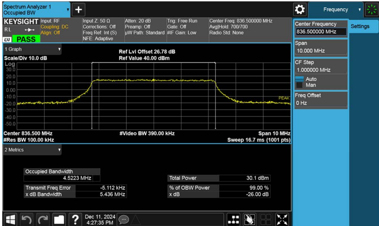
BAND 26. Occupied Bandwidth Plot (5 M BW Ch.26915 64QAM_RB25_0)
