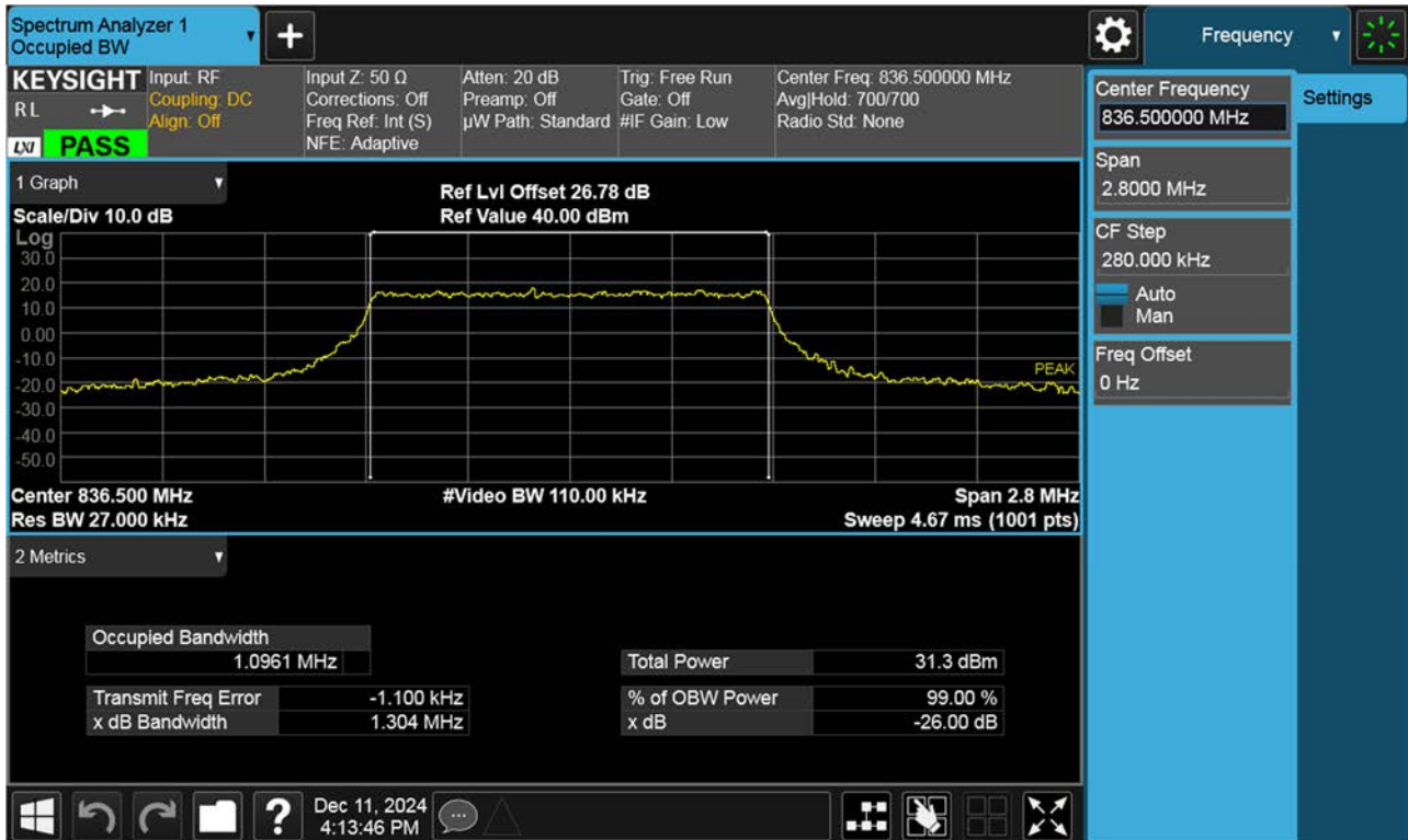
BAND 26. Occupied Bandwidth Plot (1.4 M BW Ch.26915 QPSK_RB6_0)
