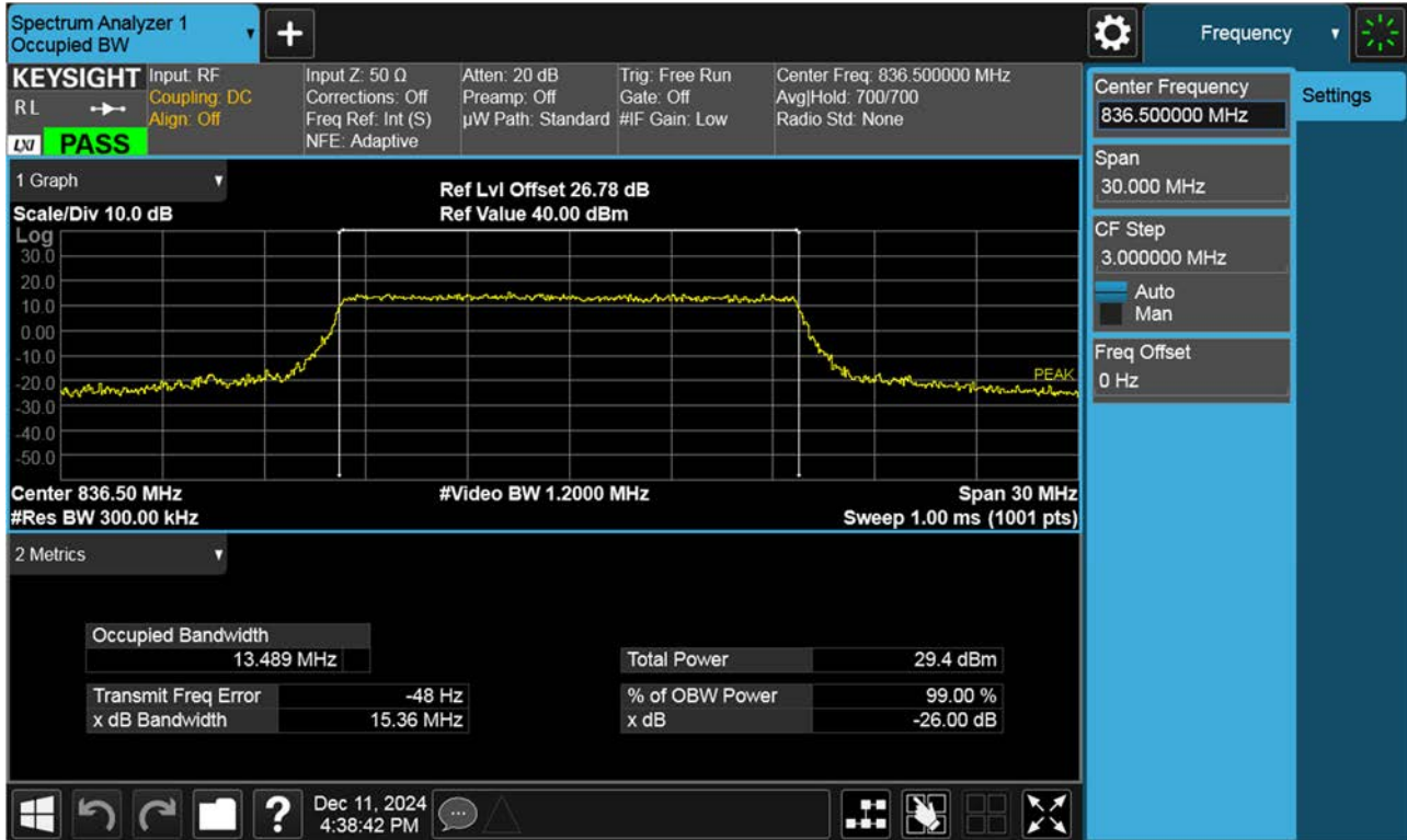
BAND 26. Occupied Bandwidth Plot (15 M BW Ch.26915 64QAM RB 75_0)
