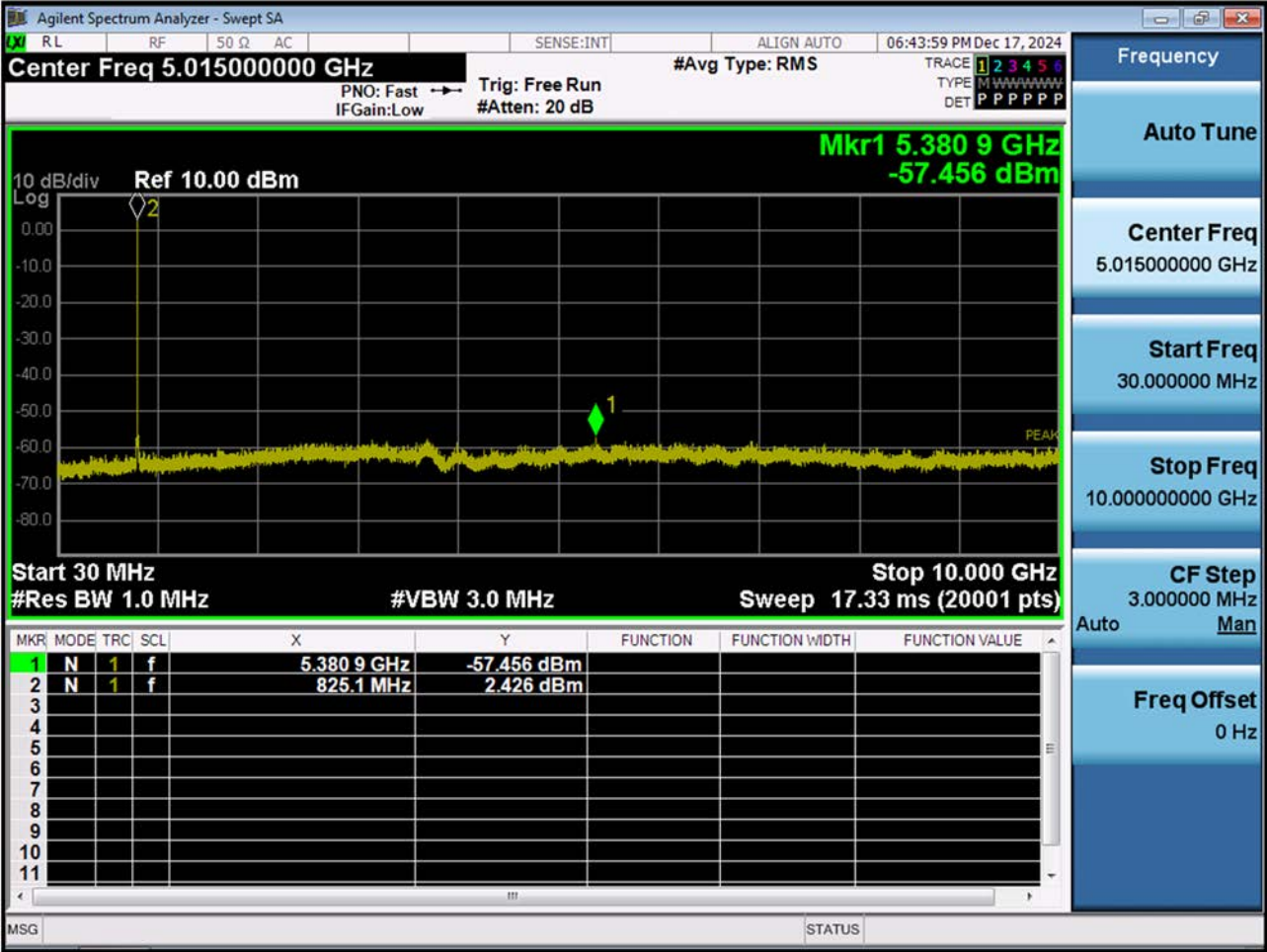
BAND 26. Conducted Spurious Plot (26797ch_1.4 MHz_QPSK_RB 1_0)
