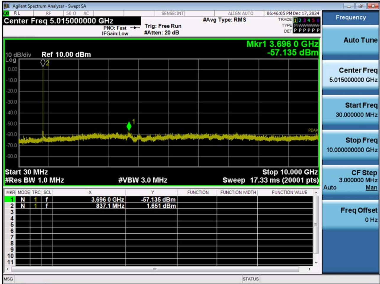
BAND 26. Conducted Spurious Plot (26915ch_1.4 MHz_QPSK_RB 1_0)
