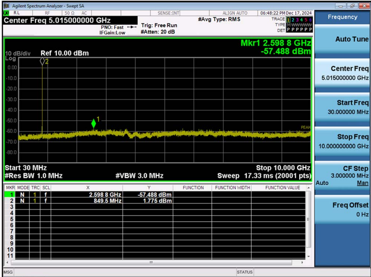
BAND 26. Conducted Spurious Plot (27033ch_1.4 MHz_QPSK_RB 1_0)
