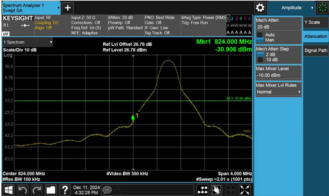
BAND 26. Lower Band Edge Plot (10 M BW Ch.26840 QPSK_RB1_Offset 0)
