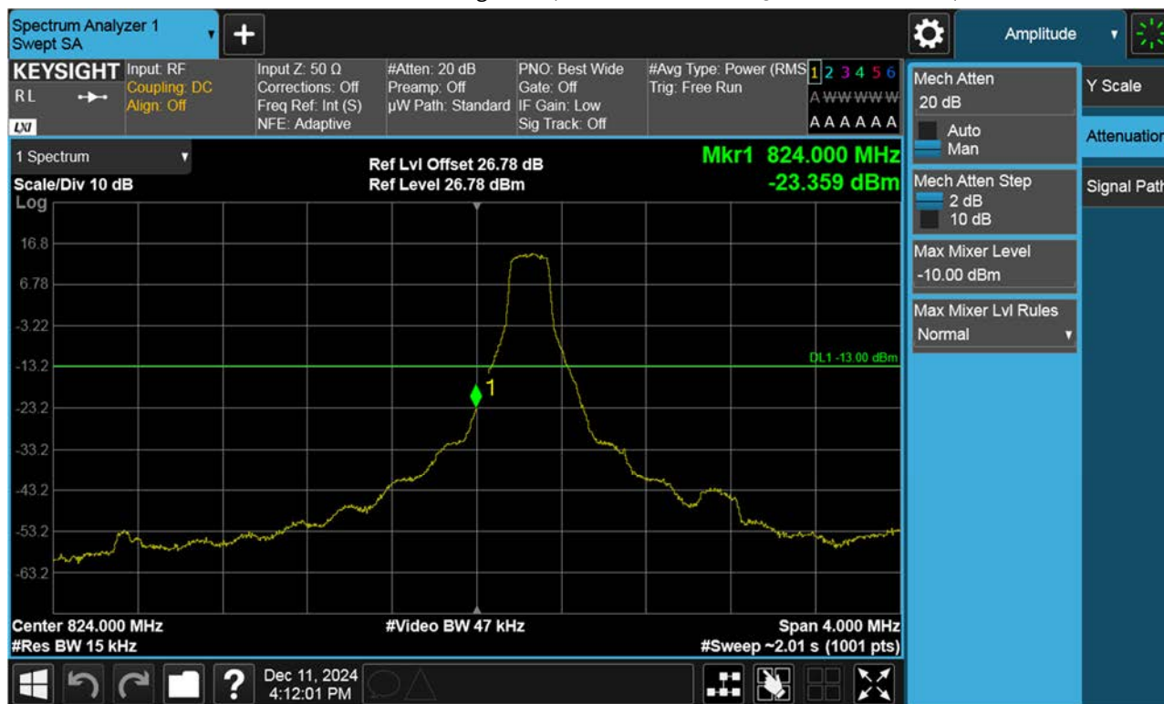
BAND 26. Lower Band Edge Plot (1.4 M BW Ch.26797 QPSK_RB1_Offset 0)
