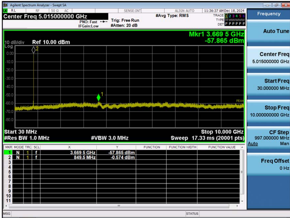
LTE B5_1.4M_Conducted Spurious(30 M-10 G)_High_QPSK_1RB
