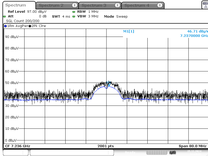
Radiated Spurious Emissions plot – Average Result (802.11b_1 Mbps, Ch.1 3rd Harmonic, Z-V)
