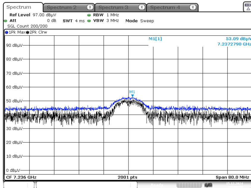
Radiated Spurious Emissions plot – Peak Result (802.11b_1 Mbps, Ch.1 3rd Harmonic, Z-V)
