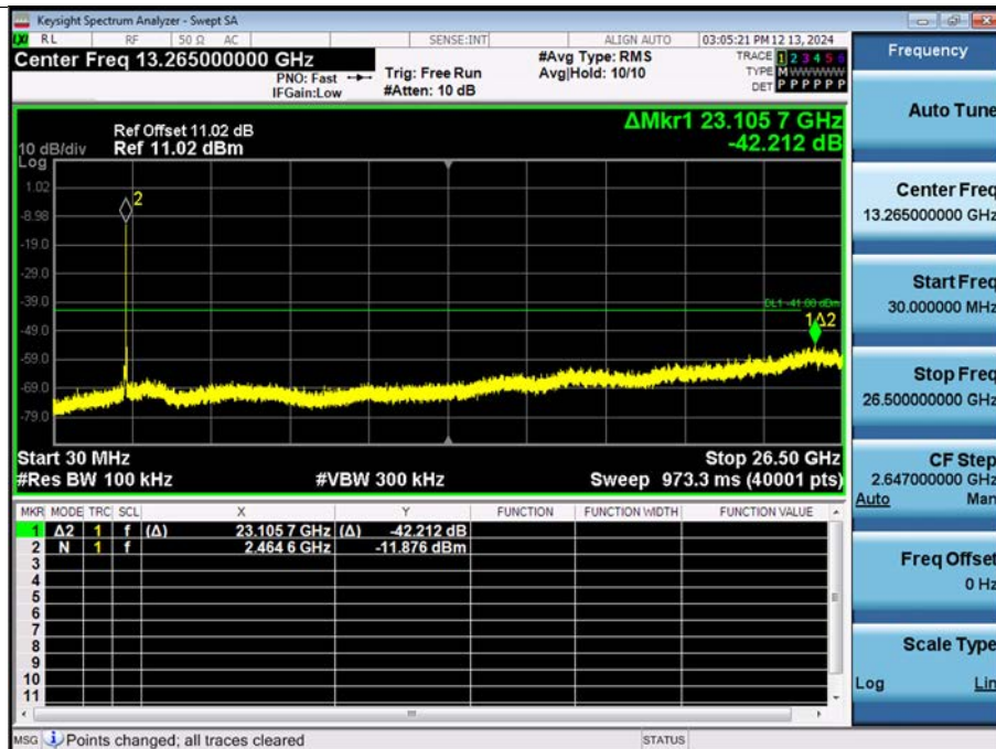
MIMO_SDM(Ant. 2) BW20M Ch.13(2 472 MHz) 26T RU 0
