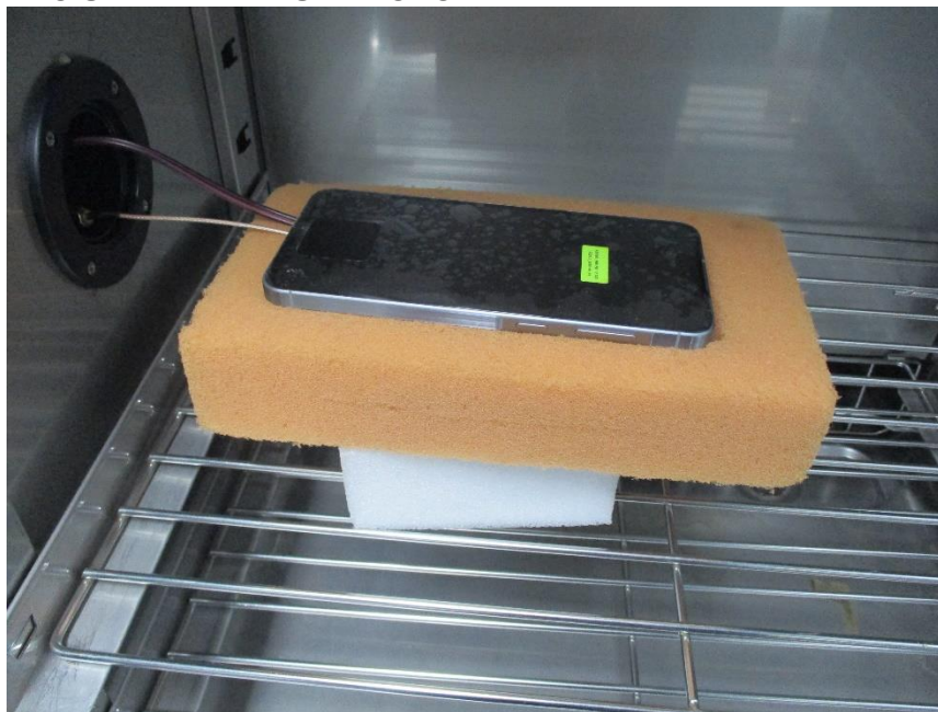
NFC STABILITY TEST PHOTO
