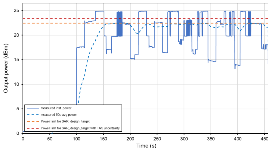
Time-Averaged Conducted Power Test Sequence B Tech: NR, Band 5
