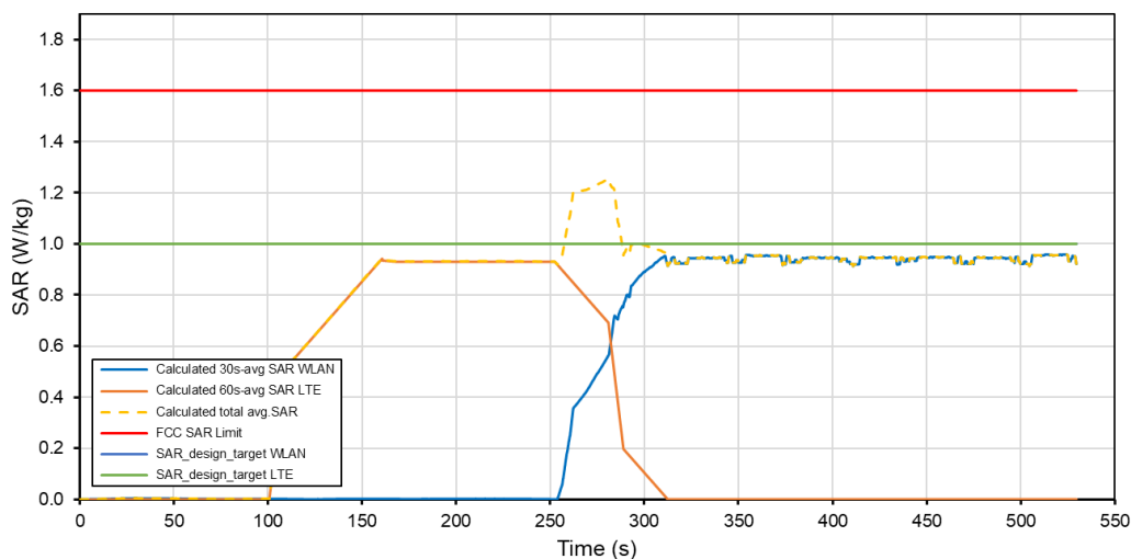
Total Time-Averaged SAR WLAN and WWAN Coex 2 Tech: WLAN 2.4GHz / LTE Band 41
