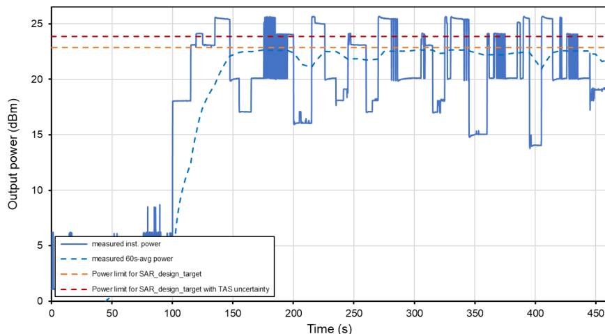
Time-Averaged Conducted Power Test Sequence B Tech: LTE, Band 12
