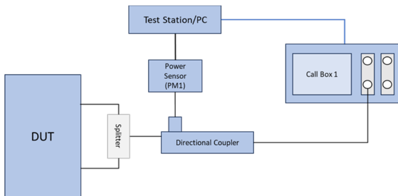
(b) Appendix A – Test Setup Photo 3
