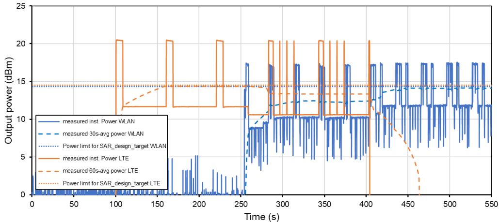
Time-Averaged Conducted Power WLAN and WWAN Coex 1 Tech: WLAN 2.4GHz / LTE Band 41
