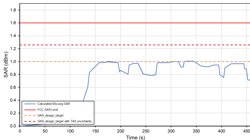
Total Time-Averaged SAR Test Sequence B Tech: NR, Band 77
