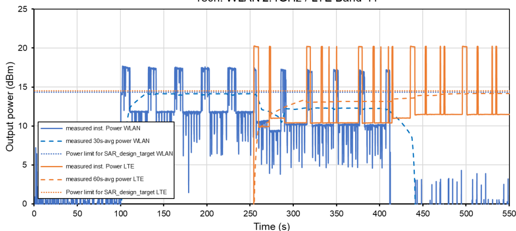
Time-Averaged Conducted Power WLAN and WWAN Coex 3 Tech: WLAN 2.4GHz / LTE Band 41
