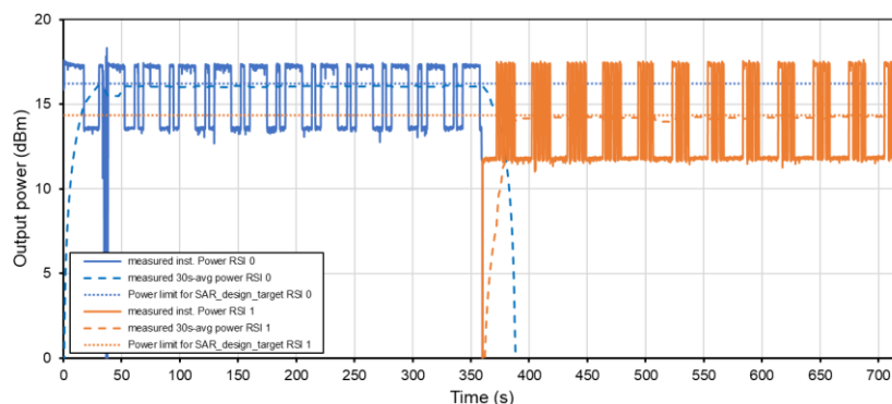
Time-Averaged Conducted Power WLAN 2.4GHz
