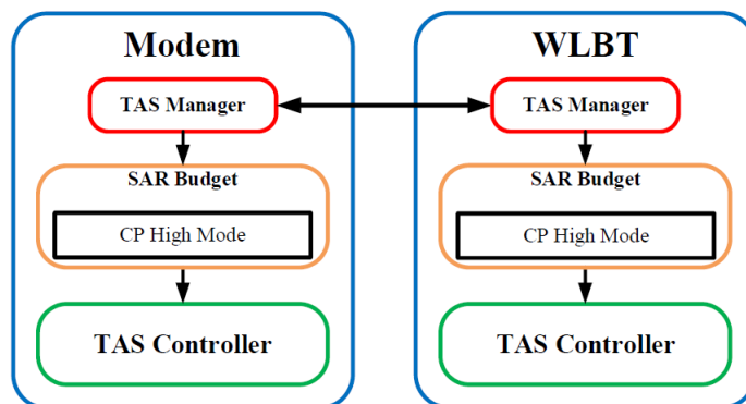
Figure 1.3-1 DC-TAS architecture
