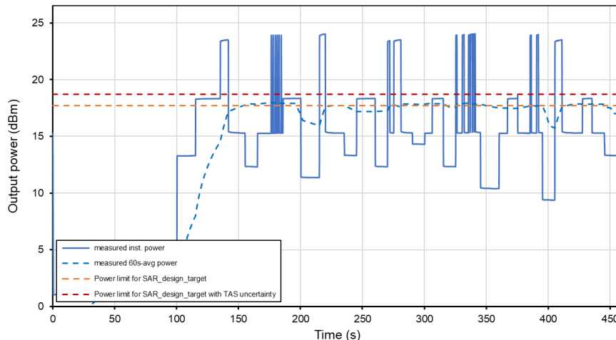
Time-Averaged Conducted Power Test Sequence B Tech: WCDMA, Band 4
