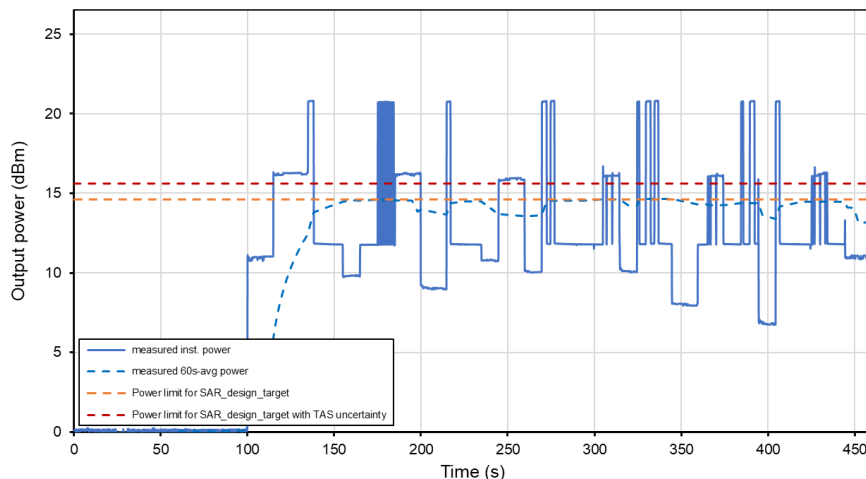
Time-Averaged Conducted Power Test Sequence B Tech: NR, Band 77
