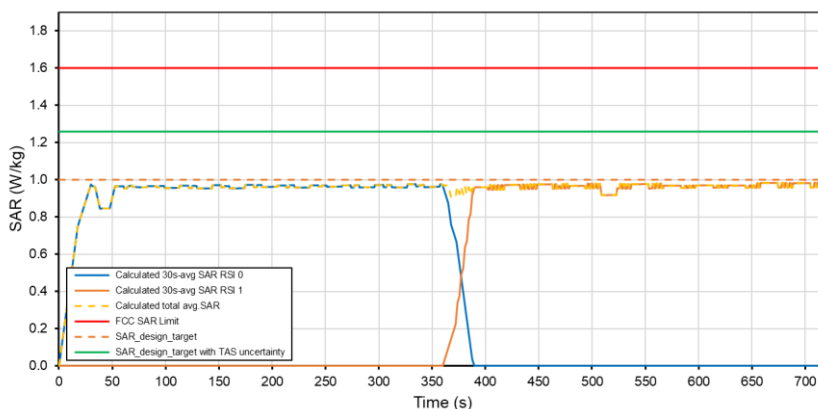
Total Time-Averaged SAR WLAN 2.4GHz
