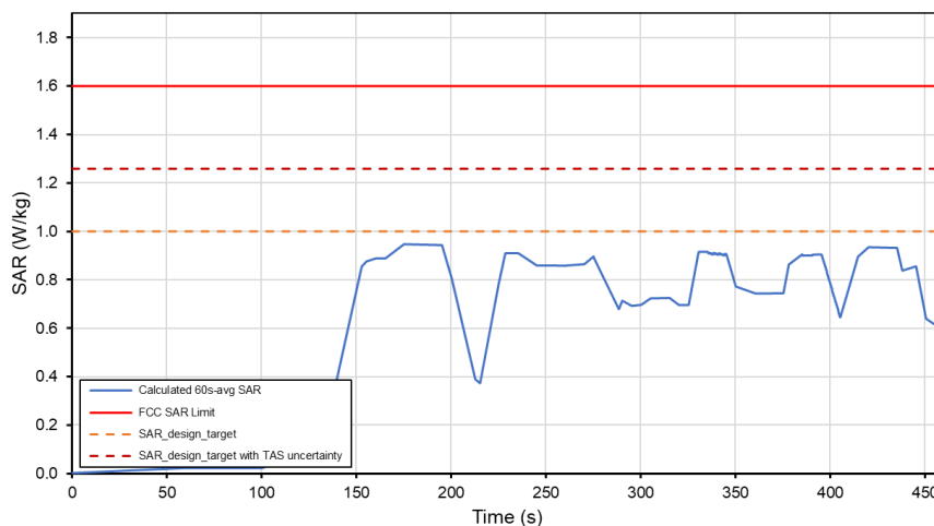
Total Time-Averaged SAR Test Sequence B Tech: LTE, Band 41 PC3
