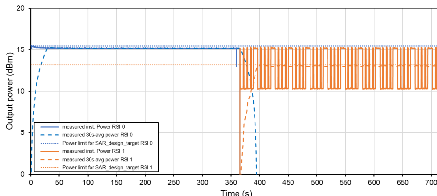
Time-Averaged Conducted Power WLAN 5GHz
