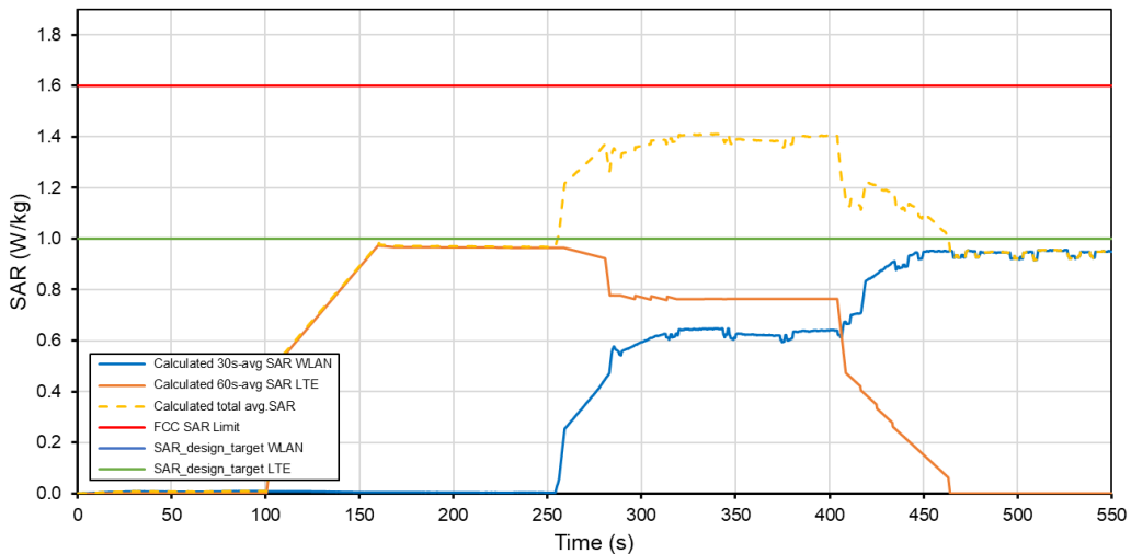
Total Time-Averaged SAR WLAN and WWAN Coex 1 Tech: WLAN 2.4GHz / LTE Band 41
