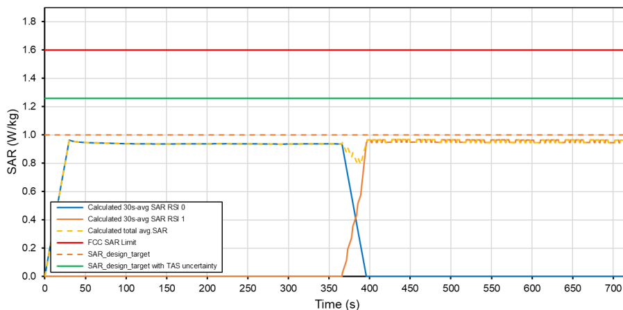
Total Time-Averaged SAR WLAN 5GHz
