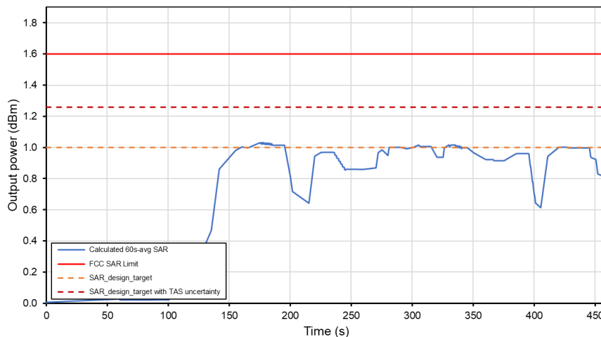
Total Time-Averaged SAR Test Sequence B Tech: WCDMA, Band 4
