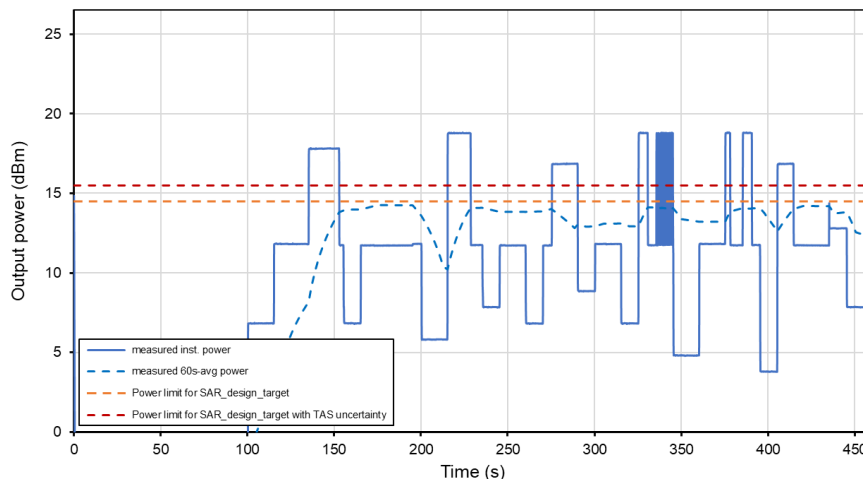
Time-Averaged Conducted Power Test Sequence B Tech: LTE, Band 41 PC3
