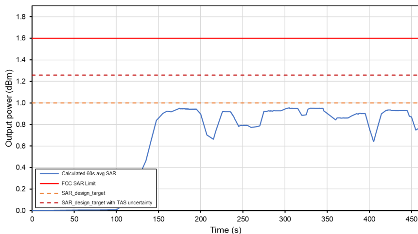
Total Time-Averaged SAR Test Sequence B Tech: LTE, Band 12
