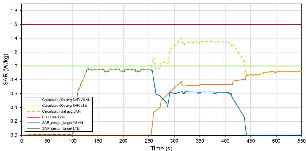
Total Time-Averaged SAR WLAN and WWAN Coex 3 Tech: WLAN 2.4GHz / LTE Band 41
