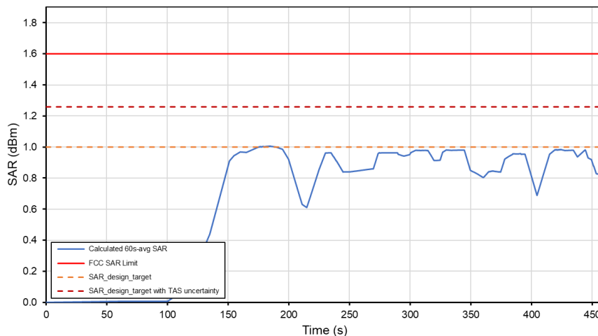
Total Time-Averaged SAR Test Sequence B Tech: NR, Band 5
