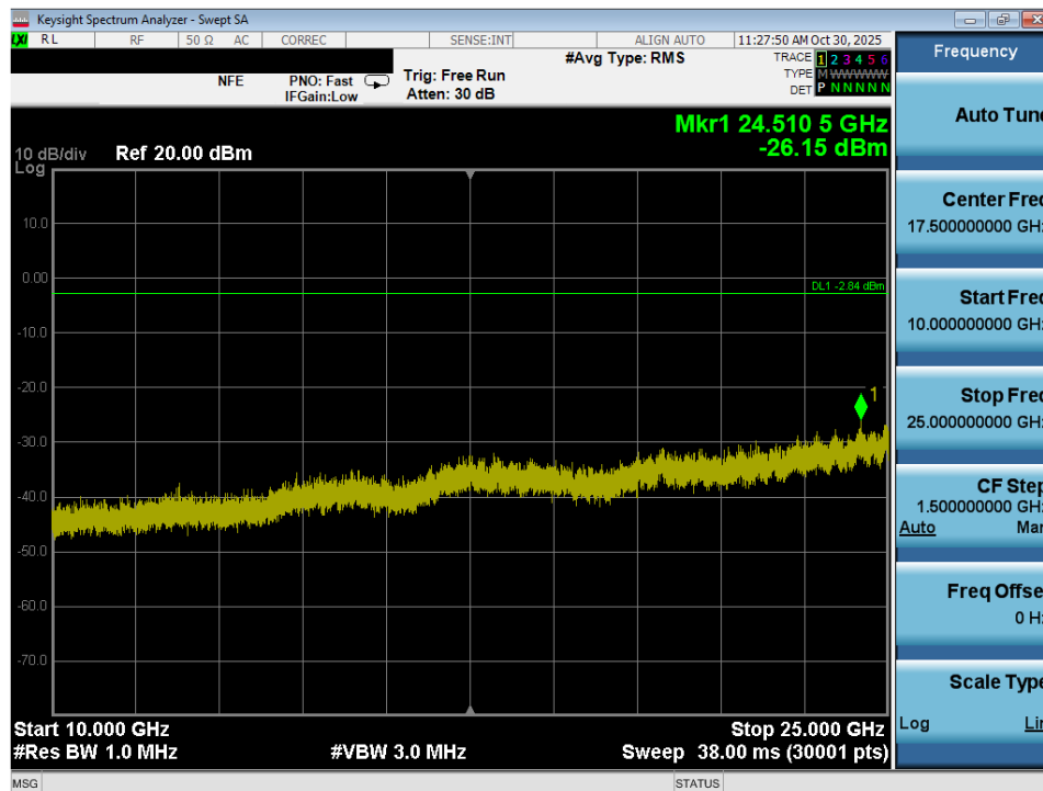
Plot 7-39. Conducted Spurious Plot (Bluetooth, 3Mbps – Ch. 39) – Ant 1
