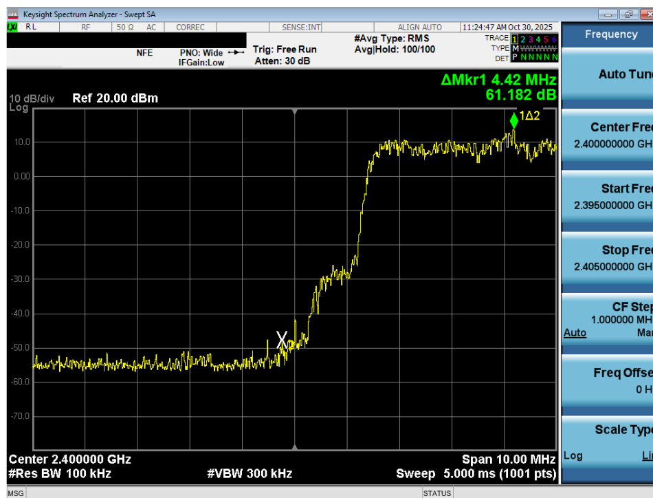
Plot 7-30. Band Edge Plot (Bluetooth with Hopping Enabled, 3 Mbps) – Ant 1
