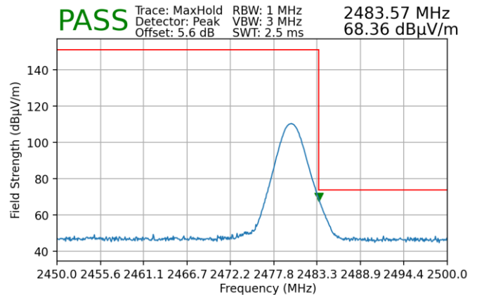
Plot 7-47. Radiated Restricted Upper Band Edge Measurement (Peak)
