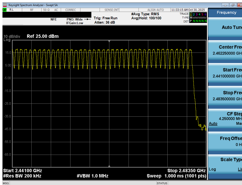
Plot 7-35. High End Spectrum Channel Hopping Plot (Bluetooth) – Ant 1
