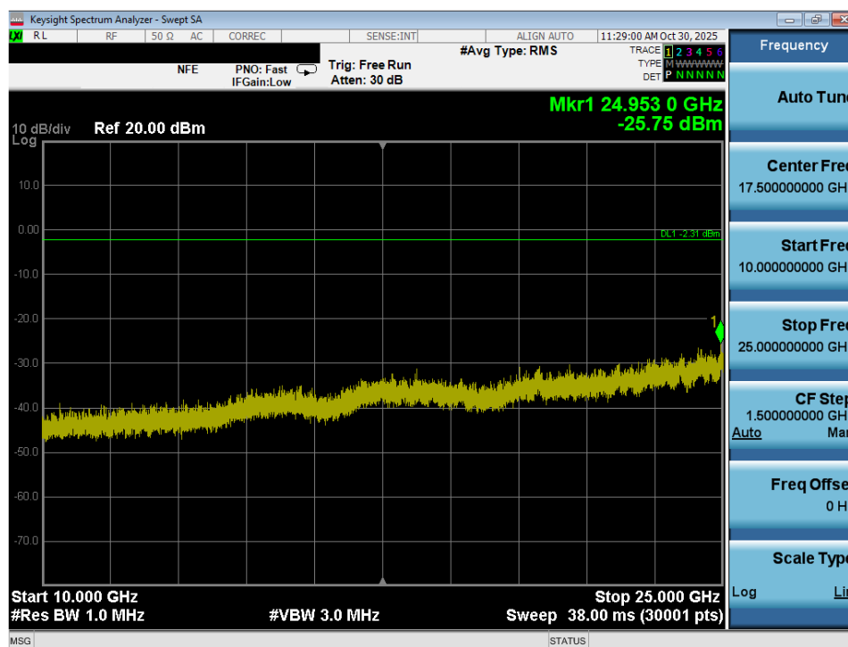
Plot 7-41. Conducted Spurious Plot (Bluetooth, 3Mbps – Ch. 78) – Ant 1
