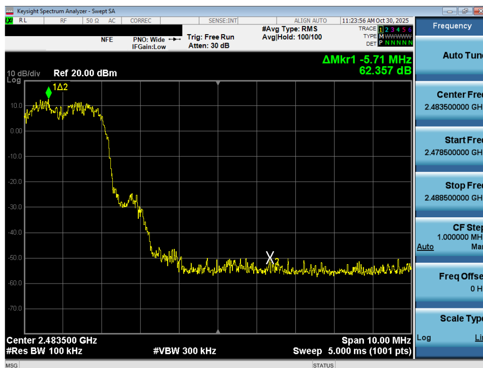
Plot 7-31. Band Edge Plot (Bluetooth with Hopping Enabled, 3 Mbps) – Ant 1
