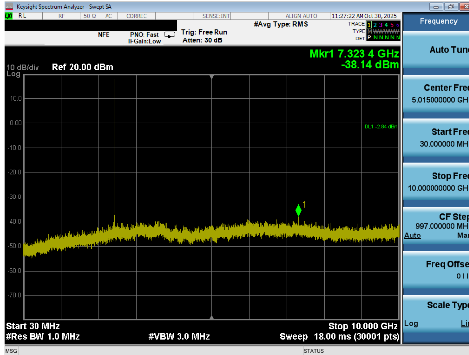
Plot 7-38. Conducted Spurious Plot (Bluetooth, 3Mbps – Ch. 39) – Ant 1
