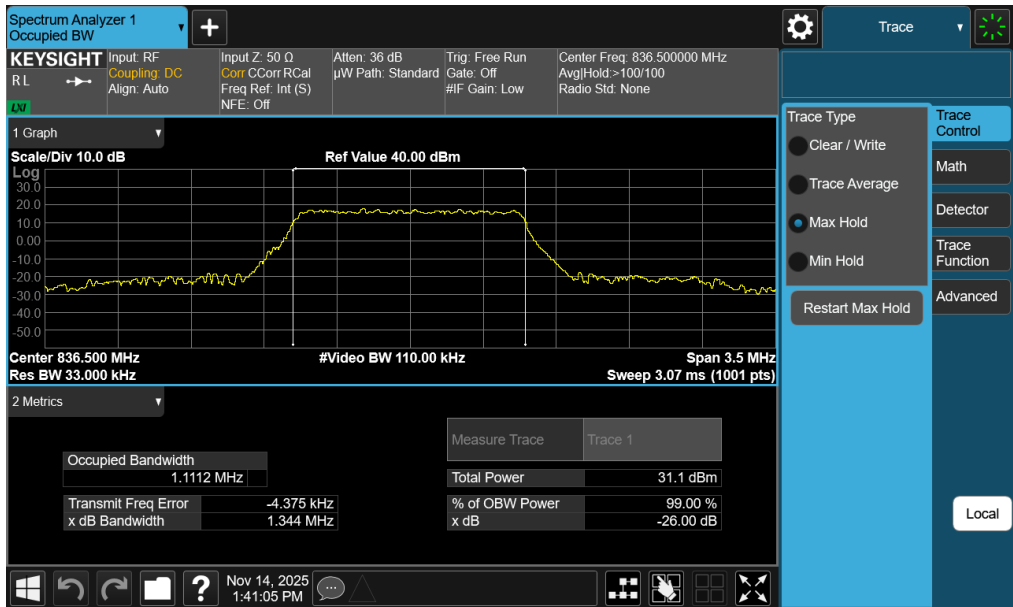
Plot 7-34. Occupied Bandwidth Plot (LTE Band 26/5 - 1.4MHz QPSK - Full RB - Ant2)
