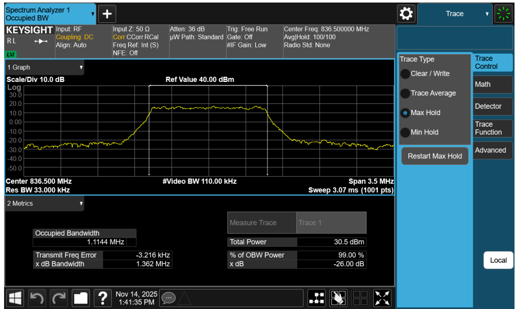
Plot 7-35. Occupied Bandwidth Plot (LTE Band 26/5 - 1.4MHz 16-QAM - Full RB - Ant2)
