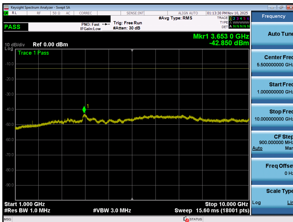
Plot 7-65. Conducted Spurious Plot (NR Band n5 - 20.0MHz - 1 RB - Mid Channel - Ant1)
