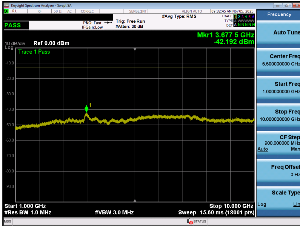
Plot 7-53. Conducted Spurious Plot (LTE Band 26 - 15MHz QPSK - 1 RB - Low Channel – Ant1)
