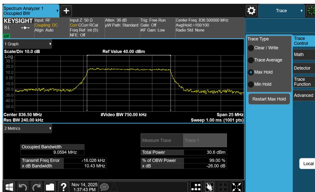
Plot 7-29. Occupied Bandwidth Plot (LTE Band 26/5 - 10MHz 16-QAM - Full RB - Ant2)
