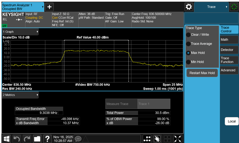
Plot 7-43. Occupied Bandwidth Plot (NR Band n5 - 10MHz QPSK - Full RB - Ant2)
