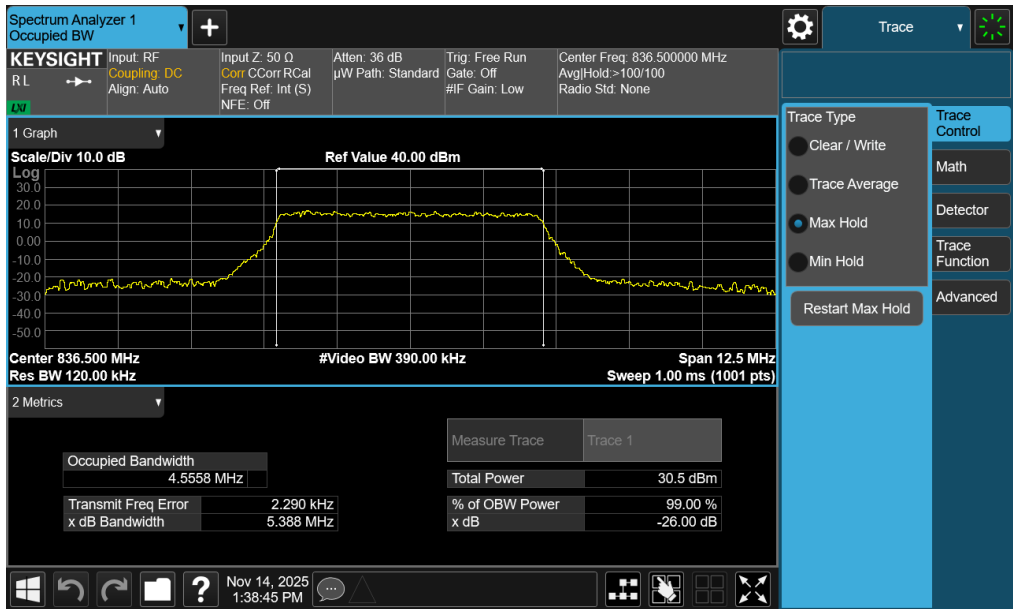
Plot 7-31. Occupied Bandwidth Plot (LTE Band 26/5 - 5MHz 16-QAM - Full RB - Ant2)
