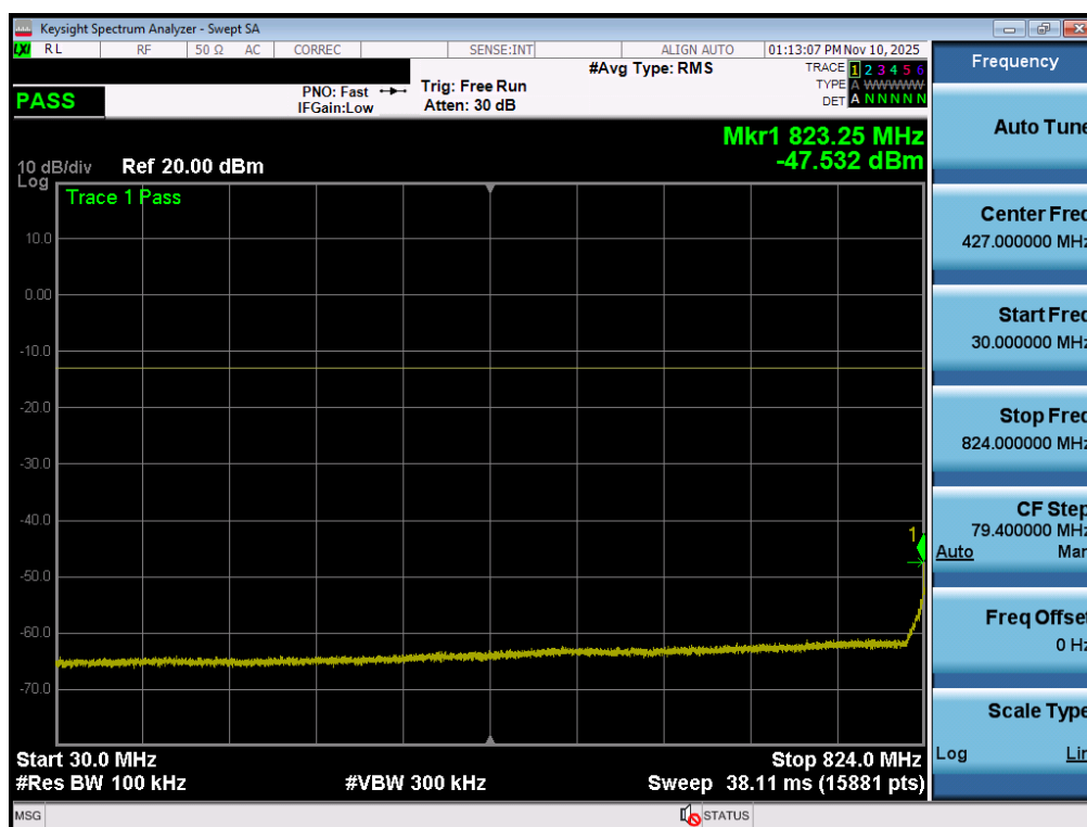
Plot 7-63. Conducted Spurious Plot (NR Band n5 - 20.0MHz - 1 RB - Mid Channel - Ant1)
