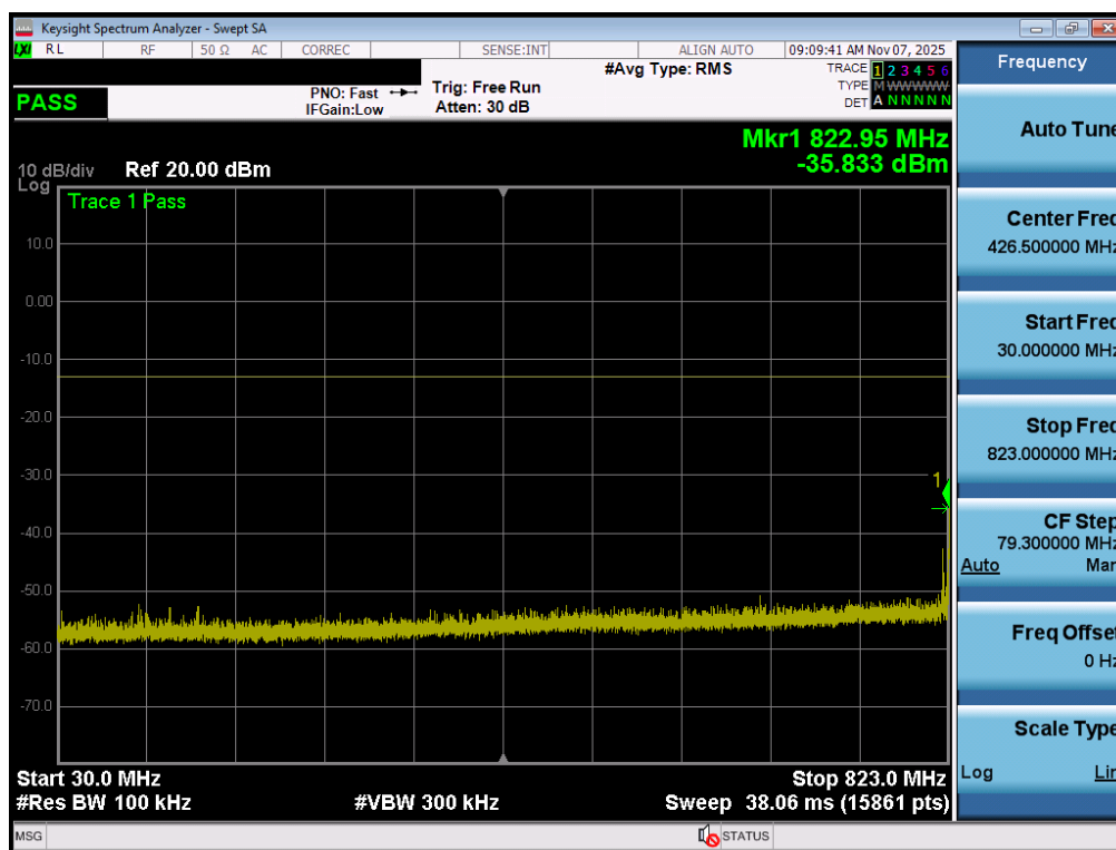
Plot 7-69. Conducted Spurious Plot (GPRS Ch. 128 – Ant1)
