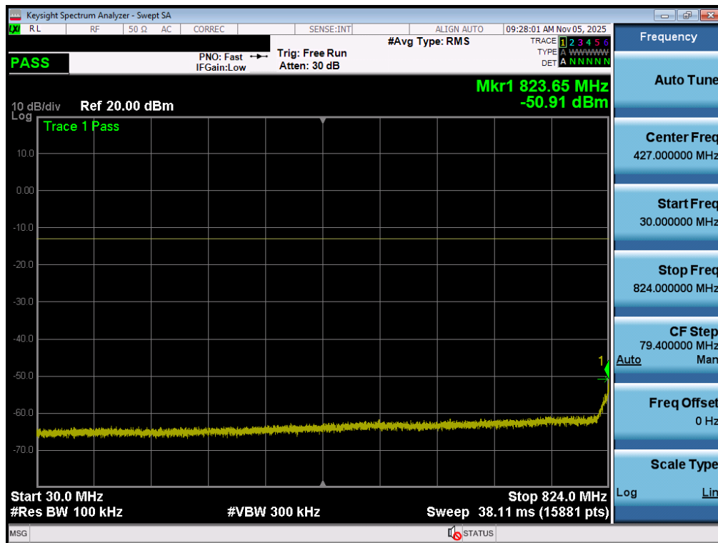
Plot 7-54. Conducted Spurious Plot (LTE Band 26 - 15MHz QPSK - 1 RB - Mid Channel – Ant1)
