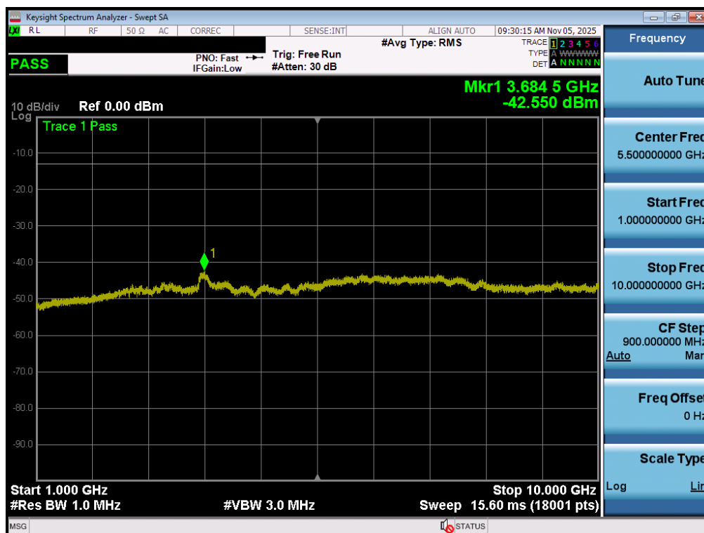
Plot 7-56. Conducted Spurious Plot (LTE Band 26 - 15MHz QPSK - 1 RB - Mid Channel – Ant1)
