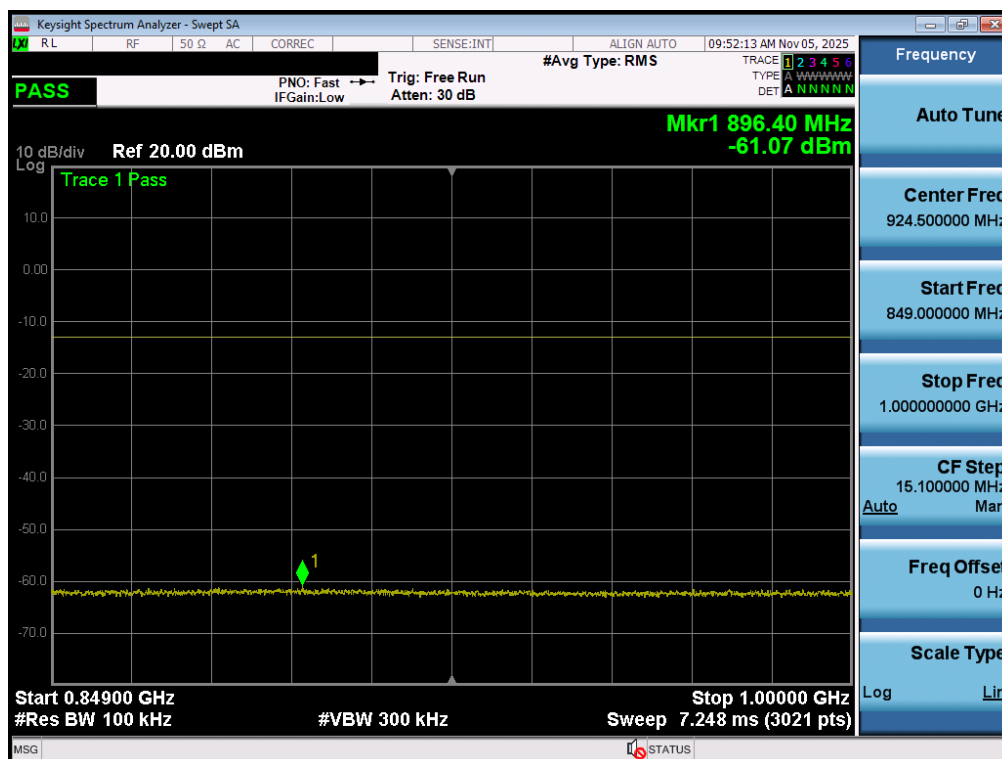
Plot 7-55. Conducted Spurious Plot (LTE Band 26 - 15MHz QPSK - 1 RB - Mid Channel – Ant1)
