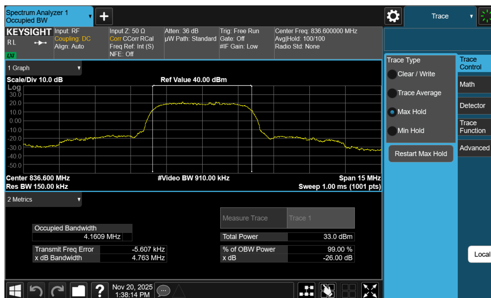
Plot 7-25. Occupied Bandwidth Plot (WCDMA, Ch. 4183 – Ant1)
