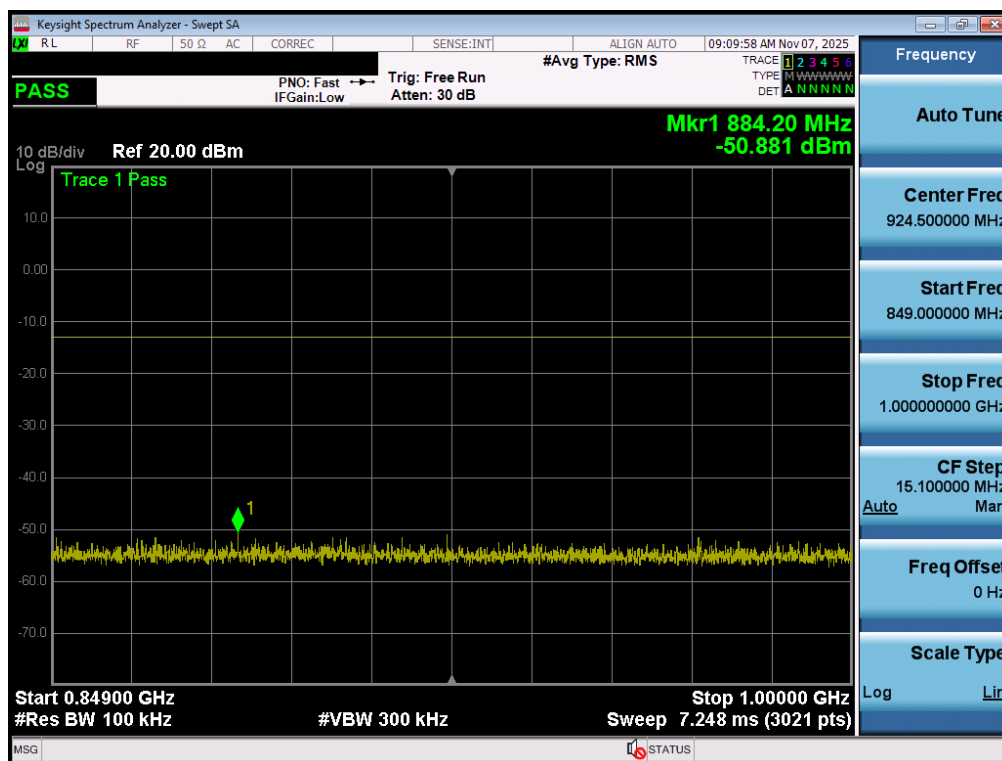
Plot 7-70. Conducted Spurious Plot (GPRS Ch. 128 – Ant1)
