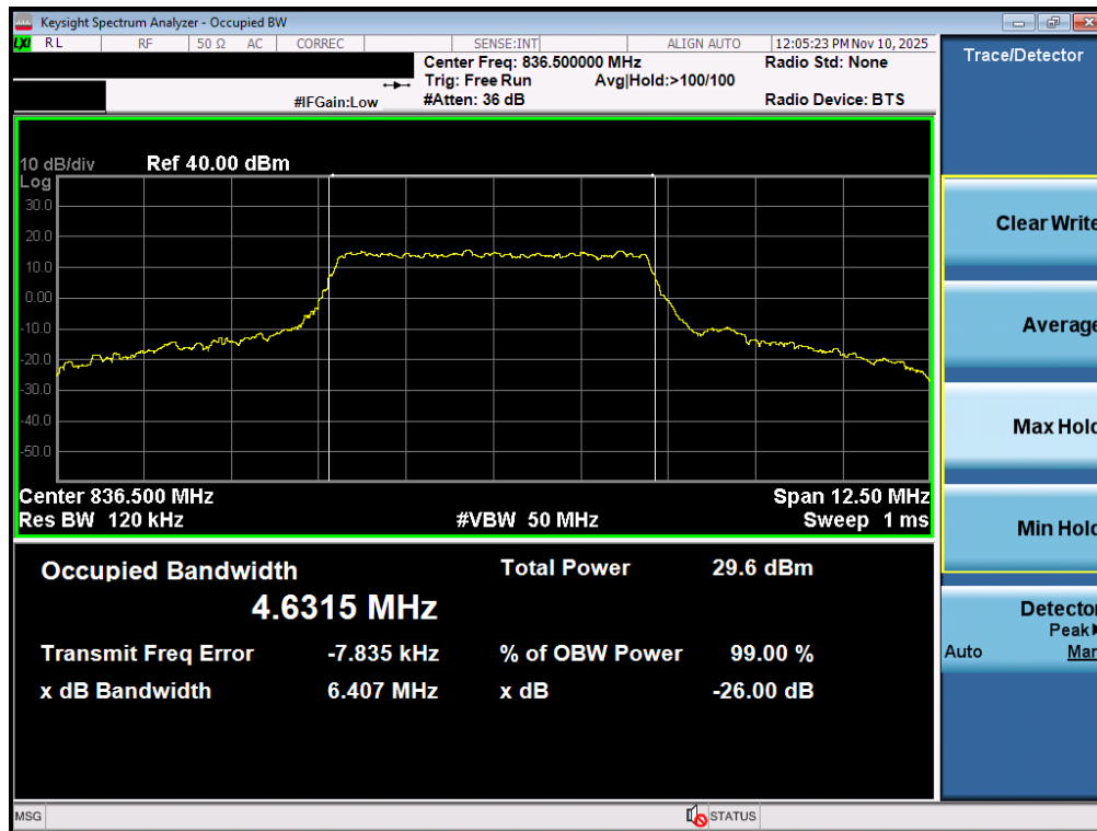
Plot 7-21. Occupied Bandwidth Plot (NR Band n5 - 5MHz QPSK - Full RB - Ant1)
