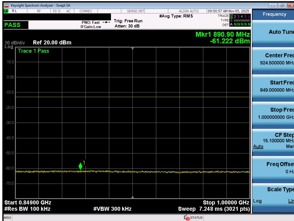
Plot 7-52. Conducted Spurious Plot (LTE Band 26 - 15MHz QPSK - 1 RB - Low Channel – Ant1)
