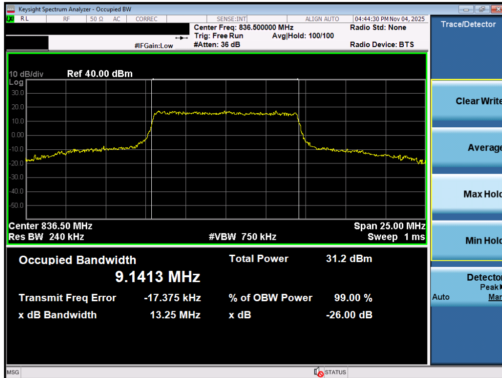
Plot 7-4. Occupied Bandwidth Plot (LTE Band 26/5 - 10MHz 16-QAM - Full RB - Ant1)
