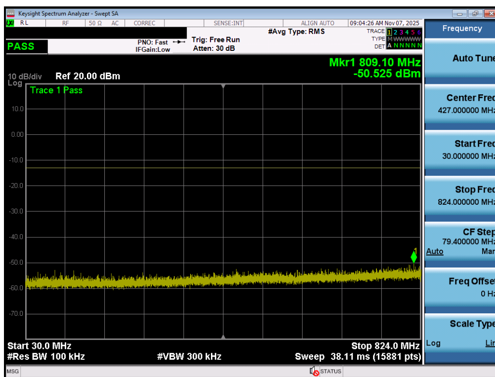
Plot 7-72. Conducted Spurious Plot (GPRS Ch. 190 – Ant1)
