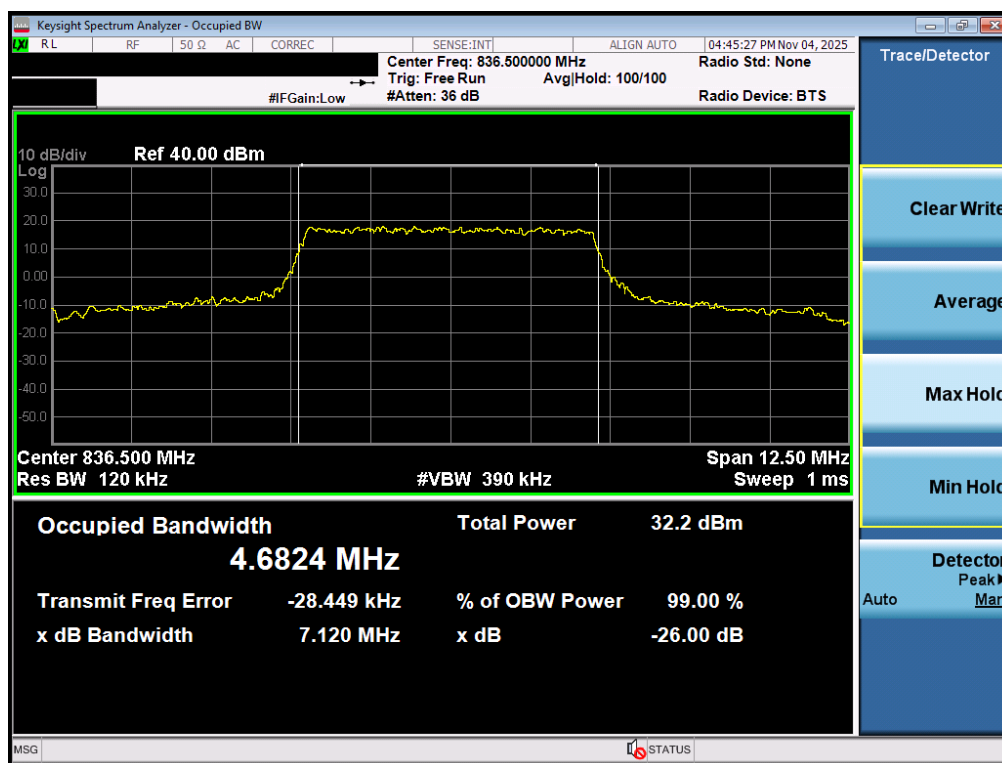
Plot 7-5. Occupied Bandwidth Plot (LTE Band 26/5 - 5MHz QPSK - Full RB - Ant1)
