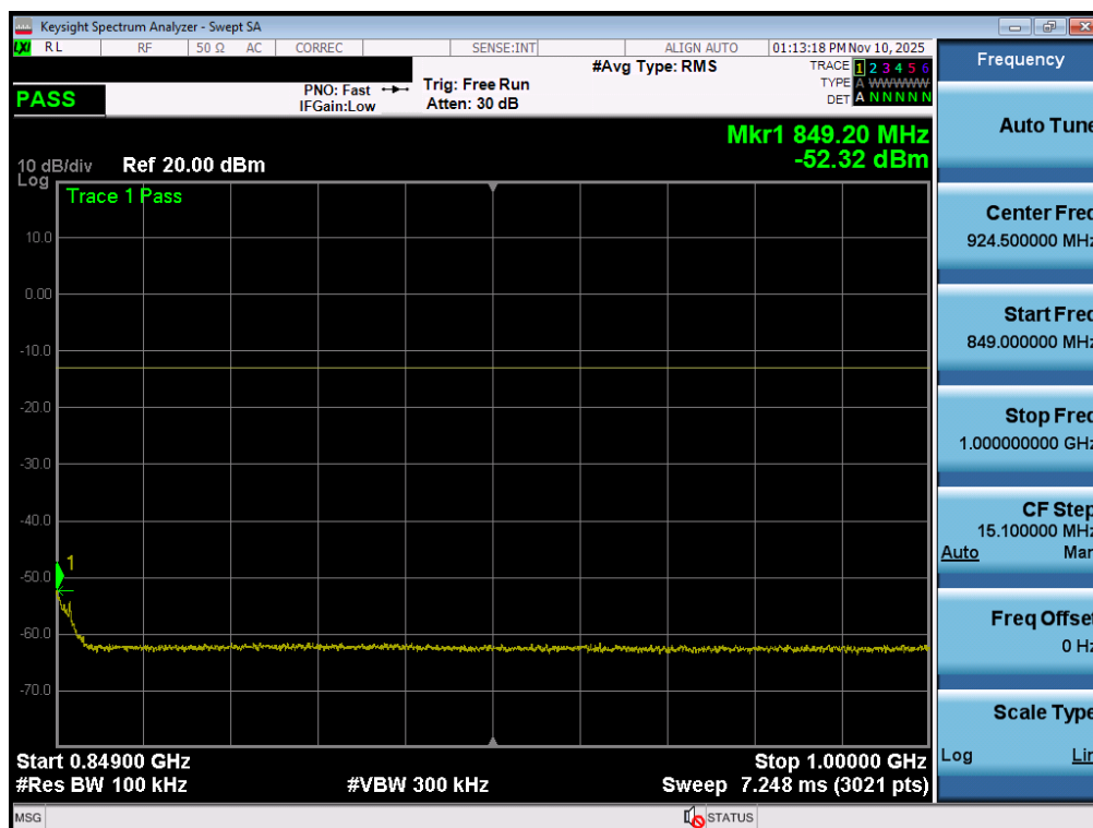
Plot 7-64. Conducted Spurious Plot (NR Band n5 - 20.0MHz - 1 RB - Mid Channel - Ant1)
