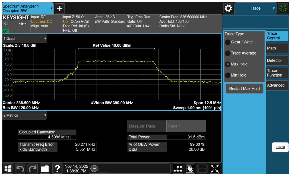
Plot 7-30. Occupied Bandwidth Plot (LTE Band 26/5 - 5MHz QPSK - Full RB - Ant2)
