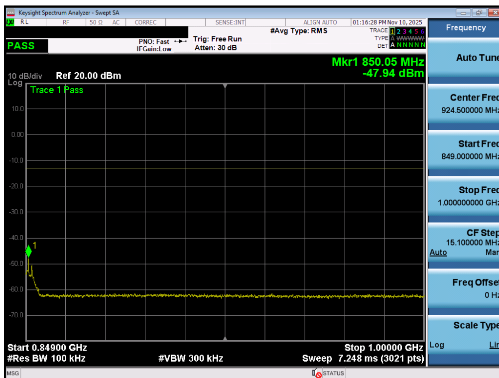
Plot 7-67. Conducted Spurious Plot (NR Band n5 - 20.0MHz - 1 RB - High Channel - Ant1)
