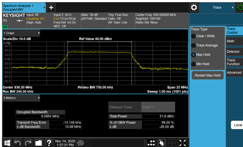
Plot 7-28. Occupied Bandwidth Plot (LTE Band 26/5 - 10MHz QPSK - Full RB - Ant2)
