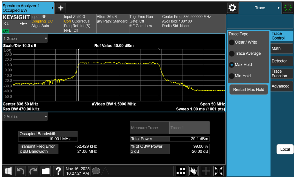
Plot 7-38. Occupied Bandwidth Plot (NR Band n5 - 20MHz 16-QAM - Full RB - Ant2)
