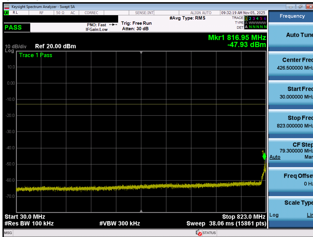
Plot 7-51. Conducted Spurious Plot (LTE Band 26 - 15MHz QPSK – 1 RB - Low Channel – Ant1)
