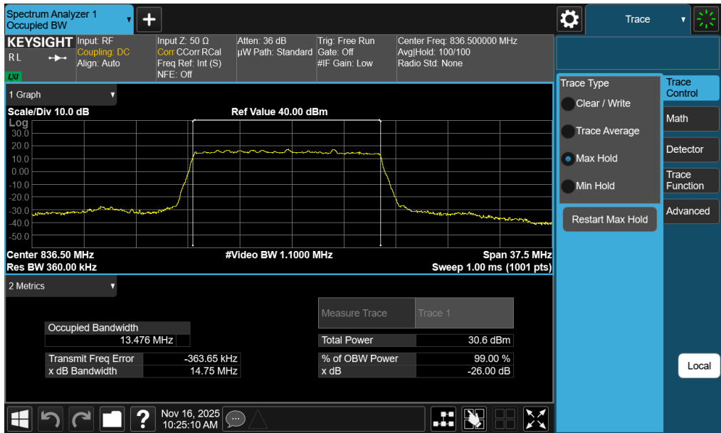
Plot 7-39. Occupied Bandwidth Plot (NR Band n5 - 15MHz \pi/2 BPSK - Full RB - Ant2)
