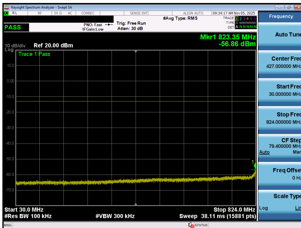
Plot 7-57. Conducted Spurious Plot (LTE Band 26 - 15MHz QPSK - 1 RB - High Channel – Ant1)
