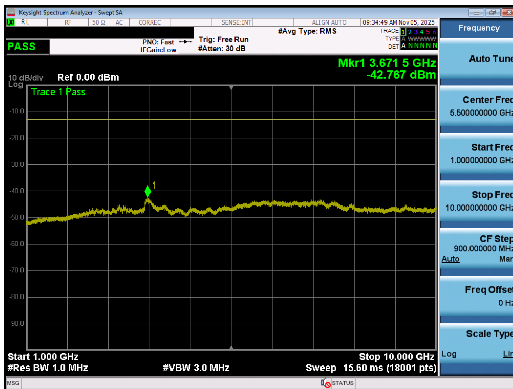
Plot 7-59. Conducted Spurious Plot (LTE Band 26 - 15MHz QPSK - 1 RB - High Channel – Ant1)
