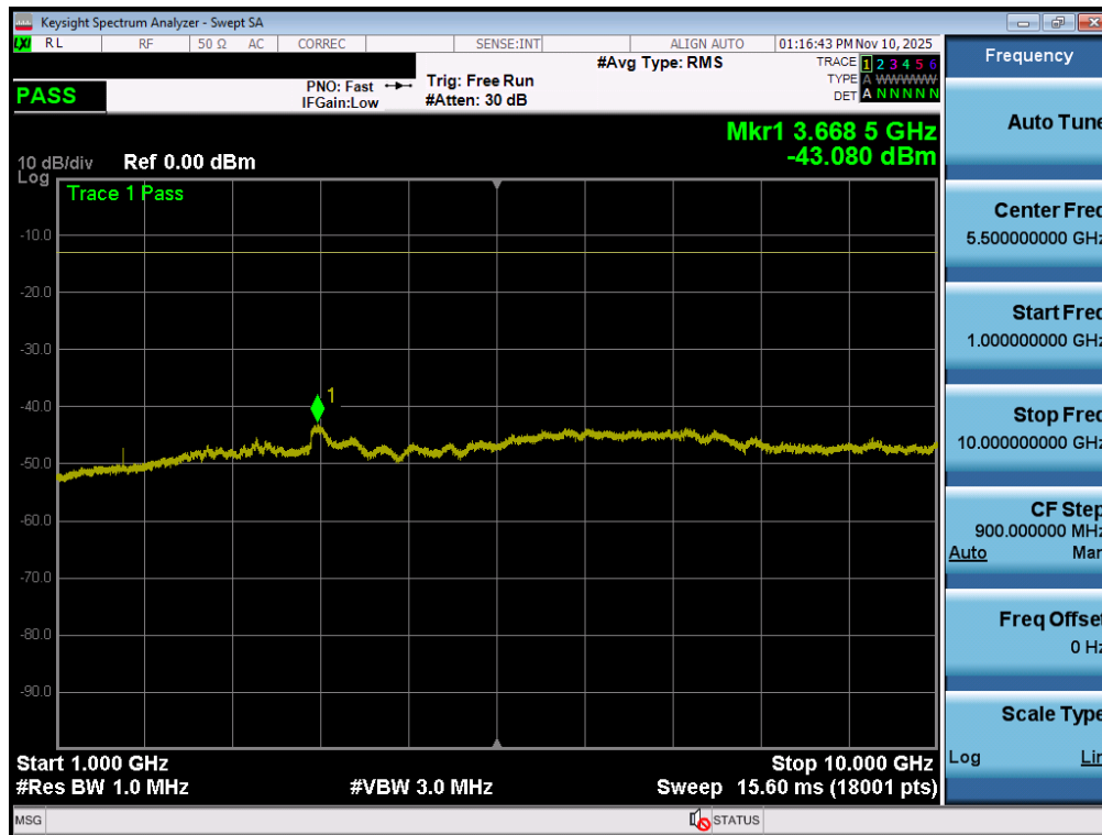
Plot 7-68. Conducted Spurious Plot (NR Band n5 - 20.0MHz - 1 RB - High Channel - Ant1)
