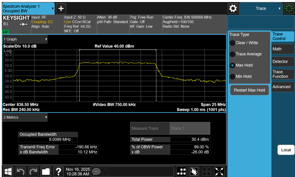
Plot 7-42. Occupied Bandwidth Plot (NR Band n5 - 10MHz \pi/2 BPSK - Full RB - Ant2)
