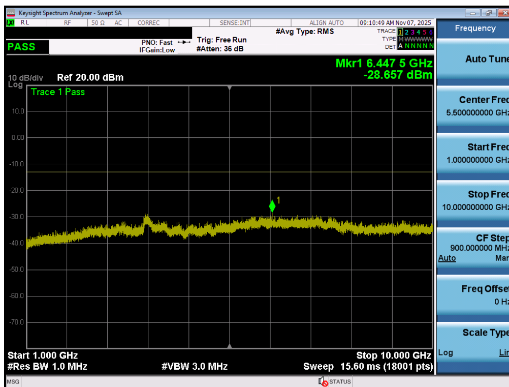
Plot 7-71. Conducted Spurious Plot (GPRS Ch. 128 – Ant1)
