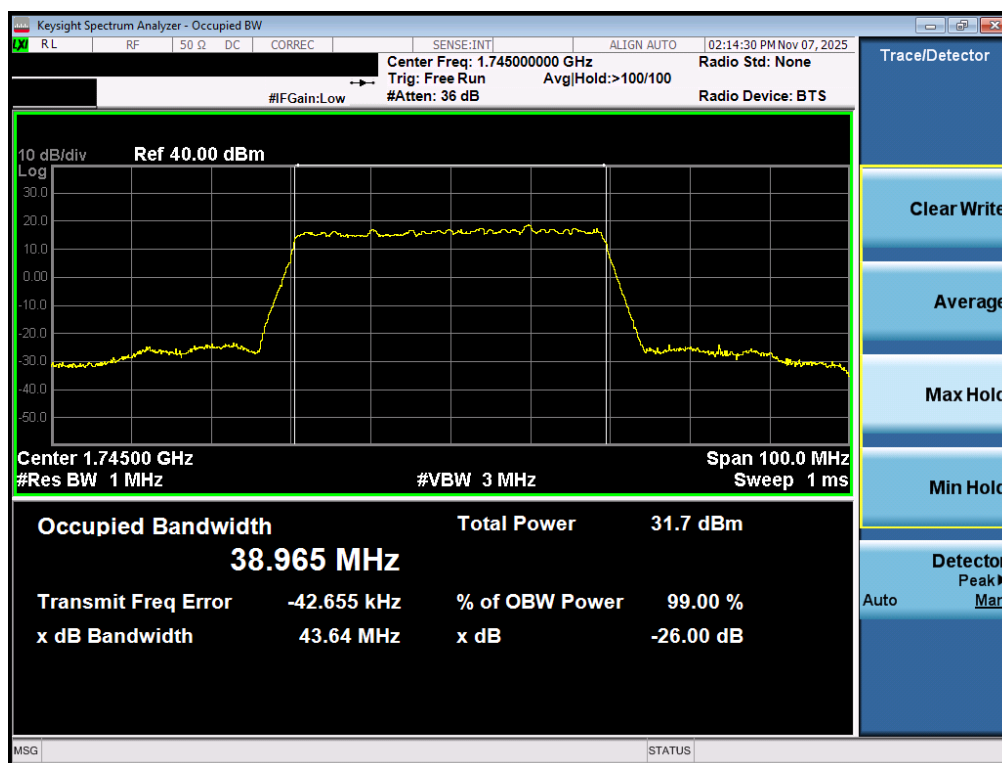
Plot 7-71. Occupied Bandwidth Plot (NR Band n66 - 40.0MHz DFT-s-OFDM BPSK - Full RB – ANT2)
