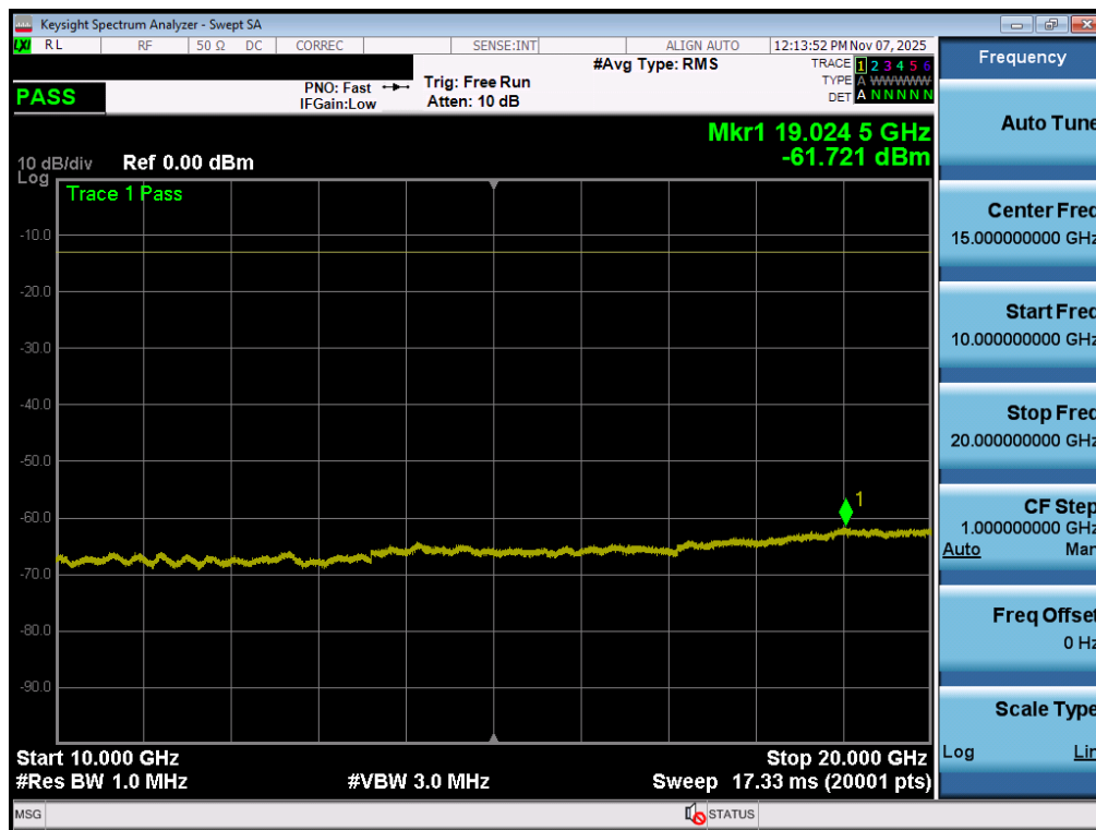
Plot 7-106. Conducted Spurious Plot (NR Band n66 - 40.0MHz - 1 RB - High Channel - ANT1)
