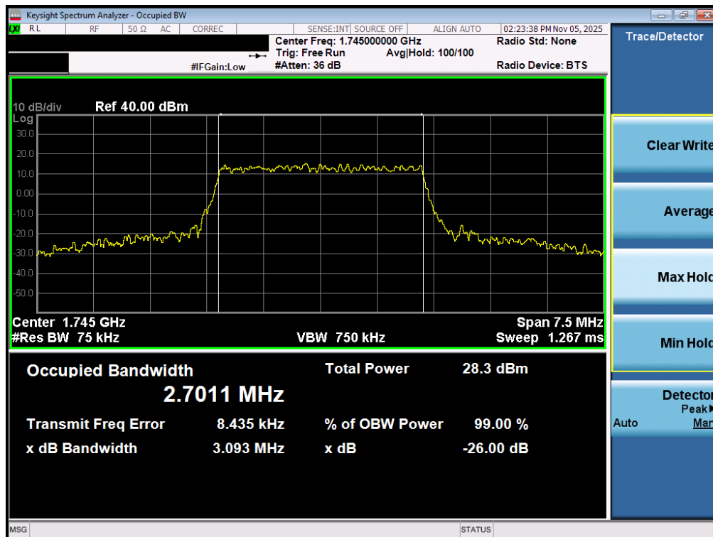
Plot 7-68. Occupied Bandwidth Plot (LTE Band 66/4 - 3MHz 16-QAM - Full RB - ANT2)
