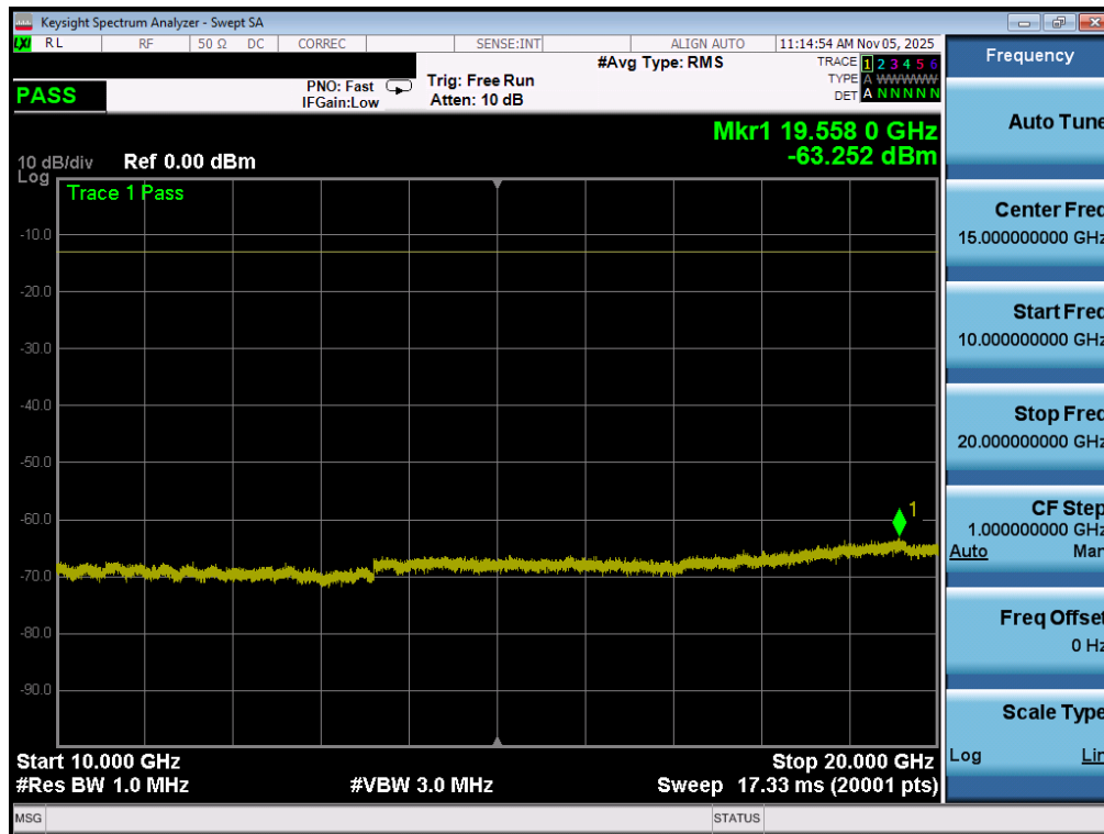
Plot 7-94. Conducted Spurious Plot (WCDMA-AWS - 5MHz QPSK - 1 RB - Low Channel)
