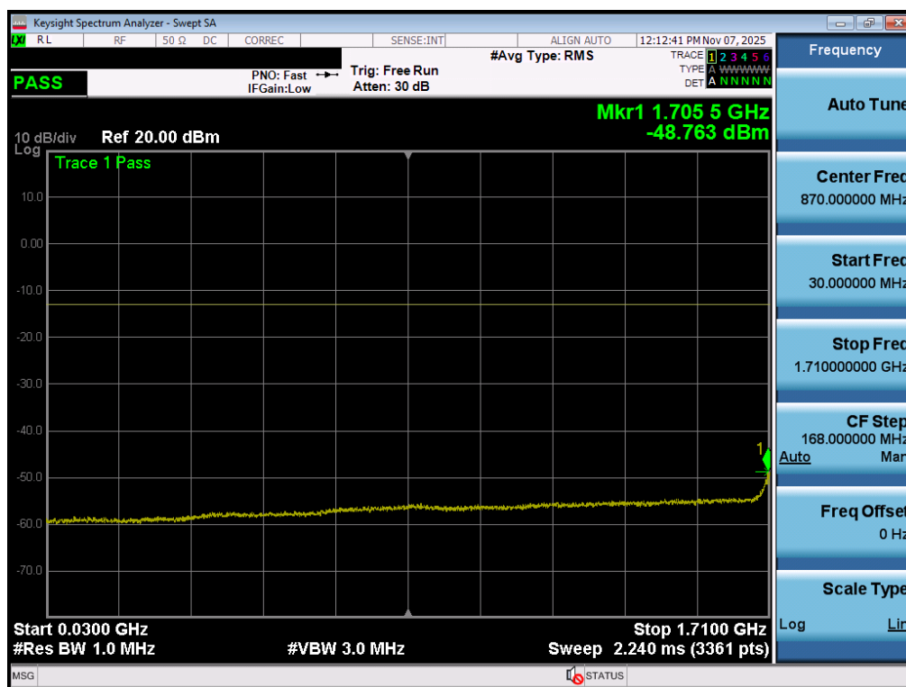
Plot 7-104. Conducted Spurious Plot (NR Band n66 - 40.0MHz - 1 RB - High Channel - ANT1)
