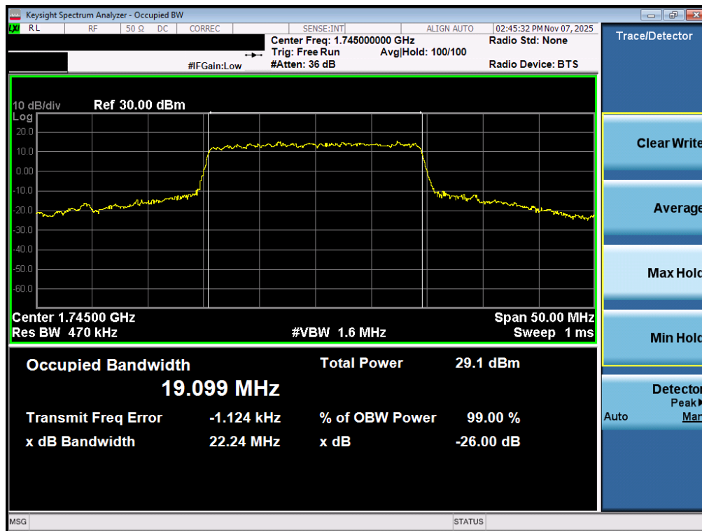
Plot 7-82. Occupied Bandwidth Plot (NR Band n66 - 20.0MHz CP-OFDM 16QAM - Full RB – ANT2)
