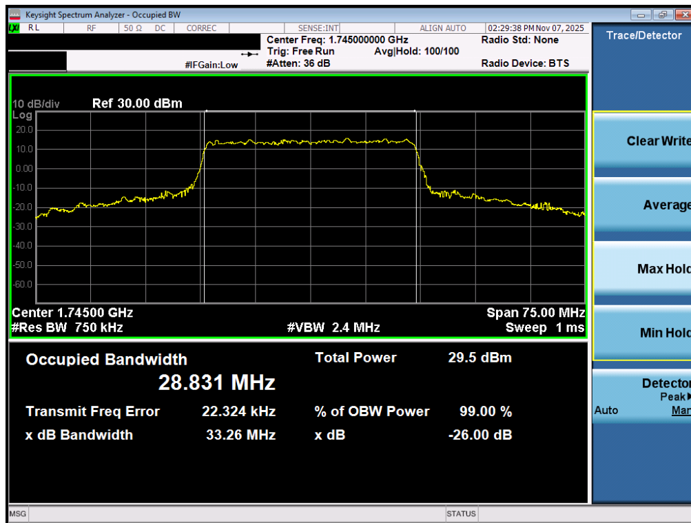
Plot 7-76. Occupied Bandwidth Plot (NR Band n66 - 30.0MHz CP-OFDM 16QAM - Full RB – ANT2)
