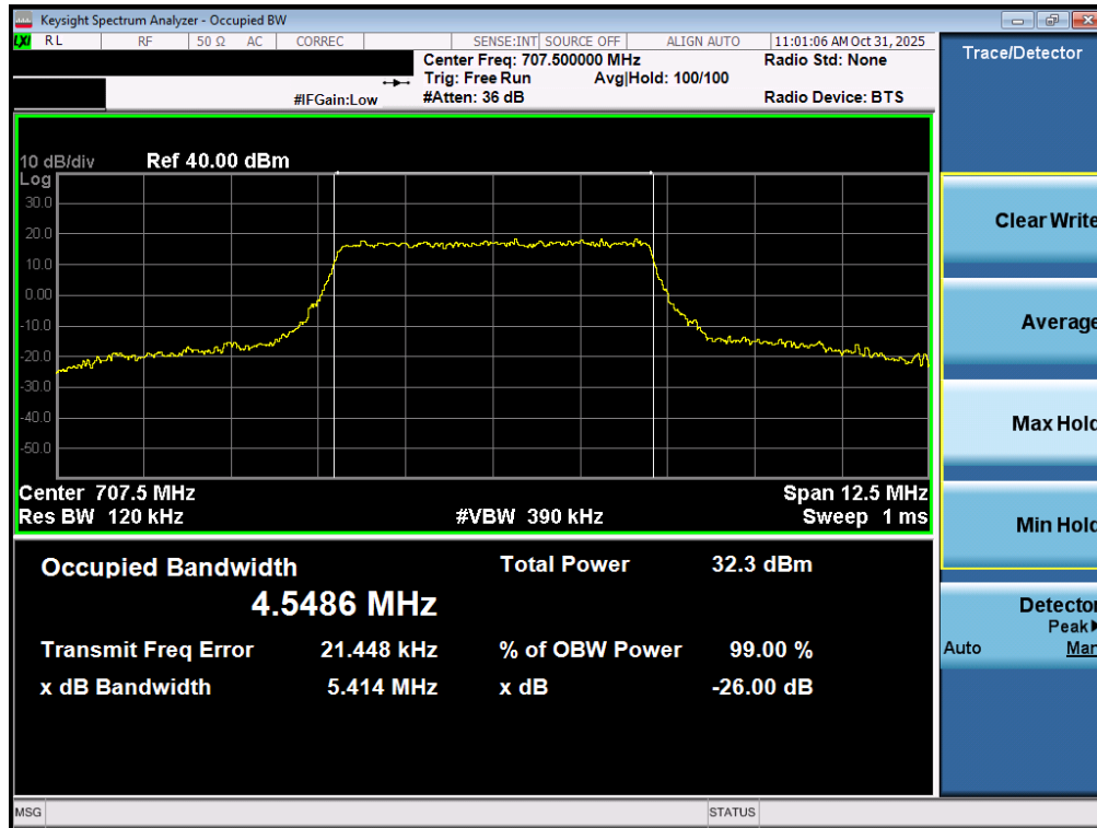
Plot 7-49. Occupied Bandwidth Plot (LTE Band 12/17 - 5MHz QPSK - Full RB – ANT2)
