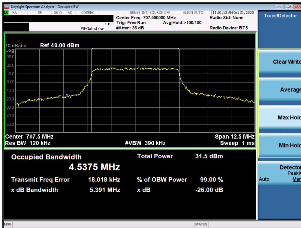
Plot 7-50. Occupied Bandwidth Plot (LTE Band 12/17 - 5MHz 16-QAM - Full RB – ANT2)
