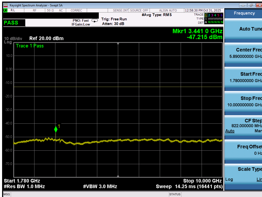
Plot 7-102. Conducted Spurious Plot (LTE Band 66/4 - 20MHz QPSK - 1 RB - Low Channel - ANT1)
