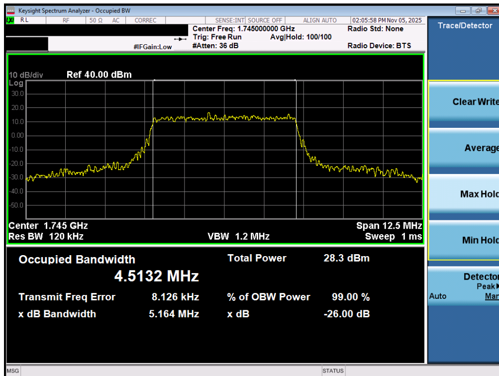
Plot 7-66. Occupied Bandwidth Plot (LTE Band 66/4 - 5MHz 16-QAM - Full RB - ANT2)
