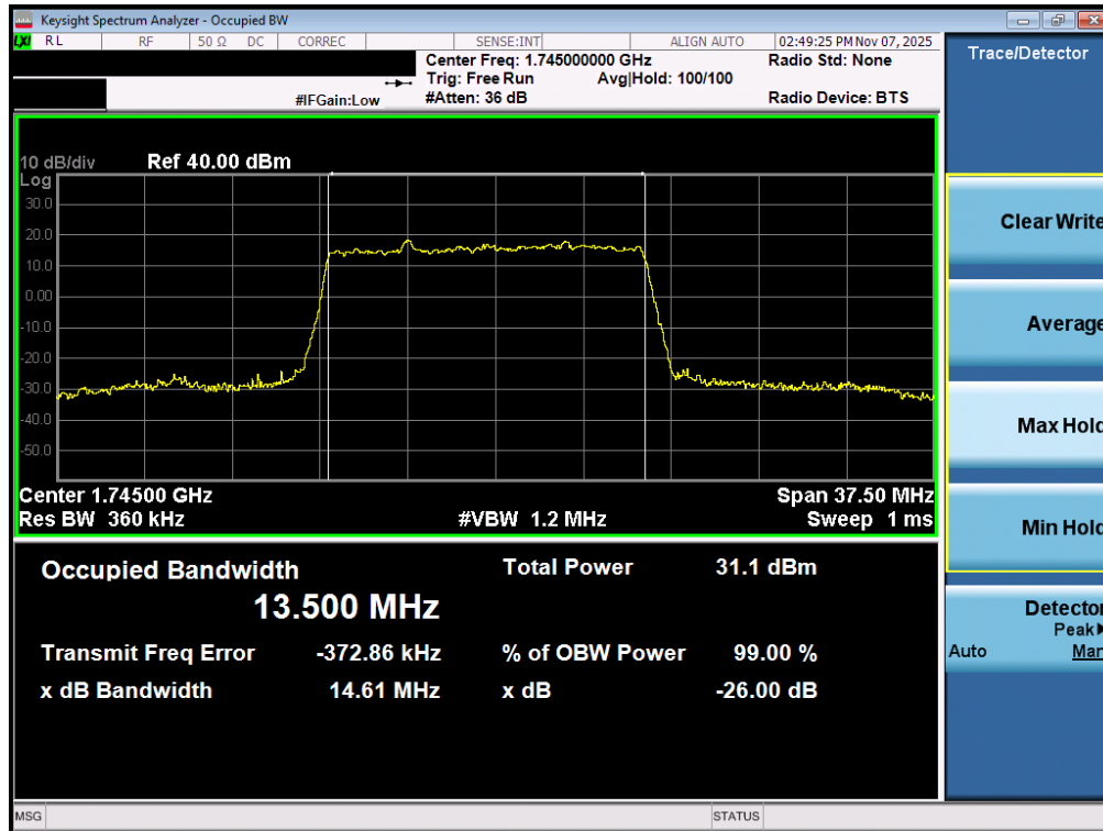
Plot 7-83. Occupied Bandwidth Plot (NR Band n66 - 15.0MHz DFT-s-OFDM BPSK - Full RB – ANT2)
