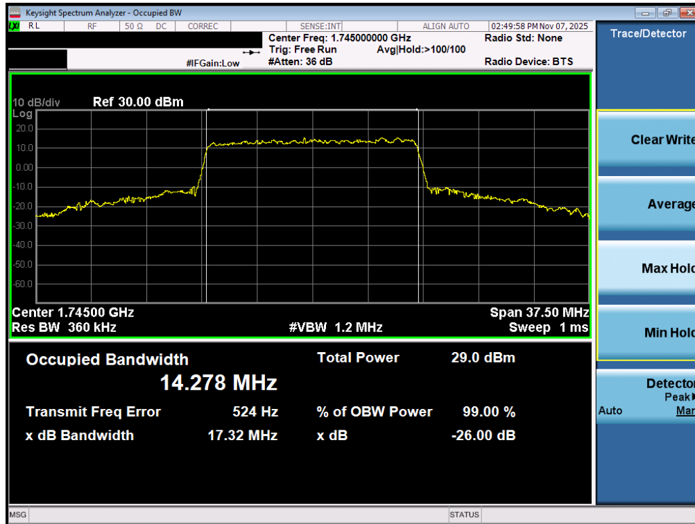
Plot 7-85. Occupied Bandwidth Plot (NR Band n66 - 15.0MHz CP-OFDM 16QAM - Full RB – ANT2)
