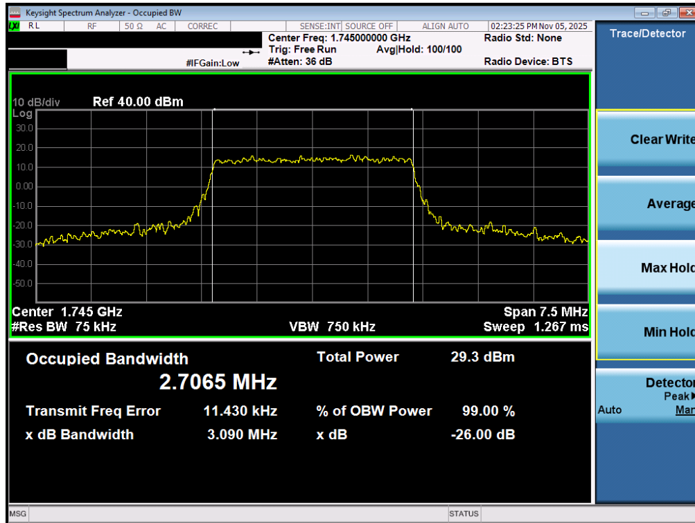
Plot 7-67. Occupied Bandwidth Plot (LTE Band 66/4 - 3MHz QPSK - Full RB - ANT2)
