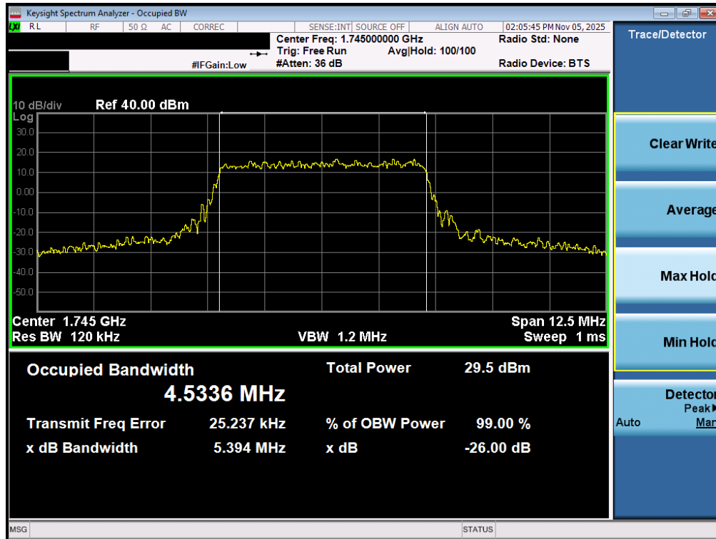
Plot 7-65. Occupied Bandwidth Plot (LTE Band 66/4 - 5MHz QPSK - Full RB - ANT2)
