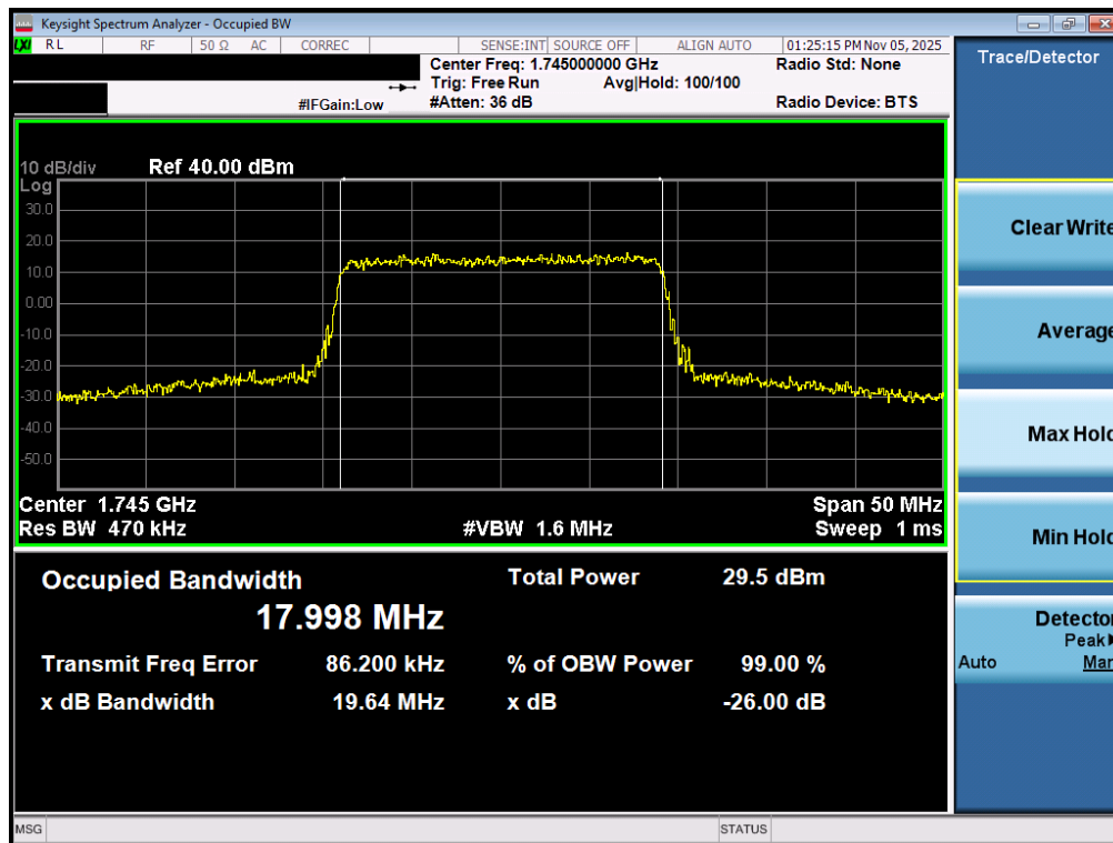
Plot 7-59. Occupied Bandwidth Plot (LTE Band 66/4 - 20MHz QPSK - Full RB - ANT2)
