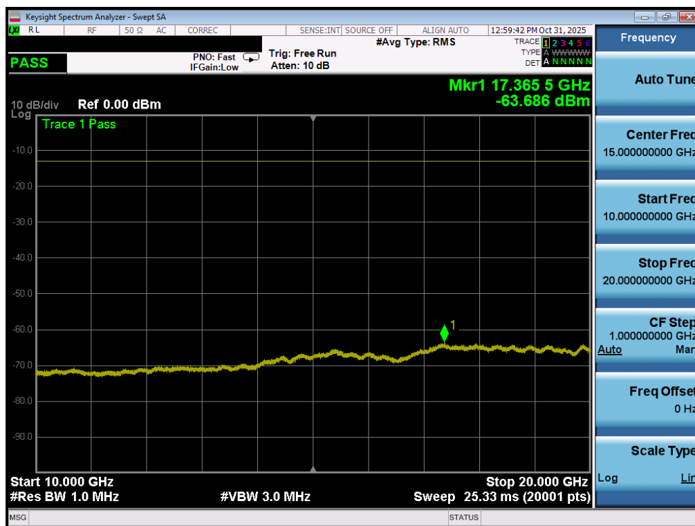
Plot 7-103. Conducted Spurious Plot (LTE Band 66/4 - 20MHz QPSK - 1 RB - Low Channel - ANT1)
