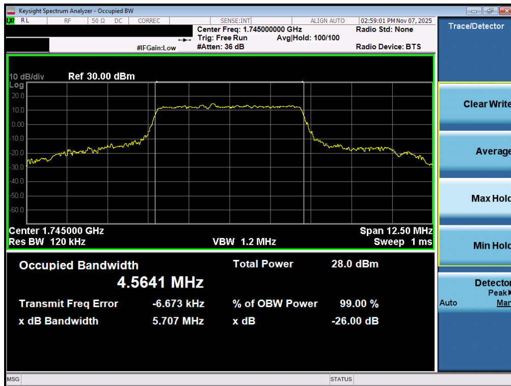
Plot 7-90. Occupied Bandwidth Plot (NR Band n66 - 5.0MHz CP-OFDM QPSK - Full RB – ANT2)
