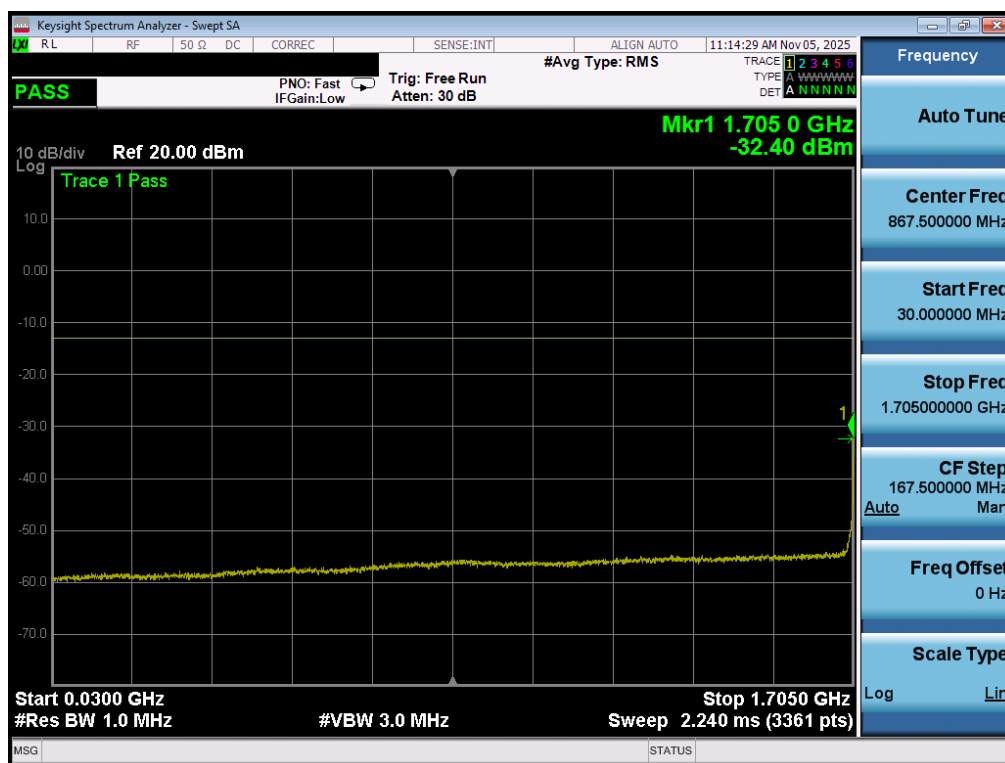
Plot 7-92. Conducted Spurious Plot (WCDMA-AWS - 5MHz QPSK - 1 RB – Low Channel)
