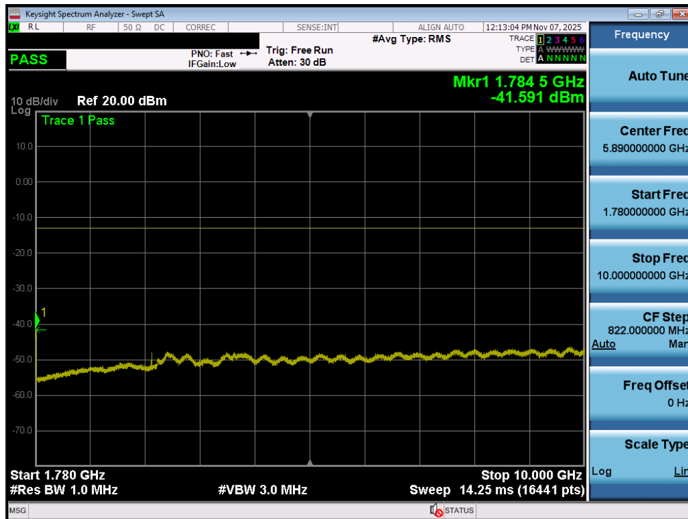
Plot 7-105. Conducted Spurious Plot (NR Band n66 - 40.0MHz - 1 RB - High Channel - ANT1)
