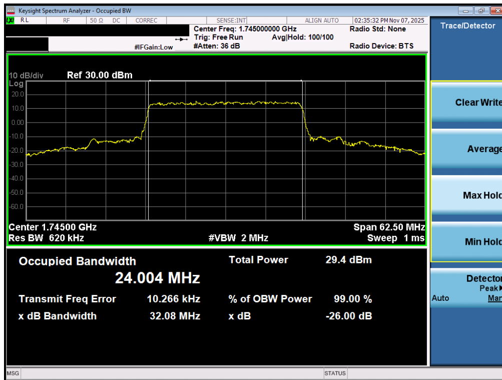
Plot 7-78. Occupied Bandwidth Plot (NR Band n66 - 25.0MHz CP-OFDM QPSK - Full RB – ANT2)
