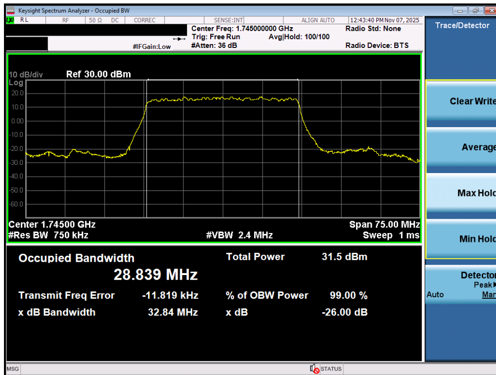
Plot 7-29. Occupied Bandwidth Plot (NR Band n66 - 30.0MHz DFT-s-OFDM BPSK - Full RB – ANT1)
