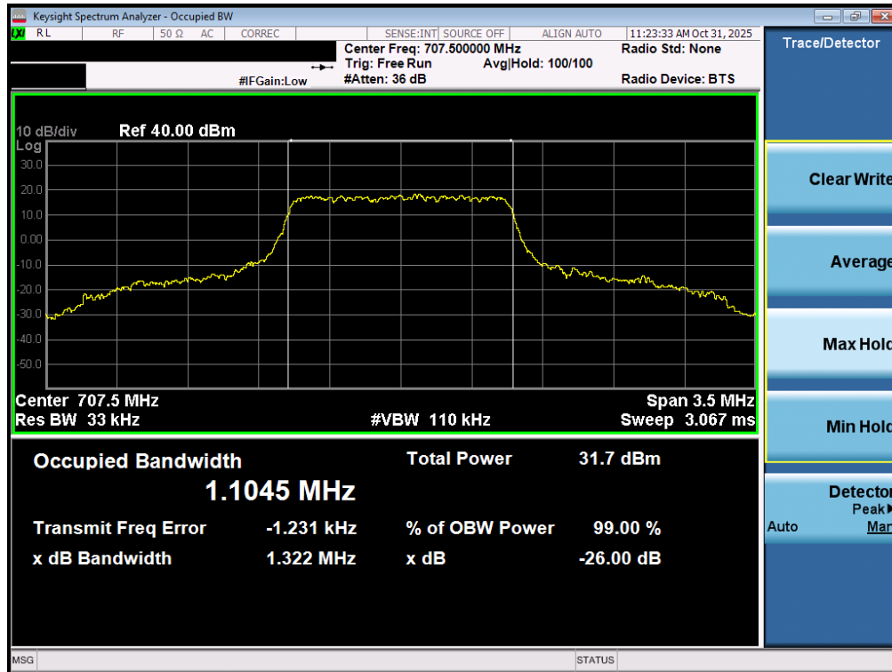
Plot 7-53. Occupied Bandwidth Plot (LTE Band 12/17 – 1.4MHz QPSK - Full RB – ANT2)
