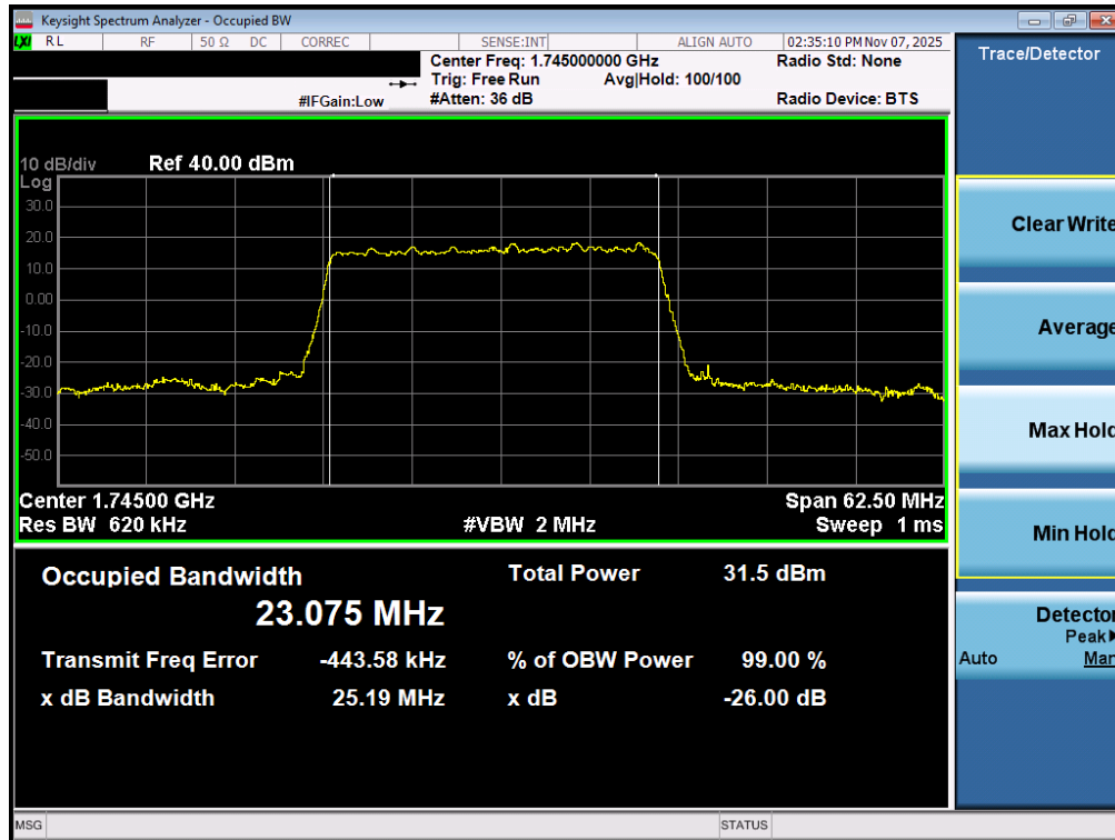
Plot 7-77. Occupied Bandwidth Plot (NR Band n66 - 25.0MHz DFT-s-OFDM BPSK - Full RB – ANT2)
