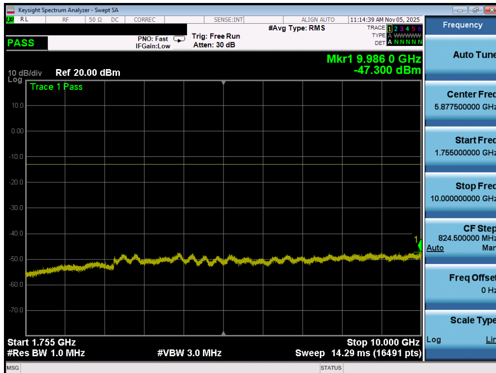
Plot 7-93. Conducted Spurious Plot (WCDMA-AWS - 5MHz QPSK - 1 RB – Low Channel)
