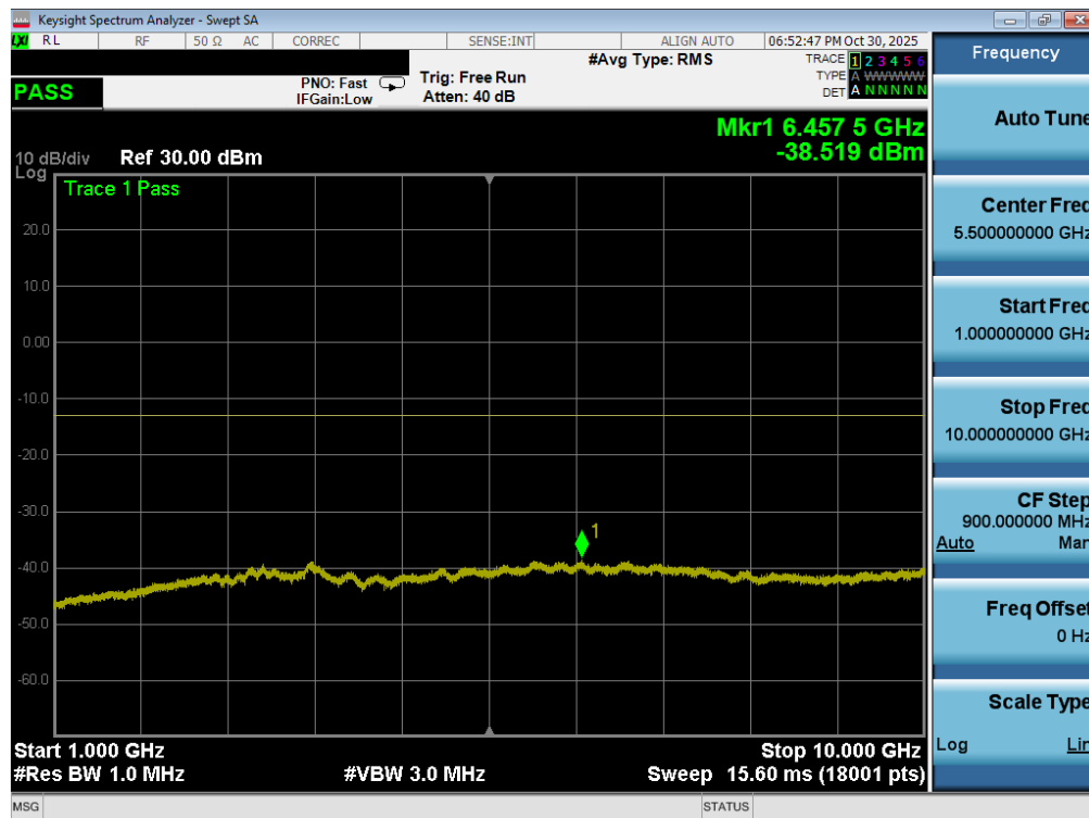
Plot 7-97. Conducted Spurious Plot (LTE Band 12/17 - 10MHz QPSK - 1 RB - Low Channel - ANT1)
