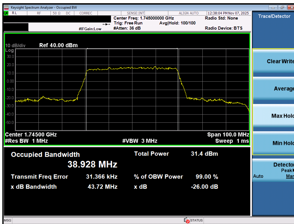
Plot 7-26. Occupied Bandwidth Plot (NR Band n66 - 40.0MHz DFT-s-OFDM BPSK - Full RB – ANT1)
