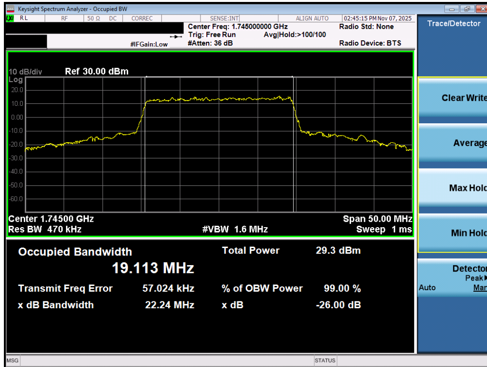
Plot 7-81. Occupied Bandwidth Plot (NR Band n66 - 20.0MHz CP-OFDM QPSK - Full RB – ANT2)
