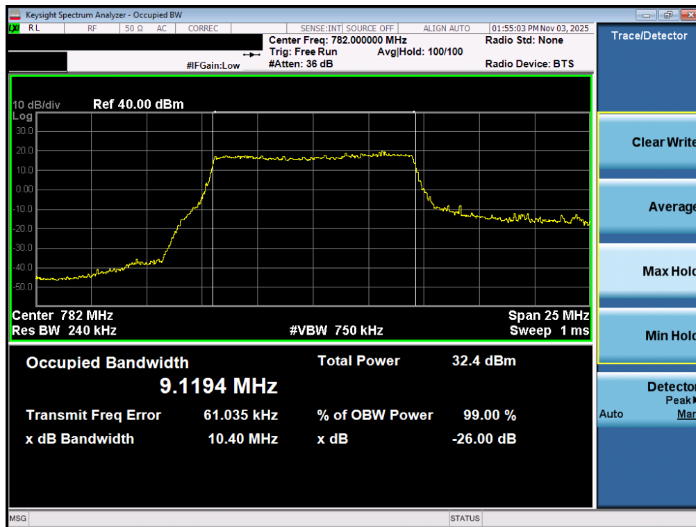
Plot 7-10. Occupied Bandwidth Plot (LTE Band 13 - 10MHz QPSK - Full RB – ANT1)
