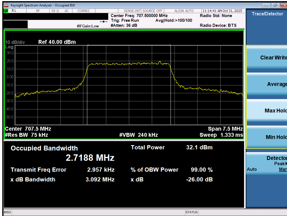
Plot 7-51. Occupied Bandwidth Plot (LTE Band 12/17 - 3MHz QPSK - Full RB – ANT2)
