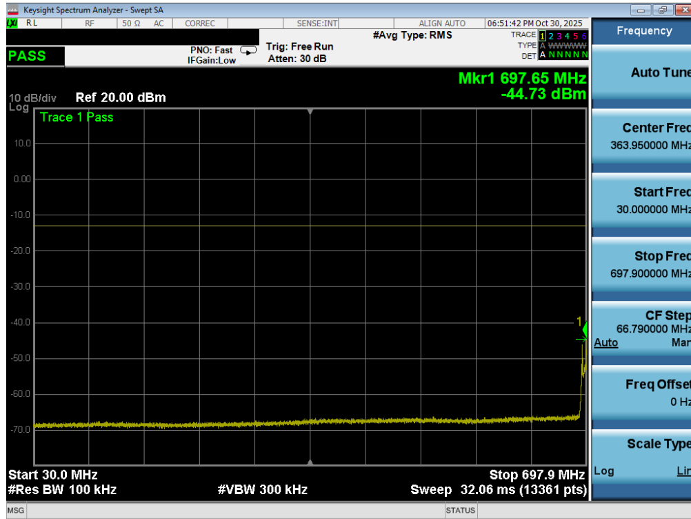
Plot 7-95. Conducted Spurious Plot (LTE Band 12/17 - 10MHz QPSK - 1 RB - Low Channel - ANT1)
