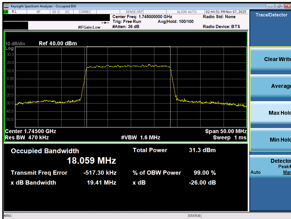
Plot 7-80. Occupied Bandwidth Plot (NR Band n66 - 20.0MHz DFT-s-OFDM BPSK - Full RB – ANT2)
