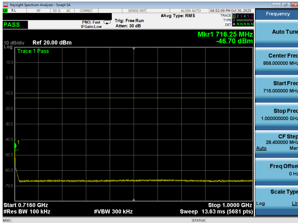
Plot 7-96. Conducted Spurious Plot (LTE Band 12/17 - 10MHz QPSK - 1 RB - Low Channel - ANT1)
