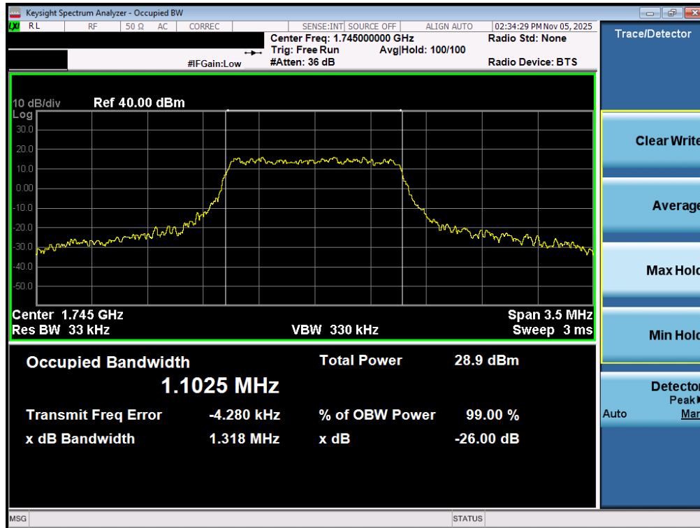
Plot 7-69. Occupied Bandwidth Plot (LTE Band 66/4 - 1.4MHz QPSK - Full RB - ANT2)
