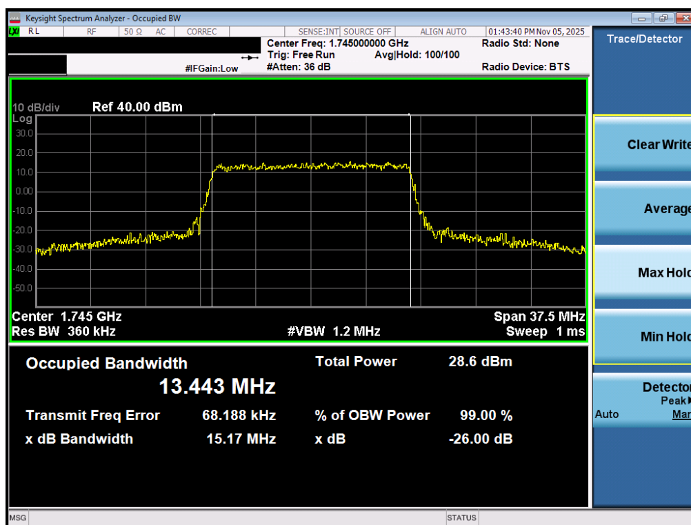
Plot 7-62. Occupied Bandwidth Plot (LTE Band 66/4 - 15MHz 16-QAM - Full RB - ANT2)
