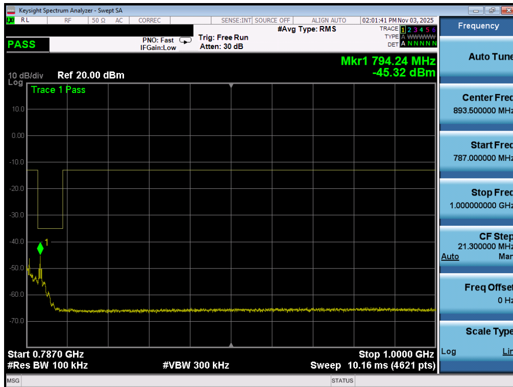
Plot 7-99. Conducted Spurious Plot (LTE Band 13 - 10MHz QPSK - 1 RB)
