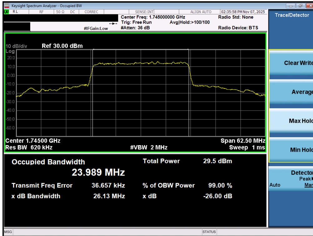
Plot 7-79. Occupied Bandwidth Plot (NR Band n66 - 25.0MHz CP-OFDM 16QAM - Full RB – ANT2)
