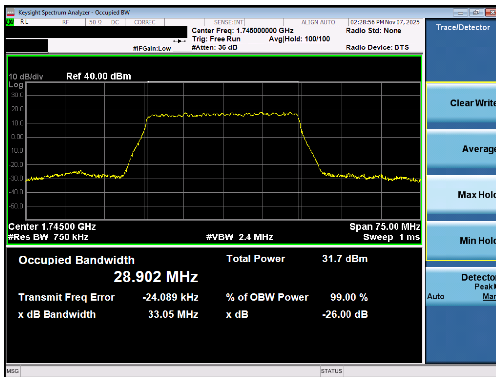
Plot 7-74. Occupied Bandwidth Plot (NR Band n66 - 30.0MHz DFT-s-OFDM BPSK - Full RB – ANT2)
