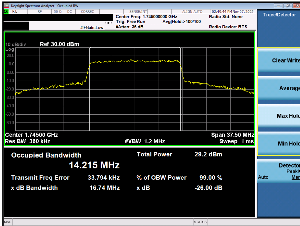
Plot 7-84. Occupied Bandwidth Plot (NR Band n66 - 15.0MHz CP-OFDM QPSK - Full RB – ANT2)
