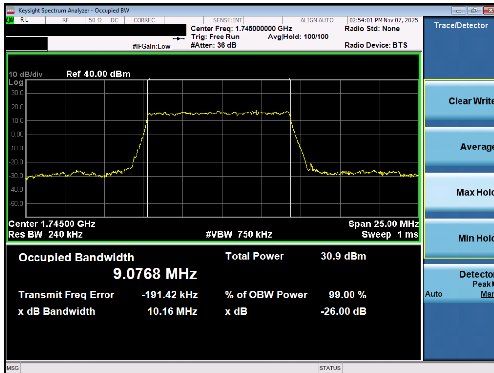
Plot 7-86. Occupied Bandwidth Plot (NR Band n66 - 10.0MHz DFT-s-OFDM BPSK - Full RB – ANT2)
