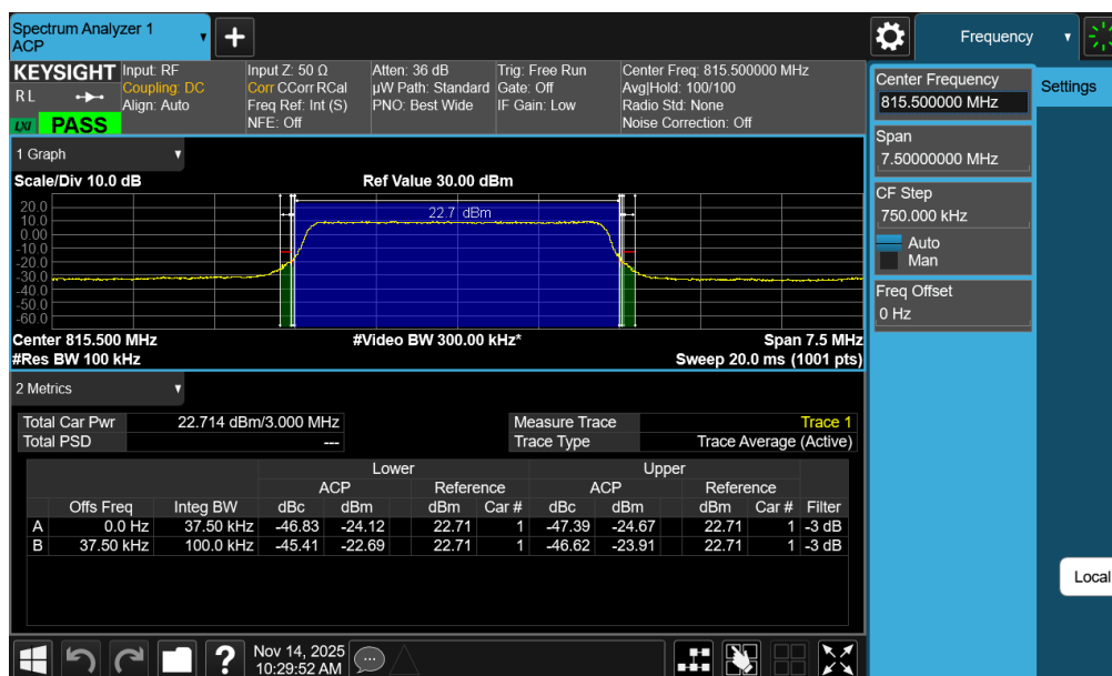
Plot 7-9. Channel - Edge Plot (LTE Band 26 - 3MHz QPSK - Low Channel)
