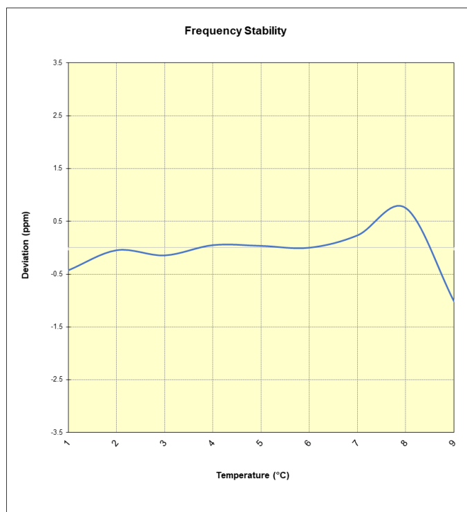
Plot 7-15. LTE Band 26 Frequency Stability Chart
