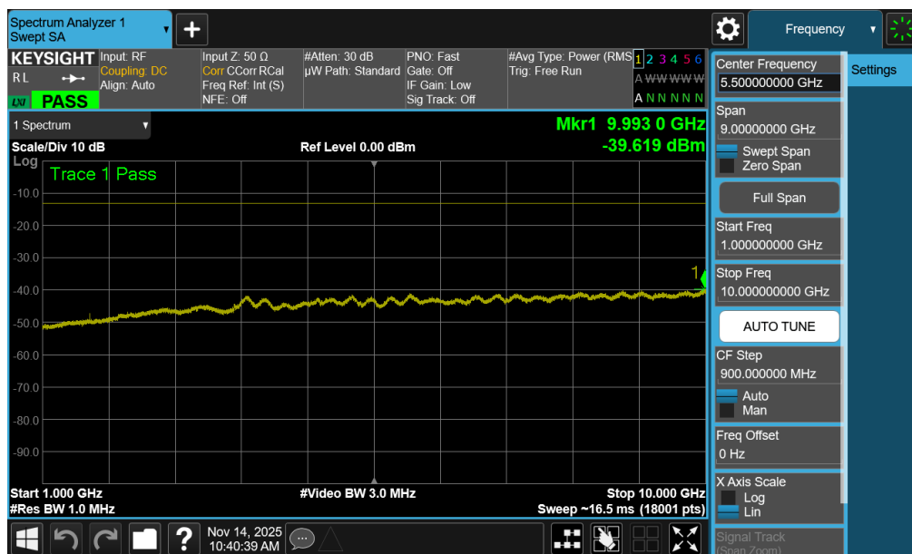
Plot 7-6. Conducted Spurious Plot (LTE Band 26 - 15MHz QPSK - RB Size 1, RB Offset 37)
