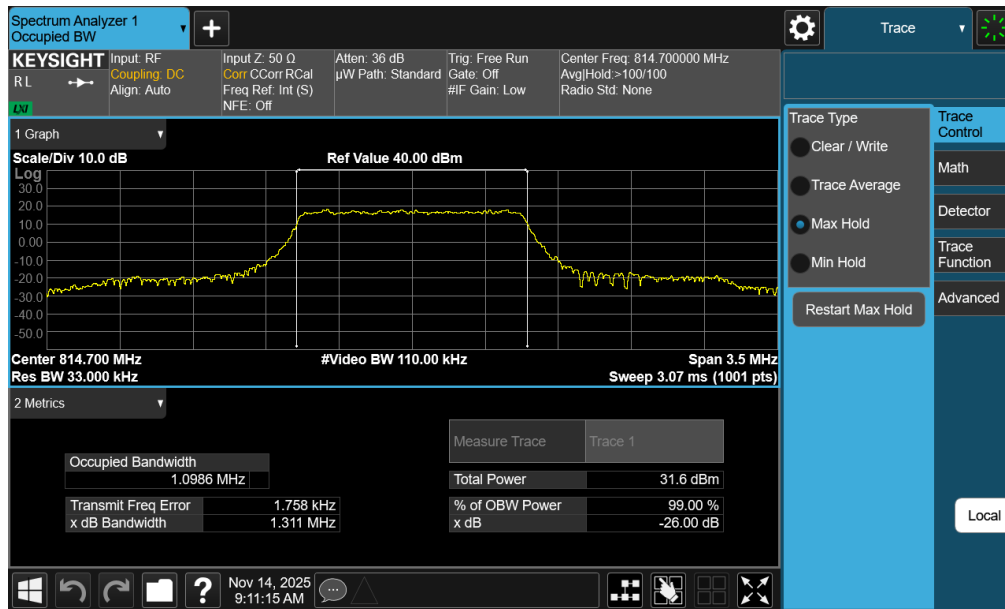
Plot 7-14. Occupied Bandwidth Plot (LTE Band 26 – 1.4MHz 16-QAM Low Channel - Full RB)
