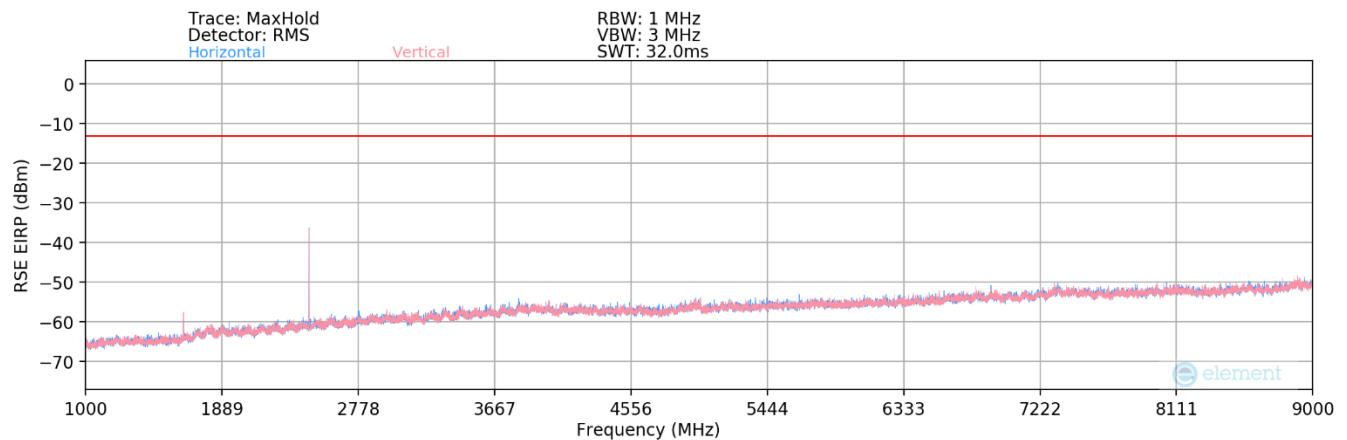
Plot 7-12. Radiated Spurious Plot Above 1GHz (LTE Band 26)
