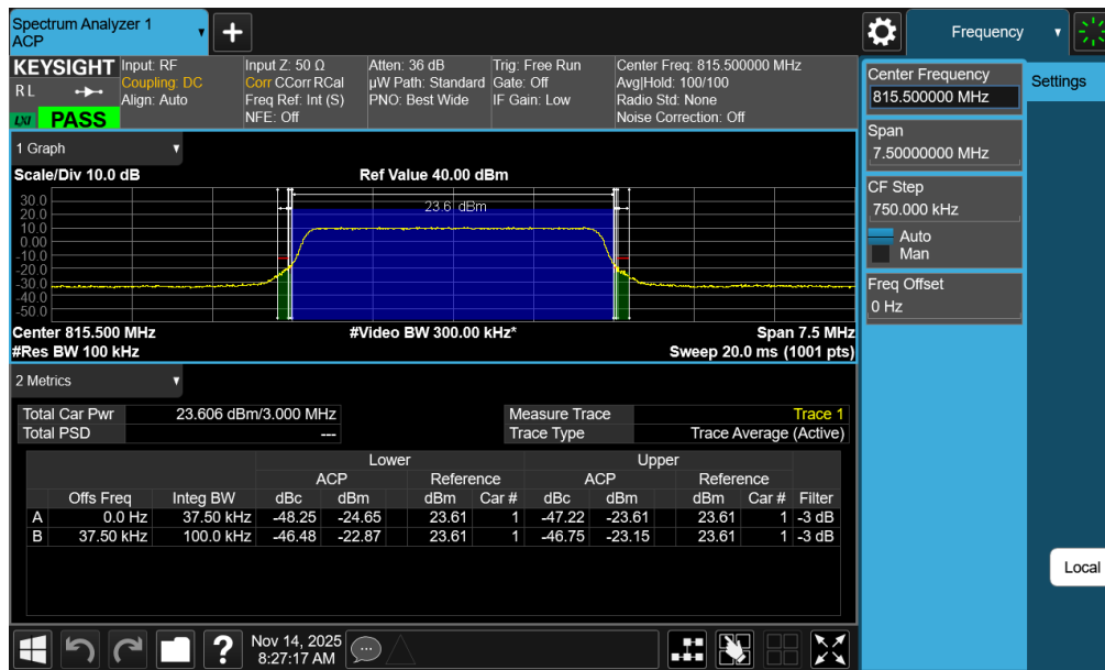
Plot 7-7. Channel - Edge Plot (LTE Band 26 - 3MHz QPSK - Low Channel)
