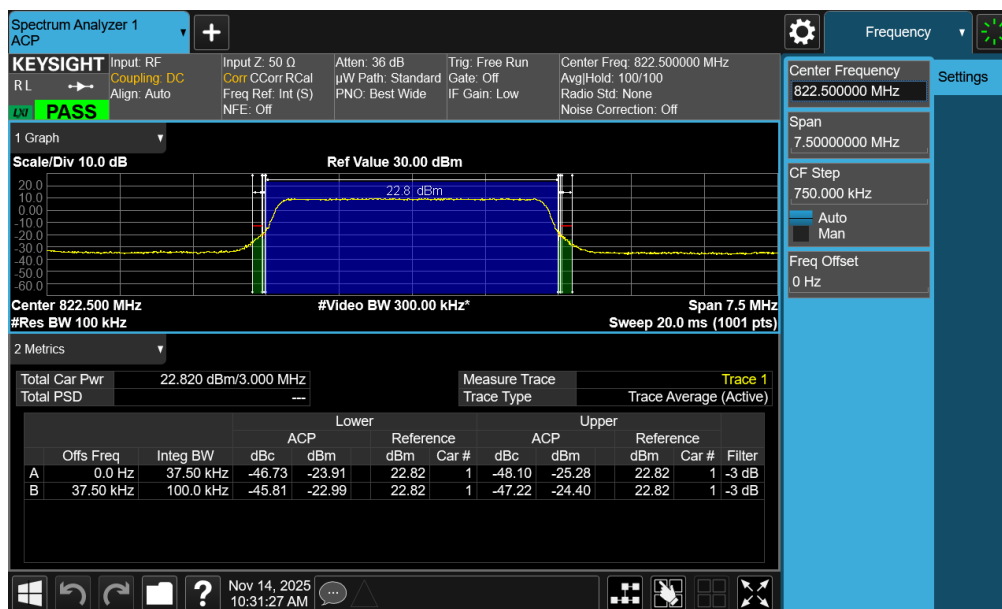
Plot 7-10. Channel - Edge Plot (LTE Band 26 - 3MHz QPSK - High Channel)
