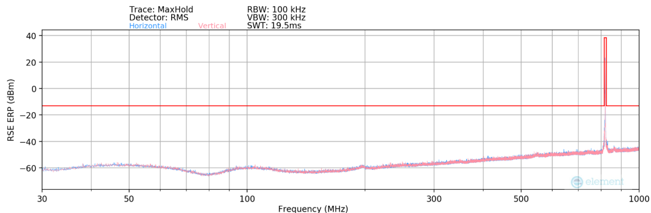
Plot 7-13. Radiated Spurious Plot Below 1GHz (LTE Band 26)
