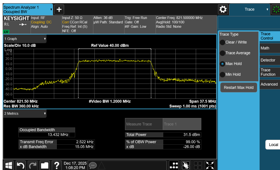
Plot 9-1. Occupied Bandwidth (Spot-check) – LTE B26
