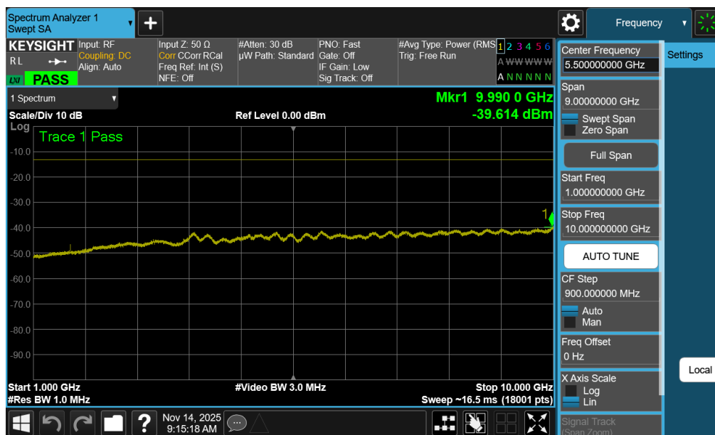
Plot 7-3. Conducted Spurious Plot (LTE Band 26 - 15MHz QPSK - RB Size 1, RB Offset 37)
