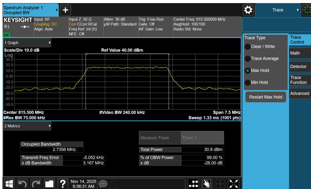
Plot 7-12. Occupied Bandwidth Plot (LTE Band 26 - 3MHz 16-QAM Low Channel - Full RB)
