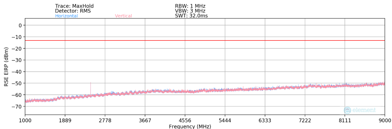
Plot 7-14. Radiated Spurious Plot Above 1GHz (LTE Band 26)
