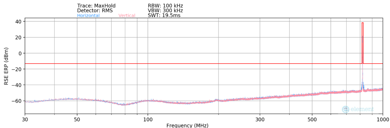
Plot 7-11. Radiated Spurious Plot Below 1GHz (LTE Band 26)
