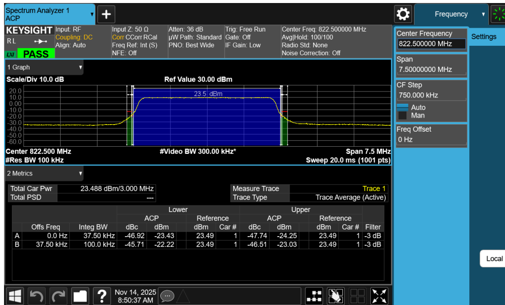
Plot 7-8. Channel - Edge Plot (LTE Band 26 - 3MHz QPSK - High Channel)
