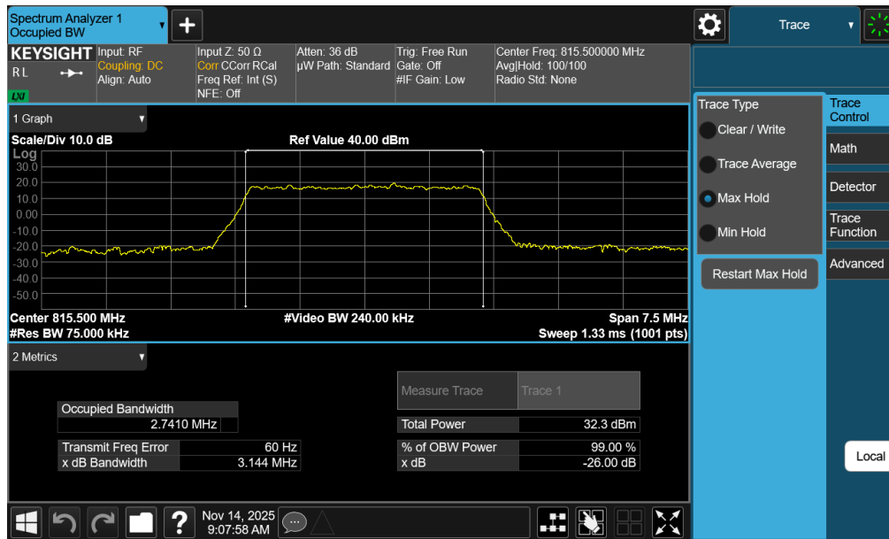
Plot 7-11. Occupied Bandwidth Plot (LTE Band 26 - 3MHz QPSK Low Channel - Full RB)
