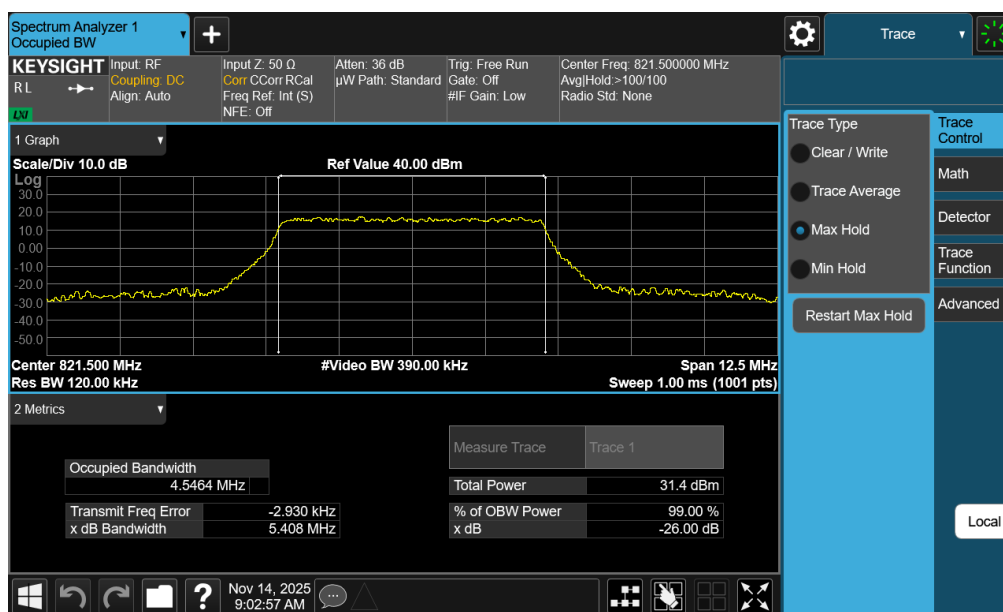
Plot 7-12. Occupied Bandwidth Plot (LTE Band 26 - 5MHz 16-QAM High Channel - Full RB)
