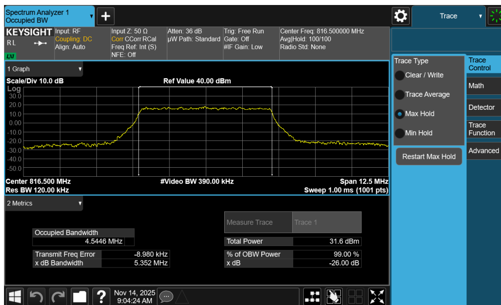
Plot 7-11. Occupied Bandwidth Plot (LTE Band 26 - 5MHz 16-QAM Low Channel - Full RB)
