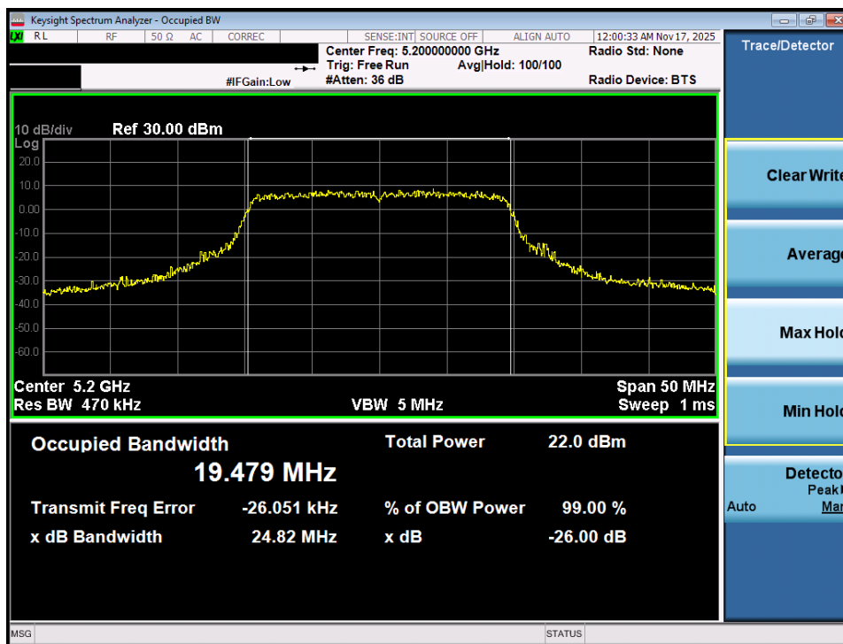
Plot 7-3. 26dB Bandwidth Plot MIMO ANT1 (20MHz BW 802.11ax (UNII Band 1) – Ch. 40)
