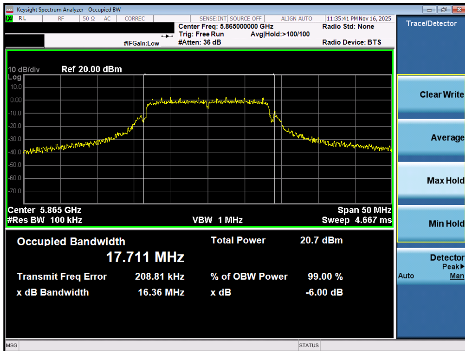
Plot 7-22. 6dB Bandwidth Plot MIMO ANT1 (802.11a (UNII Band 4) – Ch. 173)
