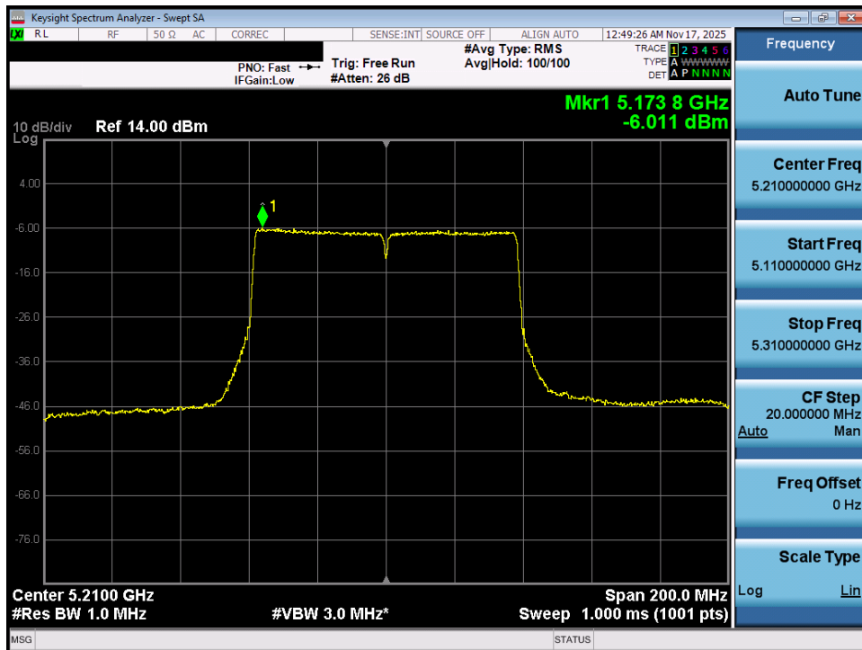
Plot 7-76. Power Spectral Density Plot MIMO ANT1 (80MHz BW 802.11ac (UNII Band 1) – Ch. 42)
