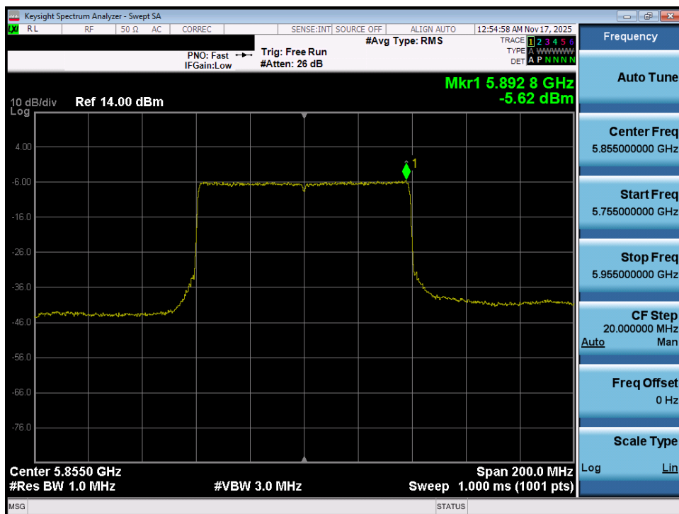
Plot 7-91. Power Spectral Density Plot MIMO ANT1 (80MHz BW 802.11ax (UNII Band 3/4) – Ch. 171)
