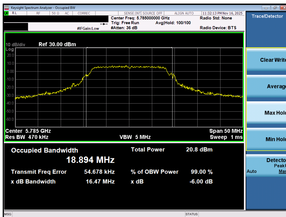
Plot 7-43. OBW Plot MIMO ANT1 (802.11a (UNII Band 3) – Ch. 157)
