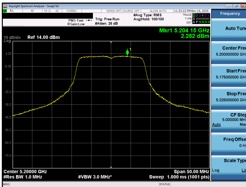
Plot 7-71. Power Spectral Density Plot MIMO ANT1 (802.11a (UNII Band 1) – Ch. 40)
