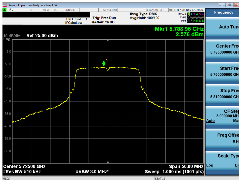
Plot 7-99. Power Spectral Density Plot MIMO ANT2 (802.11a (UNII Band 3) – Ch. 157)
