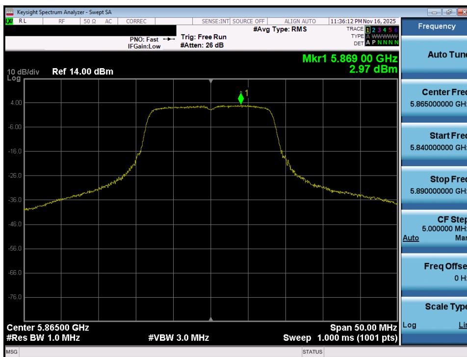
Plot 7-85. Power Spectral Density Plot MIMO ANT1 (802.11a (UNII Band 4) – Ch. 173)
