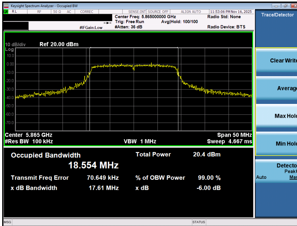
Plot 7-23. 6dB Bandwidth Plot MIMO ANT1 (20MHz BW 802.11n (UNII Band 4) – Ch. 173)
