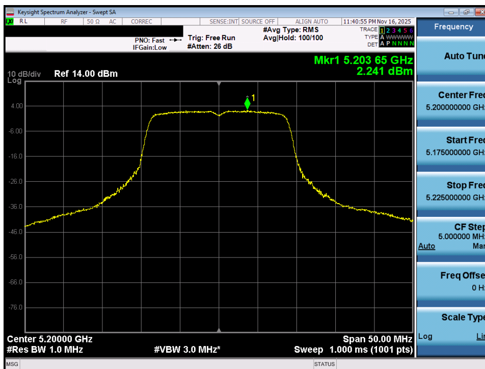
Plot 7-72. Power Spectral Density Plot MIMO ANT1 (20MHz BW 802.11n (UNII Band 1) – Ch. 40)
