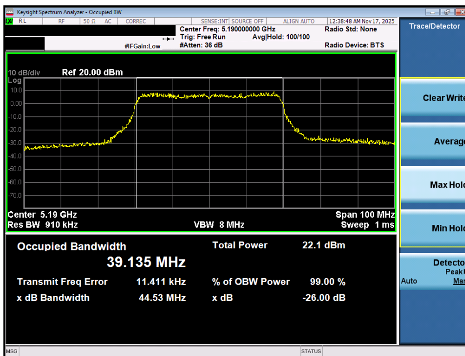
Plot 7-5. 26dB Bandwidth Plot MIMO ANT1 (40MHz BW 802.11ax (UNII Band 1) – Ch. 38)
