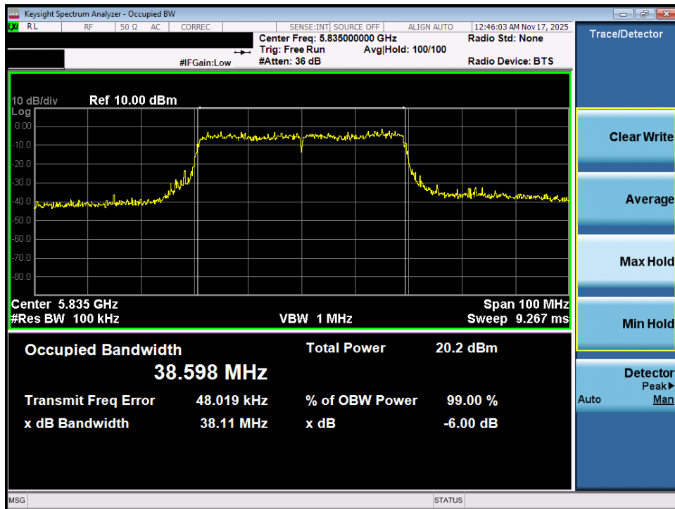
Plot 7-26. 6dB Bandwidth Plot MIMO ANT1 (40MHz BW 802.11ax (UNII Band 3/4) – Ch. 167)
