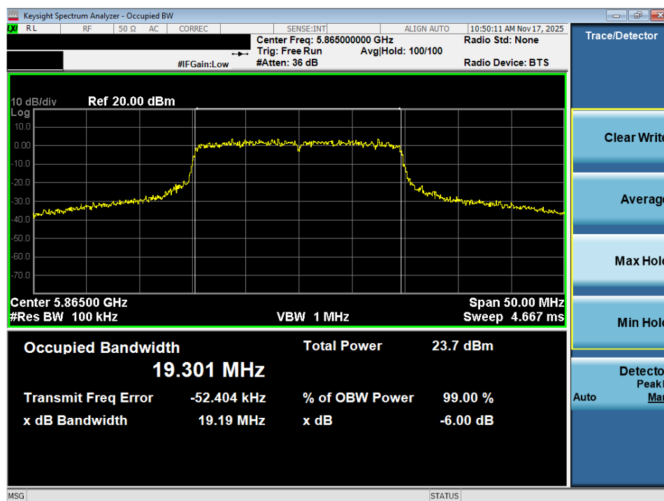
Plot 7-34. 6dB Bandwidth Plot MIMO ANT2 (20MHz BW 802.11ax – 242 Tones (UNII Band 4) – Ch. 173)
