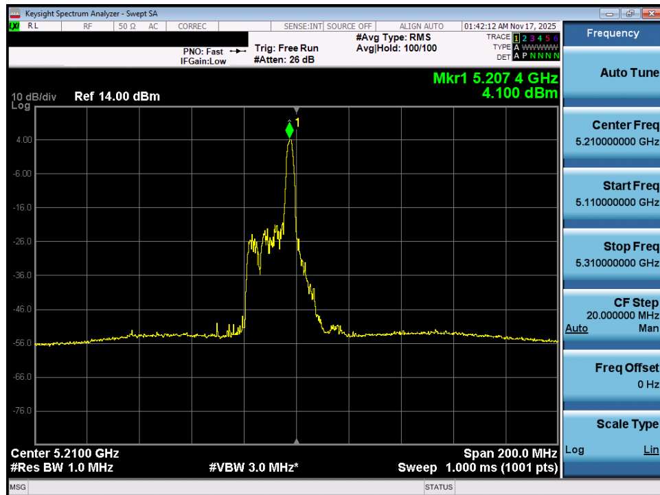
Plot 7-63. Power Spectral Density Plot MIMO ANT1 (80MHz BW 802.11ax – 26 Tones (UNII Band 1) – Ch. 42)
