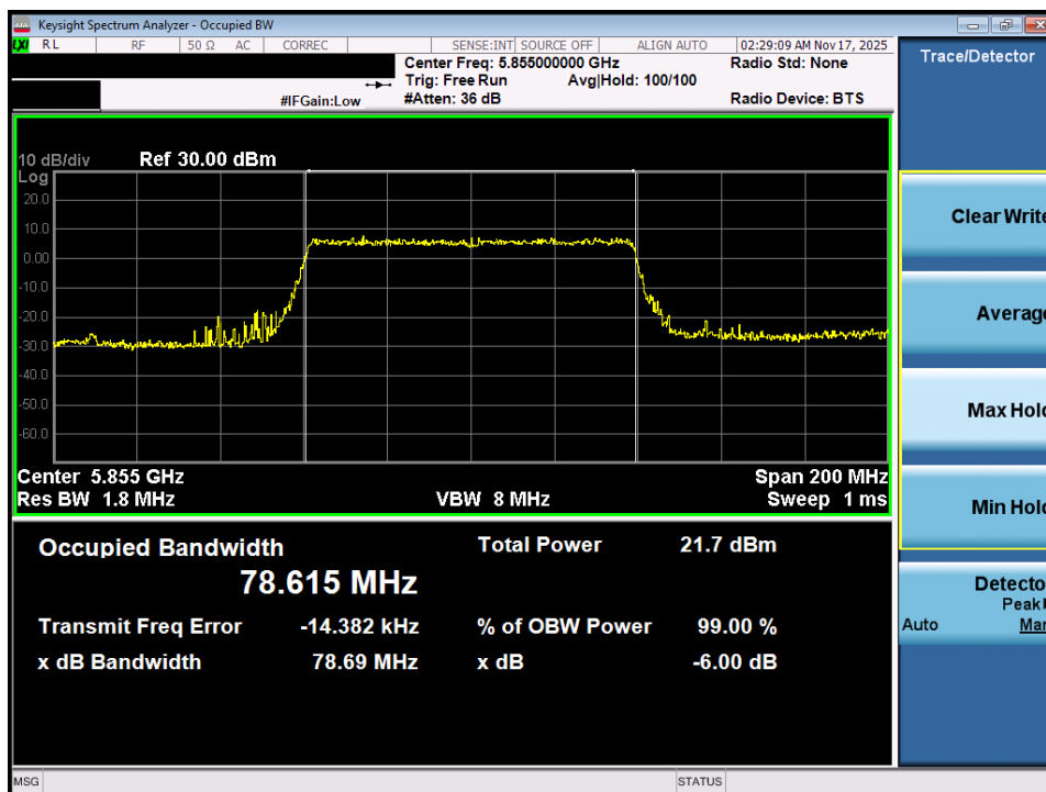
Plot 7-48. OBW Plot MIMO ANT1 (80MHz BW 802.11ax – 996 Tones (UNII Band 3/4) – Ch. 171)
