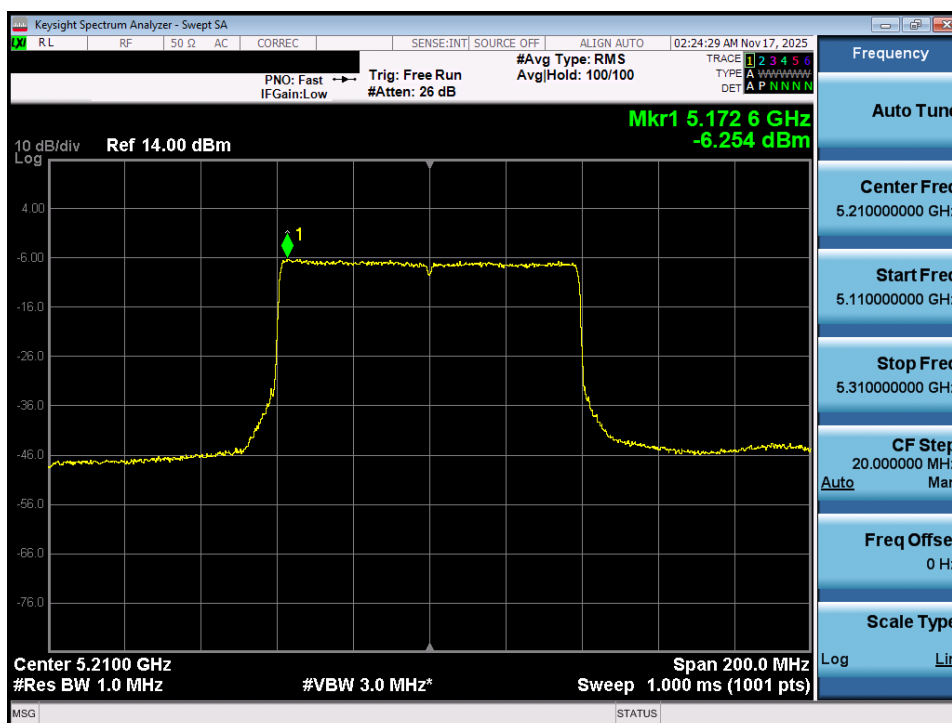
Plot 7-72. Power Spectral Density Plot MIMO ANT1 (80MHz BW 802.11ax – 996 Tones (UNII Band 1) – Ch. 42)
