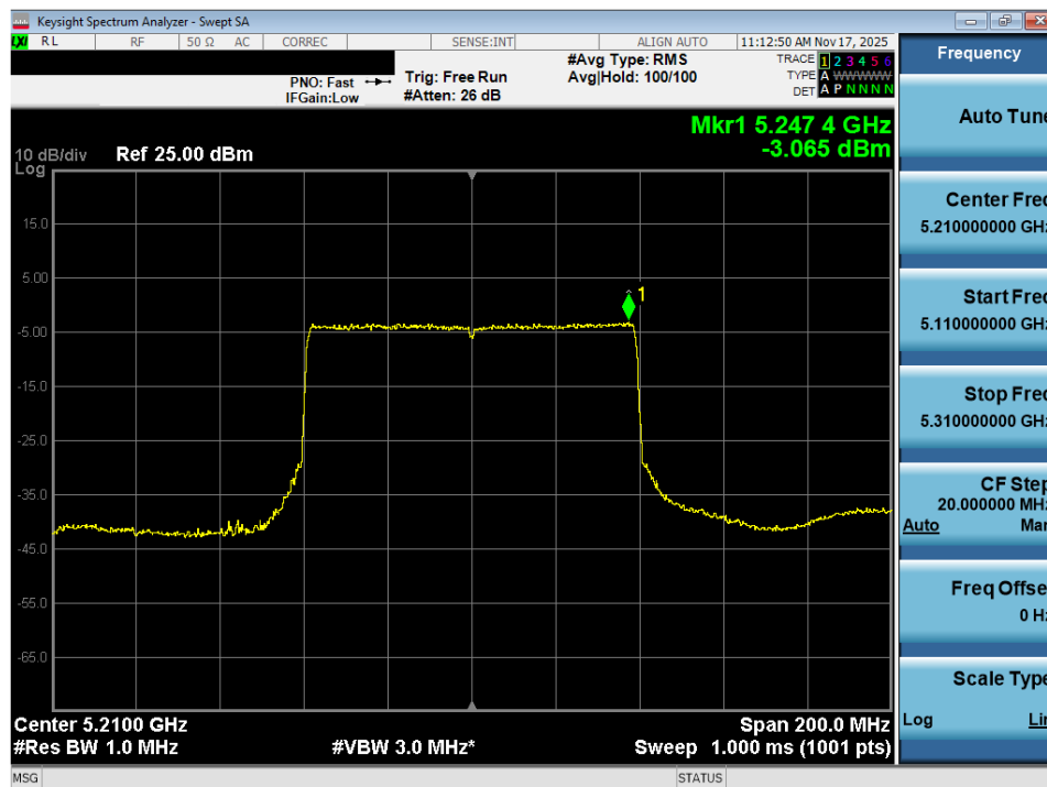
Plot 7-90. Power Spectral Density Plot MIMO ANT2 (80MHz BW 802.11ax – 996 Tones (UNII Band 1) – Ch. 42)
