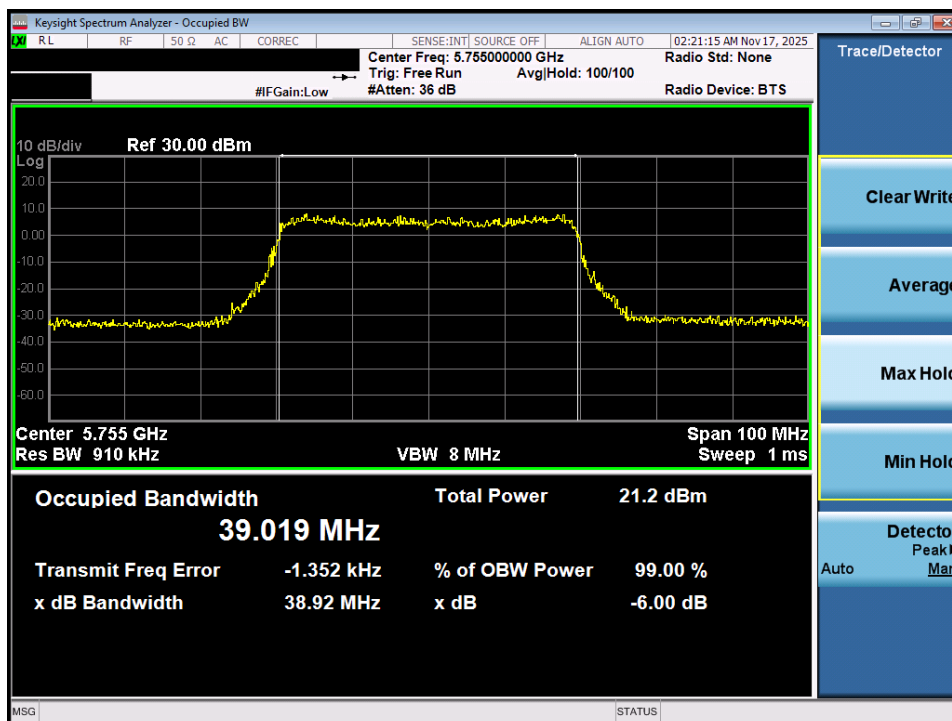
Plot 7-44. OBW Plot MIMO ANT1 (40MHz BW 802.11ax – 484 Tones (UNII Band 3) – Ch. 151)
