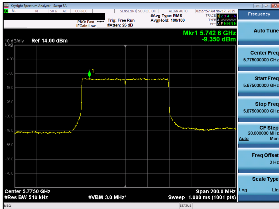
Plot 7-75. Power Spectral Density Plot MIMO ANT1 (80MHz BW 802.11ax – 996 Tones (UNII Band 3) – Ch. 155)
