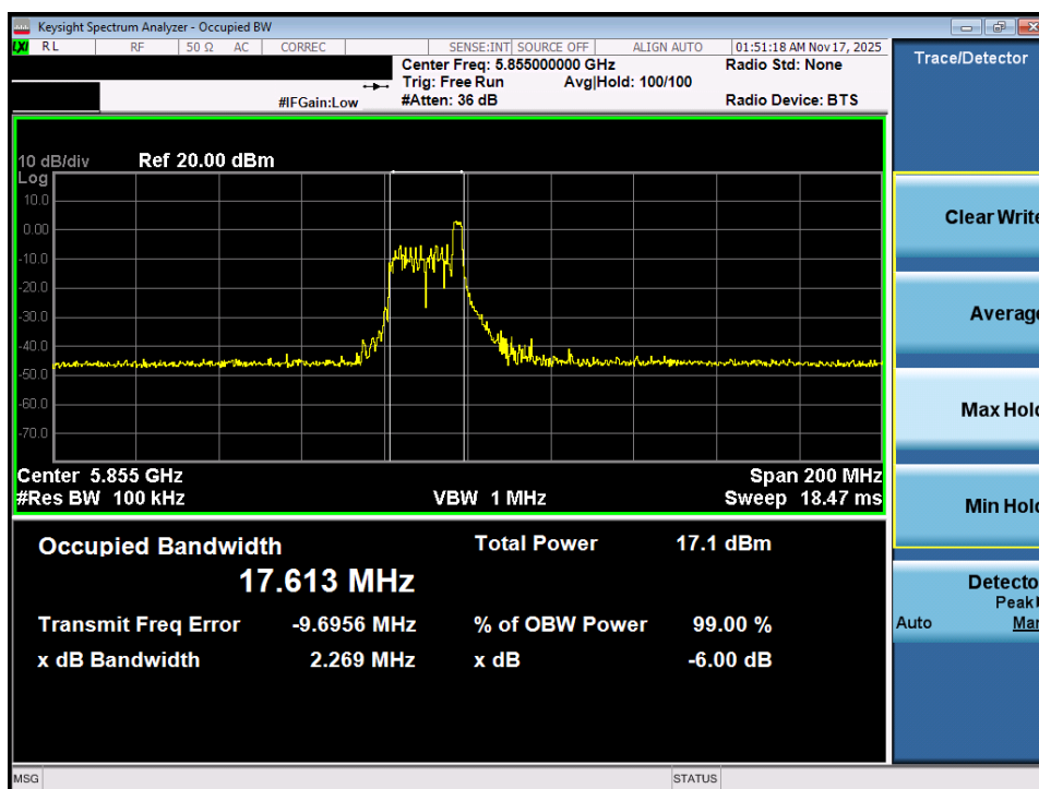
Plot 7-18. 6dB Bandwidth Plot MIMO ANT1 (80MHz BW 802.11ax – 26 Tones (UNII Band 3/4) – Ch. 171)
