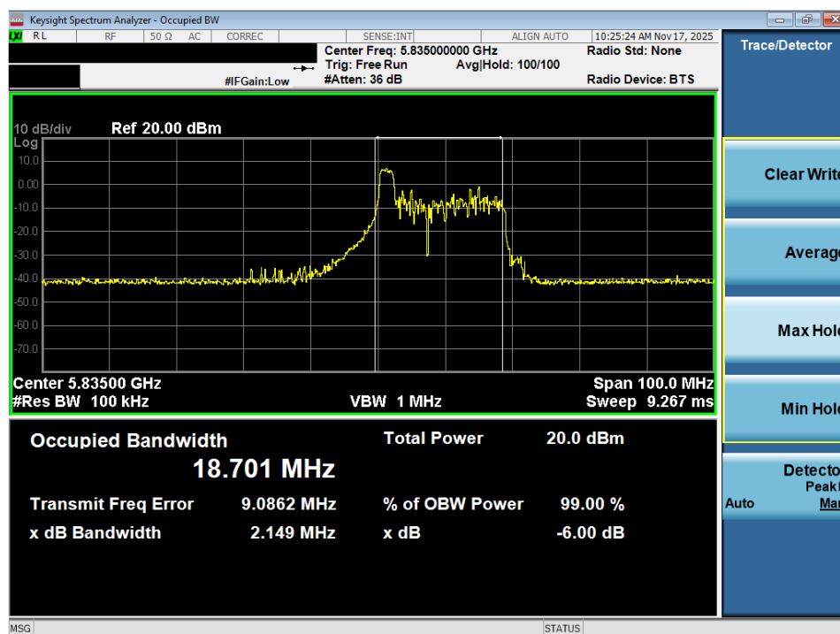
Plot 7-29. 6dB Bandwidth Plot MIMO ANT2 (40MHz BW 802.11ax – 26 Tones (UNII Band 3/4) – Ch. 167)
