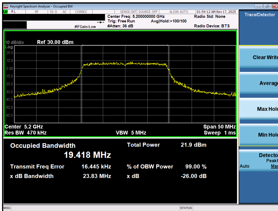
Plot 7-4. 26dB Bandwidth Plot MIMO ANT1 (20MHz BW 802.11ax – 242 Tones (UNII Band 1) – Ch. 40)
