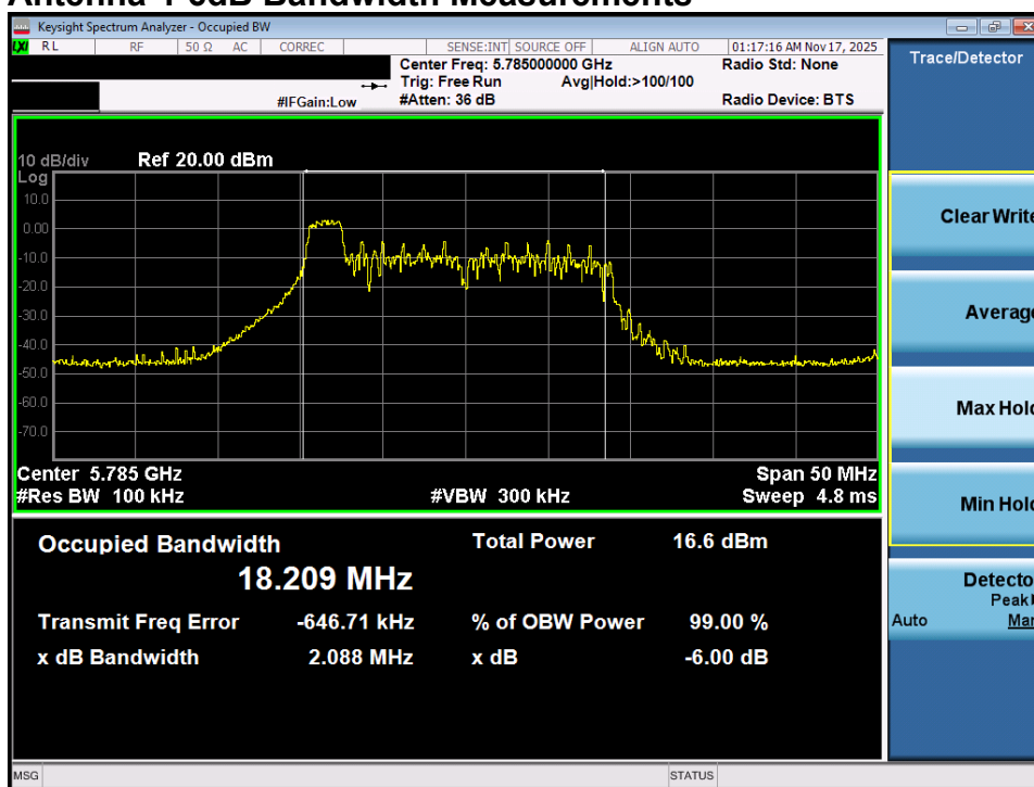
Plot 7-13. 6dB Bandwidth Plot MIMO ANT1 (20MHz BW 802.11ax – 26 Tones (UNII Band 3) – Ch. 157)
