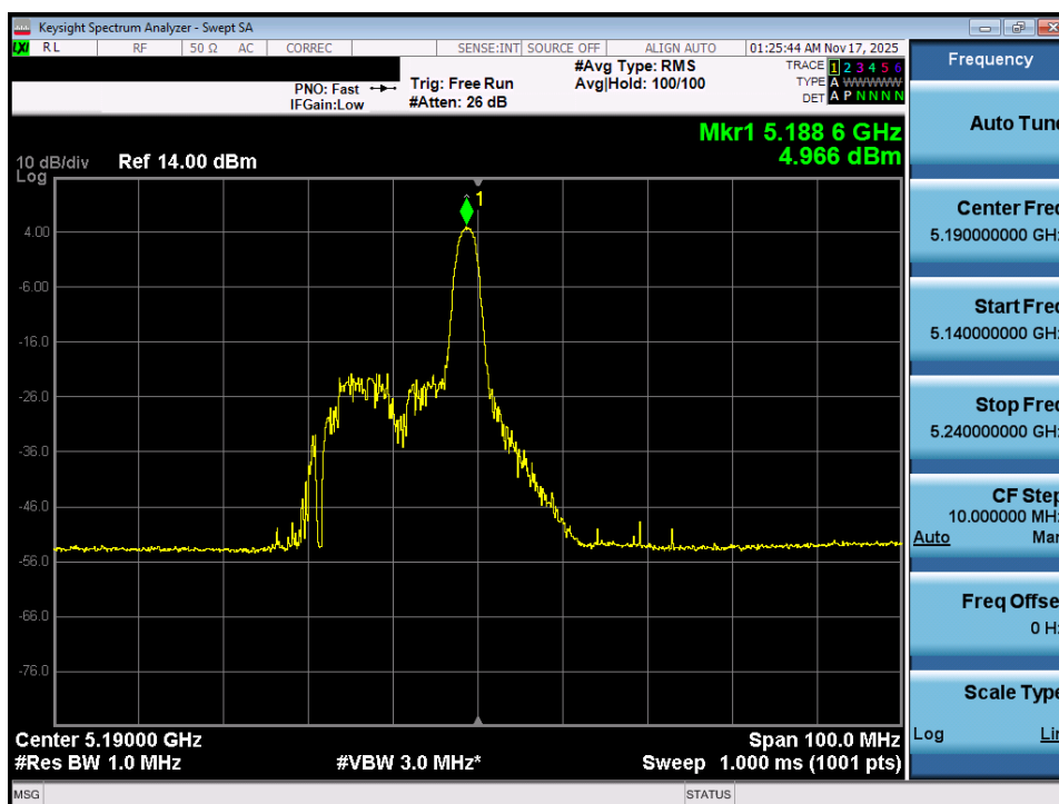
Plot 7-62. Power Spectral Density Plot MIMO ANT1 (40MHz BW 802.11ax – 26 Tones (UNII Band 1) – Ch. 38)
