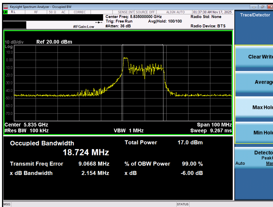
Plot 7-17. 6dB Bandwidth Plot MIMO ANT1 (40MHz BW 802.11ax – 26 Tones (UNII Band 3/4) – Ch. 167)
