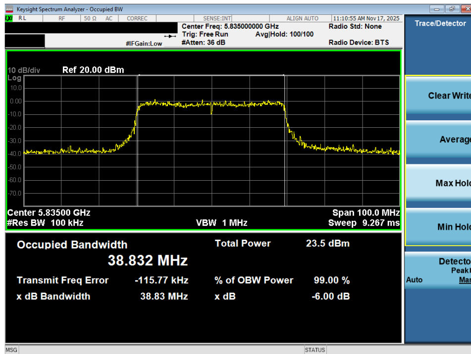
Plot 7-35. 6dB Bandwidth Plot MIMO ANT2 (40MHz BW 802.11ax – 484 Tones (UNII Band 3/4) – Ch. 167)
