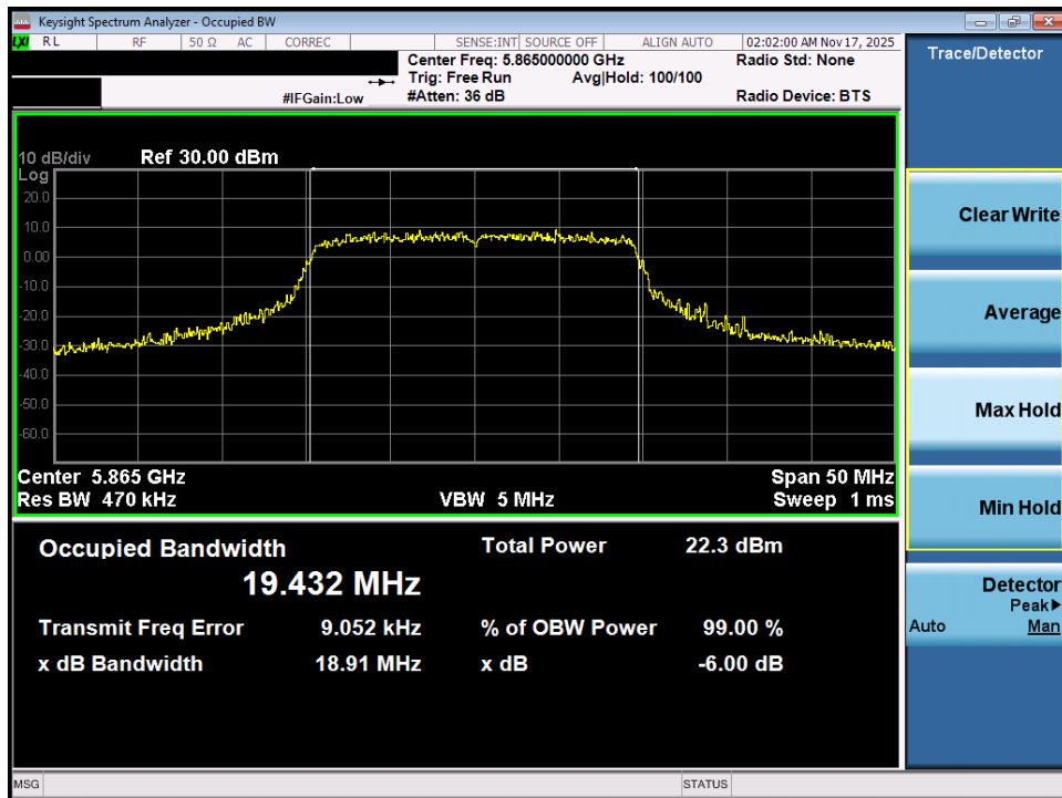
Plot 7-46. OBW Plot MIMO ANT1 (20MHz BW 802.11ax – 242 Tones (UNII Band 4) – Ch. 173)
