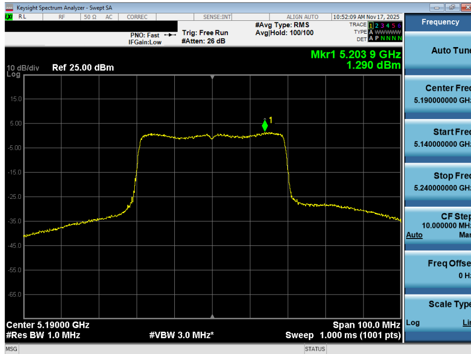
Plot 7-89. Power Spectral Density Plot MIMO ANT2 (40MHz BW 802.11ax – 484 Tones (UNII Band 1) – Ch. 38)
