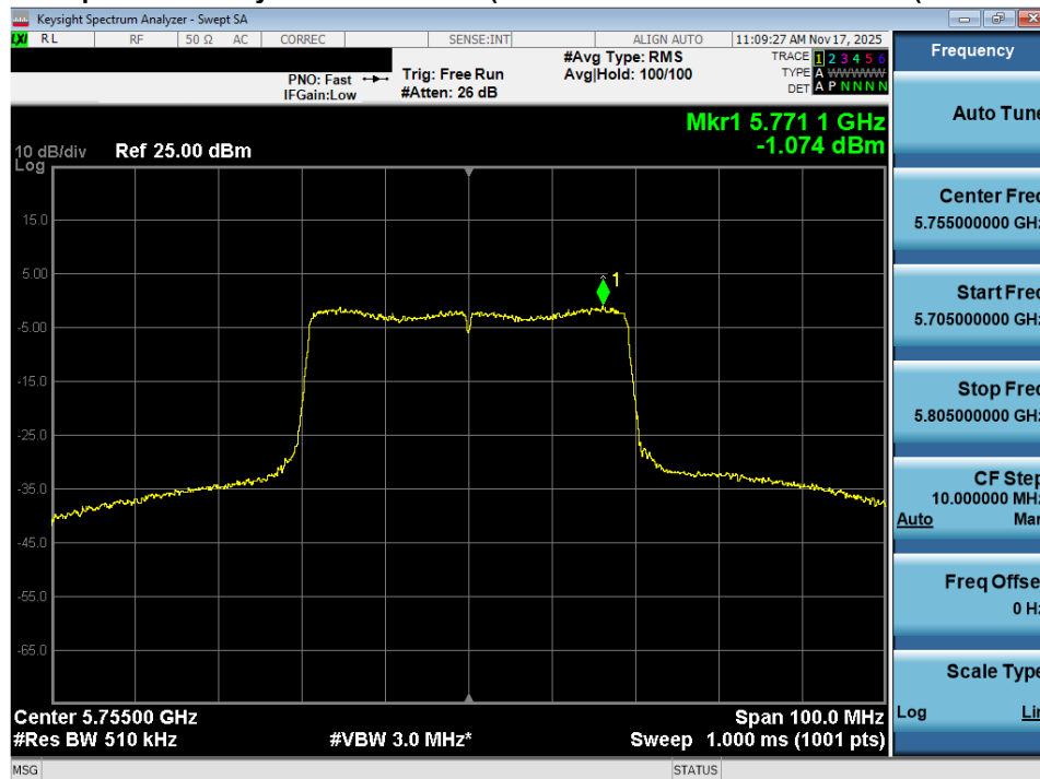
Plot 7-92. Power Spectral Density Plot MIMO ANT2 (40MHz BW 802.11ax – 484 Tones (UNII Band 3) – Ch. 151)
