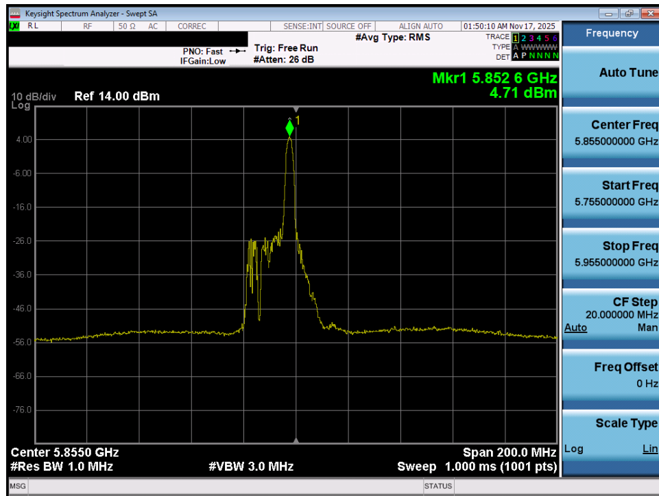
Plot 7-69. Power Spectral Density Plot MIMO ANT1 (80MHz BW 802.11ax – 26 Tones (UNII Band 3/4) – Ch. 171)
