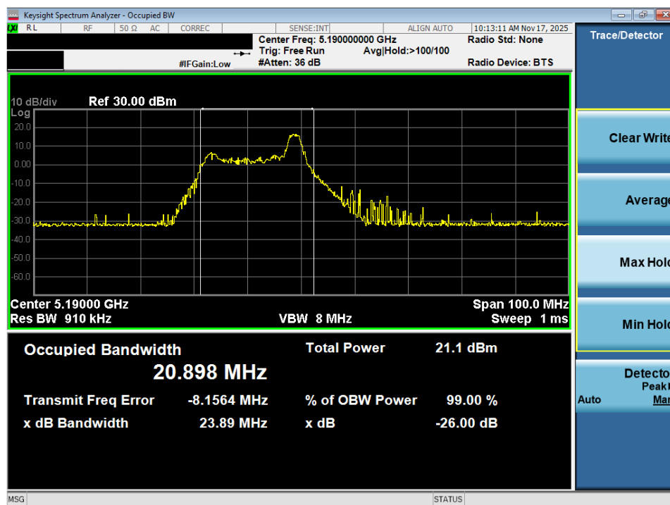
Plot 7-8. 26dB Bandwidth Plot MIMO ANT2 (40MHz BW 802.11ax – 26 Tones (UNII Band 1) – Ch. 38)
