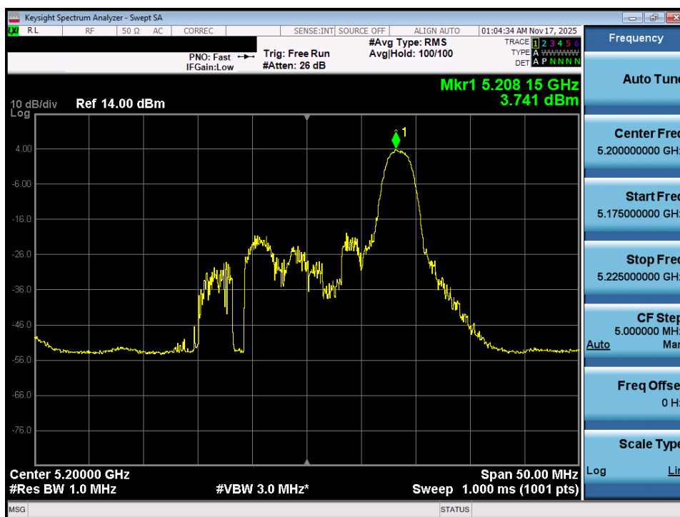
Plot 7-61. Power Spectral Density Plot MIMO ANT1 (20MHz BW 802.11ax – 26 Tones (UNII Band 1) – Ch. 40)
