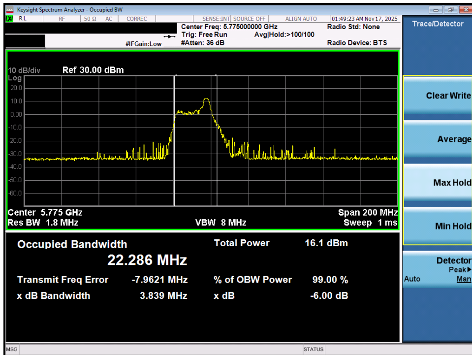
Plot 7-39. OBW Plot MIMO ANT1 (80MHz BW 802.11ax – 26 Tones (UNII Band 3) – Ch. 155)
