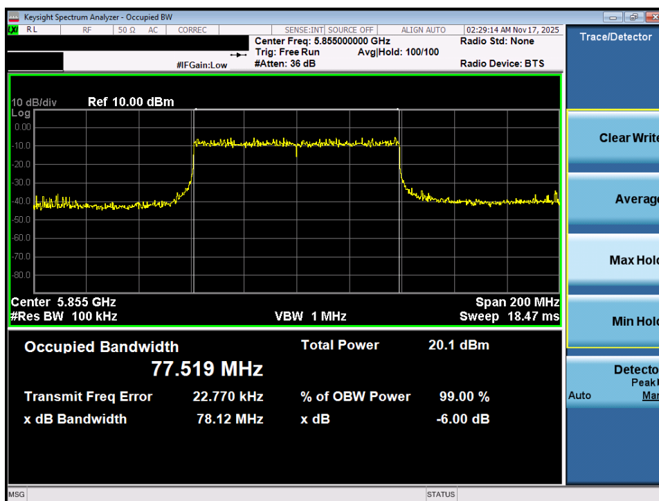
Plot 7-24. 6dB Bandwidth Plot MIMO ANT1 (80MHz BW 802.11ax – 996 Tones (UNII Band 3/4) – Ch. 171)
