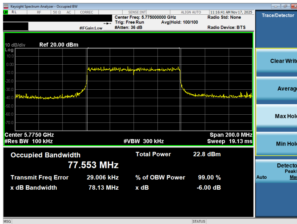
Plot 7-33. 6dB Bandwidth Plot MIMO ANT2 (80MHz BW 802.11ax – 996 Tones (UNII Band 3) – Ch. 155)
