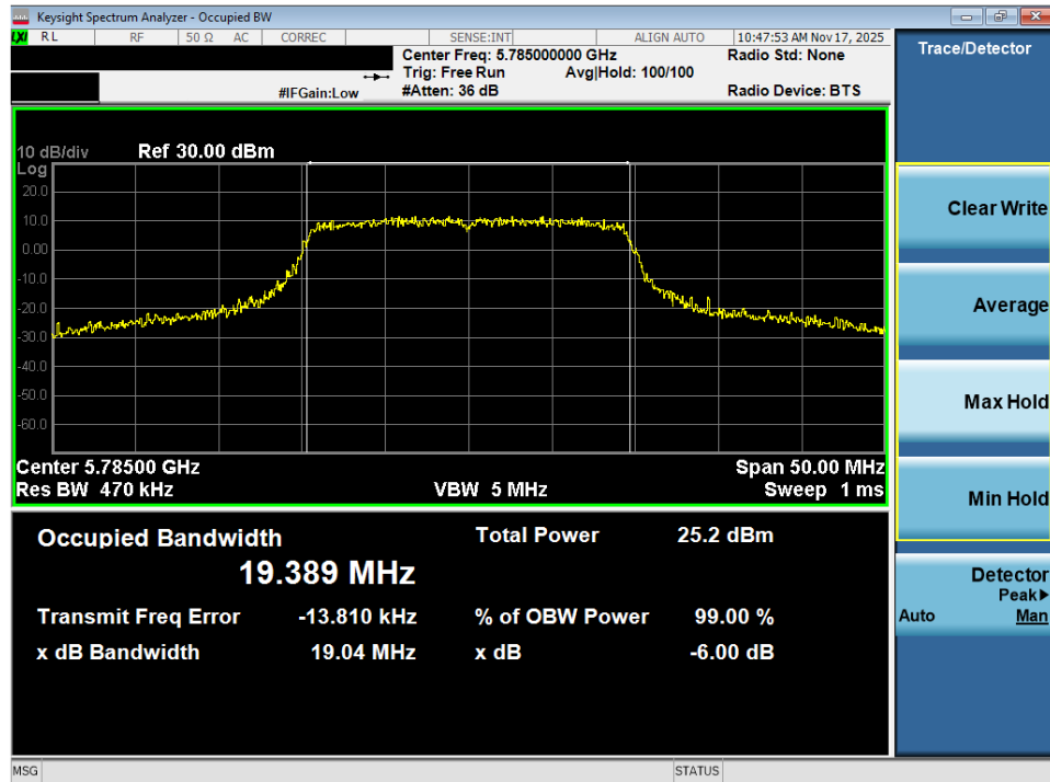
Plot 7-55. OBW Plot MIMO ANT2 (20MHz BW 802.11ax – 242 Tones (UNII Band 3) – Ch. 157)
