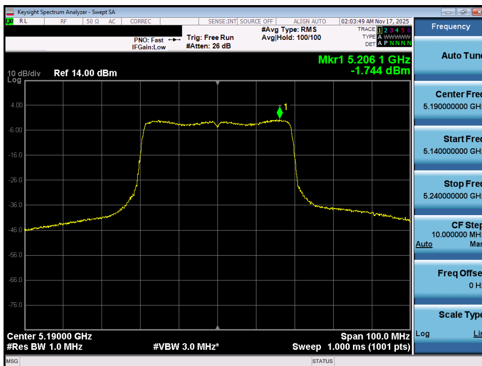
Plot 7-71. Power Spectral Density Plot MIMO ANT1 (40MHz BW 802.11ax – 484 Tones (UNII Band 1) – Ch. 38)
