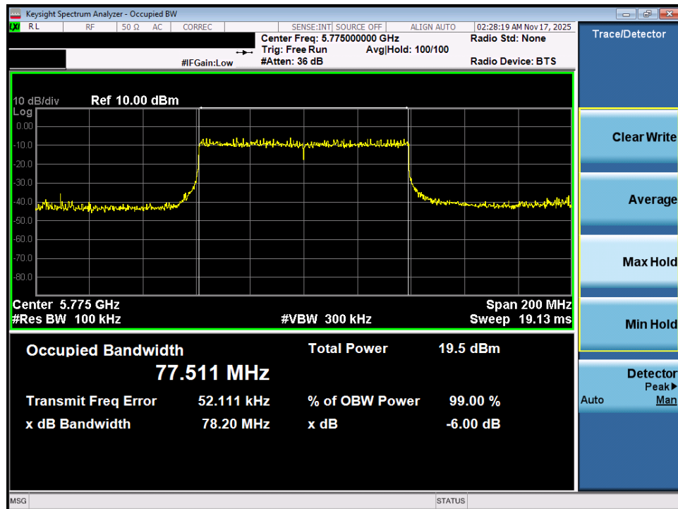
Plot 7-21. 6dB Bandwidth Plot MIMO ANT1 (80MHz BW 802.11ax – 996 Tones (UNII Band 3) – Ch. 155)
