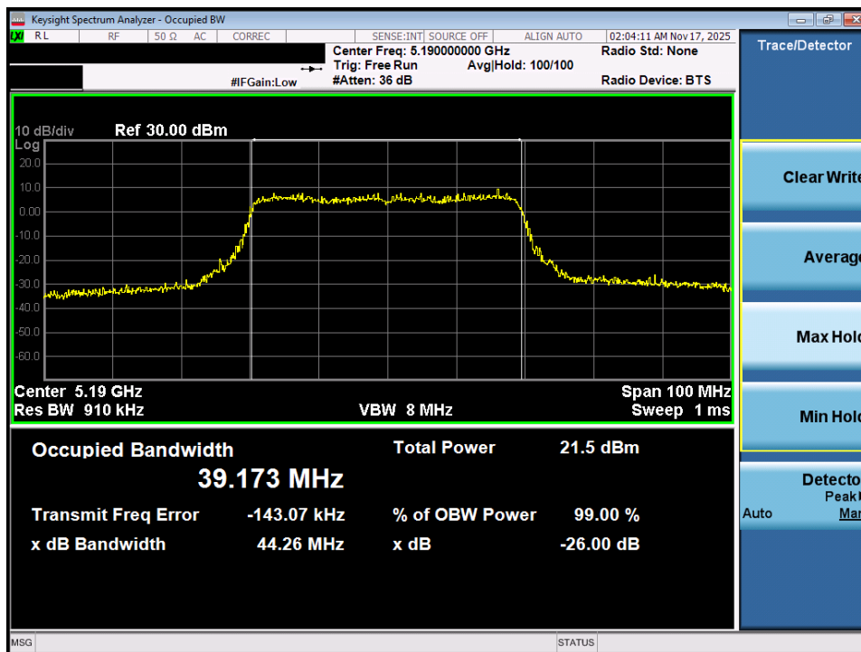
Plot 7-5. 26dB Bandwidth Plot MIMO ANT1 (40MHz BW 802.11ax – 484 Tones (UNII Band 1) – Ch. 38)
