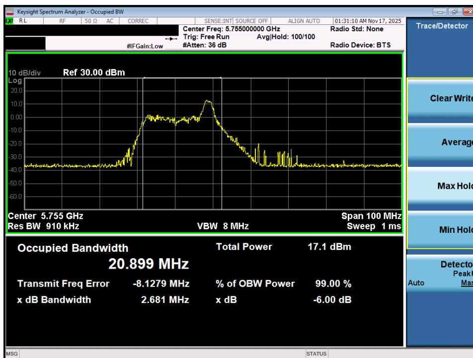
Plot 7-38. OBW Plot MIMO ANT1 (40MHz BW 802.11ax – 26 Tones (UNII Band 3) – Ch. 151)
