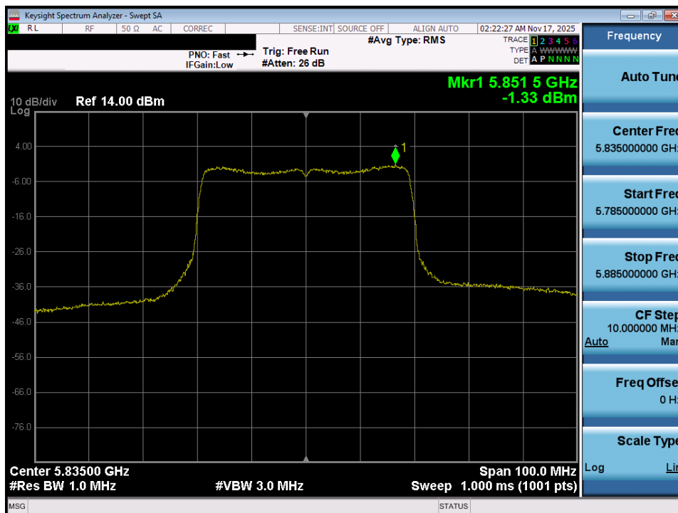
Plot 7-77. Power Spectral Density Plot MIMO ANT1 (40MHz BW 802.11ax – 484 Tones (UNII Band 3/4) – Ch. 167)
