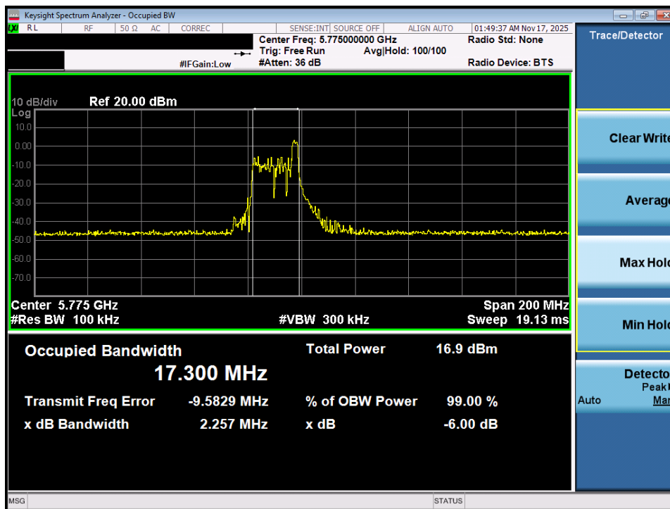
Plot 7-15. 6dB Bandwidth Plot MIMO ANT1 (80MHz BW 802.11ax – 26 Tones (UNII Band 3) – Ch. 155)
