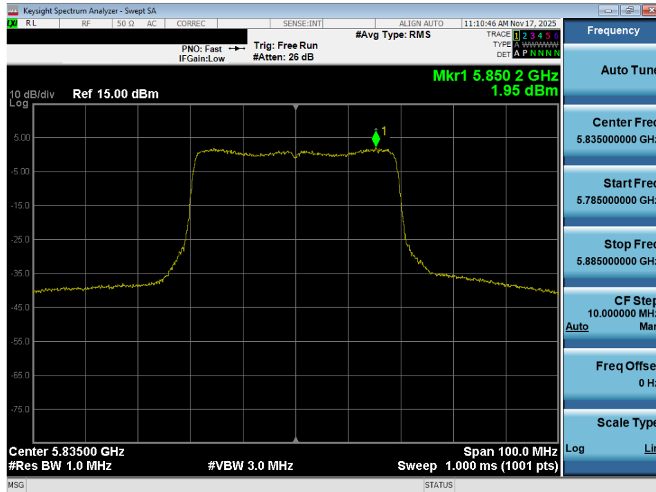
Plot 7-95. Power Spectral Density Plot MIMO ANT2 (40MHz BW 802.11ax – 484 Tones (UNII Band 3/4) – Ch. 167)
