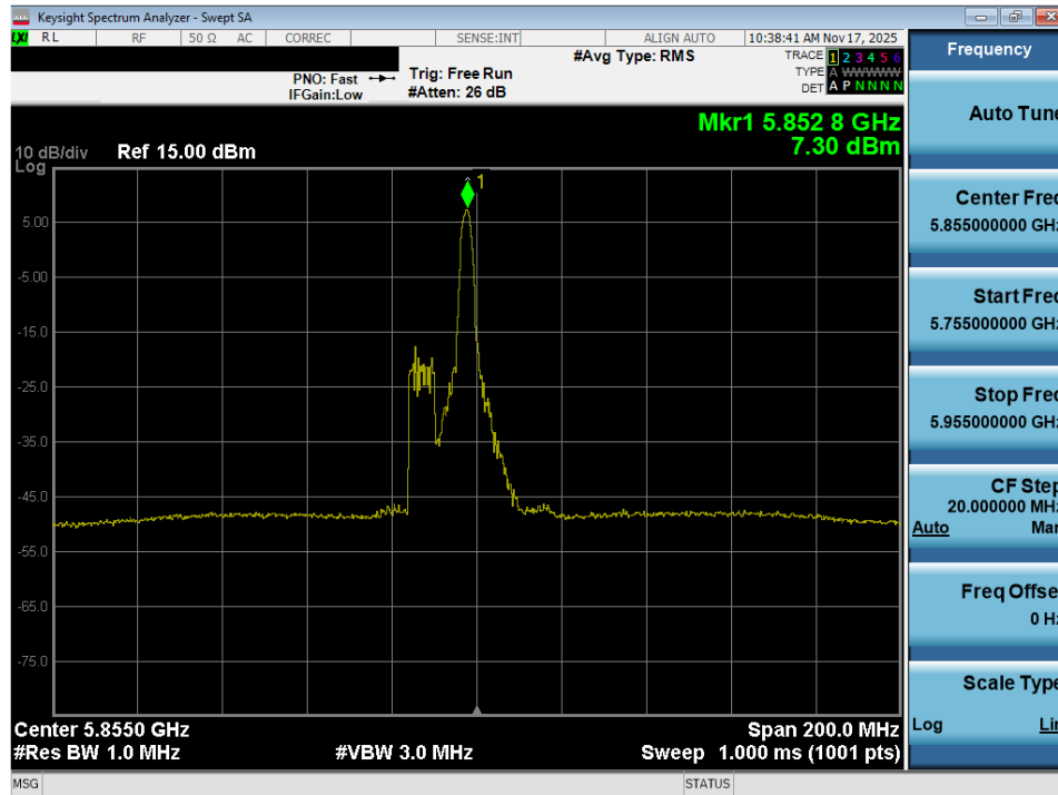
Plot 7-87. Power Spectral Density Plot MIMO ANT2 (80MHz BW 802.11ax – 26 Tones (UNII Band 3/4) – Ch. 171)
