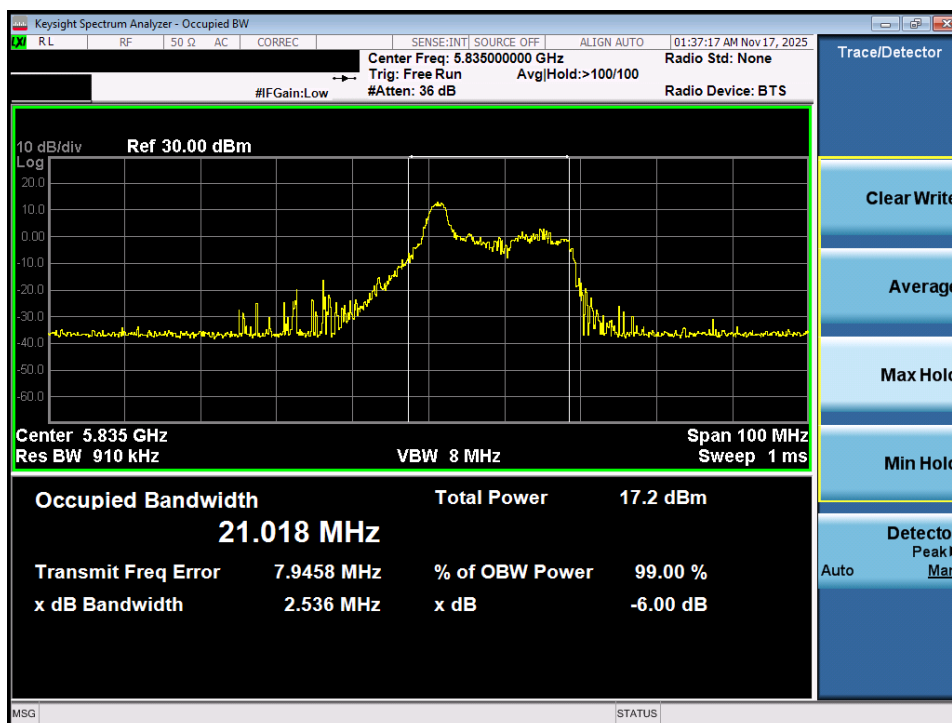
Plot 7-41. OBW Plot MIMO ANT1 (40MHz BW 802.11ax – 26 Tones (UNII Band 3/4) – Ch. 167)
