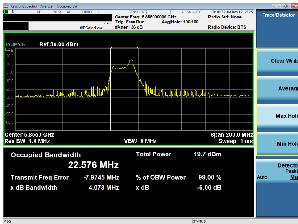
Plot 7-54. OBW Plot MIMO ANT2 (80MHz BW 802.11ax – 26 Tones (UNII Band 3/4) – Ch. 171)
