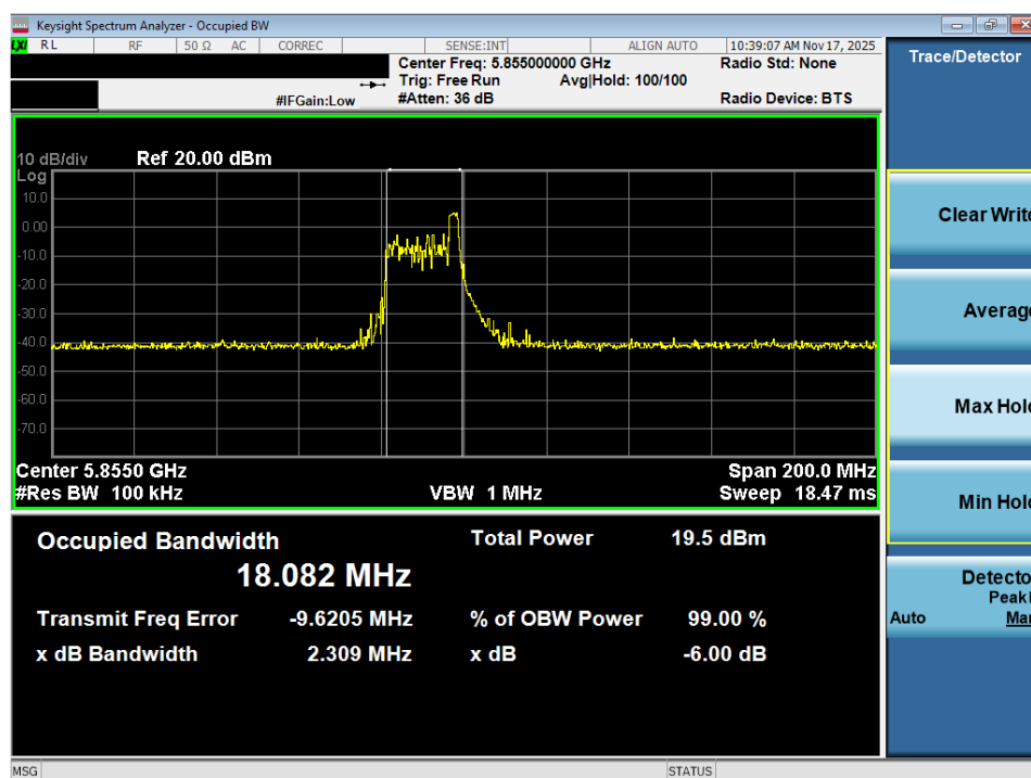
Plot 7-30. 6dB Bandwidth Plot MIMO ANT2 (80MHz BW 802.11ax – 26 Tones (UNII Band 3/4) – Ch. 171)
