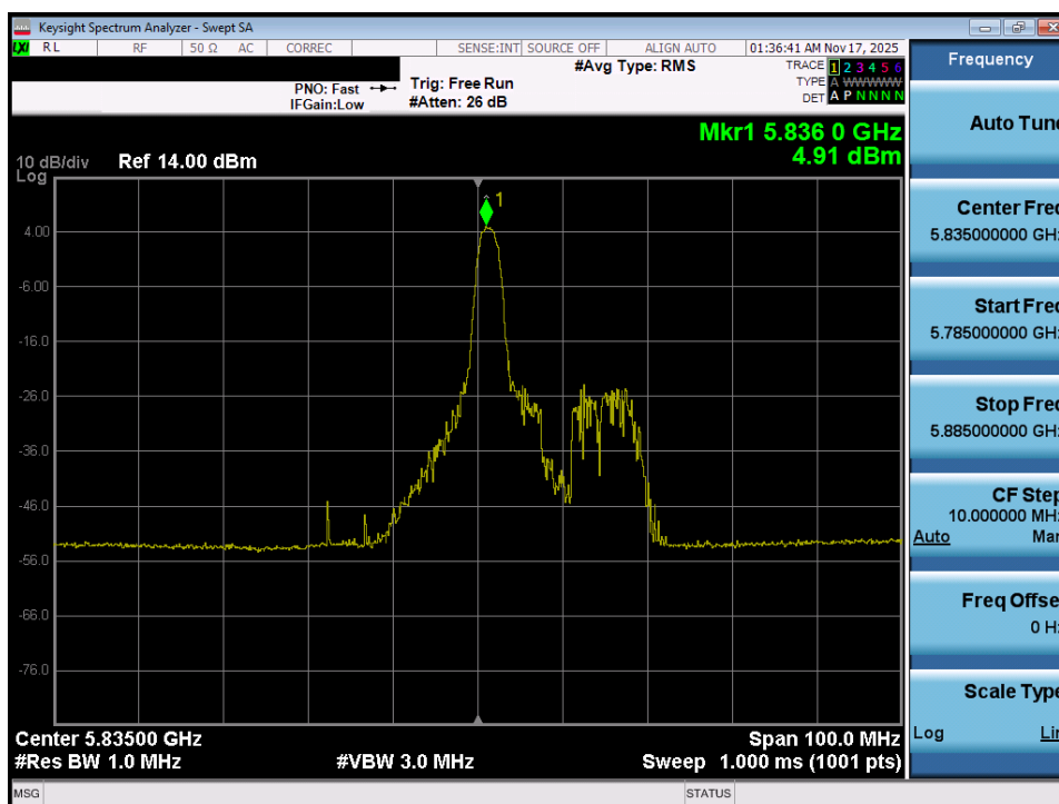
Plot 7-68. Power Spectral Density Plot MIMO ANT1 (40MHz BW 802.11ax – 26 Tones (UNII Band 3/4) – Ch. 167)
