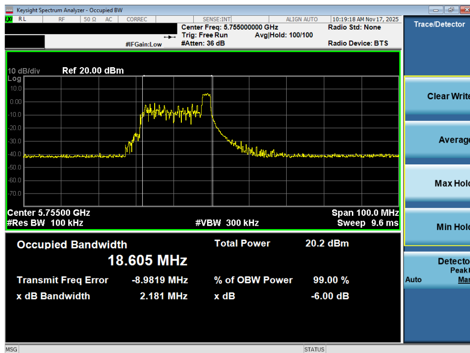
Plot 7-26. 6dB Bandwidth Plot MIMO ANT2 (40MHz BW 802.11ax – 26 Tones (UNII Band 3) – Ch. 151)
