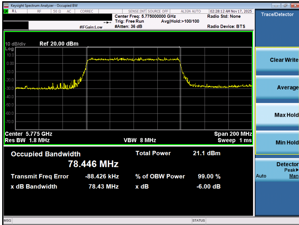
Plot 7-45. OBW Plot MIMO ANT1 (80MHz BW 802.11ax – 996 Tones (UNII Band 3) – Ch. 155)
