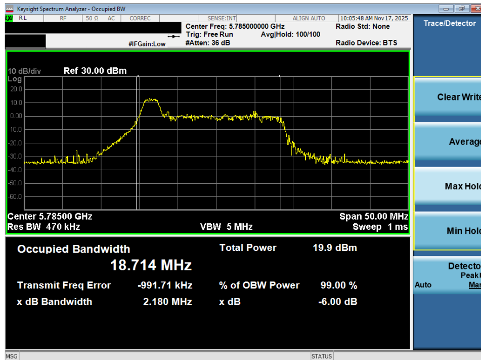
Plot 7-49. OBW Plot MIMO ANT2 (20MHz BW 802.11ax – 26 Tones (UNII Band 3) – Ch. 157)
