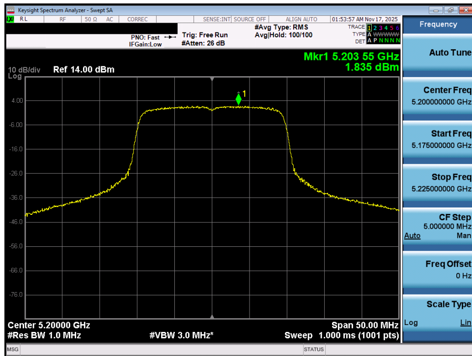
Plot 7-70. Power Spectral Density Plot MIMO ANT1 (20MHz BW 802.11ax – 242 Tones (UNII Band 1) – Ch. 40)
