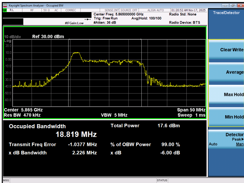
Plot 7-40. OBW Plot MIMO ANT1 (20MHz BW 802.11ax – 26 Tones (UNII Band 4) – Ch. 173)
