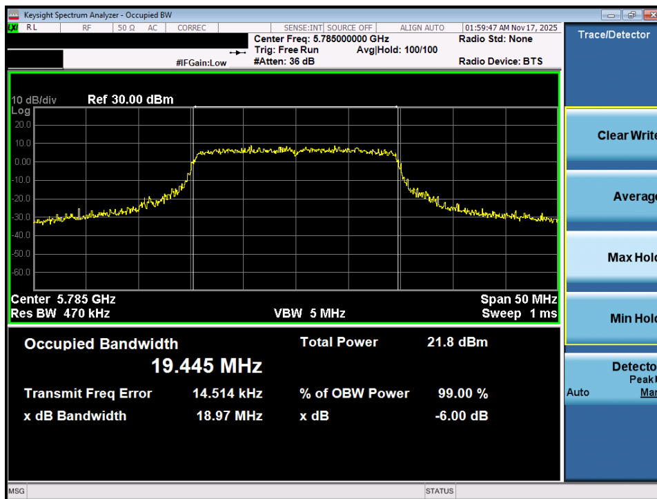
Plot 7-43. OBW Plot MIMO ANT1 (20MHz BW 802.11ax – 242 Tones (UNII Band 3) – Ch. 157)
