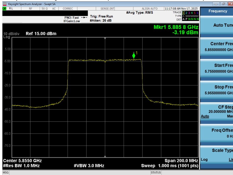
Plot 7-96. Power Spectral Density Plot MIMO ANT2 (80MHz BW 802.11ax – 996 Tones (UNII Band 3/4) – Ch. 171)
