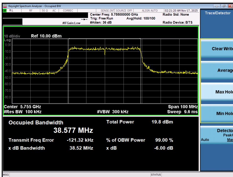
Plot 7-20. 6dB Bandwidth Plot MIMO ANT1 (40MHz BW 802.11ax – 484 Tones (UNII Band 3) – Ch. 151)
