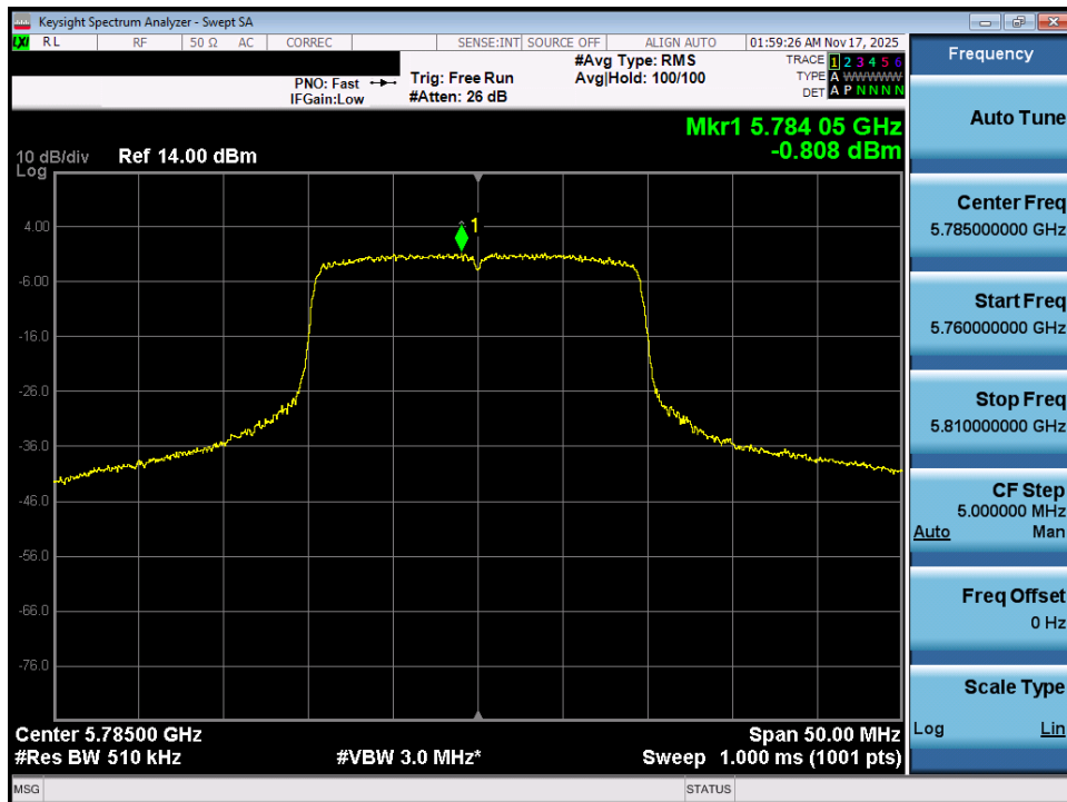
Plot 7-73. Power Spectral Density Plot MIMO ANT1 (20MHz BW 802.11ax – 242 Tones (UNII Band 3) – Ch. 157)
