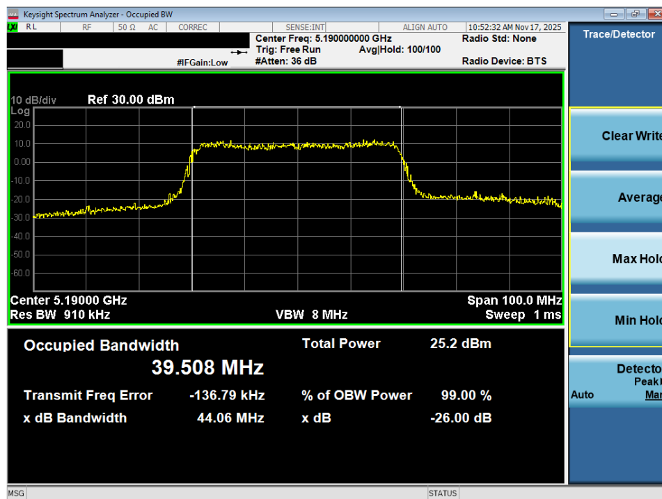
Plot 7-11. 26dB Bandwidth Plot MIMO ANT2 (40MHz BW 802.11ax – 484 Tones (UNII Band 1) – Ch. 38)
