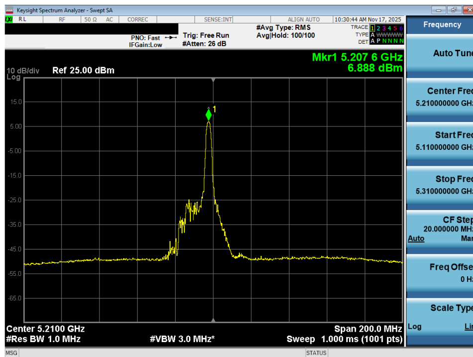
Plot 7-81. Power Spectral Density Plot MIMO ANT2 (80MHz BW 802.11ax – 26 Tones (UNII Band 1) – Ch. 42)
