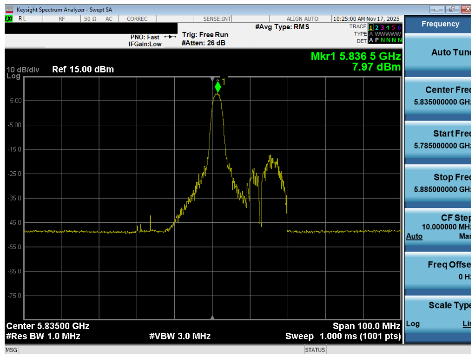
Plot 7-86. Power Spectral Density Plot MIMO ANT2 (40MHz BW 802.11ax – 26 Tones (UNII Band 3/4) – Ch. 167)
