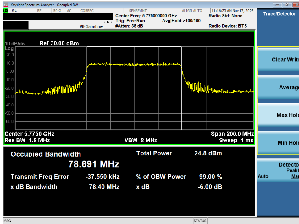
Plot 7-57. OBW Plot MIMO ANT2 (80MHz BW 802.11ax – 996 Tones (UNII Band 3) – Ch. 155)
