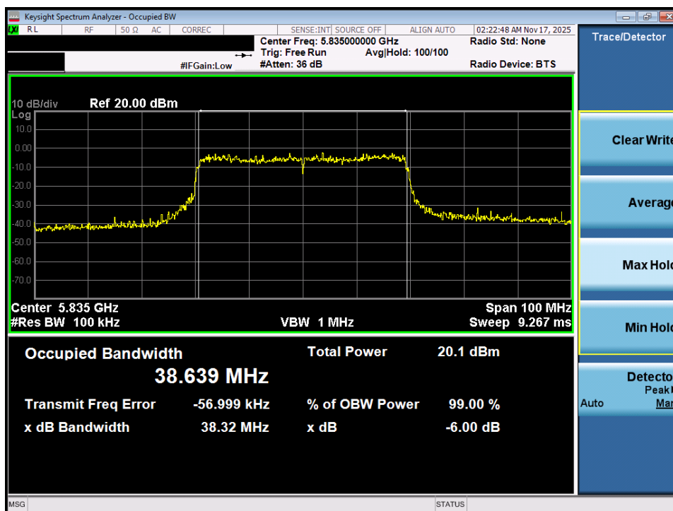
Plot 7-23. 6dB Bandwidth Plot MIMO ANT1 (40MHz BW 802.11ax – 484 Tones (UNII Band 3/4) – Ch. 167)
