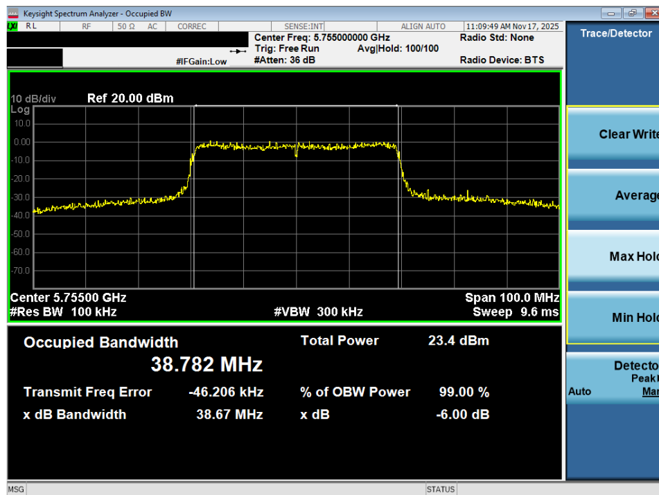
Plot 7-32. 6dB Bandwidth Plot MIMO ANT2 (40MHz BW 802.11ax – 484 Tones (UNII Band 3) – Ch. 151)
