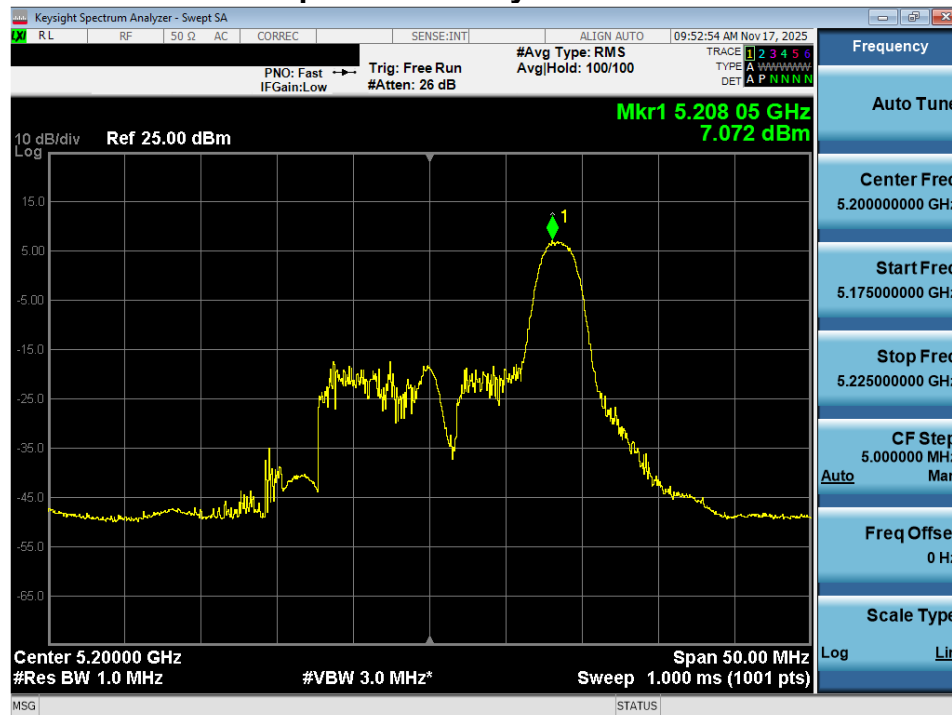
Plot 7-79. Power Spectral Density Plot MIMO ANT2 (20MHz BW 802.11ax – 26 Tones (UNII Band 1) – Ch. 40)
