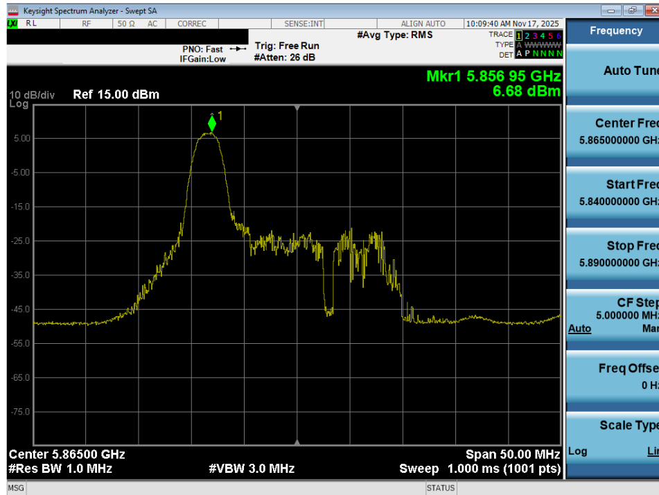
Plot 7-85. Power Spectral Density Plot MIMO ANT2 (20MHz BW 802.11ax – 26 Tones (UNII Band 4) – Ch. 173)
