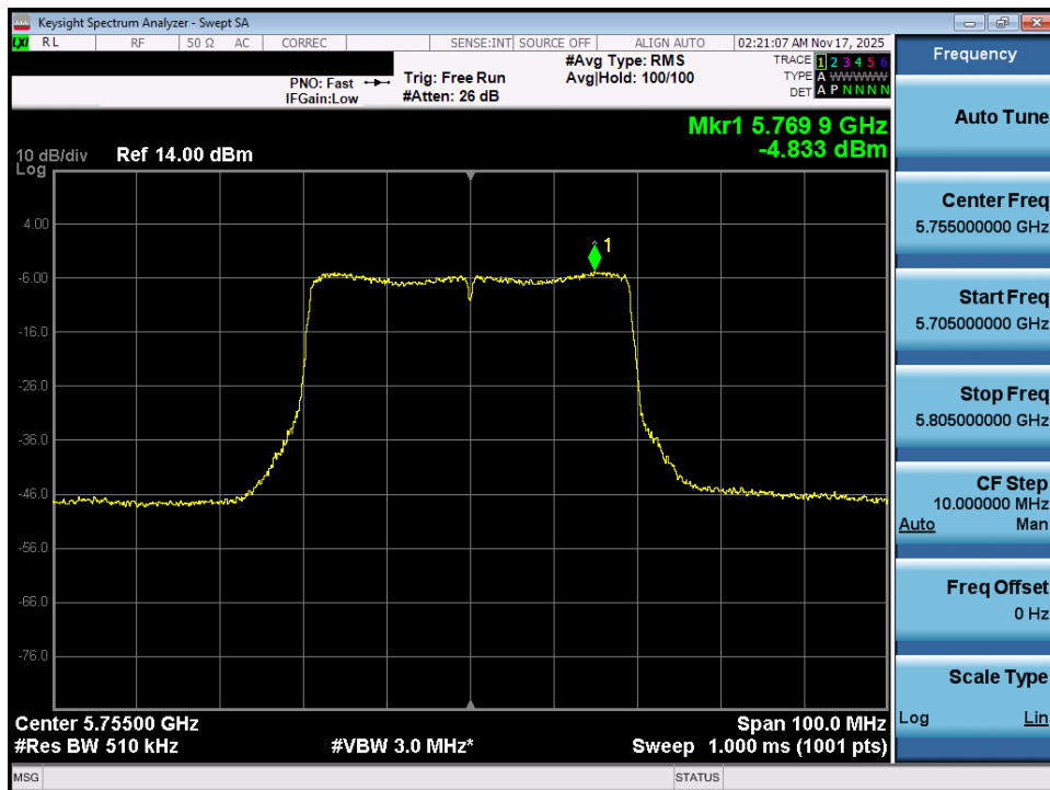
Plot 7-74. Power Spectral Density Plot MIMO ANT1 (40MHz BW 802.11ax – 484 Tones (UNII Band 3) – Ch. 151)
