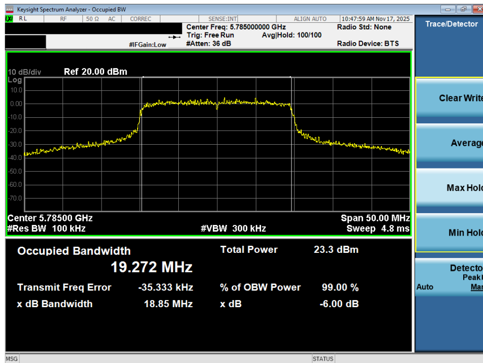
Plot 7-31. 6dB Bandwidth Plot MIMO ANT2 (20MHz BW 802.11ax – 242 Tones (UNII Band 3) – Ch. 157)
