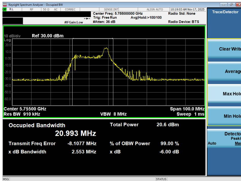
Plot 7-50. OBW Plot MIMO ANT2 (40MHz BW 802.11ax – 26 Tones (UNII Band 3) – Ch. 151)
