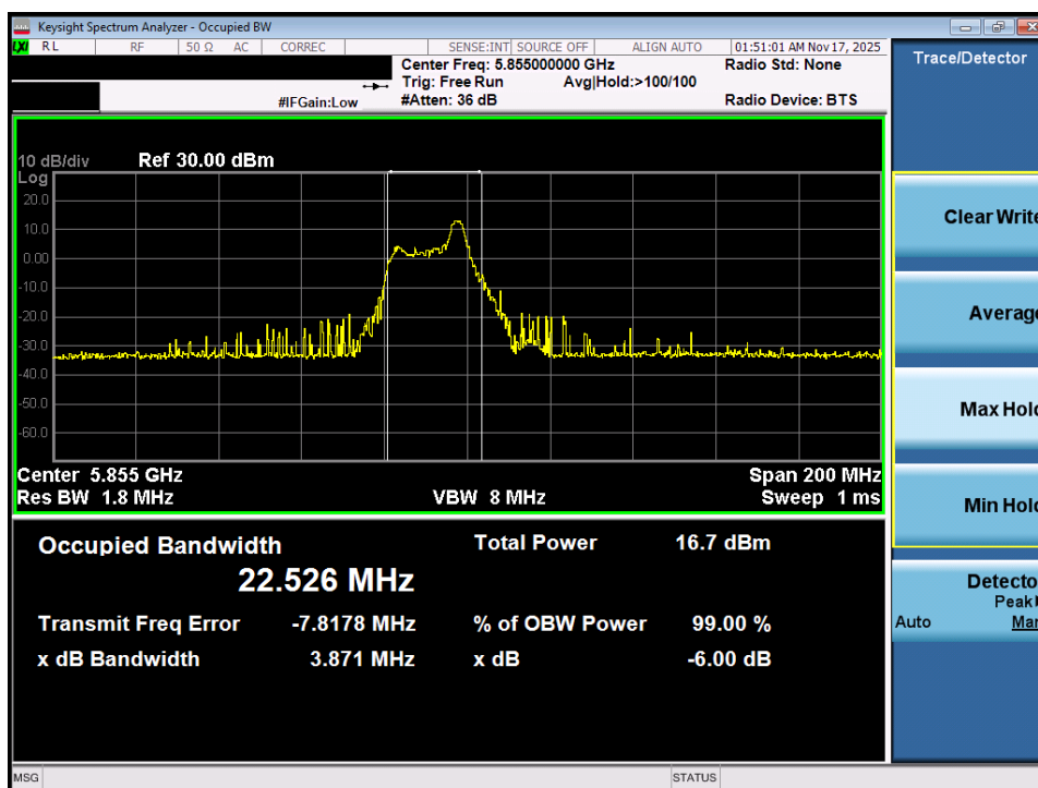
Plot 7-42. OBW Plot MIMO ANT1 (80MHz BW 802.11ax – 26 Tones (UNII Band 3/4) – Ch. 171)
