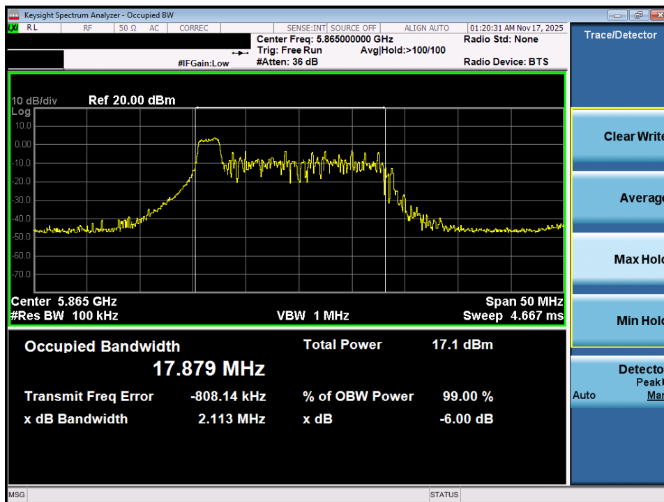
Plot 7-16. 6dB Bandwidth Plot MIMO ANT1 (20MHz BW 802.11ax – 26 Tones (UNII Band 4) – Ch. 173)
