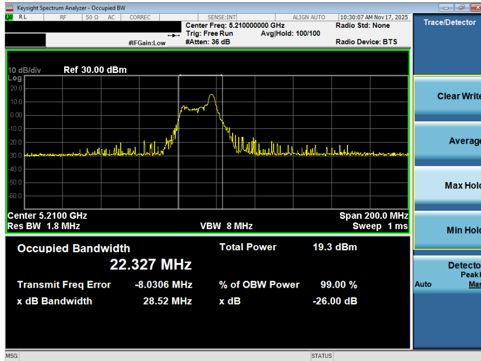
Plot 7-9. 26dB Bandwidth Plot MIMO ANT2 (80MHz BW 802.11ax – 26 Tones (UNII Band 1) – Ch. 42)
