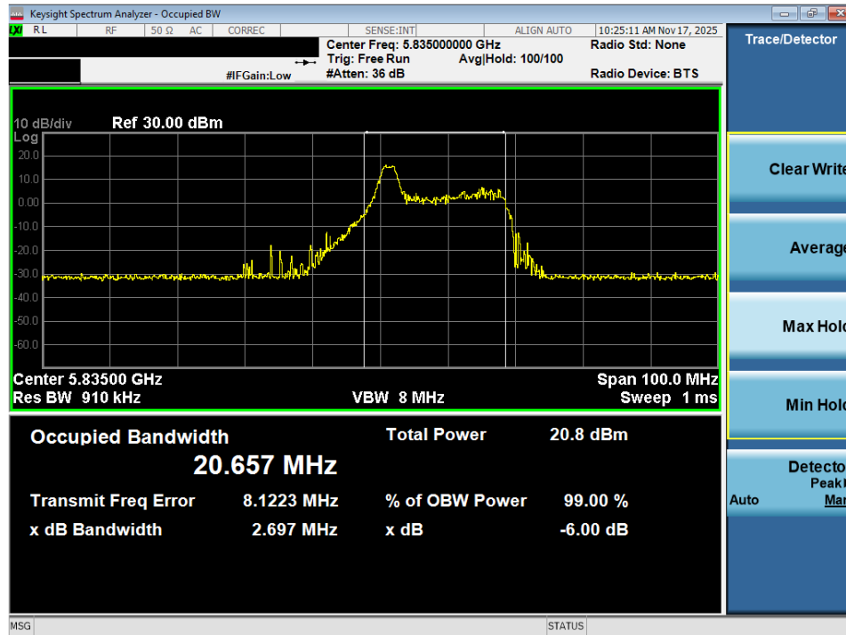
Plot 7-53. OBW Plot MIMO ANT2 (40MHz BW 802.11ax – 26 Tones (UNII Band 3/4) – Ch. 167)
