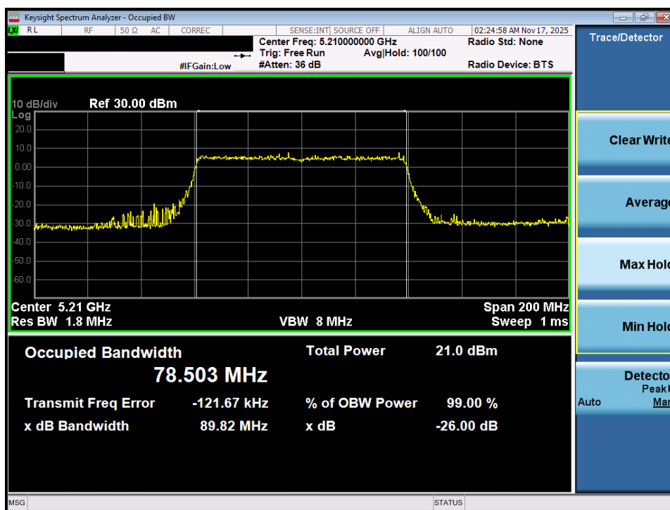
Plot 7-6. 26dB Bandwidth Plot MIMO ANT1 (80MHz BW 802.11ax – 996 Tones (UNII Band 1) – Ch. 42)
