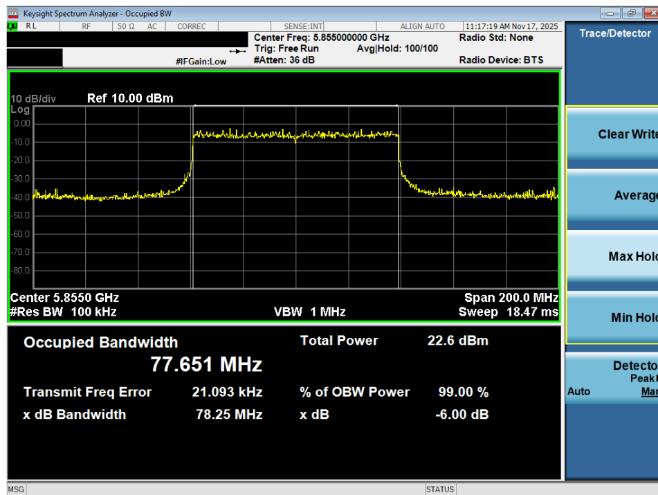
Plot 7-36. 6dB Bandwidth Plot MIMO ANT2 (80MHz BW 802.11ax – 996 Tones (UNII Band 3/4) – Ch. 171)
