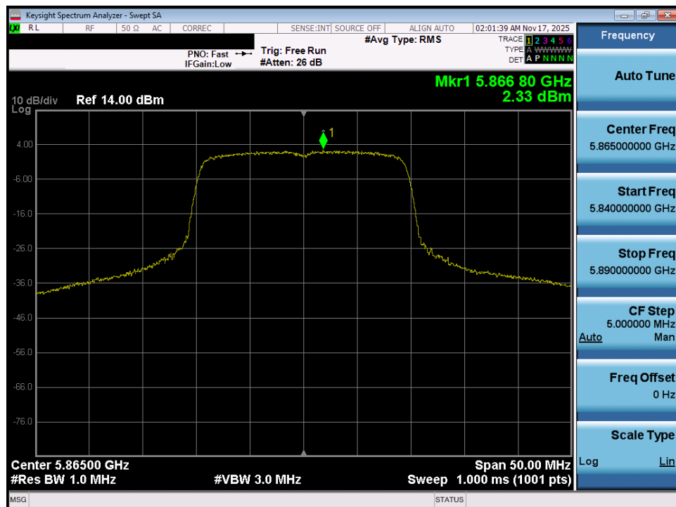
Plot 7-76. Power Spectral Density Plot MIMO ANT1 (20MHz BW 802.11ax – 242 Tones (UNII Band 4) – Ch. 173)
