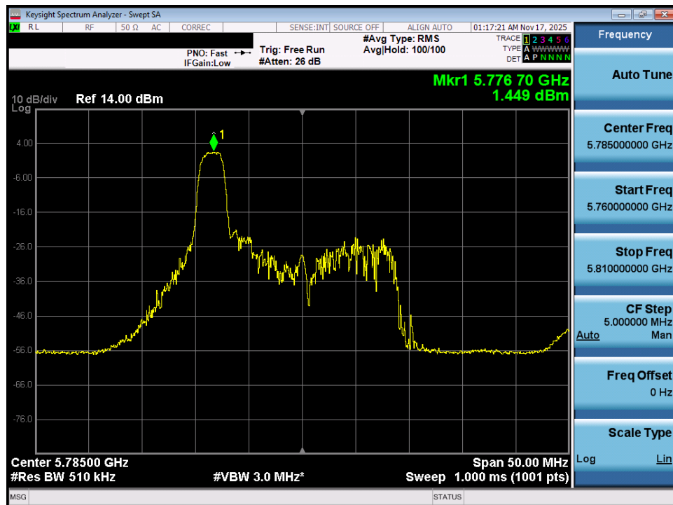
Plot 7-64. Power Spectral Density Plot MIMO ANT1 (20MHz BW 802.11ax – 26 Tones (UNII Band 3) – Ch. 157)
