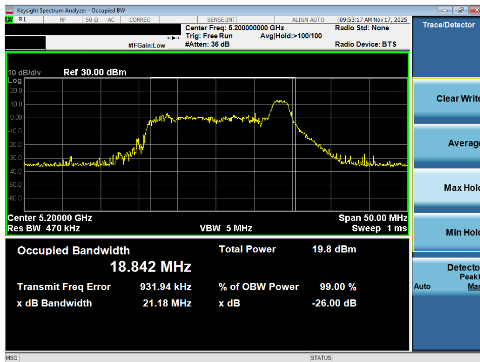
Plot 7-7. 26dB Bandwidth Plot MIMO ANT2 (20MHz BW 802.11ax – 26 Tones (UNII Band 1) – Ch. 40)
