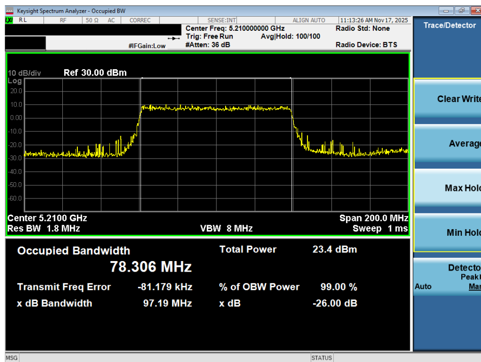
Plot 7-12. 26dB Bandwidth Plot MIMO ANT2 (80MHz BW 802.11ax – 996 Tones (UNII Band 1) – Ch. 42)
