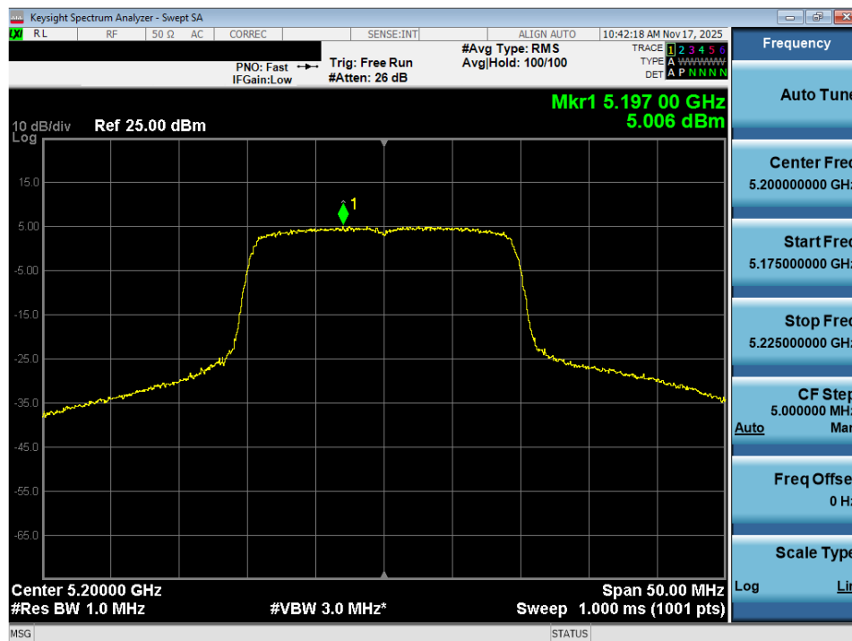
Plot 7-88. Power Spectral Density Plot MIMO ANT2 (20MHz BW 802.11ax – 242 Tones (UNII Band 1) – Ch. 40)
