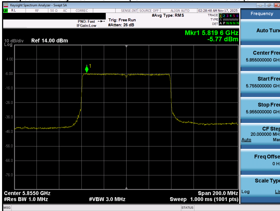
Plot 7-78. Power Spectral Density Plot MIMO ANT1 (80MHz BW 802.11ax – 996 Tones (UNII Band 3/4) – Ch. 171)
