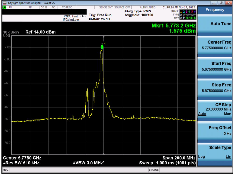
Plot 7-66. Power Spectral Density Plot MIMO ANT1 (80MHz BW 802.11ax – 26 Tones (UNII Band 3) – Ch. 155)
