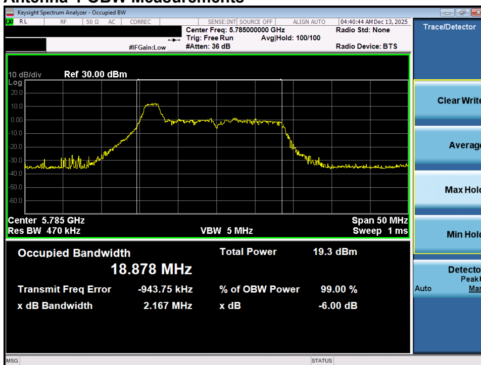
Plot 7-37. OBW Plot MIMO ANT1 (20MHz BW 802.11ax – 26 Tones (UNII Band 3) – Ch. 157)
