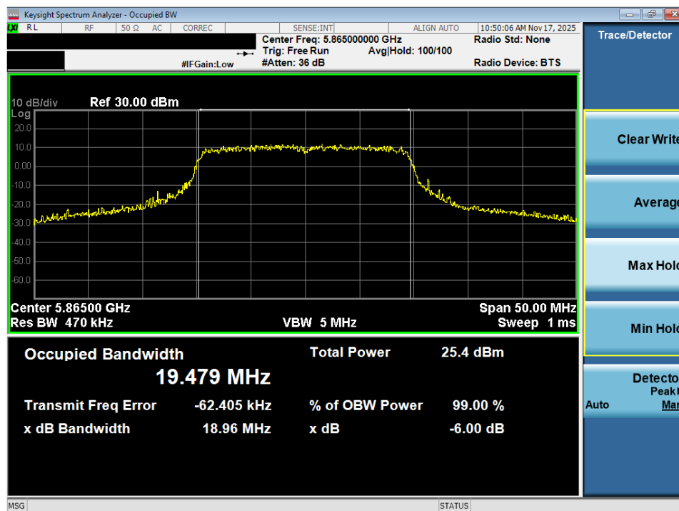
Plot 7-58. OBW Plot MIMO ANT2 (20MHz BW 802.11ax – 242 Tones (UNII Band 4) – Ch. 173)
