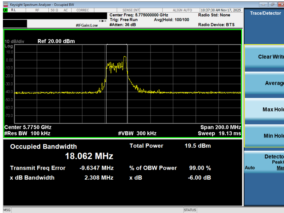
Plot 7-27. 6dB Bandwidth Plot MIMO ANT2 (80MHz BW 802.11ax – 26 Tones (UNII Band 3) – Ch. 155)
