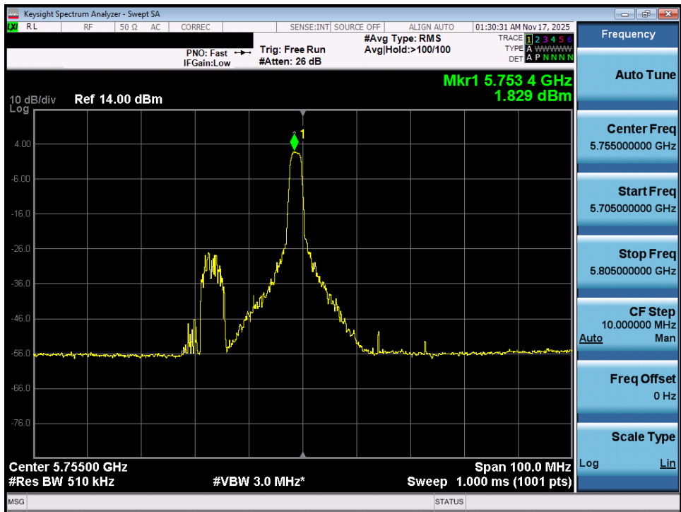
Plot 7-65. Power Spectral Density Plot MIMO ANT1 (40MHz BW 802.11ax – 26 Tones (UNII Band 3) – Ch. 151)
