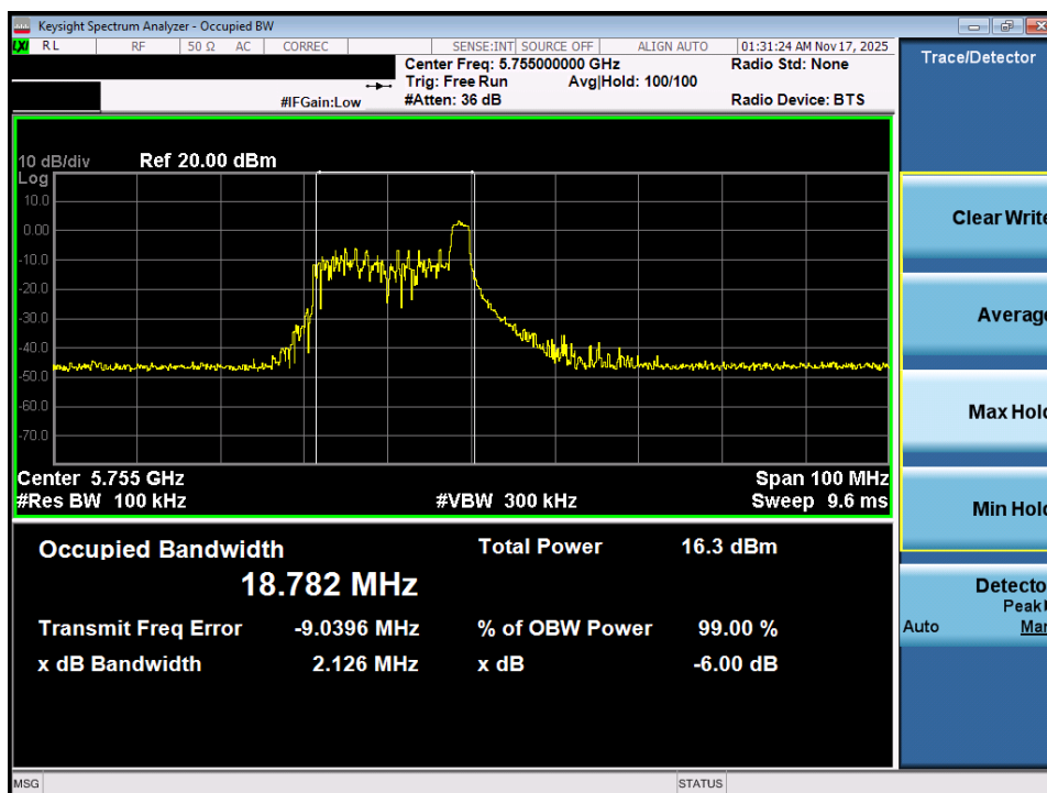
Plot 7-14. 6dB Bandwidth Plot MIMO ANT1 (40MHz BW 802.11ax – 26 Tones (UNII Band 3) – Ch. 151)
