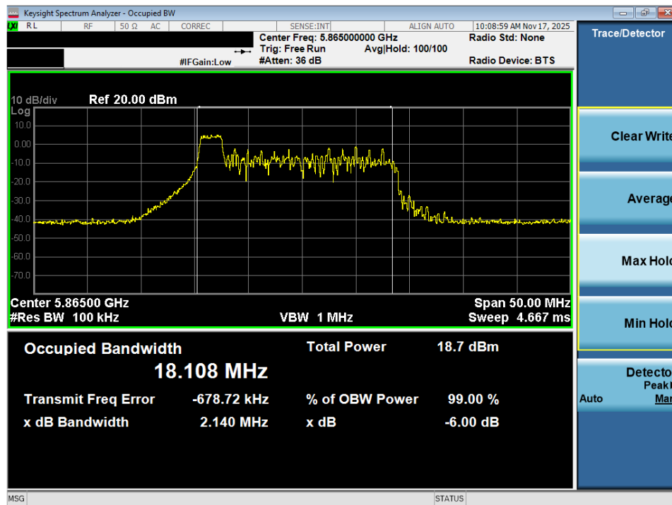
Plot 7-28. 6dB Bandwidth Plot MIMO ANT2 (20MHz BW 802.11ax – 26 Tones (UNII Band 4) – Ch. 173)
