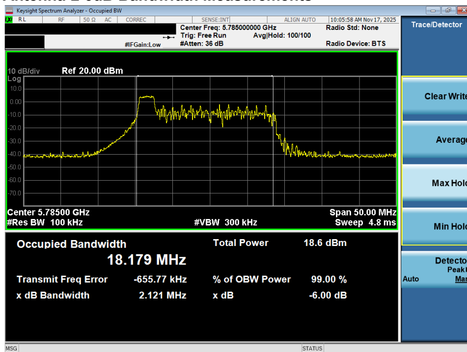
Plot 7-25. 6dB Bandwidth Plot MIMO ANT2 (20MHz BW 802.11ax – 26 Tones (UNII Band 3) – Ch. 157)
