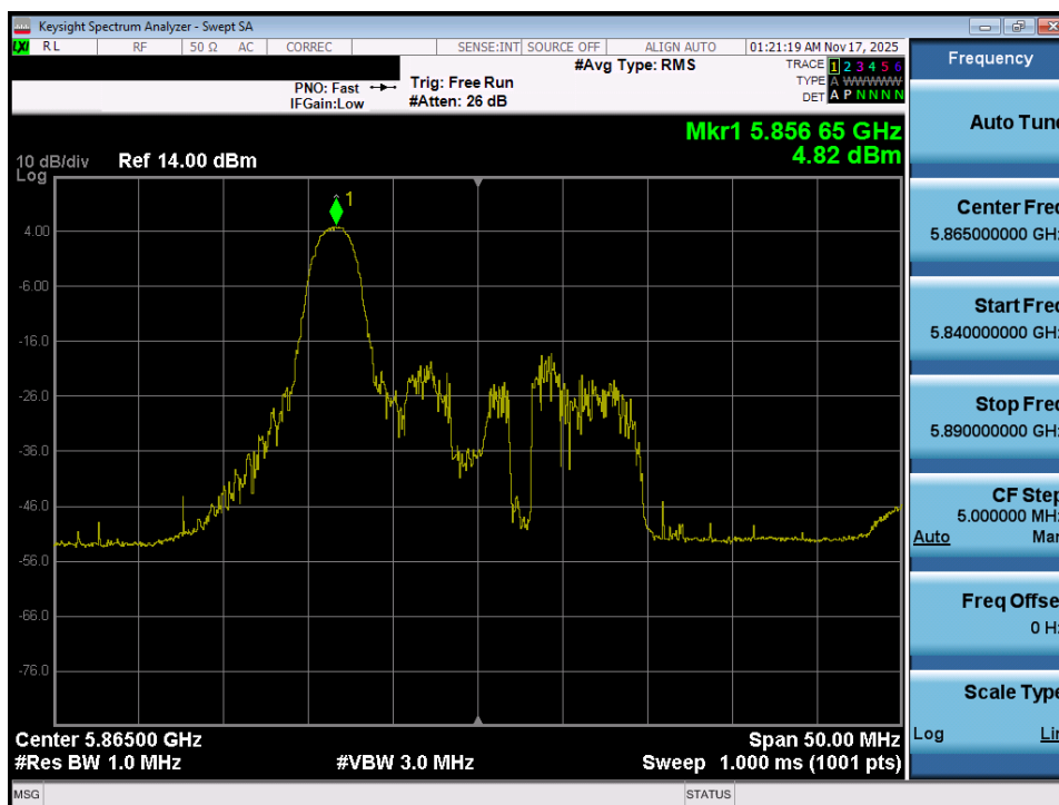
Plot 7-67. Power Spectral Density Plot MIMO ANT1 (20MHz BW 802.11ax – 26 Tones (UNII Band 4) – Ch. 173)
