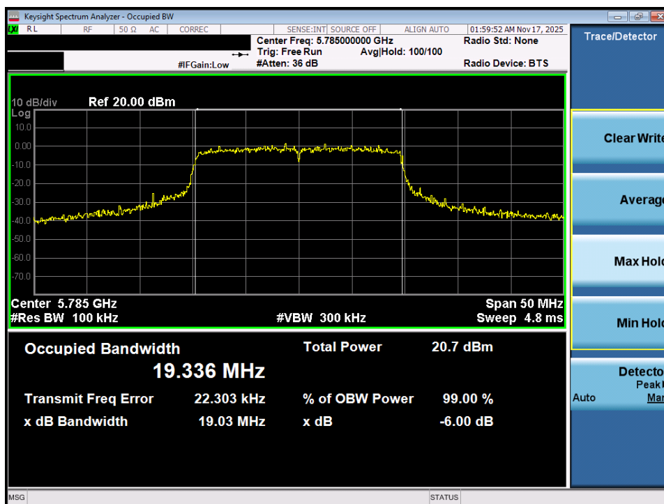
Plot 7-19. 6dB Bandwidth Plot MIMO ANT1 (20MHz BW 802.11ax – 242 Tones (UNII Band 3) – Ch. 157)
