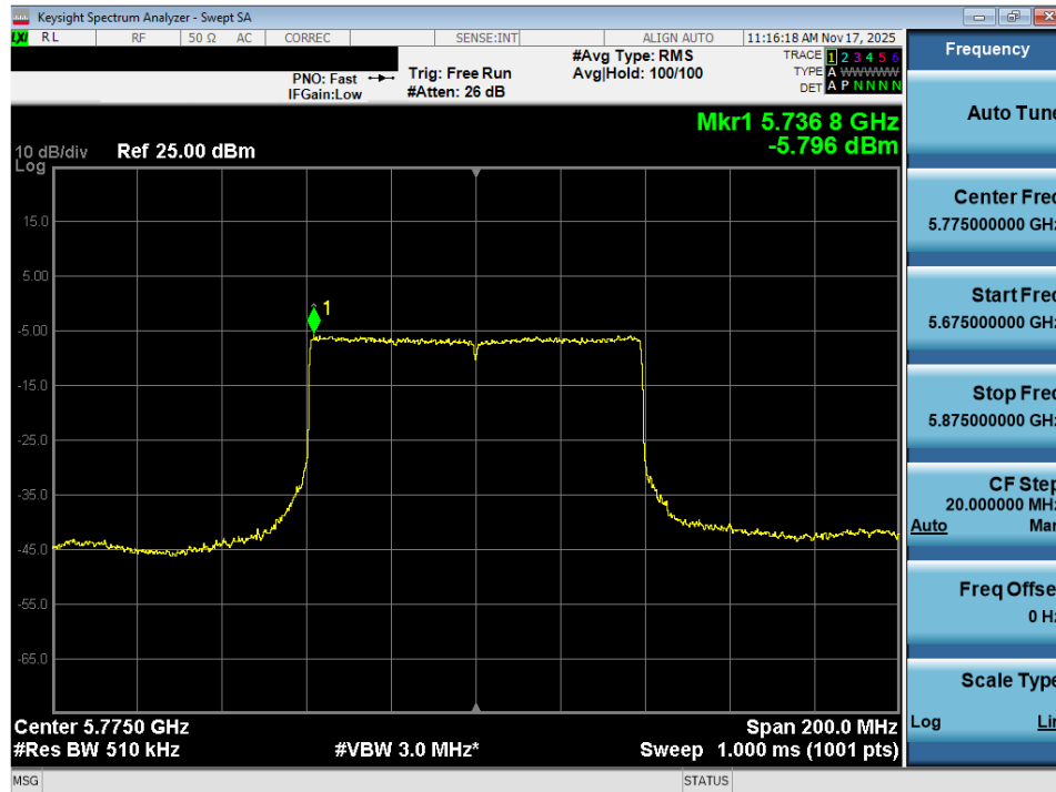
Plot 7-93. Power Spectral Density Plot MIMO ANT2 (80MHz BW 802.11ax – 996 Tones (UNII Band 3) – Ch. 155)
