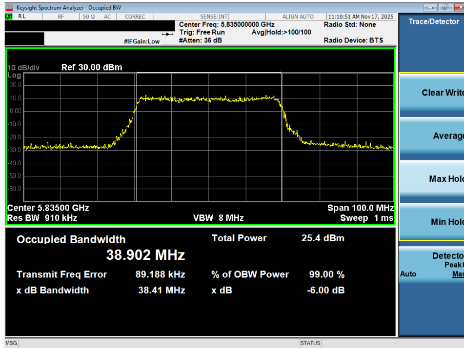
Plot 7-59. OBW Plot MIMO ANT2 (40MHz BW 802.11ax – 484 Tones (UNII Band 3/4) – Ch. 167)
