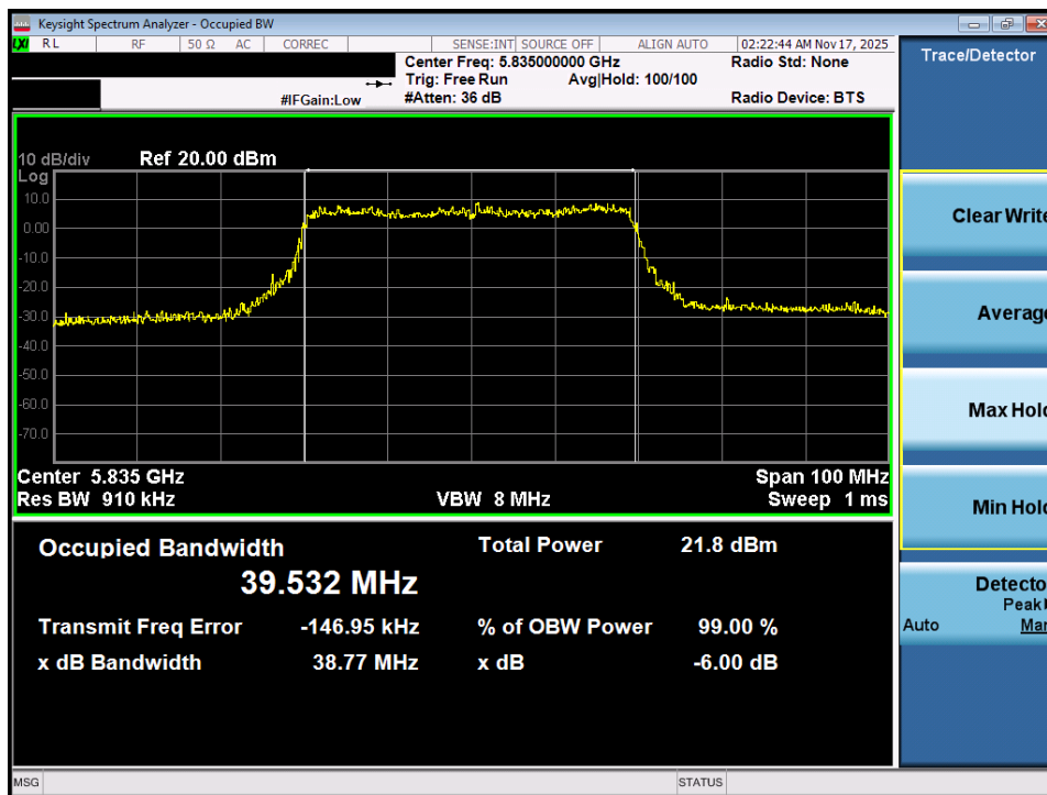
Plot 7-47. OBW Plot MIMO ANT1 (40MHz BW 802.11ax – 484 Tones (UNII Band 3/4) – Ch. 167)
