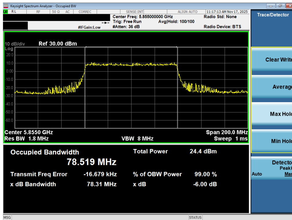
Plot 7-60. OBW Plot MIMO ANT2 (80MHz BW 802.11ax – 996 Tones (UNII Band 3/4) – Ch. 171)
