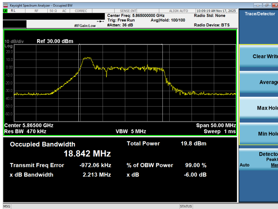
Plot 7-52. OBW Plot MIMO ANT2 (20MHz BW 802.11ax – 26 Tones (UNII Band 4) – Ch. 173)
