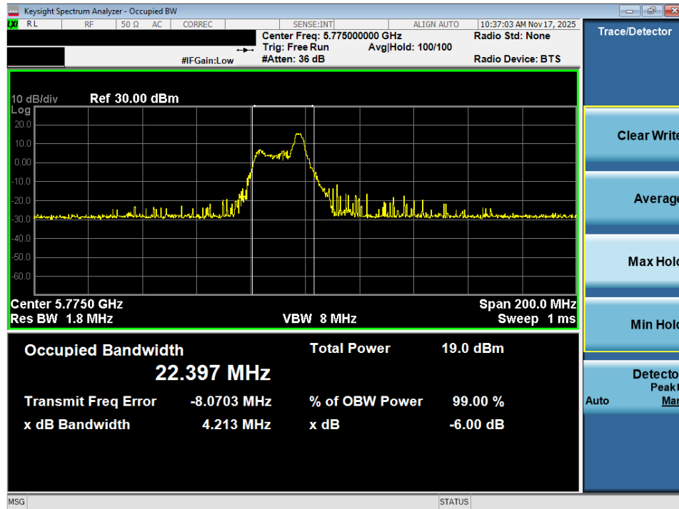
Plot 7-51. OBW Plot MIMO ANT2 (80MHz BW 802.11ax – 26 Tones (UNII Band 3) – Ch. 155)
