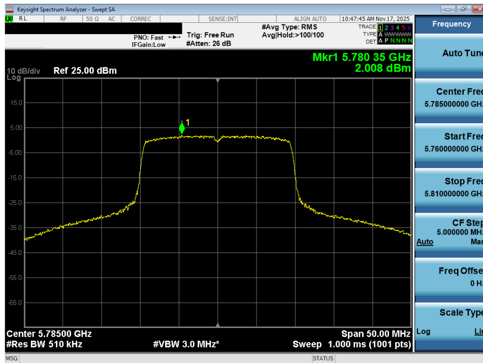
Plot 7-91. Power Spectral Density Plot MIMO ANT2 (20MHz BW 802.11ax – 242 Tones (UNII Band 3) – Ch. 157)
