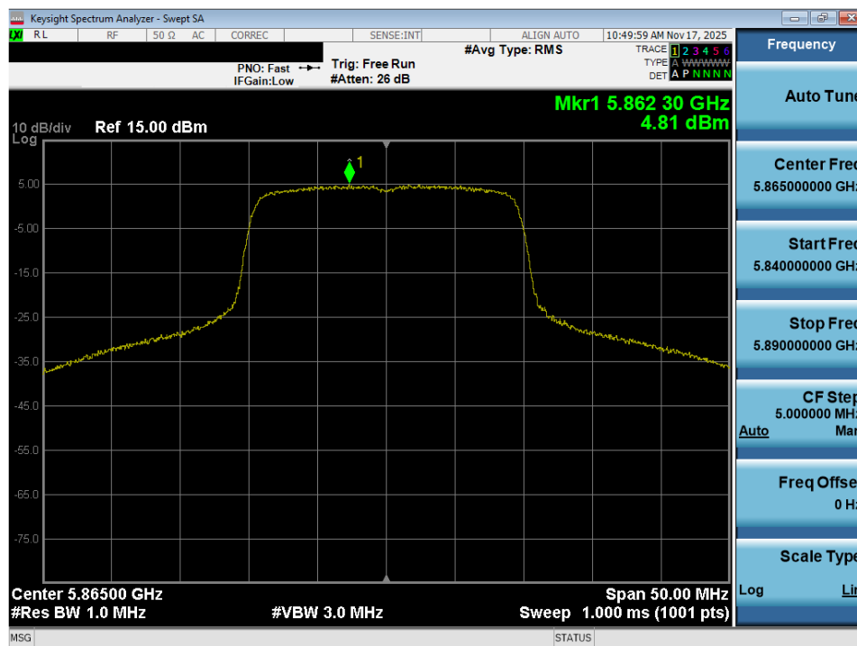
Plot 7-94. Power Spectral Density Plot MIMO ANT2 (20MHz BW 802.11ax – 242 Tones (UNII Band 4) – Ch. 173)
