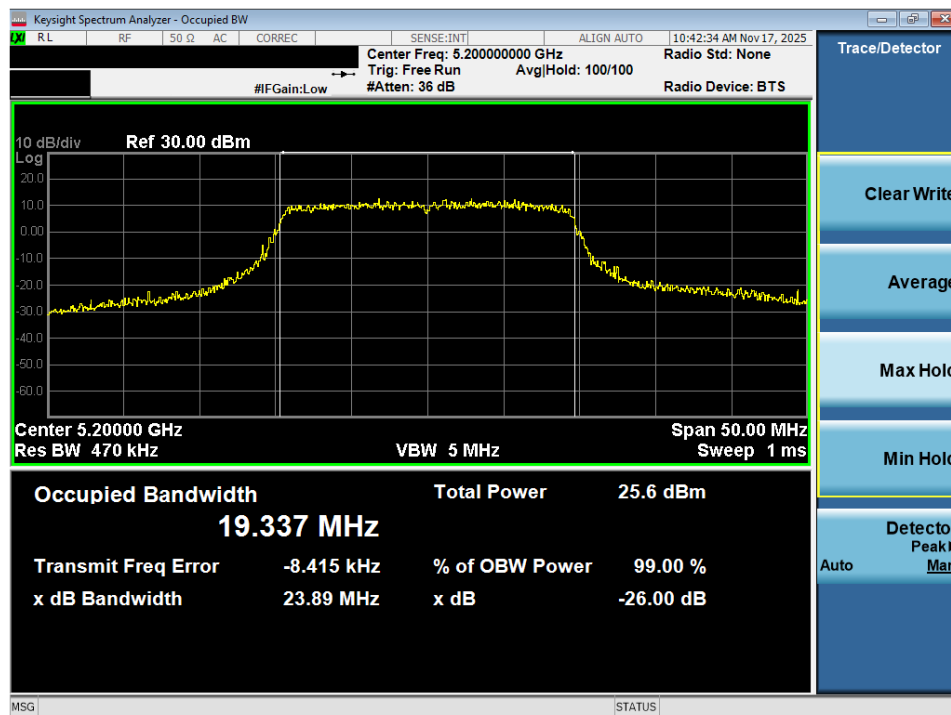
Plot 7-10. 26dB Bandwidth Plot MIMO ANT2 (20MHz BW 802.11ax – 242 Tones (UNII Band 1) – Ch. 40)
