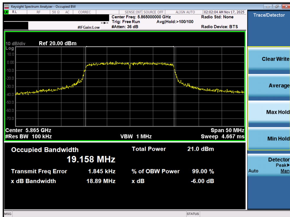
Plot 7-22. 6dB Bandwidth Plot MIMO ANT1 (20MHz BW 802.11ax – 242 Tones (UNII Band 4) – Ch. 173)
