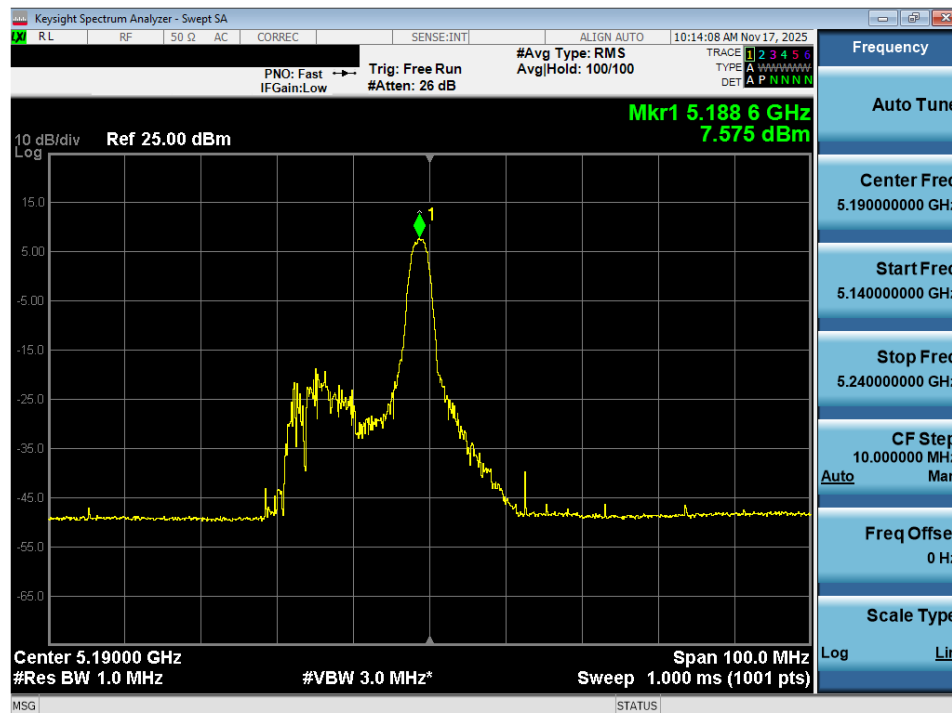
Plot 7-80. Power Spectral Density Plot MIMO ANT2 (40MHz BW 802.11ax – 26 Tones (UNII Band 1) – Ch. 38)
