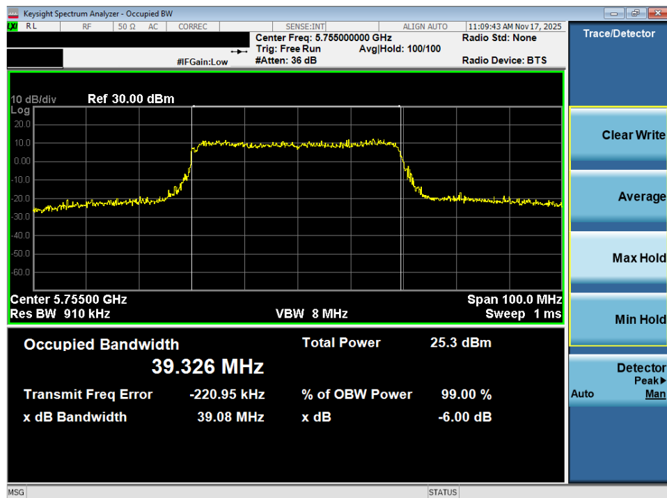
Plot 7-56. OBW Plot MIMO ANT2 (40MHz BW 802.11ax – 484 Tones (UNII Band 3) – Ch. 151)
