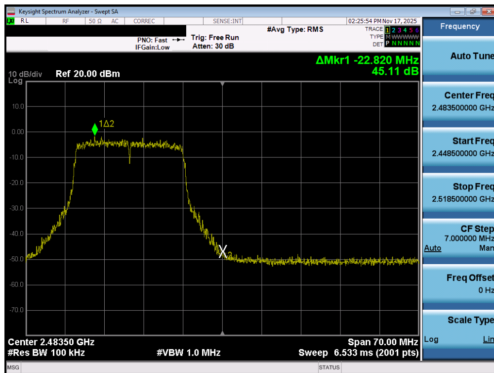
Plot 7-90. Band Edge Plot MIMO ANT1 (802.11ax (2.4GHz) – Ch. 12)
