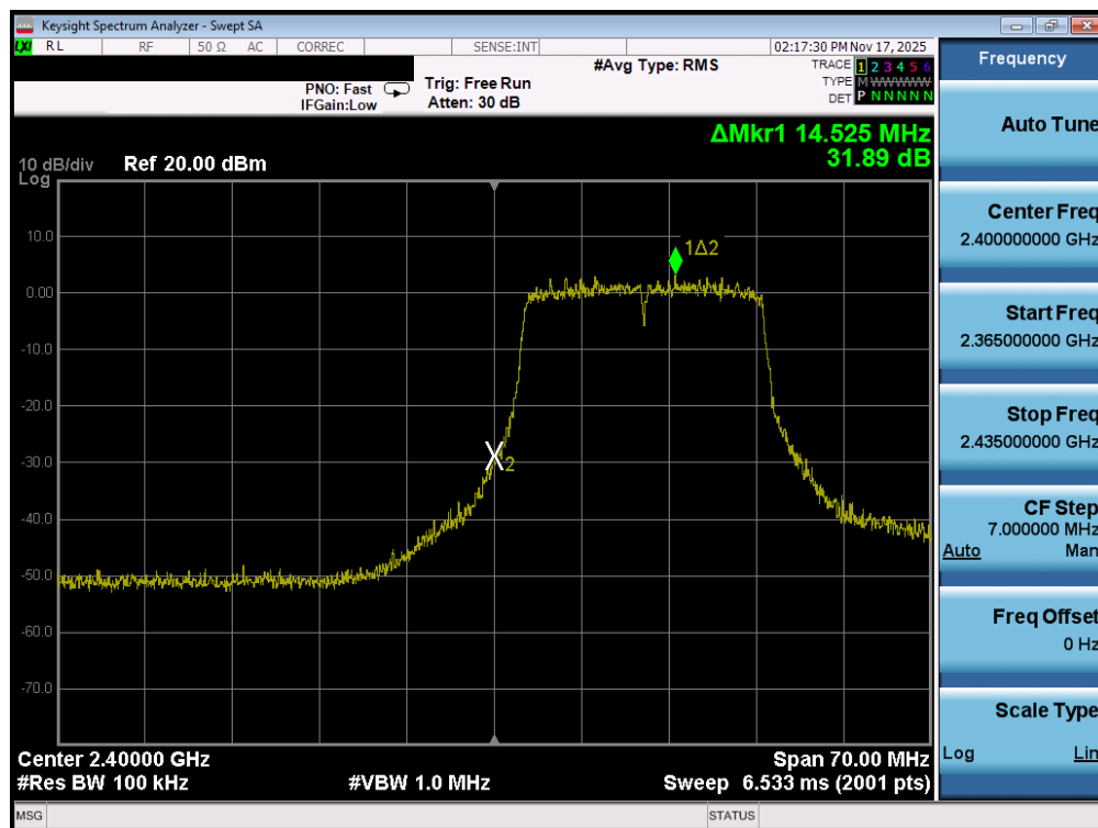
Plot 7-87. Band Edge Plot MIMO ANT1 (802.11ax (2.4GHz) – Ch. 1)
