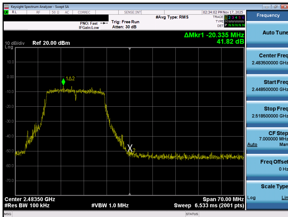
Plot 7-85. Band Edge Plot MIMO ANT1 (802.11n(2.4GHz) – Ch. 12)
