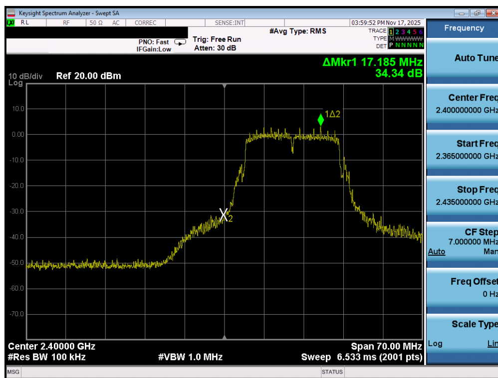
Plot 7-96. Band Edge Plot MIMO ANT2 (802.11g– Ch. 1)
