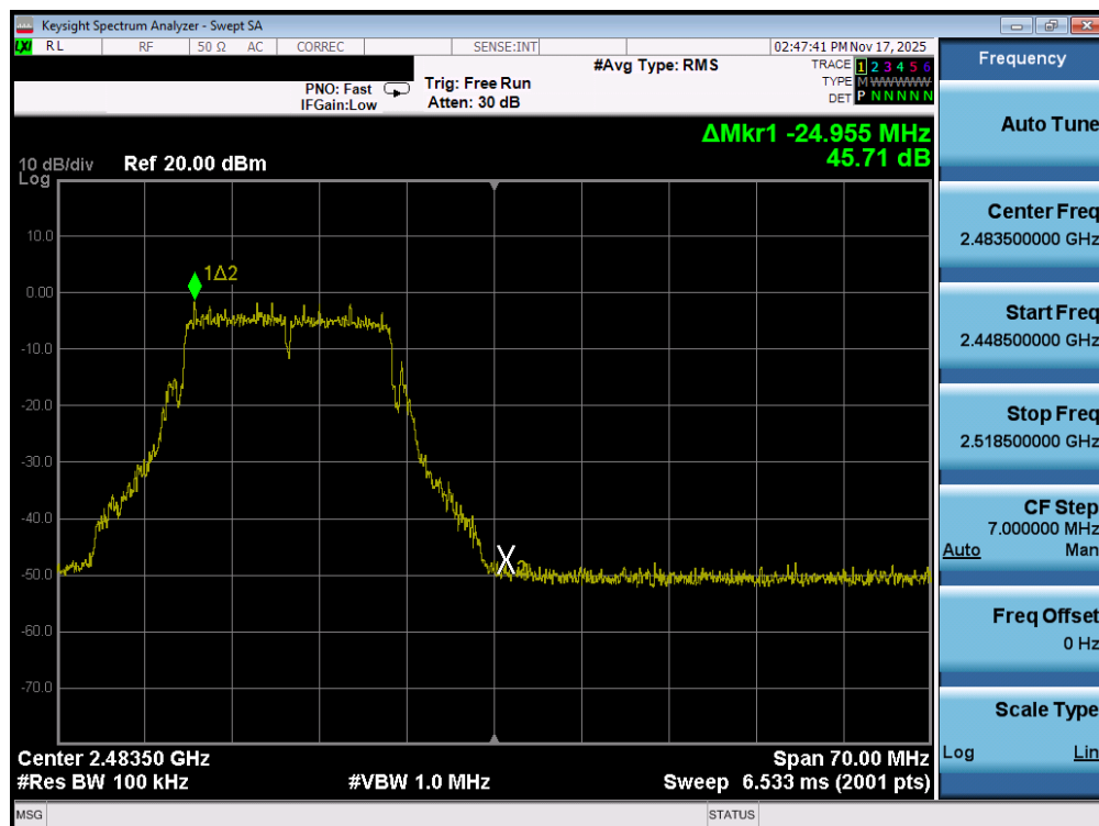
Plot 7-80. Band Edge Plot MIMO ANT1 (802.11g - Ch. 12)
