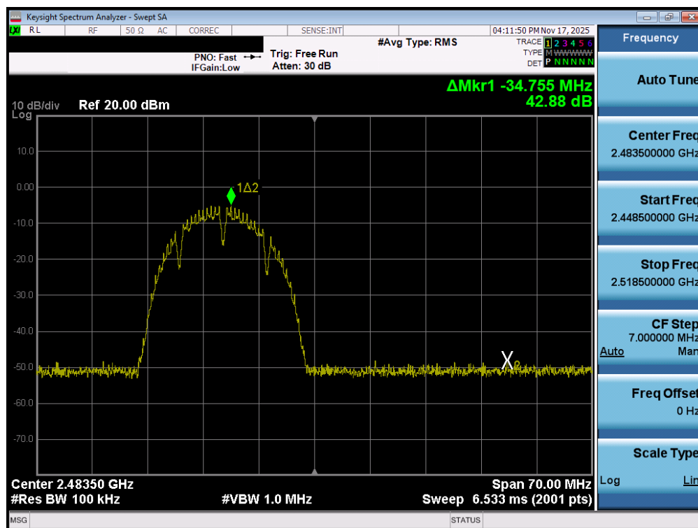
Plot 7-95. Band Edge Plot MIMO ANT2 (802.11b – Ch. 13)
