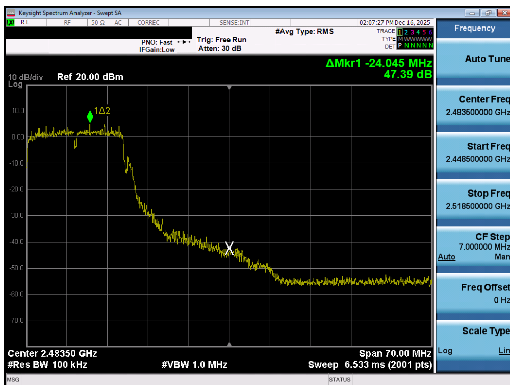
Plot 7-78. Band Edge Plot MIMO ANT1 (802.11g - Ch. 10)
