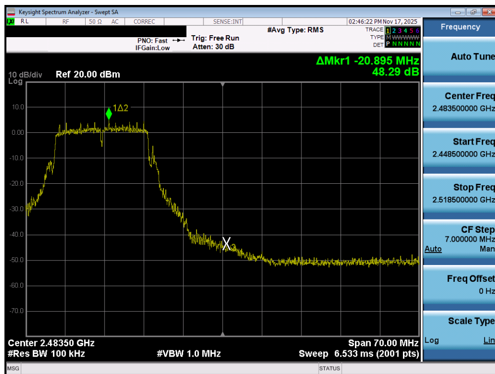
Plot 7-79. Band Edge Plot MIMO ANT1 (802.11g - Ch. 11)
