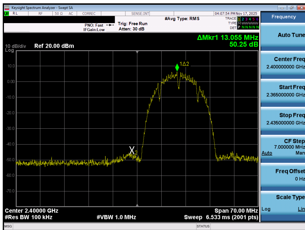
Plot 7-92. Band Edge Plot MIMO ANT2 (802.11b – Ch. 1)
