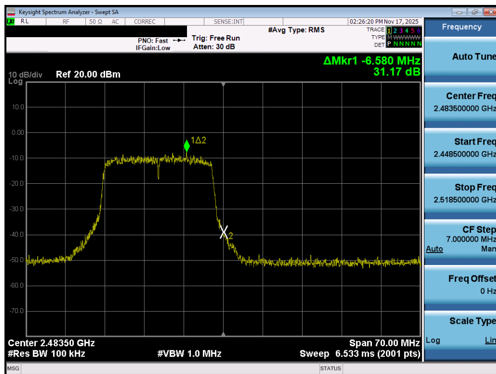
Plot 7-91. Band Edge Plot MIMO ANT1 (802.11ax (2.4GHz) – Ch. 13)
