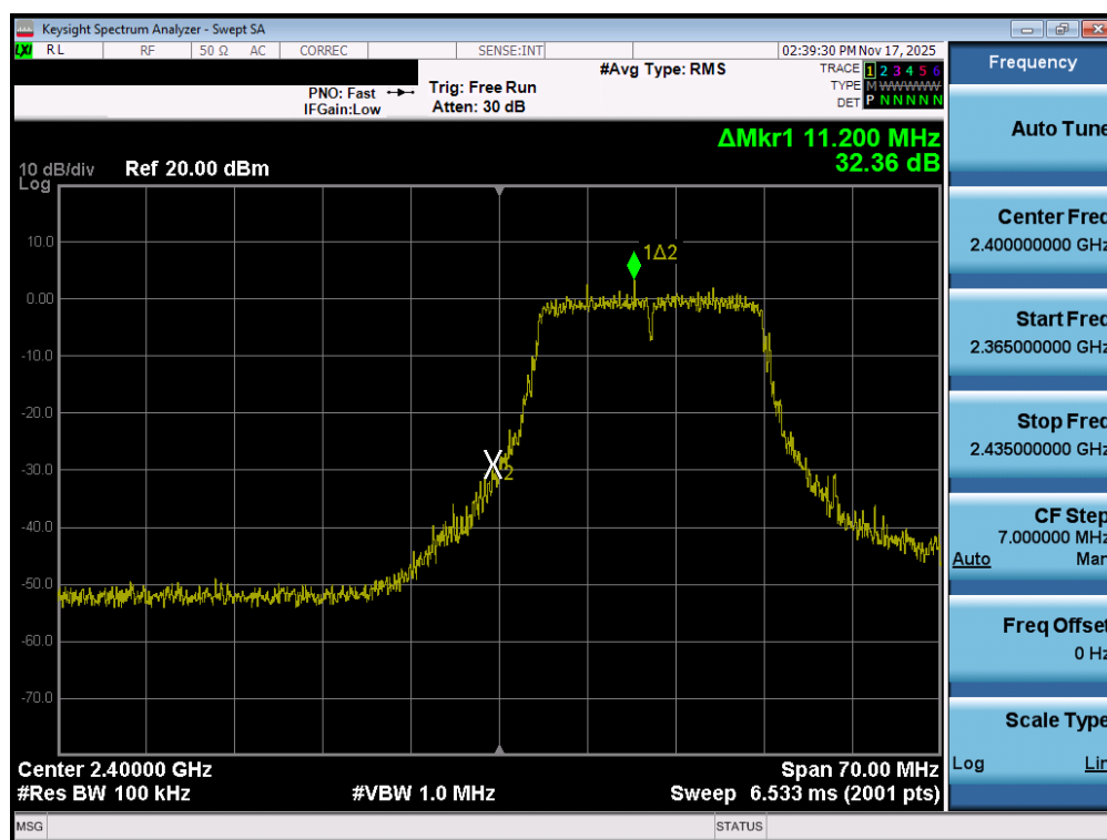
Plot 7-82. Band Edge Plot MIMO ANT1 (802.11n(2.4GHz) – Ch. 1)
