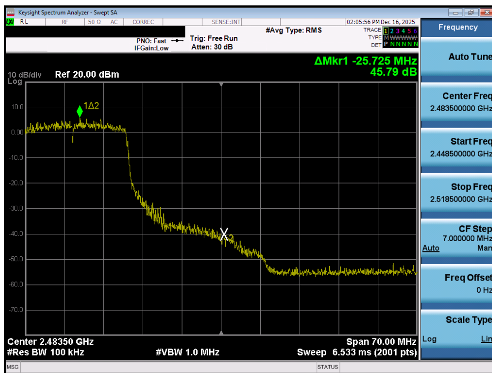
Plot 7-88. Band Edge Plot MIMO ANT1 (802.11ax (2.4GHz) – Ch. 10)
