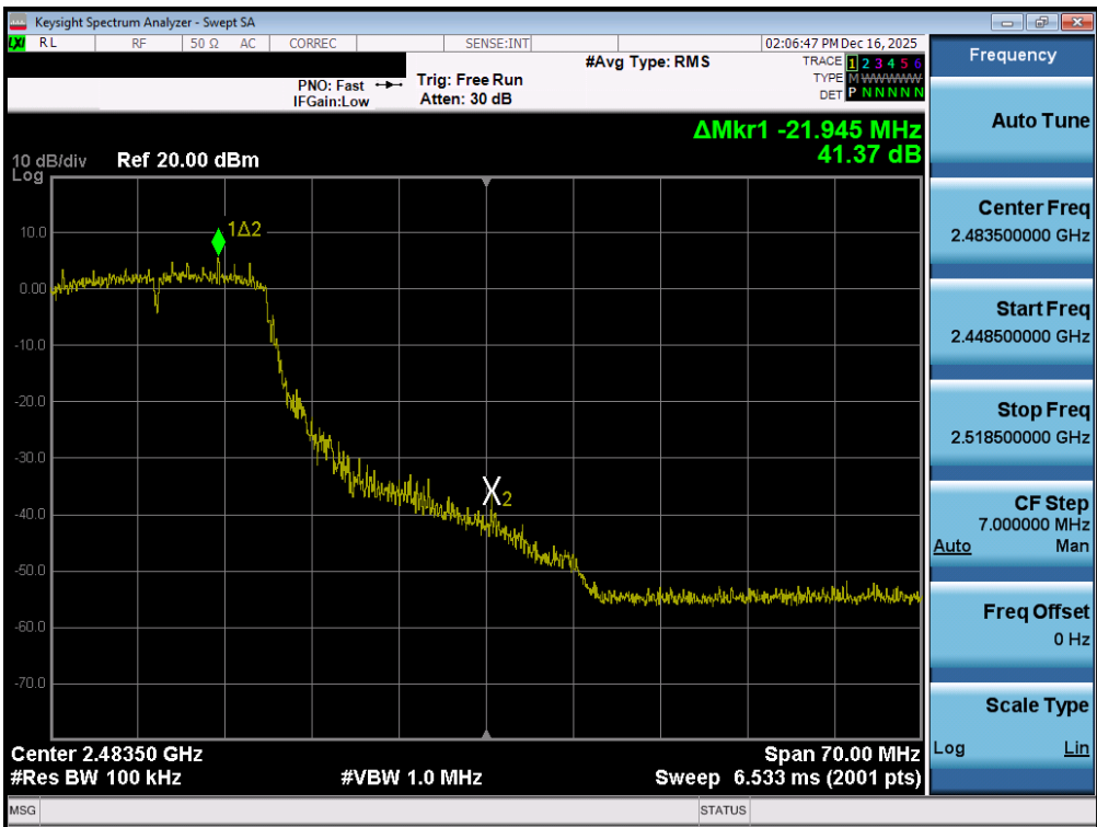
Plot 7-83. Band Edge Plot MIMO ANT1 (802.11n(2.4GHz) – Ch. 10)
