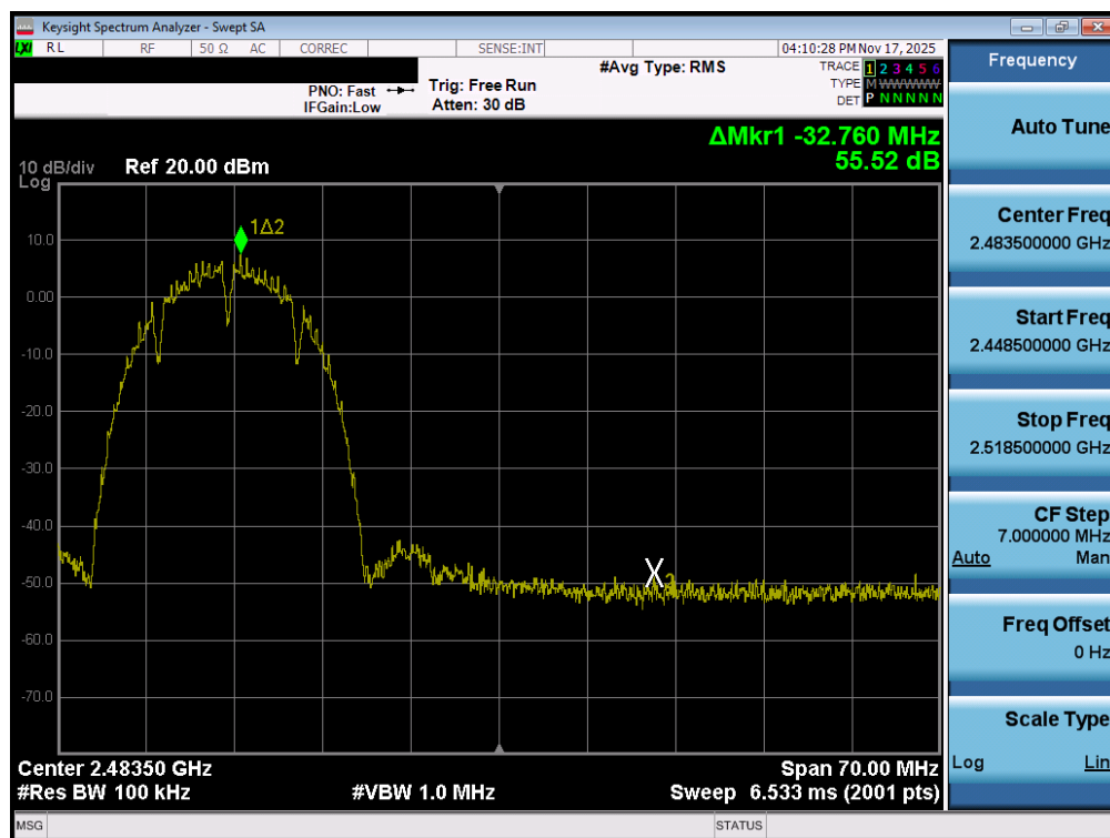
Plot 7-93. Band Edge Plot MIMO ANT2 (802.11b – Ch. 11)
