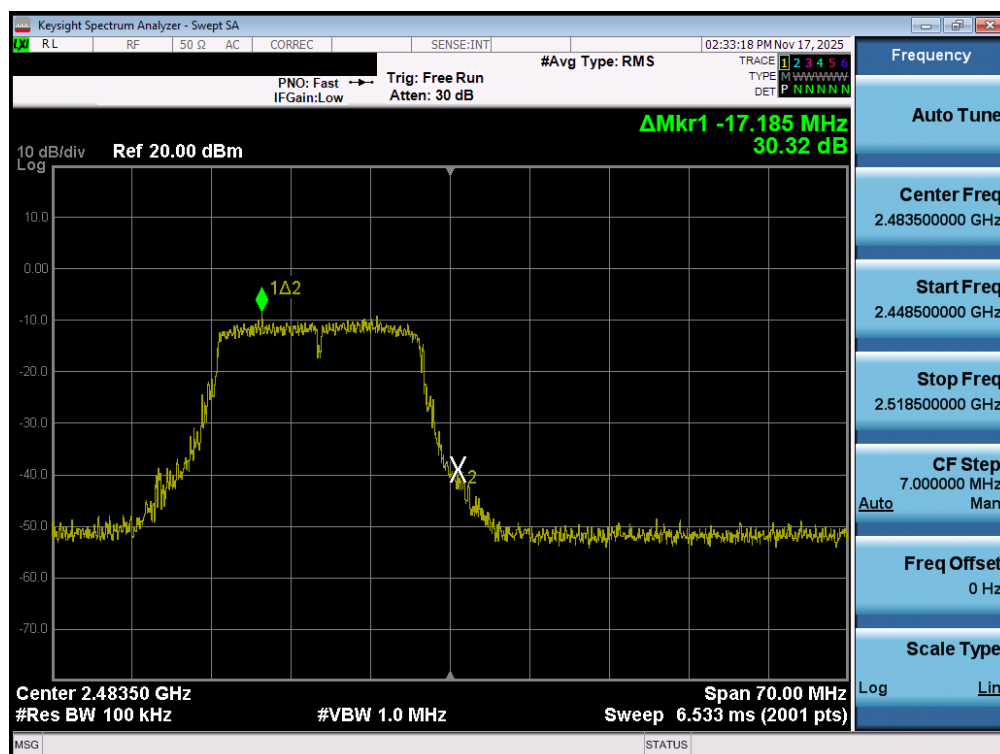
Plot 7-86. Band Edge Plot MIMO ANT1 (802.11n(2.4GHz) – Ch. 13)
