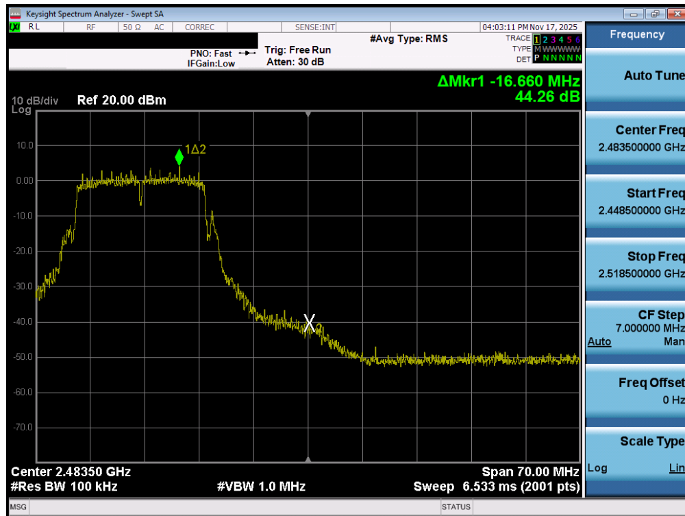
Plot 7-98. Band Edge Plot MIMO ANT2 (802.11g - Ch. 11)
