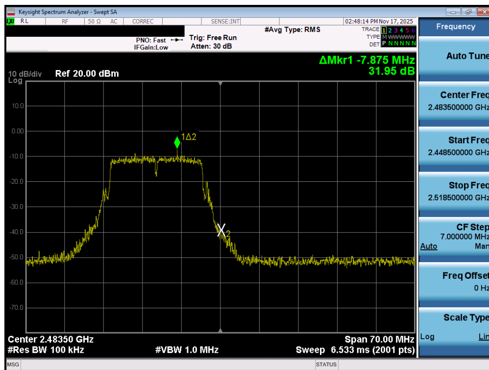
Plot 7-81. Band Edge Plot MIMO ANT1 (802.11g – Ch. 13)
