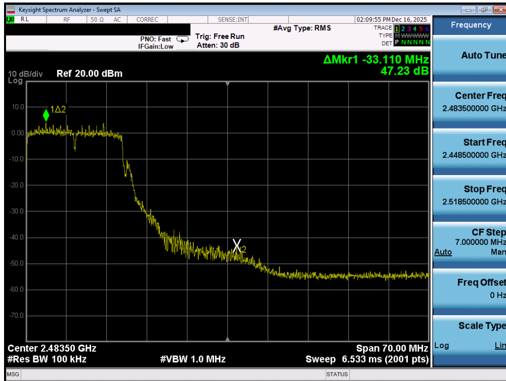
Plot 7-97. Band Edge Plot MIMO ANT2 (802.11g - Ch. 10)
