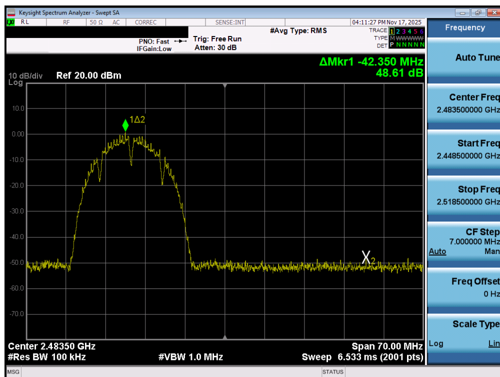
Plot 7-94. Band Edge Plot MIMO ANT2 (802.11b – Ch. 12)
