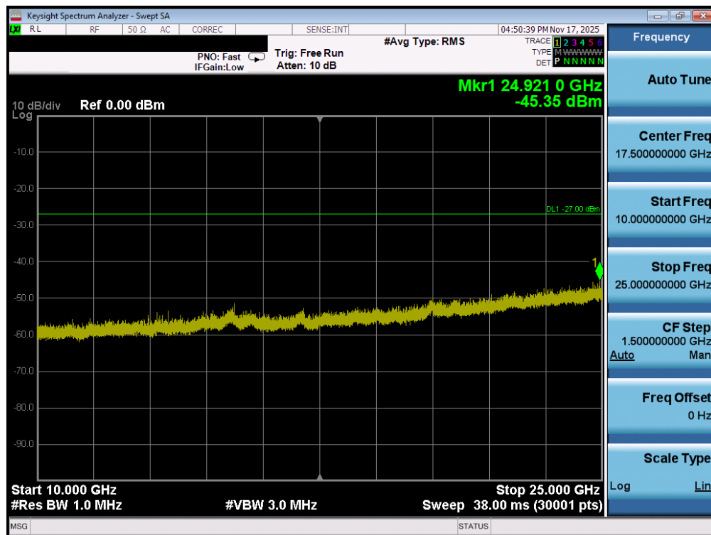
Plot 7-58. Conducted Spurious Plot MIMO ANT1 (802.11ax OFDMA – 26 Tones – Ch. 1)
