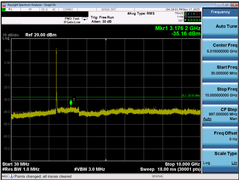
Plot 7-75. Conducted Spurious Plot MIMO ANT2 (802.11ax OFDMA – 242 Tones – Ch. 1)
