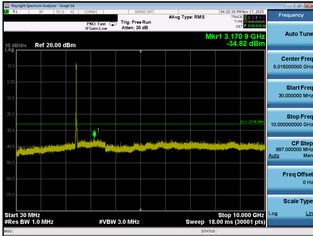
Plot 7-77. Conducted Spurious Plot MIMO ANT2 (802.11ax OFDMA – 242 Tones – Ch. 6)
