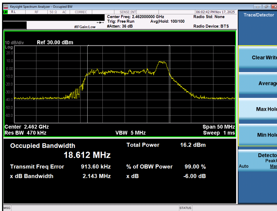
Plot 7-21. OBW Plot MIMO ANT2 (802.11ax OFDMA – 26 Tones – Ch. 11)
