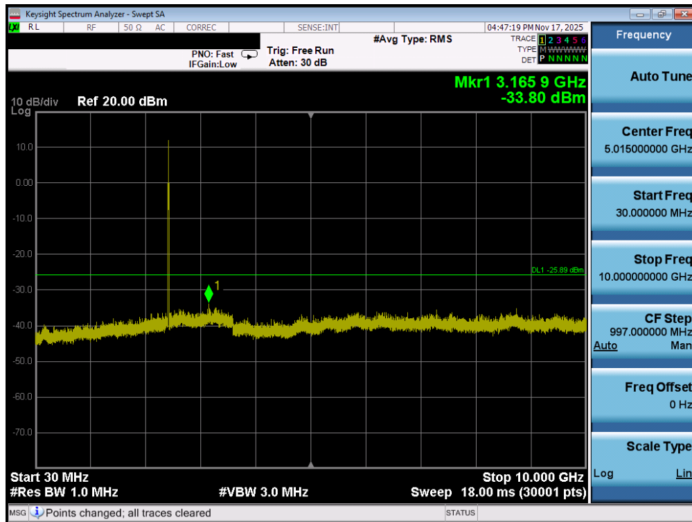
Plot 7-59. Conducted Spurious Plot MIMO ANT1 (802.11ax OFDMA – 26 Tones – Ch. 6)
