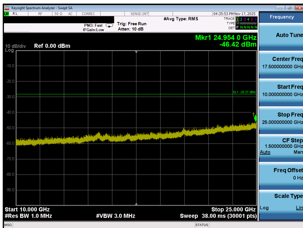
Plot 7-74. Conducted Spurious Plot MIMO ANT2 (802.11ax OFDMA – 26 Tones – Ch. 11)
