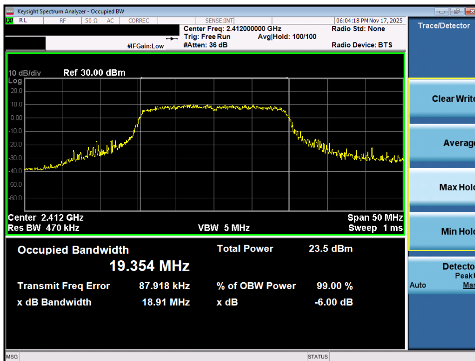
Plot 7-22. OBW Plot MIMO ANT2 (802.11ax OFDMA – 242 Tones – Ch. 1)
