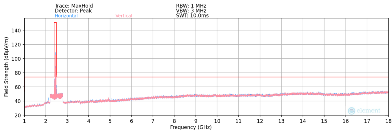
Plot 7-87. Radiated Spurious Plot above 1GHz MIMO (802.11ax OFDMA – 242 Tones – Ch. 11)
