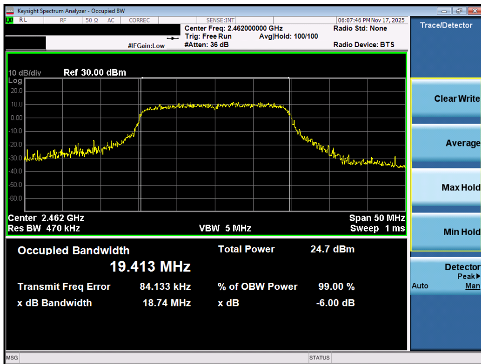
Plot 7-18. OBW Plot MIMO ANT1 (802.11ax OFDMA – 242 Tones – Ch. 11)
