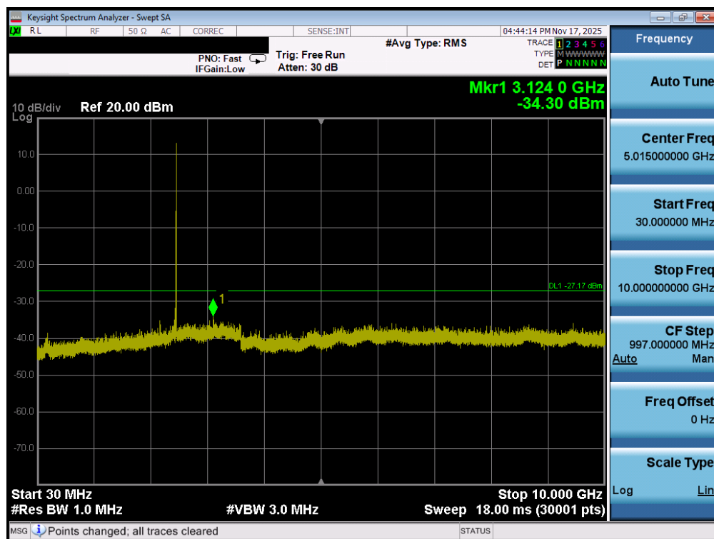
Plot 7-61. Conducted Spurious Plot MIMO ANT1 (802.11ax OFDMA – 26 Tones – Ch. 11)
