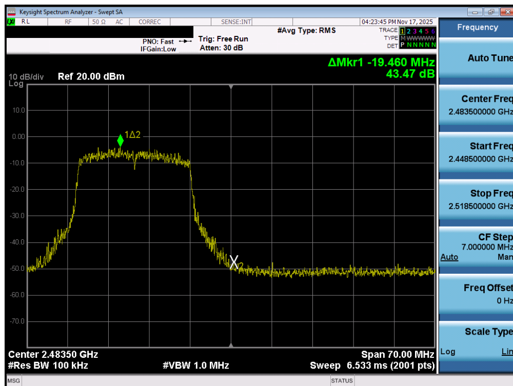
Plot 7-55. Band Edge Plot MIMO ANT2 (802.11ax OFDMA – 242 Tones – Ch. 12)
