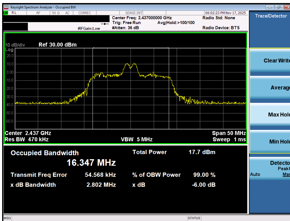
Plot 7-20. OBW Plot MIMO ANT2 (802.11ax OFDMA – 26 Tones – Ch. 6)
