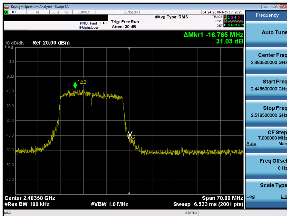
Plot 7-56. Band Edge Plot MIMO ANT2 (802.11ax OFDMA – 242 Tones – Ch. 13)
