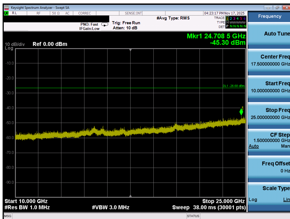
Plot 7-80. Conducted Spurious Plot MIMO ANT2 (802.11ax OFDMA – 242 Tones – Ch. 11)
