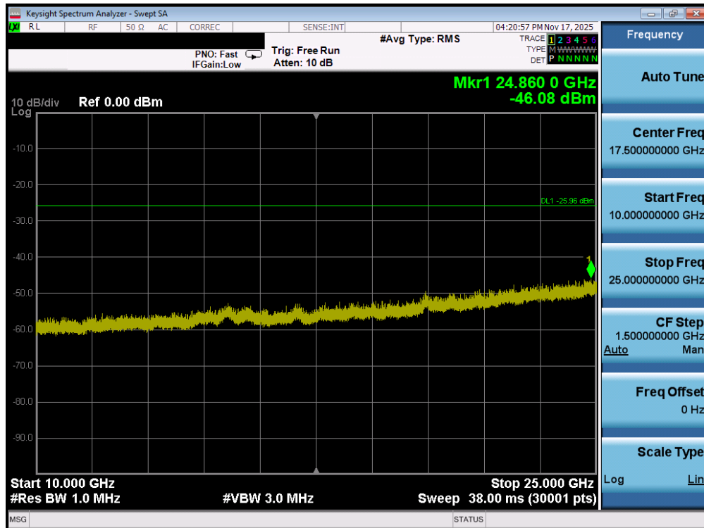
Plot 7-78. Conducted Spurious Plot MIMO ANT2 (802.11ax OFDMA – 242 Tones – Ch. 6)
