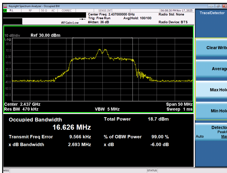
Plot 7-14. OBW Plot MIMO ANT1 (802.11ax OFDMA – 26 Tones – Ch. 6)
