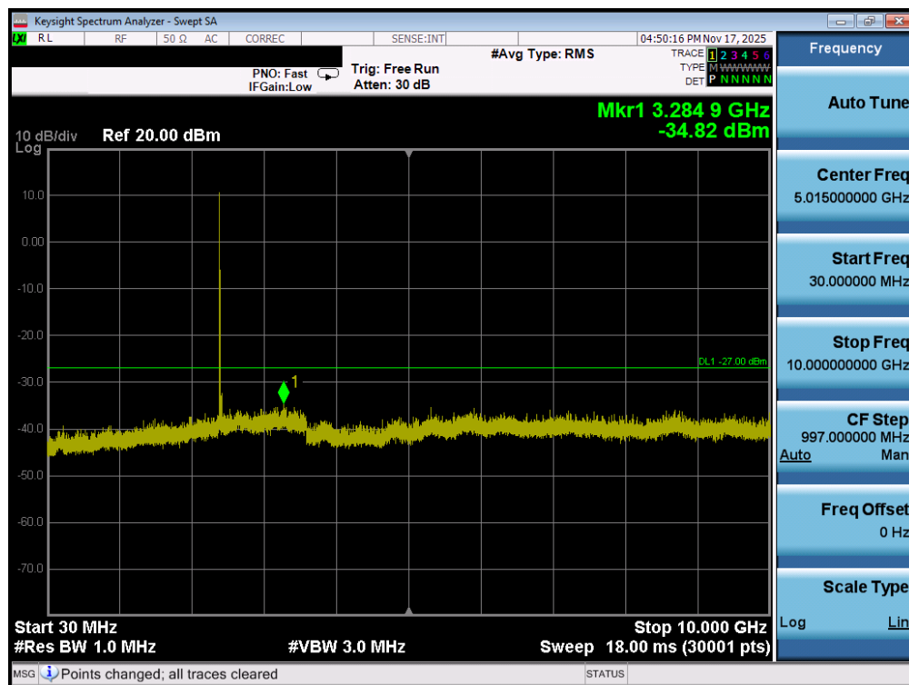
Plot 7-57. Conducted Spurious Plot MIMO ANT1 (802.11ax OFDMA – 26 Tones – Ch. 1)
