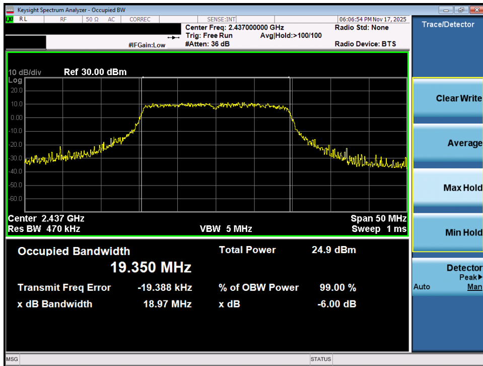
Plot 7-17. OBW Plot MIMO ANT1 (802.11ax OFDMA – 242 Tones – Ch. 6)
