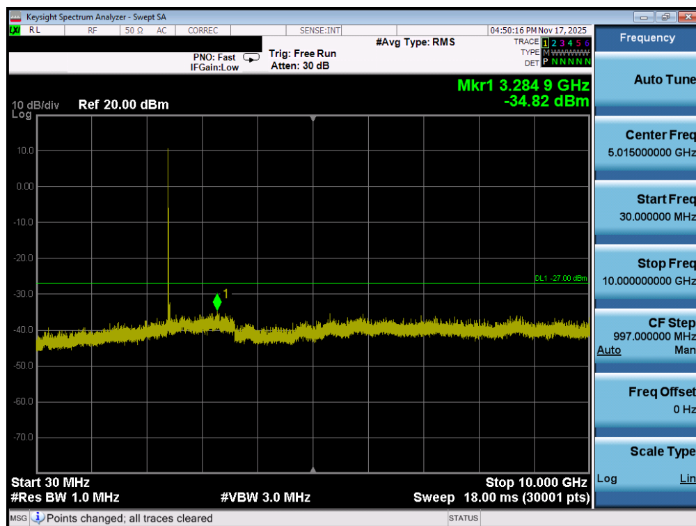
Plot 7-69. Conducted Spurious Plot MIMO ANT1 (802.11ax OFDMA – 26 Tones – Ch. 1)
