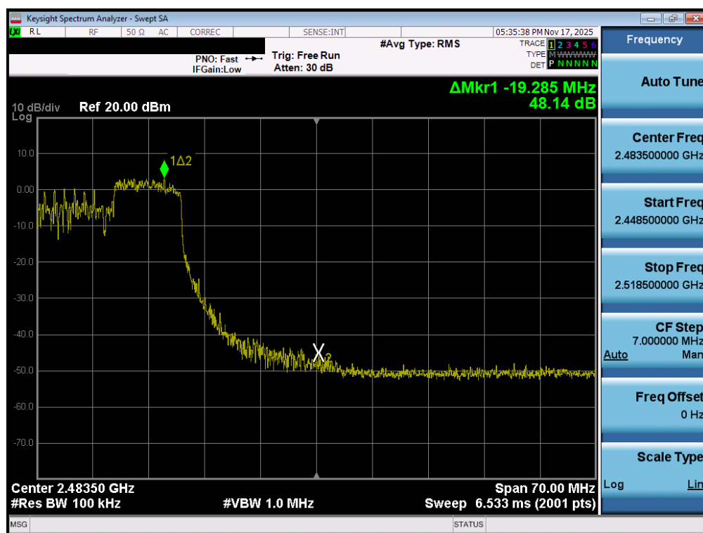
Plot 7-48. Band Edge Plot MIMO ANT2 (802.11ax OFDMA – 106 Tones – Ch. 10)
