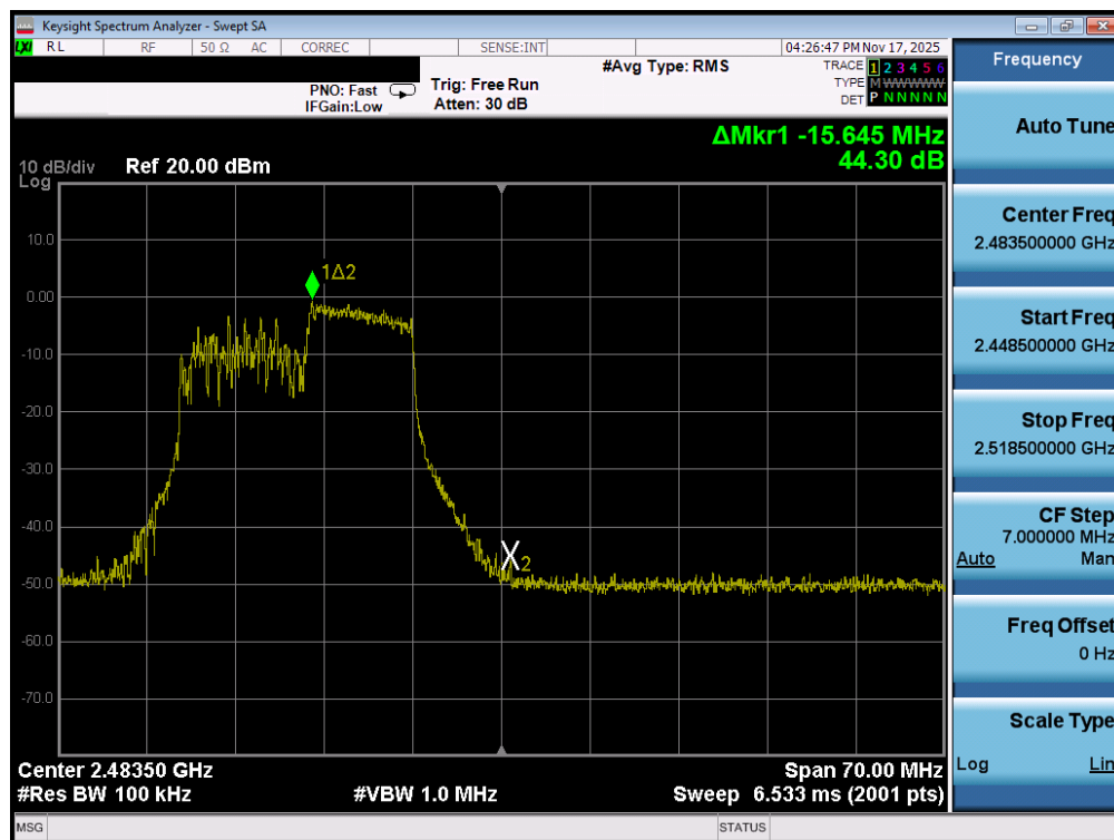
Plot 7-50. Band Edge Plot MIMO ANT2 (802.11ax OFDMA – 106 Tones – Ch. 12)
