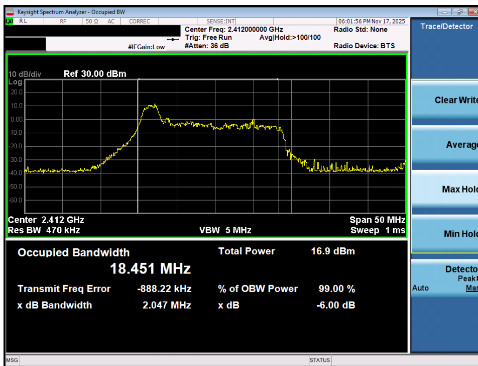
Plot 7-19. OBW Plot MIMO ANT2 (802.11ax OFDMA – 26 Tones – Ch. 1)
