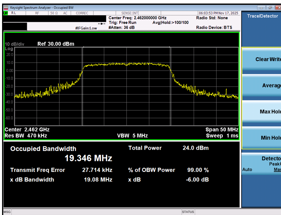
Plot 7-24. OBW Plot MIMO ANT2 (802.11ax OFDMA – 242 Tones – Ch. 11)
