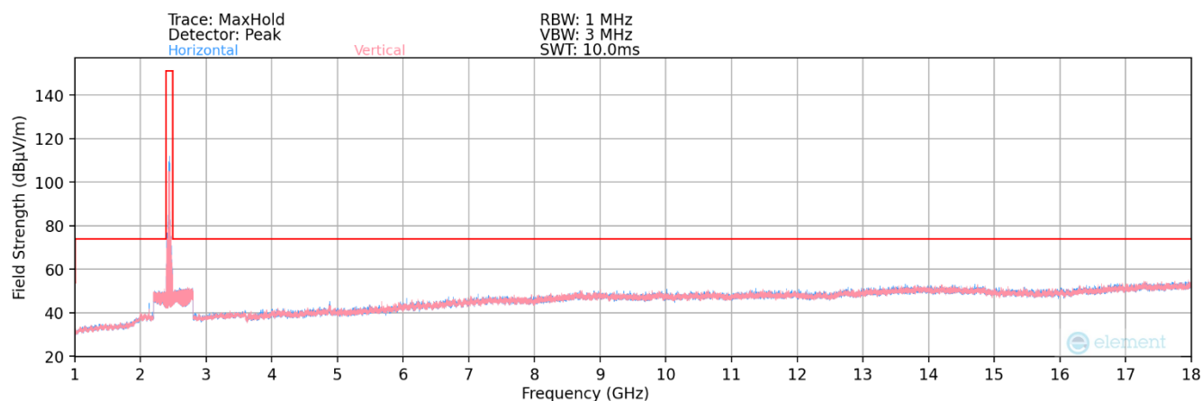
Plot 7-86. Radiated Spurious Plot above 1GHz MIMO (802.11ax OFDMA – 242 Tones – Ch. 6)
