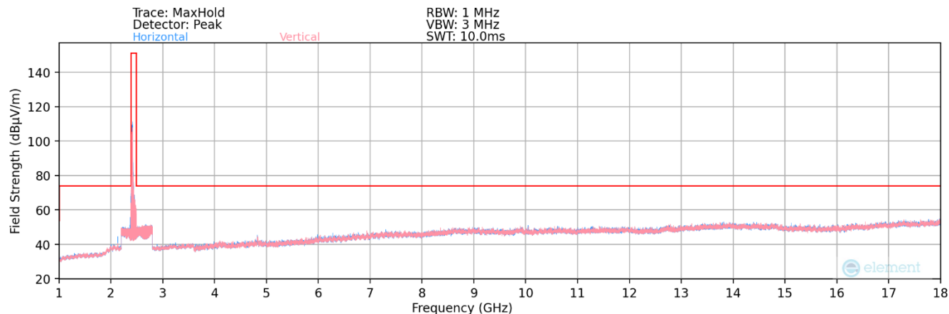
Plot 7-85. Radiated Spurious Plot above 1GHz MIMO (802.11ax OFDMA – 242 Tones – Ch. 1)
