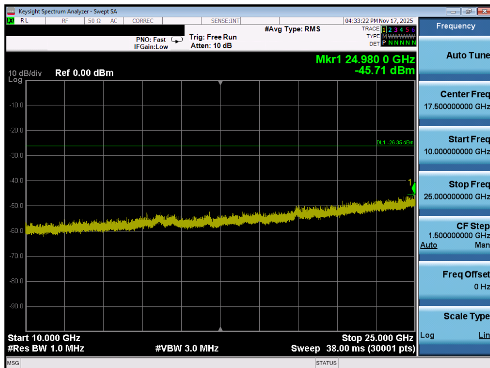
Plot 7-72. Conducted Spurious Plot MIMO ANT2 (802.11ax OFDMA – 26 Tones – Ch. 6)
