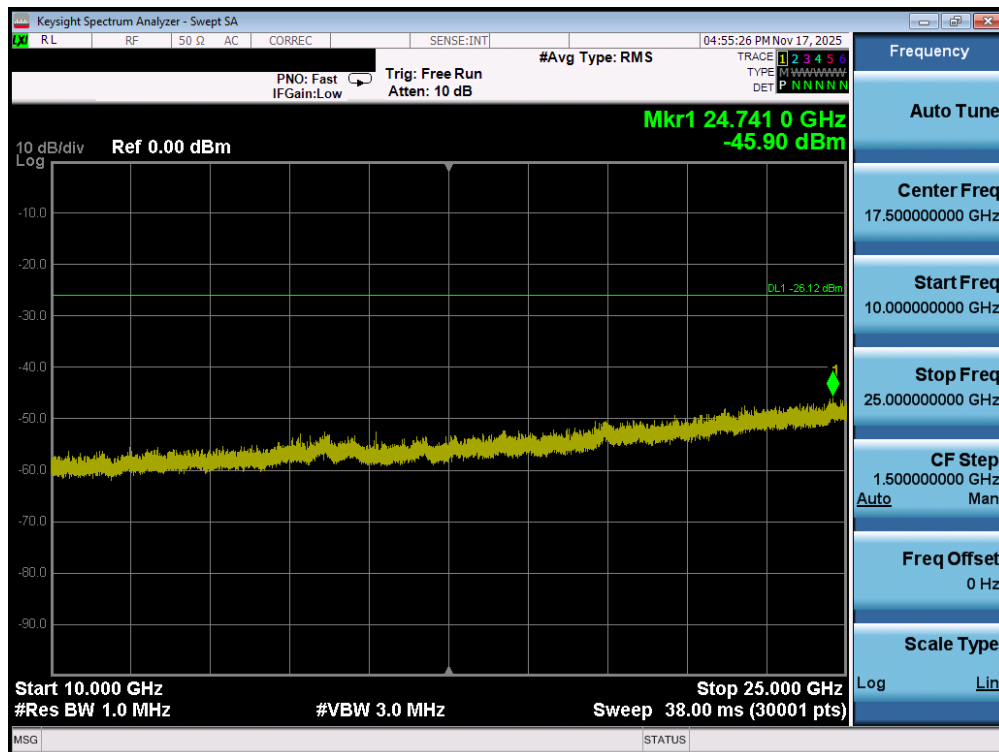
Plot 7-66. Conducted Spurious Plot MIMO ANT1 (802.11ax OFDMA – 242 Tones – Ch. 6)
