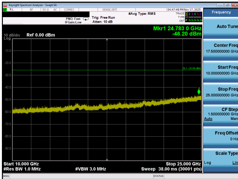
Plot 7-60. Conducted Spurious Plot MIMO ANT1 (802.11ax OFDMA – 26 Tones – Ch. 6)
