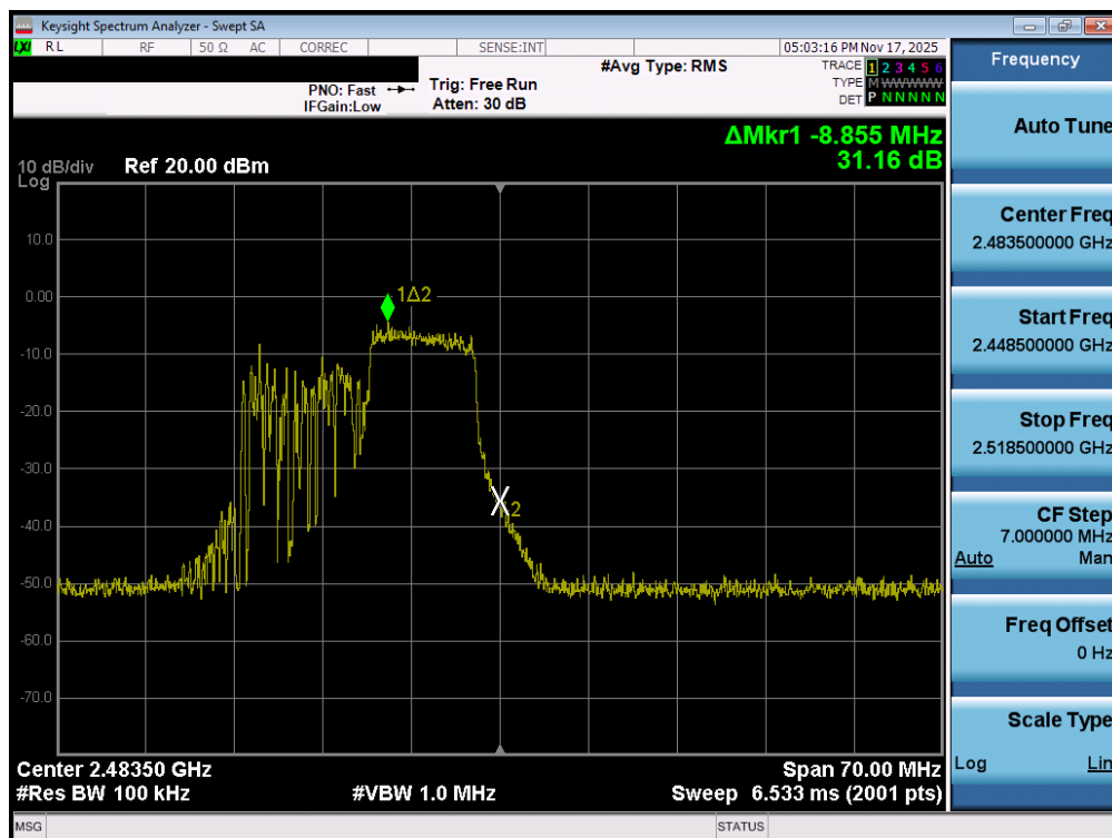
Plot 7-41. Band Edge Plot MIMO ANT1 (802.11ax OFDMA – 106 Tones – Ch. 13)
