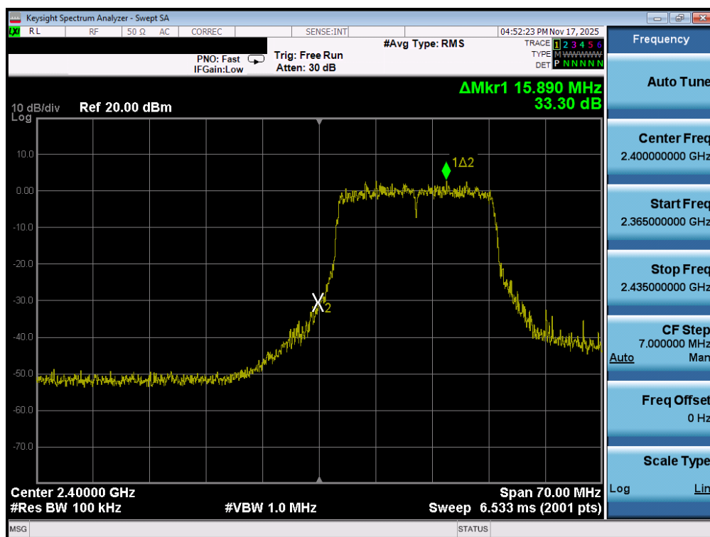
Plot 7-42. Band Edge Plot MIMO ANT1 (802.11ax OFDMA – 242 Tones – Ch. 1)
