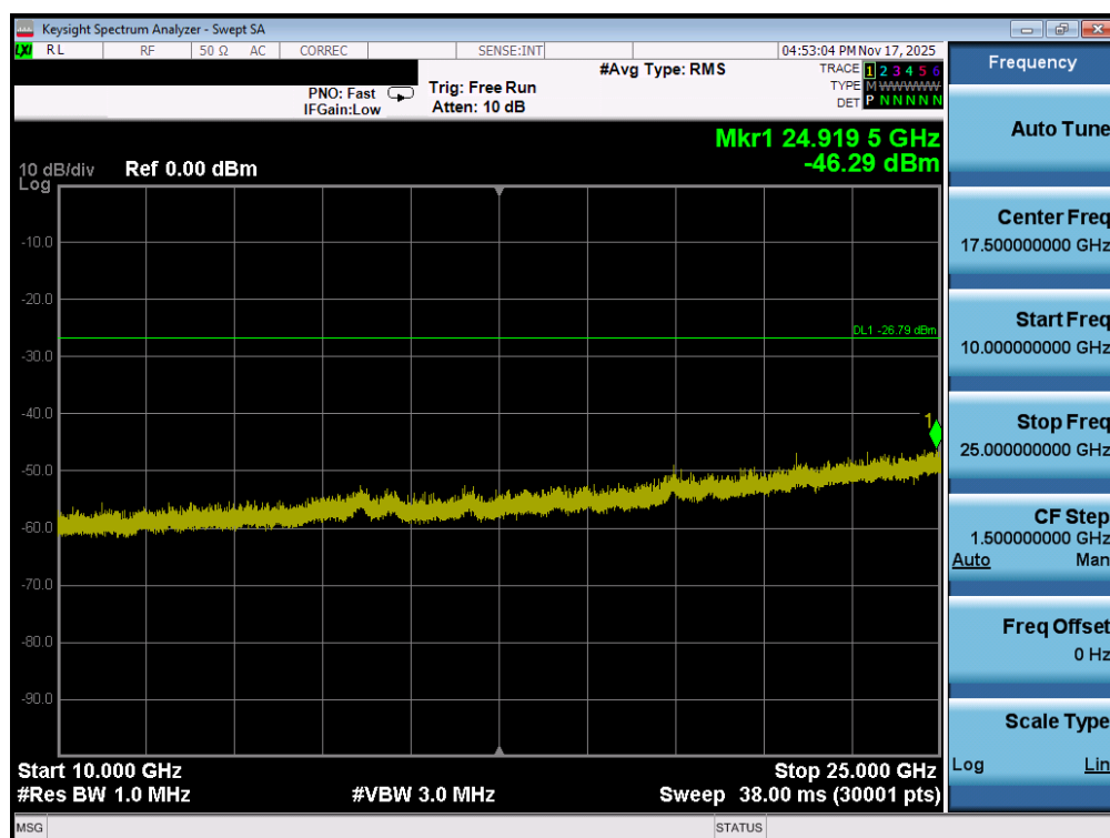
Plot 7-64. Conducted Spurious Plot MIMO ANT1 (802.11ax OFDMA – 242 Tones – Ch. 1)
