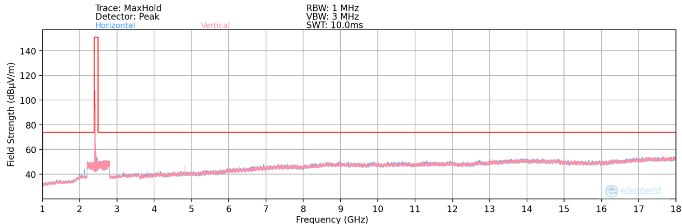
Plot 7-81. Radiated Spurious Plot above 1GHz MIMO (802.11ax OFDMA – 26 Tones – Ch. 1)
