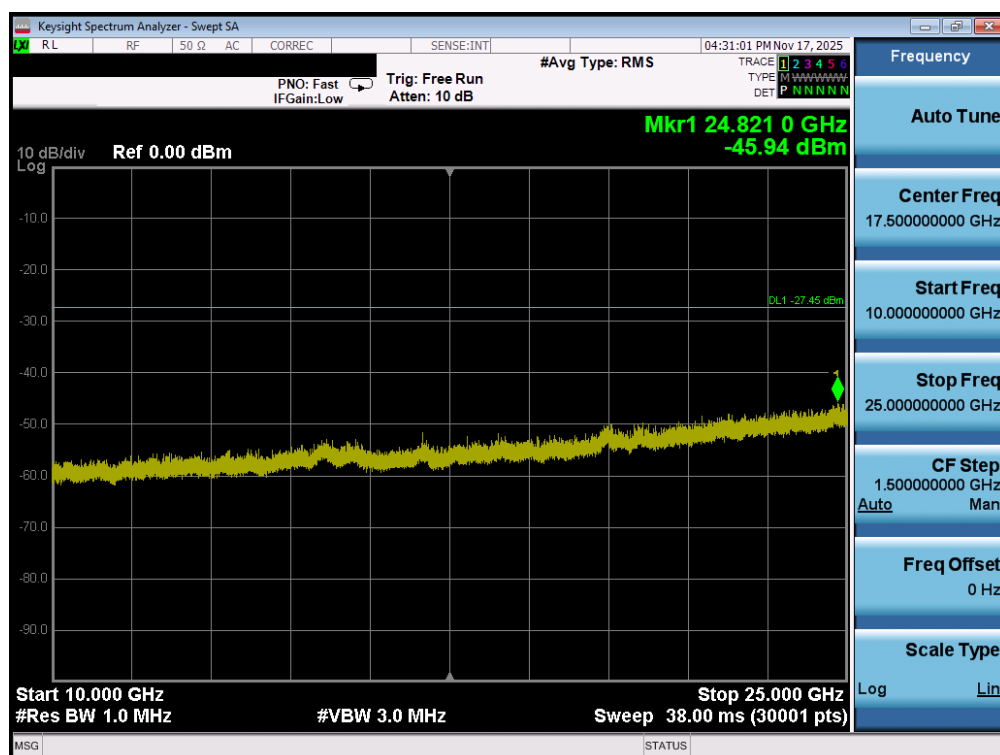
Plot 7-70. Conducted Spurious Plot MIMO ANT2 (802.11ax OFDMA – 26 Tones – Ch. 1)
