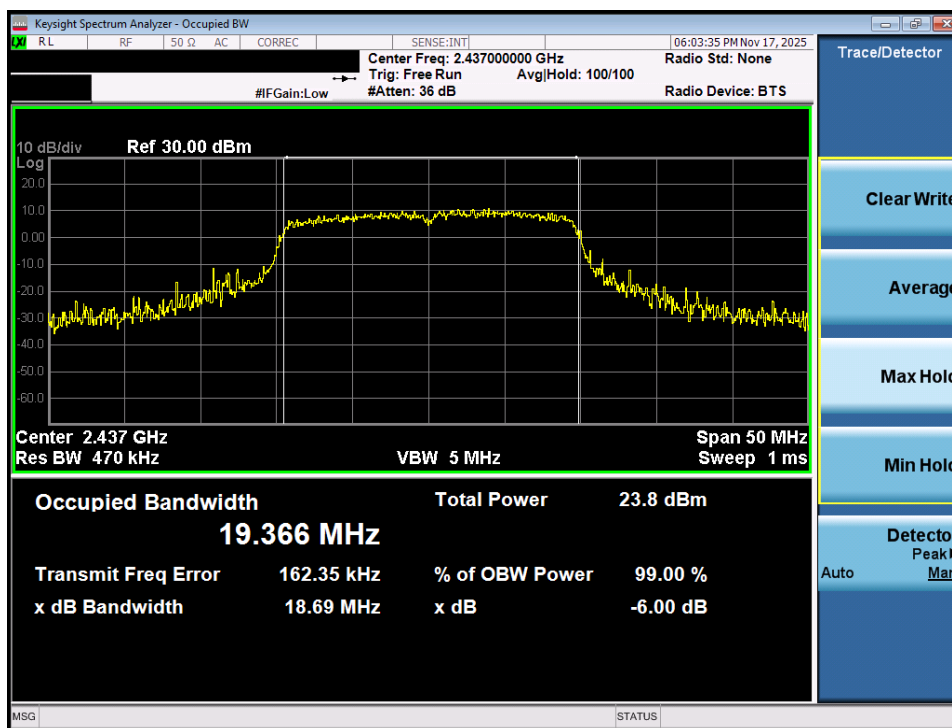
Plot 7-23. OBW Plot MIMO ANT2 (802.11ax OFDMA – 242 Tones – Ch. 6)
