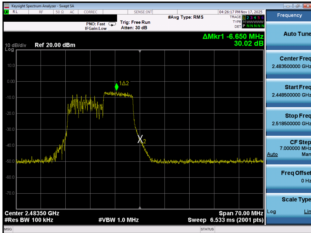
Plot 7-51. Band Edge Plot MIMO ANT2 (802.11ax OFDMA – 106 Tones – Ch. 13)
