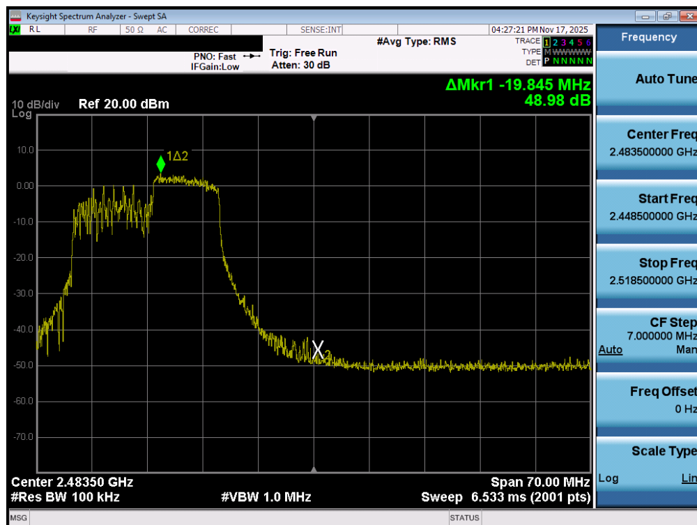
Plot 7-49. Band Edge Plot MIMO ANT2 (802.11ax OFDMA – 106 Tones – Ch. 11)
