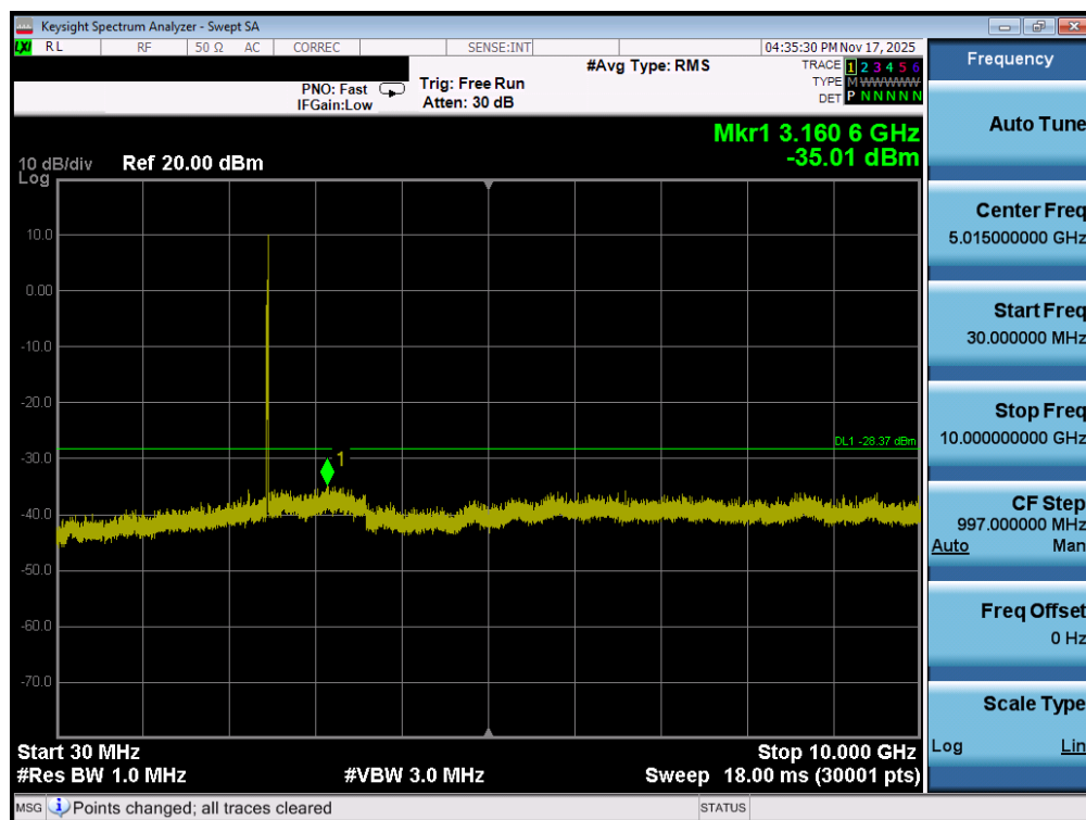
Plot 7-73. Conducted Spurious Plot MIMO ANT2 (802.11ax OFDMA – 26 Tones – Ch. 11)
