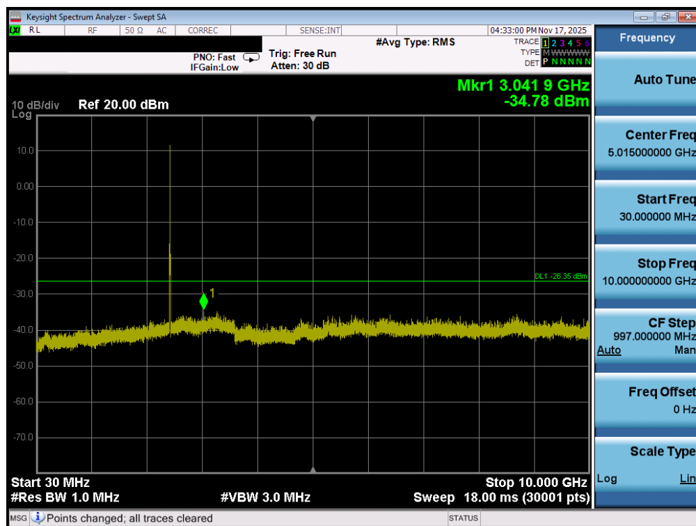
Plot 7-71. Conducted Spurious Plot MIMO ANT2 (802.11ax OFDMA – 26 Tones – Ch. 6)
