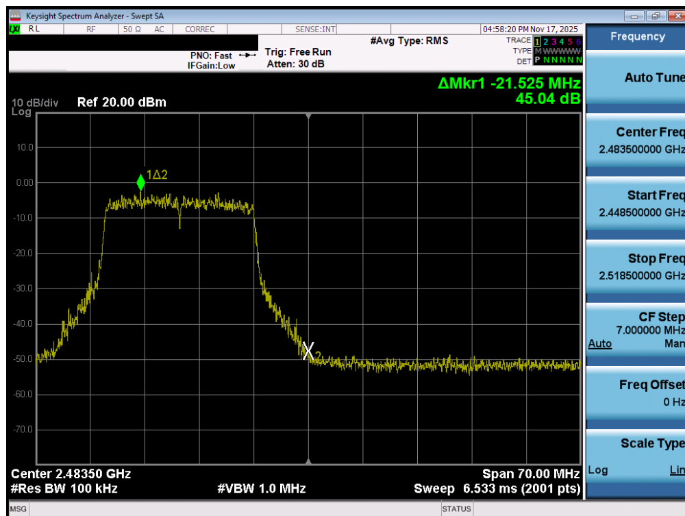
Plot 7-45. Band Edge Plot MIMO ANT1 (802.11ax OFDMA – 242 Tones – Ch. 12)
