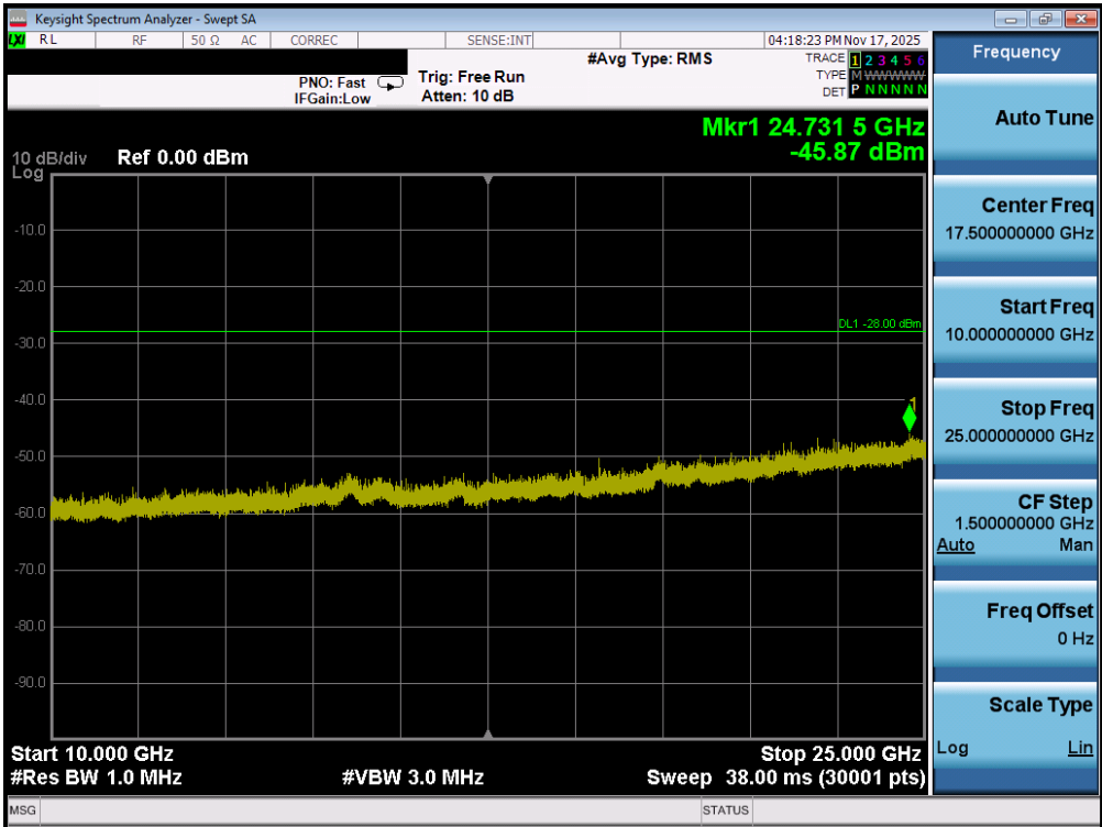
Plot 7-76. Conducted Spurious Plot MIMO ANT2 (802.11ax OFDMA – 242 Tones – Ch. 1)
