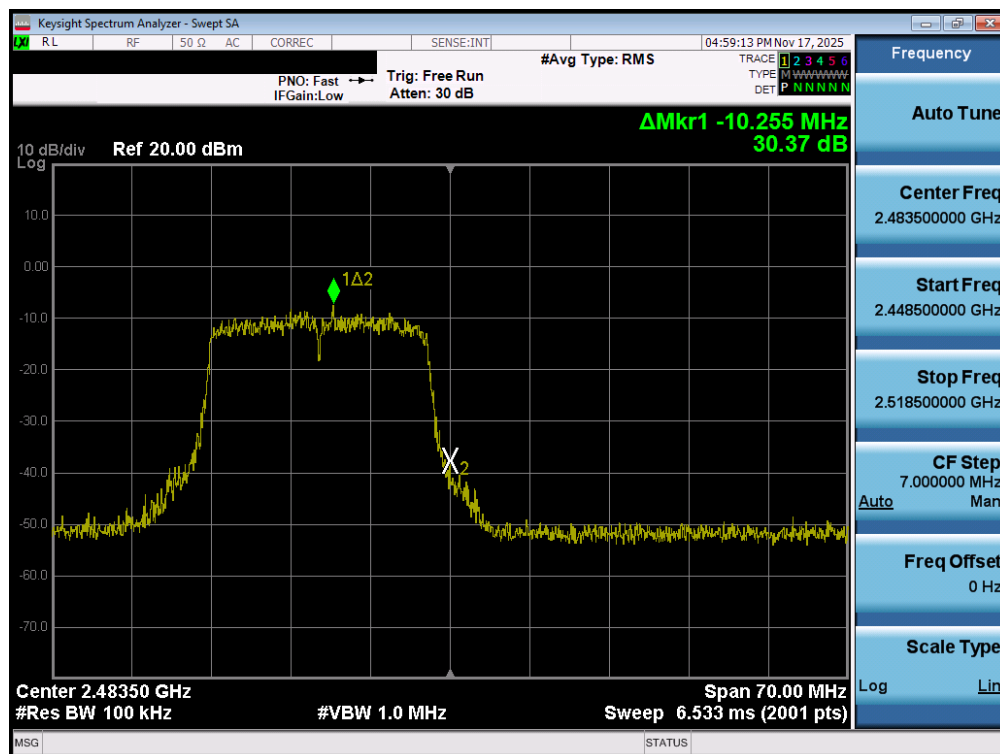
Plot 7-46. Band Edge Plot MIMO ANT1 (802.11ax OFDMA – 242 Tones – Ch. 13)
