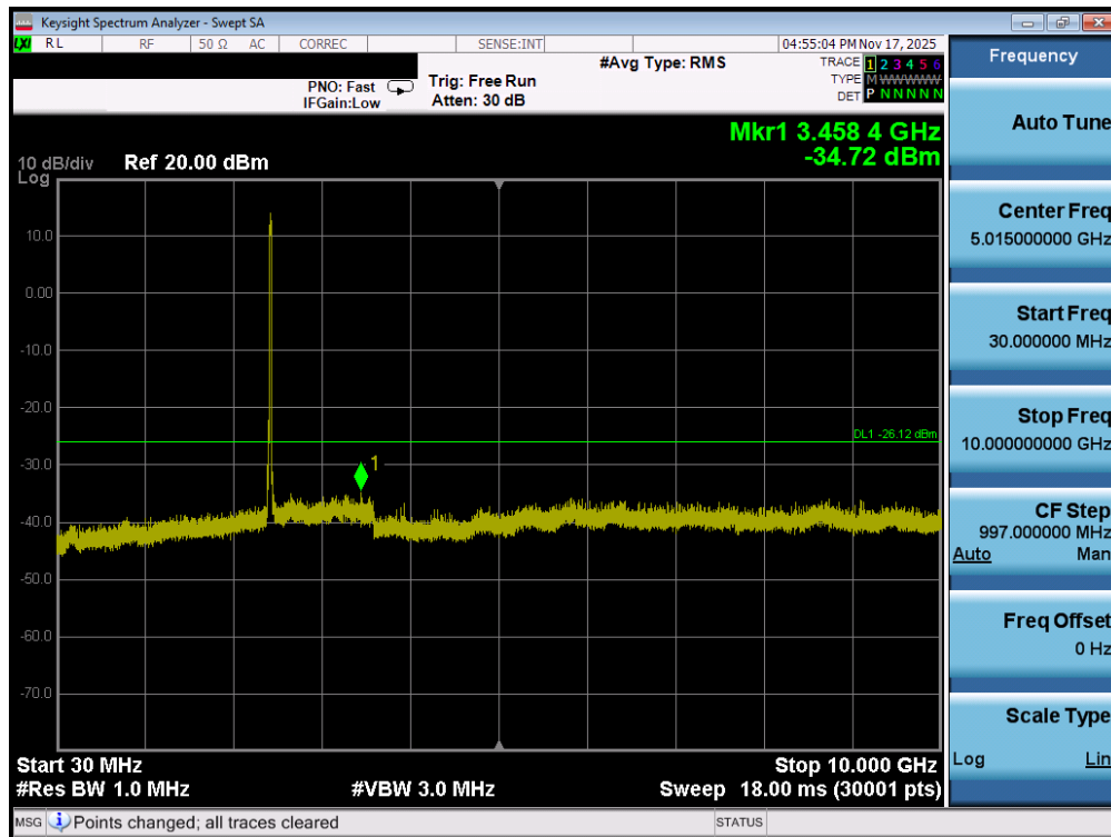
Plot 7-65. Conducted Spurious Plot MIMO ANT1 (802.11ax OFDMA – 242 Tones – Ch. 6)
