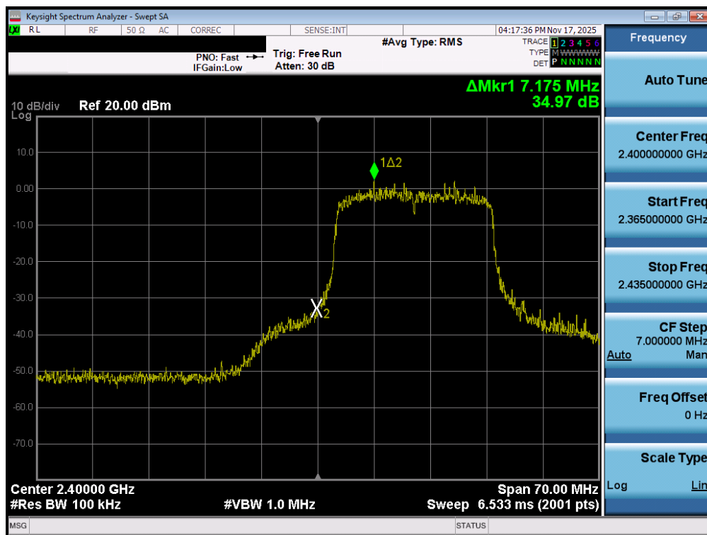
Plot 7-52. Band Edge Plot MIMO ANT2 (802.11ax OFDMA – 242 Tones – Ch. 1)
