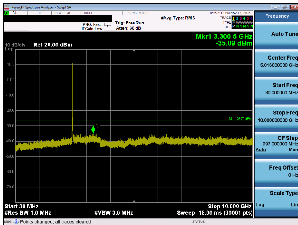
Plot 7-63. Conducted Spurious Plot MIMO ANT1 (802.11ax OFDMA – 242 Tones – Ch. 1)
