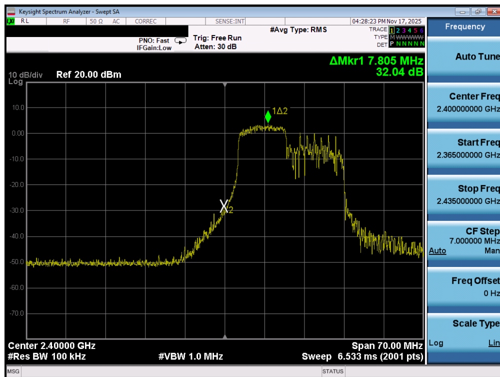
Plot 7-47. Band Edge Plot MIMO ANT2 (802.11ax OFDMA – 106 Tones – Ch. 1)
