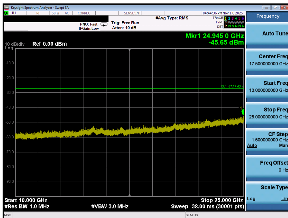
Plot 7-62. Conducted Spurious Plot MIMO ANT1 (802.11ax OFDMA – 26 Tones – Ch. 11)
