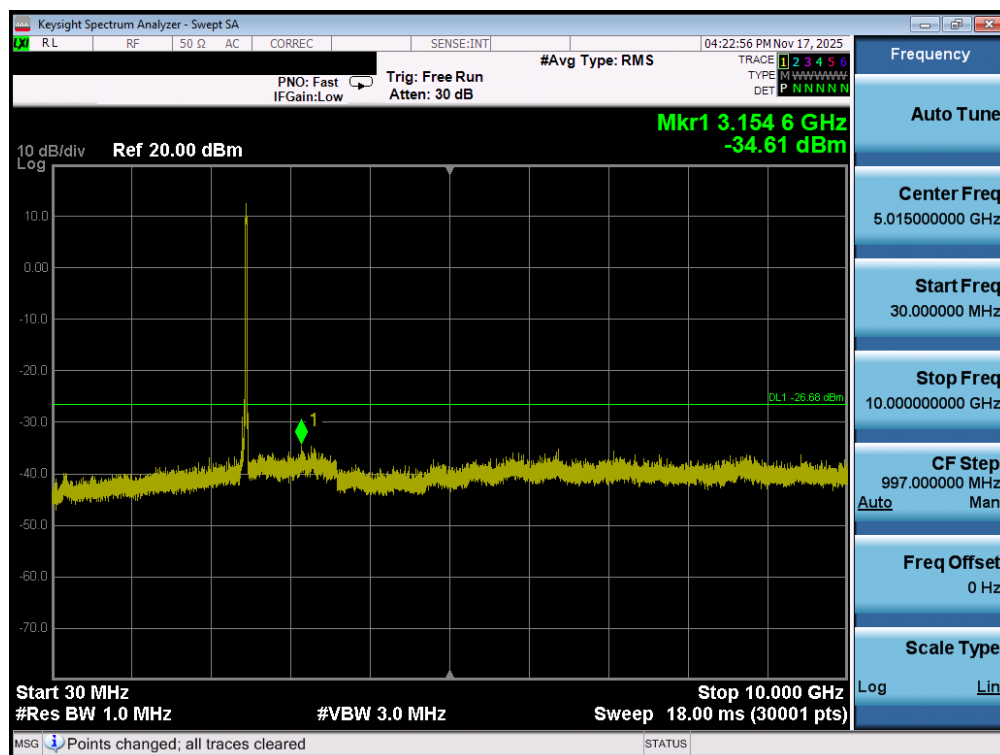
Plot 7-79. Conducted Spurious Plot MIMO ANT2 (802.11ax OFDMA – 242 Tones – Ch. 11)
