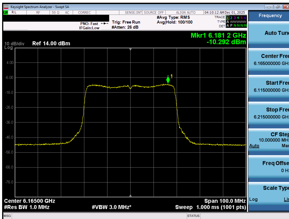
Plot 7-17. Power Spectral Density Plot MIMO ANT1 (40MHz 802.11ax (Full Tones) (UNII Band 5) – Ch. 43) - VLP
