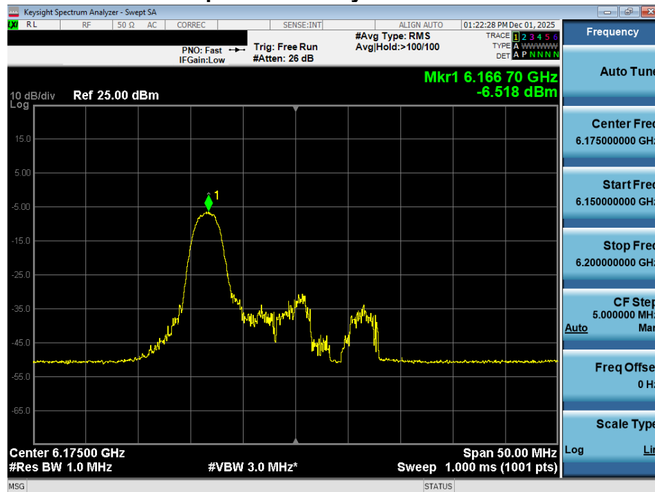
Plot 7-19. Power Spectral Density Plot MIMO ANT2 (20MHz 802.11ax (26 Tones) (UNII Band 5) – Ch. 45) - VLP
