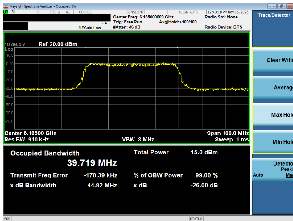
Plot 7-11. 26dB Bandwidth Plot MIMO ANT2 (40MHz 802.11ax (Full Tones) (UNII Band 5) – Ch. 43) - VLP
