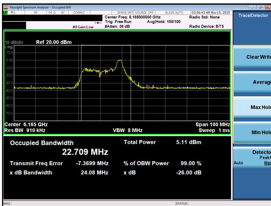
Plot 7-2. 26dB Bandwidth Plot MIMO ANT1 (40MHz 802.11ax (26 Tones) (UNII Band 5) – Ch. 43) - VLP
