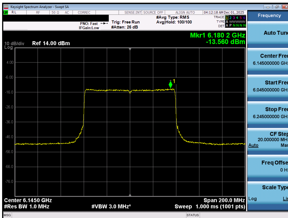
Plot 7-18. Power Spectral Density Plot MIMO ANT1 (80MHz 802.11ax (Full Tones) (UNII Band 5) – Ch. 39) - VLP
