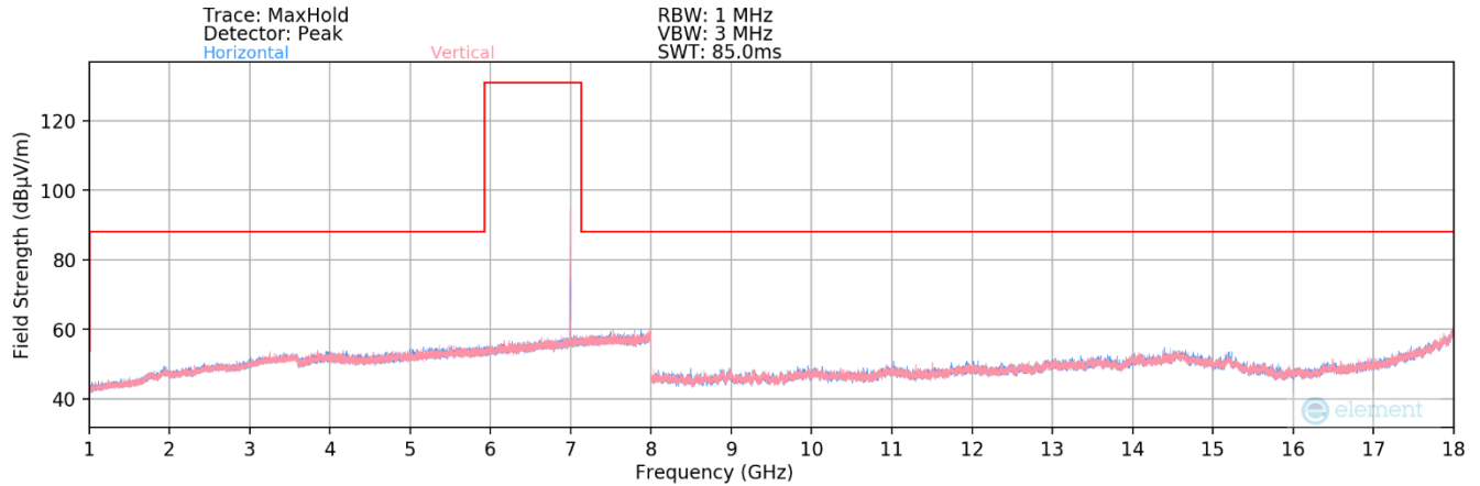
Plot 7-40. Radiated Spurious Plot 1GHz – 18GHz MIMO (802.11ax – U Band 8 Ch. 209)
