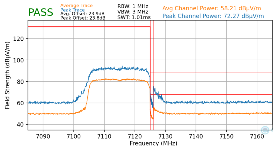
Plot 7-52. Radiated Upper Band Edge Plot MIMO (Average & Peak – UNII Band 8 – 242T)
