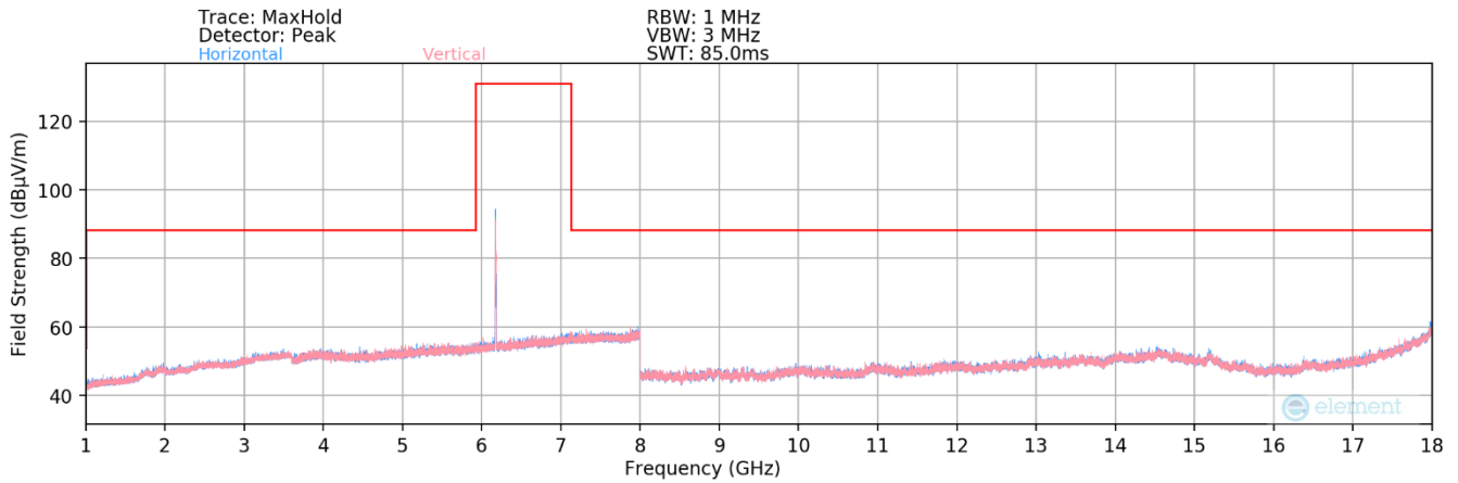
Plot 7-37. Radiated Spurious Plot 1GHz – 18GHz MIMO (802.11ax – UNII Band 5 Ch. 45)
