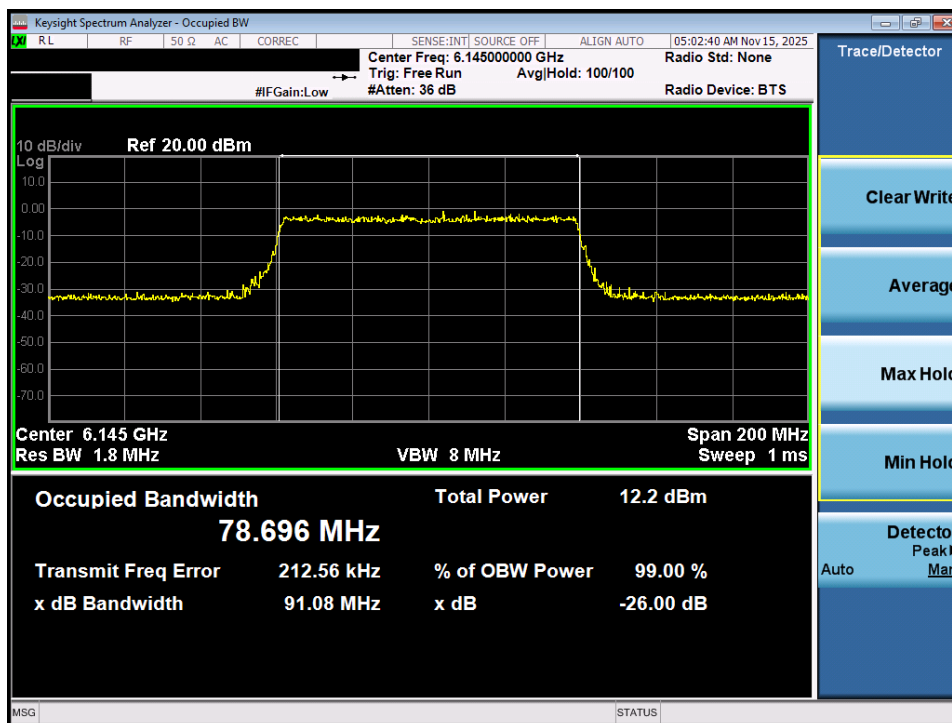
Plot 7-6. 26dB Bandwidth Plot MIMO ANT1 (80MHz 802.11ax (Full Tones) (UNII Band 5) – Ch. 39) - VLP
