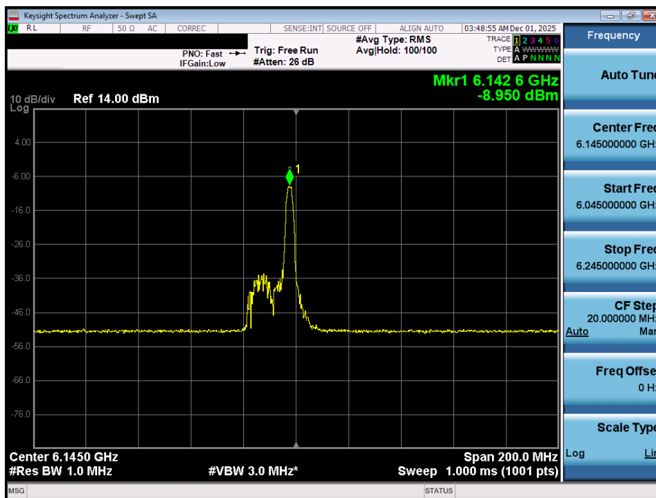
Plot 7-15. Power Spectral Density Plot MIMO ANT1 (80MHz 802.11ax (26 Tones) (UNII Band 5) – Ch. 39) - VLP
