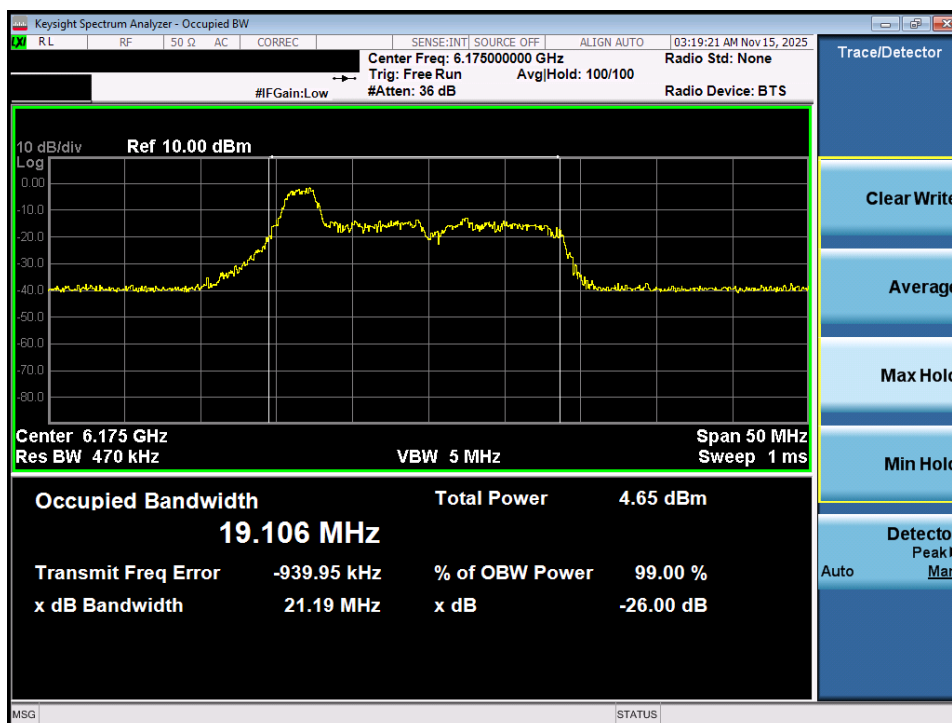
Plot 7-1. 26dB Bandwidth Plot MIMO ANT1 (20MHz 802.11ax (26 Tones) (UNII Band 5) – Ch. 45) - VLP
