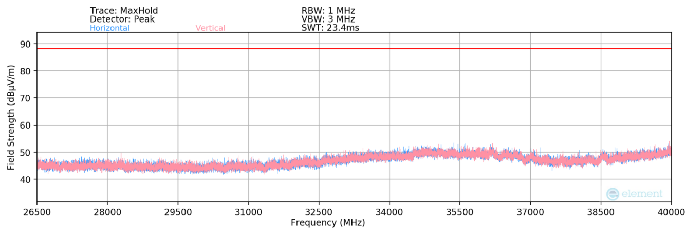
Plot 7-48. Radiated Spurious Plot 26.5GHz - 40GHz (802.11ax)
