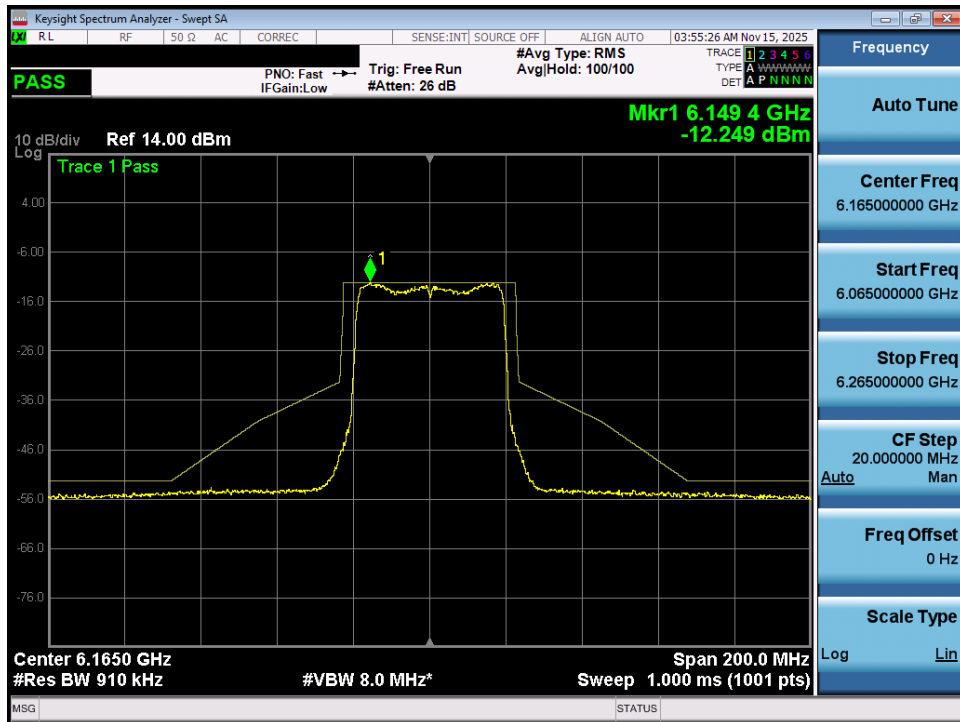
Plot 7-29. In Band Emissions Plot MIMO ANT1 (40MHz 802.11ax (Full Tones) (UNII Band 5) – Ch. 43) - VLP
