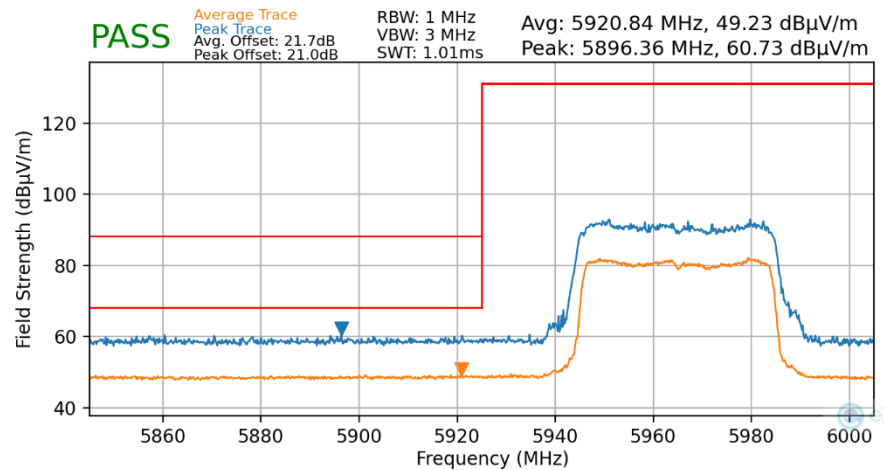
Plot 7-53. Radiated Lower Band Edge Plot MIMO (Average & Peak – UNII Band 5 – 484T)
