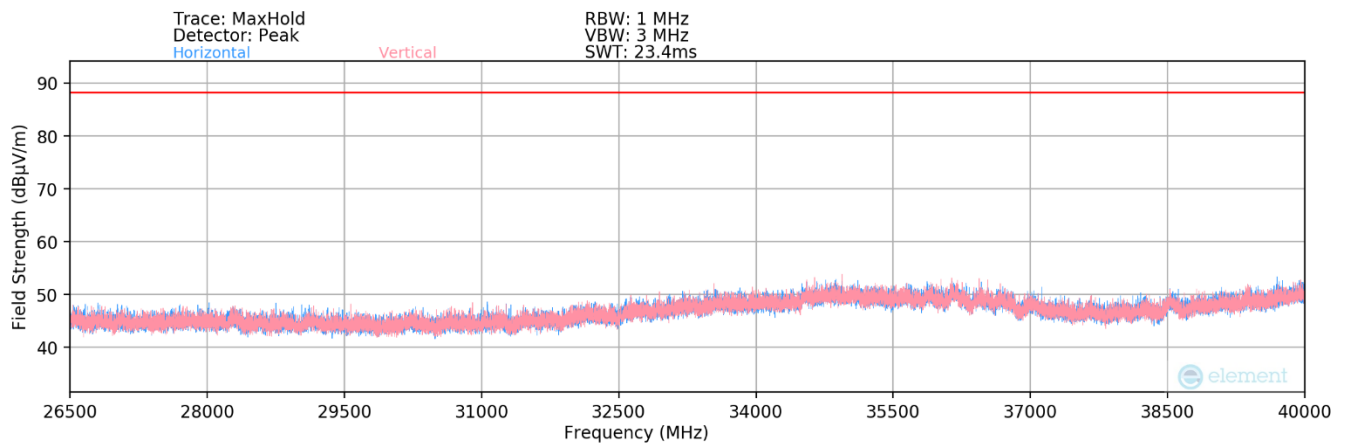
Plot 7-42. Radiated Spurious Plot 26.5GHz - 40GHz (802.11ax)
