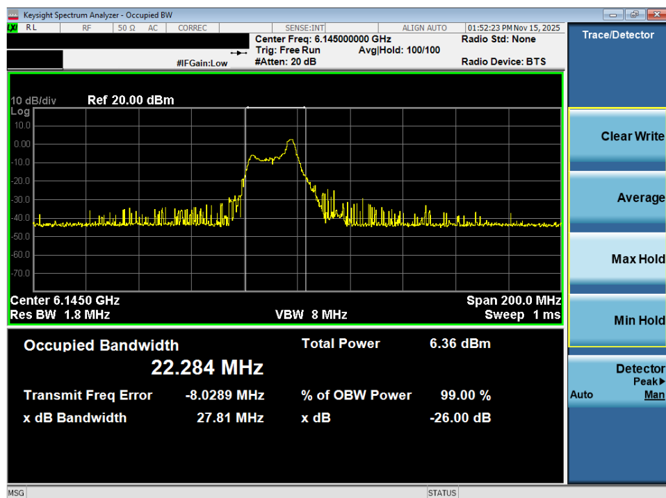
Plot 7-9. 26dB Bandwidth Plot MIMO ANT2 (80MHz 802.11ax (26 Tones) (UNII Band 5) – Ch. 39) - VLP
