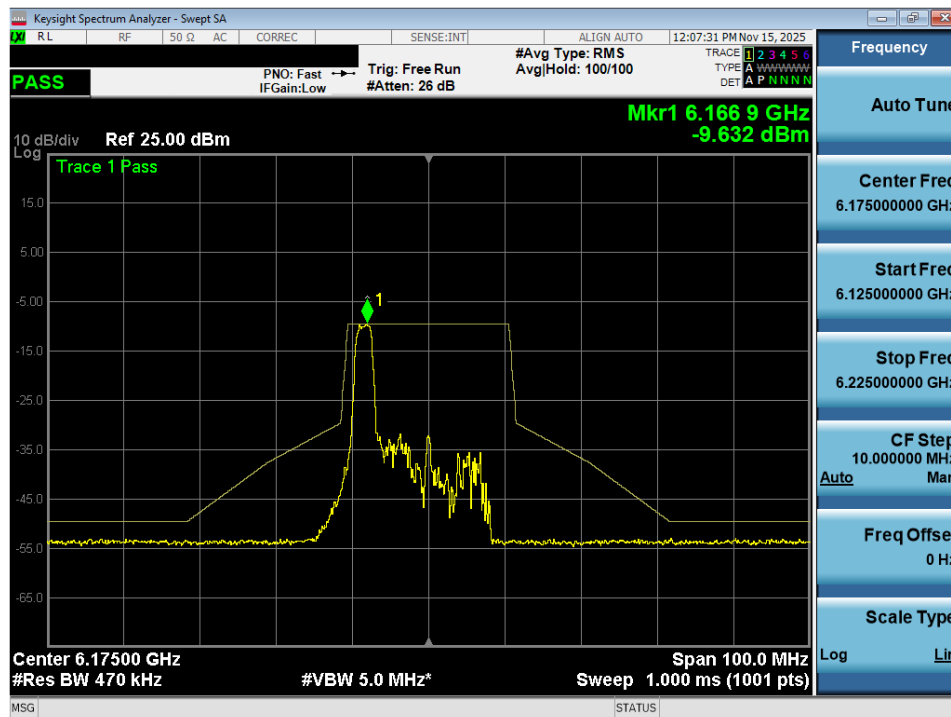
Plot 7-31. In Band Emissions Plot MIMO ANT2 (20MHz 802.11ax (26 Tones) (UNII Band 5) – Ch. 45) - VLP
