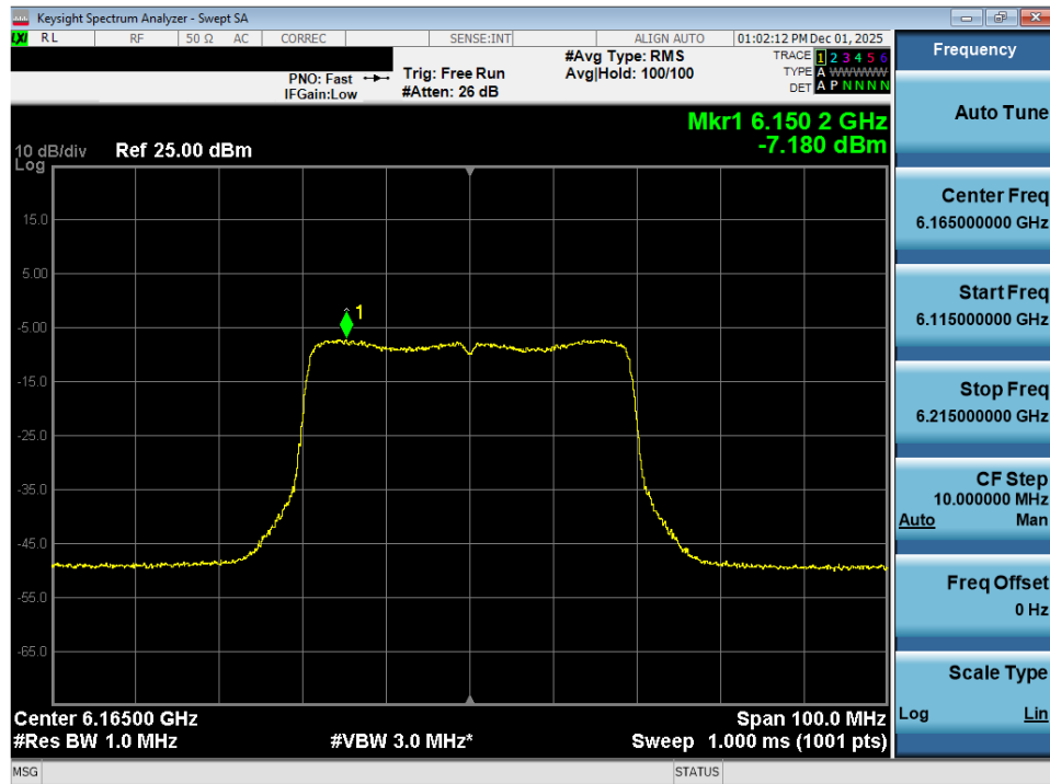
Plot 7-23. Power Spectral Density Plot MIMO ANT2 (40MHz 802.11ax (Full Tones) (UNII Band 5) – Ch. 43) - VLP
