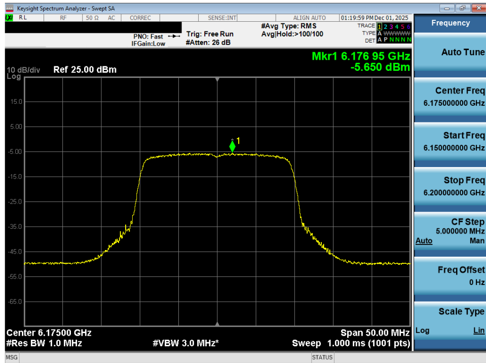
Plot 7-22. Power Spectral Density Plot MIMO ANT2 (20MHz 802.11ax (Full Tones) (UNII Band 5) – Ch. 45) - VLP
