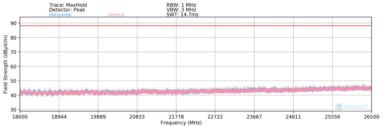
Plot 7-41. Radiated Spurious Plot 18GHz - 26.5GHz (802.11ax)
