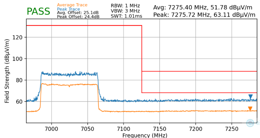
Plot 7-56. Radiated Upper Band Edge Plot MIMO (Average & Peak – UNII Band 8 – 996T)
