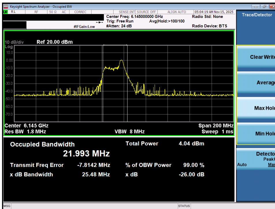
Plot 7-3. 26dB Bandwidth Plot MIMO ANT1 (80MHz 802.11ax (26 Tones) (UNII Band 5) – Ch. 39) - VLP
