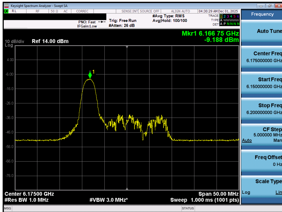
Plot 7-13. Power Spectral Density Plot MIMO ANT1 (20MHz 802.11ax (26 Tones) (UNII Band 5) – Ch. 45) - VLP
