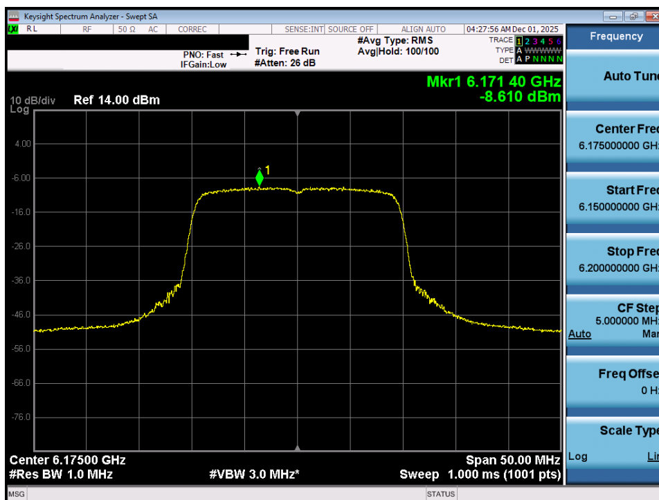
Plot 7-16. Power Spectral Density Plot MIMO ANT1 (20MHz 802.11ax (Full Tones) (UNII Band 5) – Ch. 45) - VLP
