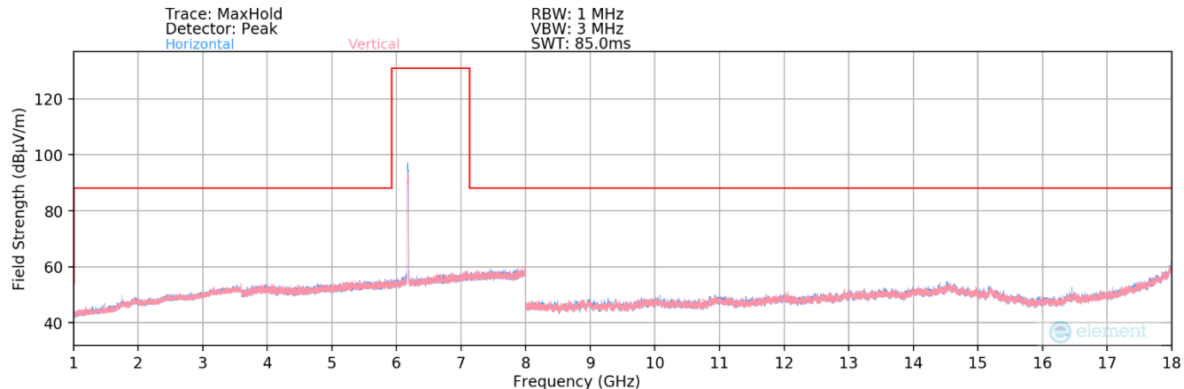
Plot 7-43. Radiated Spurious Plot 1GHz – 18GHz MIMO (802.11ax – UNII Band 5 Ch. 45)
