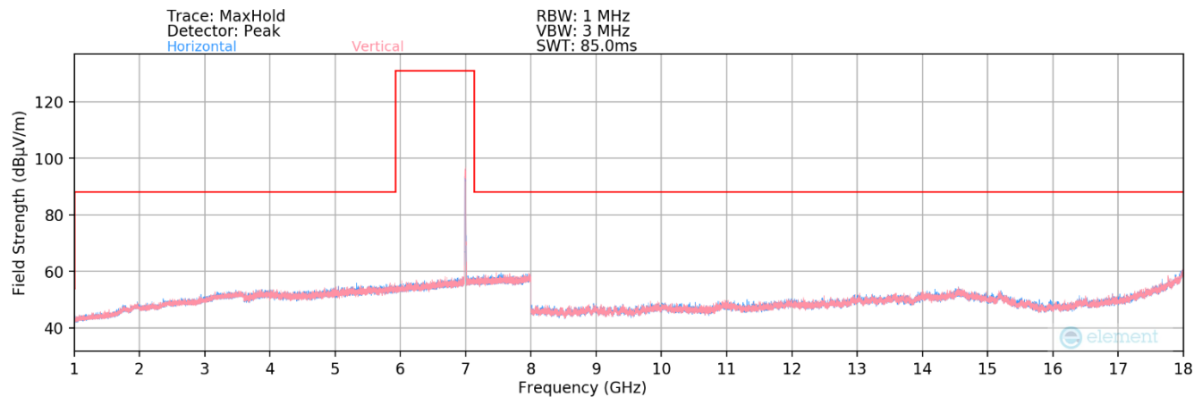
Plot 7-46. Radiated Spurious Plot 1GHz – 18GHz MIMO (802.11ax – U Band 8 Ch. 209)
