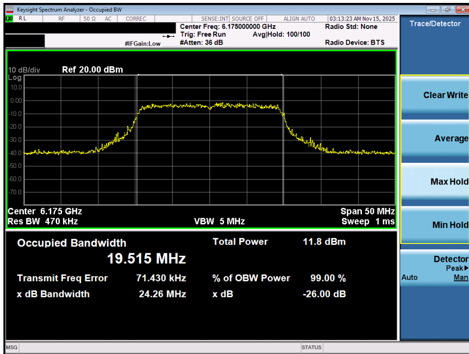
Plot 7-4. 26dB Bandwidth Plot MIMO ANT1 (20MHz 802.11ax (Full Tones) (UNII Band 5) – Ch. 45) - VLP
