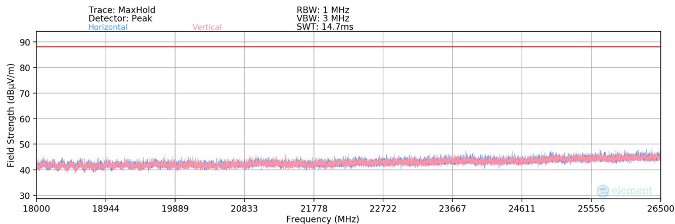
Plot 7-47. Radiated Spurious Plot 18GHz - 26.5GHz (802.11ax)
