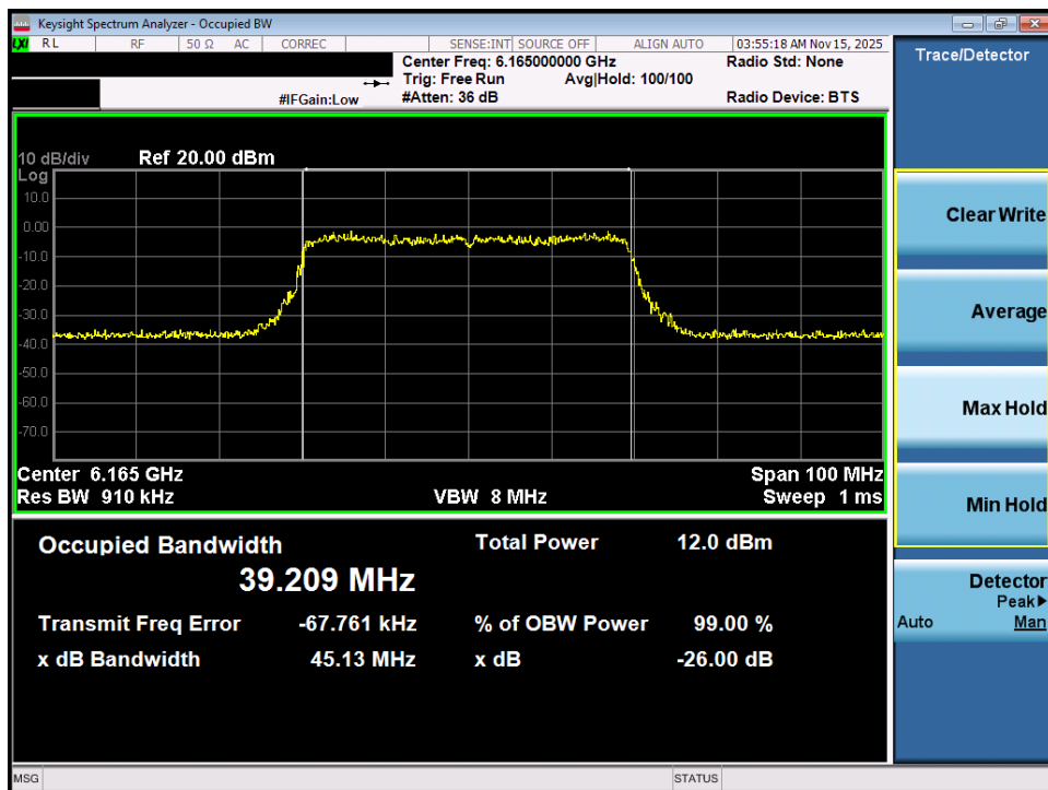
Plot 7-5. 26dB Bandwidth Plot MIMO ANT1 (40MHz 802.11ax (Full Tones) (UNII Band 5) – Ch. 43) - VLP
