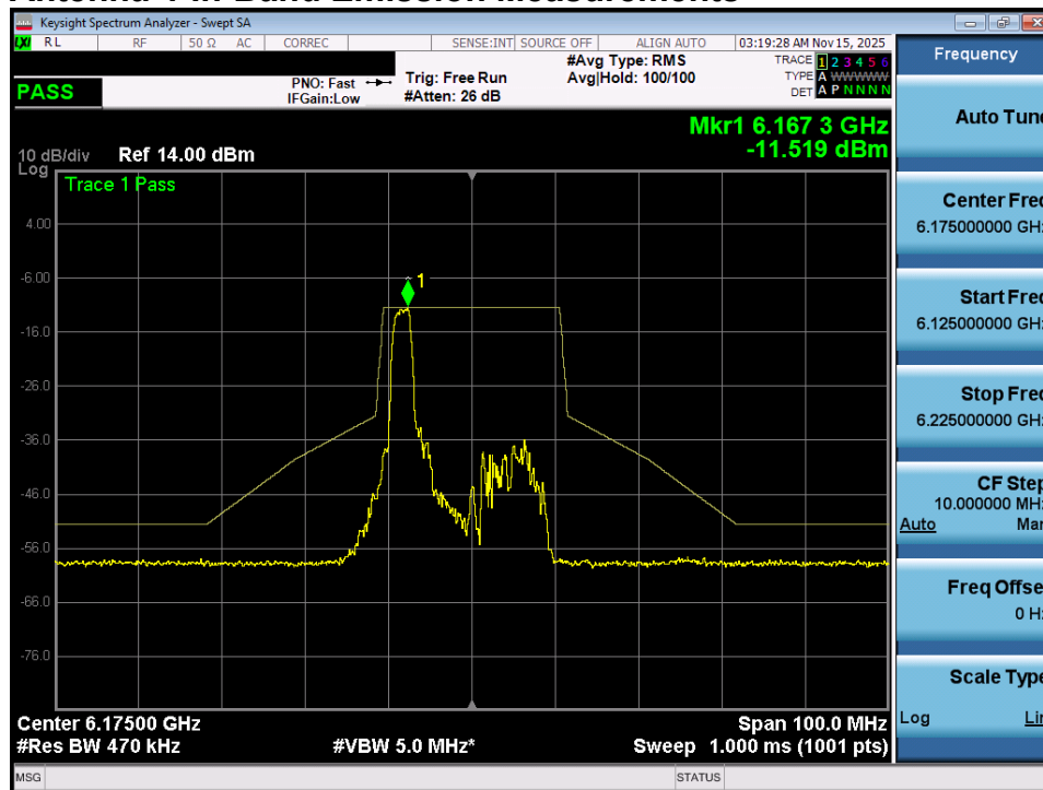
Plot 7-25. In Band Emissions Plot MIMO ANT1 (20MHz 802.11ax (26 Tones) (UNII Band 5) – Ch. 45) - VLP
