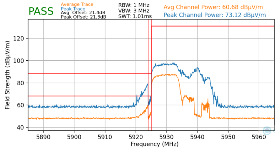
Plot 7-49. Radiated Lower Band Edge Plot MIMO (Average & Peak – UNII Band 5 – 106T)
