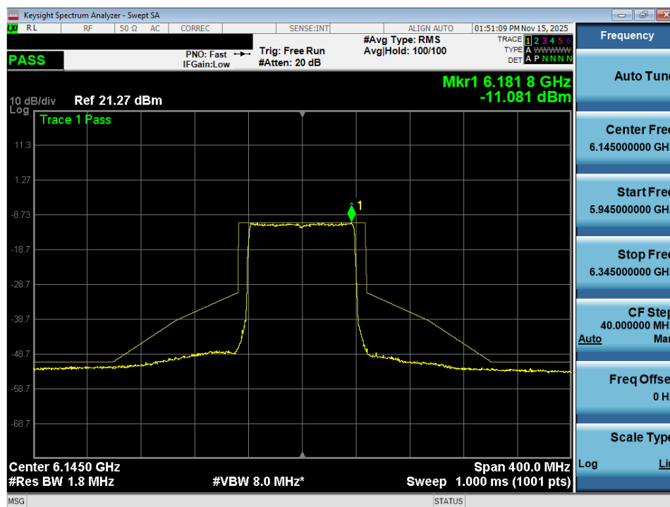
Plot 7-36. In Band Emissions Plot MIMO ANT2 (80MHz 802.11ax (Full Tones) (UNII Band 5) – Ch. 39) - VLP
