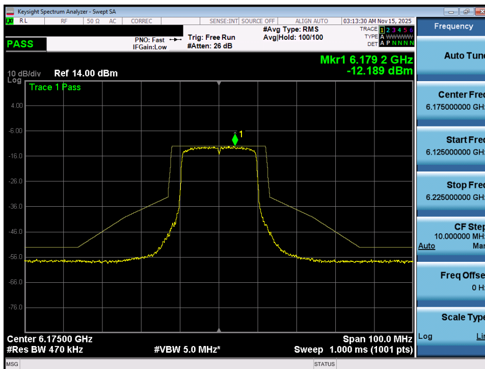
Plot 7-28. In Band Emissions Plot MIMO ANT1 (20MHz 802.11ax (Full Tones) (UNII Band 5) – Ch. 45) - VLP
