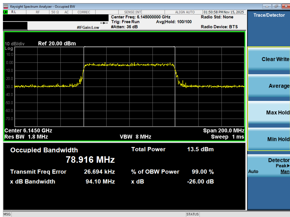
Plot 7-12. 26dB Bandwidth Plot MIMO ANT2 (80MHz 802.11ax (Full Tones) (UNII Band 5) – Ch. 39) - VLP
