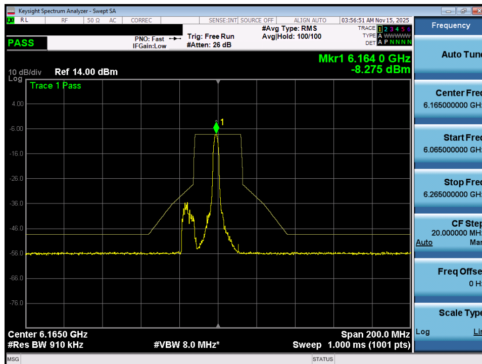
Plot 7-26. In Band Emissions Plot MIMO ANT1 (40MHz 802.11ax (26 Tones) (UNII Band 5) – Ch. 43) - VLP
