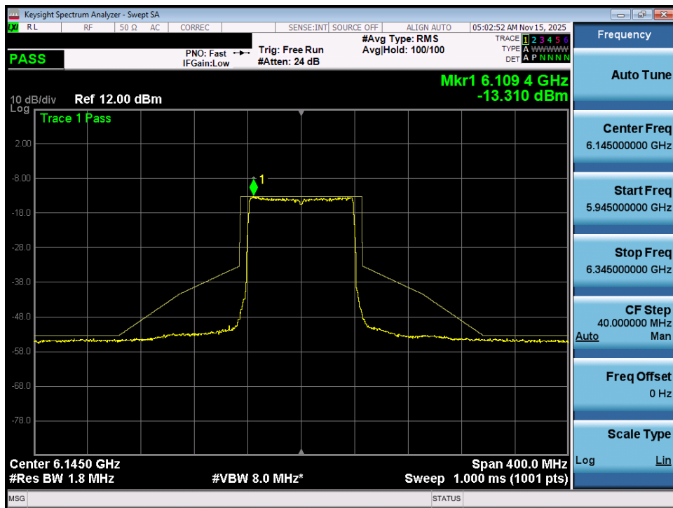
Plot 7-30. In Band Emissions Plot MIMO ANT1 (80MHz 802.11ax (Full Tones) (UNII Band 5) – Ch. 39) - VLP
