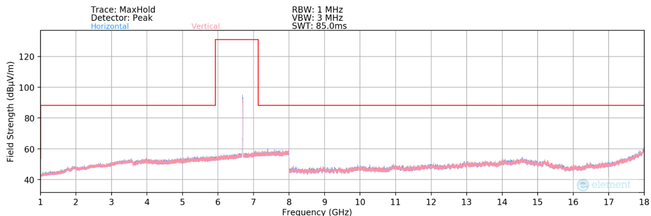
Plot 7-45. Radiated Spurious Plot 1GHz – 18GHz MIMO (802.11ax – UNII Band 7 Ch. 149)
