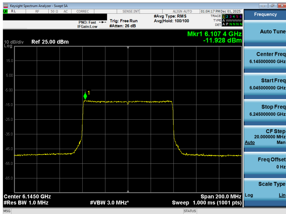
Plot 7-24. Power Spectral Density Plot MIMO ANT2 (80MHz 802.11ax (Full Tones) (UNII Band 5) – Ch. 39) - VLP
