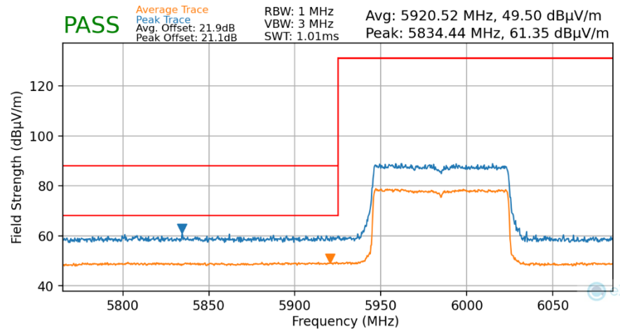
Plot 7-55. Radiated Lower Band Edge Plot MIMO (Average & Peak – UNII Band 5 – 996T)
