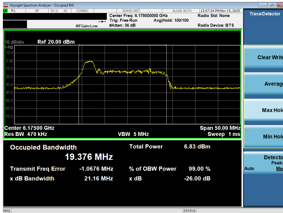
Plot 7-7. 26dB Bandwidth Plot MIMO ANT2 (20MHz 802.11ax (26 Tones) (UNII Band 5) – Ch. 45) - VLP
