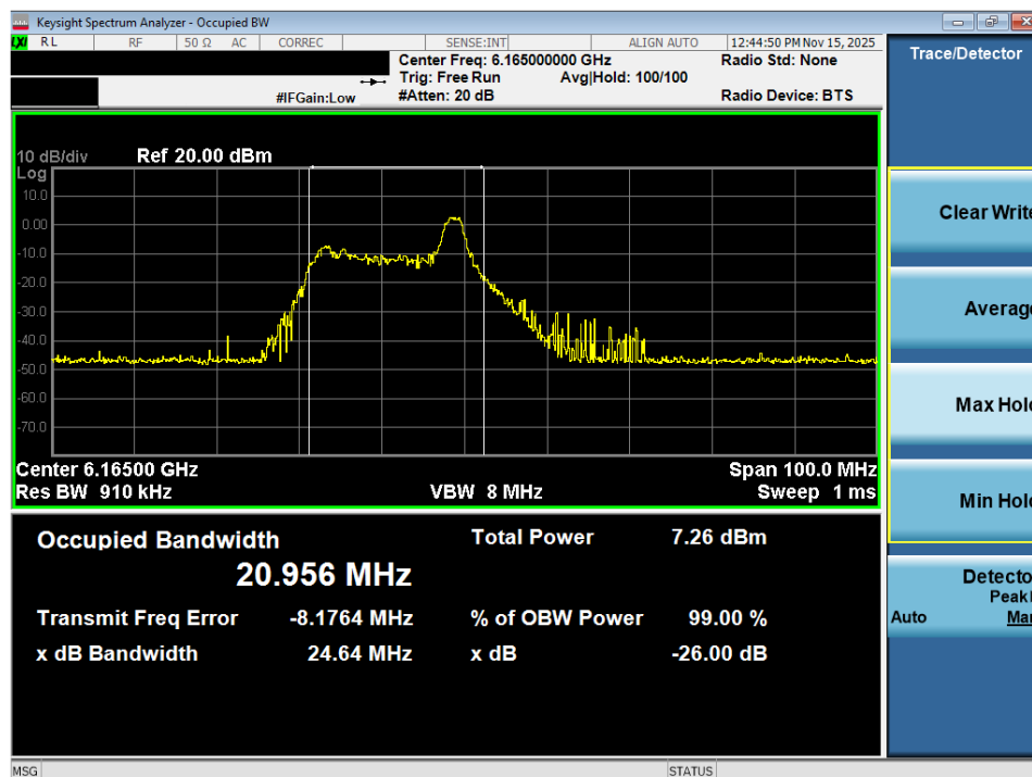
Plot 7-8. 26dB Bandwidth Plot MIMO ANT2 (40MHz 802.11ax (26 Tones) (UNII Band 5) – Ch. 43) - VLP
