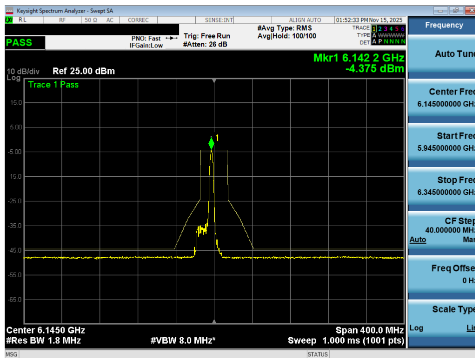
Plot 7-33. In Band Emissions Plot MIMO ANT2 (80MHz 802.11ax (26 Tones) (UNII Band 5) – Ch. 39) - VLP
