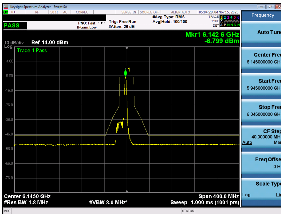
Plot 7-27. In Band Emissions Plot MIMO ANT1 (80MHz 802.11ax (26 Tones) (UNII Band 5) – Ch. 39) - VLP
