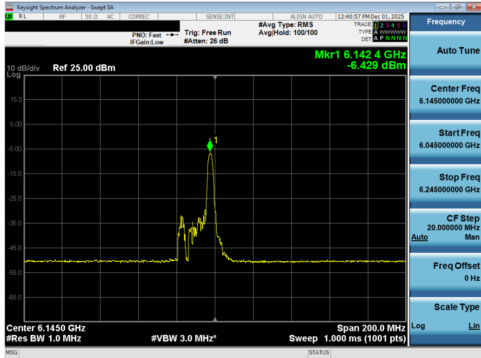
Plot 7-21. Power Spectral Density Plot MIMO ANT2 (80MHz 802.11ax (26 Tones) (UNII Band 5) – Ch. 39) - VLP
