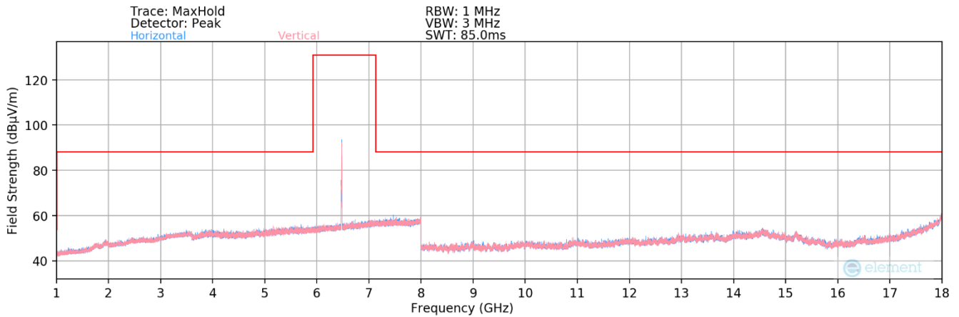
Plot 7-38. Radiated Spurious Plot 1GHz – 18GHz MIMO (802.11ax – UNII Band 6 Ch. 105)
