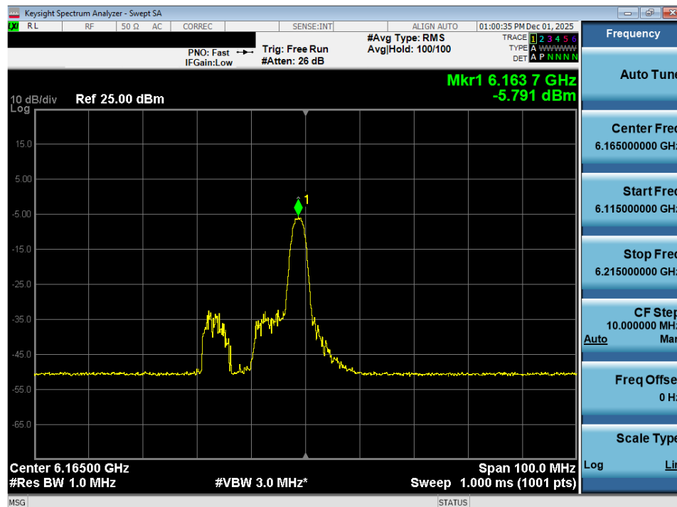
Plot 7-20. Power Spectral Density Plot MIMO ANT2 (40MHz 802.11ax (26 Tones) (UNII Band 5) – Ch. 43) - VLP
