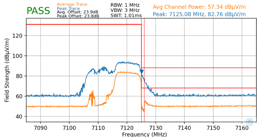
Plot 7-50. Radiated Upper Band Edge Plot MIMO (Average & Peak – UNII Band 8 – 106T)
