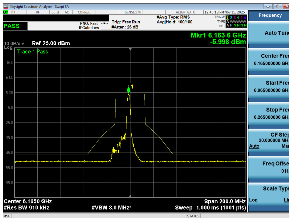
Plot 7-32. In Band Emissions Plot MIMO ANT2 (40MHz 802.11ax (26 Tones) (UNII Band 5) – Ch. 43) - VLP
