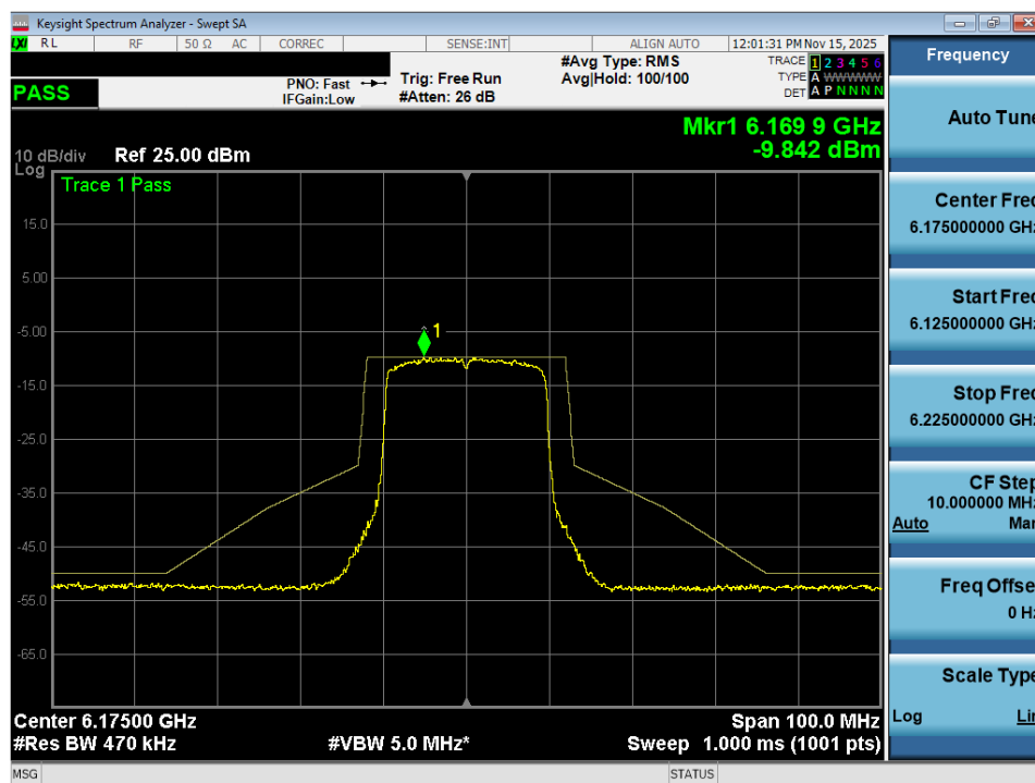
Plot 7-34. In Band Emissions Plot MIMO ANT2 (20MHz 802.11ax (Full Tones) (UNII Band 5) – Ch. 45) - VLP
