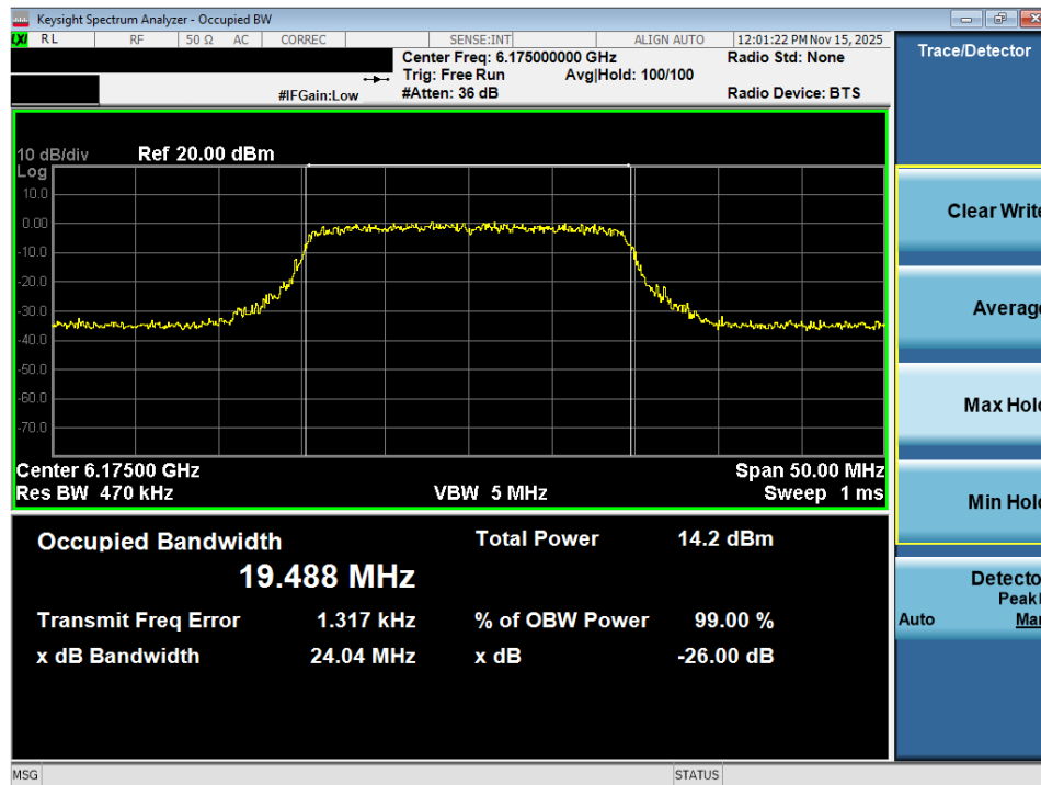
Plot 7-10. 26dB Bandwidth Plot MIMO ANT2 (20MHz 802.11ax (Full Tones) (UNII Band 5) – Ch. 45) - VLP
