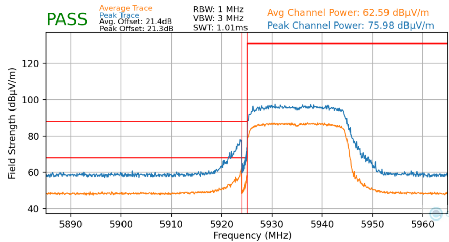
Plot 7-51. Radiated Lower Band Edge Plot MIMO (Average & Peak – UNII Band 5 – 242T)
