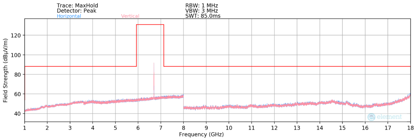
Plot 7-39. Radiated Spurious Plot 1GHz – 18GHz MIMO (802.11ax – UNII Band 7 Ch. 149)
