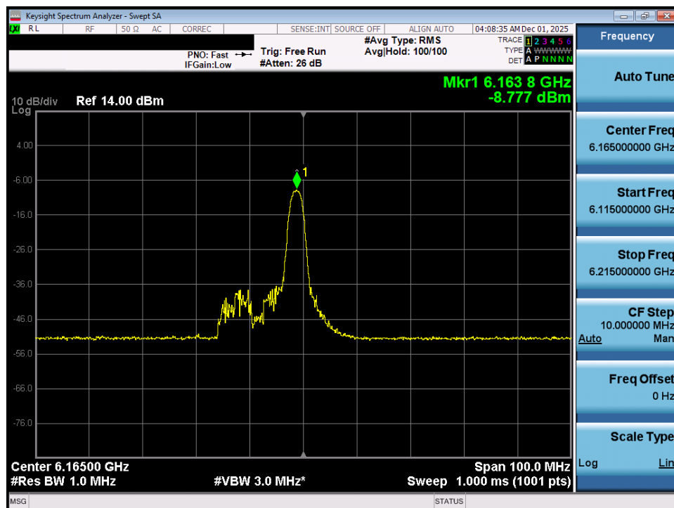
Plot 7-14. Power Spectral Density Plot MIMO ANT1 (40MHz 802.11ax (26 Tones) (UNII Band 5) – Ch. 43) - VLP
