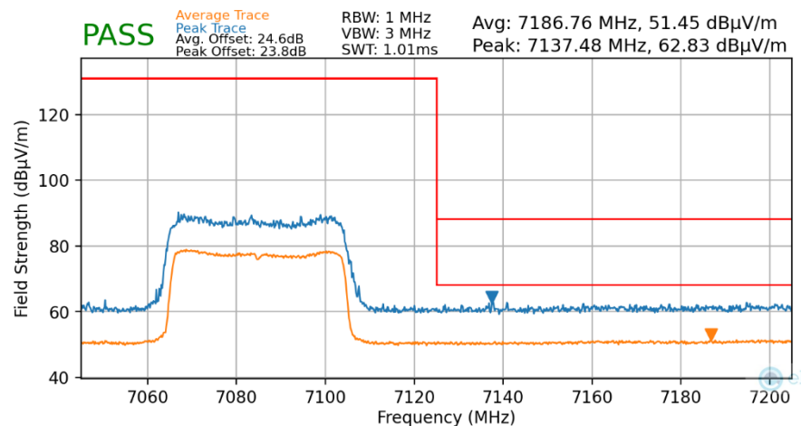
Plot 7-54. Radiated Upper Band Edge Plot MIMO (Average & Peak – UNII Band 8 – 484T)
