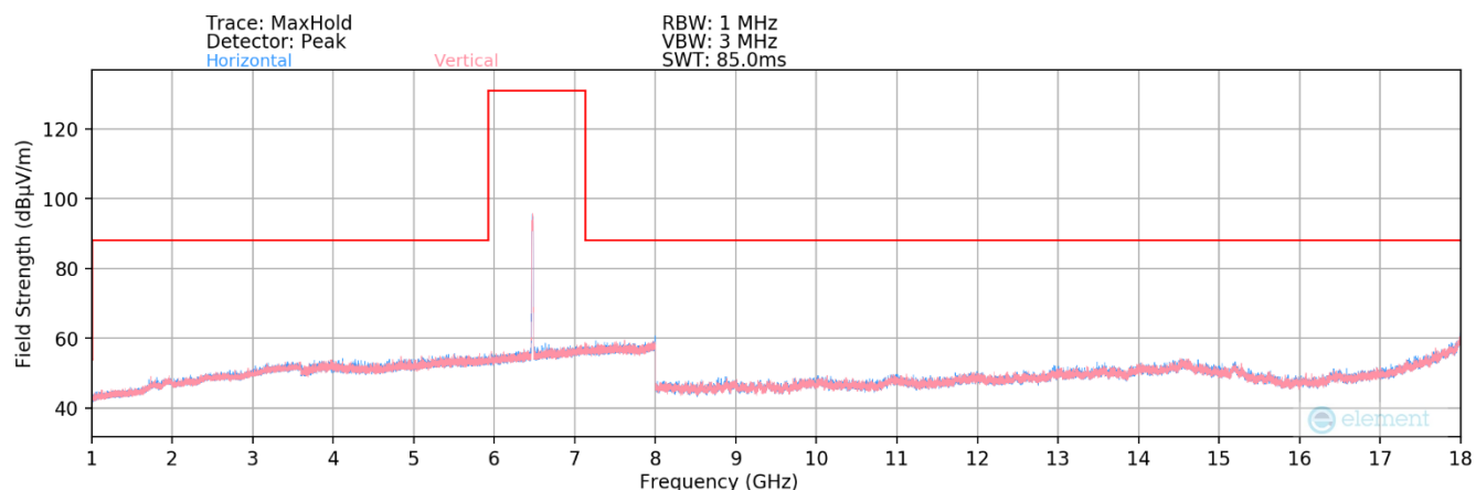
Plot 7-44. Radiated Spurious Plot 1GHz – 18GHz MIMO (802.11ax – UNII Band 6 Ch. 105)
