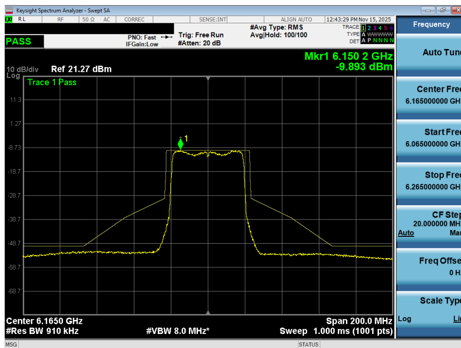
Plot 7-35. In Band Emissions Plot MIMO ANT2 (40MHz 802.11ax (Full Tones) (UNII Band 5) – Ch. 43) - VLP
