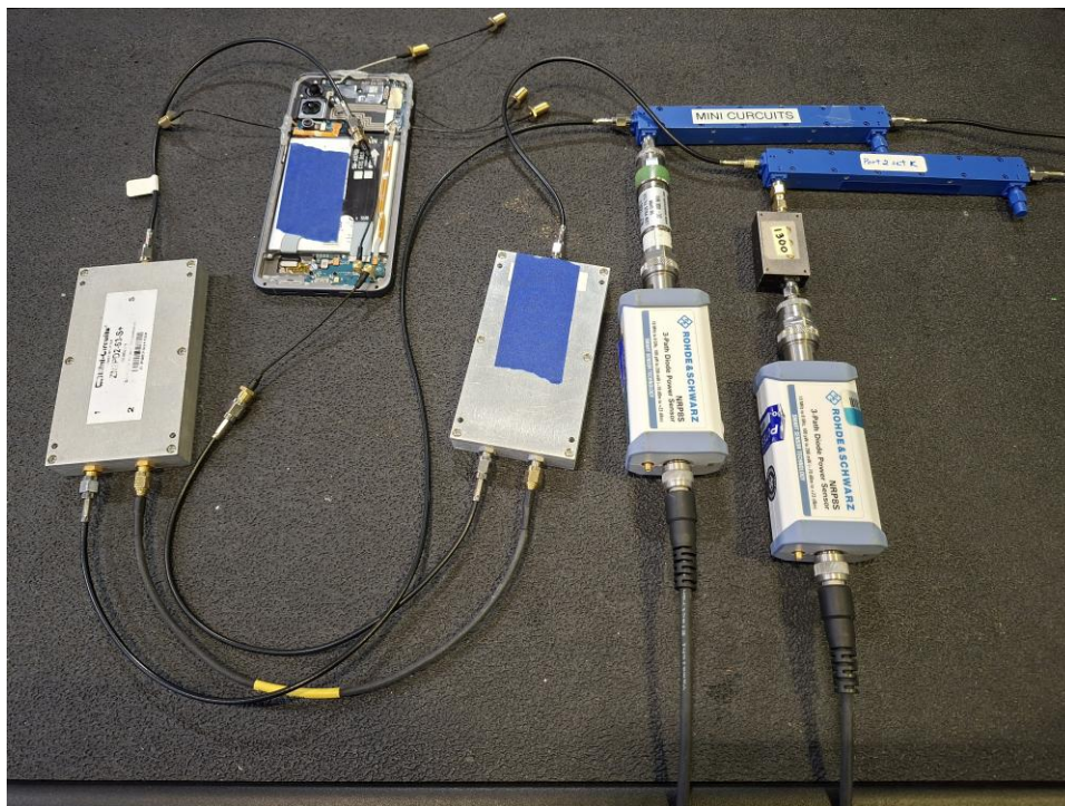
Test Setup Photo 6 – Conducted Test Setup (Figure 7.2-1e)
