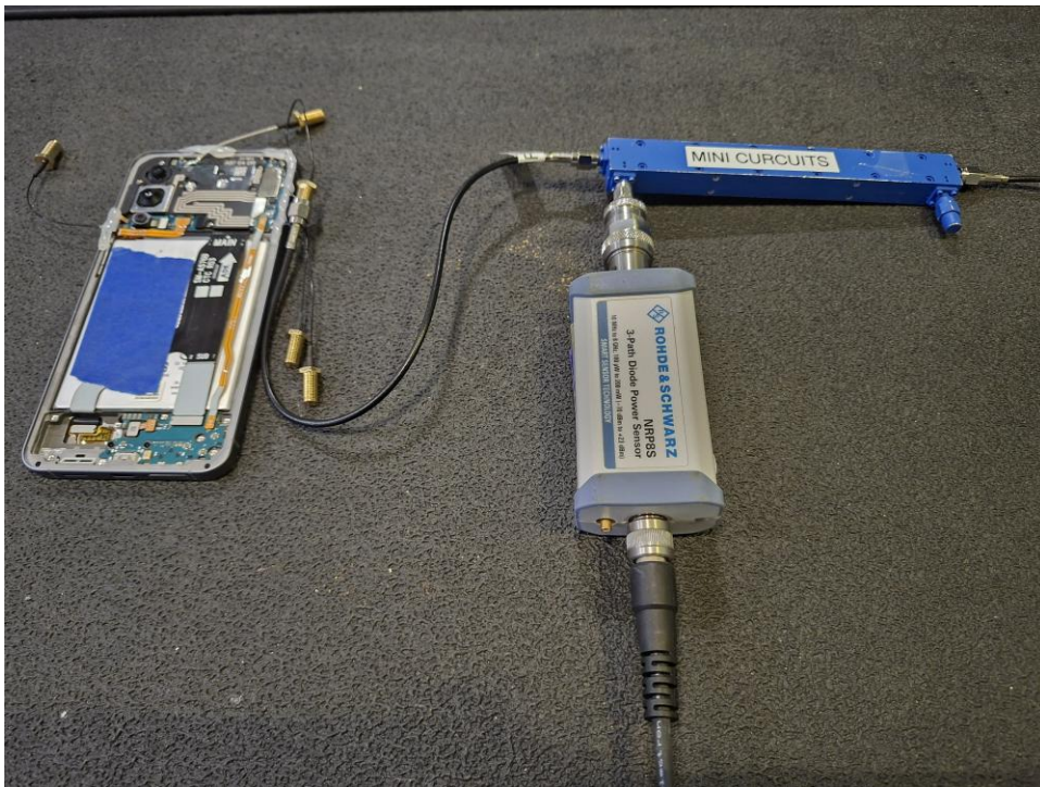
Test Setup Photo 8 – Conducted Test Setup (Figure 7.2-1a)
