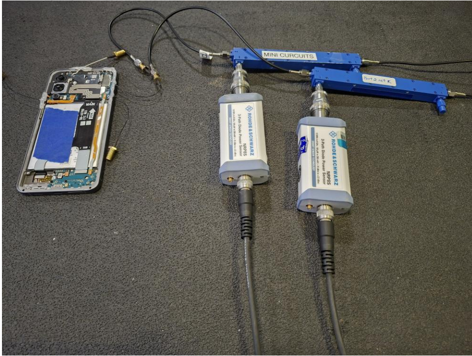
Test Setup Photo 9 – Conducted Test Setup (Figure 7.2-1f)
