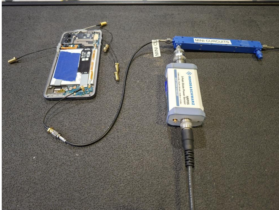
Test Setup Photo 1 – Conducted Test Setup (Figure 7.2-1a)
