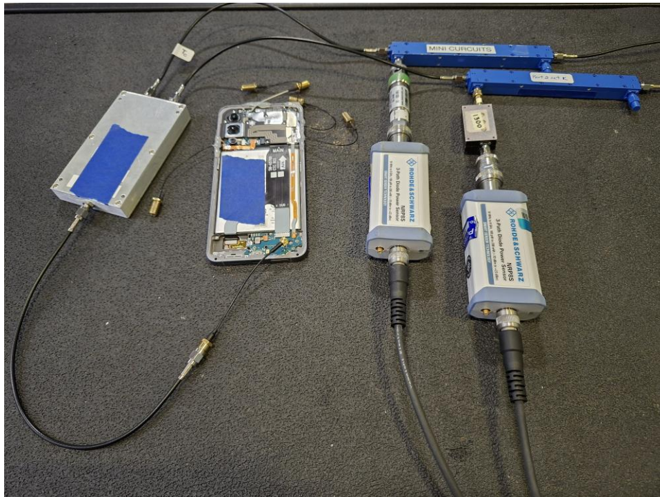
Test Setup Photo 5 – Conducted Test Setup (Figure 7.2-1d)
