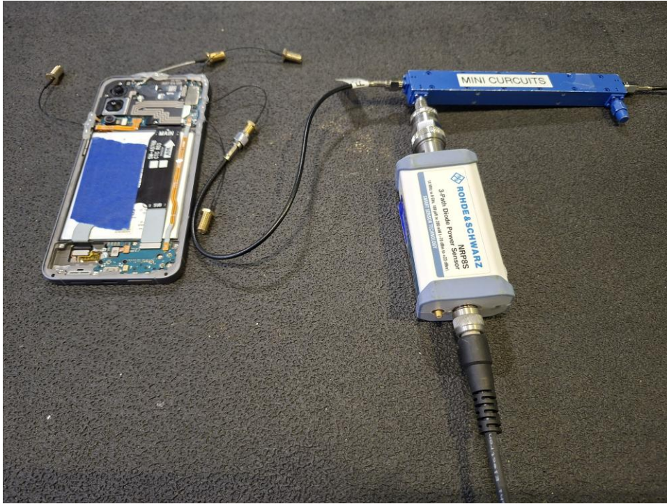
Test Setup Photo 7 – Conducted Test Setup (Figure 7.2-1a)
