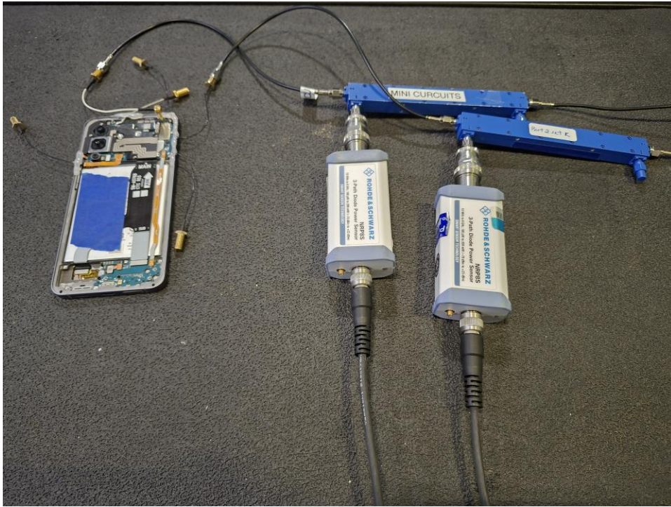
Test Setup Photo 10 – Conducted Test Setup (Figure 7.2-1g)
