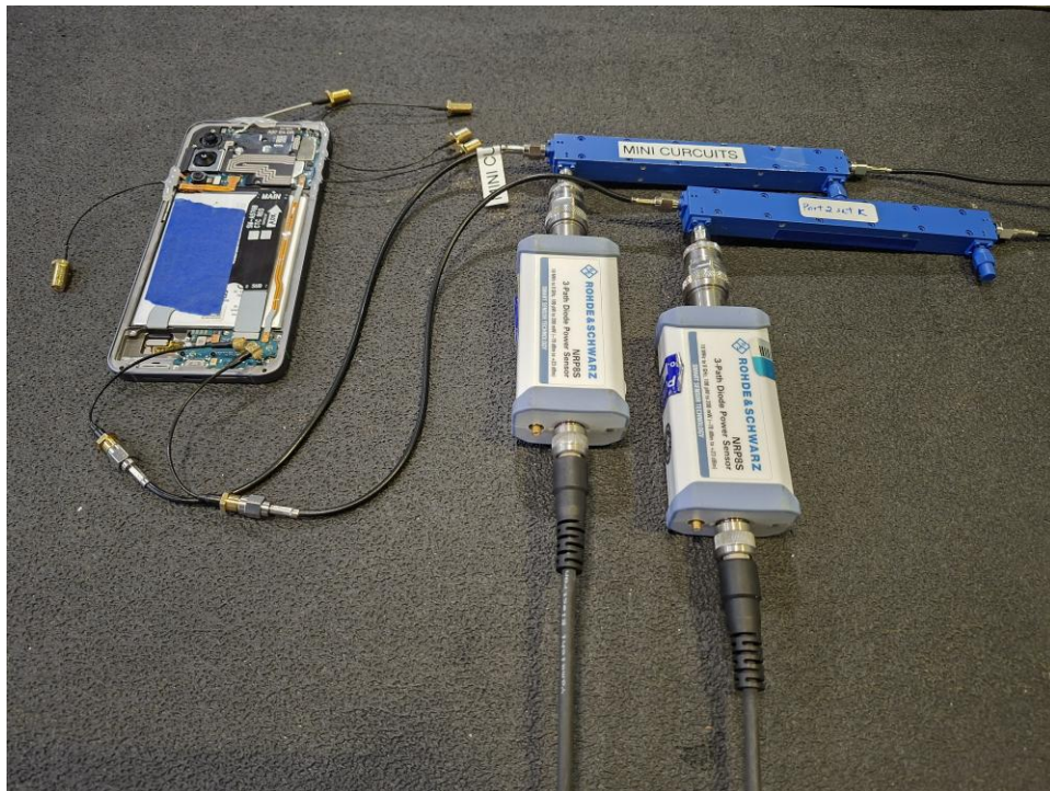
Test Setup Photo 4 – Conducted Test Setup (Figure 7.2-1c)
