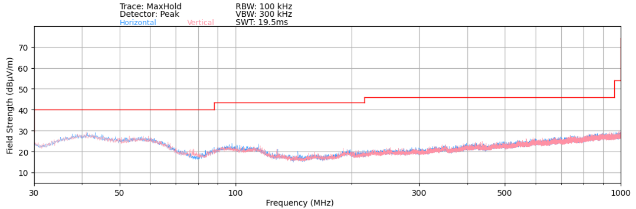
Plot 7-57. Radiated Spurious Plot below 1GHz
