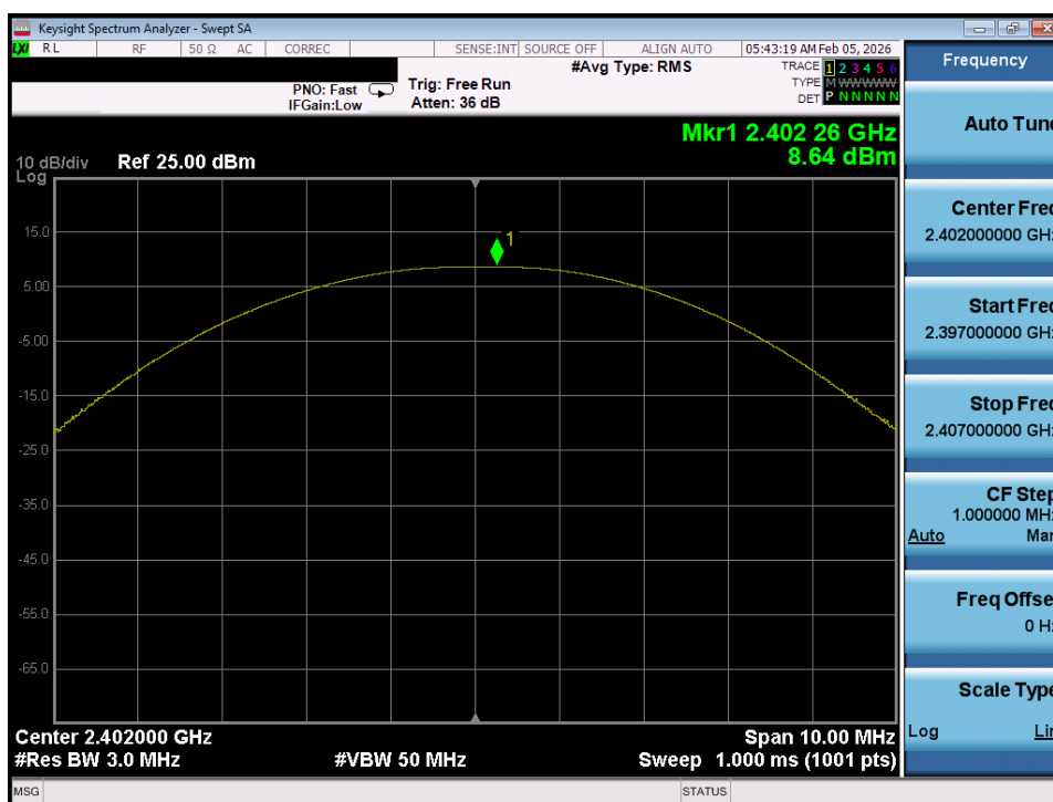
Plot 7-16. Peak Power Plot (Bluetooth (LE), 500kbps – Ch. 37)
