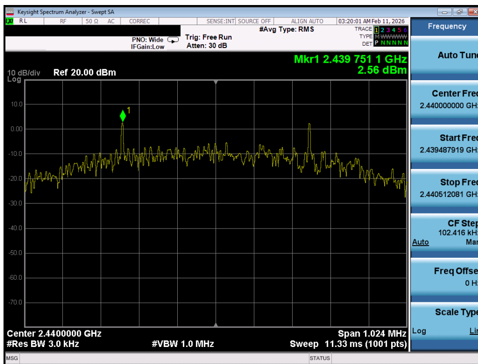
Plot 7-29. Power Spectral Density Plot (Bluetooth (LE), 500kbps – Ch. 17)
