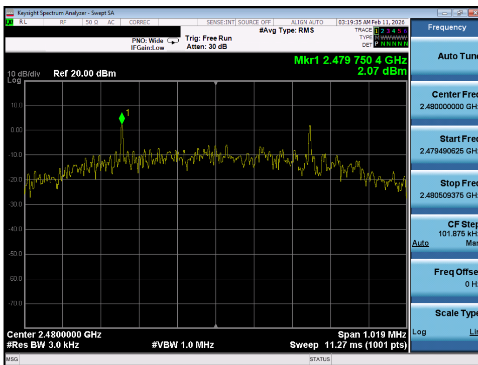
Plot 7-30. Power Spectral Density Plot (Bluetooth (LE), 500kbps – Ch. 39)
