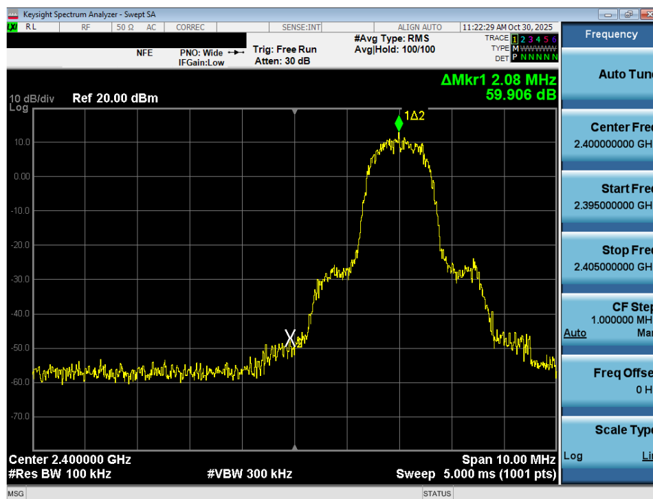
Plot 7-28. Band Edge Plot (Bluetooth with Hopping Disabled, 3 Mbps – Ch. 0) – Ant 1
