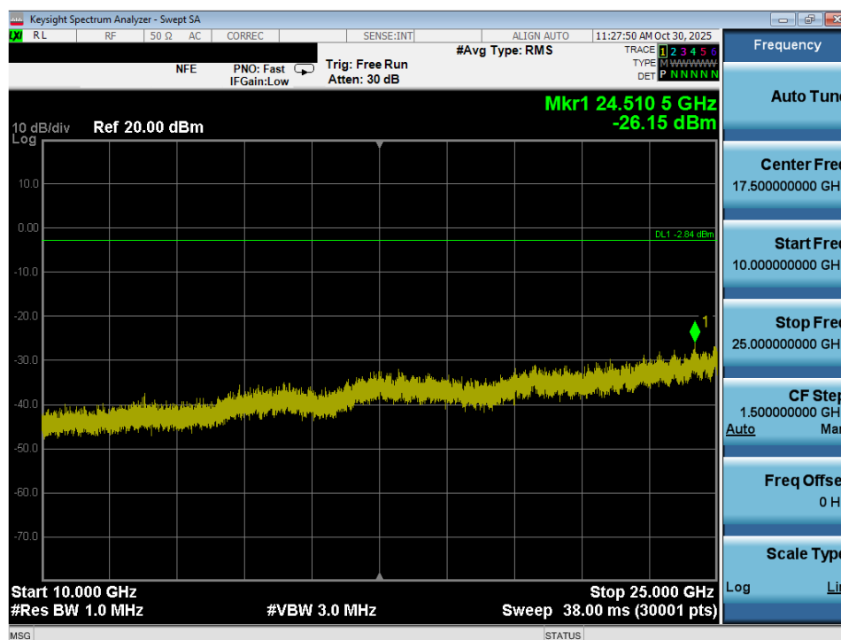
Plot 7-39. Conducted Spurious Plot (Bluetooth, 3Mbps – Ch. 39) – Ant 1
