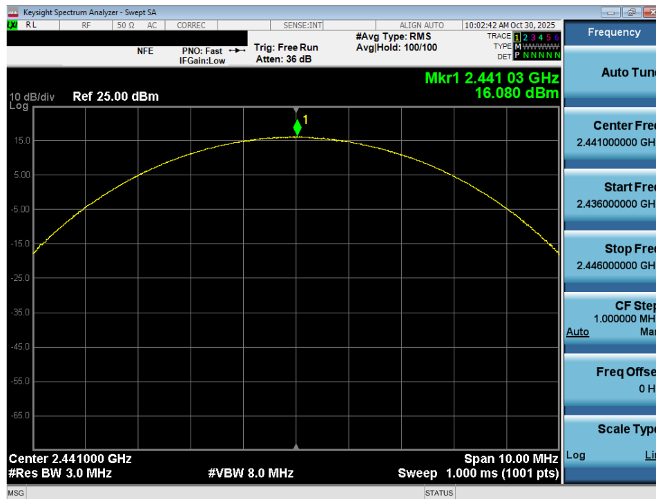
Plot 7-17. Peak Conducted Power (3Mbps – Ch. 39) – Ant 1
