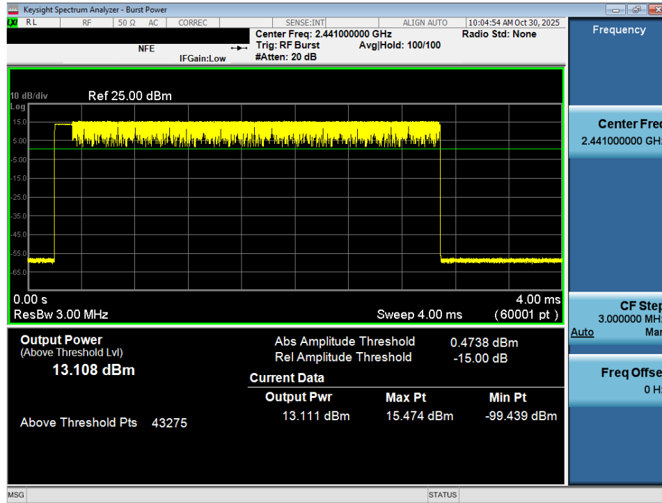
Plot 7-23. Average Conducted Power (2Mbps – Ch. 39) – Ant 1
