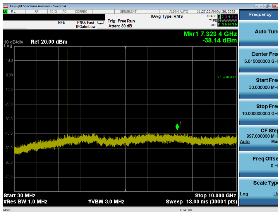
Plot 7-38. Conducted Spurious Plot (Bluetooth, 3Mbps – Ch. 39) – Ant 1
