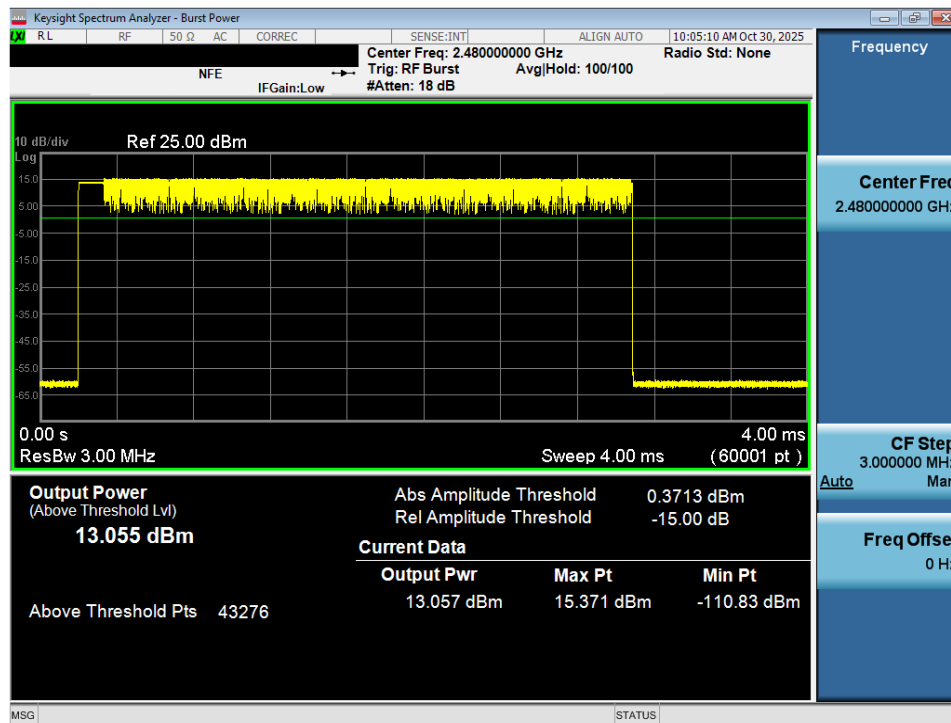
Plot 7-24. Average Conducted Power (2Mbps – Ch. 78) – Ant 1
