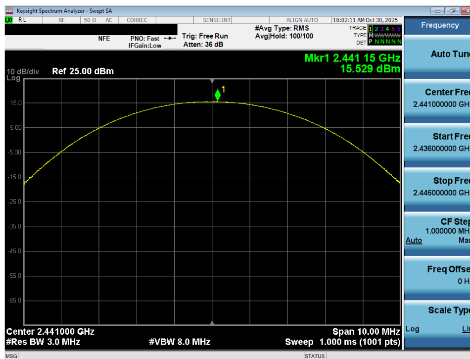
Plot 7-14. Peak Conducted Power (2Mbps – Ch. 39) – Ant 1
