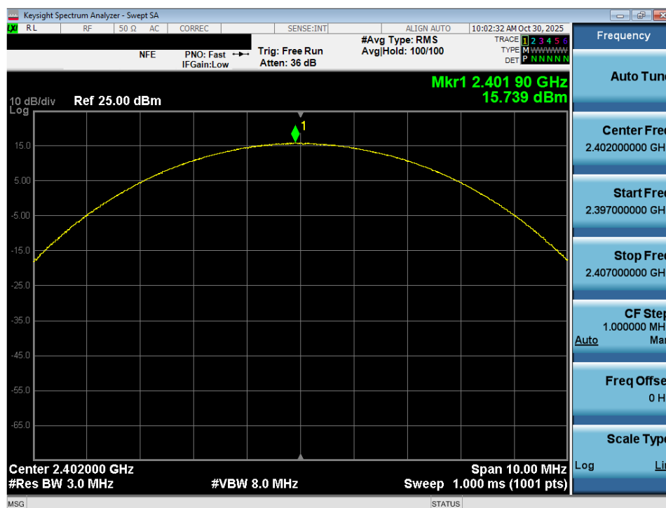
Plot 7-16. Peak Conducted Power (3Mbps – Ch. 0) – Ant 1
