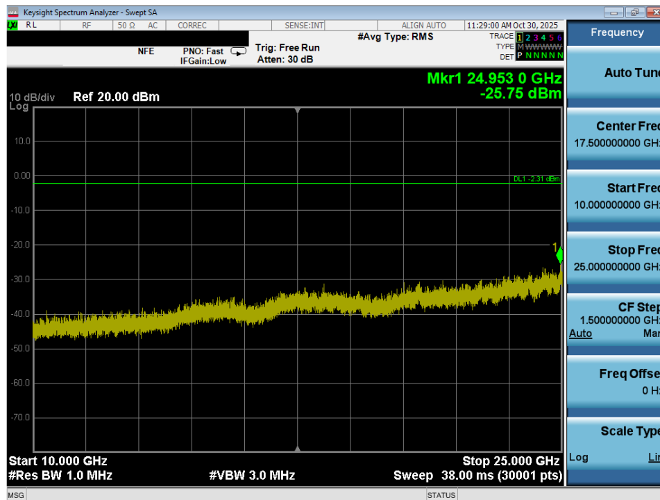
Plot 7-41. Conducted Spurious Plot (Bluetooth, 3Mbps – Ch. 78) – Ant 1
