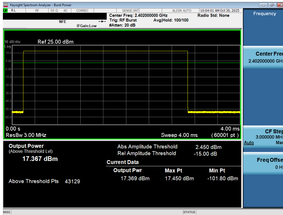
Plot 7-19. Average Conducted Power (1Mbps – Ch. 0) – Ant 1
