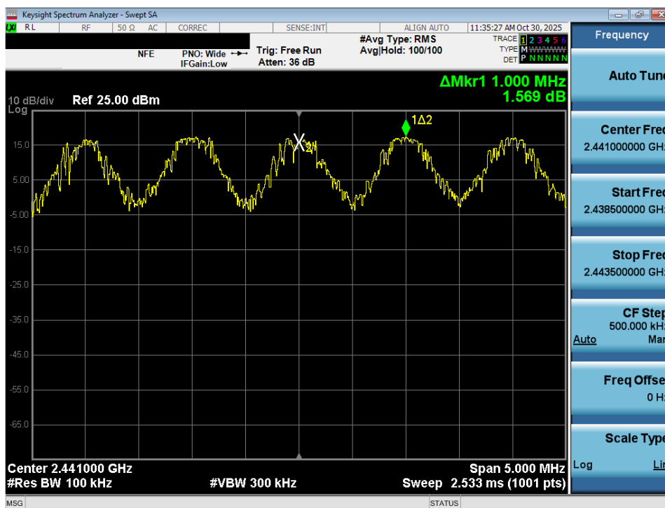
Plot 7-32. Channel Spacing Plot (Bluetooth) – Ant 1
