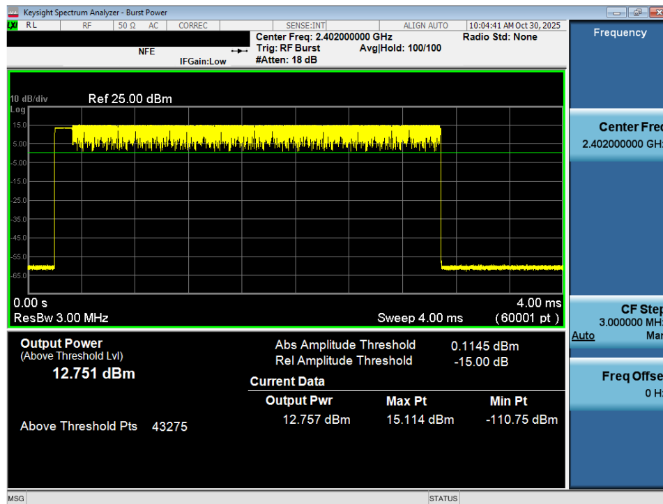
Plot 7-22. Average Conducted Power (2Mbps – Ch. 0) – Ant 1
