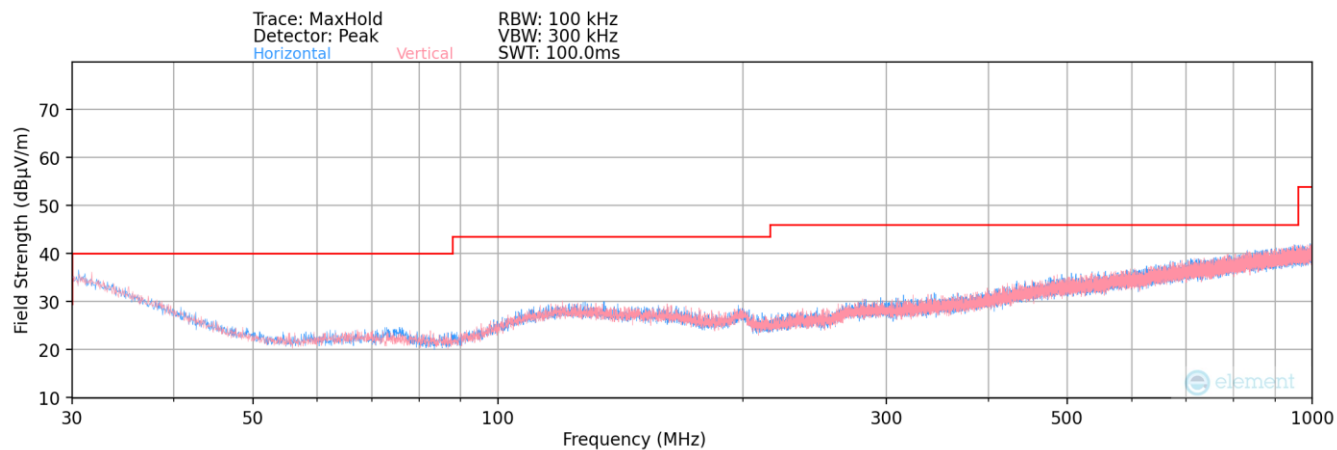
Plot 7-48. Radiated Spurious Plot below 1GHz – Ant 1
