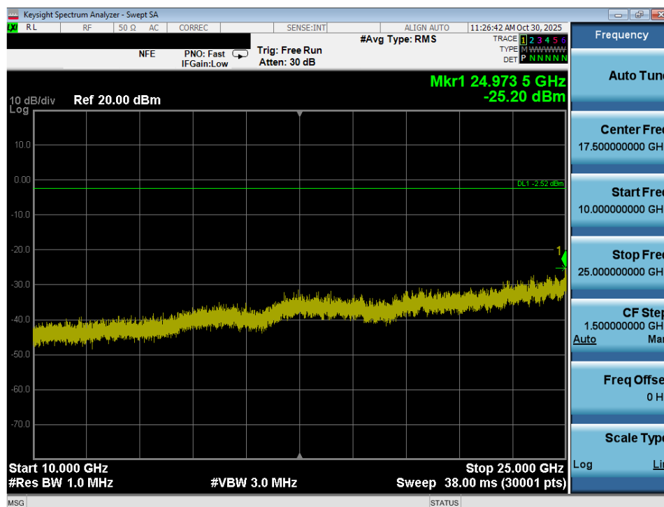
Plot 7-37. Conducted Spurious Plot (Bluetooth, 3Mbps - Ch. 0) - Ant 1
