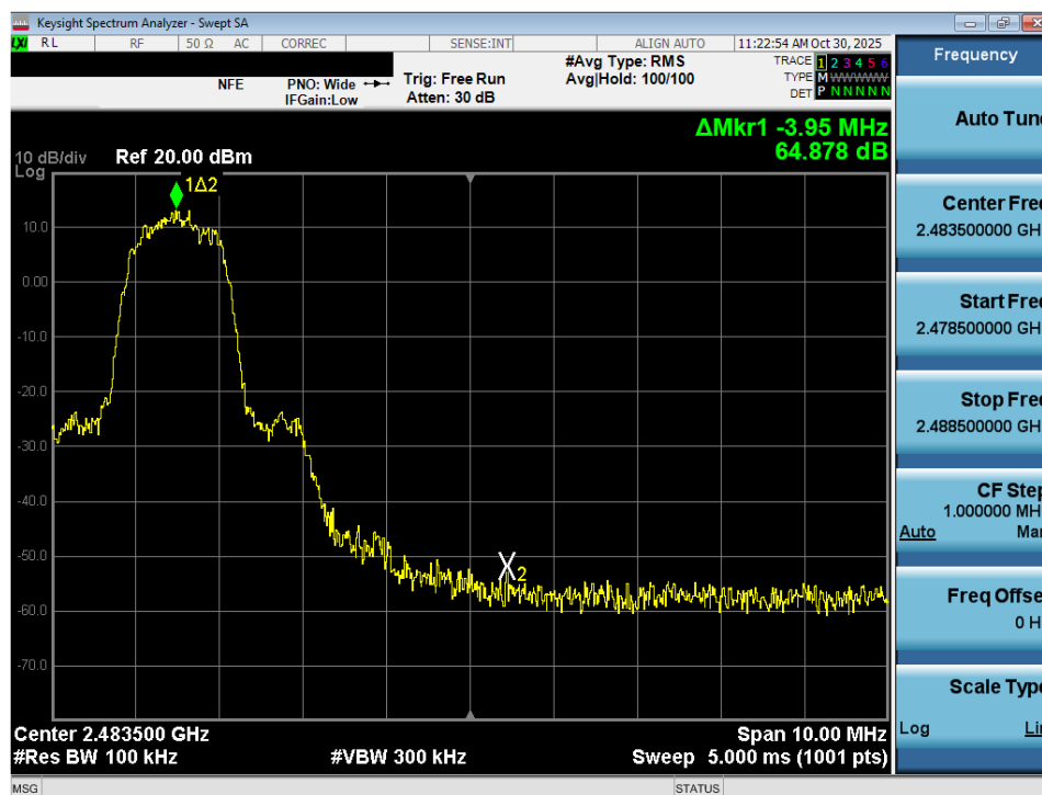
Plot 7-29. Band Edge Plot (Bluetooth with Hopping Disabled, 3 Mbps – Ch. 78) – Ant 1
