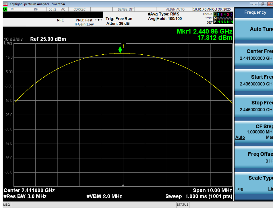
Plot 7-11. Peak Conducted Power (1Mbps – Ch. 39) – Ant 1
