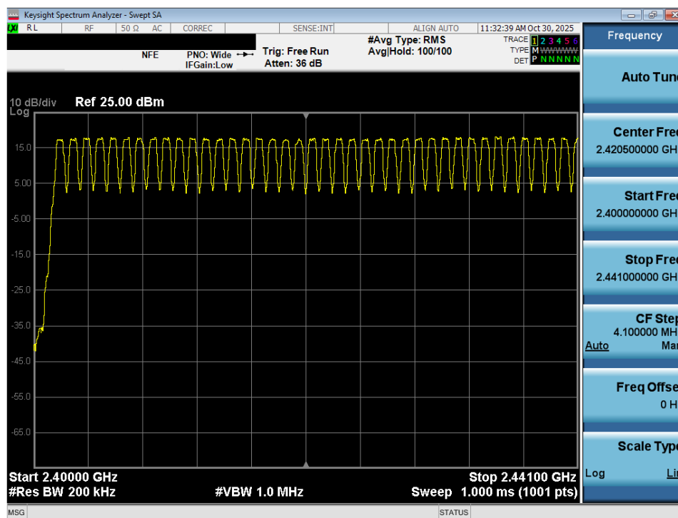
Plot 7-34. Low End Spectrum Channel Hopping Plot (Bluetooth) – Ant 1
