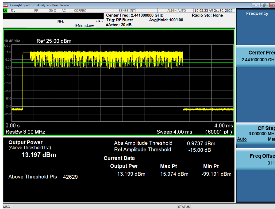
Plot 7-26. Average Conducted Power (3Mbps – Ch. 39) – Ant 1
