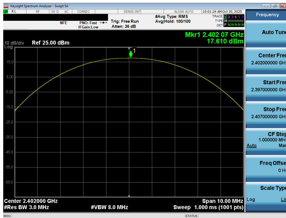
Plot 7-10. Peak Conducted Power (1Mbps – Ch. 0) – Ant 1
