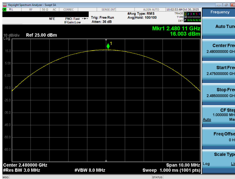
Plot 7-18. Peak Conducted Power (3Mbps – Ch. 78) – Ant 1
