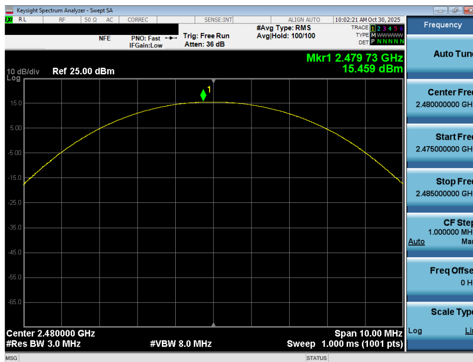
Plot 7-15. Peak Conducted Power (2Mbps – Ch. 78) – Ant 1
