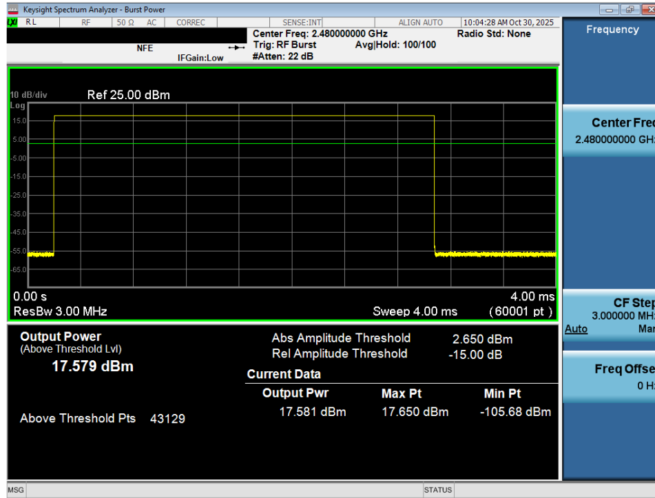
Plot 7-21. Average Conducted Power (1Mbps – Ch. 78) – Ant 1
