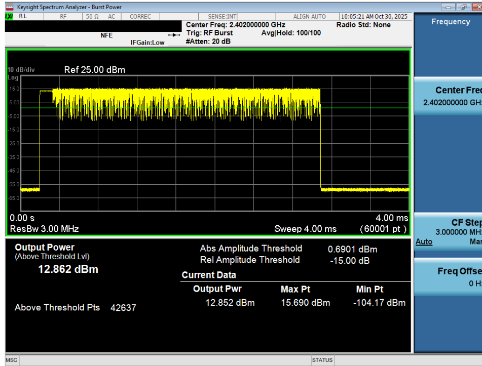
Plot 7-25. Average Conducted Power (3Mbps – Ch. 0) – Ant 1
