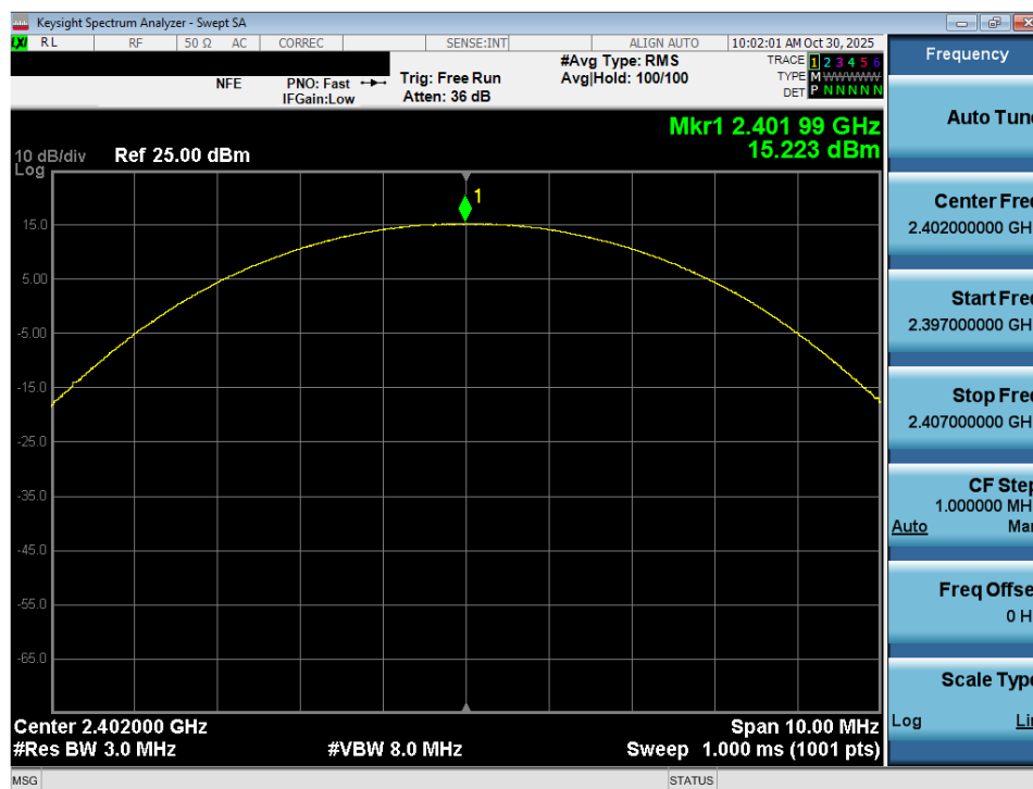
Plot 7-13. Peak Conducted Power (2Mbps – Ch. 0) – Ant 1
