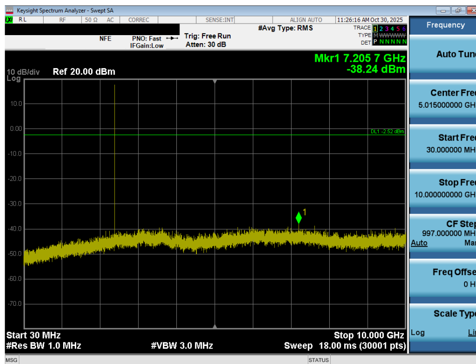
Plot 7-36. Conducted Spurious Plot (Bluetooth, 3Mbps - Ch. 0) - Ant 1
