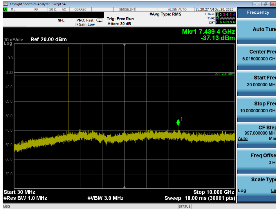
Plot 7-40. Conducted Spurious Plot (Bluetooth, 3Mbps – Ch. 78) – Ant 1
