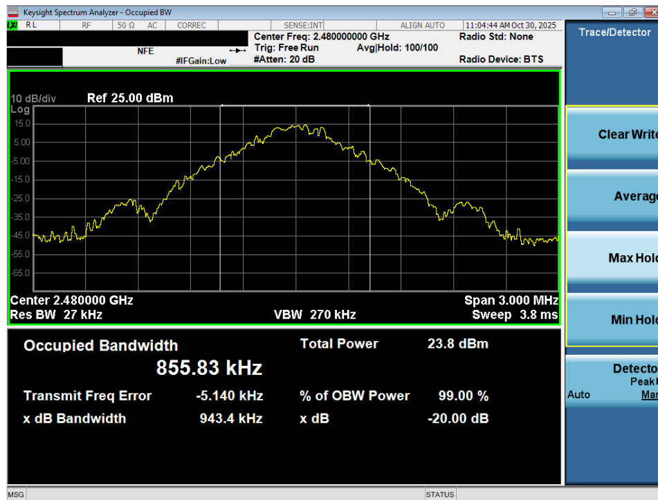
Plot 7-3. 20dB Bandwidth Plot (Bluetooth, 1Mbps – Ch. 78) – Ant 1
