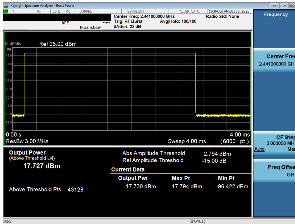
Plot 7-20. Average Conducted Power (1Mbps – Ch. 39) – Ant 1
