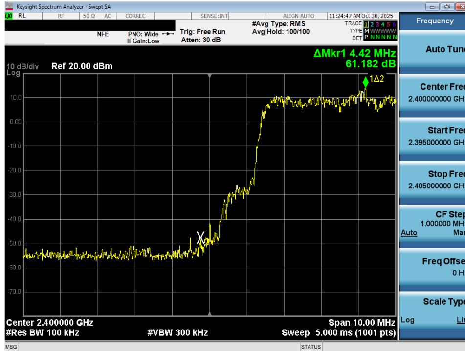
Plot 7-30. Band Edge Plot (Bluetooth with Hopping Enabled, 3 Mbps) – Ant 1
