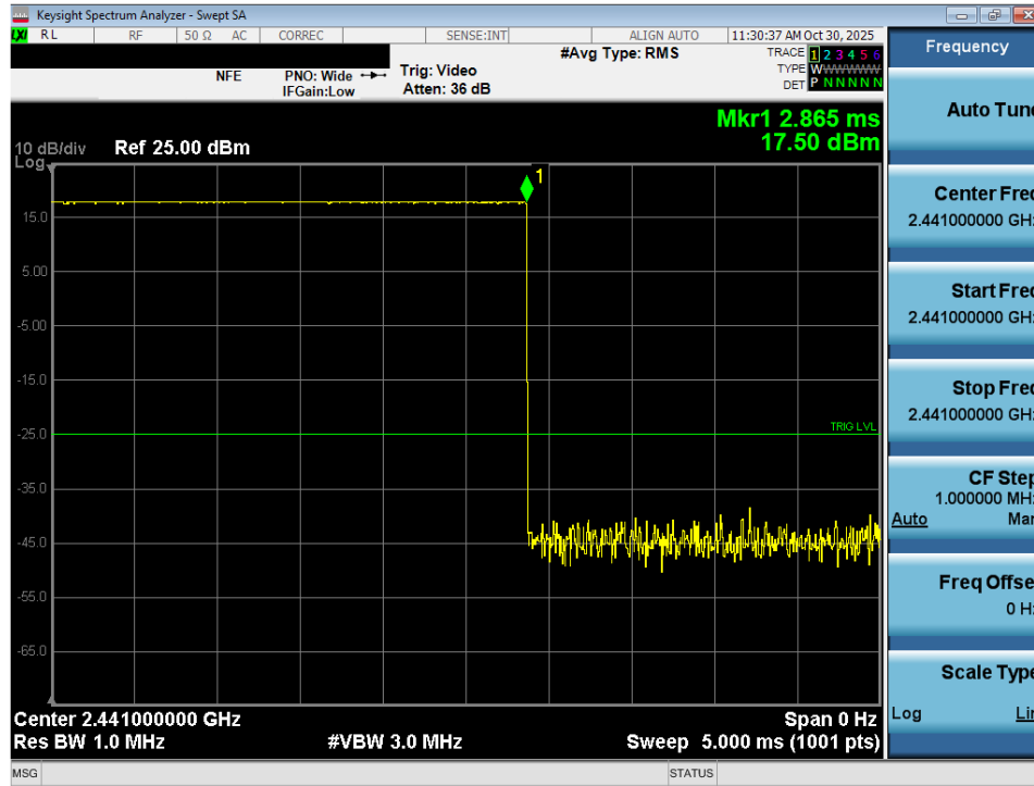
Plot 7-33. Time of Occupancy Plot (Bluetooth) – Ant 1
