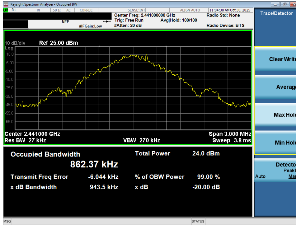
Plot 7-2. 20dB Bandwidth Plot (Bluetooth, 1Mbps – Ch. 39) – Ant 1
