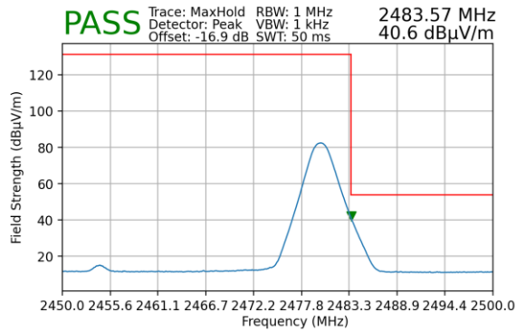
Plot 9-2. Radiated Restricted Upper Band Edge Measurement (Average) – Spot-check
