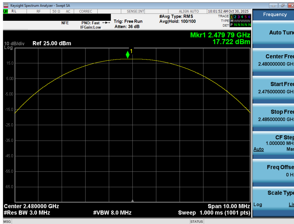
Plot 7-12. Peak Conducted Power (1Mbps – Ch. 78) – Ant 1
