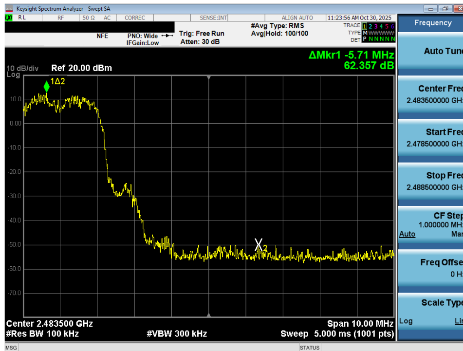
Plot 7-31. Band Edge Plot (Bluetooth with Hopping Enabled, 3 Mbps) – Ant 1
