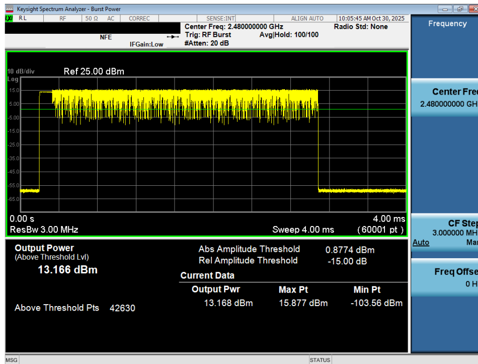
Plot 7-27. Average Conducted Power (3Mbps – Ch. 78) – Ant 1
