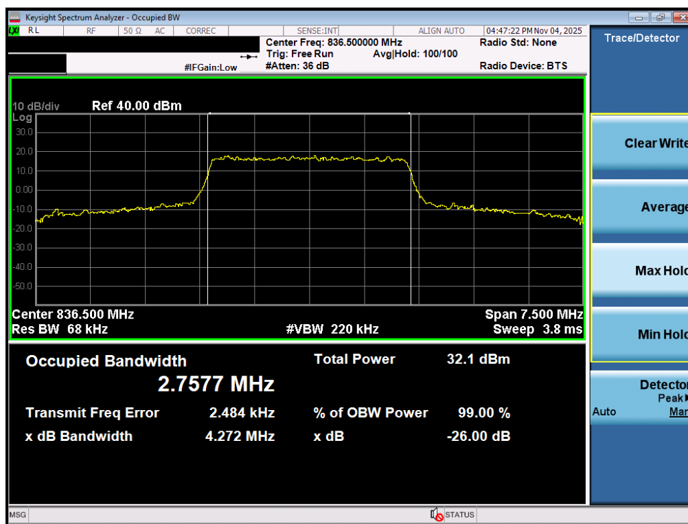
Plot 7-7. Occupied Bandwidth Plot (LTE Band 26/5 - 3MHz QPSK - Full RB - Ant1)
