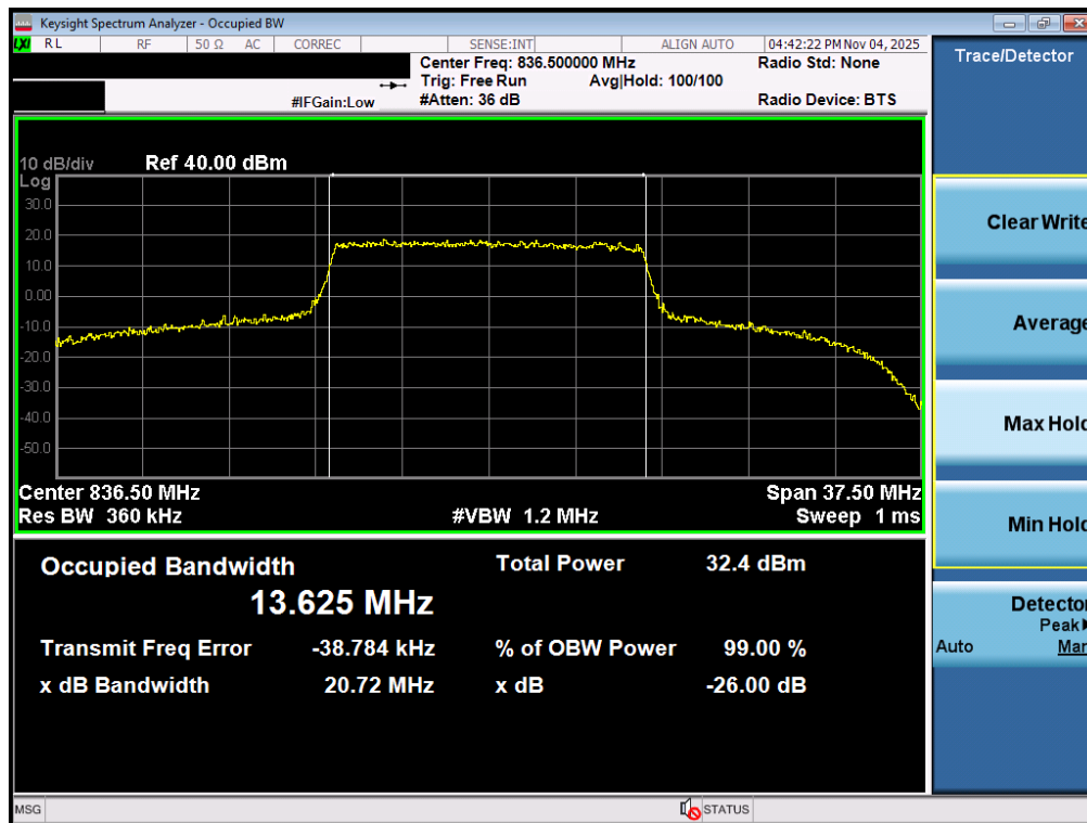
Plot 7-2. Occupied Bandwidth Plot (LTE Band 26 - 15MHz 16-QAM - Full RB - Ant1)
