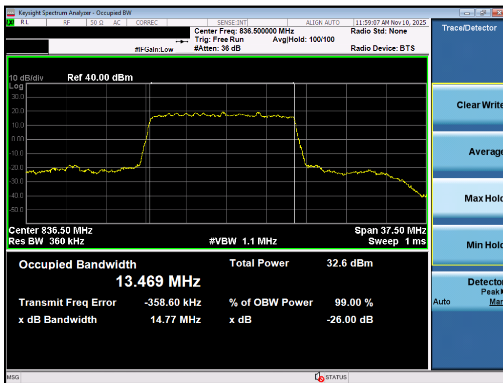
Plot 7-14. Occupied Bandwidth Plot (NR Band n5 - 15MHz \pi/2 BPSK - Full RB - Ant1)
