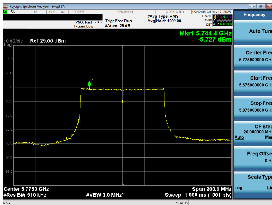
Plot 7-104. Power Spectral Density Plot MIMO ANT2 (80MHz BW 802.11ac (UNII Band 3) – Ch. 155)
