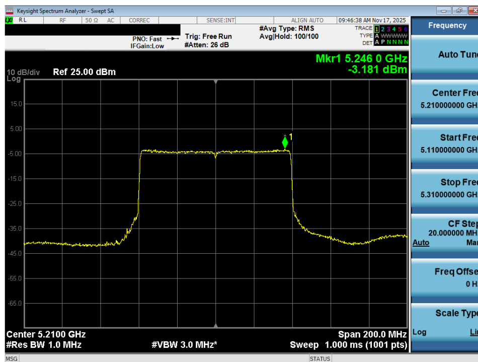
Plot 7-98. Power Spectral Density Plot MIMO ANT2 (80MHz BW 802.11ax (UNII Band 1) – Ch. 42)
