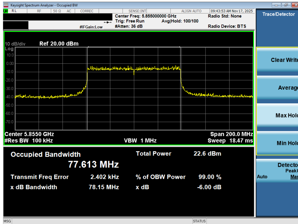
Plot 7-42. 6dB Bandwidth Plot MIMO ANT2 (80MHz BW 802.11ax (UNII Band 3/4) – Ch. 171)
