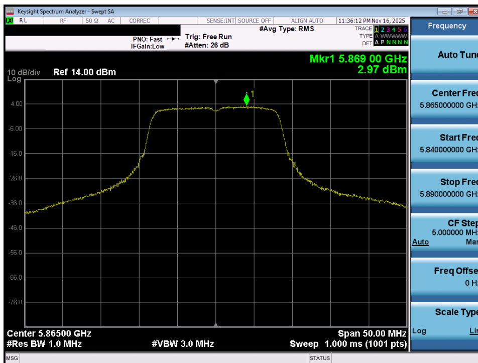
Plot 7-85. Power Spectral Density Plot MIMO ANT1 (802.11a (UNII Band 4) – Ch. 173)
