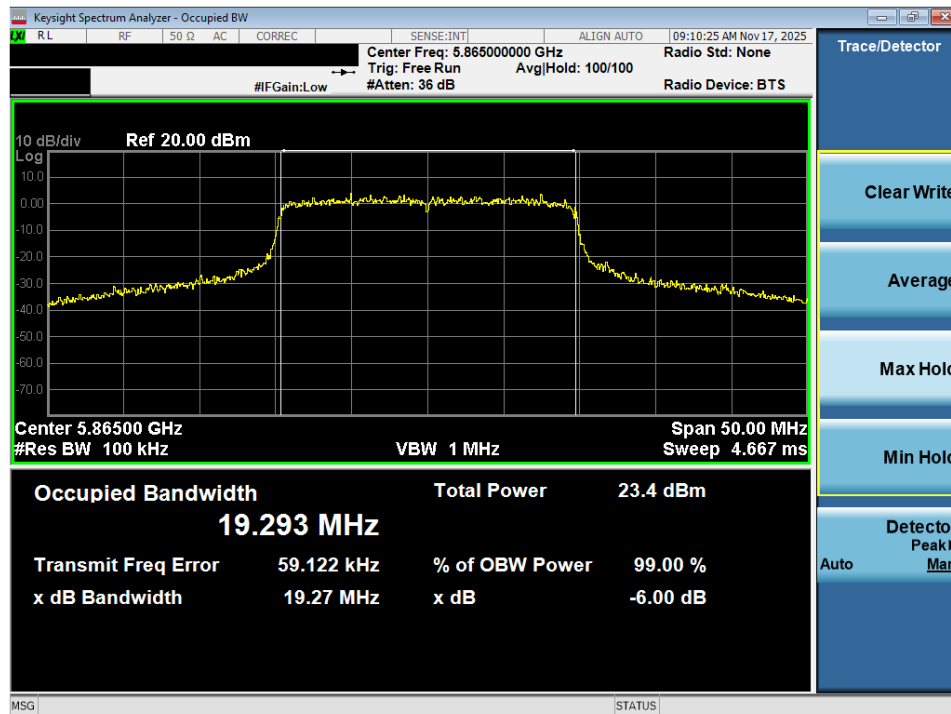
Plot 7-38. 6dB Bandwidth Plot MIMO ANT2 (20MHz BW 802.11ax (UNII Band 3/4) – Ch. 173)
