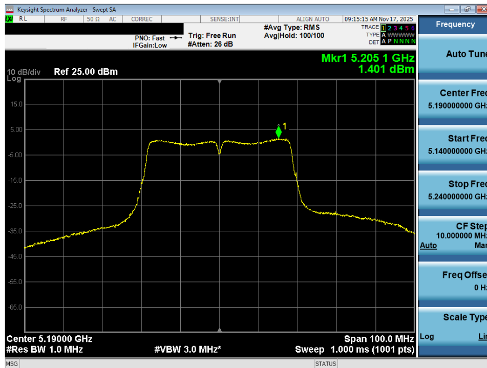
Plot 7-95. Power Spectral Density Plot MIMO ANT2 (40MHz BW 802.11n (UNII Band 1) – Ch. 38)
