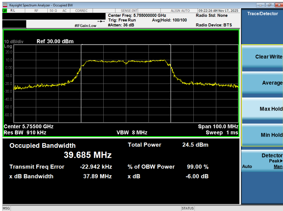
Plot 7-60. OBW Plot MIMO ANT2 (40MHz BW 802.11n (UNII Band 3) – Ch. 151)
