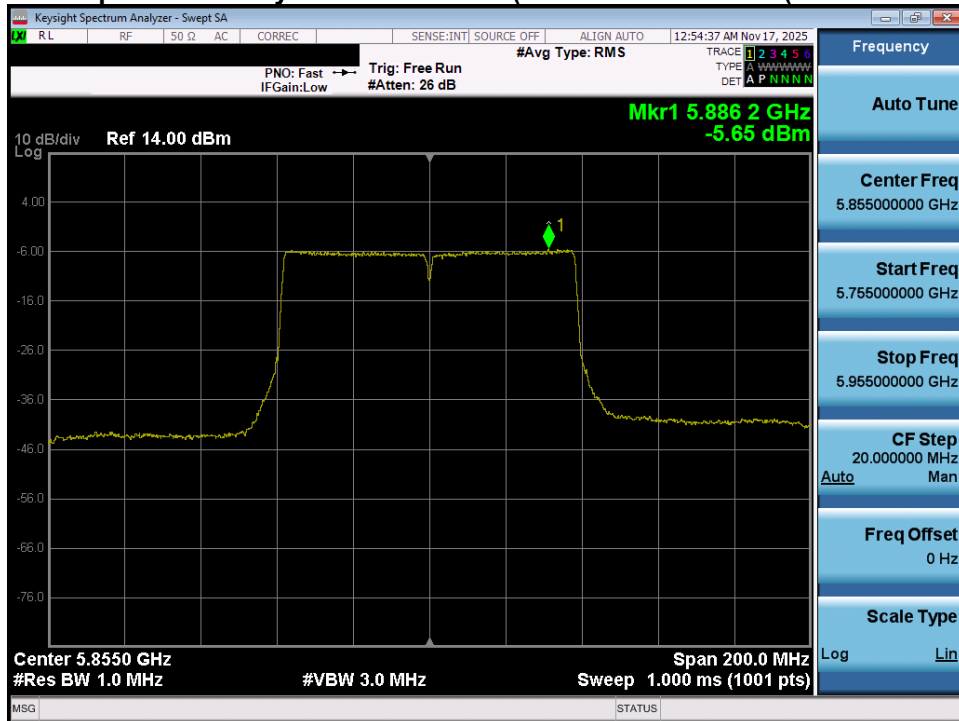
Plot 7-90. Power Spectral Density Plot MIMO ANT1 (80MHz BW 802.11ac (UNII Band 3/4) – Ch. 171)
