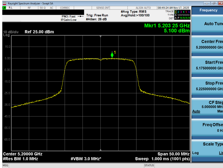
Plot 7-94. Power Spectral Density Plot MIMO ANT2 (20MHz BW 802.11ax (UNII Band 1) – Ch. 40)
