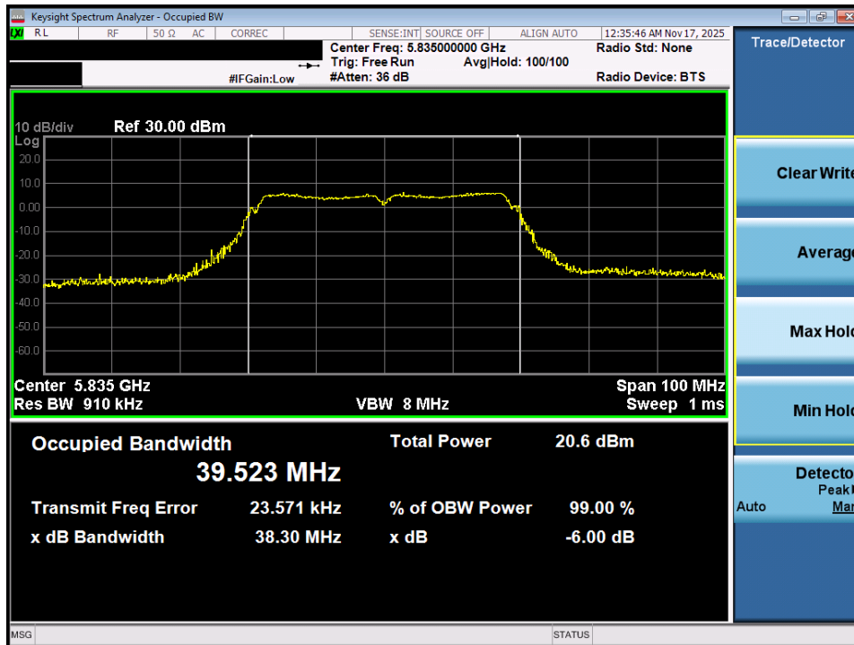
Plot 7-53. OBW Plot MIMO ANT1 (40MHz BW 802.11n (UNII Band 3/4) – Ch. 167)
