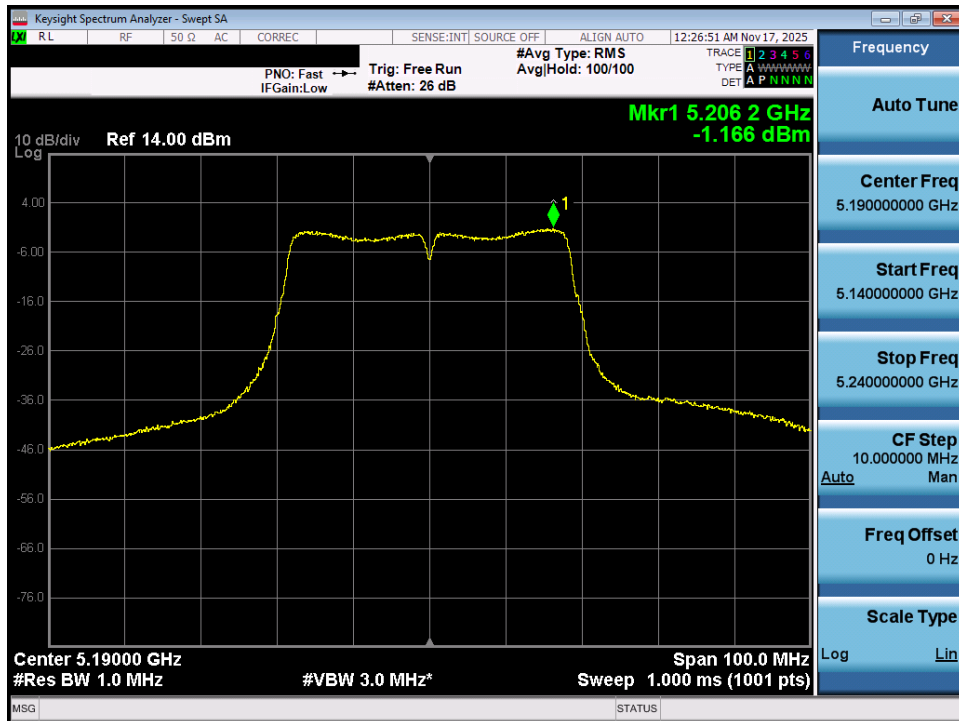
Plot 7-74. Power Spectral Density Plot MIMO ANT1 (40MHz BW 802.11n (UNII Band 1) – Ch. 38)
