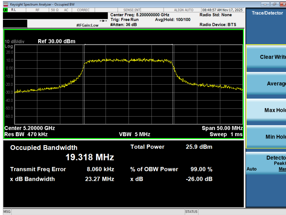
Plot 7-10. 26dB Bandwidth Plot MIMO ANT2 (20MHz BW 802.11ax (UNII Band 1) – Ch. 40)
