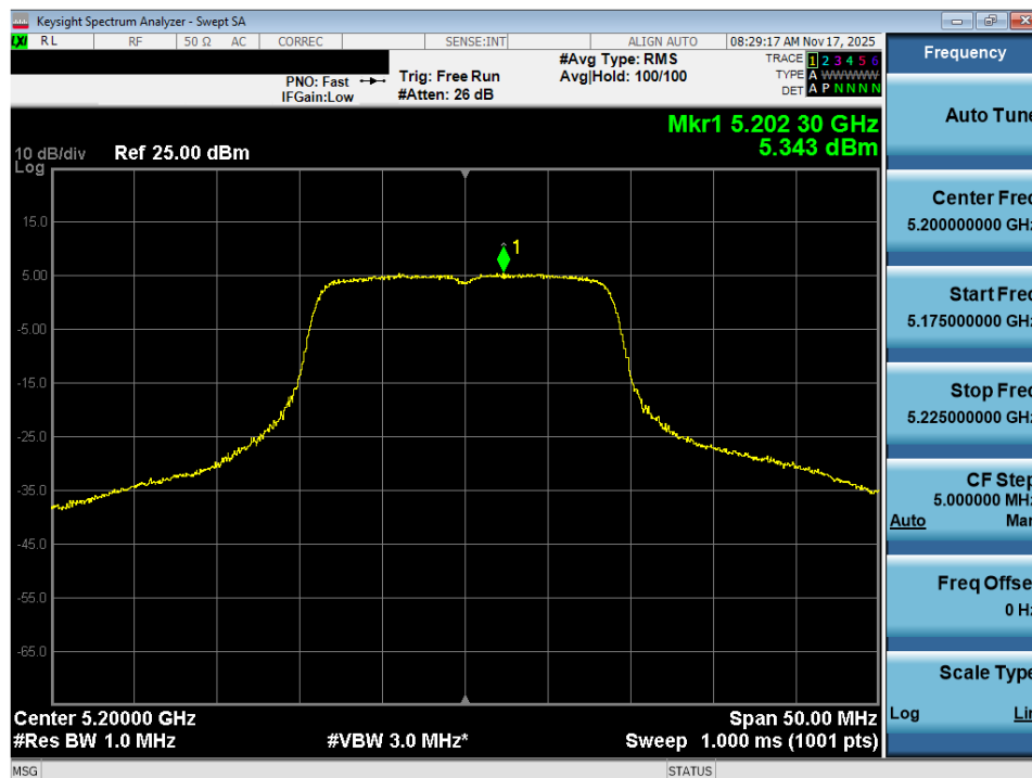
Plot 7-93. Power Spectral Density Plot MIMO ANT2 (20MHz BW 802.11n (UNII Band 1) – Ch. 40)
