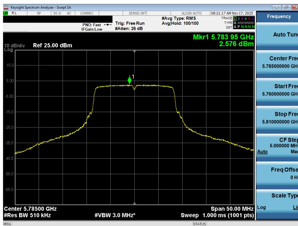
Plot 7-99. Power Spectral Density Plot MIMO ANT2 (802.11a (UNII Band 3) – Ch. 157)
