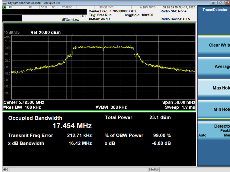
Plot 7-29. 6dB Bandwidth Plot MIMO ANT2 (802.11a (UNII Band 3) – Ch. 157)
