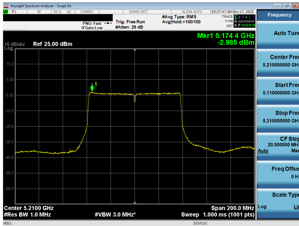
Plot 7-97. Power Spectral Density Plot MIMO ANT2 (80MHz BW 802.11ac (UNII Band 1) – Ch. 42)
