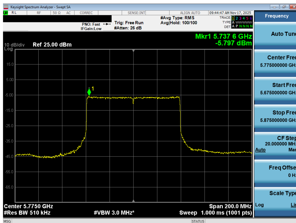
Plot 7-105. Power Spectral Density Plot MIMO ANT2 (80MHz BW 802.11ax (UNII Band 3) – Ch. 155)
