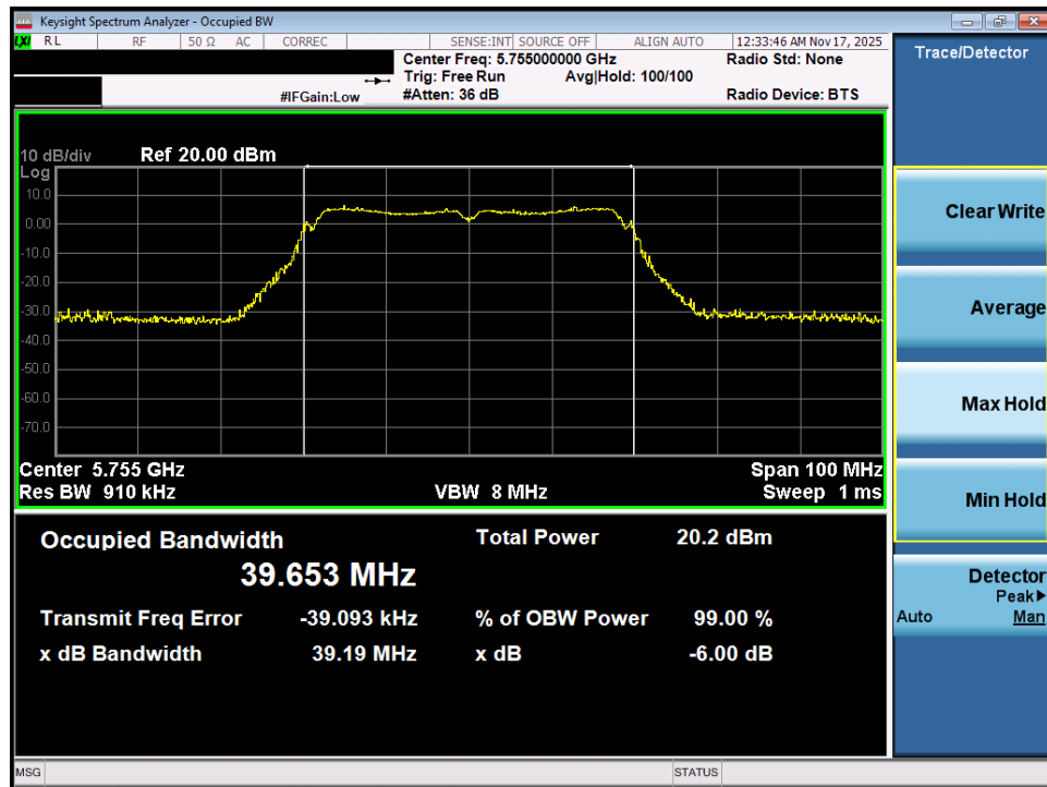
Plot 7-46. OBW Plot MIMO ANT1 (40MHz BW 802.11n (UNII Band 3) – Ch. 151)
