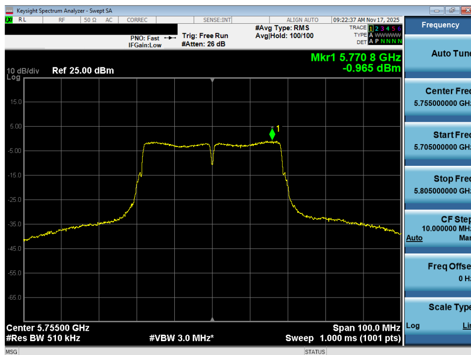
Plot 7-102. Power Spectral Density Plot MIMO ANT2 (40MHz BW 802.11n (UNII Band 3) – Ch. 151)
