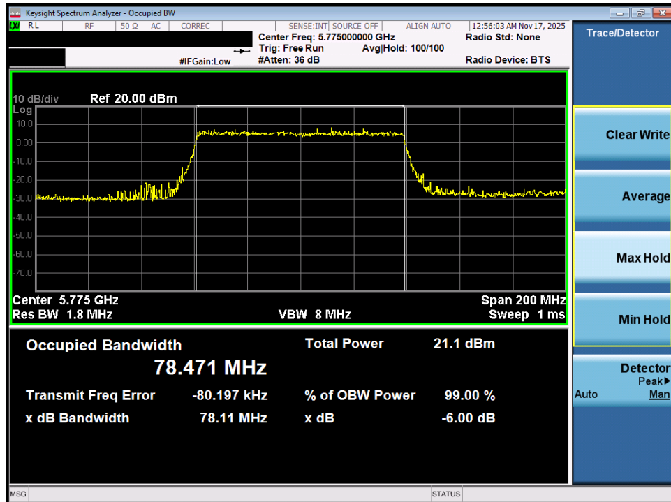
Plot 7-49. OBW Plot MIMO ANT1 (80MHz BW 802.11ax (UNII Band 3) – Ch. 155)
