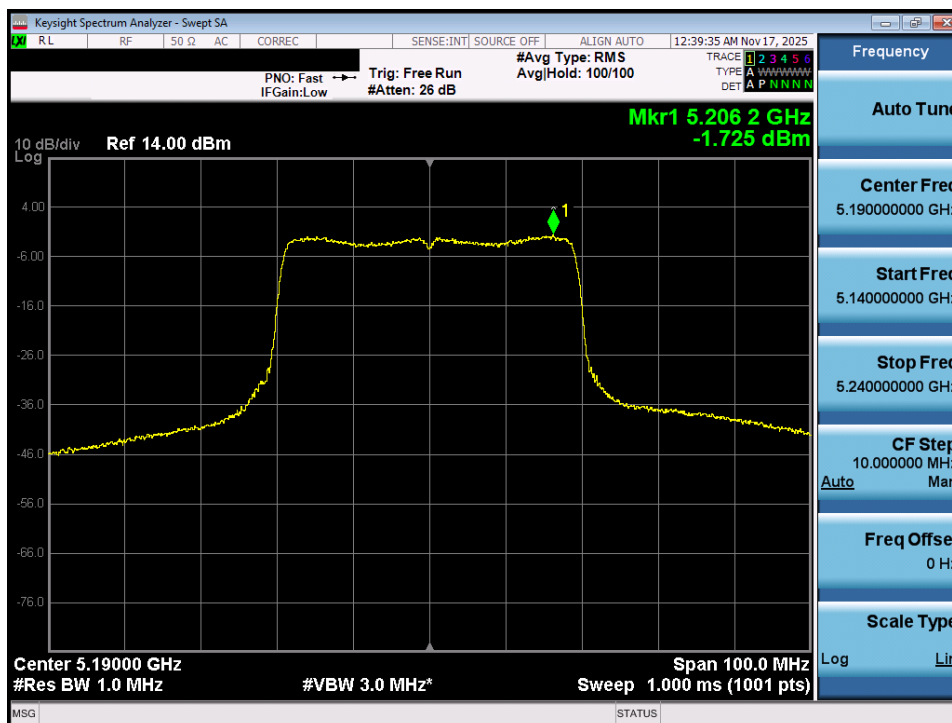
Plot 7-75. Power Spectral Density Plot MIMO ANT1 (40MHz BW 802.11ax (UNII Band 1) – Ch. 38)
