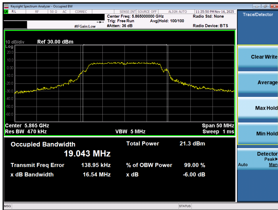
Plot 7-50. OBW Plot MIMO ANT1 (802.11a (UNII Band 4) – Ch. 173)
