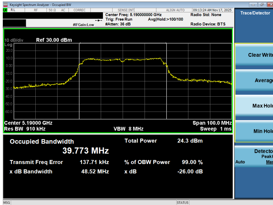
Plot 7-11. 26dB Bandwidth Plot MIMO ANT2 (40MHz BW 802.11n (UNII Band 1) – Ch. 38)
