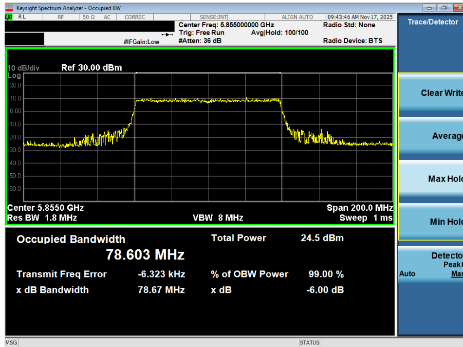
Plot 7-70. OBW Plot MIMO ANT2 (80MHz BW 802.11ax (UNII Band 3/4) – Ch. 171)
