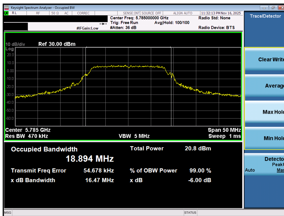
Plot 7-43. OBW Plot MIMO ANT1 (802.11a (UNII Band 3) – Ch. 157)
