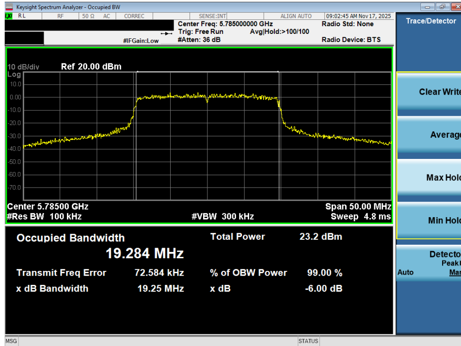
Plot 7-31. 6dB Bandwidth Plot MIMO ANT2 (20MHz BW 802.11ax (UNII Band 3) – Ch. 157)
