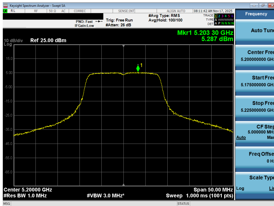
Plot 7-92. Power Spectral Density Plot MIMO ANT2 (802.11a (UNII Band 1) – Ch. 40)
