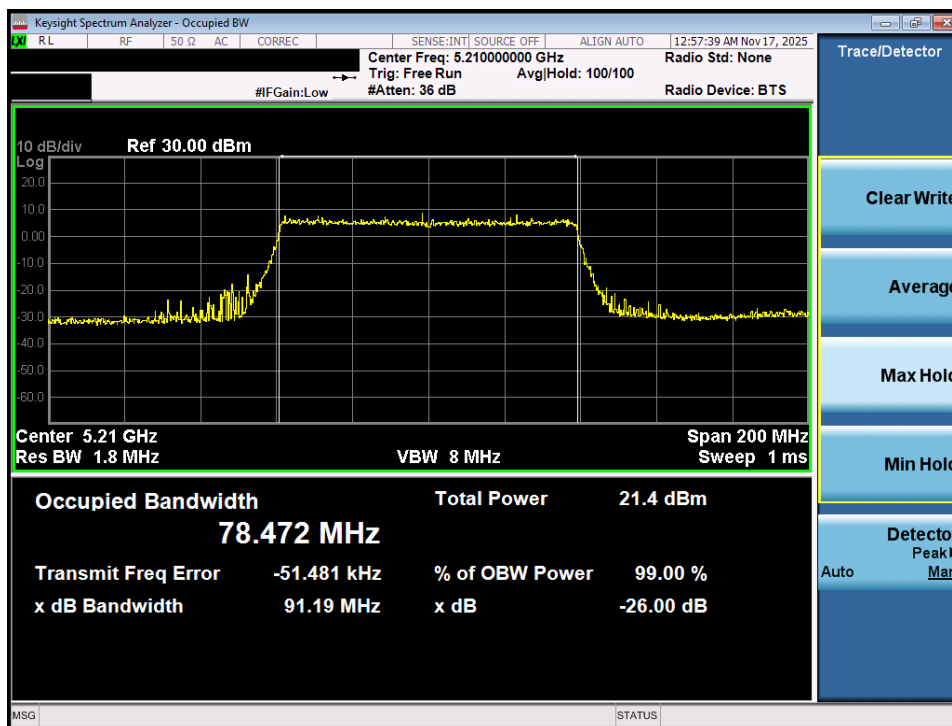
Plot 7-7. 26dB Bandwidth Plot MIMO ANT1 (80MHz BW 802.11ax (UNII Band 1) – Ch. 42)
