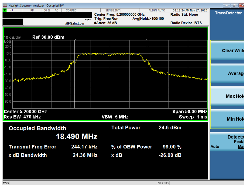
Plot 7-8. 26dB Bandwidth Plot MIMO ANT2 (802.11a (UNII Band 1) – Ch. 40)
