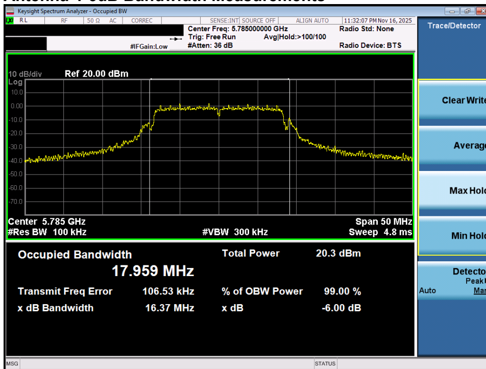
Plot 7-15. 6dB Bandwidth Plot MIMO ANT1 (802.11a (UNII Band 3) – Ch. 157)
