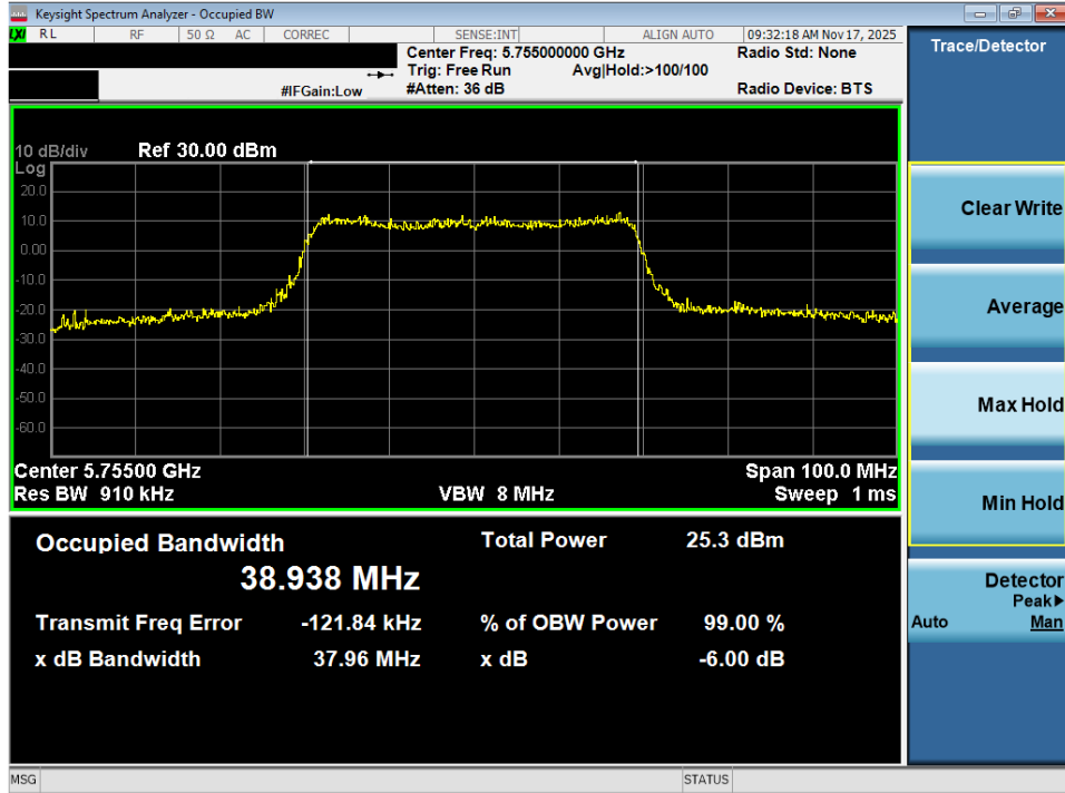
Plot 7-61. OBW Plot MIMO ANT2 (40MHz BW 802.11ax (UNII Band 3) – Ch. 151)
