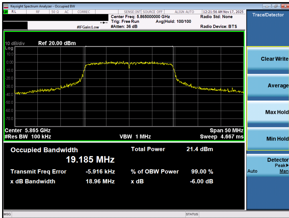
Plot 7-24. 6dB Bandwidth Plot MIMO ANT1 (20MHz BW 802.11ax (UNII Band 4) – Ch. 173)
