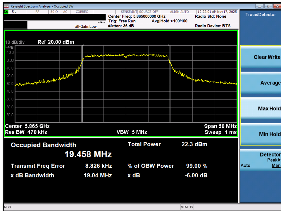
Plot 7-52. OBW Plot MIMO ANT1 (20MHz BW 802.11ax (UNII Band 4) – Ch. 173)
