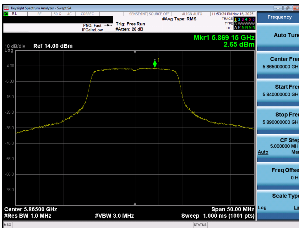
Plot 7-86. Power Spectral Density Plot MIMO ANT1 (20MHz BW 802.11n (UNII Band 4) – Ch. 173)
