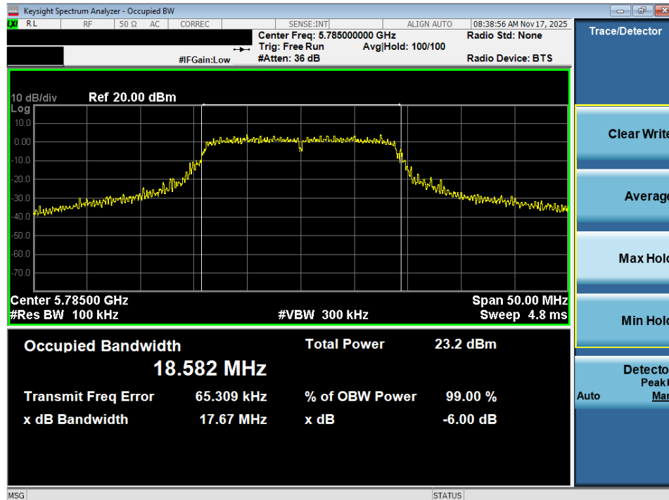
Plot 7-30. 6dB Bandwidth Plot MIMO ANT2 (20MHz BW 802.11n (UNII Band 3) – Ch. 157)
