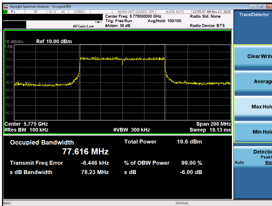
Plot 7-21. 6dB Bandwidth Plot MIMO ANT1 (80MHz BW 802.11ax (UNII Band 3) – Ch. 155)
