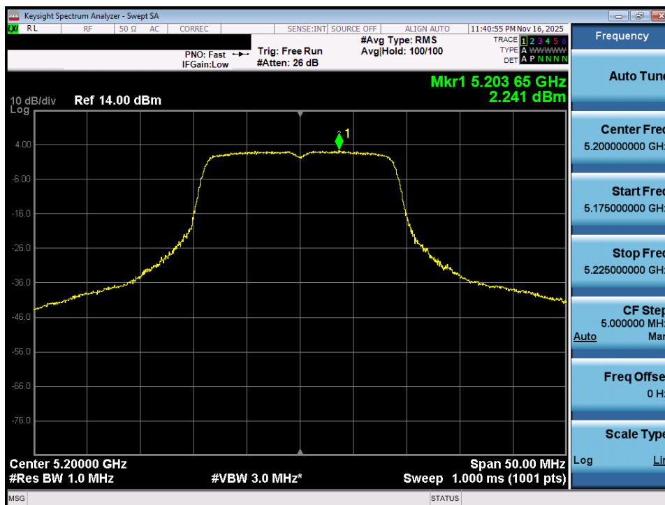
Plot 7-72. Power Spectral Density Plot MIMO ANT1 (20MHz BW 802.11n (UNII Band 1) – Ch. 40)
