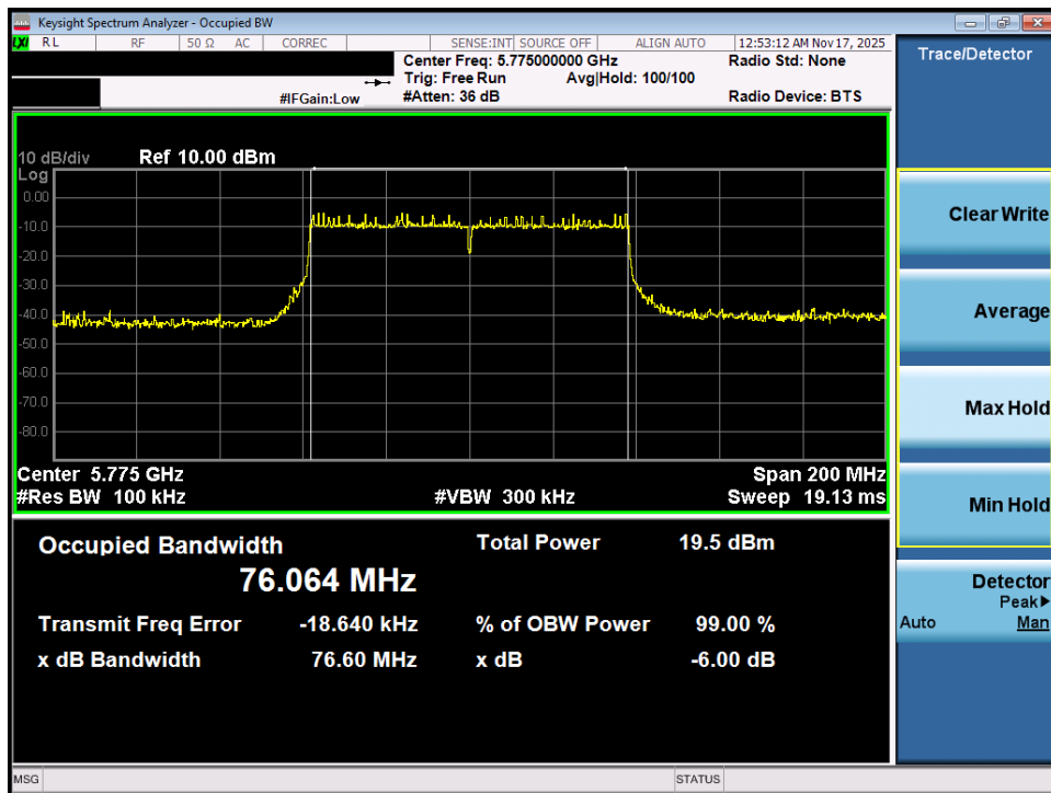
Plot 7-20. 6dB Bandwidth Plot MIMO ANT1 (80MHz BW 802.11ac (UNII Band 3) – Ch. 155)
