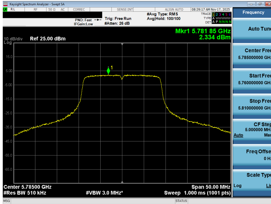
Plot 7-100. Power Spectral Density Plot MIMO ANT2 (20MHz BW 802.11n (UNII Band 3) – Ch. 157)
