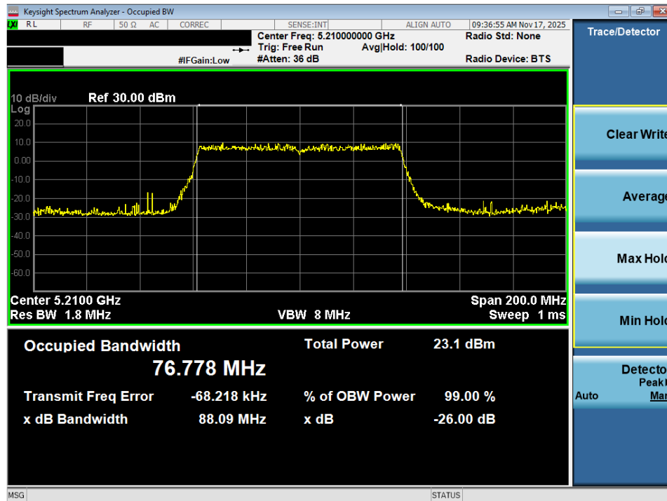
Plot 7-13. 26dB Bandwidth Plot MIMO ANT2 (80MHz BW 802.11ac (UNII Band 1) – Ch. 42)
