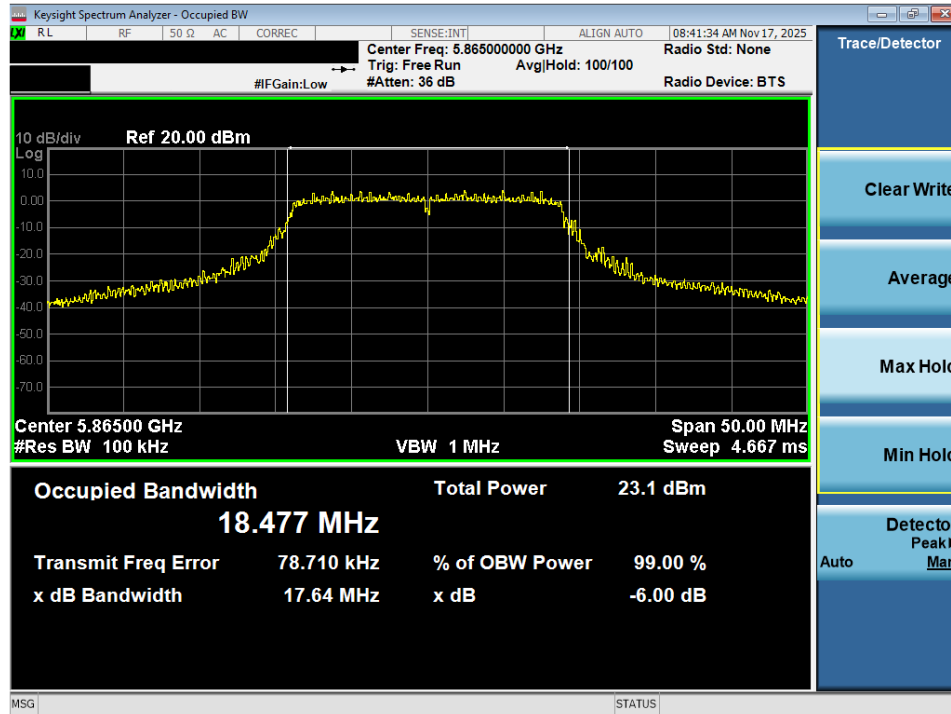
Plot 7-37. 6dB Bandwidth Plot MIMO ANT2 (20MHz BW 802.11n (UNII Band 3/4) – Ch. 173)
