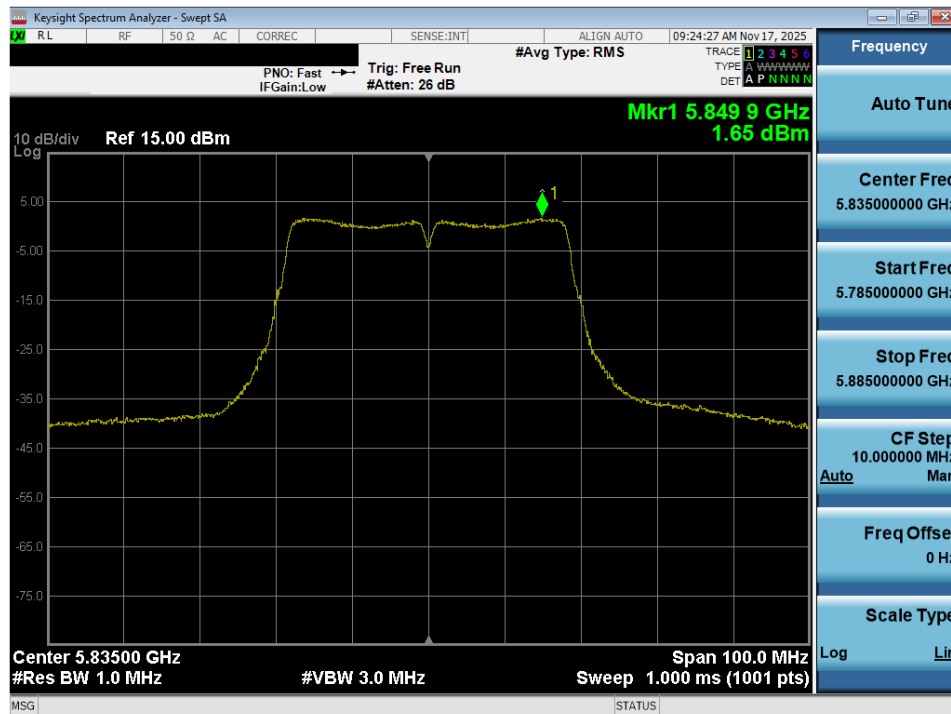
Plot 7-109. Power Spectral Density Plot MIMO ANT2 (40MHz BW 802.11n (UNII Band 3/4) – Ch. 167)
