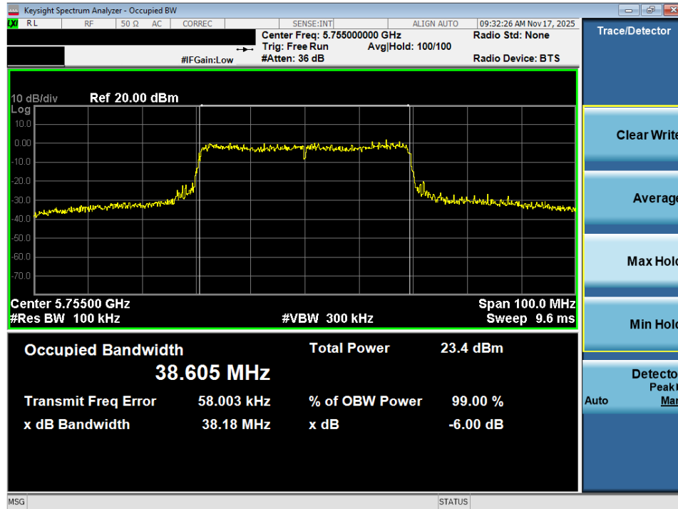
Plot 7-33. 6dB Bandwidth Plot MIMO ANT2 (40MHz BW 802.11ax (UNII Band 3) – Ch. 151)
