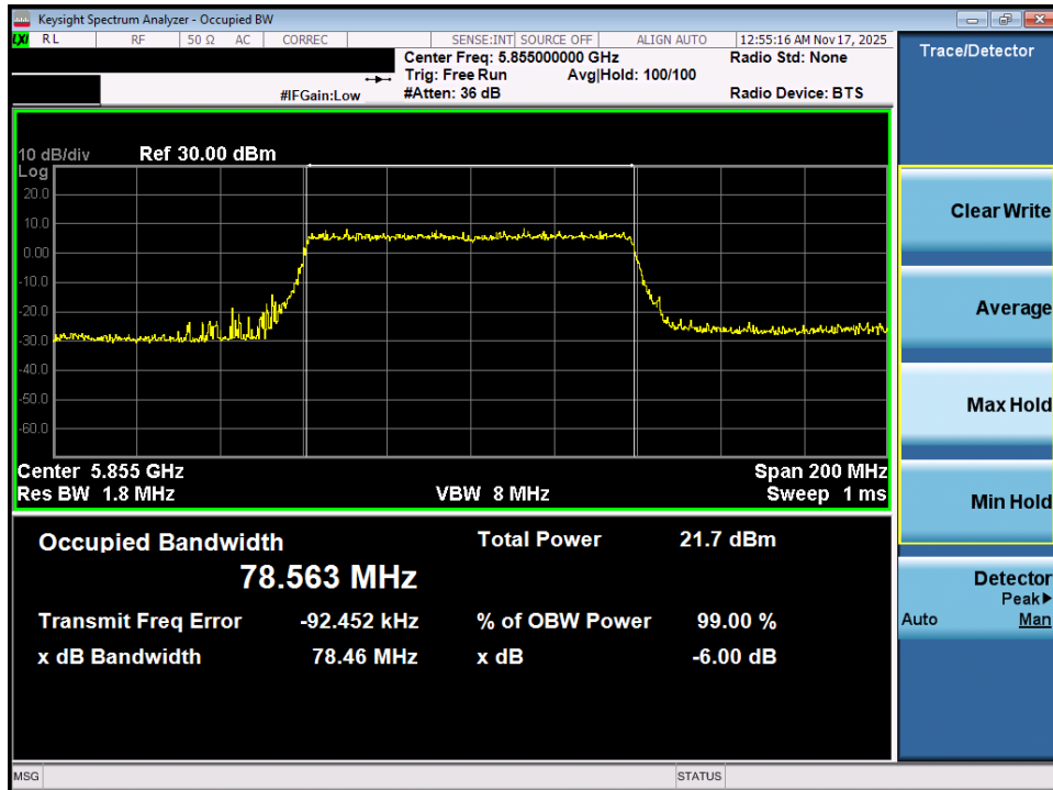
Plot 7-56. OBW Plot MIMO ANT1 (80MHz BW 802.11ax (UNII Band 3/4) – Ch. 171)
