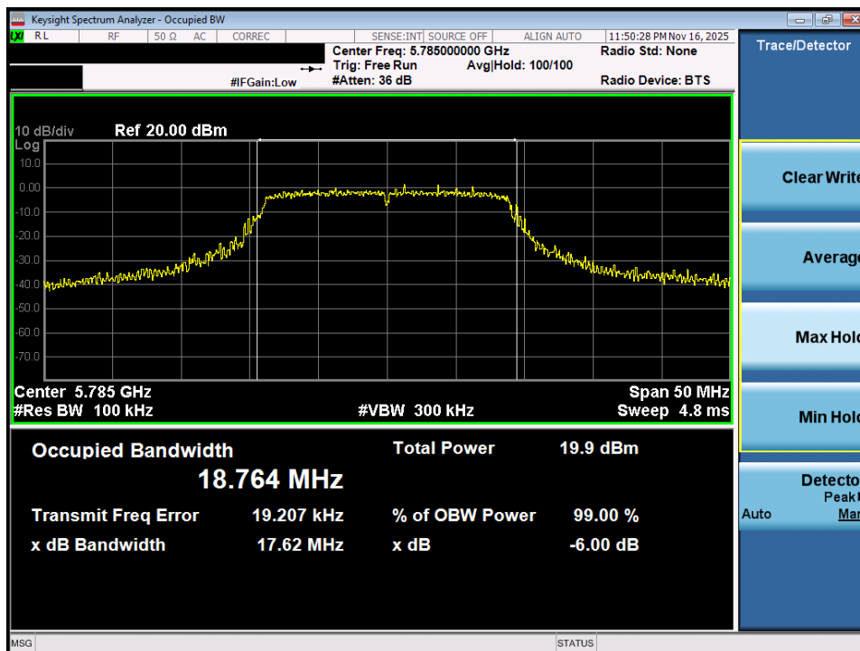
Plot 7-16. 6dB Bandwidth Plot MIMO ANT1 (20MHz BW 802.11n (UNII Band 3) – Ch. 157)
