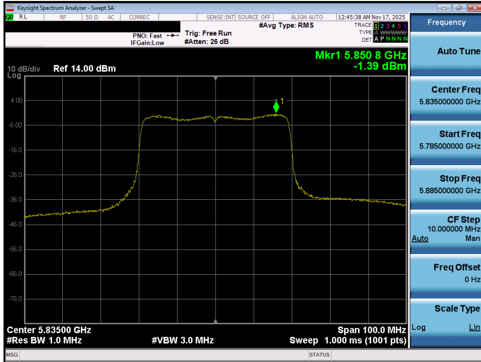
Plot 7-89. Power Spectral Density Plot MIMO ANT1 (40MHz BW 802.11ax (UNII Band 3/4) – Ch. 167)
