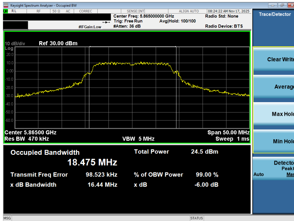
Plot 7-64. OBW Plot MIMO ANT2 (802.11a (UNII Band 3/4) – Ch. 173)
