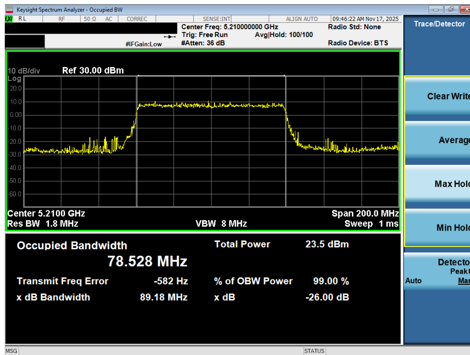
Plot 7-14. 26dB Bandwidth Plot MIMO ANT2 (80MHz BW 802.11ax (UNII Band 1) – Ch. 42)
