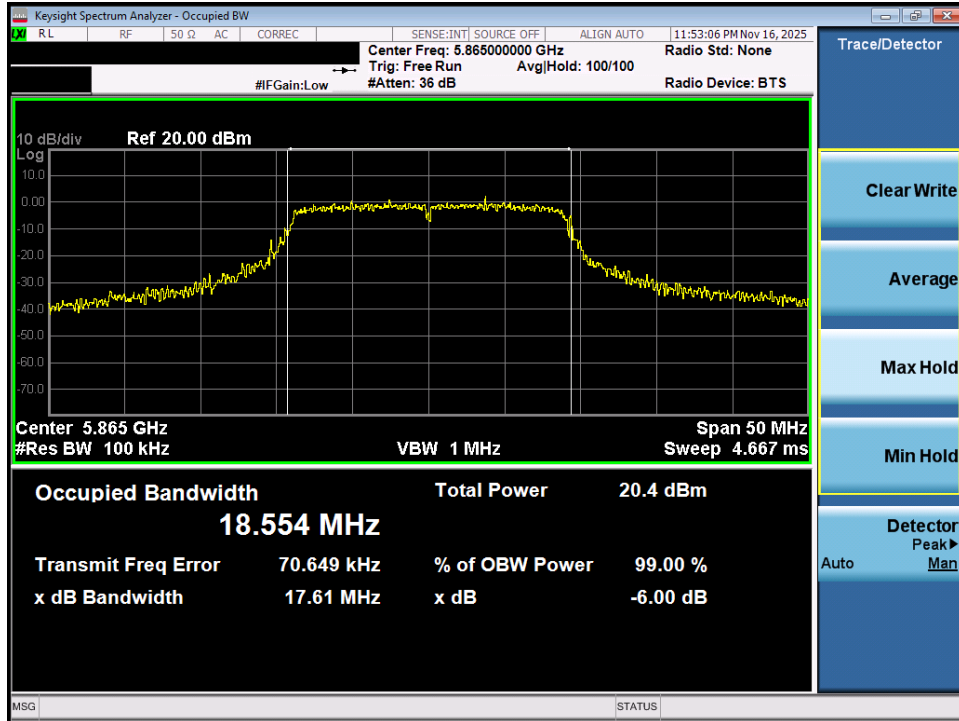
Plot 7-23. 6dB Bandwidth Plot MIMO ANT1 (20MHz BW 802.11n (UNII Band 4) – Ch. 173)
