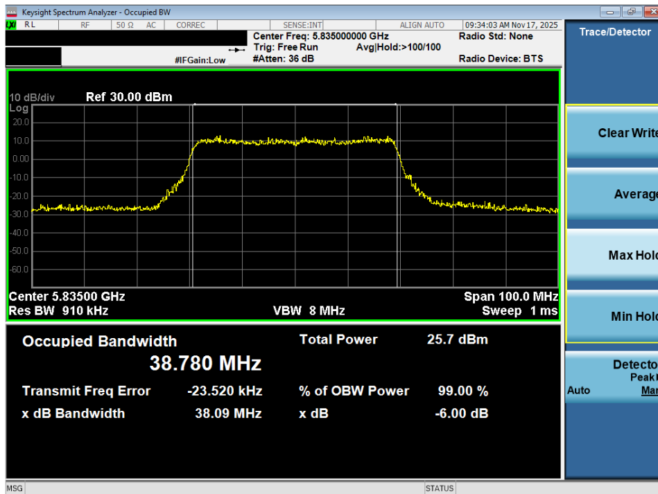
Plot 7-68. OBW Plot MIMO ANT2 (40MHz BW 802.11ax (UNII Band 3/4) – Ch. 167)
