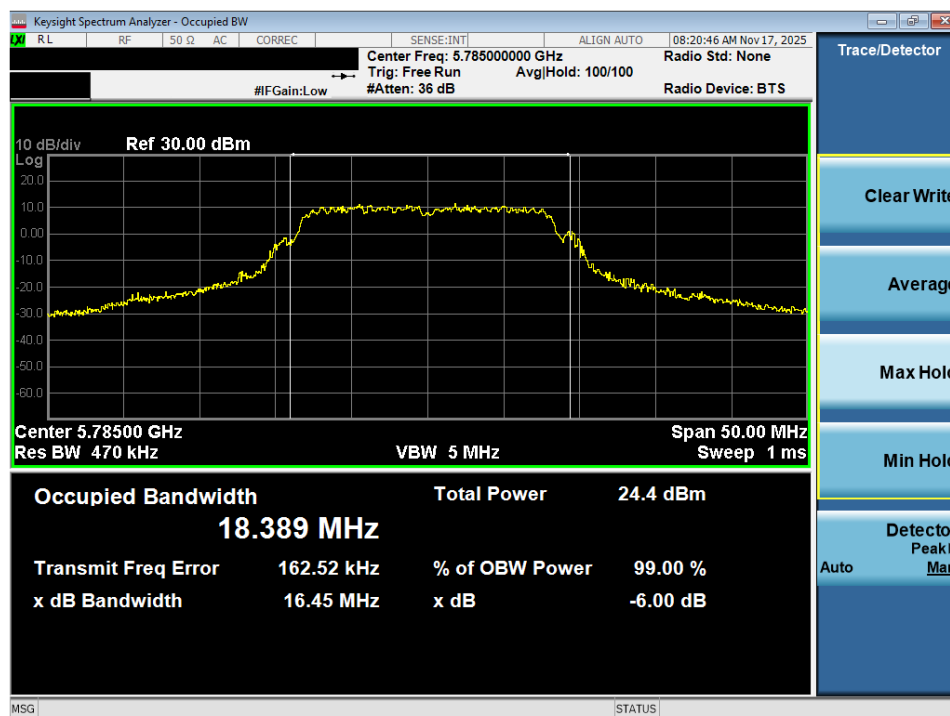
Plot 7-57. OBW Plot MIMO ANT2 (802.11a (UNII Band 3) – Ch. 157)
