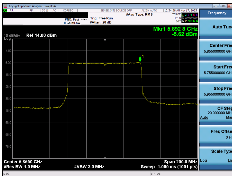
Plot 7-91. Power Spectral Density Plot MIMO ANT1 (80MHz BW 802.11ax (UNII Band 3/4) – Ch. 171)
