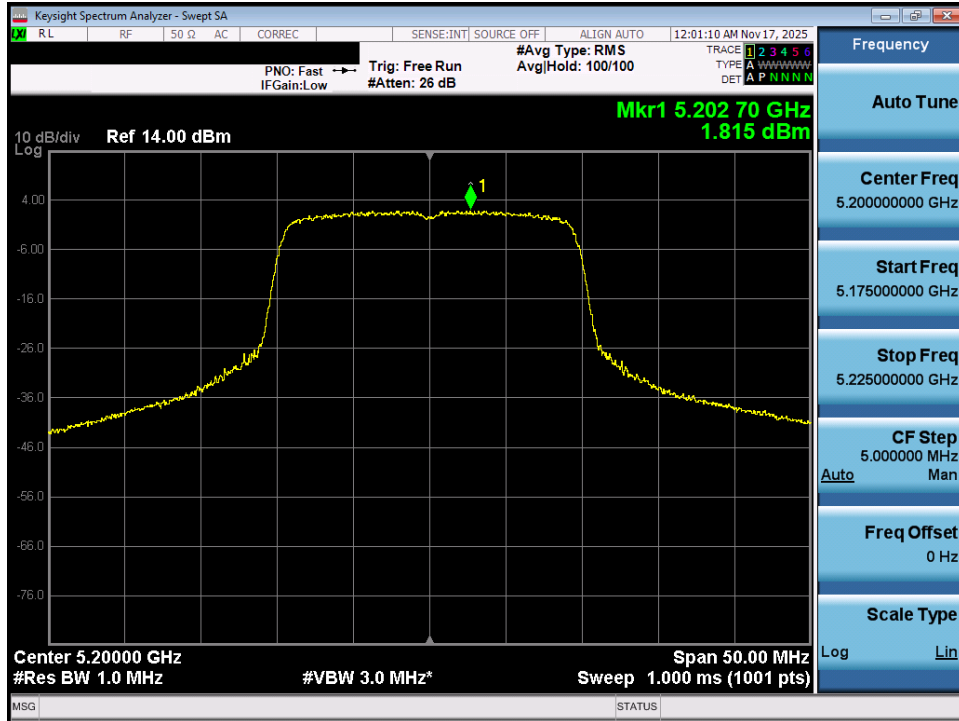
Plot 7-73. Power Spectral Density Plot MIMO ANT1 (20MHz BW 802.11ax (UNII Band 1) – Ch. 40)
