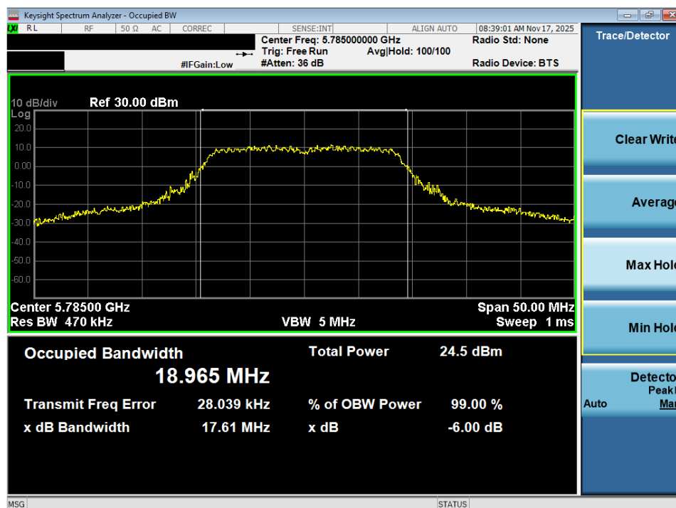
Plot 7-58. OBW Plot MIMO ANT2 (20MHz BW 802.11n (UNII Band 3) – Ch. 157)
