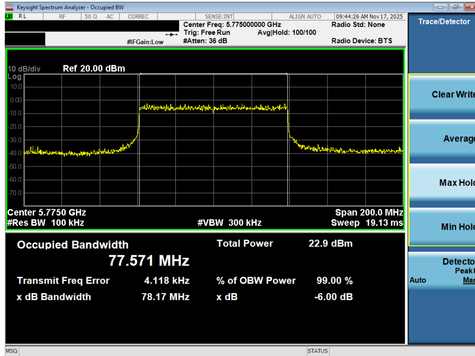
Plot 7-35. 6dB Bandwidth Plot MIMO ANT2 (80MHz BW 802.11ax (UNII Band 3) – Ch. 155)
