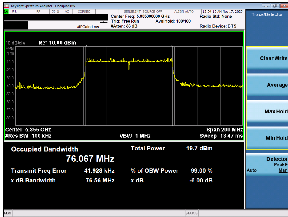
Plot 7-27. 6dB Bandwidth Plot MIMO ANT1 (80MHz BW 802.11ac (UNII Band 3/4) – Ch. 171)
