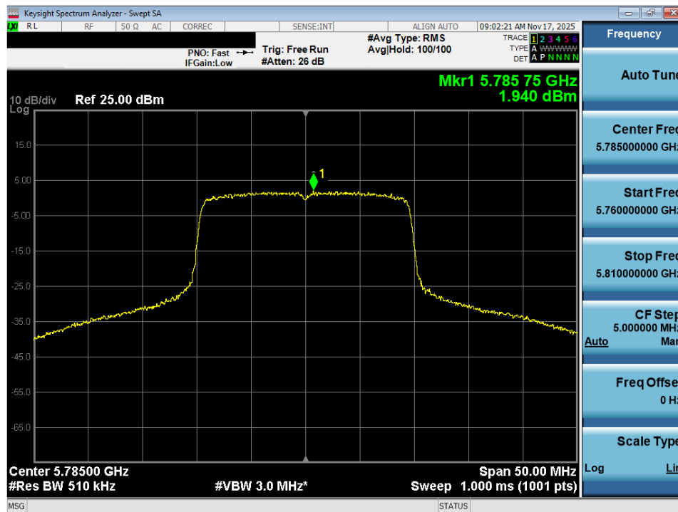
Plot 7-101. Power Spectral Density Plot MIMO ANT2 (20MHz BW 802.11ax (UNII Band 3) – Ch. 157)
