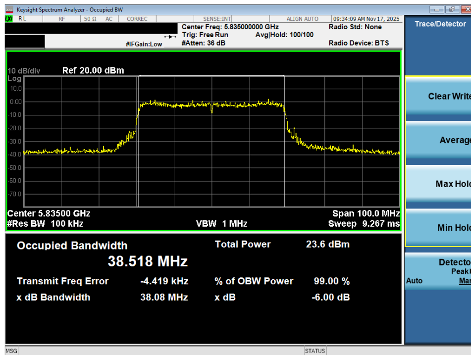
Plot 7-40. 6dB Bandwidth Plot MIMO ANT2 (40MHz BW 802.11ax (UNII Band 3/4) – Ch. 167)
