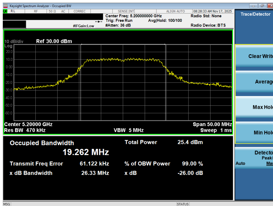
Plot 7-9. 26dB Bandwidth Plot MIMO ANT2 (20MHz BW 802.11n (UNII Band 1) – Ch. 40)
