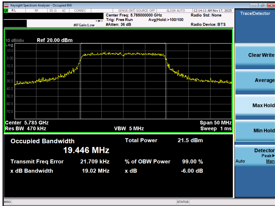
Plot 7-45. OBW Plot MIMO ANT1 (20MHz BW 802.11ax (UNII Band 3) – Ch. 157)
