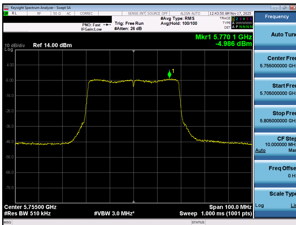
Plot 7-82. Power Spectral Density Plot MIMO ANT1 (40MHz BW 802.11ax (UNII Band 3) – Ch. 151)
