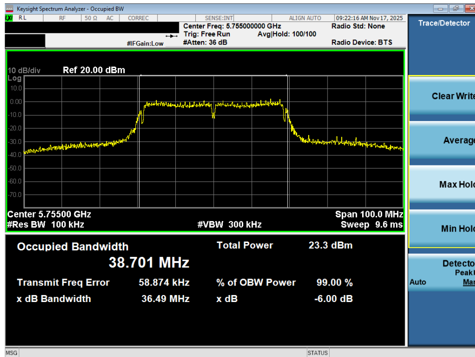
Plot 7-32. 6dB Bandwidth Plot MIMO ANT2 (40MHz BW 802.11n (UNII Band 3) – Ch. 151)
