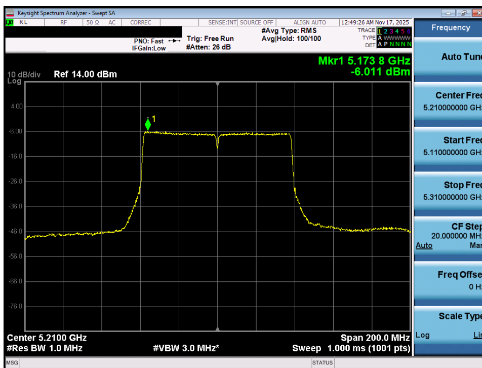
Plot 7-76. Power Spectral Density Plot MIMO ANT1 (80MHz BW 802.11ac (UNII Band 1) – Ch. 42)
