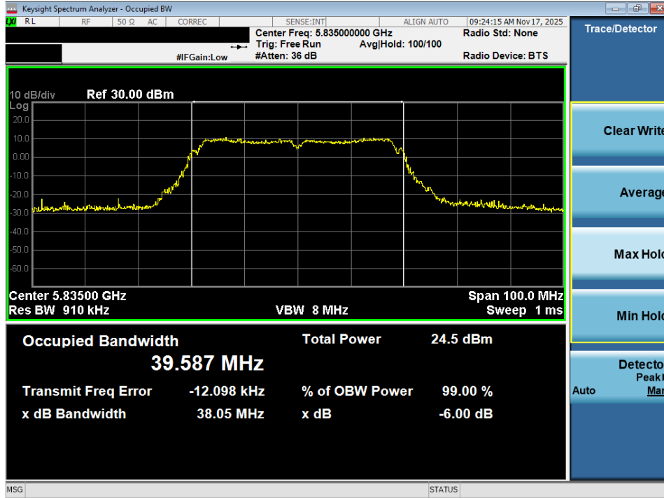
Plot 7-67. OBW Plot MIMO ANT2 (40MHz BW 802.11n (UNII Band 3/4) – Ch. 167)
