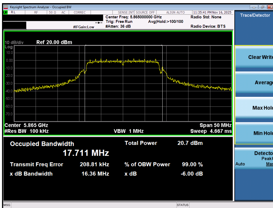
Plot 7-22. 6dB Bandwidth Plot MIMO ANT1 (802.11a (UNII Band 4) – Ch. 173)
