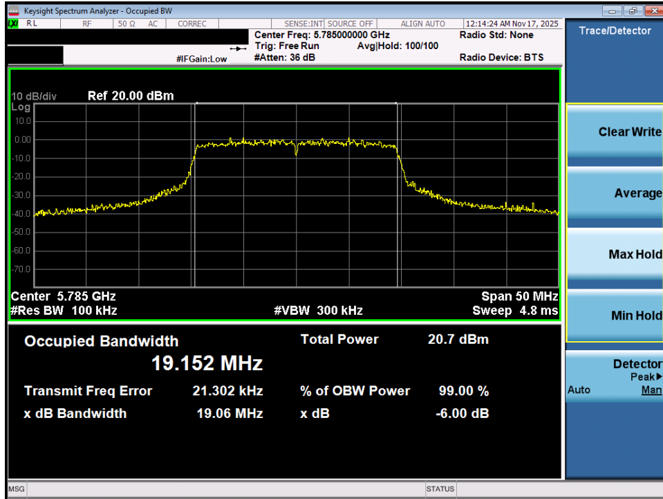
Plot 7-17. 6dB Bandwidth Plot MIMO ANT1 (20MHz BW 802.11ax (UNII Band 3) – Ch. 157)
