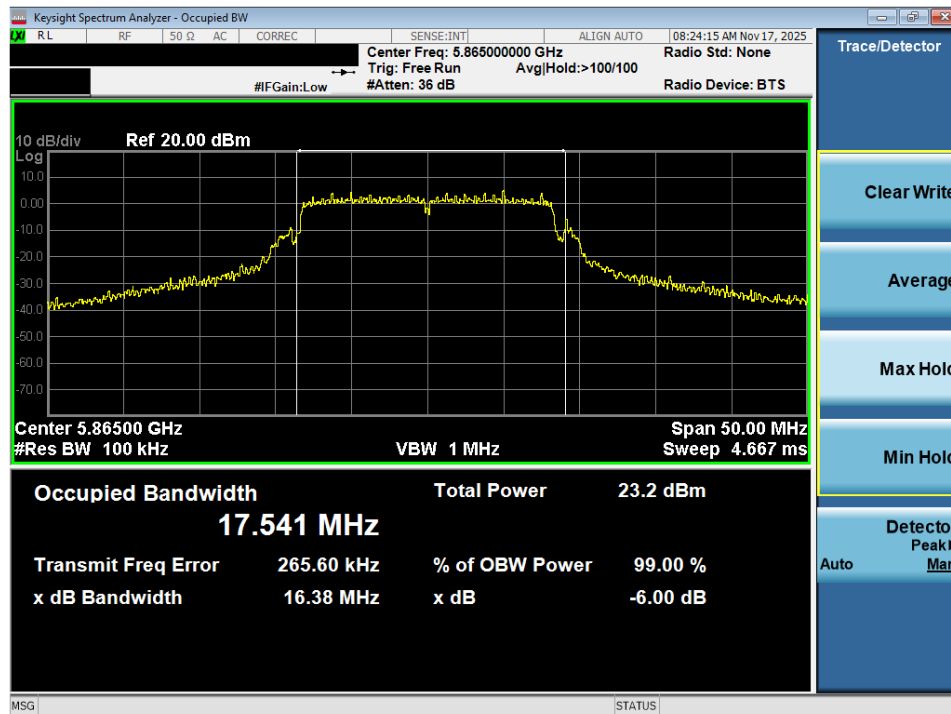
Plot 7-36. 6dB Bandwidth Plot MIMO ANT2 (802.11a (UNII Band 3/4) – Ch. 173)
