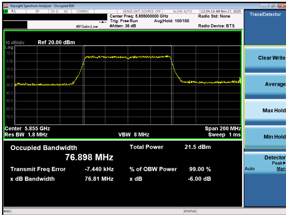
Plot 7-55. OBW Plot MIMO ANT1 (80MHz BW 802.11ac (UNII Band 3/4) – Ch. 171)
