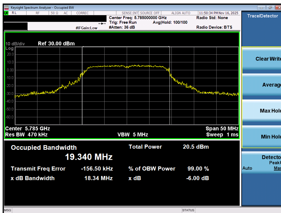
Plot 7-44. OBW Plot MIMO ANT1 (20MHz BW 802.11n (UNII Band 3) – Ch. 157)
