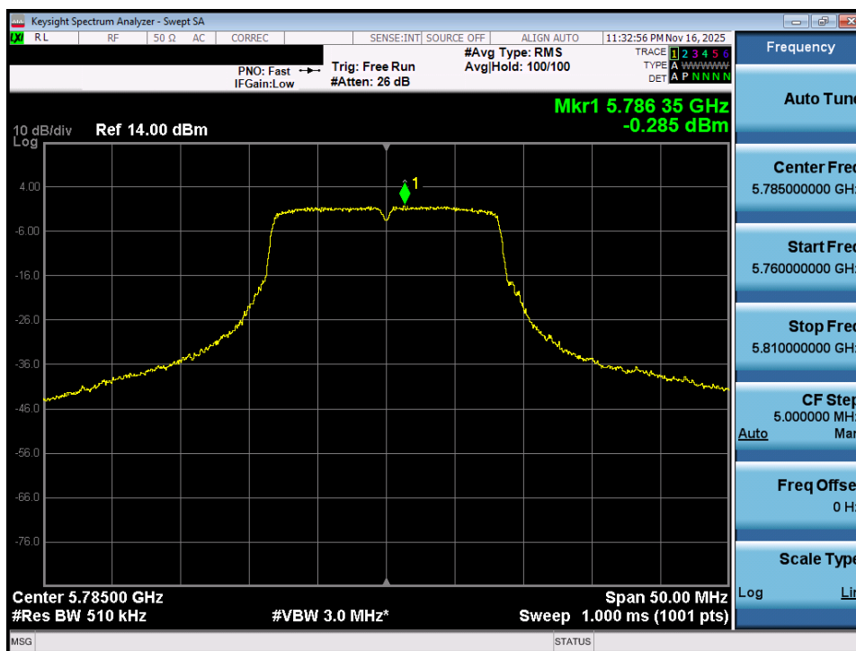
Plot 7-78. Power Spectral Density Plot MIMO ANT1 (802.11a (UNII Band 3) – Ch. 157)
