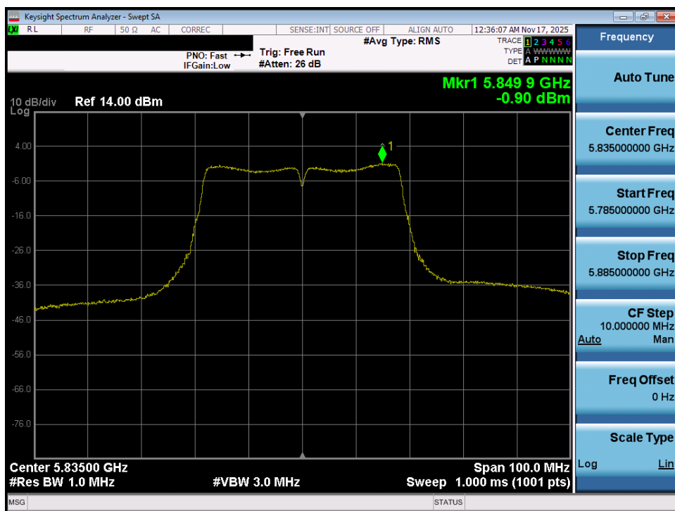
Plot 7-88. Power Spectral Density Plot MIMO ANT1 (40MHz BW 802.11n (UNII Band 3/4) – Ch. 167)
