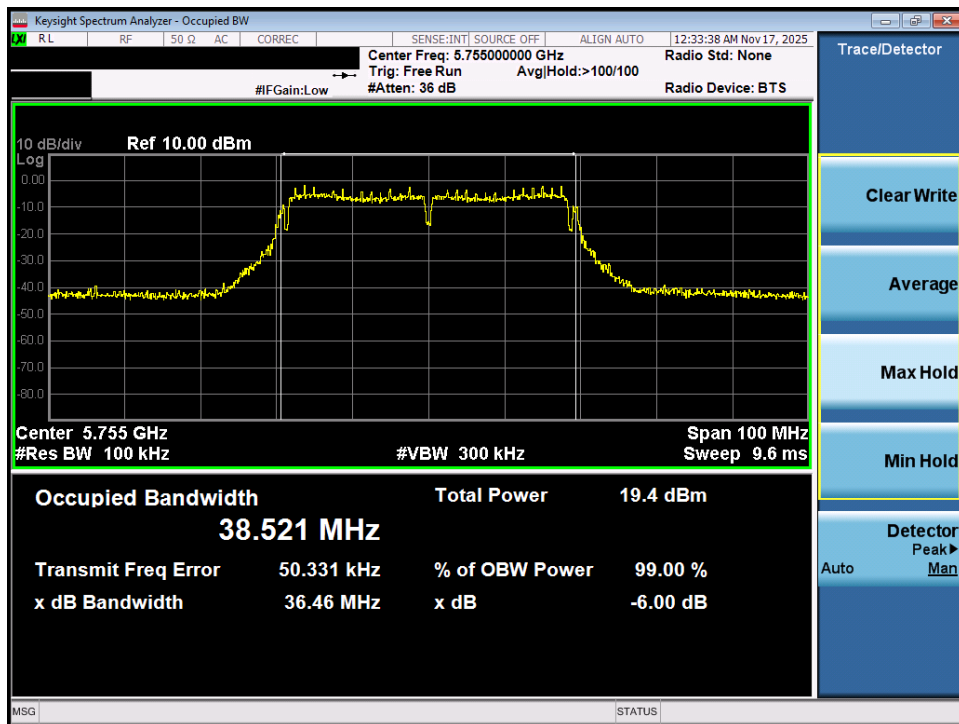
Plot 7-18. 6dB Bandwidth Plot MIMO ANT1 (40MHz BW 802.11n (UNII Band 3) – Ch. 151)
