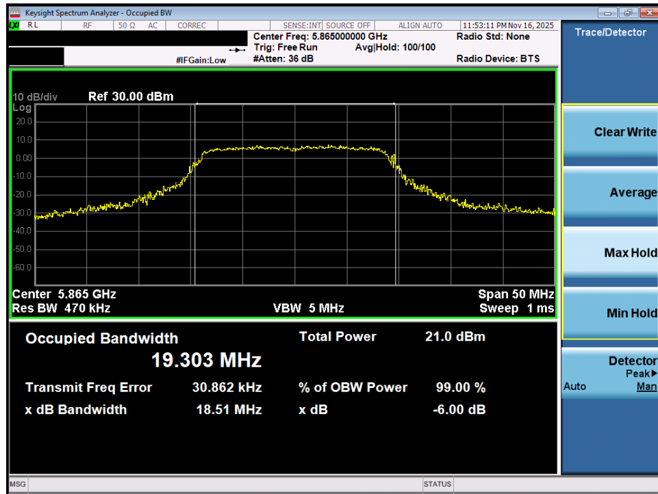
Plot 7-51. OBW Plot MIMO ANT1 (20MHz BW 802.11n (UNII Band 4) – Ch. 173)
