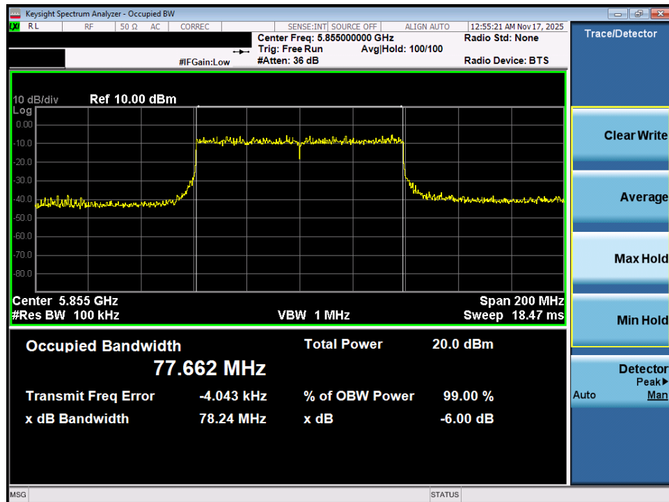
Plot 7-28. 6dB Bandwidth Plot MIMO ANT1 (80MHz BW 802.11ax (UNII Band 3/4) – Ch. 171)
