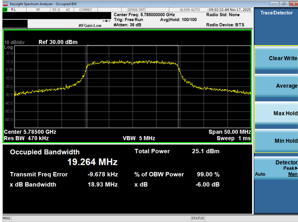
Plot 7-59. OBW Plot MIMO ANT2 (20MHz BW 802.11ax (UNII Band 3) – Ch. 157)
