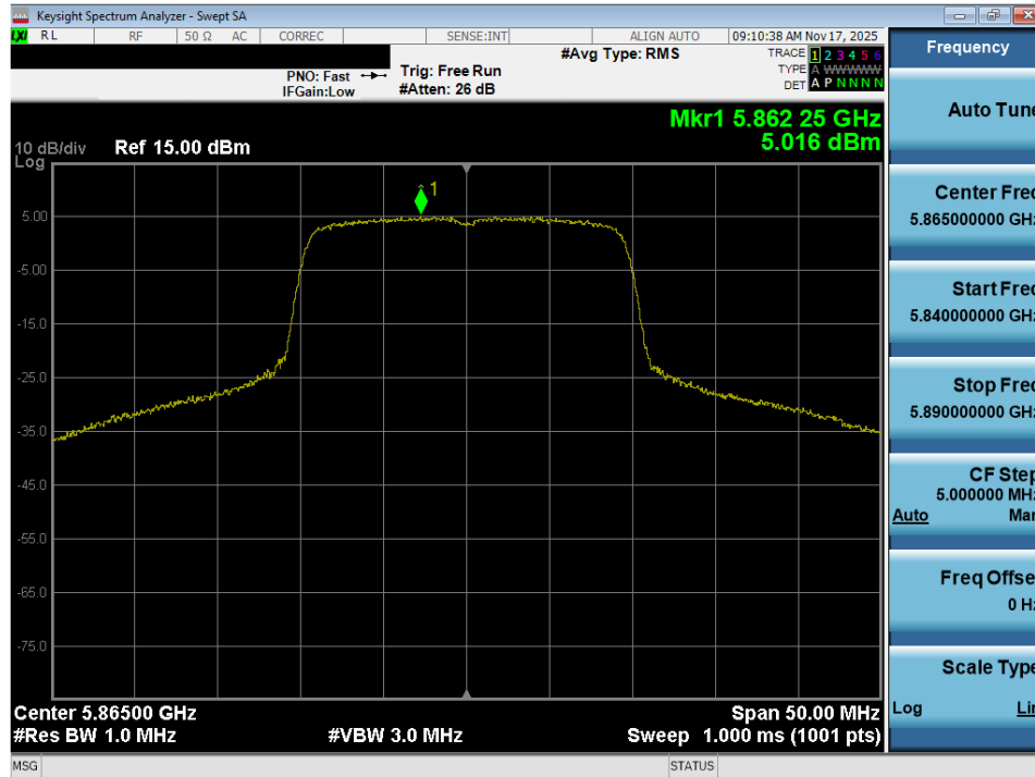
Plot 7-108. Power Spectral Density Plot MIMO ANT2 (20MHz BW 802.11ax (UNII Band 4) – Ch. 173)
