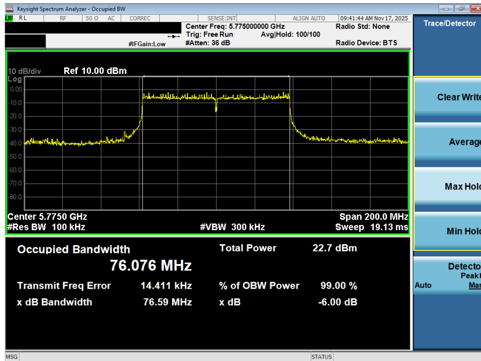
Plot 7-34. 6dB Bandwidth Plot MIMO ANT2 (80MHz BW 802.11ac (UNII Band 3) – Ch. 155)
