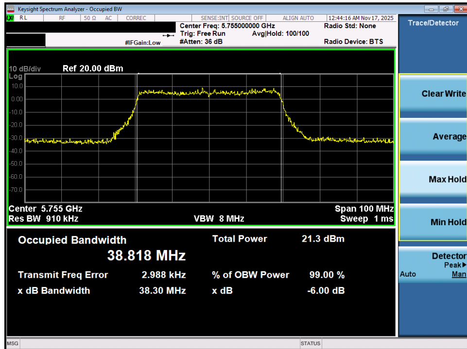
Plot 7-47. OBW Plot MIMO ANT1 (40MHz BW 802.11ax (UNII Band 3) – Ch. 151)
