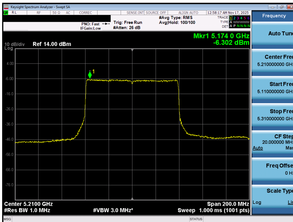
Plot 7-77. Power Spectral Density Plot MIMO ANT1 (80MHz BW 802.11ax (UNII Band 1) – Ch. 42)
