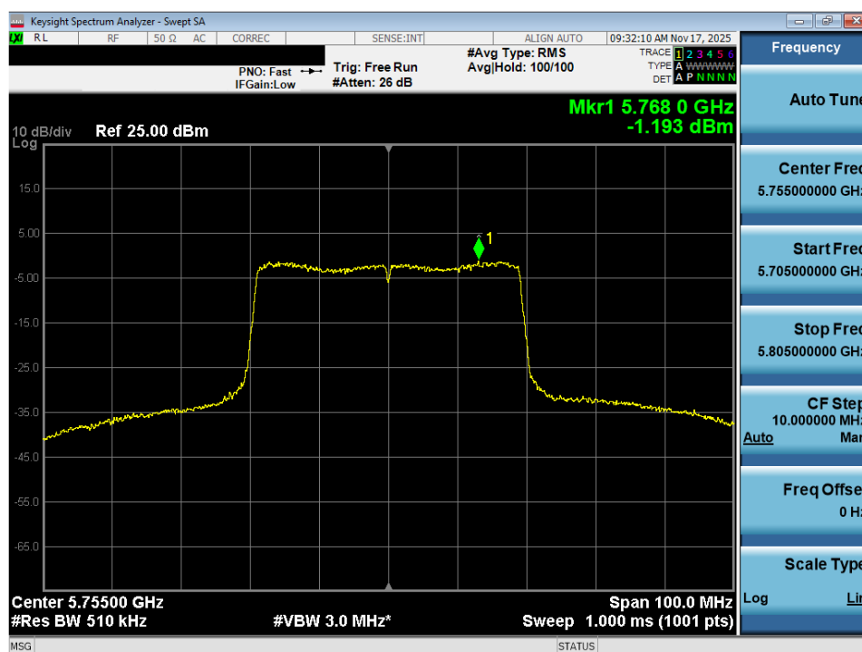
Plot 7-103. Power Spectral Density Plot MIMO ANT2 (40MHz BW 802.11ax (UNII Band 3) – Ch. 151)
