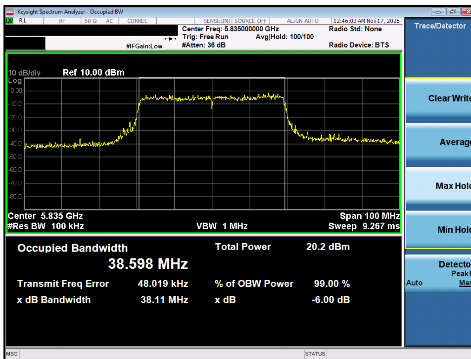
Plot 7-26. 6dB Bandwidth Plot MIMO ANT1 (40MHz BW 802.11ax (UNII Band 3/4) – Ch. 167)
