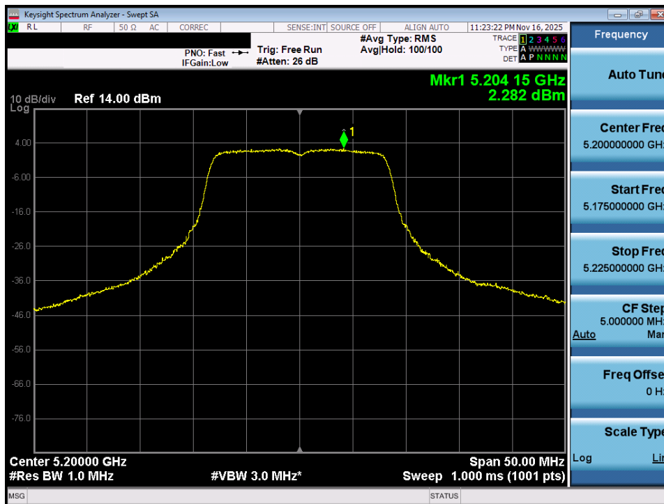
Plot 7-71. Power Spectral Density Plot MIMO ANT1 (802.11a (UNII Band 1) – Ch. 40)
