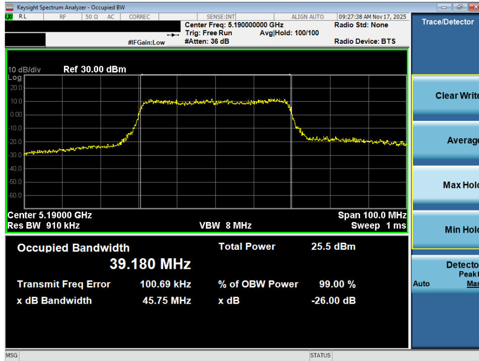
Plot 7-12. 26dB Bandwidth Plot MIMO ANT2 (40MHz BW 802.11ax (UNII Band 1) – Ch. 38)
