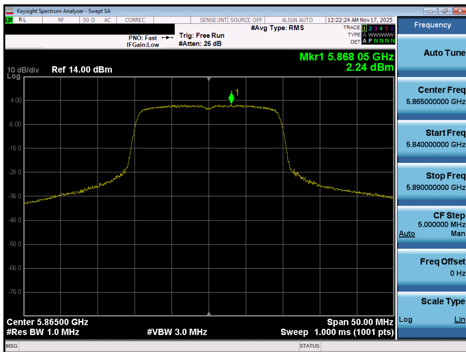
Plot 7-87. Power Spectral Density Plot MIMO ANT1 (20MHz BW 802.11ax (UNII Band 4) – Ch. 173)
