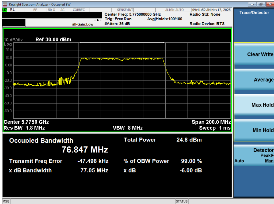
Plot 7-62. OBW Plot MIMO ANT2 (80MHz BW 802.11ac (UNII Band 3) – Ch. 155)
