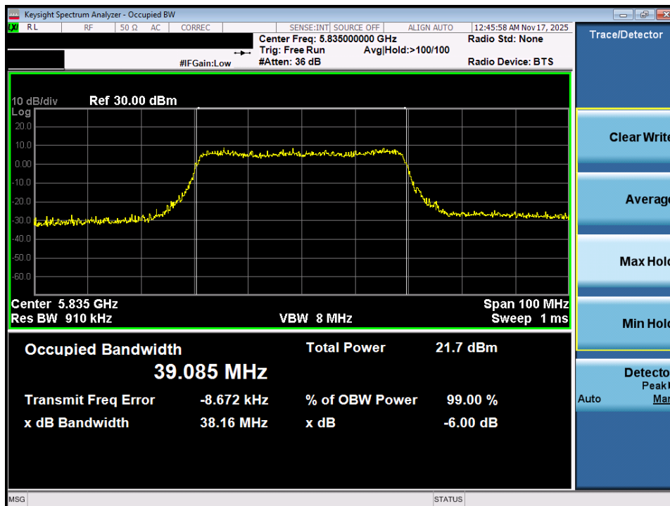
Plot 7-54. OBW Plot MIMO ANT1 (40MHz BW 802.11ax (UNII Band 3/4) – Ch. 167)
