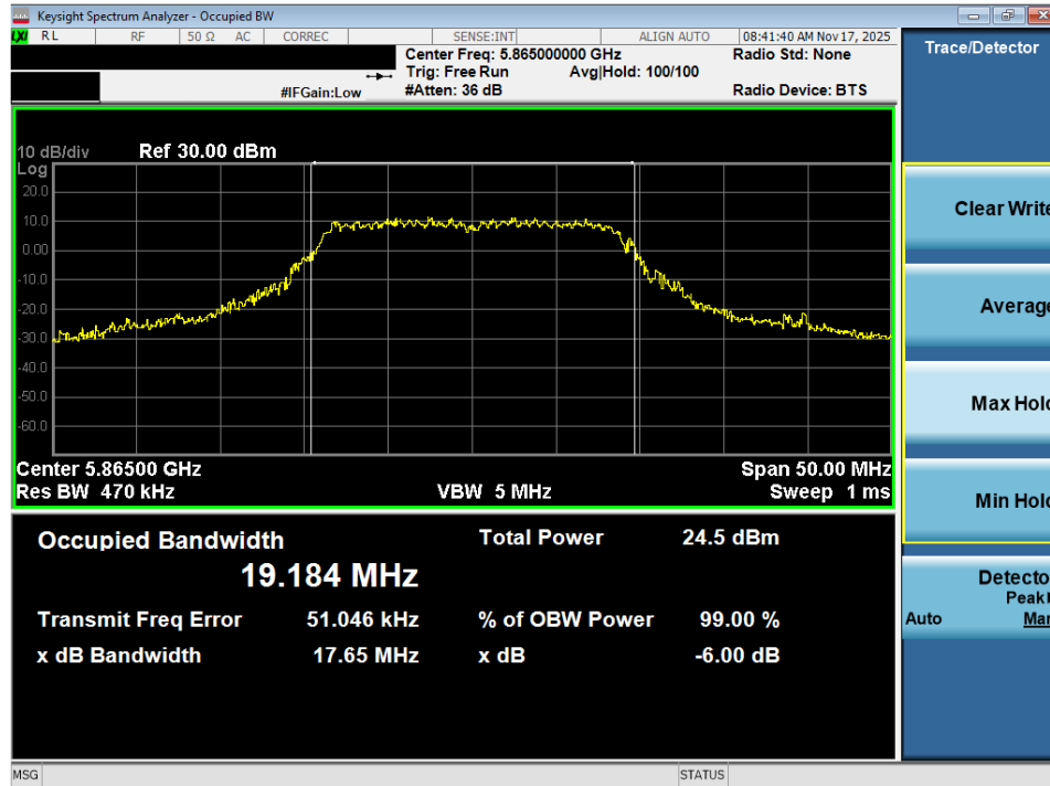
Plot 7-65. OBW Plot MIMO ANT2 (20MHz BW 802.11n (UNII Band 3/4) – Ch. 173)
