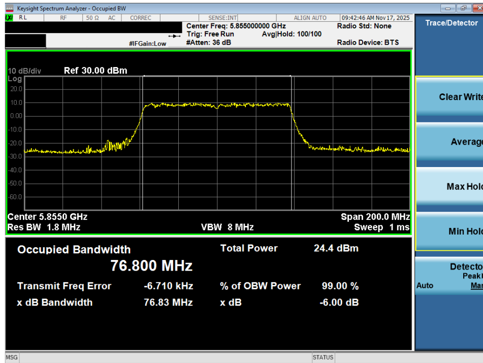
Plot 7-69. OBW Plot MIMO ANT2 (80MHz BW 802.11ac (UNII Band 3/4) – Ch. 171)
