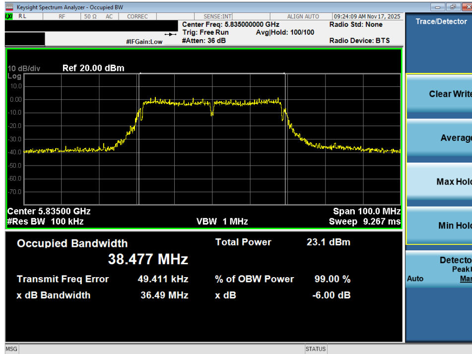
Plot 7-39. 6dB Bandwidth Plot MIMO ANT2 (40MHz BW 802.11n (UNII Band 3/4) – Ch. 167)
