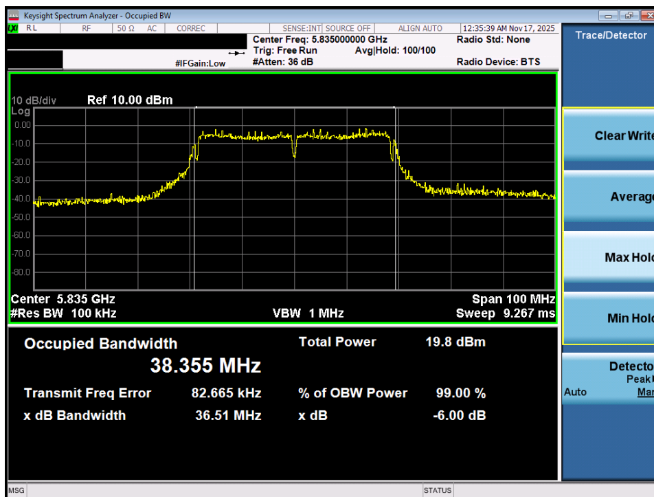
Plot 7-25. 6dB Bandwidth Plot MIMO ANT1 (40MHz BW 802.11n (UNII Band 3/4) – Ch. 167)
