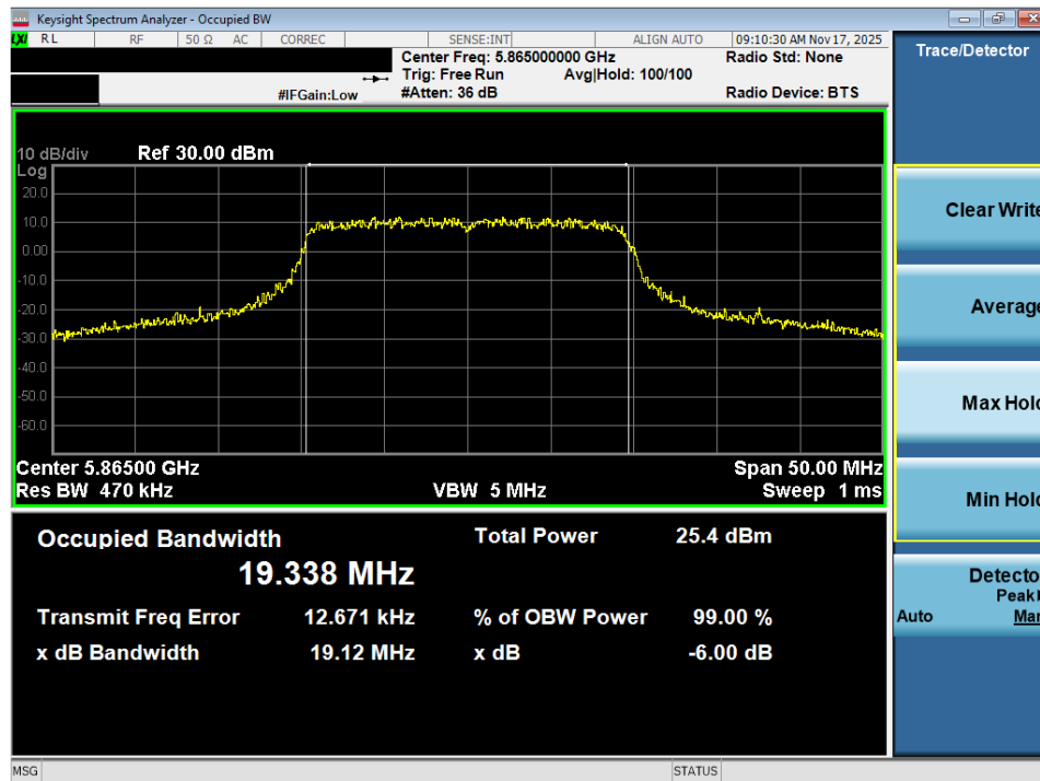
Plot 7-66. OBW Plot MIMO ANT2 (20MHz BW 802.11ax (UNII Band 3/4) – Ch. 173)
