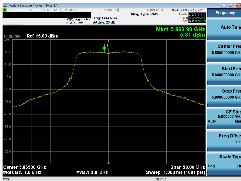
Plot 7-106. Power Spectral Density Plot MIMO ANT2 (802.11a (UNII Band 4) – Ch. 173)
