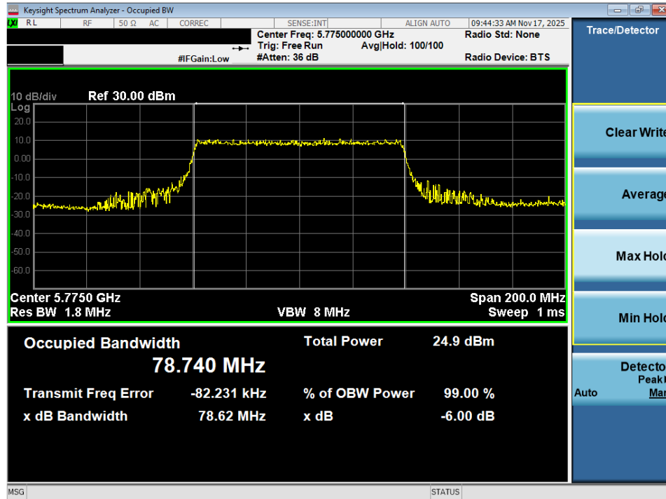
Plot 7-63. OBW Plot MIMO ANT2 (80MHz BW 802.11ax (UNII Band 3) – Ch. 155)
