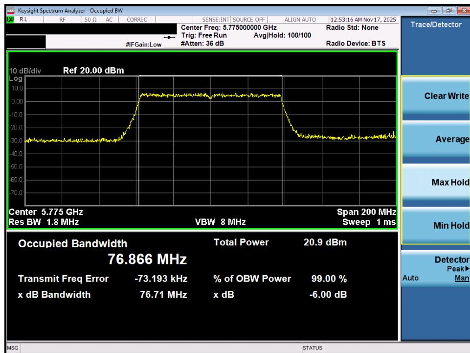
Plot 7-48. OBW Plot MIMO ANT1 (80MHz BW 802.11ac (UNII Band 3) – Ch. 155)
