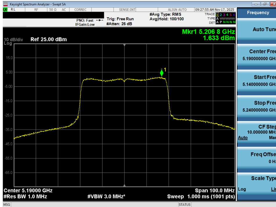
Plot 7-96. Power Spectral Density Plot MIMO ANT2 (40MHz BW 802.11ax (UNII Band 1) – Ch. 38)
