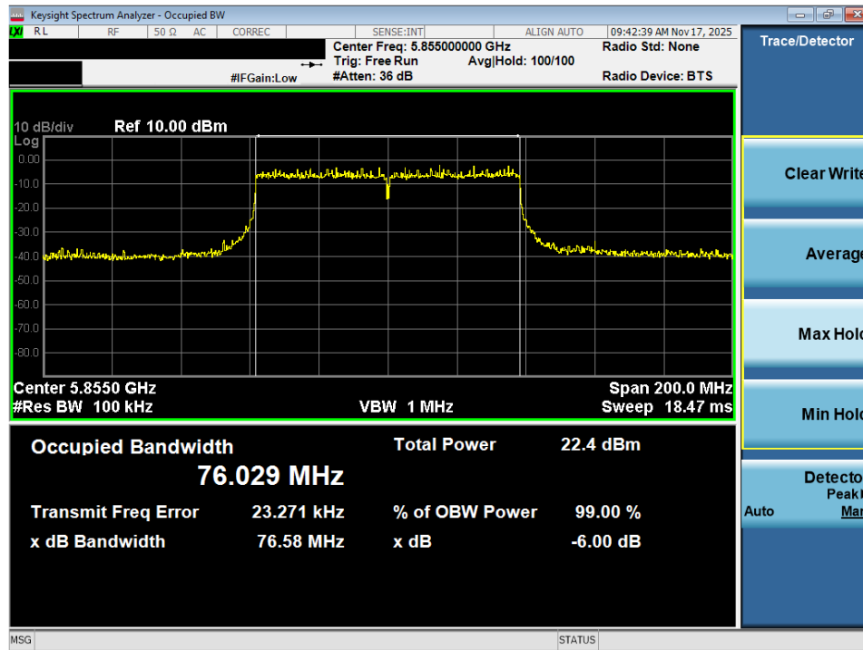
Plot 7-41. 6dB Bandwidth Plot MIMO ANT2 (80MHz BW 802.11ac (UNII Band 3/4) – Ch. 171)
