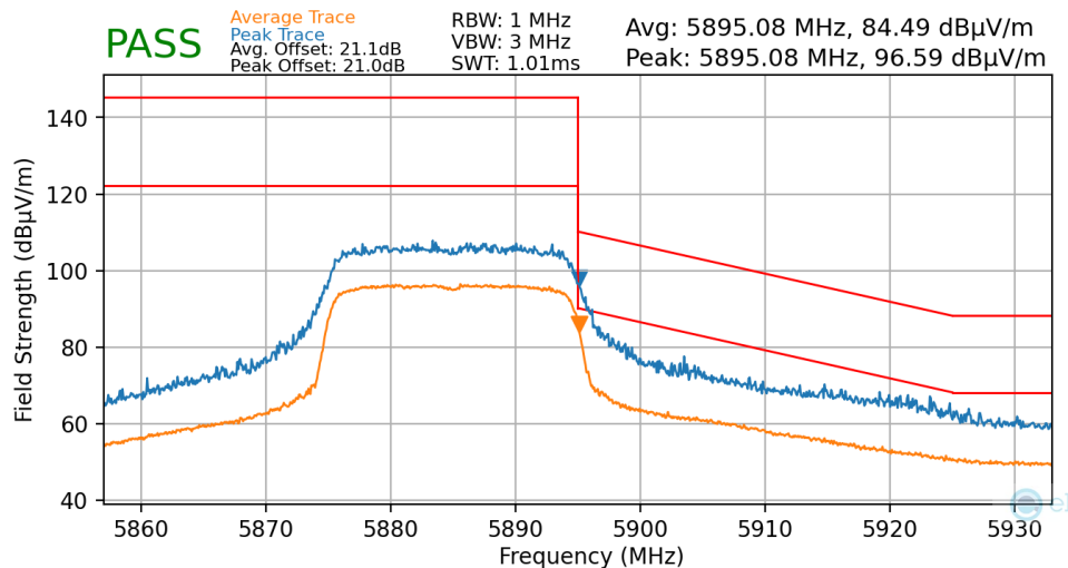
Plot 7-131. Radiated Upper Band Edge Plot MIMO (Average & Peak – UNII Band 4)
