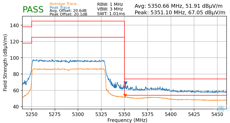
Plot 7-140. Radiated Upper Band Edge Plot MIMO (Average & Peak – UNII Band 2A)
