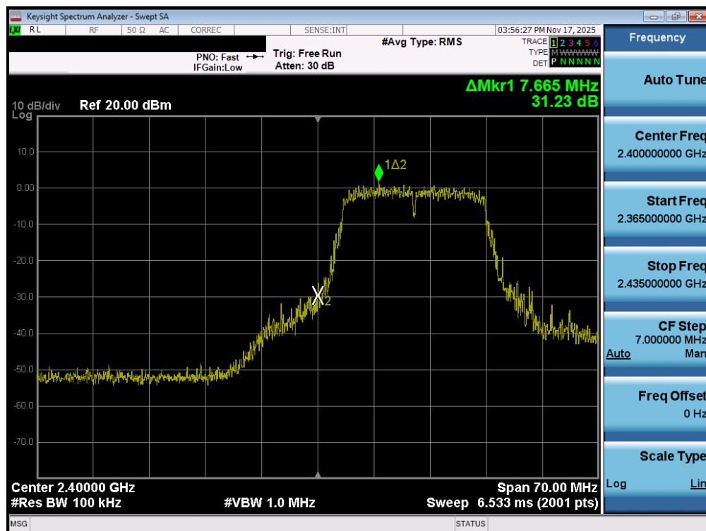
Plot 7-101. Band Edge Plot MIMO ANT2 (802.11n(2.4GHz) – Ch. 1)
