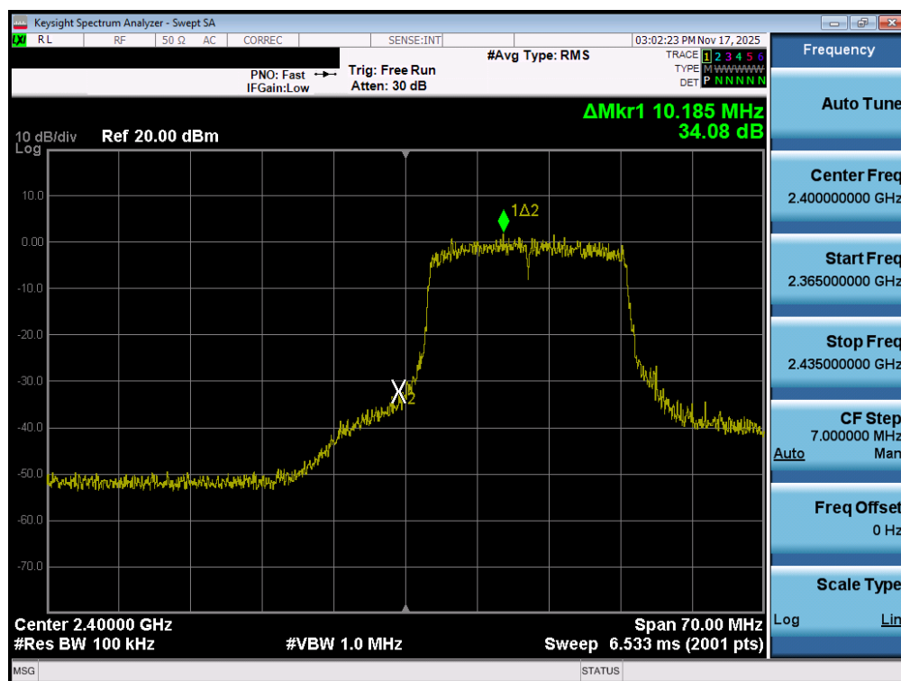
Plot 7-106. Band Edge Plot MIMO ANT2 (802.11ax (2.4GHz) – Ch. 1)
