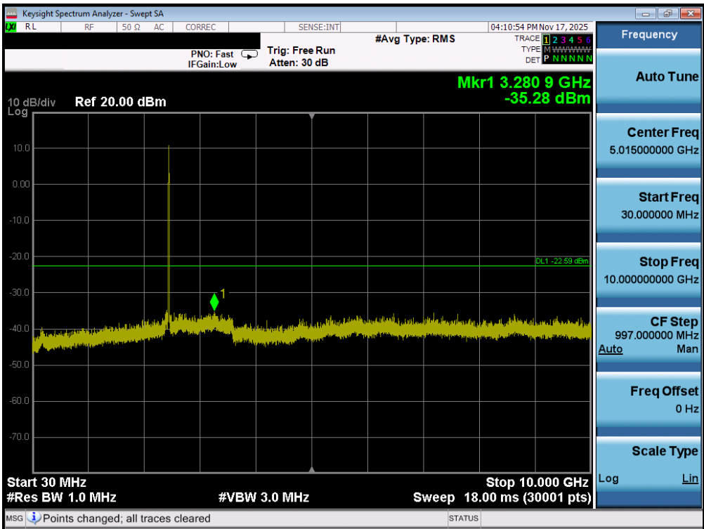
Plot 7-121. Conducted Spurious Plot MIMO ANT2 (802.11b – Ch. 11)
