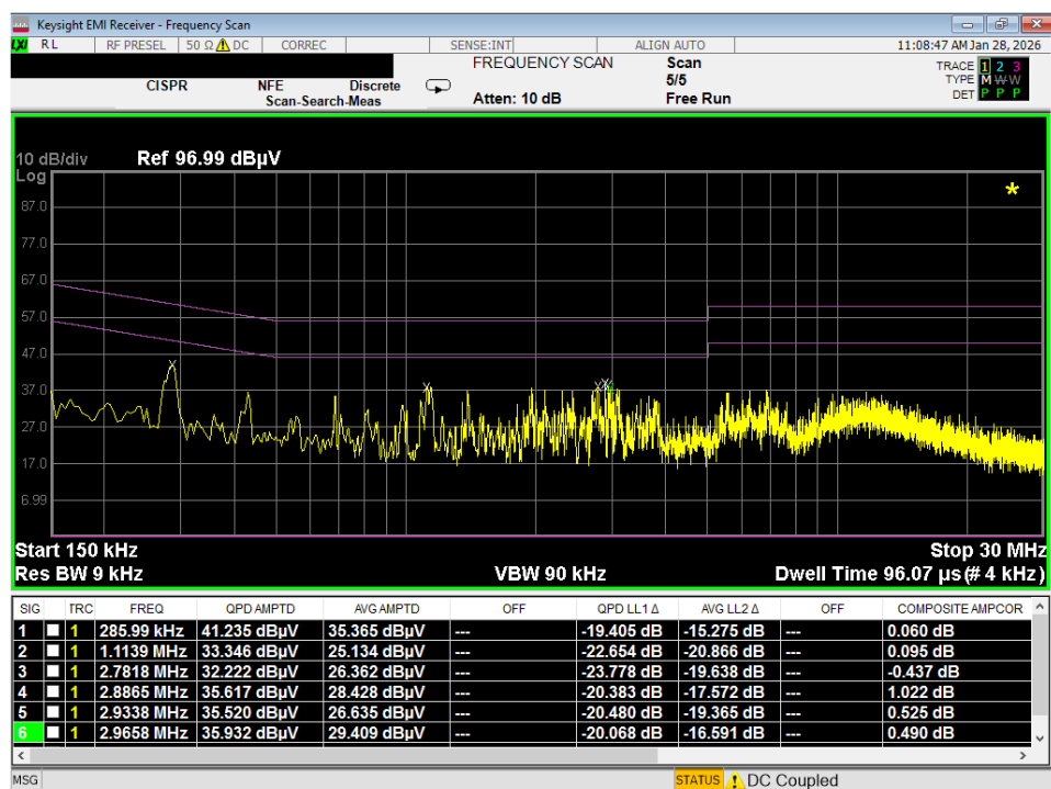
Plot 7-134. Line Conducted Plot with 802.11b (N)
