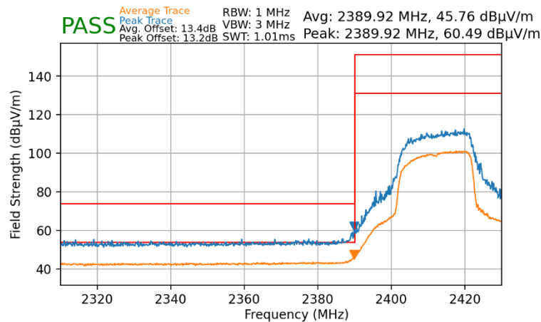
Plot 7-128. Radiated Restricted Lower Band Edge Measurement MIMO (Average & Peak)
