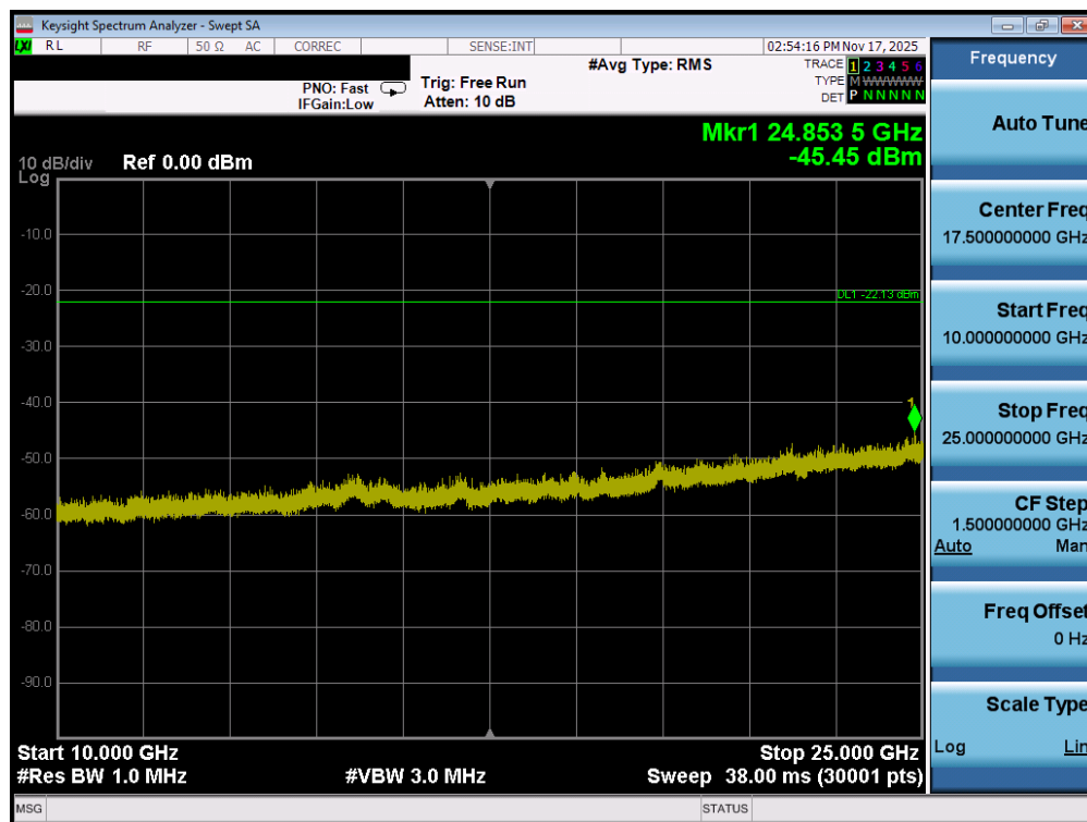
Plot 7-112. Conducted Spurious Plot MIMO ANT1 (802.11b – Ch. 1)
