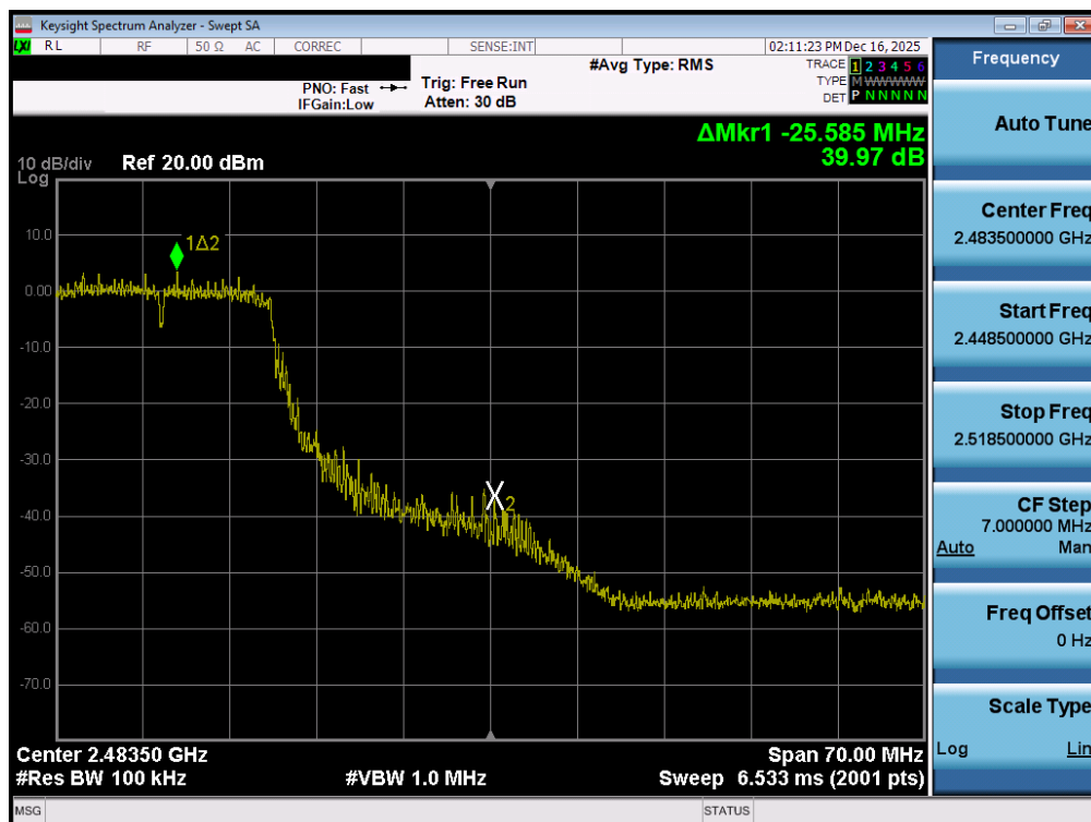
Plot 7-102. Band Edge Plot MIMO ANT2 (802.11n(2.4GHz) – Ch. 10)
