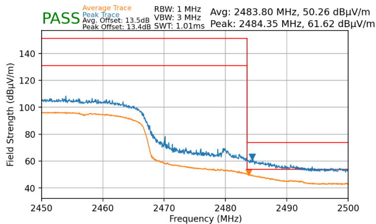
Plot 7-129. Radiated Restricted Upper Band Edge Measurement MIMO (Average & Peak)
