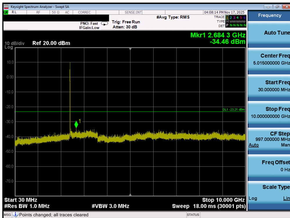
Plot 7-117. Conducted Spurious Plot MIMO ANT2 (802.11b – Ch. 1)
