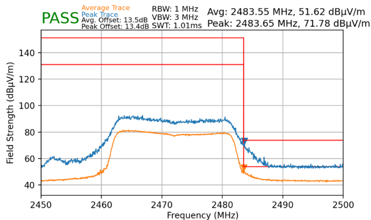
Plot 7-132. Radiated Restricted Upper Band Edge Measurement MIMO (Average & Peak)
