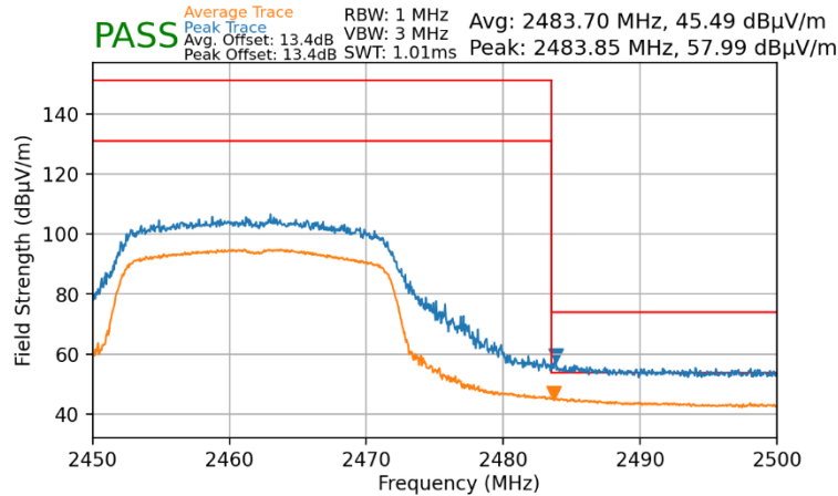
Plot 7-130. Radiated Restricted Upper Band Edge Measurement MIMO (Average & Peak)
