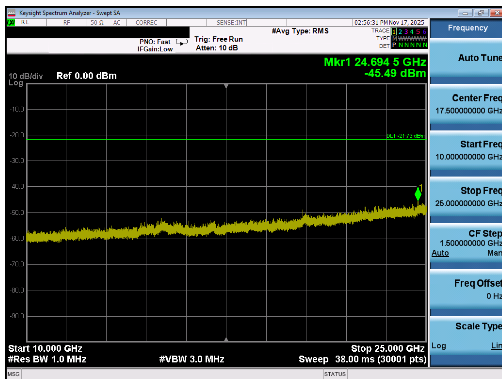
Plot 7-114. Conducted Spurious Plot MIMO ANT1 (802.11b – Ch. 6)
