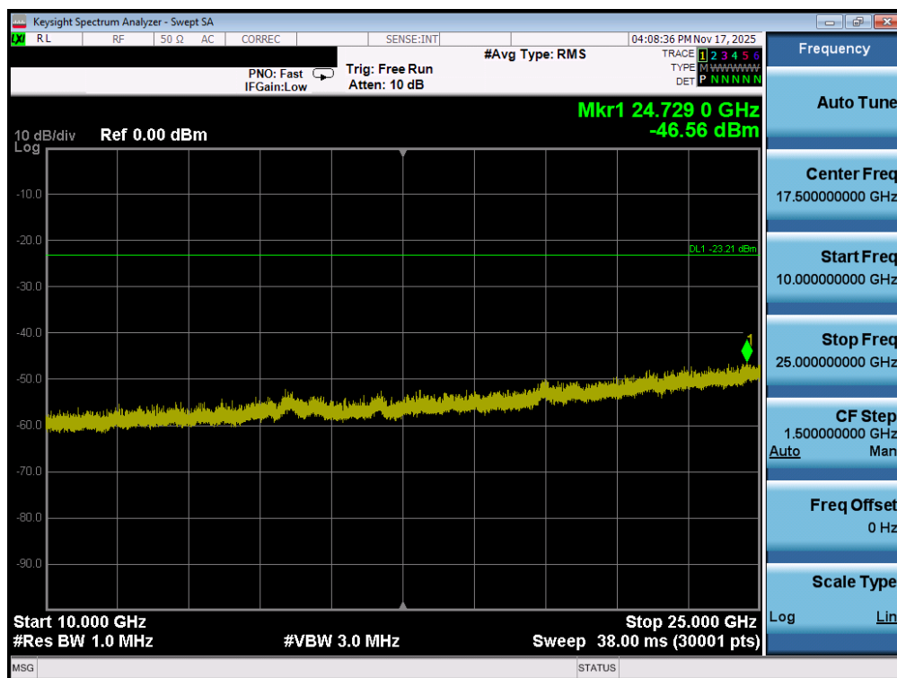
Plot 7-118. Conducted Spurious Plot MIMO ANT2 (802.11b – Ch. 1)
