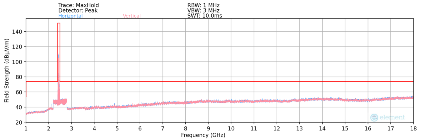
Plot 7-125. Radiated Spurious Plot above 1GHz MIMO (802.11b – Ch. 6)
