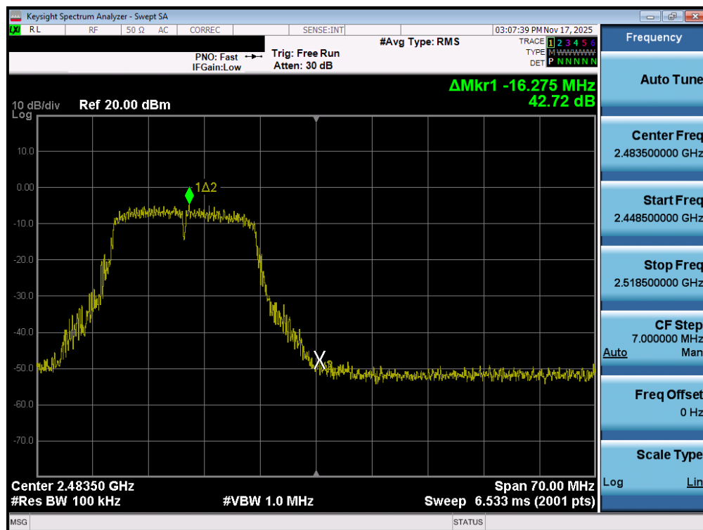
Plot 7-104. Band Edge Plot MIMO ANT2 (802.11n(2.4GHz) – Ch. 12)
