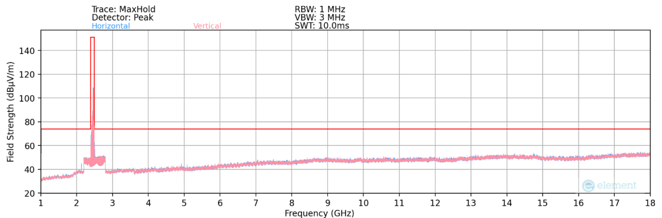
Plot 7-126. Radiated Spurious Plot above 1GHz MIMO (802.11b – Ch. 11)
