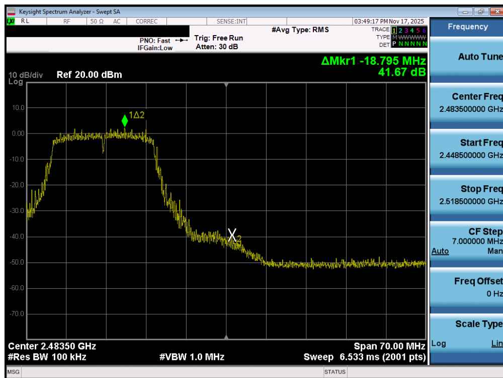
Plot 7-103. Band Edge Plot MIMO ANT2 (802.11n(2.4GHz) – Ch. 11)
