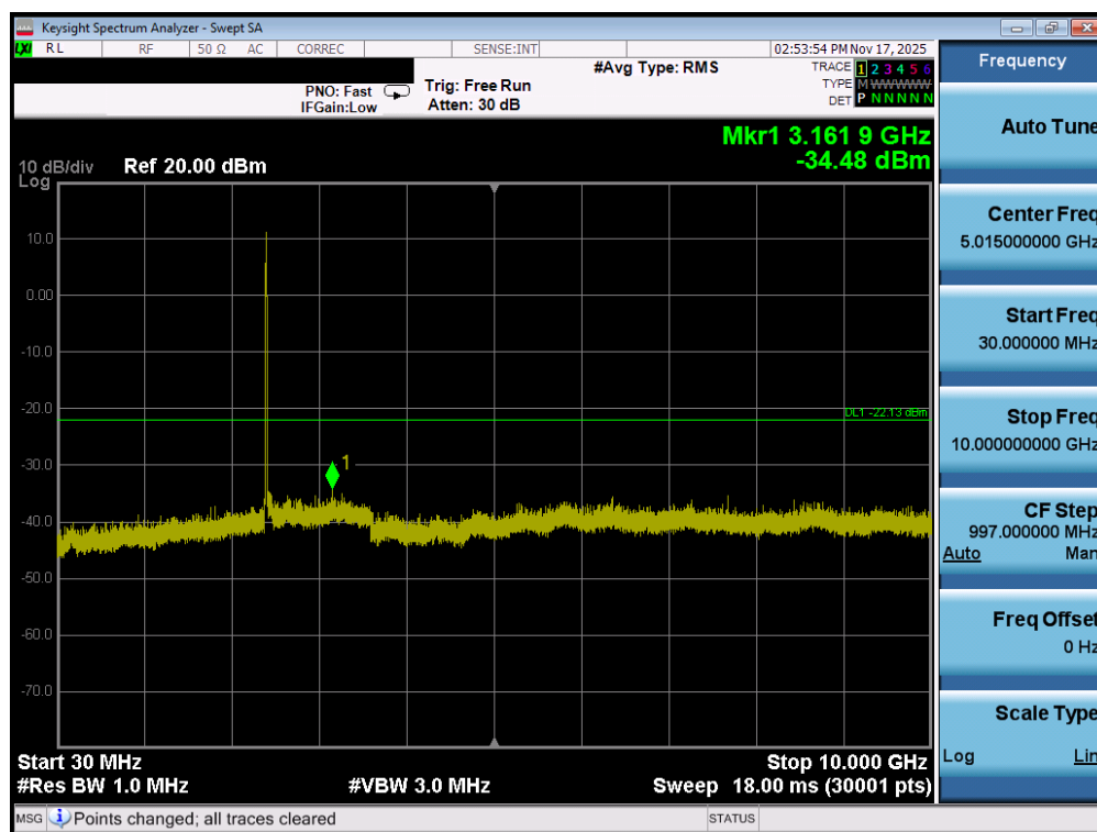
Plot 7-111. Conducted Spurious Plot MIMO ANT1 (802.11b – Ch. 1)
