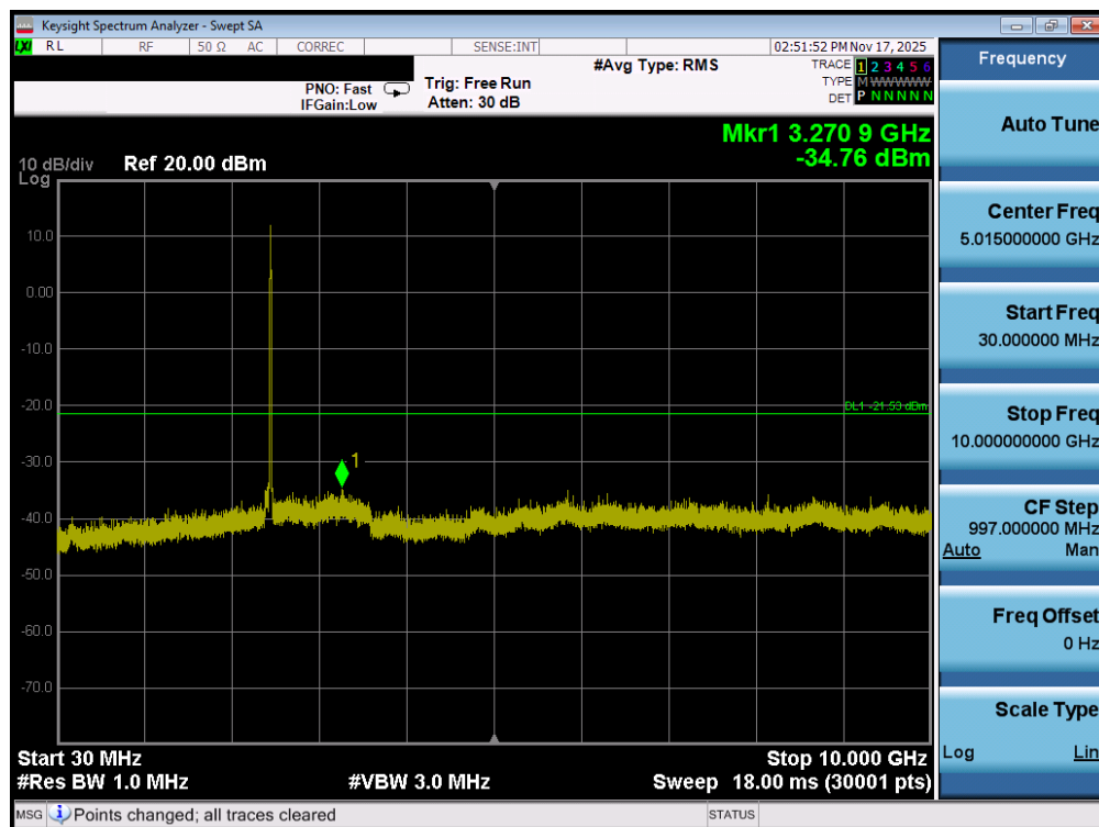
Plot 7-115. Conducted Spurious Plot MIMO ANT1 (802.11b – Ch. 11)
