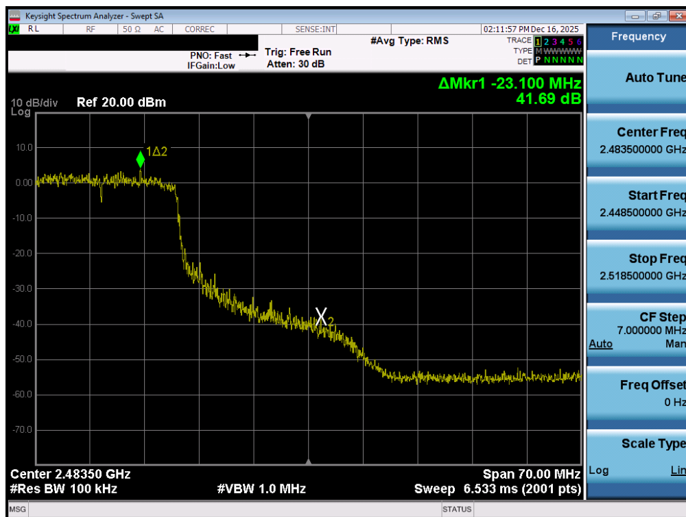
Plot 7-107. Band Edge Plot MIMO ANT2 (802.11ax (2.4GHz) – Ch. 10)
