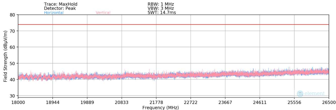
Plot 7-127. Radiated Spurious Plot above 18GHz MIMO
