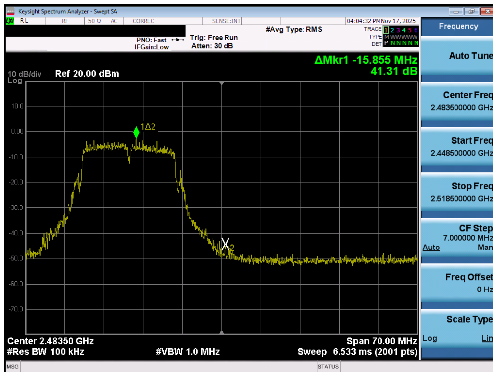
Plot 7-99. Band Edge Plot MIMO ANT2 (802.11g - Ch. 12)
