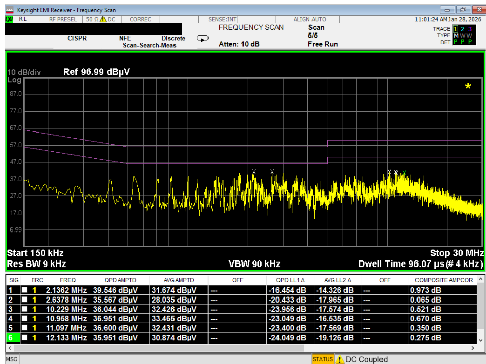
Plot 7-133. Line Conducted Plot with 802.11b (L1)
