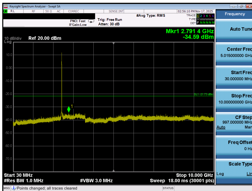
Plot 7-113. Conducted Spurious Plot MIMO ANT1 (802.11b – Ch. 6)
