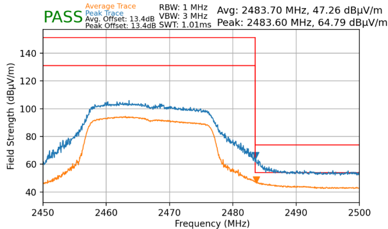
Plot 7-131. Radiated Restricted Upper Band Edge Measurement MIMO (Average & Peak)
