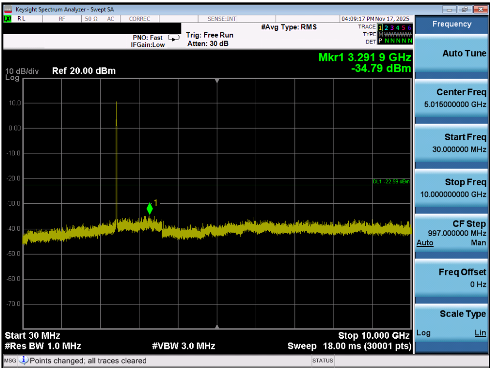
Plot 7-119. Conducted Spurious Plot MIMO ANT2 (802.11b – Ch. 6)
