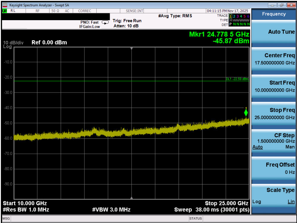
Plot 7-122. Conducted Spurious Plot MIMO ANT2 (802.11b – Ch. 11)
