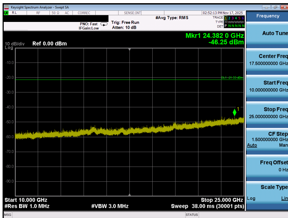
Plot 7-116. Conducted Spurious Plot MIMO ANT1 (802.11b – Ch. 11)
