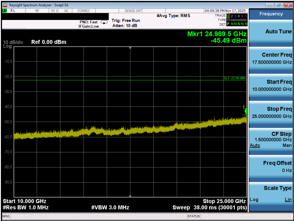
Plot 7-120. Conducted Spurious Plot MIMO ANT2 (802.11b – Ch. 6)
