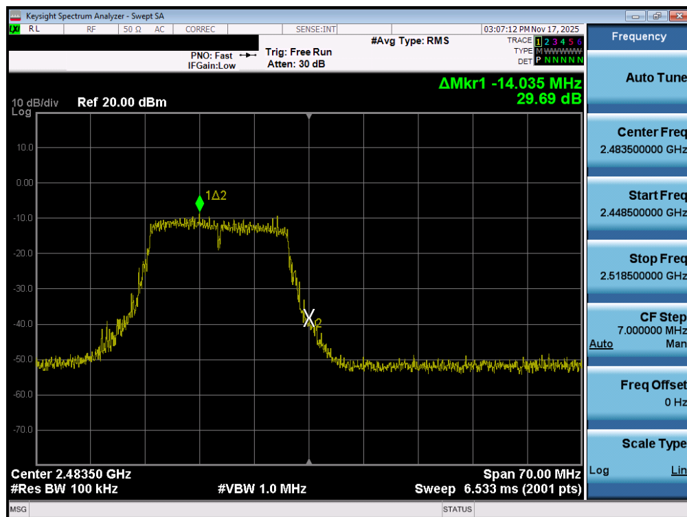
Plot 7-105. Band Edge Plot MIMO ANT2 (802.11n(2.4GHz) – Ch. 13)
