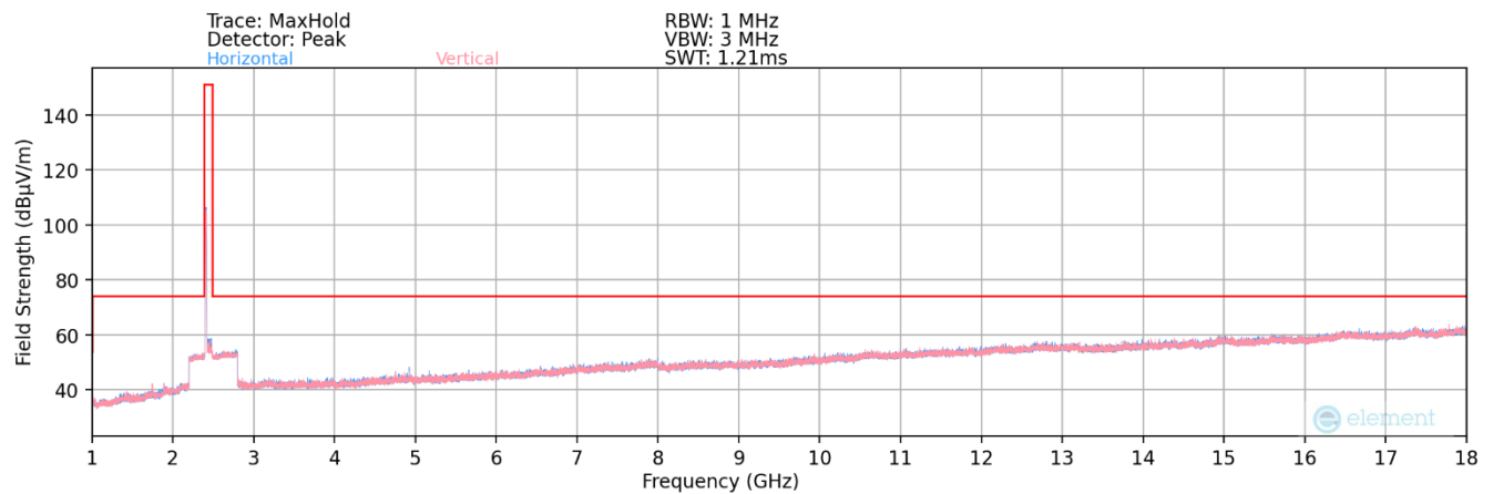
Plot 7-124. Radiated Spurious Plot above 1GHz MIMO (802.11b – Ch. 1)
