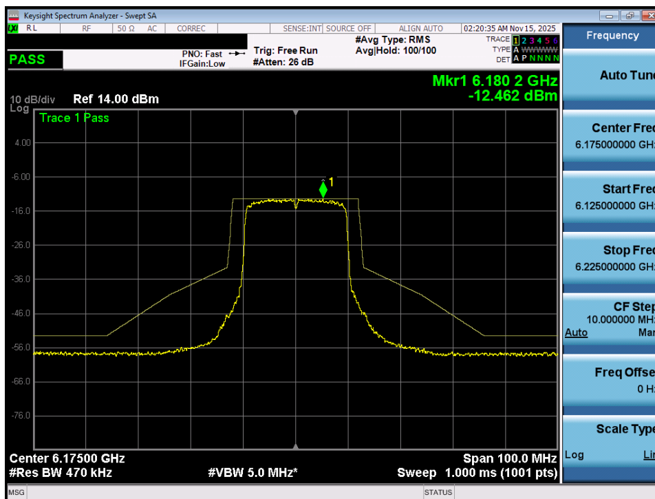
Plot 7-18. In Band Emissions Plot MIMO ANT1 (20MHz 802.11ax (UNII Band 5) – Ch. 45) - VLP
