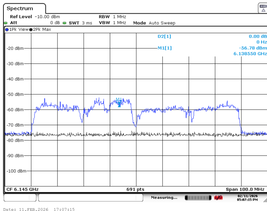
Plot 7-43. CBP 80MHz Channel - Injection Center – [6145 MHz]
