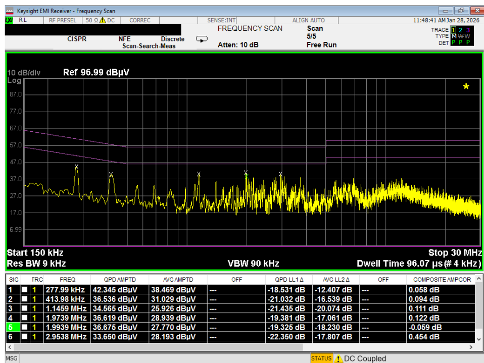
Plot 7-61. Line Conducted Plot with 802.11a UNII Band 5 (N)
