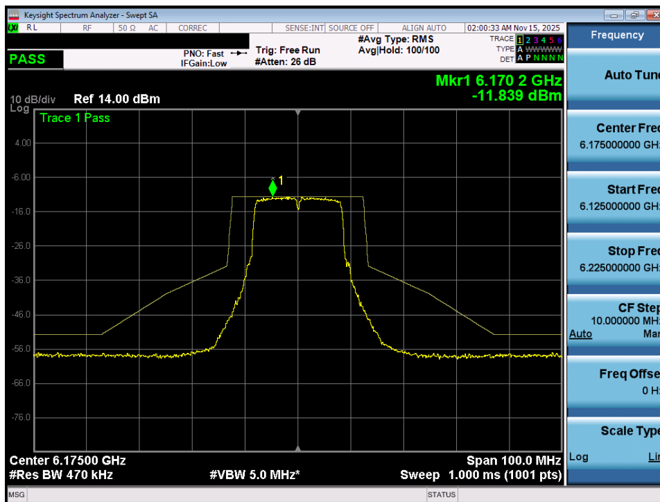
Plot 7-17. In Band Emissions Plot MIMO ANT1 (20MHz 802.11a (UNII Band 5) – Ch. 45) - VLP
