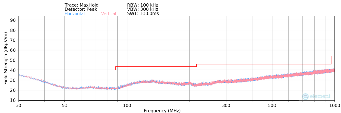
Plot 7-47. Radiated Spurious Plot below 1GHz MIMO (802.11a)
