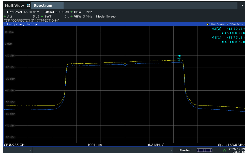
Plot 7-46. Power Spectral Density Plot – ANT2 (80MHz Bandwidth, RSSI level at -44dBm (yellow) and -28dBm (blue))
