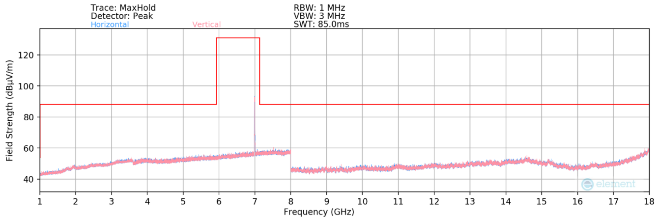
Plot 7-51. Radiated Spurious Plot 1GHz – 18GHz MIMO (802.11a – UNII Band 8 Ch. 209)
