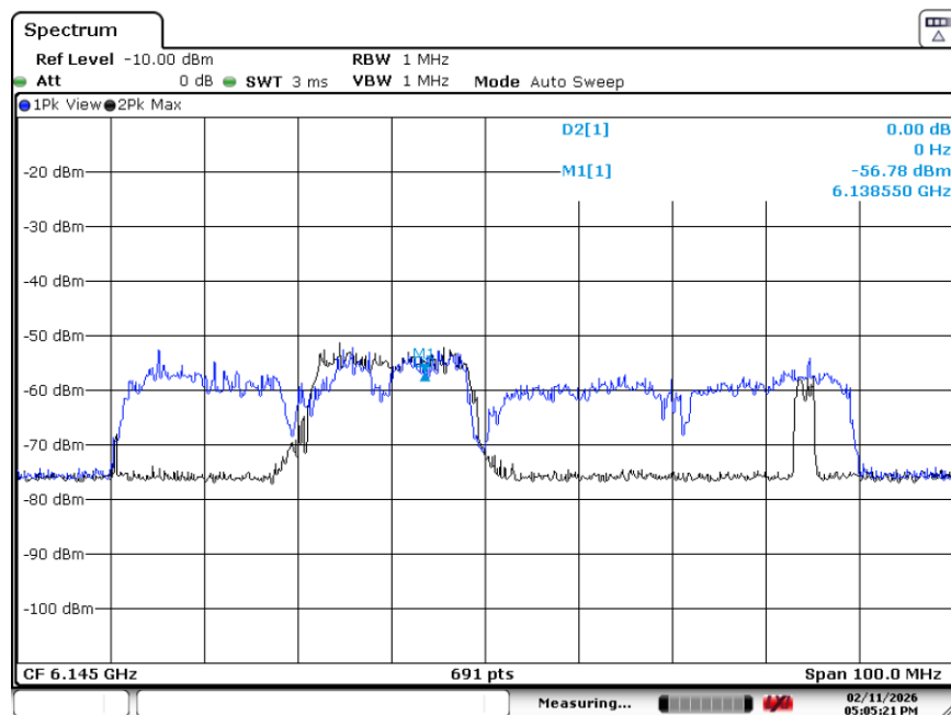
Plot 7-42. CBP 80MHz Channel - Injection Lower Edge – [6110 MHz]
