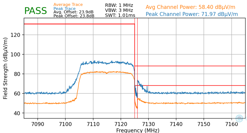
Plot 7-55. Radiated Upper Band Edge Plot MIMO (Average & Peak – UNII Band 8)
