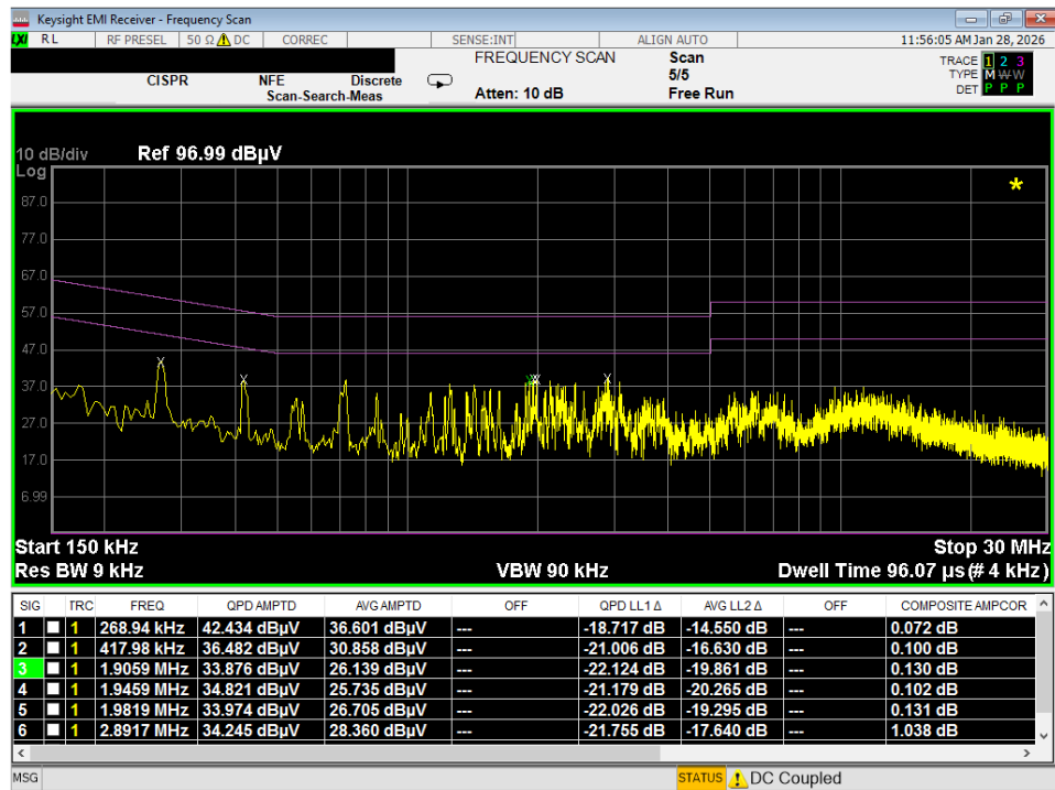
Plot 7-67. Line Conducted Plot with 802.11a UNII Band 8 (N)
