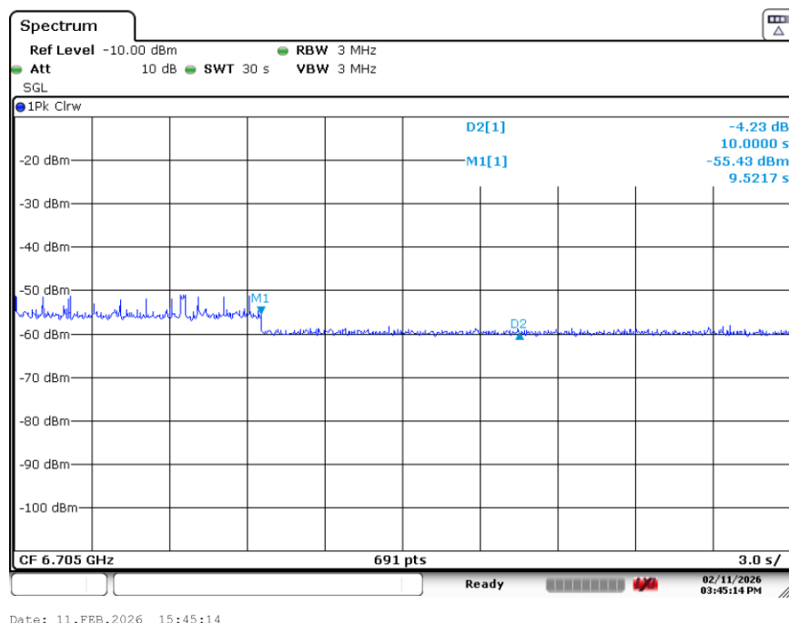
Plot 7-36. Contention Based Protocol Timing Plot (80MHz (UNII Band 7) – Ch. 151 Mid)
