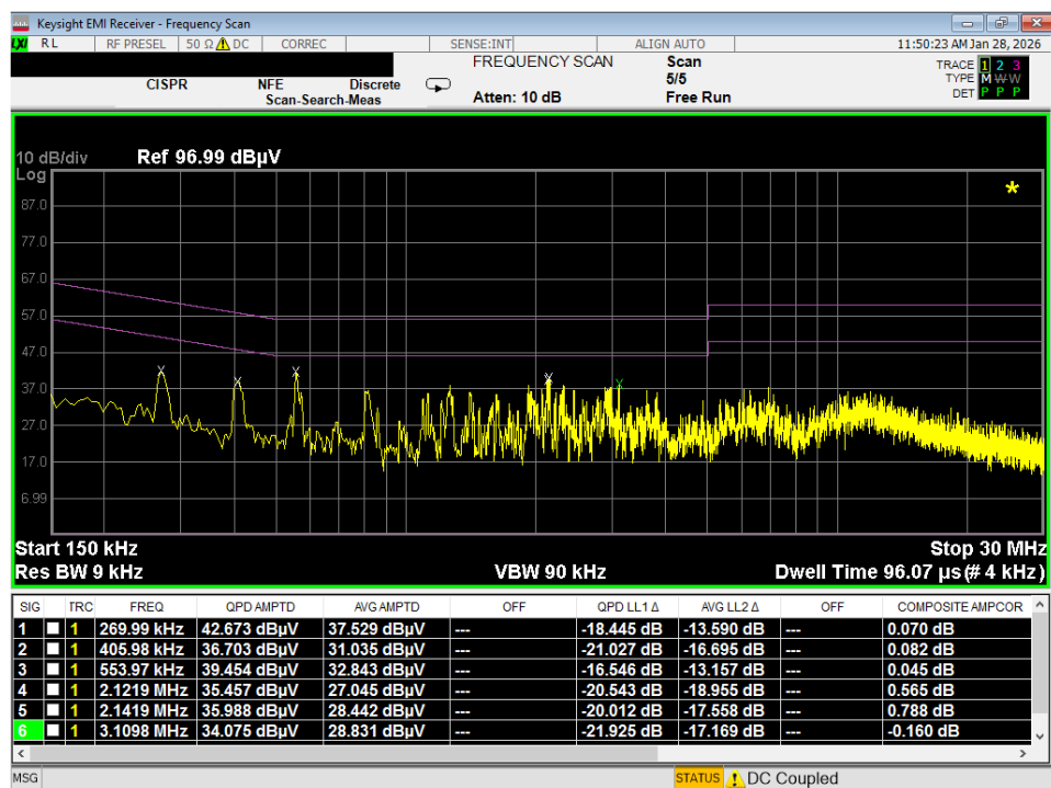
Plot 7-63. Line Conducted Plot with 802.11a UNII Band 6 (N)
