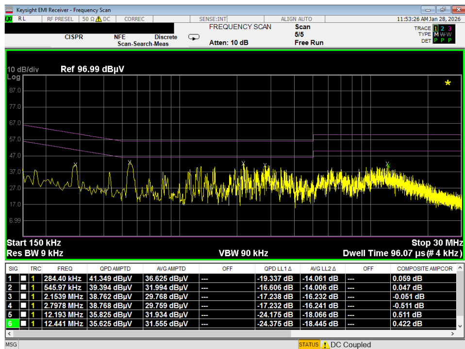
Plot 7-64. Line Conducted Plot with 802.11a UNII Band 7 (L1)
