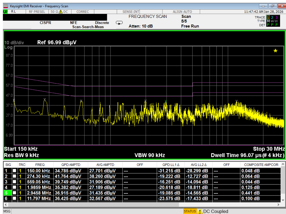
Plot 7-60. Line Conducted Plot with 802.11a UNII Band 5 (L1)
