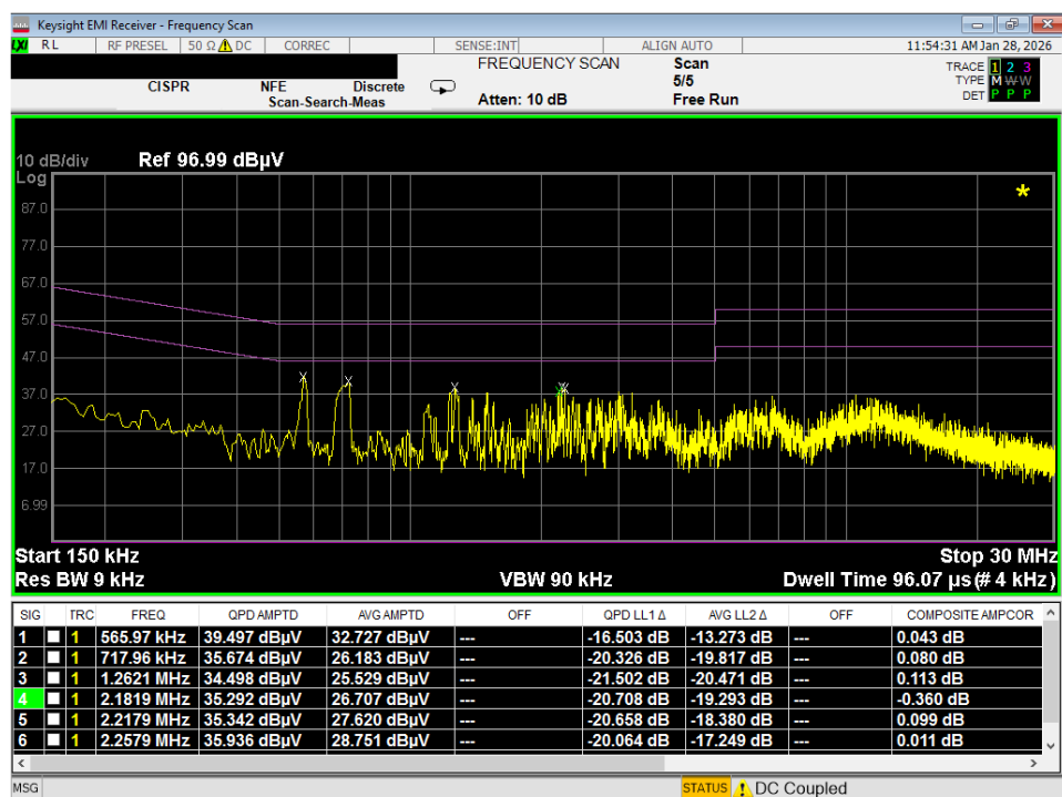
Plot 7-65. Line Conducted Plot with 802.11a UNII Band 7 (N)
