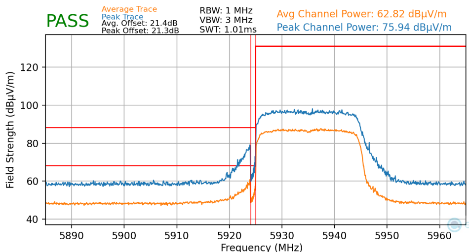
Plot 7-54. Radiated Lower Band Edge Plot MIMO (Average & Peak – UNII Band 5)
