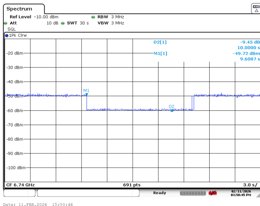
Plot 7-37. Contention Based Protocol Timing Plot (80MHz (UNII Band 7) – Ch. 151 High)
