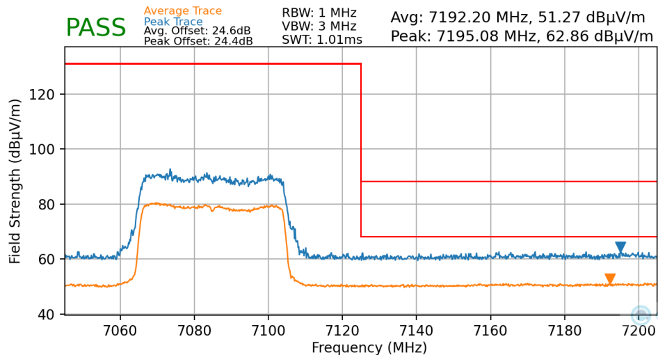
Plot 7-57. Radiated Upper Band Edge Plot MIMO (Average & Peak – UNII Band 8)
