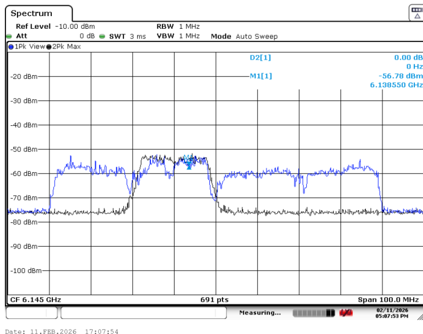
Plot 7-44. CBP 80MHz Channel - Injection Upper Edge – [6180 MHz]
