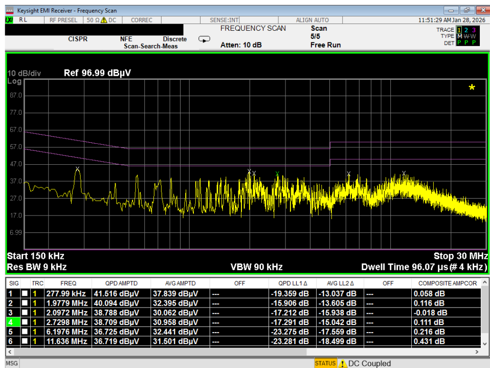
Plot 7-62. Line Conducted Plot with 802.11a UNII Band 6 (L1)
