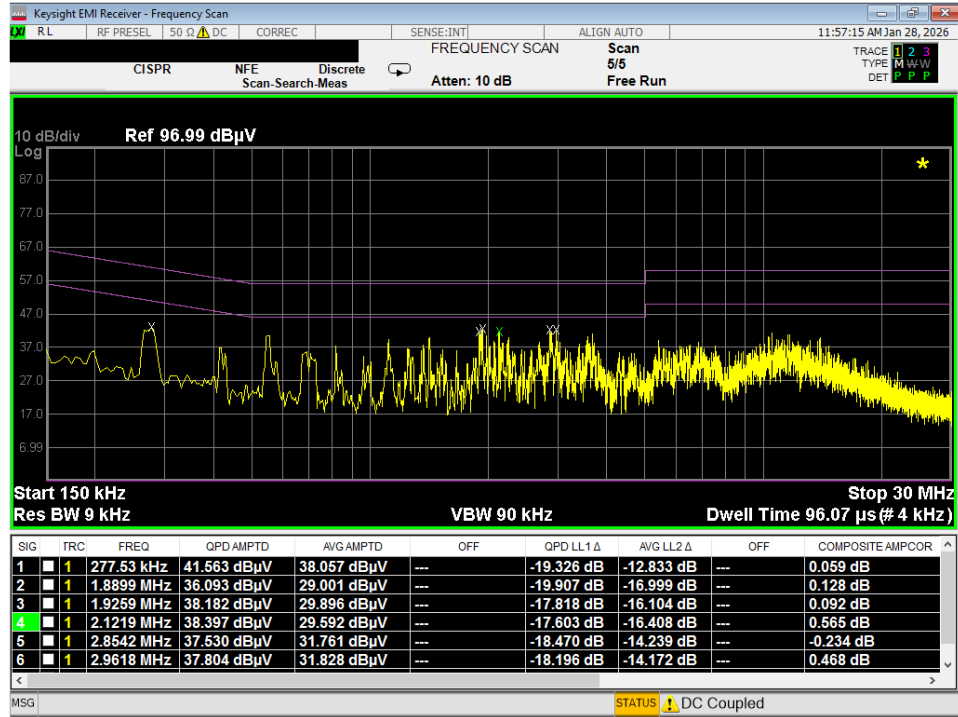
Plot 7-66. Line Conducted Plot with 802.11a UNII Band 8 (L1)
