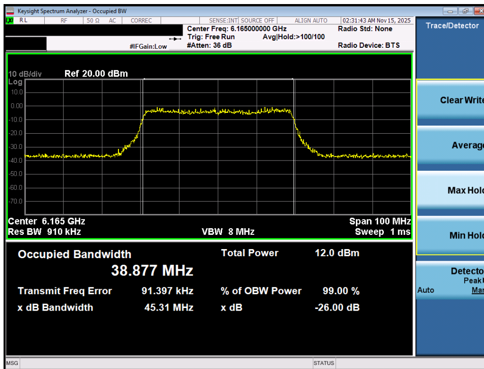
Plot 7-3. 26dB Bandwidth Plot MIMO ANT1 (40MHz 802.11ax (UNII Band 5) – Ch. 43) - VLP
