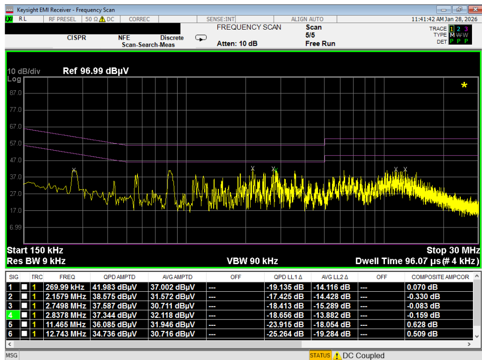
Plot 7-66. Line Conducted Plot with 802.11a UNII Band 7 (L1)
