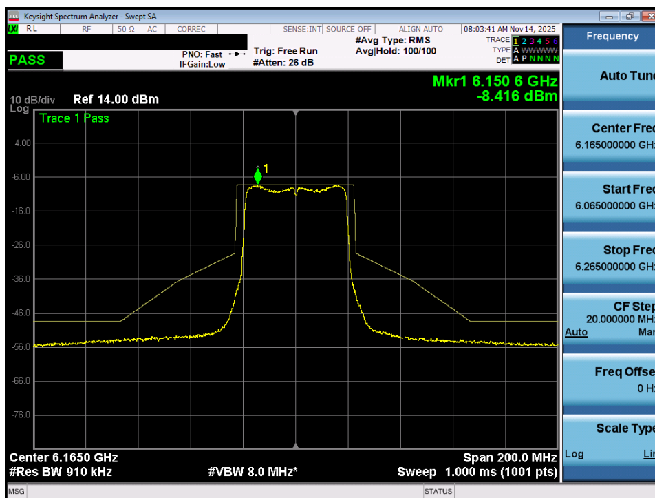
Plot 7-19. In Band Emissions Plot MIMO ANT1 (40MHz 802.11ax (UNII Band 5) – Ch. 43) - LPI/SP
