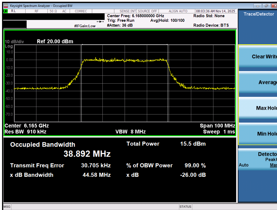
Plot 7-3. 26dB Bandwidth Plot MIMO ANT1 (40MHz 802.11ax (UNII Band 5) – Ch. 43) - LPI/SP
