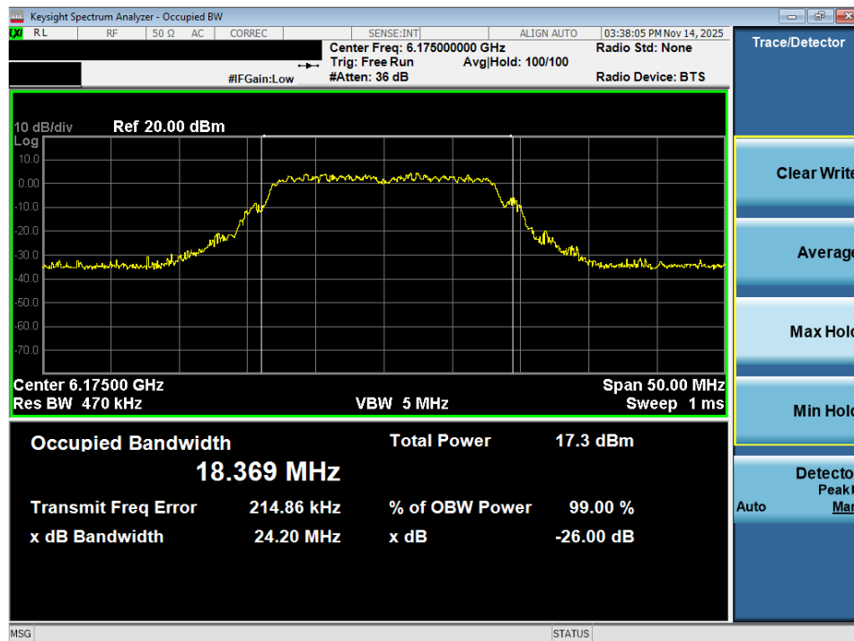
Plot 7-5. 26dB Bandwidth Plot MIMO ANT2 (20MHz 802.11a (UNII Band 5) – Ch. 45) - LPI/SP
