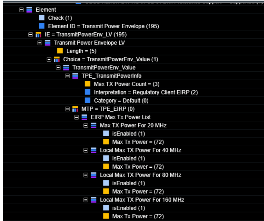
Figure 7-7. Callbox Power Authorization – 36.00dBm
