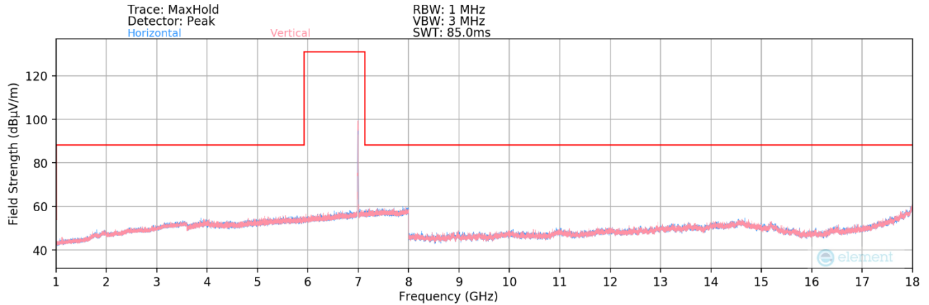
Plot 7-49. Radiated Spurious Plot 1GHz – 18GHz MIMO (802.11a – U Band 8 Ch. 209)
