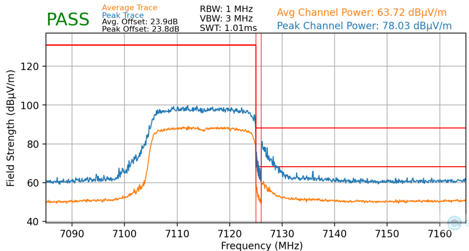
Plot 7-57. Radiated Upper Band Edge Plot MIMO (Average & Peak – UNII Band 8)
