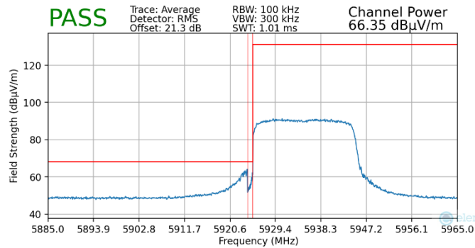
Plot 9-1. Radiated Lower Band Edge Plot MIMO (Average – UNII Band 5)
