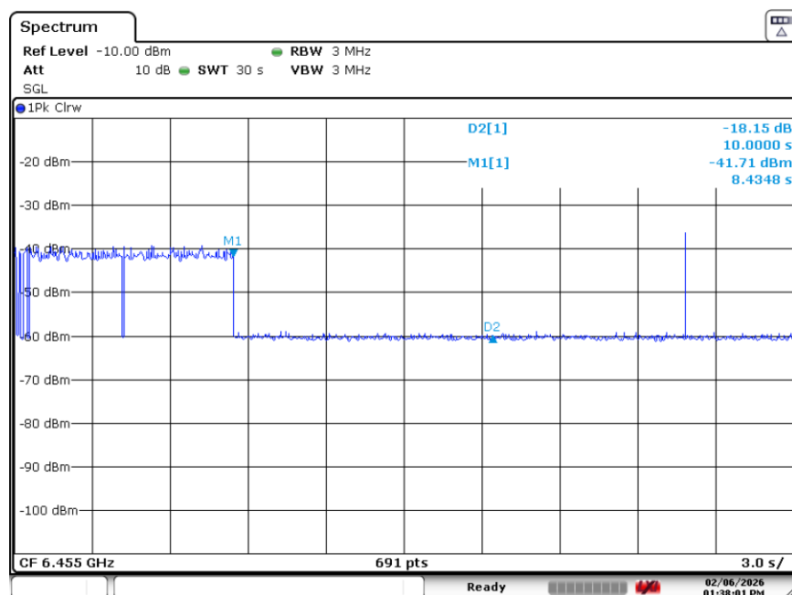
Plot 7-30. Contention Based Protocol Timing Plot (20MHz (UNII Band 6) – Ch. 101)
