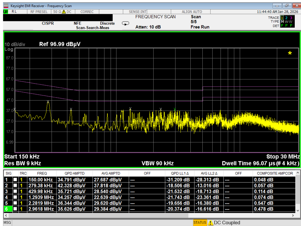
Plot 7-69. Line Conducted Plot with 802.11a UNII Band 8 (N)
