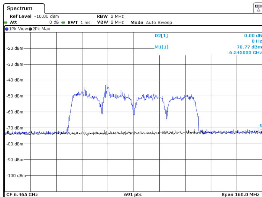
Plot 7-43. CBP 80MHz Channel - Injection Center – [6465 MHz]
