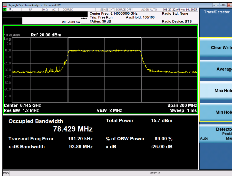
Plot 7-4. 26dB Bandwidth Plot MIMO ANT1 (80MHz 802.11ax (UNII Band 5) – Ch. 39) – LPI/SP
