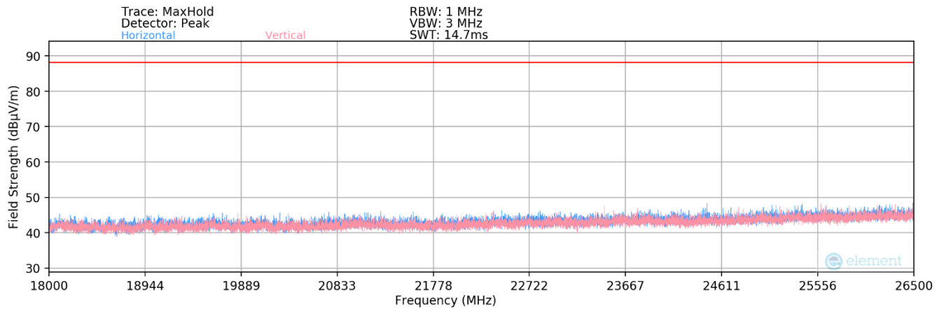
Plot 7-50. Radiated Spurious Plot 18GHz - 26.5GHz (802.11a)
