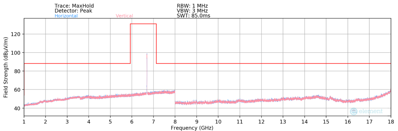
Plot 7-48. Radiated Spurious Plot 1GHz – 18GHz MIMO (802.11a – UNII Band 7 Ch. 149)
