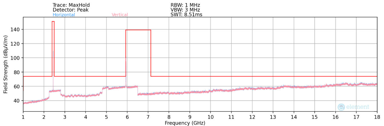
Plot 7-53. Radiated Spurious Plot above 1GHz Bluetooth (1Mbps – CH39) + MIMO 802.11a (6GHz – Ch.2)
