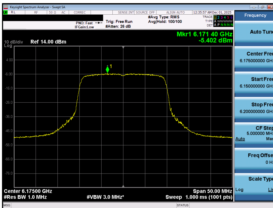
Plot 7-10. Power Spectral Density Plot MIMO ANT1 (20MHz 802.11ax (UNII Band 5) – Ch. 45) - LPI/SP
