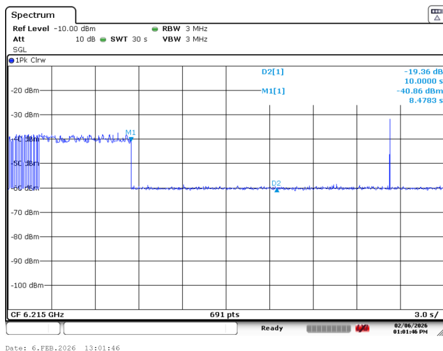
Plot 7-26. Contention Based Protocol Timing Plot (20MHz (UNII Band 5) – Ch. 53)
