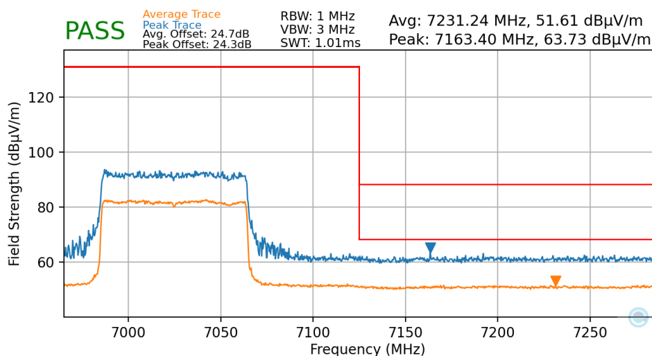
Plot 7-61. Radiated Upper Band Edge Plot MIMO (Average & Peak – UNII Band 8)
