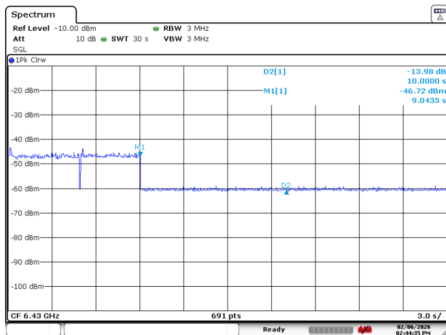
Plot 7-31. Contention Based Protocol Timing Plot (80MHz (UNII Band 6) – Ch. 103 Low)
