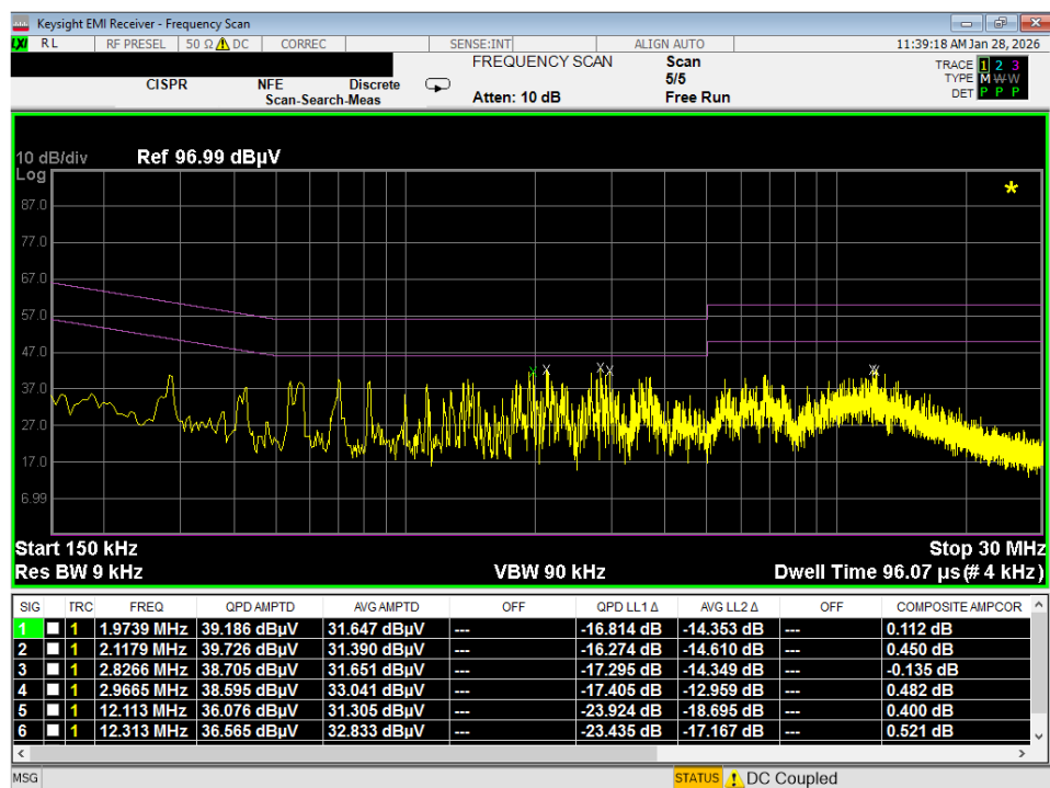
Plot 7-64. Line Conducted Plot with 802.11a UNII Band 6 (L1)
