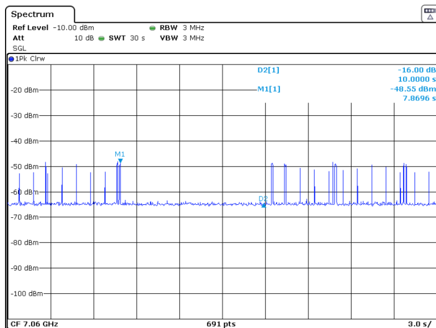
Plot 7-41. Contention Based Protocol Timing Plot (80MHz (UNII Band 8) – Ch. 215 High)
