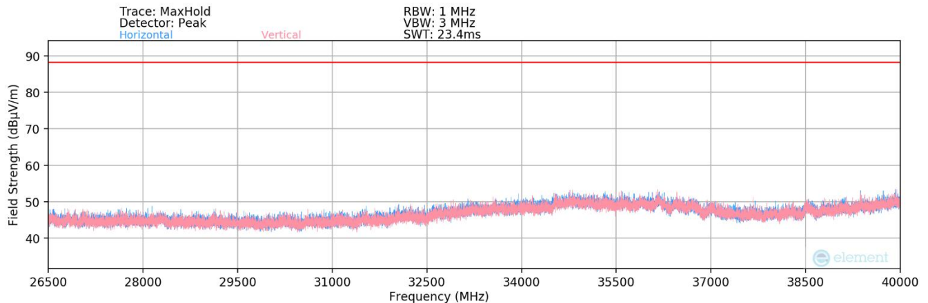
Plot 7-51. Radiated Spurious Plot 26.5GHz - 40GHz (802.11a)
