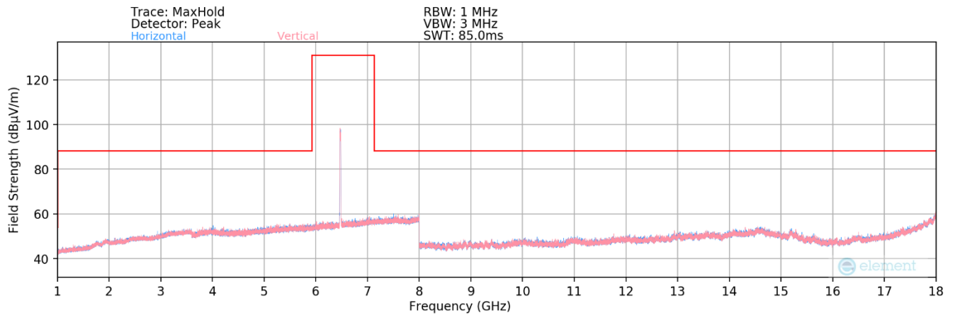
Plot 7-47. Radiated Spurious Plot 1GHz – 18GHz MIMO (802.11a – UNII Band 6 Ch. 105)
