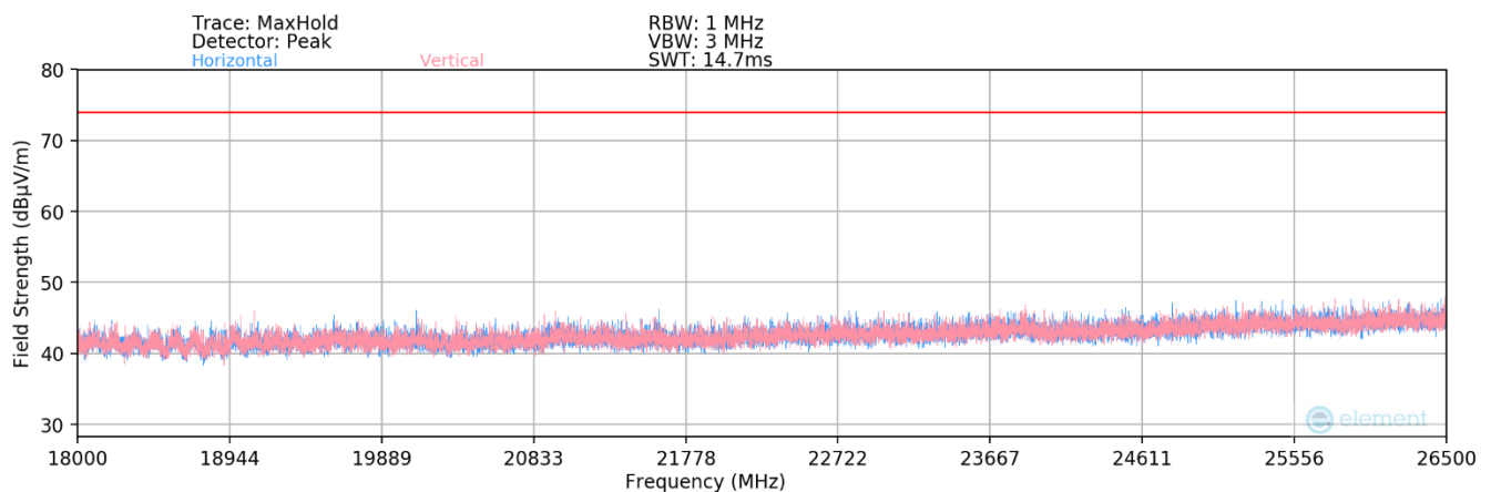
Plot 7-54. Radiated Spurious Plot 18GHz – 26.5GHz Bluetooth (1Mbps – CH39) + MIMO 802.11a (6GHz – Ch.2)
