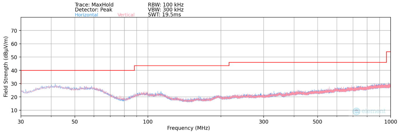
Plot 7-52. Radiated Spurious Plot below 1GHz Bluetooth (1Mbps – CH39) + MIMO 802.11a (6GHz – Ch.2)
