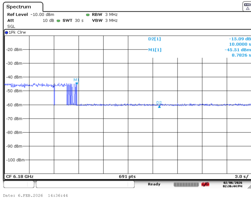
Plot 7-29. Contention Based Protocol Timing Plot (80MHz (UNII Band 5) – Ch. 39 High)
