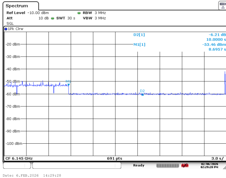
Plot 7-28. Contention Based Protocol Timing Plot (80MHz (UNII Band 5) – Ch. 39 Mid)
