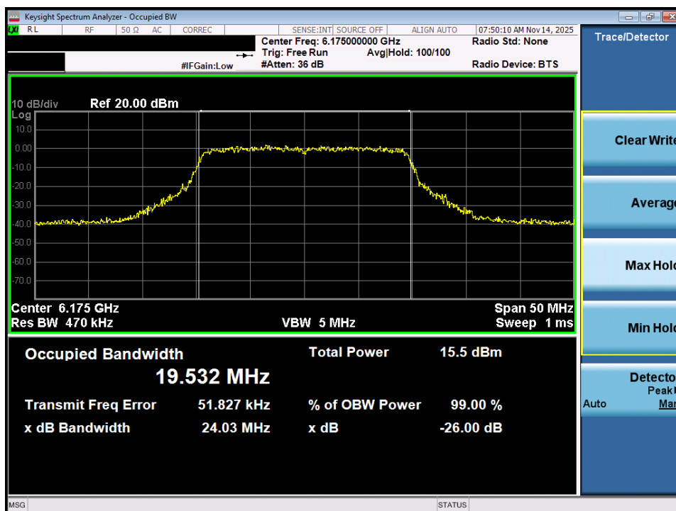
Plot 7-2. 26dB Bandwidth Plot MIMO ANT1 (20MHz 802.11ax (UNII Band 5) – Ch. 45) - LPI/SP
