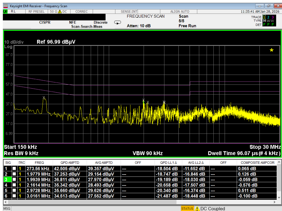
Plot 7-63. Line Conducted Plot with 802.11a UNII Band 5 (N)
