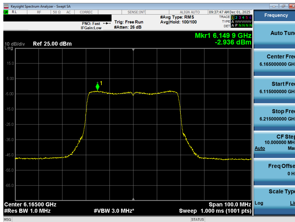
Plot 7-15. Power Spectral Density Plot MIMO ANT2 (40MHz 802.11ax (UNII Band 5) – Ch. 43) - LPI/SP
