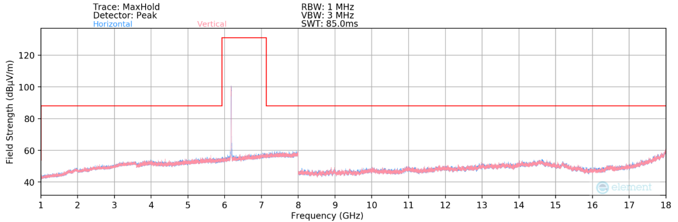
Plot 7-46. Radiated Spurious Plot 1GHz – 18GHz MIMO (802.11a – UNII Band 5 Ch. 45)
