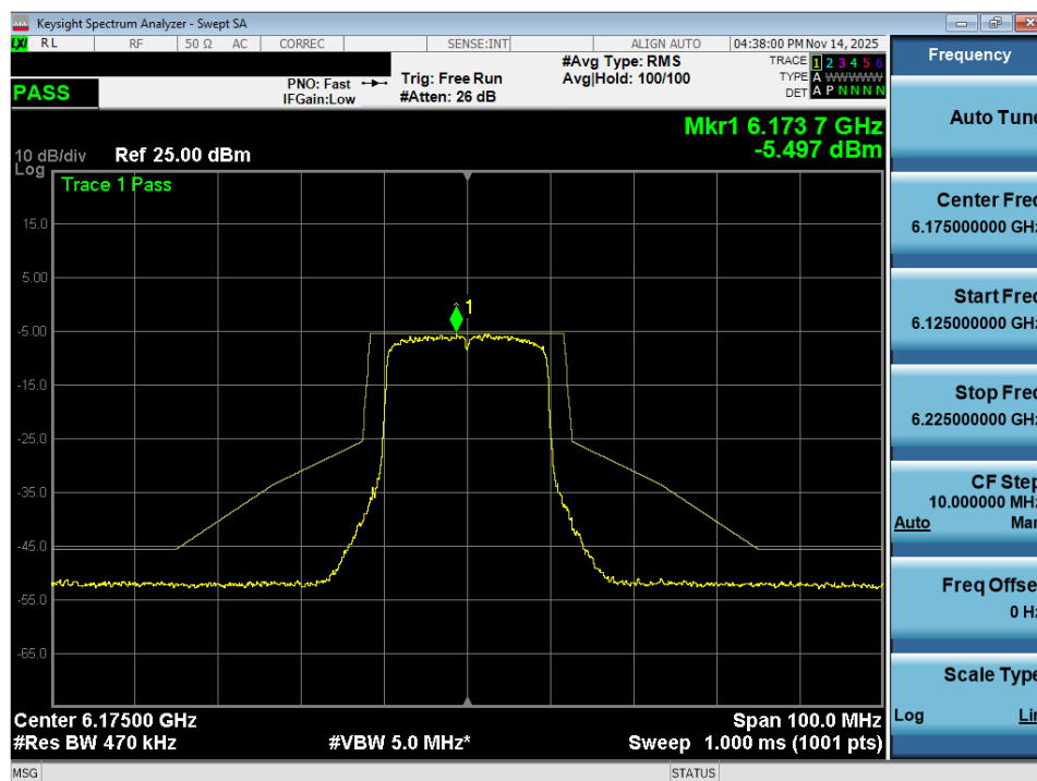
Plot 7-22. In Band Emissions Plot MIMO ANT2 (20MHz 802.11ax (UNII Band 5) – Ch. 45) - LPI/SP
