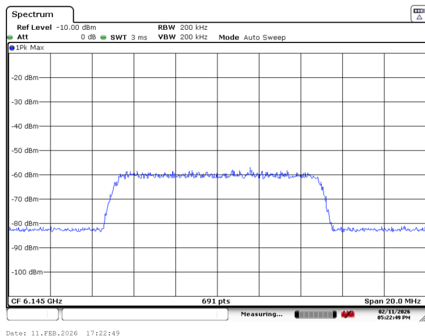
Plot 7-25. AWGN Signal (Demonstration)
