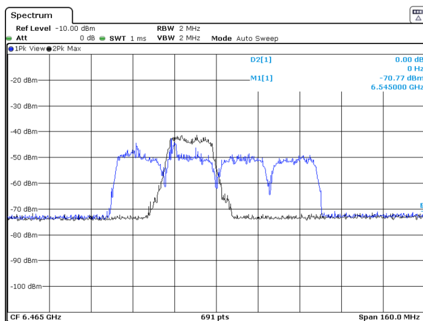
Plot 7-42. CBP 80MHz Channel - Injection Lower Edge – [6430 MHz]
