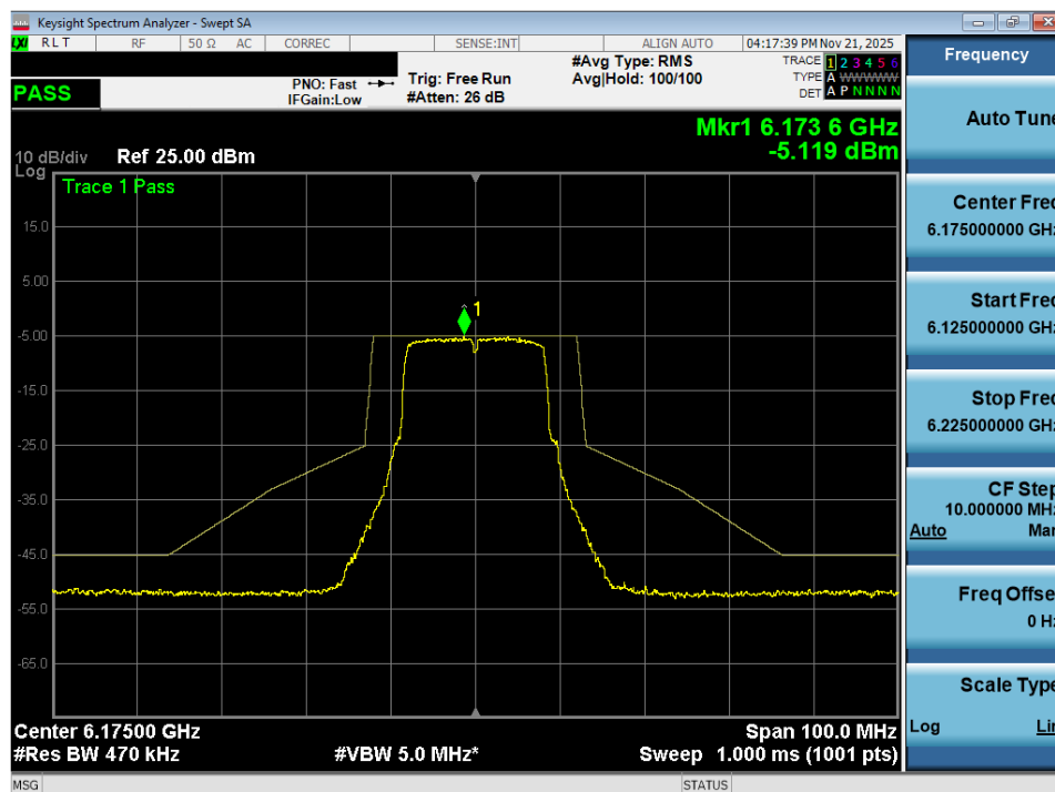
Plot 7-21. In Band Emissions Plot MIMO ANT2 (20MHz 802.11a (UNII Band 5) – Ch. 45) - LPI/SP
