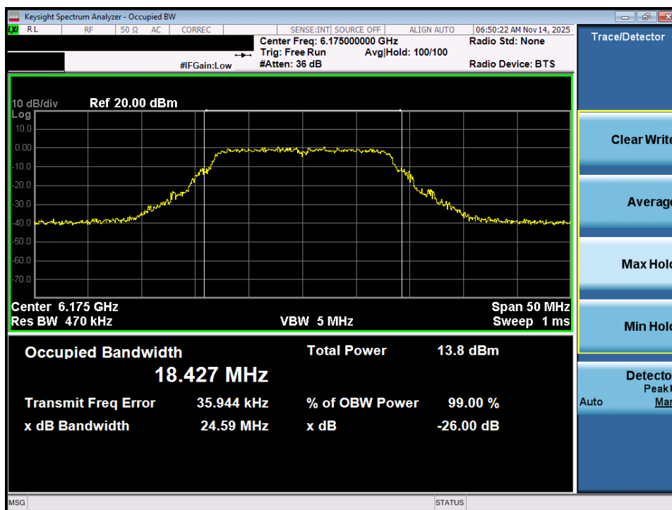
Plot 7-1. 26dB Bandwidth Plot MIMO ANT1 (20MHz 802.11a (UNII Band 5) – Ch. 45) - LPI/SP
