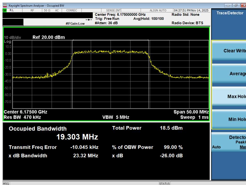
Plot 7-6. 26dB Bandwidth Plot MIMO ANT2 (20MHz 802.11ax (UNII Band 5) – Ch. 45) - LPI/SP
