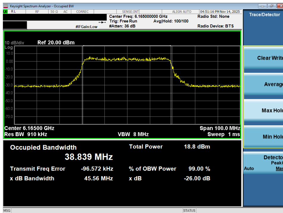
Plot 7-7. 26dB Bandwidth Plot MIMO ANT2 (40MHz 802.11ax (UNII Band 5) – Ch. 43) - LPI/SP
