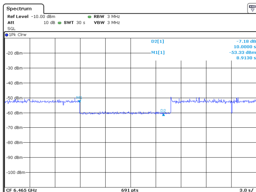
Plot 7-32. Contention Based Protocol Timing Plot (80MHz (UNII Band 6) – Ch. 103 Mid)
