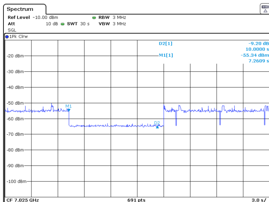
Plot 7-40. Contention Based Protocol Timing Plot (80MHz (UNII Band 8) – Ch. 215 Mid)
