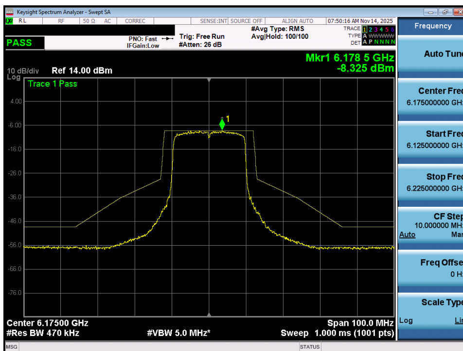
Plot 7-18. In Band Emissions Plot MIMO ANT1 (20MHz 802.11ax (UNII Band 5) – Ch. 45) - LPI/SP
