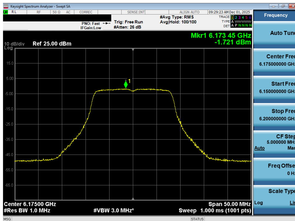
Plot 7-13. Power Spectral Density Plot MIMO ANT2 (20MHz 802.11a (UNII Band 5) – Ch. 45) - LPI/SP
