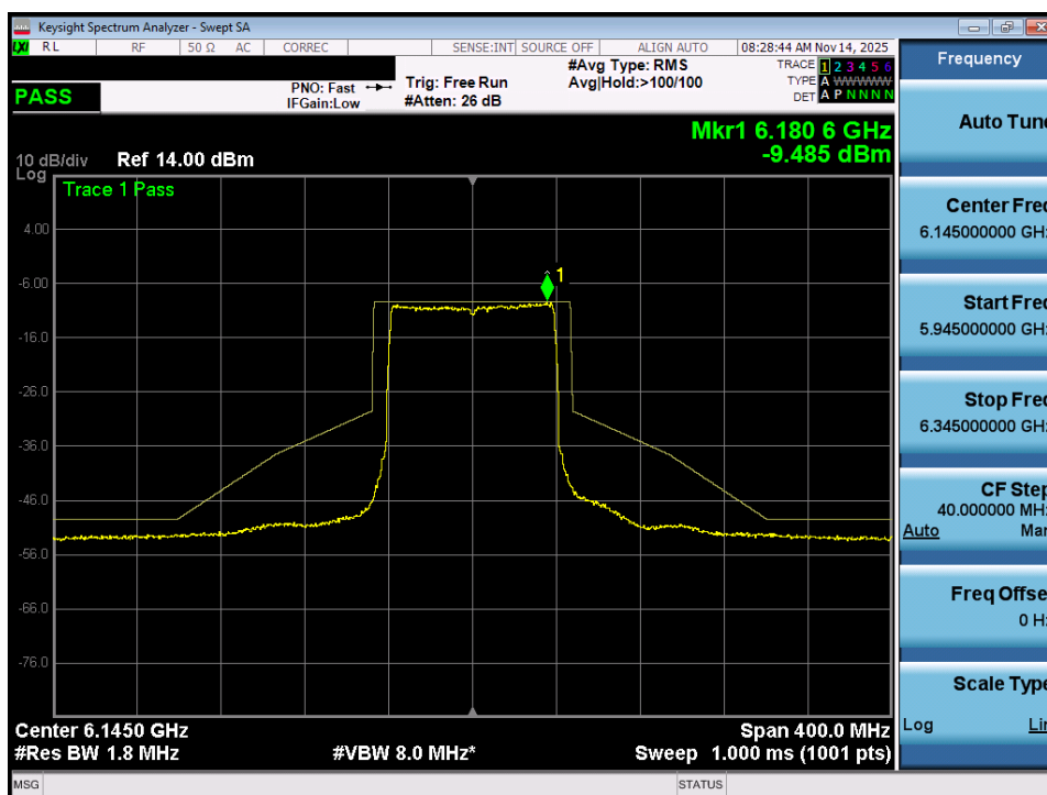
Plot 7-20. In Band Emissions Plot MIMO ANT1 (80MHz 802.11ax (UNII Band 5) – Ch. 39) – LPI/SP
