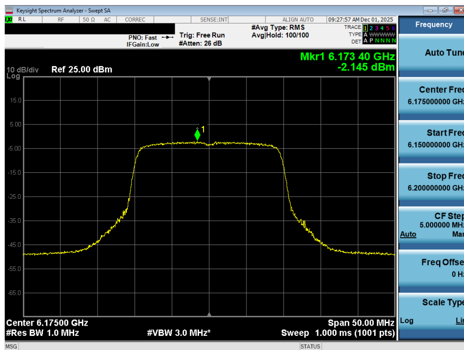
Plot 7-14. Power Spectral Density Plot MIMO ANT2 (20MHz 802.11ax (UNII Band 5) – Ch. 45) - LPI/SP
