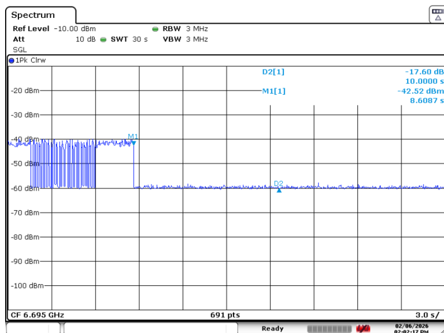
Plot 7-34. Contention Based Protocol Timing Plot (20MHz (UNII Band 7) – Ch. 149)
