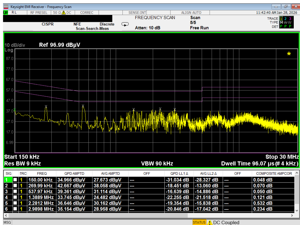
Plot 7-67. Line Conducted Plot with 802.11a UNII Band 7 (N)
