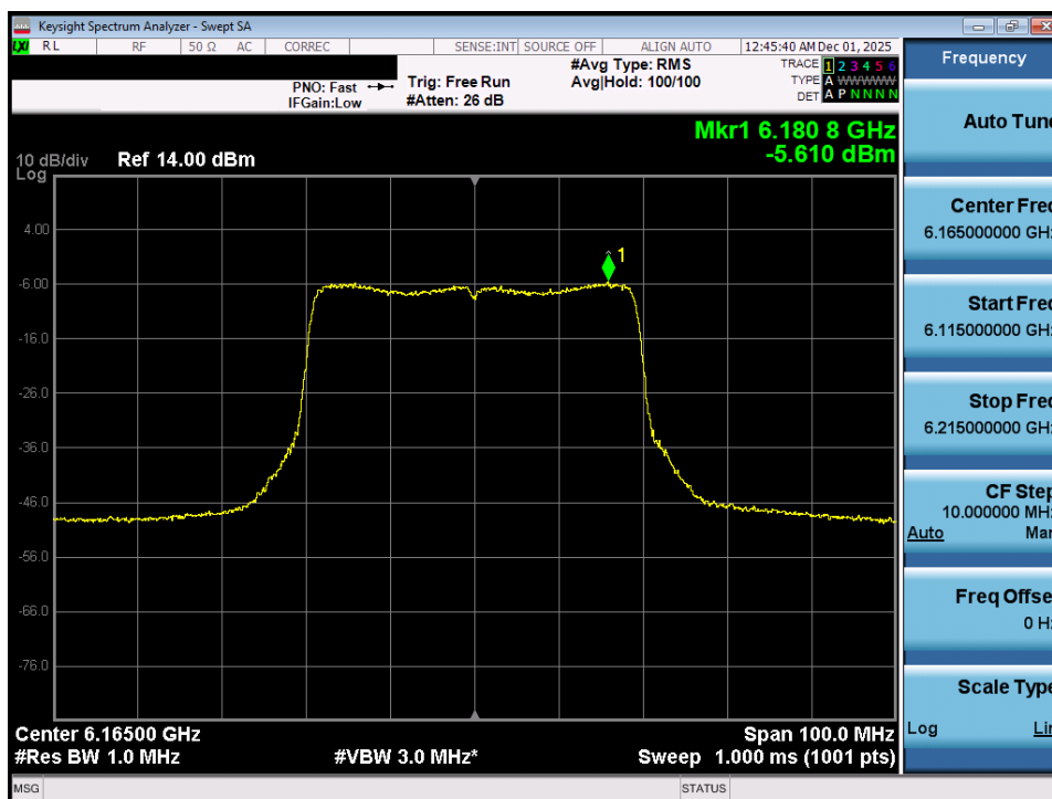
Plot 7-11. Power Spectral Density Plot MIMO ANT1 (40MHz 802.11ax (UNII Band 5) – Ch. 43) - LPI/SP
