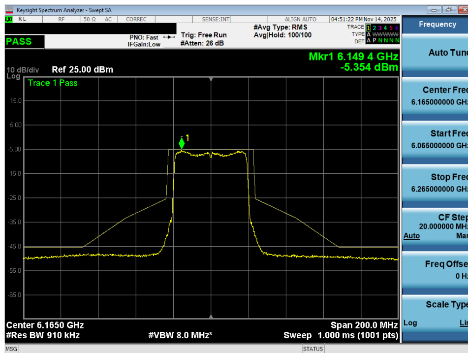
Plot 7-23. In Band Emissions Plot MIMO ANT2 (40MHz 802.11ax (UNII Band 5) – Ch. 43) - LPI/SP
