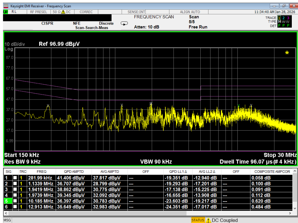
Plot 7-62. Line Conducted Plot with 802.11a UNII Band 5 (L1)
