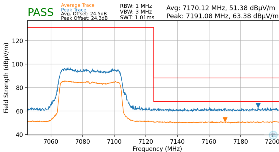
Plot 7-59. Radiated Upper Band Edge Plot MIMO (Average & Peak – UNII Band 8)
