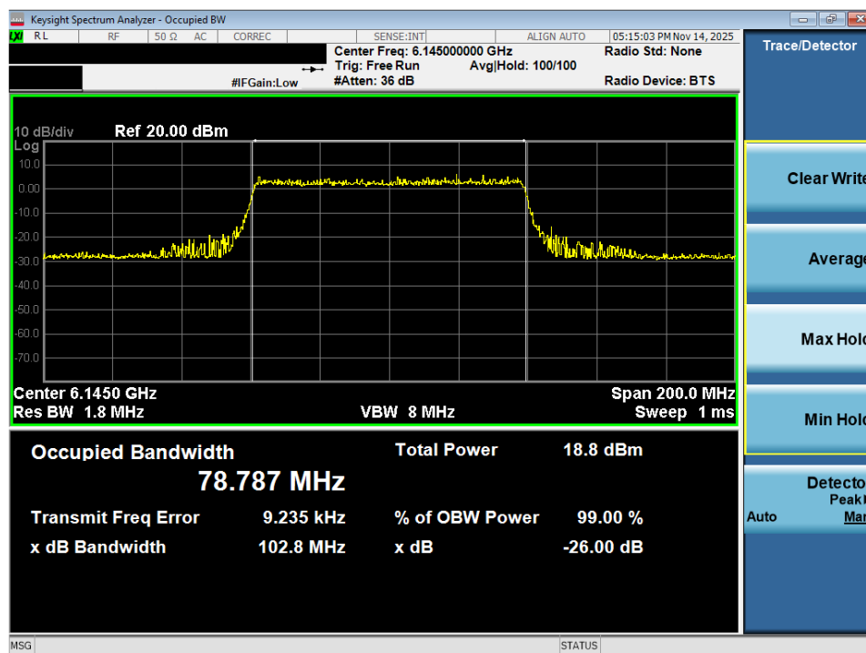
Plot 7-8. 26dB Bandwidth Plot MIMO ANT2 (80MHz 802.11ax (UNII Band 5) – Ch. 39) – LPI/SP
