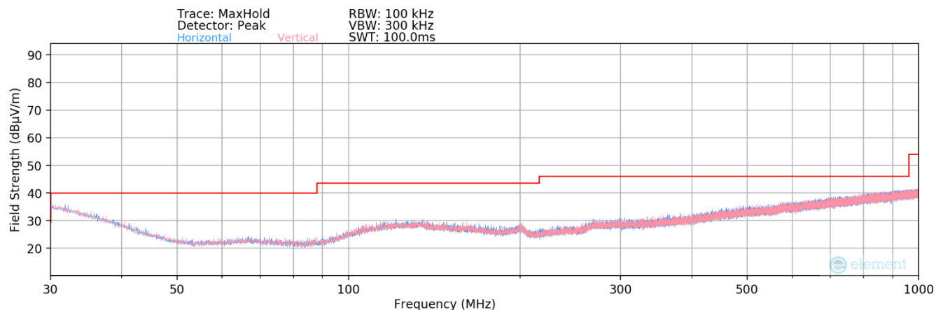
Plot 7-45. Radiated Spurious Plot below 1GHz MIMO (802.11a)
