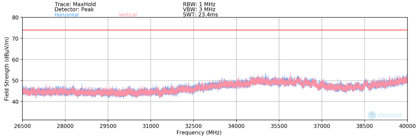
Plot 7-55. Radiated Spurious Plot 26.5GHz – 40GHz Bluetooth (1Mbps – CH39) + MIMO 802.11a (6GHz – Ch.2)
