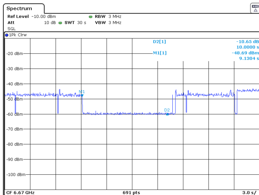
Plot 7-35. Contention Based Protocol Timing Plot (80MHz (UNII Band 7) – Ch. 151 Low)
