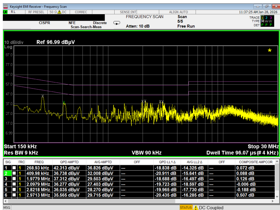
Plot 7-65. Line Conducted Plot with 802.11a UNII Band 6 (N)
