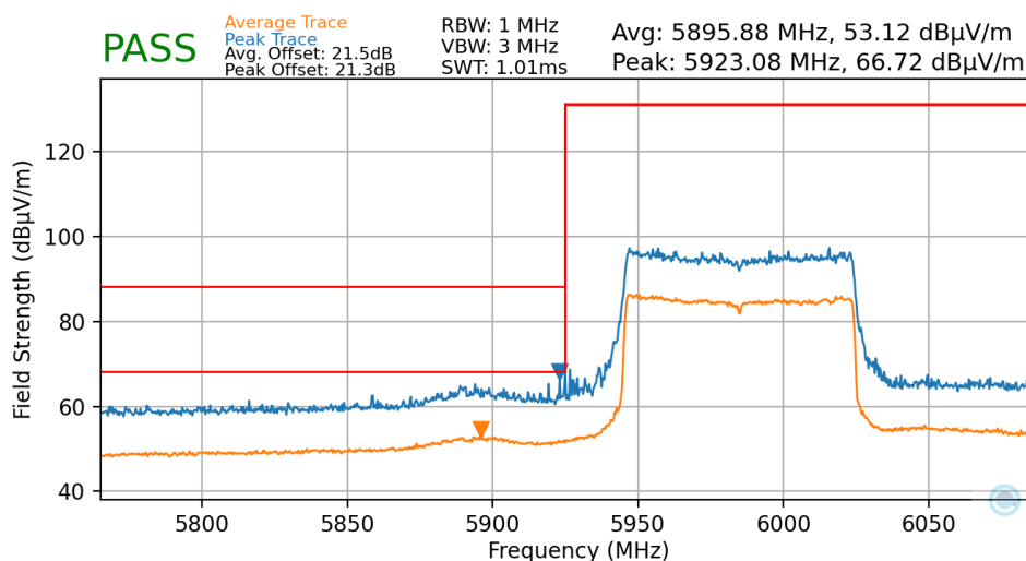
Plot 7-60. Radiated Lower Band Edge Plot MIMO (Average & Peak – UNII Band 5)
