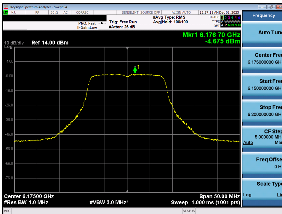
Plot 7-9. Power Spectral Density Plot MIMO ANT1 (20MHz 802.11a (UNII Band 5) – Ch. 45) - LPI/SP
