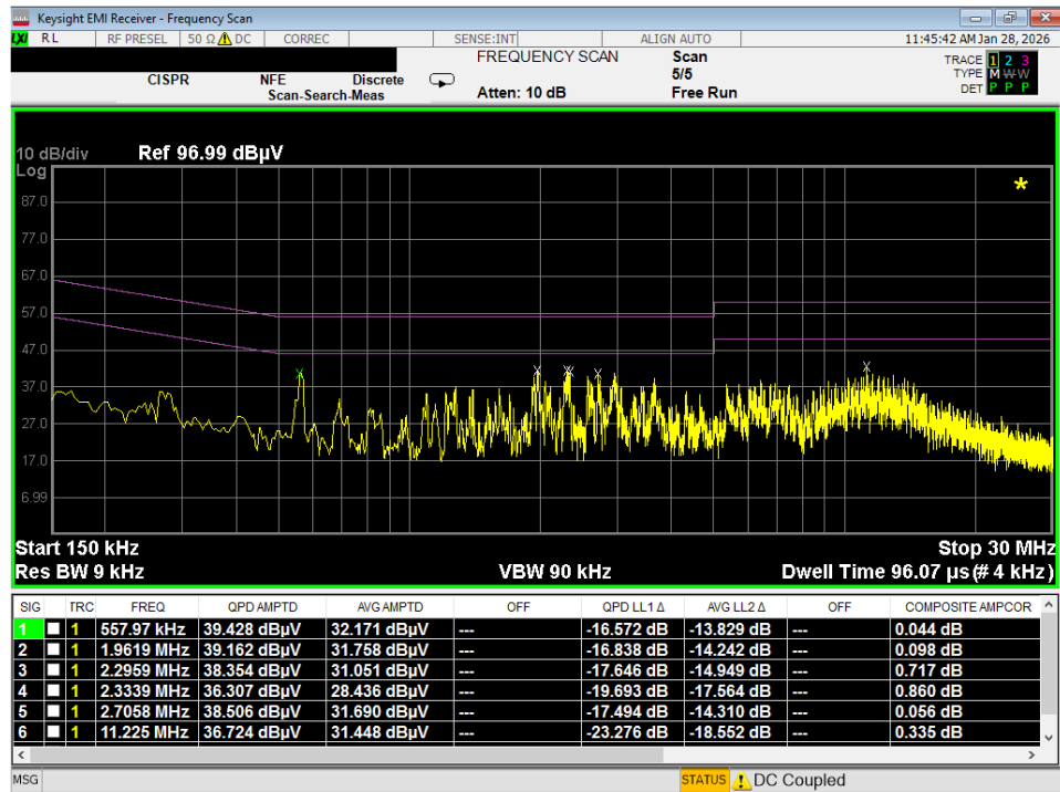
Plot 7-68. Line Conducted Plot with 802.11a UNII Band 8 (L1)
