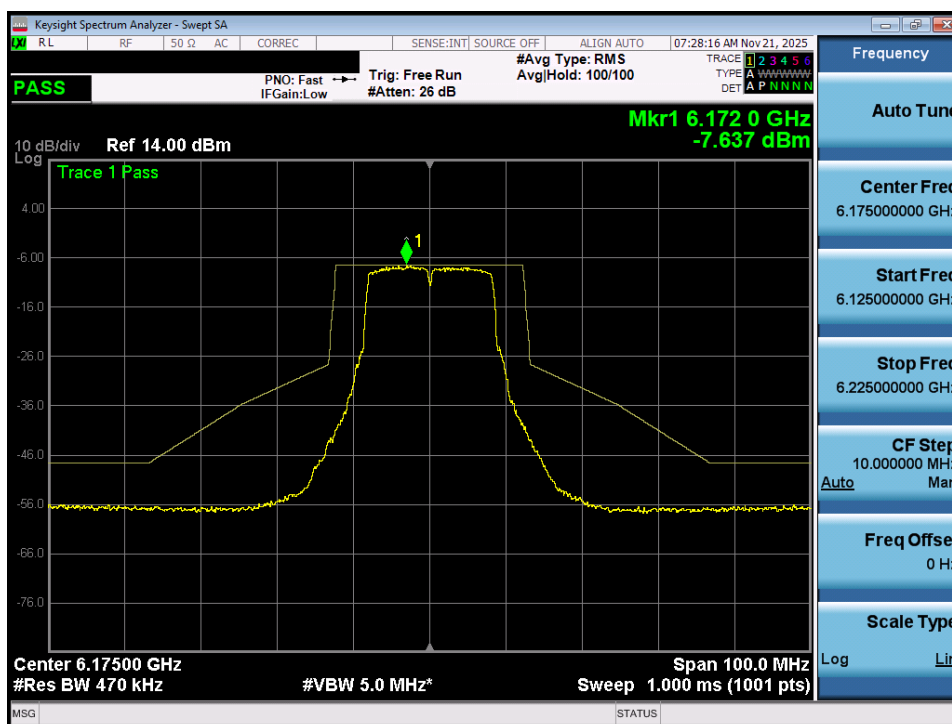
Plot 7-17. In Band Emissions Plot MIMO ANT1 (20MHz 802.11a (UNII Band 5) – Ch. 45) - LPI/SP
