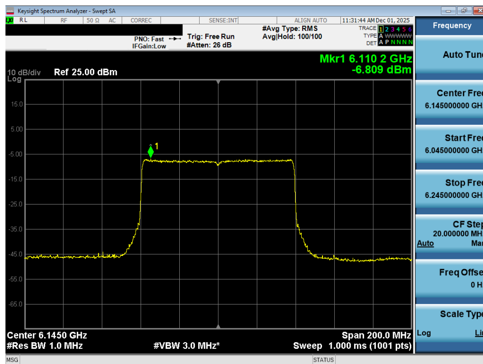
Plot 7-16. Power Spectral Density Plot MIMO ANT2 (80MHz 802.11ax (UNII Band 5) – Ch. 39) – LPI/SP
