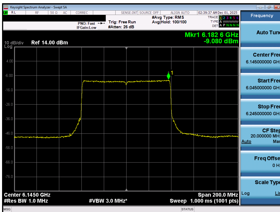
Plot 7-12. Power Spectral Density Plot MIMO ANT1 (80MHz 802.11ax (UNII Band 5) – Ch. 39) - LPI/SP
