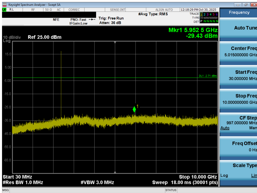
Plot 7-57. Conducted Spurious Plot (Bluetooth (LE), 1Mbps – Ch. 37)
