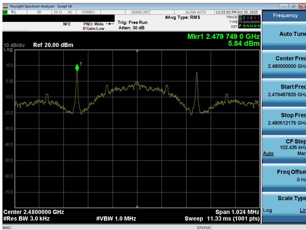
Plot 7-39. Power Spectral Density Plot (Bluetooth (LE), 125kbps – Ch. 39)
