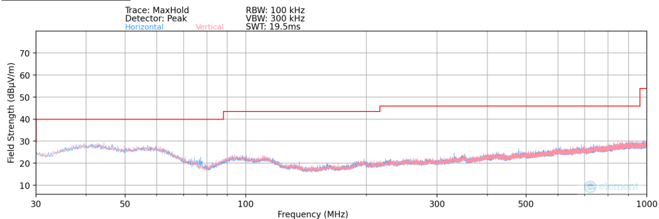
Plot 7-69. Radiated Spurious Plot below 1GHz
