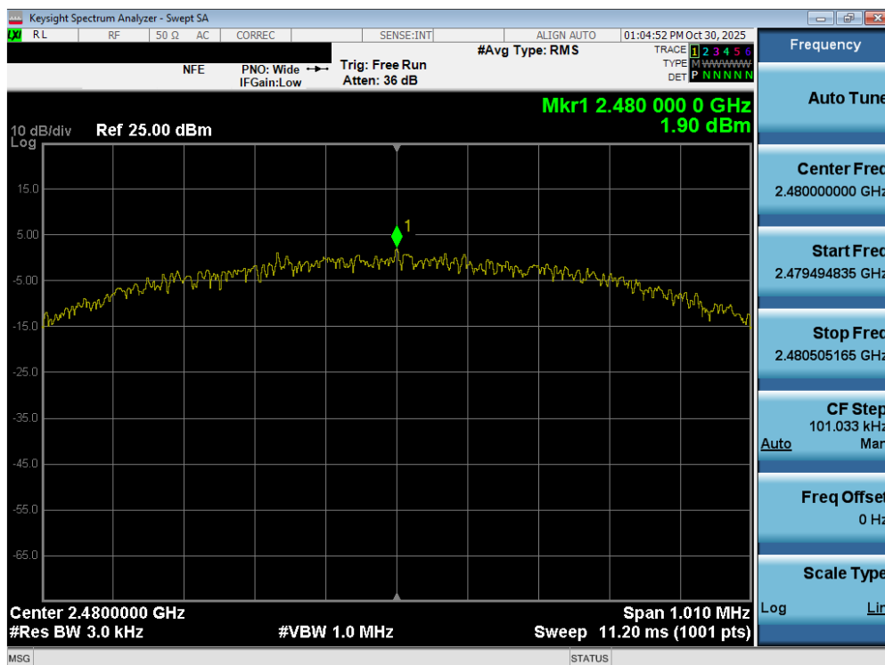
Plot 7-45. Power Spectral Density Plot (Bluetooth (LE), 1Mbps – Ch. 39)
