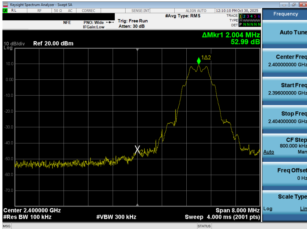
Plot 7-49. Band Edge Plot (Bluetooth (LE), 125kbps – Ch. 37)
