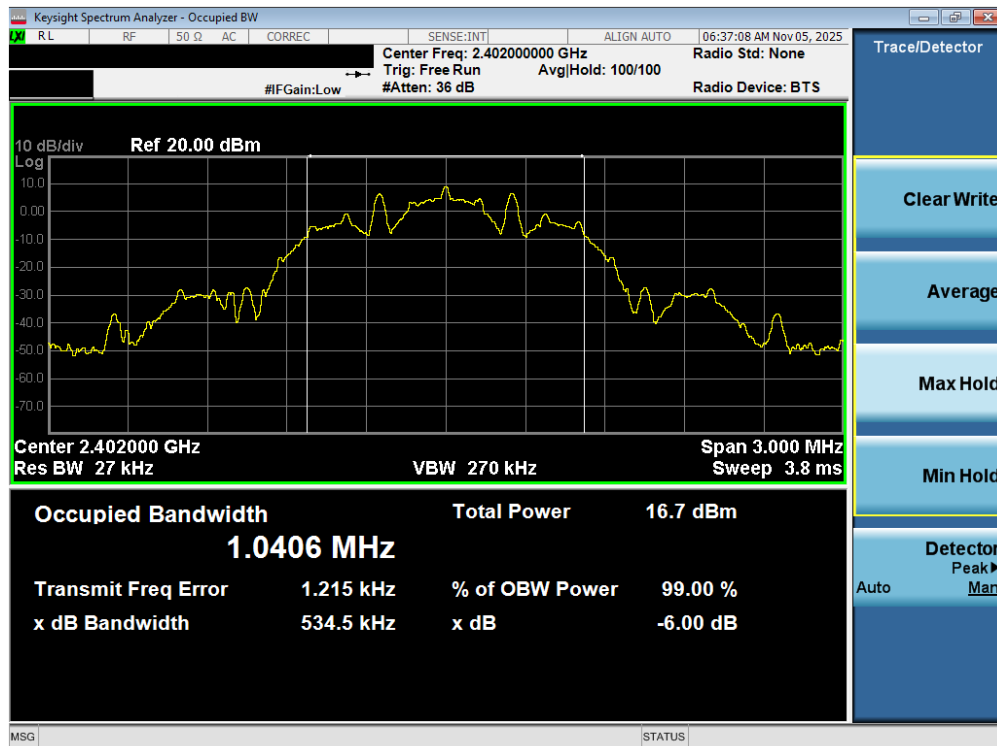
Plot 7-13. OBW Plot (Bluetooth (LE), 125kbps – Ch. 37)
