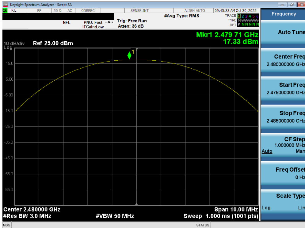
Plot 7-33. Peak Power Plot (Bluetooth (LE), 1Mbps – Ch. 39)
