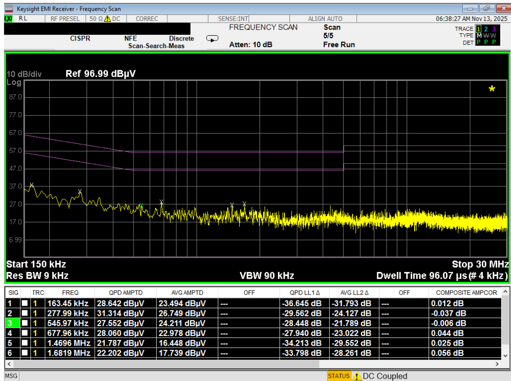
Plot 7-71. Line Conducted Plot with Bluetooth LE (N)
