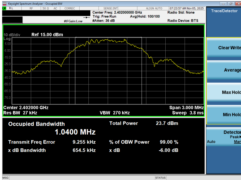
Plot 7-19. OBW Plot (Bluetooth (LE), 1Mbps – Ch. 37)
