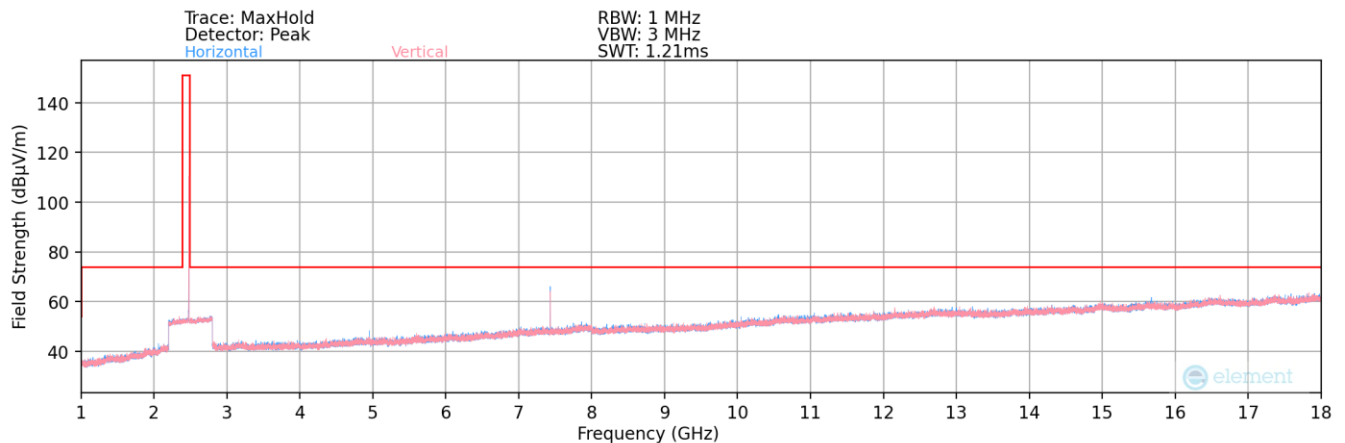
Plot 7-65. Radiated Spurious Plot above 1GHz (Bluetooth (LE) – Ch. 39)
