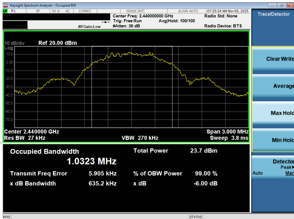
Plot 7-20. OBW Plot (Bluetooth (LE), 1Mbps – Ch. 17)
