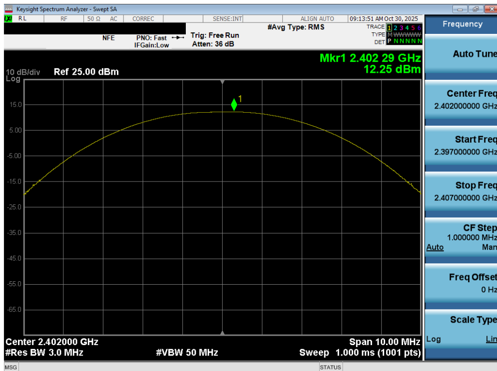
Plot 7-28. Peak Power Plot (Bluetooth (LE), 500kbps – Ch. 37)
