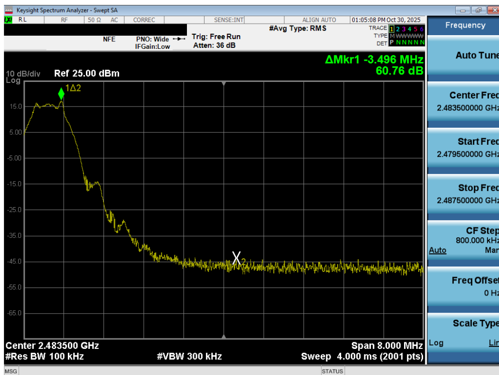
Plot 7-54. Band Edge Plot (Bluetooth (LE), 1Mbps – Ch. 39)
