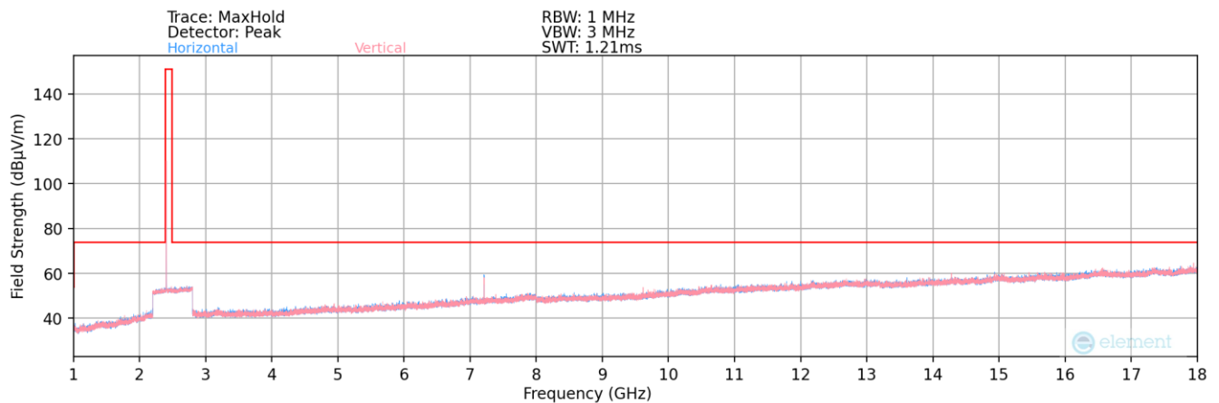
Plot 7-63. Radiated Spurious Plot above 1GHz (Bluetooth (LE) – Ch. 37)
