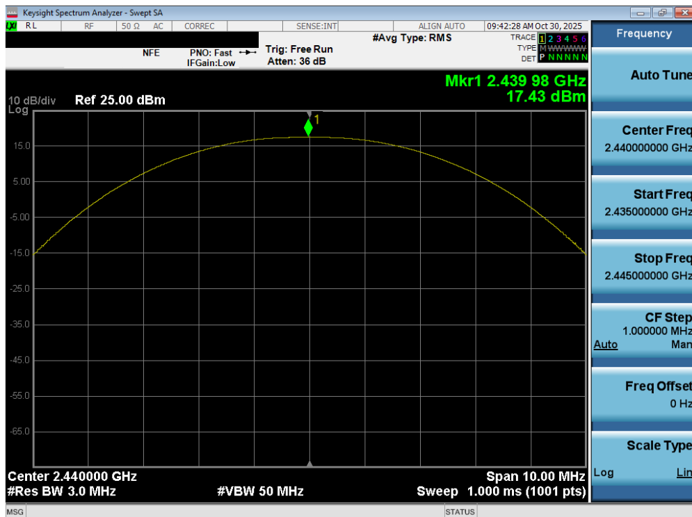
Plot 7-32. Peak Power Plot (Bluetooth (LE), 1Mbps – Ch. 17)
