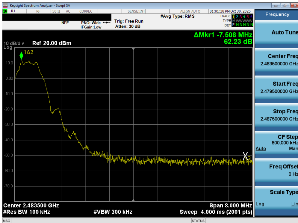
Plot 7-52. Band Edge Plot (Bluetooth (LE), 500kbps – Ch. 39)
