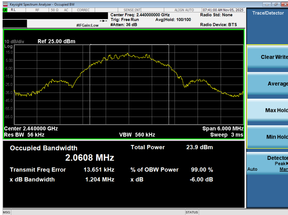
Plot 7-23. OBW Plot (Bluetooth (LE), 2Mbps – Ch. 17)
