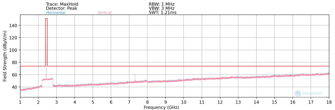
Plot 7-64. Radiated Spurious Plot above 1GHz (Bluetooth (LE) – Ch. 17)
