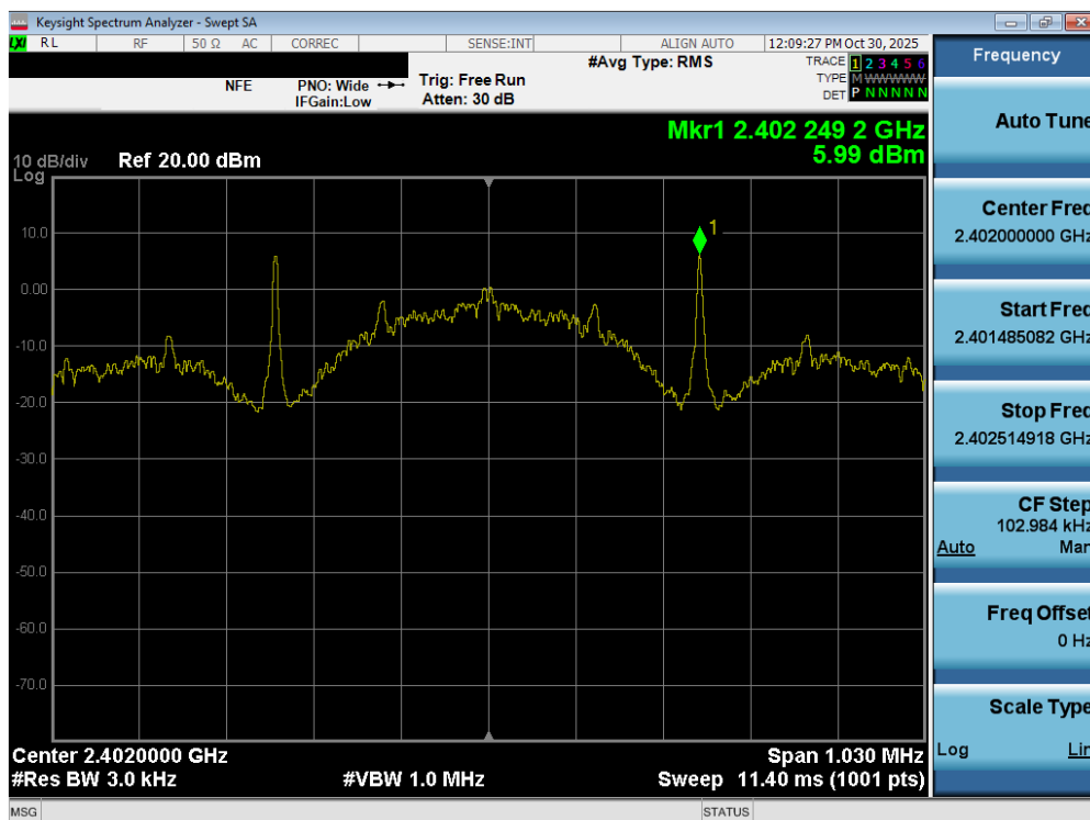
Plot 7-37. Power Spectral Density Plot (Bluetooth (LE), 125kbps – Ch. 37)
