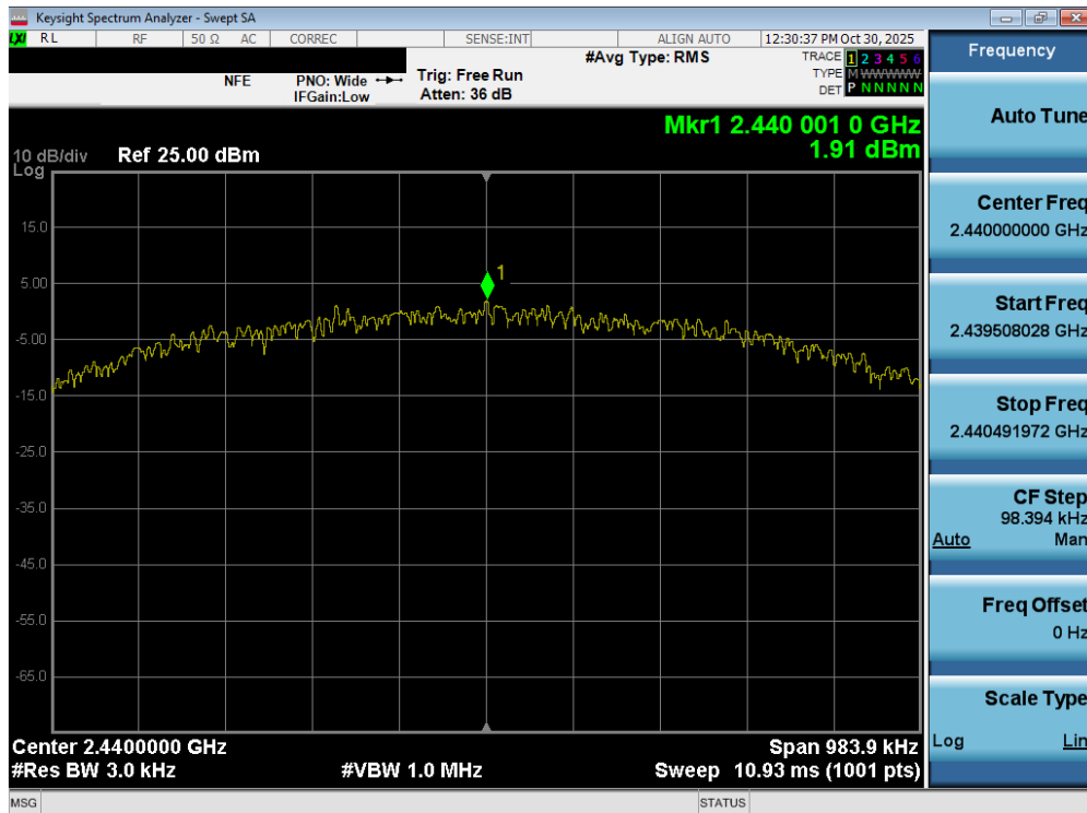
Plot 7-44. Power Spectral Density Plot (Bluetooth (LE), 1Mbps – Ch. 17)
