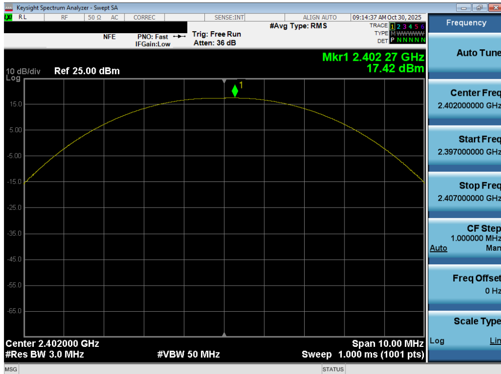
Plot 7-31. Peak Power Plot (Bluetooth (LE), 1Mbps – Ch. 37)
