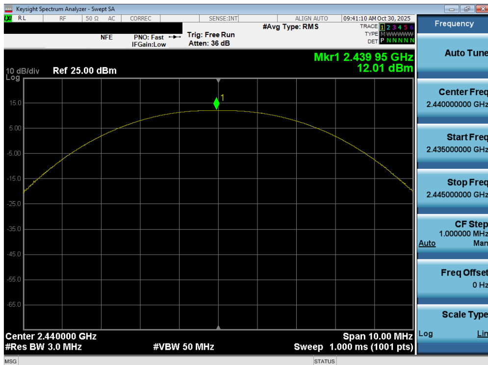
Plot 7-26. Peak Power Plot (Bluetooth (LE), 125kbps – Ch. 17)
