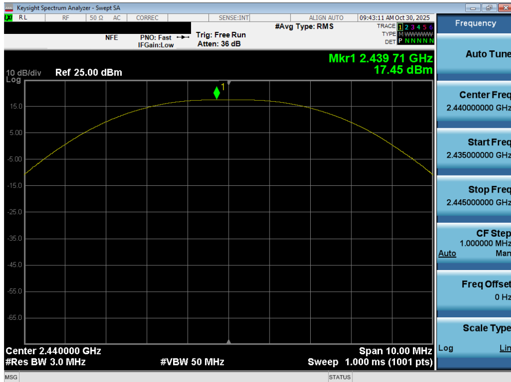
Plot 7-35. Peak Power Plot (Bluetooth (LE), 2Mbps – Ch. 17)
