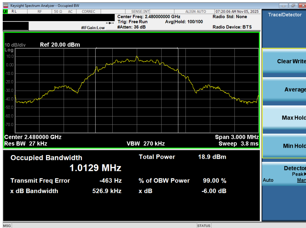
Plot 7-18. OBW Plot (Bluetooth (LE), 500kbps – Ch. 39)
