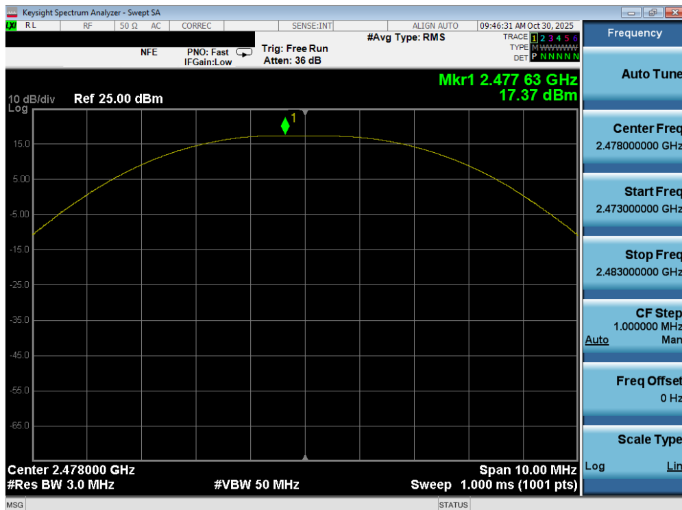
Plot 7-36. Peak Power Plot (Bluetooth (LE), 2Mbps – Ch. 36)
