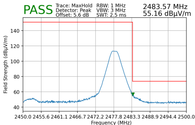
Plot 7-68. Radiated Restricted Upper Band Edge Measurement (Peak)
