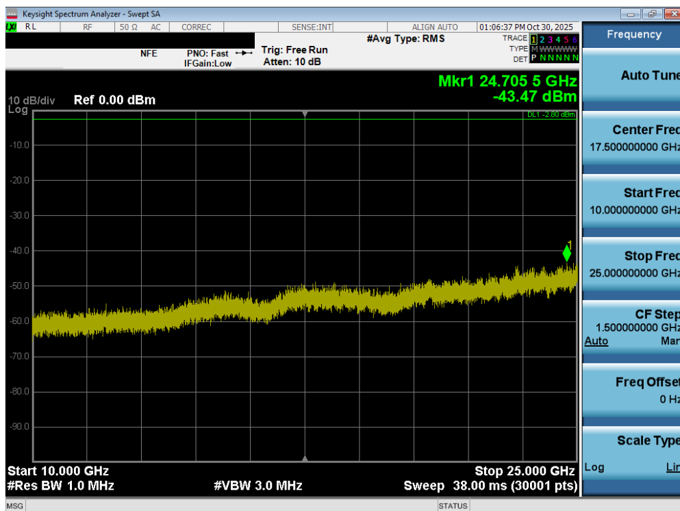
Plot 7-62. Conducted Spurious Plot (Bluetooth (LE), 1Mbps – Ch. 39)
