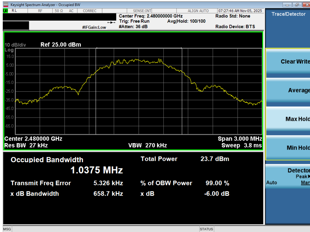
Plot 7-21. OBW Plot (Bluetooth (LE), 1Mbps – Ch. 39)
