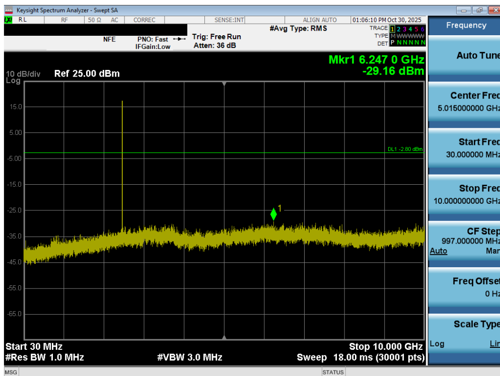
Plot 7-61. Conducted Spurious Plot (Bluetooth (LE), 1Mbps – Ch. 39)
