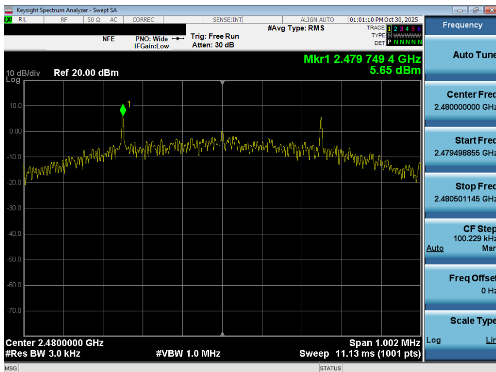
Plot 7-42. Power Spectral Density Plot (Bluetooth (LE), 500kbps – Ch. 39)
