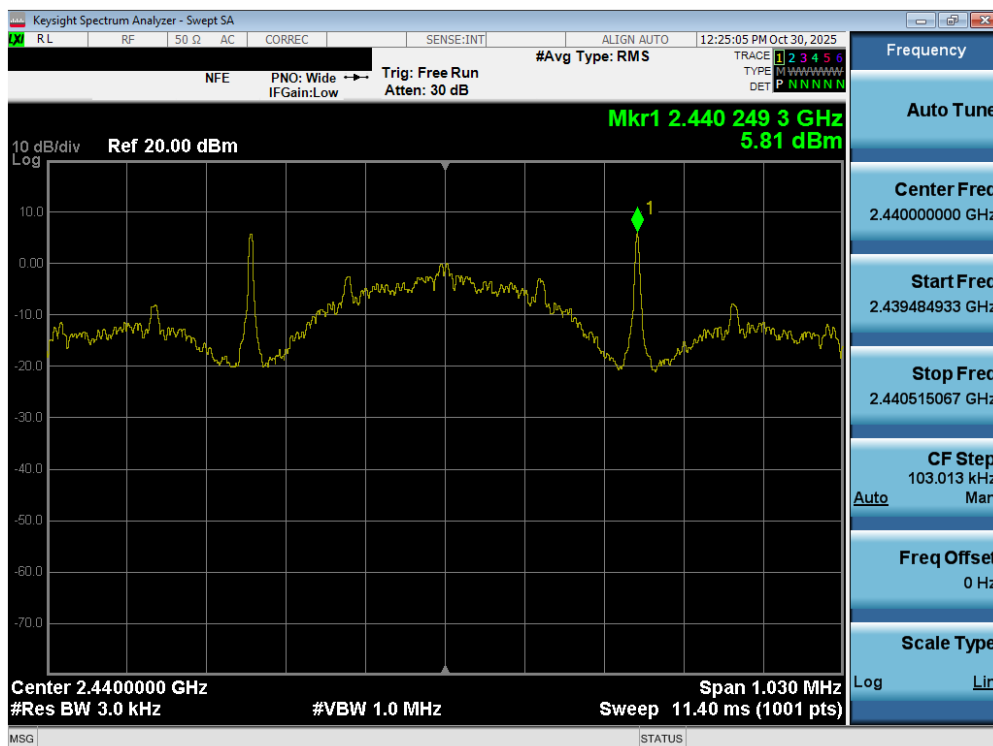
Plot 7-38. Power Spectral Density Plot (Bluetooth (LE), 125kbps – Ch. 17)
