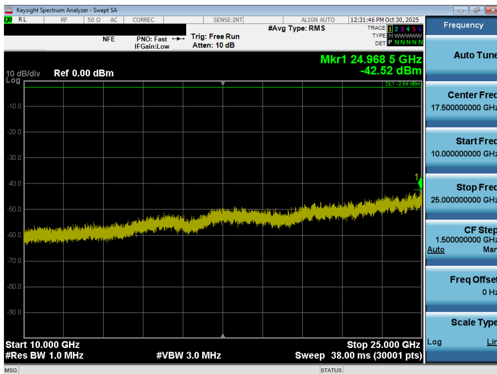
Plot 7-60. Conducted Spurious Plot (Bluetooth (LE), 1Mbps – Ch. 17)
