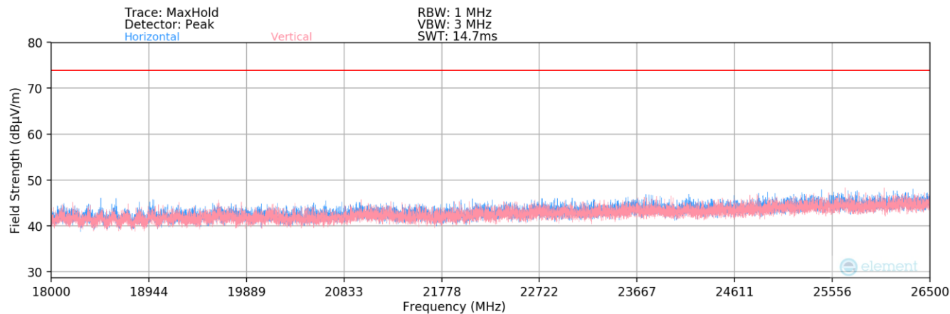
Plot 7-66. Radiated Spurious Plot above 18GHz (Bluetooth (LE) – Ch. 17)
