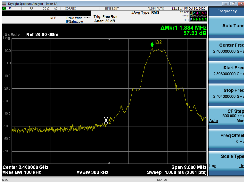
Plot 7-51. Band Edge Plot (Bluetooth (LE), 500kbps – Ch. 37)
