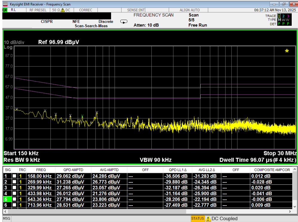
Plot 7-70. Line Conducted Plot with Bluetooth LE (L1)
