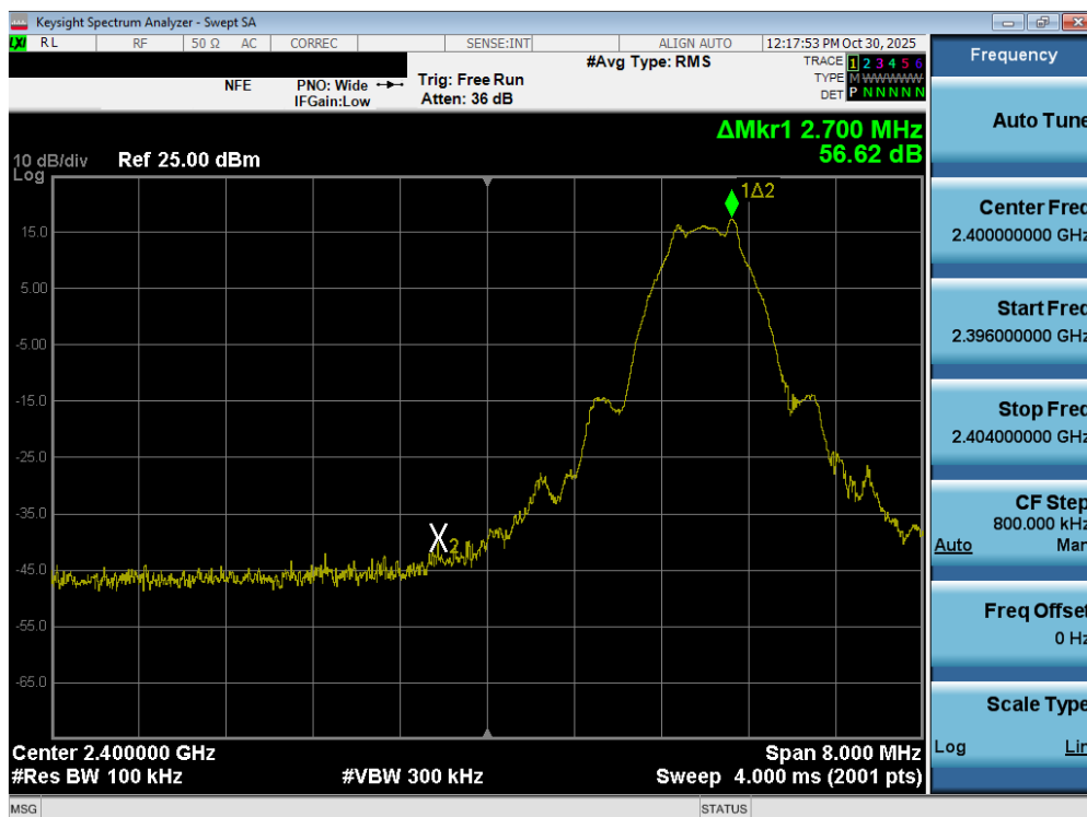
Plot 7-53. Band Edge Plot (Bluetooth (LE), 1Mbps – Ch. 37)
