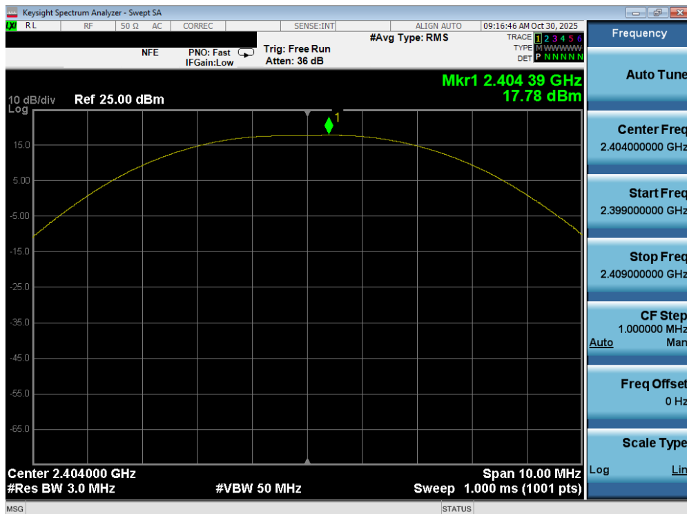
Plot 7-34. Peak Power Plot (Bluetooth (LE), 2Mbps – Ch. 0)
