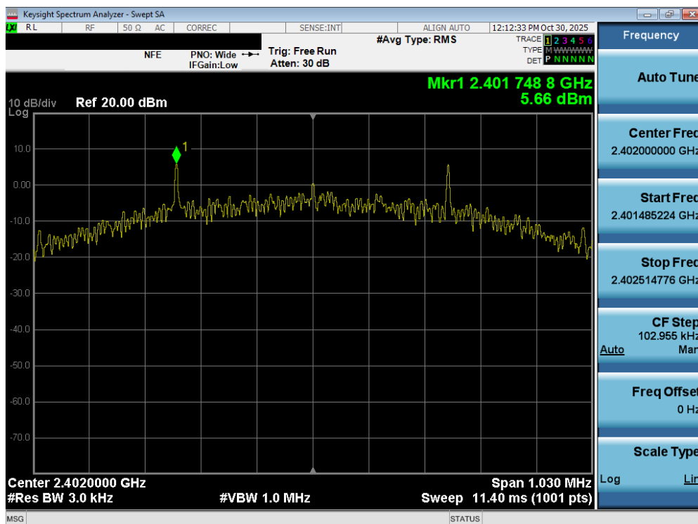
Plot 7-40. Power Spectral Density Plot (Bluetooth (LE), 500kbps – Ch. 37)
