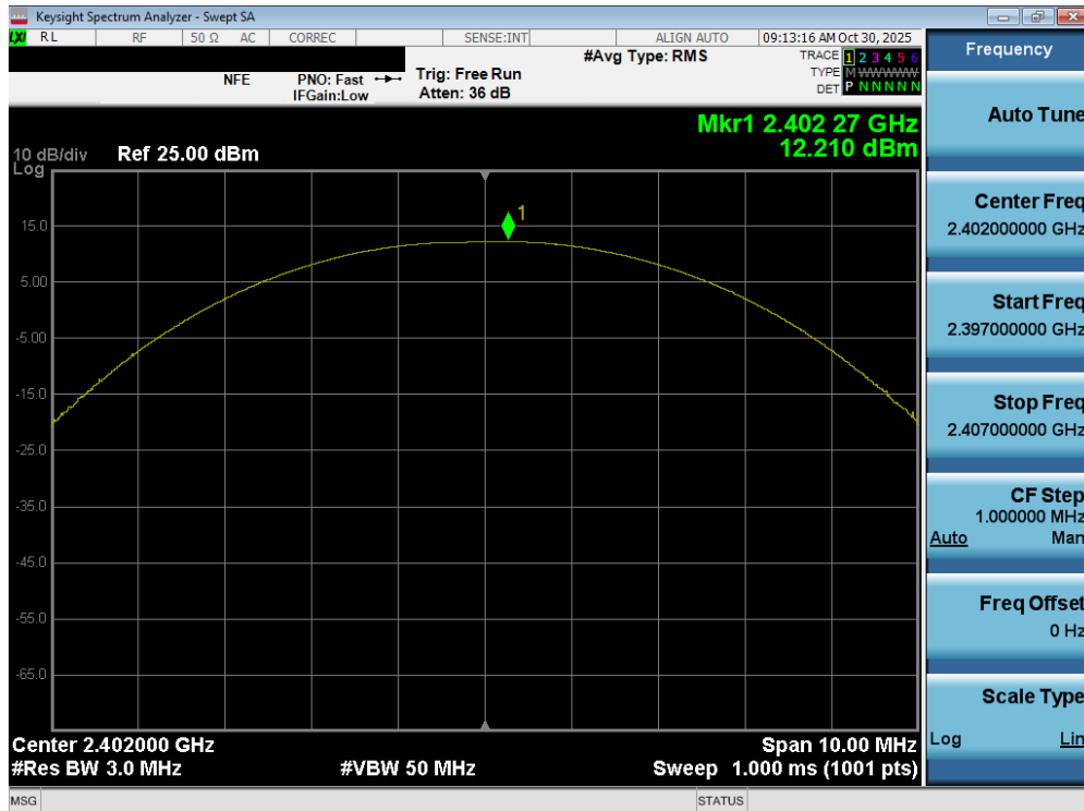
Plot 7-25. Peak Power Plot (Bluetooth (LE), 125kbps – Ch. 37)
