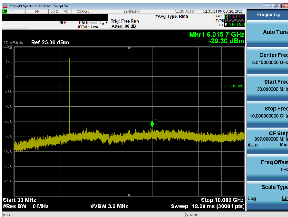
Plot 7-59. Conducted Spurious Plot (Bluetooth (LE), 1Mbps – Ch. 17)
