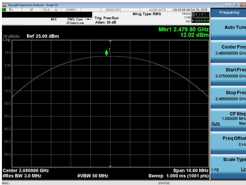
Plot 7-30. Peak Power Plot (Bluetooth (LE), 500kbps – Ch. 39)
