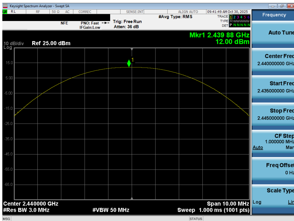
Plot 7-29. Peak Power Plot (Bluetooth (LE), 500kbps – Ch. 17)
