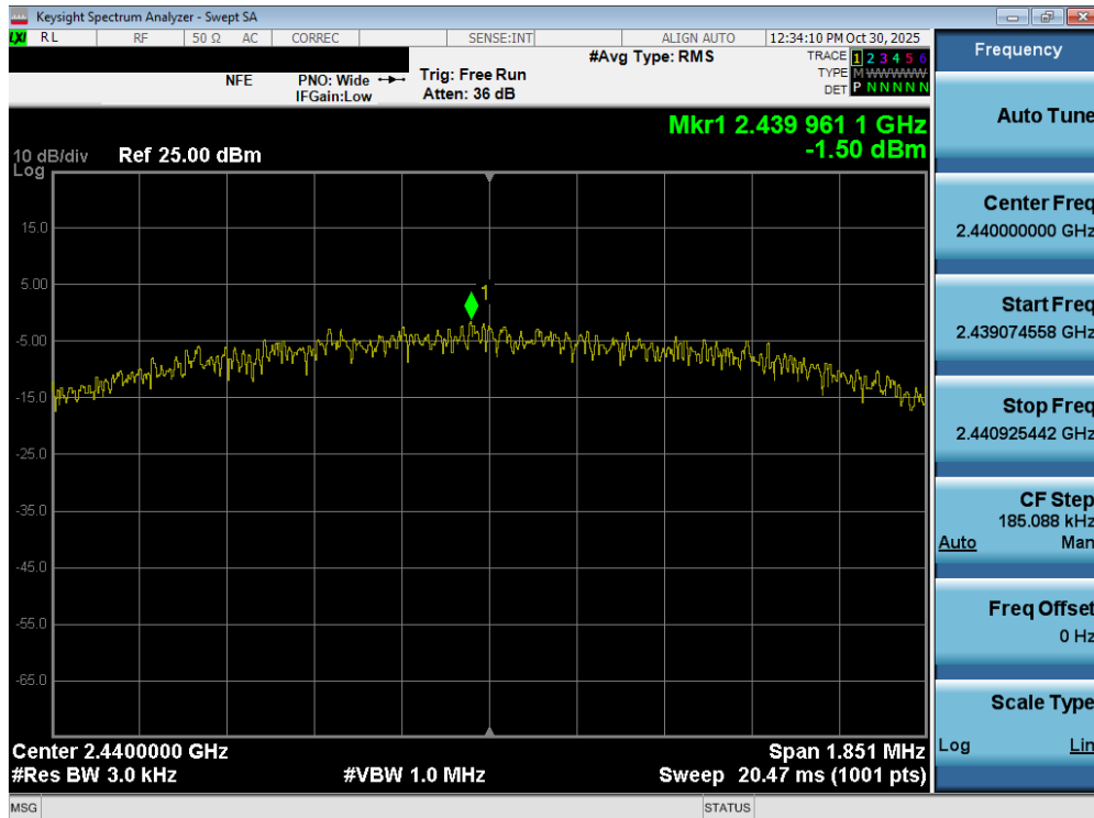
Plot 7-47. Power Spectral Density Plot (Bluetooth (LE), 2Mbps – Ch. 17)
