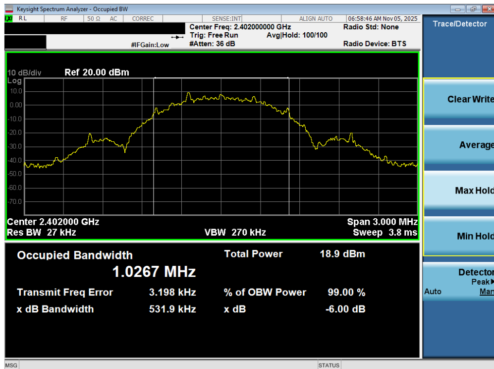
Plot 7-16. OBW Plot (Bluetooth (LE), 500kbps – Ch. 37)
