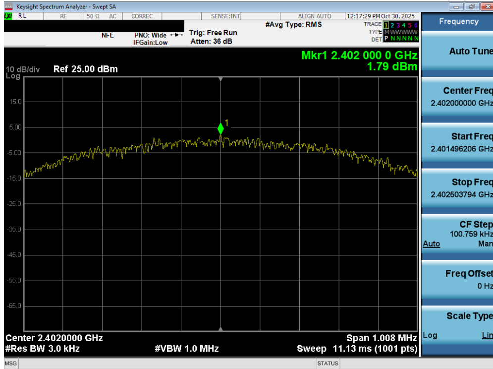
Plot 7-43. Power Spectral Density Plot (Bluetooth (LE), 1Mbps – Ch. 37)
