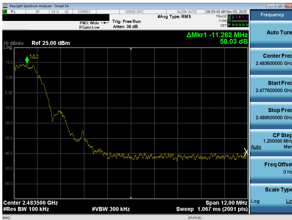
Plot 7-56. Band Edge Plot (Bluetooth (LE), 2Mbps – Ch. 36)
