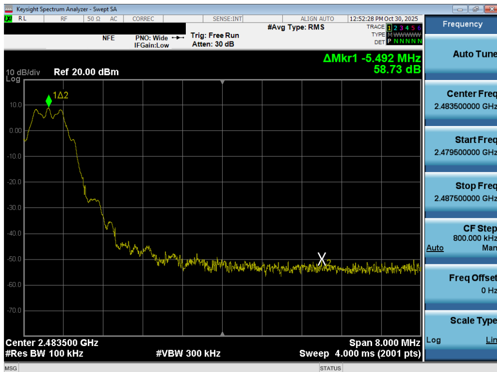
Plot 7-50. Band Edge Plot (Bluetooth (LE), 125kbps – Ch. 39)
