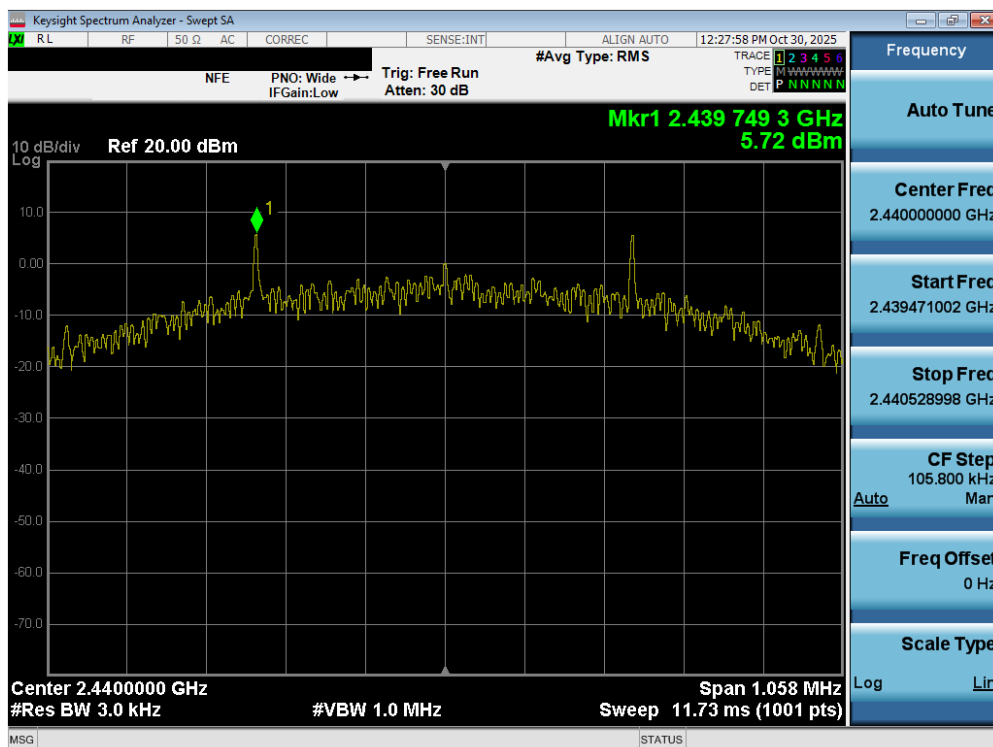
Plot 7-41. Power Spectral Density Plot (Bluetooth (LE), 500kbps – Ch. 17)
