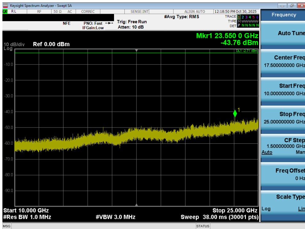
Plot 7-58. Conducted Spurious Plot (Bluetooth (LE), 1Mbps – Ch. 37)
