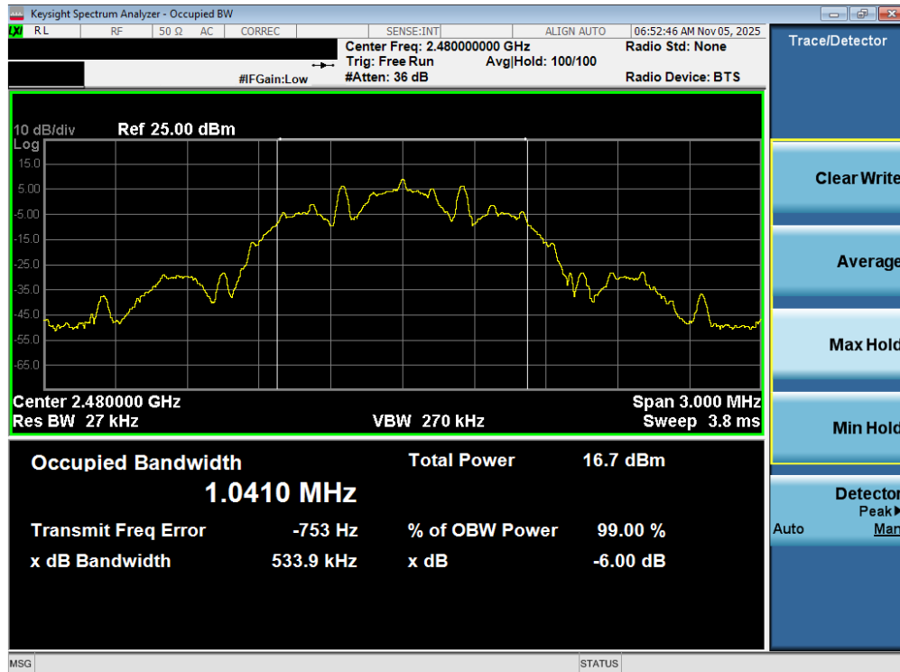
Plot 7-15. OBW Plot (Bluetooth (LE), 125kbps – Ch. 39)
