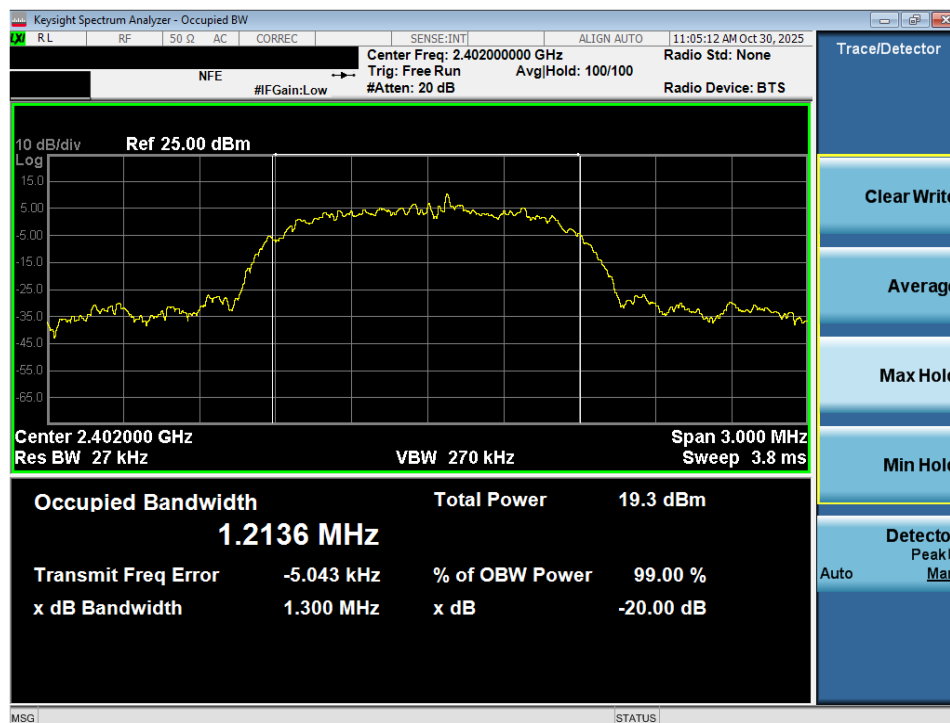
Plot 7-7. 20dB Bandwidth Plot (Bluetooth, 3Mbps – Ch. 0) – Ant 1
