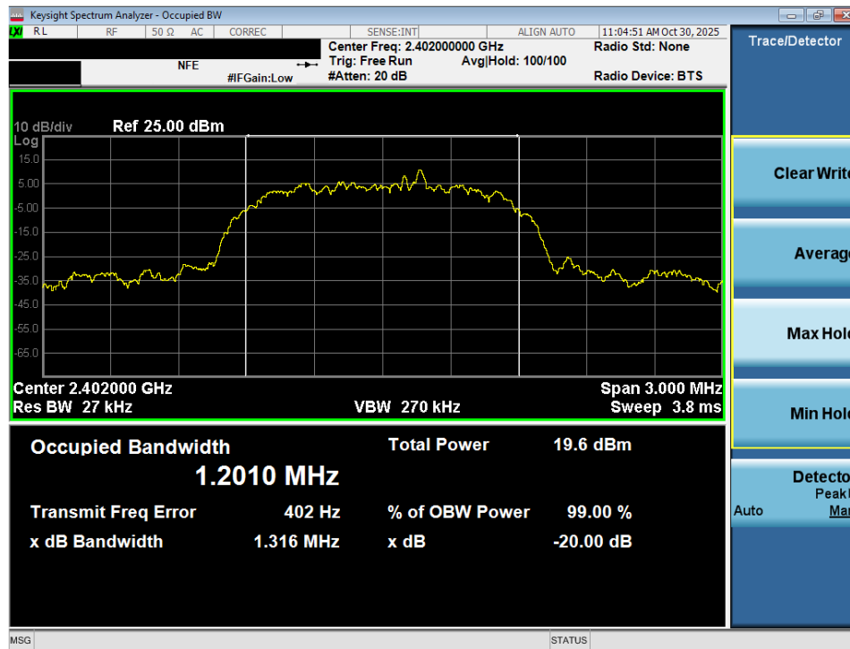
Plot 7-4. 20dB Bandwidth Plot (Bluetooth, 2Mbps – Ch. 0) – Ant 1
