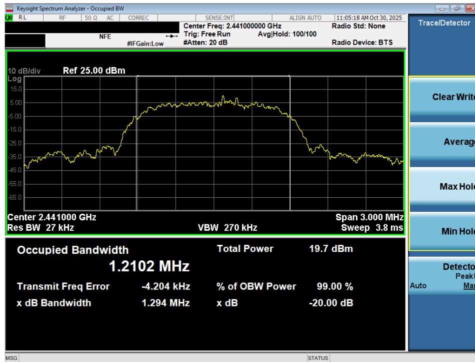
Plot 7-8. 20dB Bandwidth Plot (Bluetooth, 3Mbps – Ch. 39) – Ant 1
