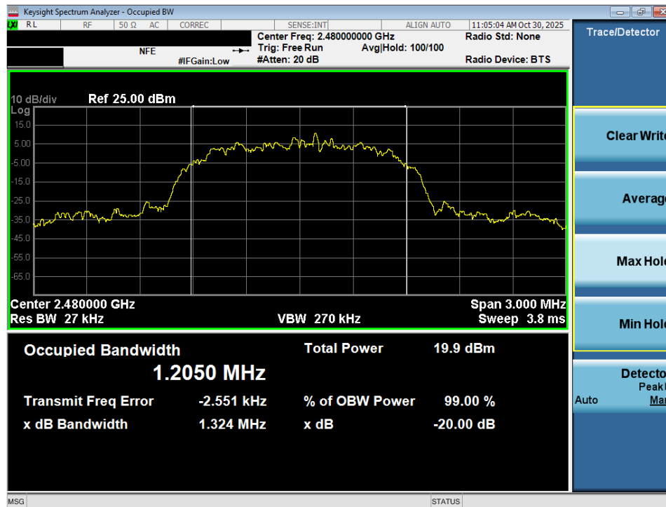
Plot 7-6. 20dB Bandwidth Plot (Bluetooth, 2Mbps – Ch. 78) – Ant 1
