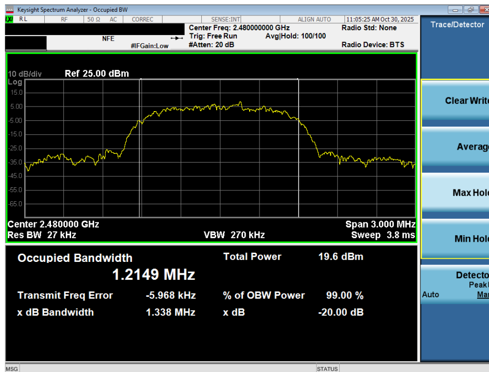
Plot 7-9. 20dB Bandwidth Plot (Bluetooth, 3Mbps – Ch. 78) – Ant 1
