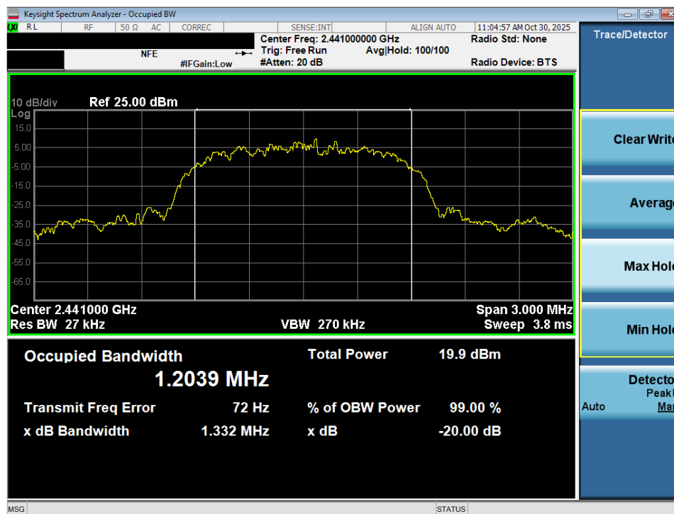
Plot 7-5. 20dB Bandwidth Plot (Bluetooth, 2Mbps – Ch. 39) – Ant 1
