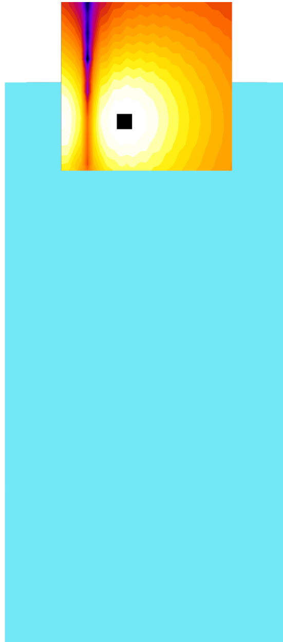
Figure 7-1 T-Coil Scan Overlay Magnetic Field Distributions
