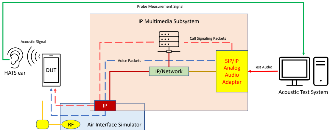
Figure 7-1 Test Setup for VoNR over IMS Volume Control Measurements
