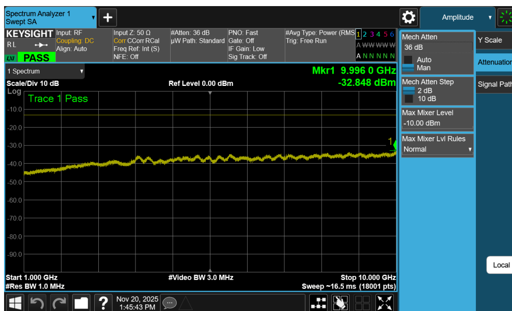
Plot 7-83. Conducted Spurious Plot (WCDMA Ch. 4183 – Ant1)
