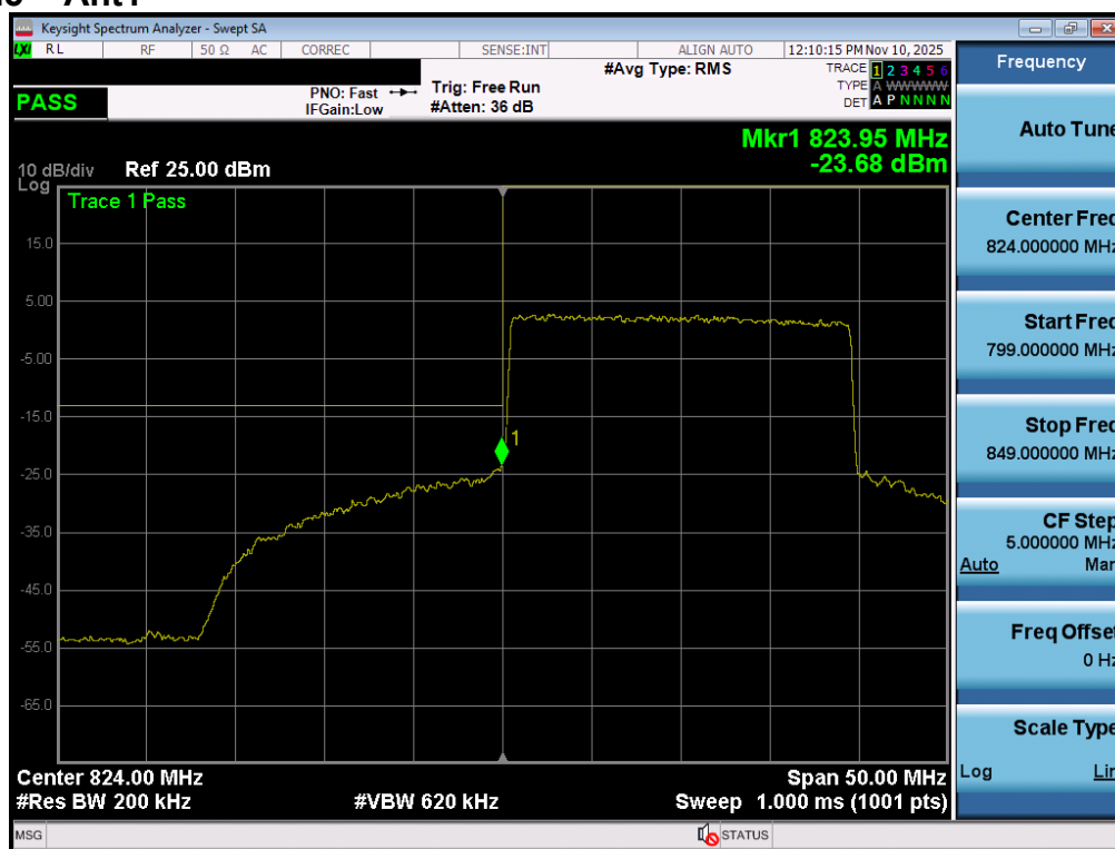
Plot 7-133. Lower Band Edge Plot (NR Band n5 – 20.0MHz - Full RB - Ant1)
