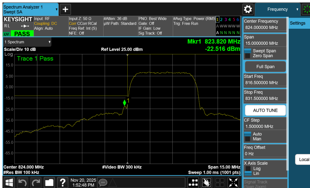
Plot 7-143. Lower Band Edge Plot (WCDMA Cell – Ch. 4132 – Ant1)
