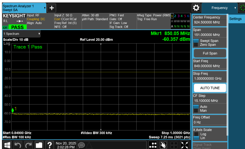
Plot 7-115. Conducted Spurious Plot (WCDMA Ch. 4132 – Ant2)
