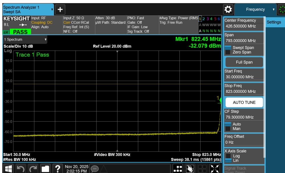
Plot 7-114. Conducted Spurious Plot (WCDMA Ch. 4132 – Ant2)
