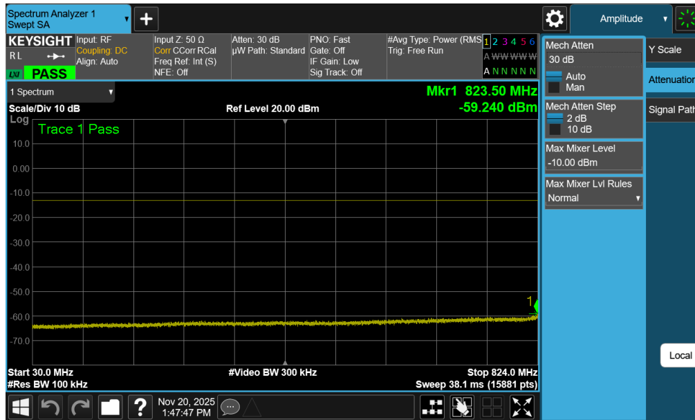
Plot 7-84. Conducted Spurious Plot (WCDMA Ch. 4233 – Ant1)
