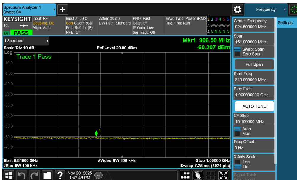
Plot 7-79. Conducted Spurious Plot (WCDMA Ch. 4132 – Ant1)
