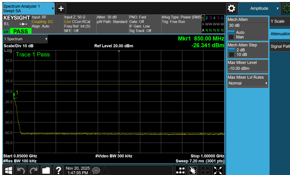
Plot 7-85. Conducted Spurious Plot (WCDMA Ch. 4233 – Ant1)
