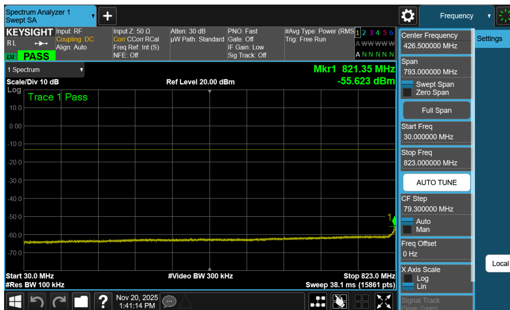
Plot 7-78. Conducted Spurious Plot (WCDMA Ch. 4132 – Ant1)
