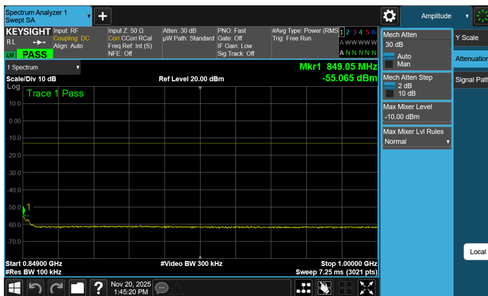
Plot 7-82. Conducted Spurious Plot (WCDMA Ch. 4183 – Ant1)
