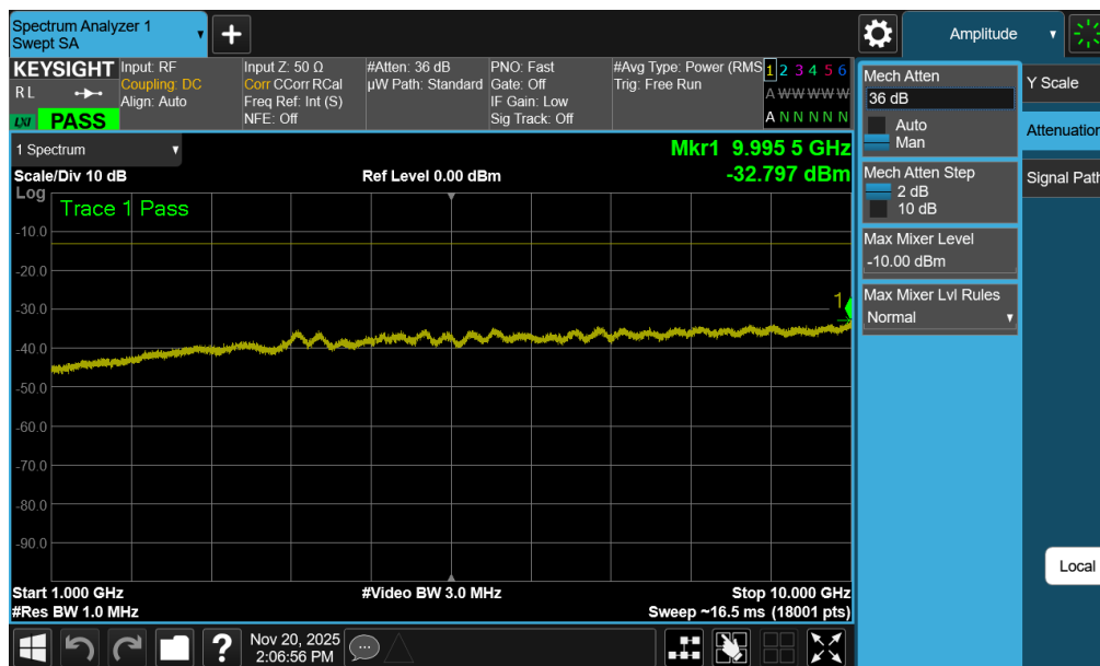
Plot 7-122. Conducted Spurious Plot (WCDMA Ch. 4233 – Ant2)
