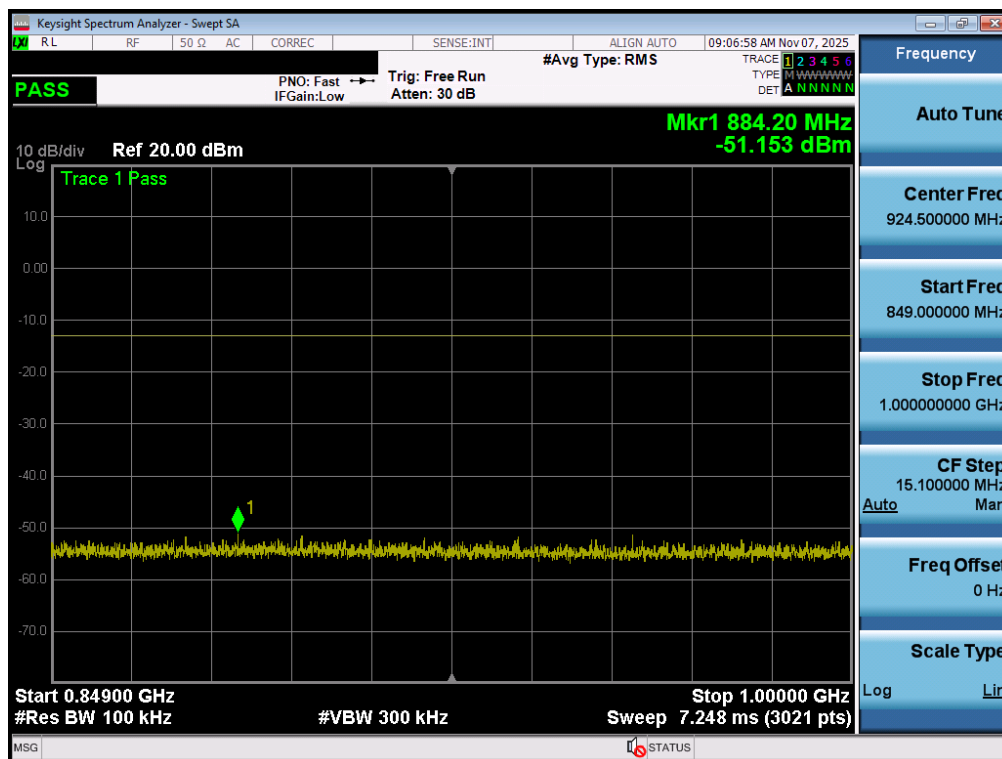
Plot 7-73. Conducted Spurious Plot (GPRS Ch. 190 – Ant1)
