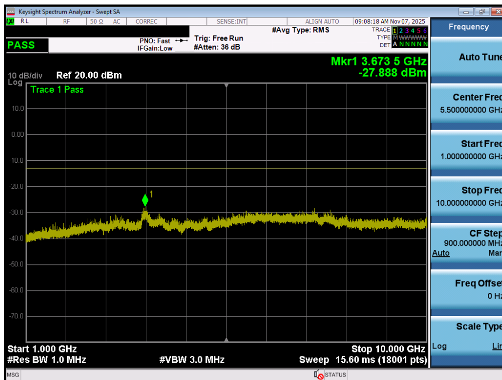
Plot 7-74. Conducted Spurious Plot (GPRS Ch. 190 – Ant1)
