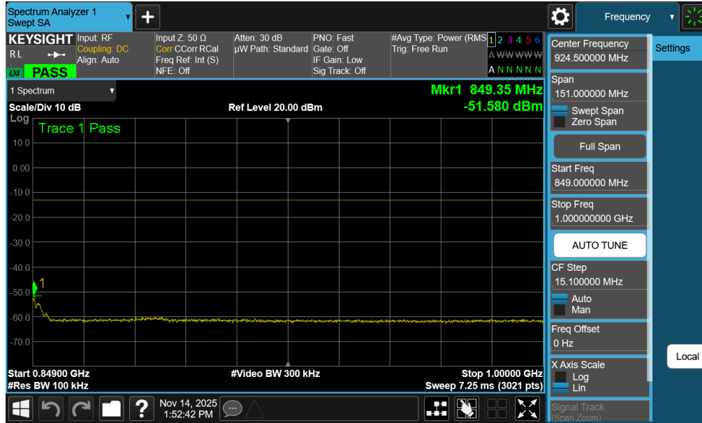
Plot 7-91. Conducted Spurious Plot (LTE Band 26 - 15MHz QPSK - 1 RB - Mid Channel – Ant2)
