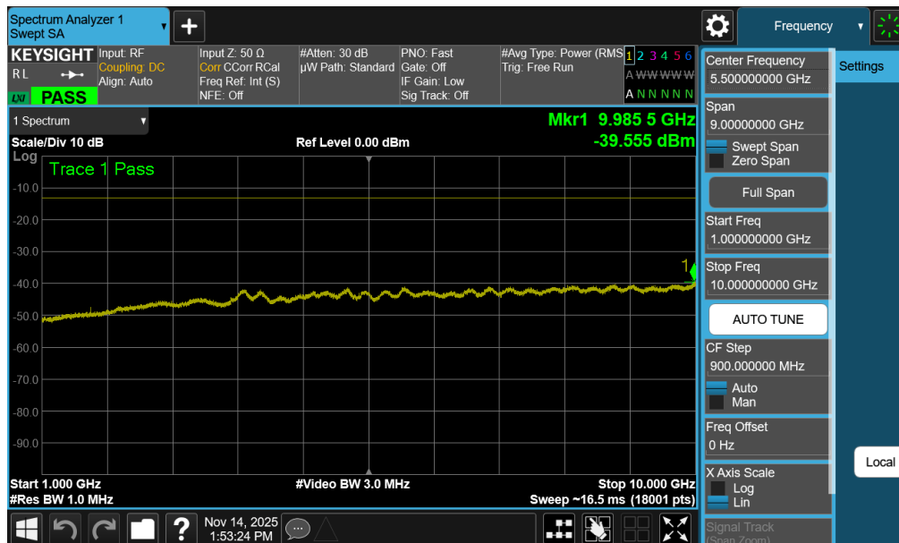
Plot 7-92. Conducted Spurious Plot (LTE Band 26 - 15MHz QPSK - 1 RB - Mid Channel – Ant2)
