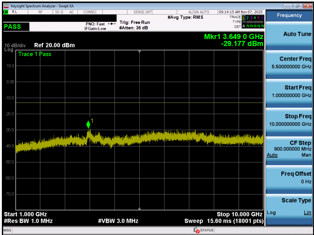
Plot 7-77. Conducted Spurious Plot (GPRS Ch. 251 – Ant1)
