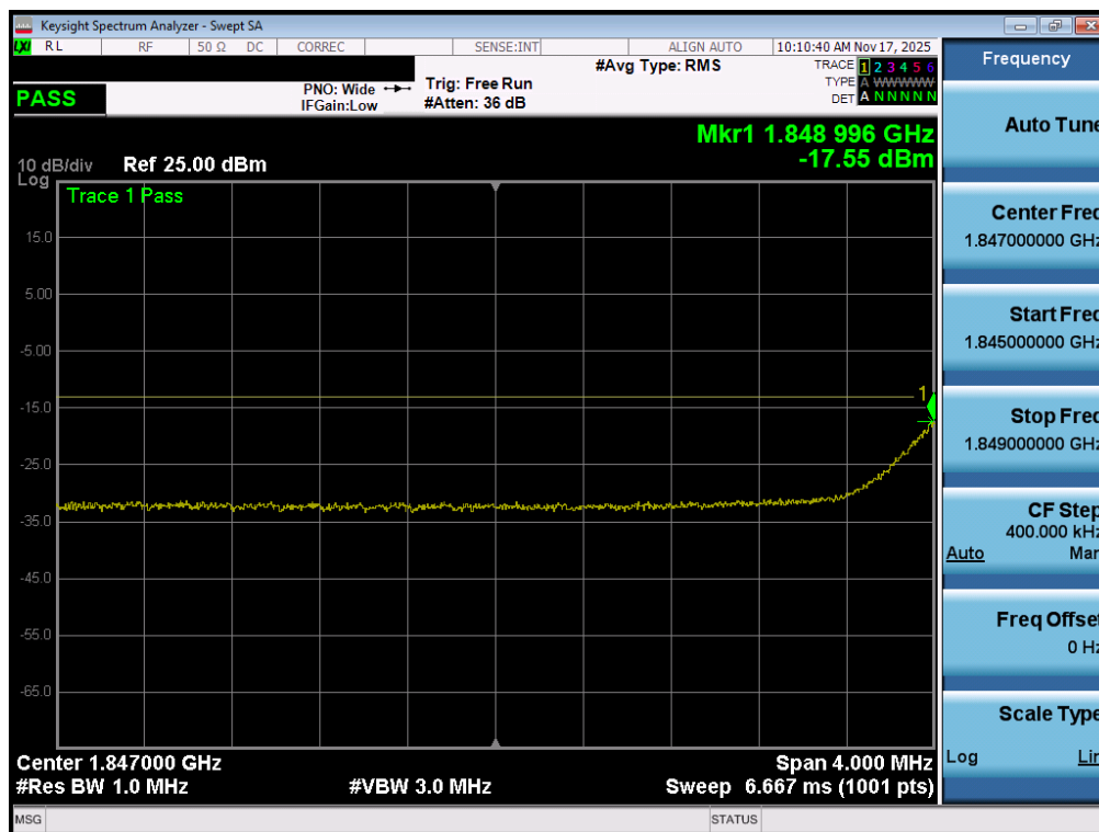
Plot 7-103. Extended Lower Band Edge Plot (NR Band n25/2 - 10MHz QPSK – Full RB - Ant1)
