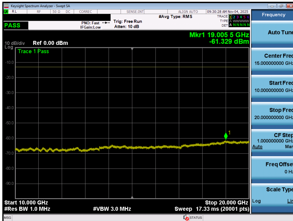
Plot 7-81. Conducted Spurious Plot (NR Band n25/2 - 40.0MHz - 1RB - Low Channel - Ant1)
