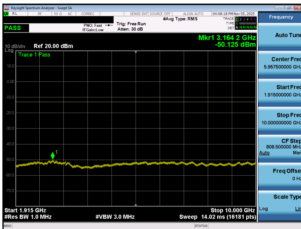
Plot 7-83. Conducted Spurious Plot (LTE Band 25/2 - 20MHz QPSK - 1RB - Low Channel - Ant2)
