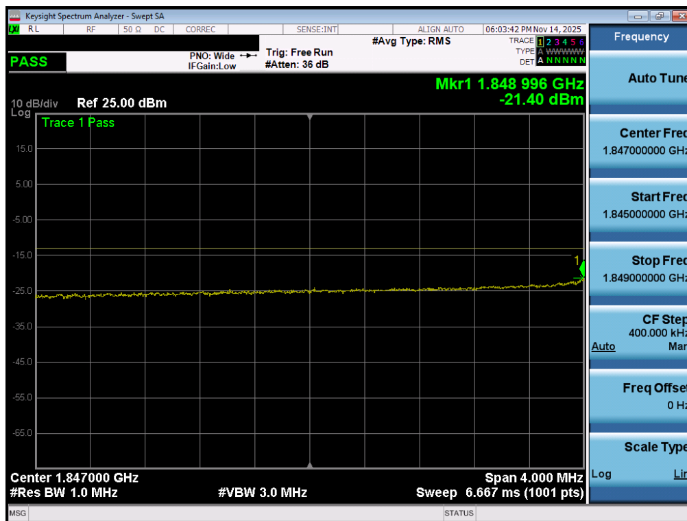
Plot 7-97. Extended Lower Band Edge Plot (LTE Band 25/2 - 10MHz QPSK – Full RB - Ant1)
