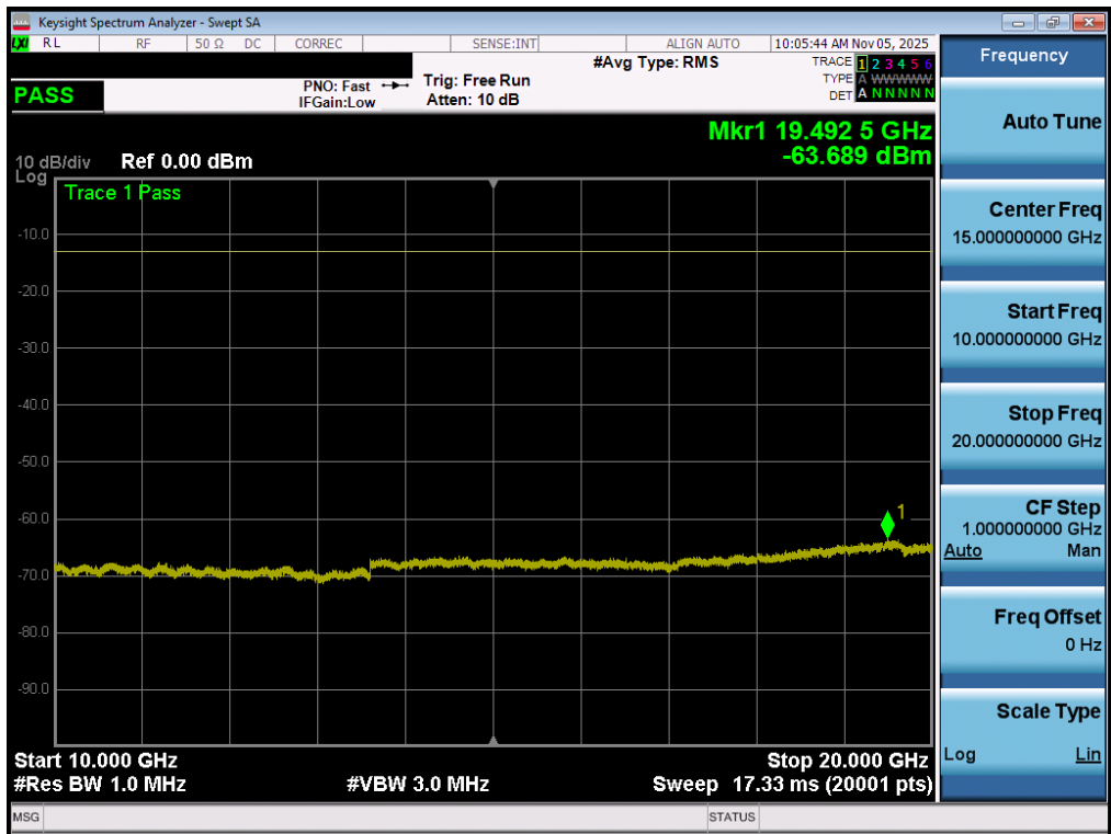
Plot 7-75. Conducted Spurious Plot (WCDMA Ch. 9538 - Ant1)
