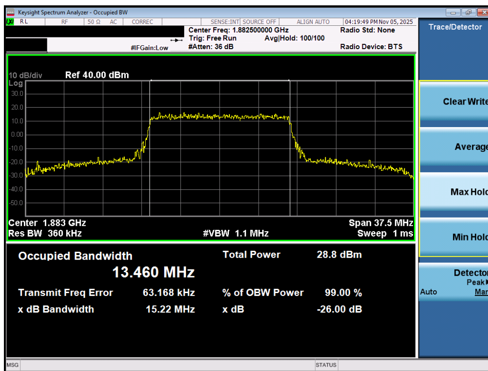
Plot 7-40. Occupied Bandwidth Plot (LTE Band 25/2 - 15MHz 16-QAM - Full RB - Ant2)
