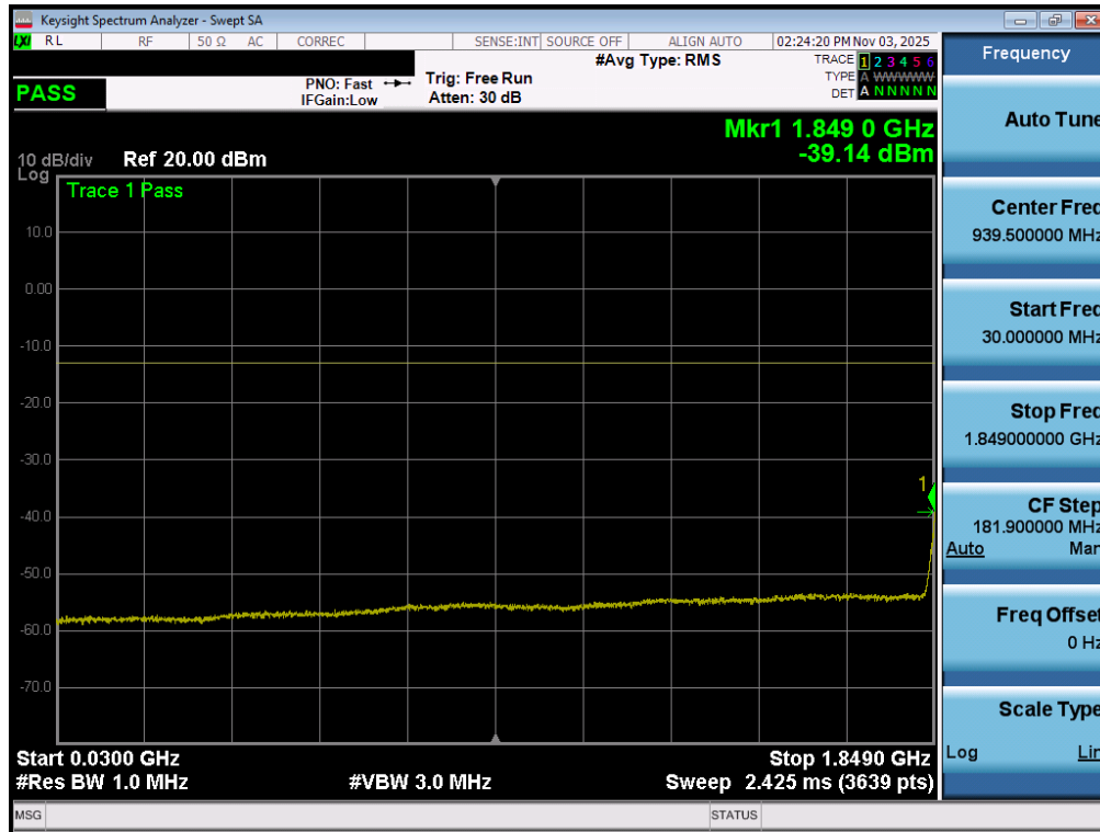
Plot 7-76. Conducted Spurious Plot (LTE Band 25/2 - 20MHz QPSK - 1RB - Low Channel - Ant1)
