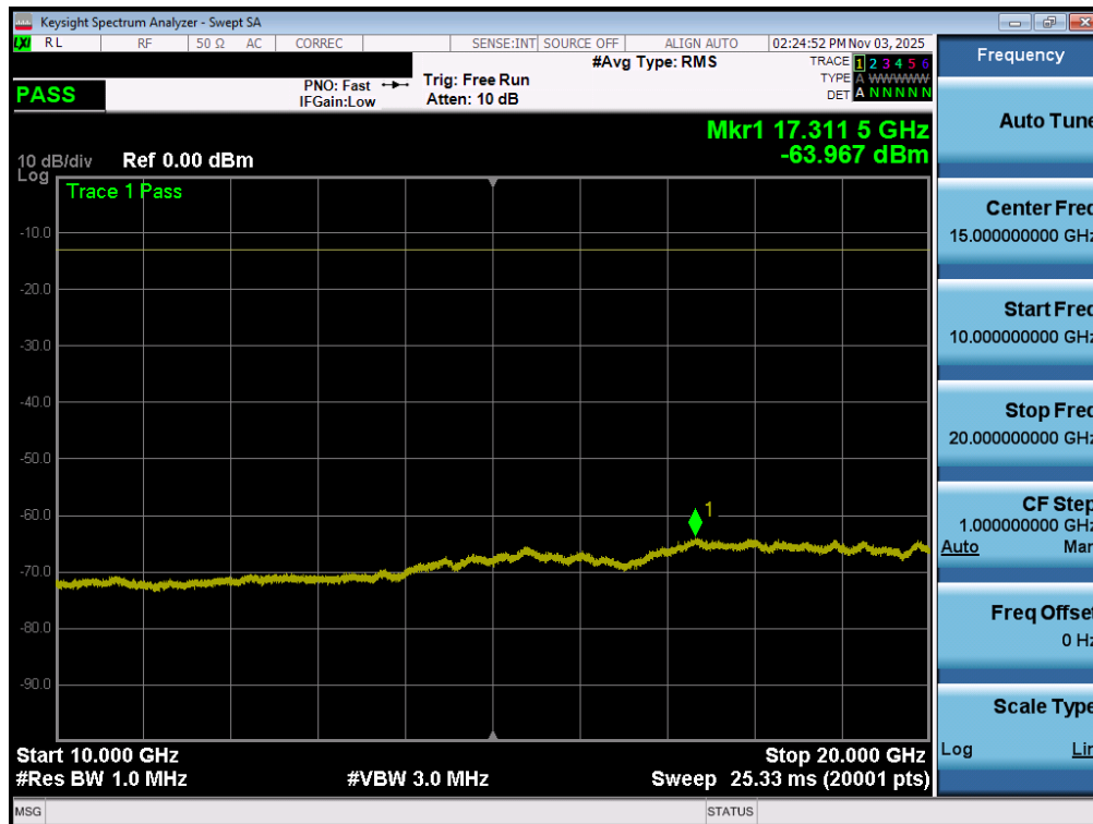
Plot 7-78. Conducted Spurious Plot (LTE Band 25/2 - 20MHz QPSK - 1RB - Low Channel - Ant1)
