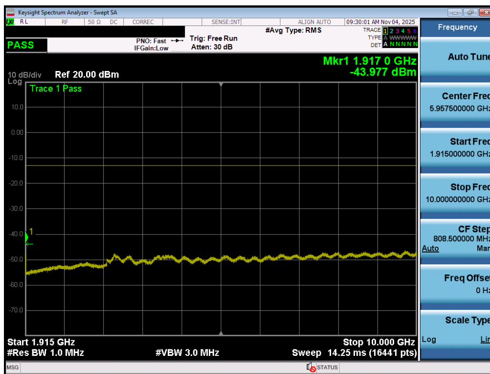
Plot 7-80. Conducted Spurious Plot (NR Band n25/2 - 40.0MHz - 1RB - Low Channel - Ant1)
