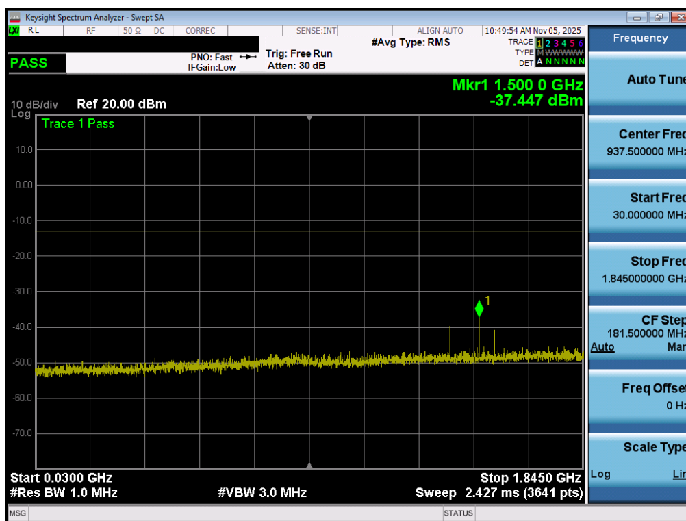
Plot 7-70. Conducted Spurious Plot (GPRS Ch. 512 - Ant1)
