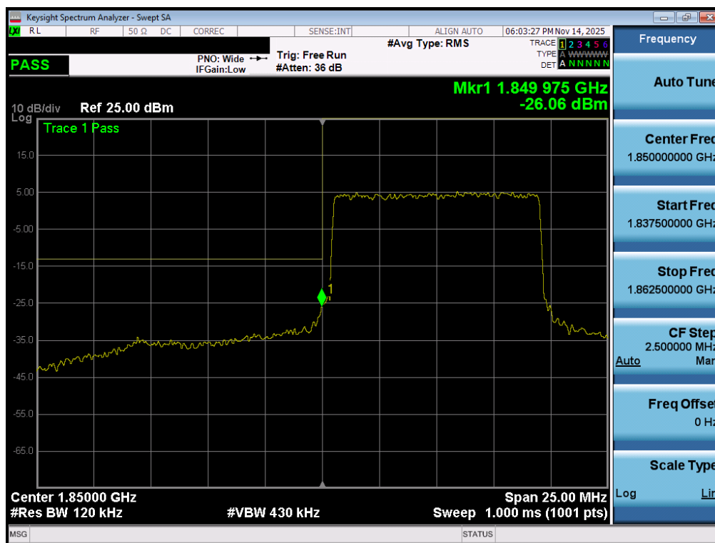
Plot 7-96. Lower Band Edge Plot (LTE Band 25/2 - 10MHz QPSK – Full RB - Ant1)
