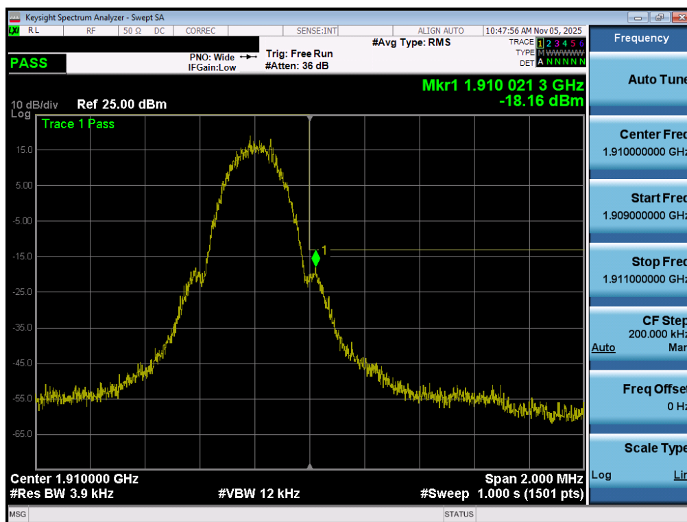
Plot 7-90. Upper Band Edge Plot (GPRS PCS – Ch. 810 - Ant1)
