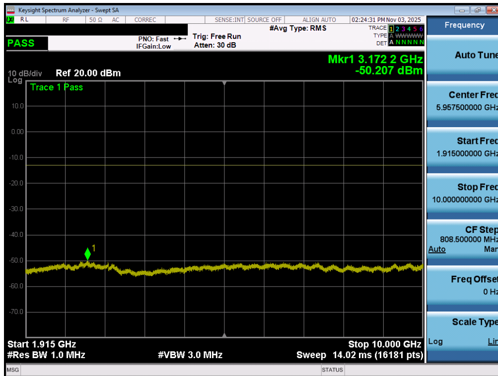
Plot 7-77. Conducted Spurious Plot (LTE Band 25/2 - 20MHz QPSK - 1RB - Low Channel - Ant1)
