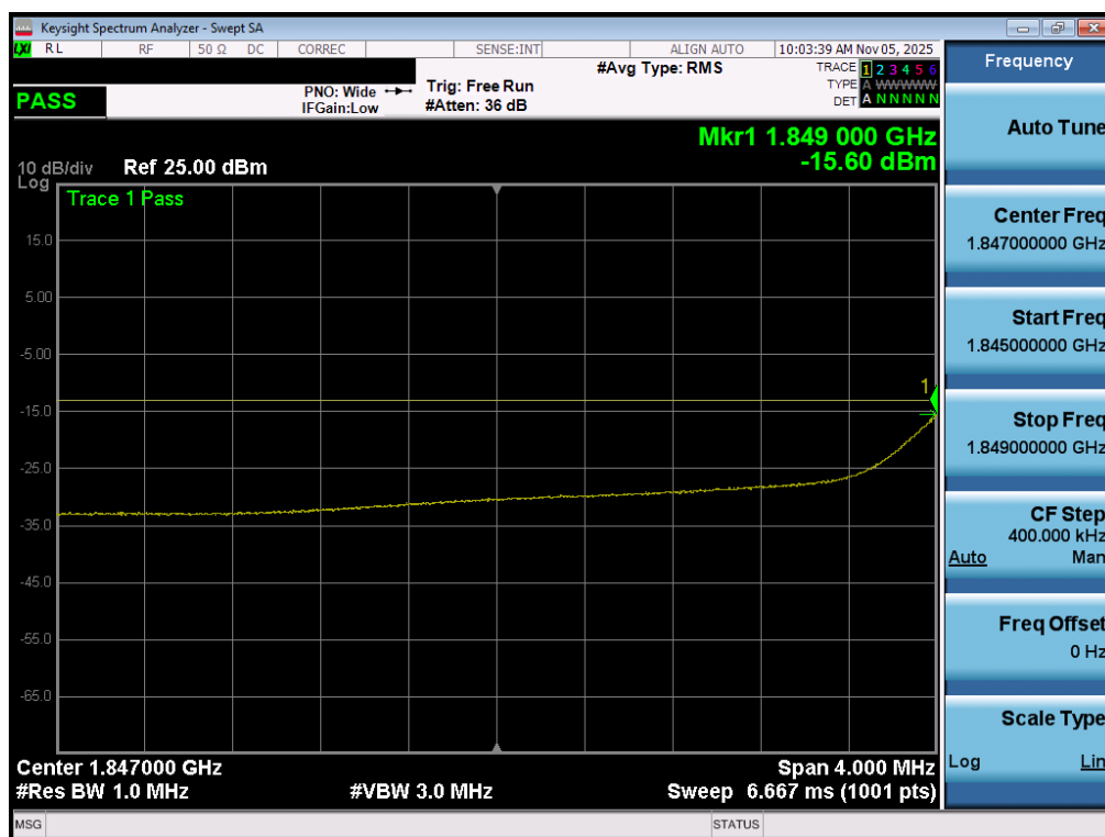
Plot 7-93. Extended Lower Band Edge Plot (WCDMA PCS – Ch. 9262 - Ant1)
