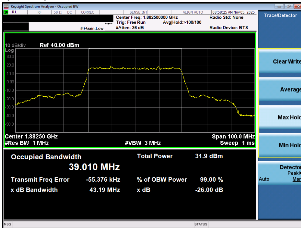
Plot 7-49. Occupied Bandwidth Plot (NR Band n25/2 - 40.0MHz DFT-s-OFDM BPSK - Full RB - ANT2)
