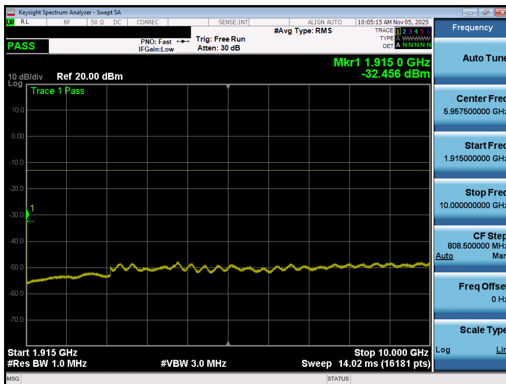
Plot 7-74. Conducted Spurious Plot (WCDMA Ch. 9538 - Ant1)
