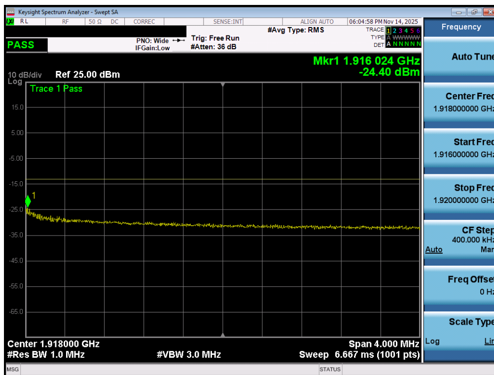
Plot 7-101. Extended Upper Band Edge Plot (LTE Band 25 - 10MHz QPSK – Full RB - Ant1)
