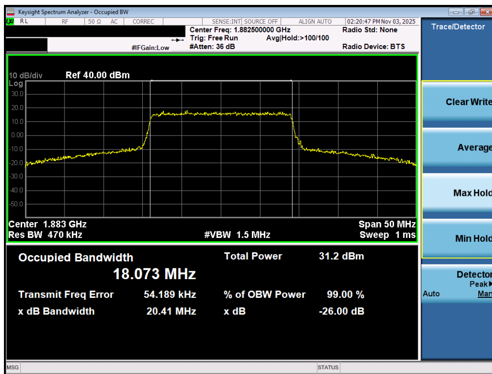
Plot 7-4. Occupied Bandwidth Plot (LTE Band 25/2 - 20MHz QPSK - Full RB - Ant1)
