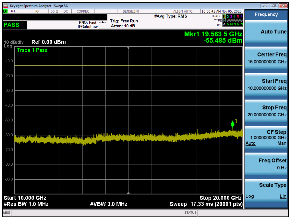
Plot 7-72. Conducted Spurious Plot (GPRS Ch. 512 - Ant1)
