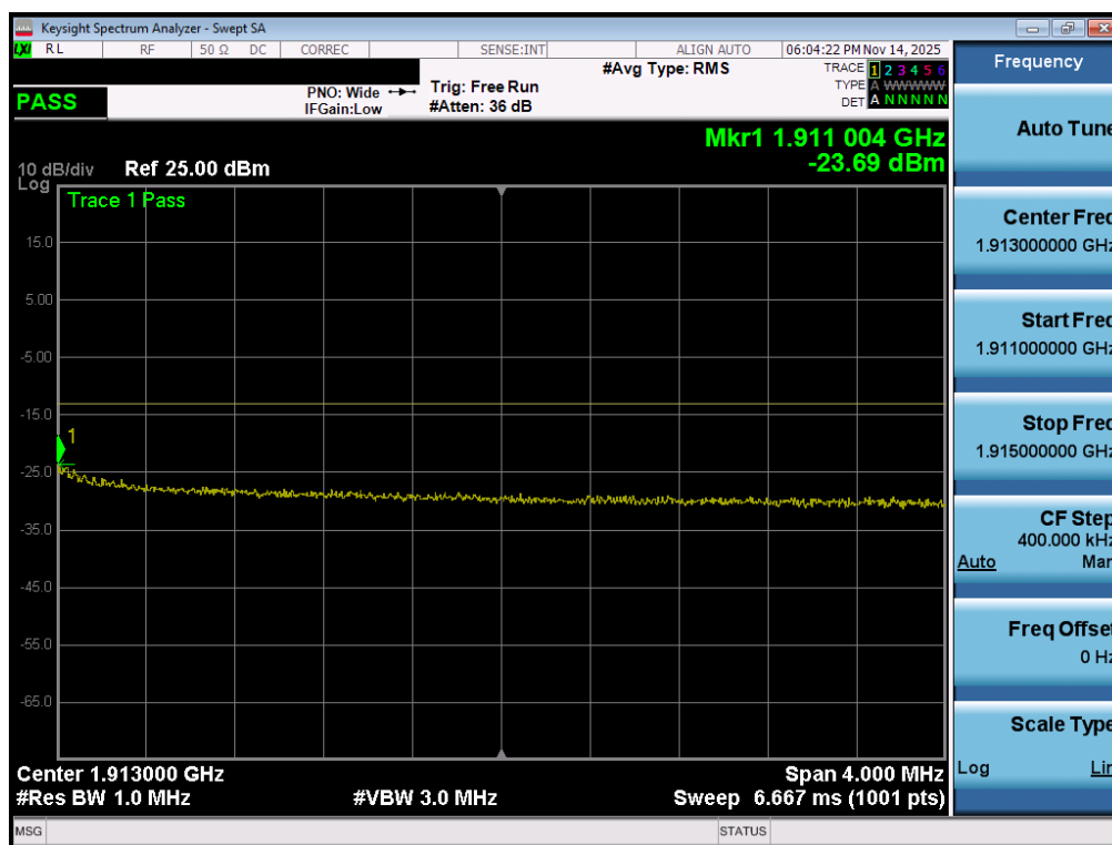
Plot 7-99. Extended Upper Band Edge Plot (LTE Band 2 - 10MHz QPSK – Full RB - Ant1)
