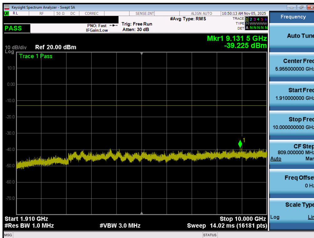
Plot 7-71. Conducted Spurious Plot (GPRS Ch. 512 - Ant1)
