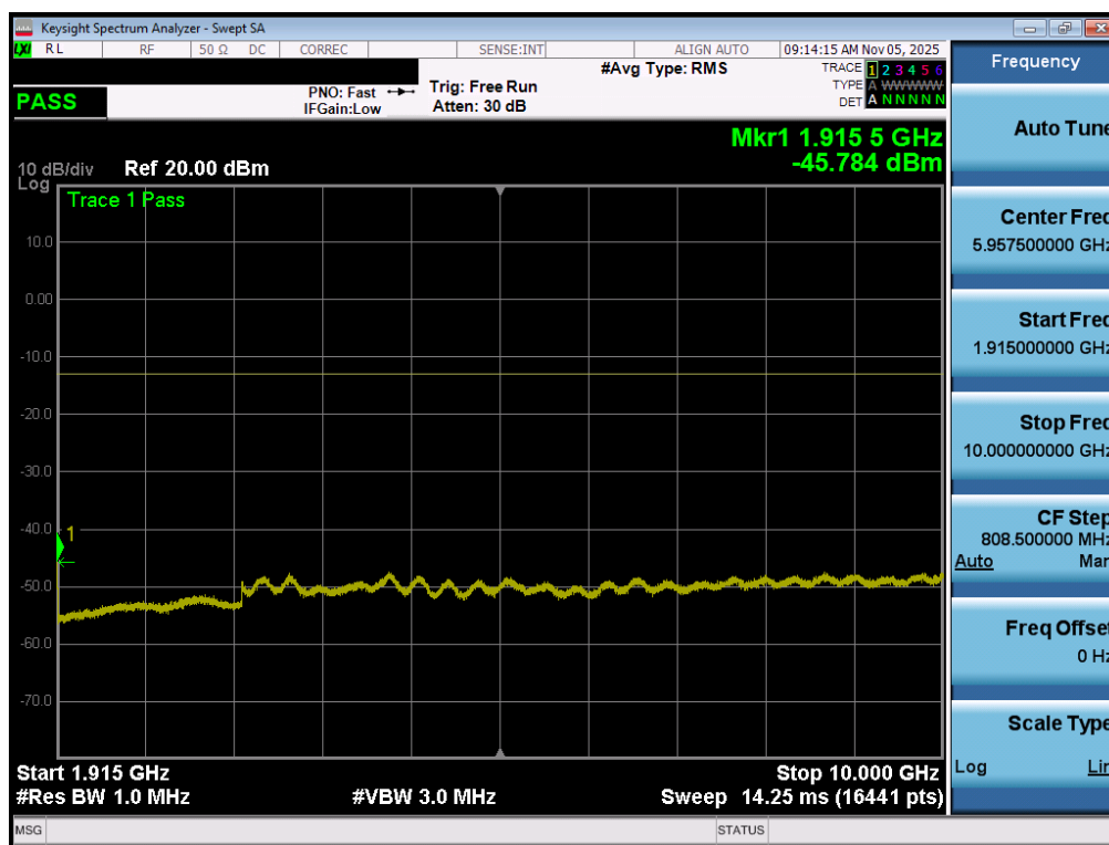
Plot 7-86. Conducted Spurious Plot (NR Band n25/2 - 40.0MHz - 1RB - Low Channel - Ant2)
