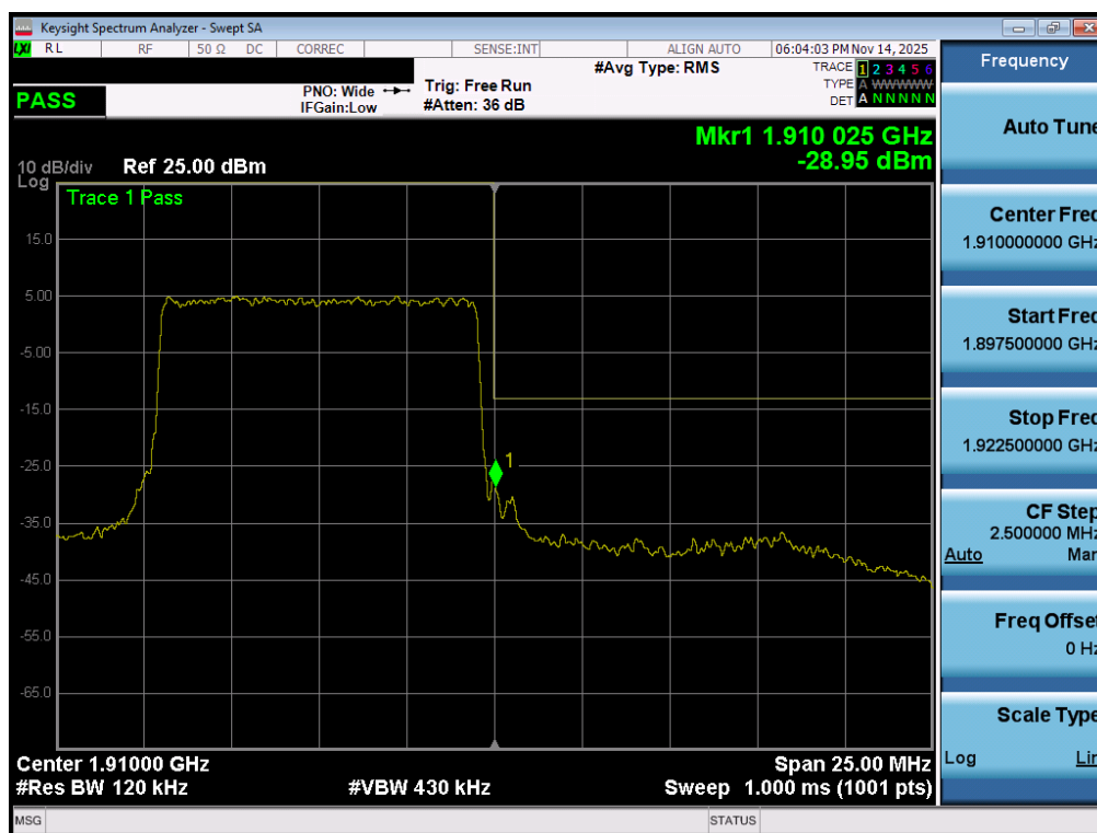
Plot 7-98. Upper Band Edge Plot (LTE Band 2 - 10MHz QPSK – Full RB - Ant1)
