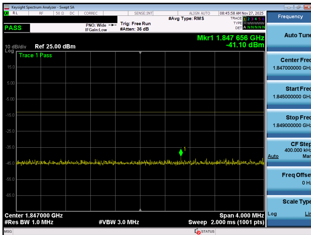
Plot 7-89. Extended Lower Band Edge Plot (GPRS PCS – Ch. 512 - Ant1)
