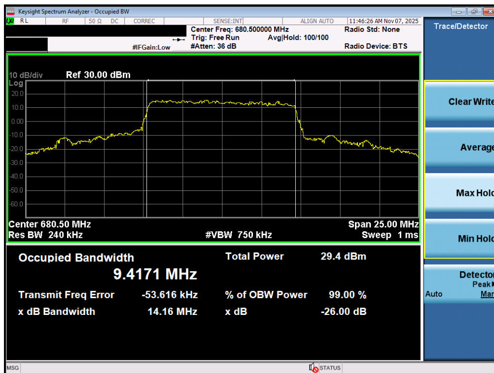
Plot 7-41. Occupied Bandwidth Plot (NR Band n71 - 10MHz CP-OFDM QPSK - Full RB – ANT1)
