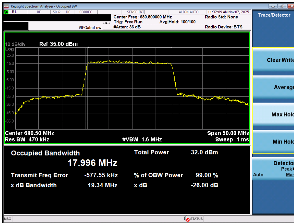
Plot 7-34. Occupied Bandwidth Plot (NR Band n71 - 20MHz DFT-s-OFDM BPSK - Full RB – ANT1)
