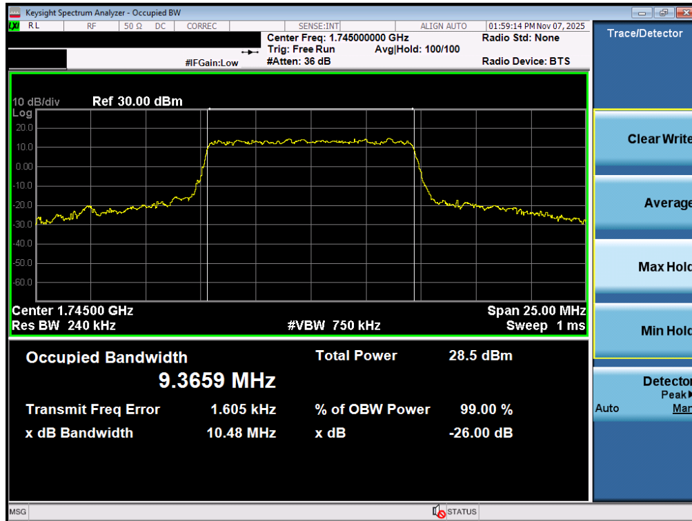
Plot 7-71. Occupied Bandwidth Plot (NR Band n66 - 10.0MHz CP-OFDM QPSK - Full RB – ANT1)
