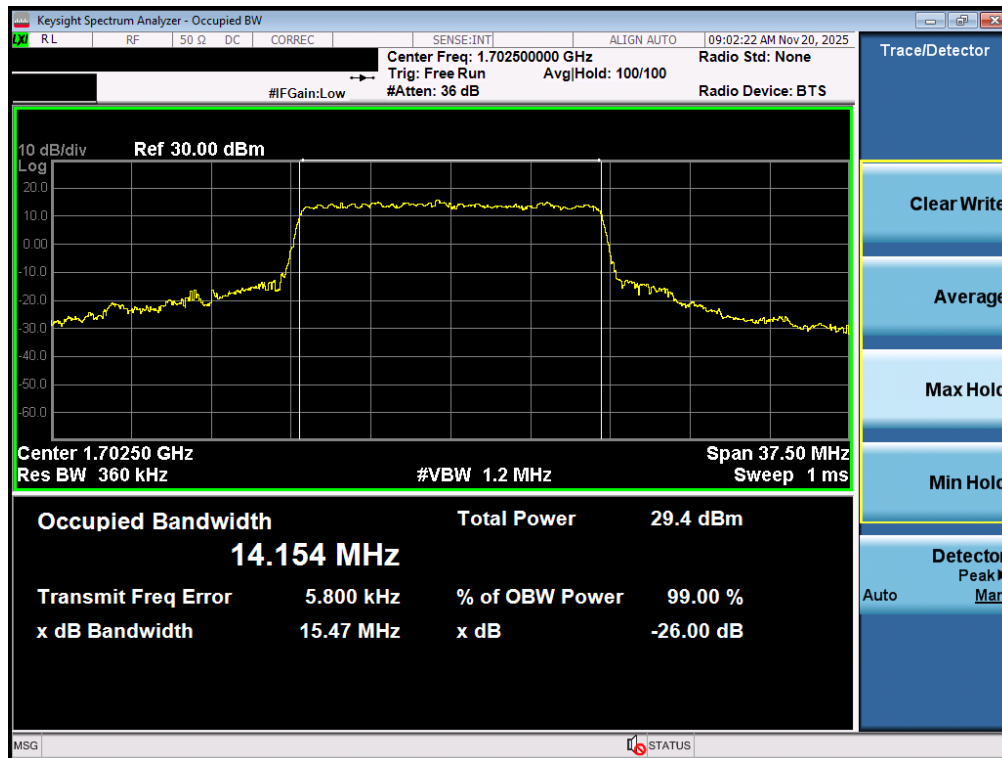
Plot 7-47. Occupied Bandwidth Plot (NR Band n70 - 15.0MHz CP-OFDM QPSK - Full RB – ANT1)
