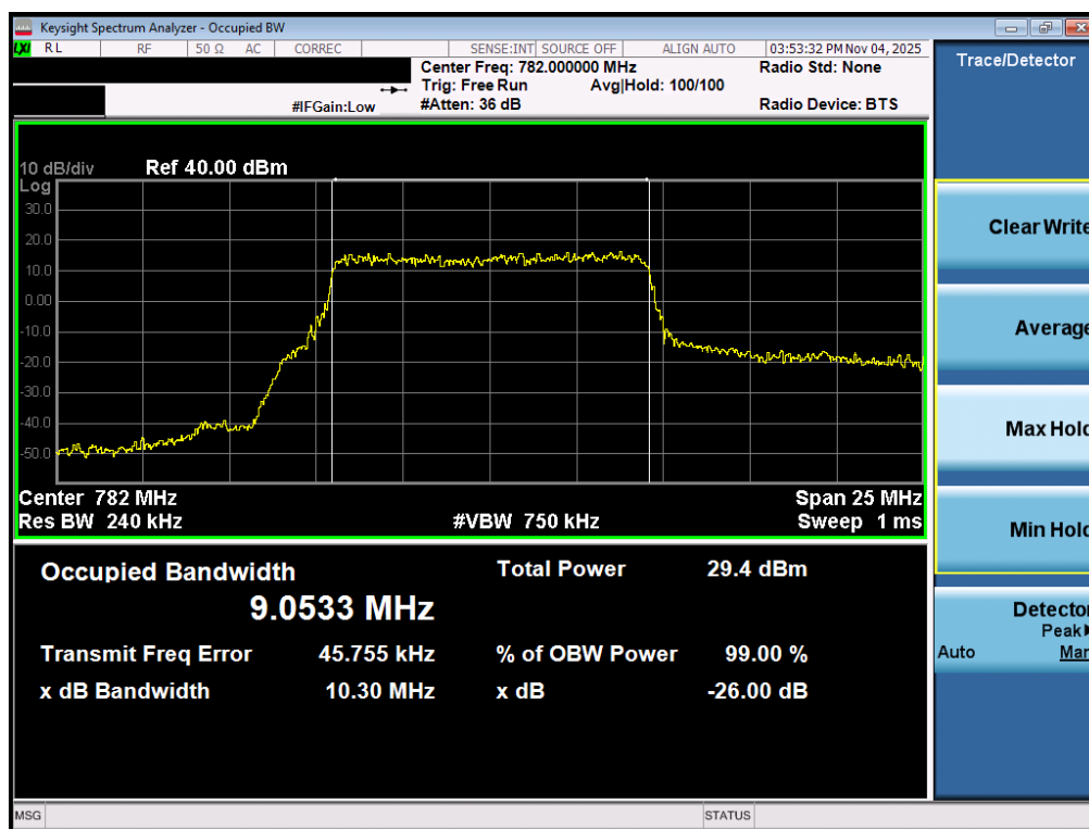
Plot 7-92. Occupied Bandwidth Plot (LTE Band 13 - 10MHz QPSK - Full RB – ANT2)
