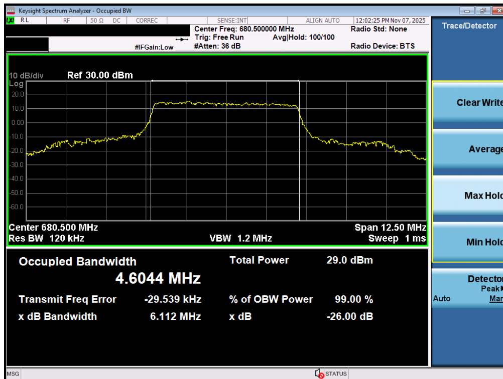
Plot 7-45. Occupied Bandwidth Plot (NR Band n71 - 5MHz CP-OFDM 16-QAM - Full RB – ANT1)
