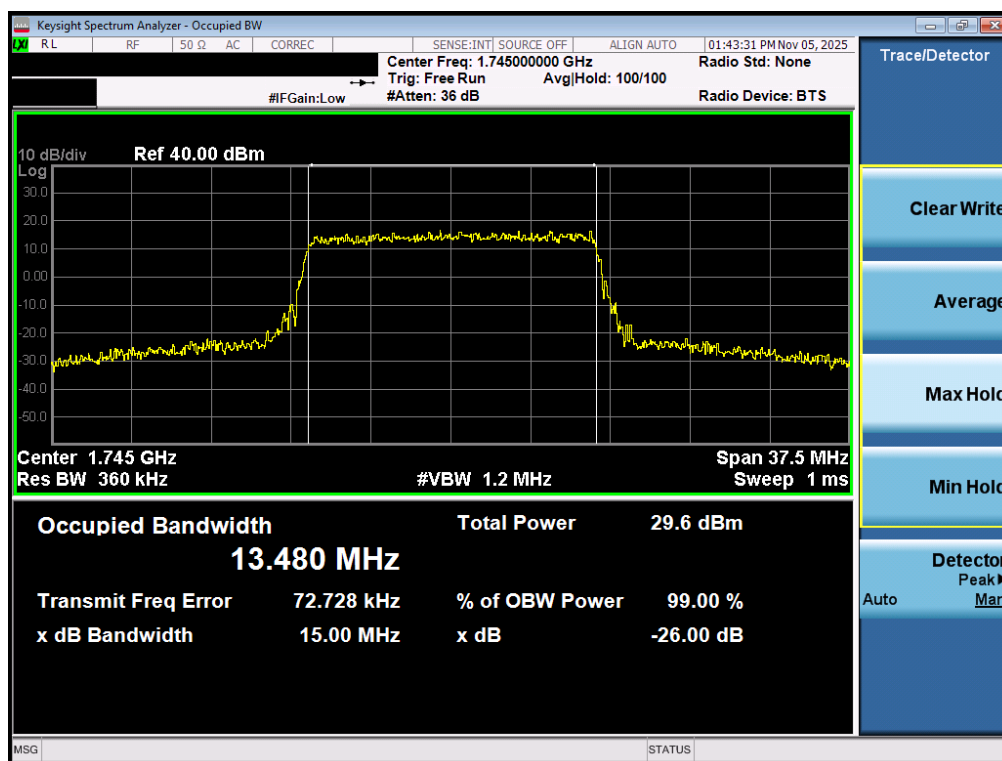
Plot 7-98. Occupied Bandwidth Plot (LTE Band 66/4 - 15MHz QPSK - Full RB - ANT2)
