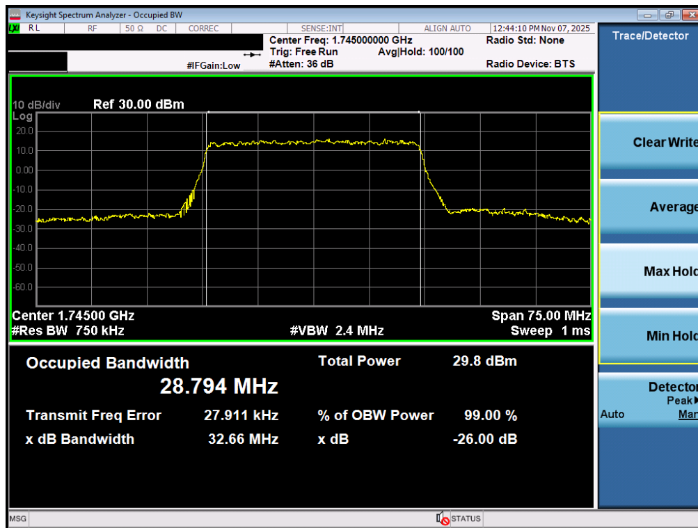
Plot 7-60. Occupied Bandwidth Plot (NR Band n66 - 30.0MHz CP-OFDM 16QAM - Full RB – ANT1)
