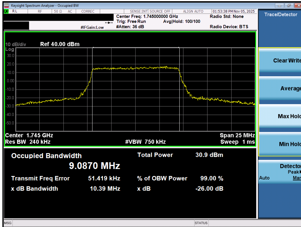
Plot 7-100. Occupied Bandwidth Plot (LTE Band 66/4 - 10MHz QPSK - Full RB - ANT2)
