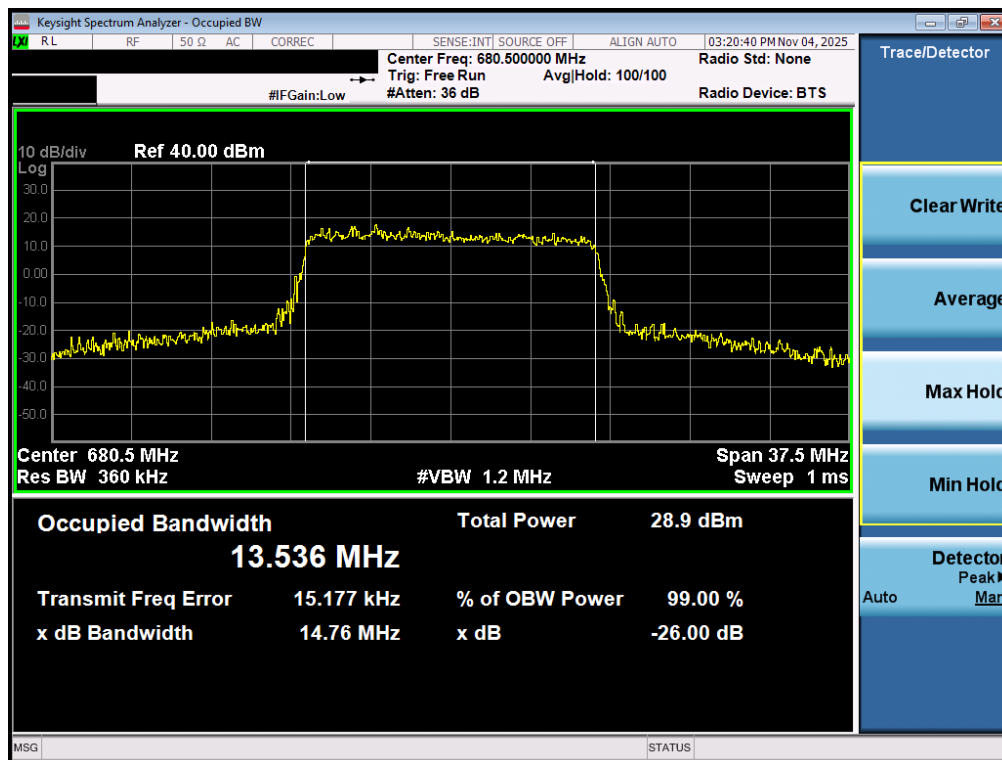
Plot 7-79. Occupied Bandwidth Plot (LTE Band 71 - 15MHz 16-QAM - Full RB – ANT2)
