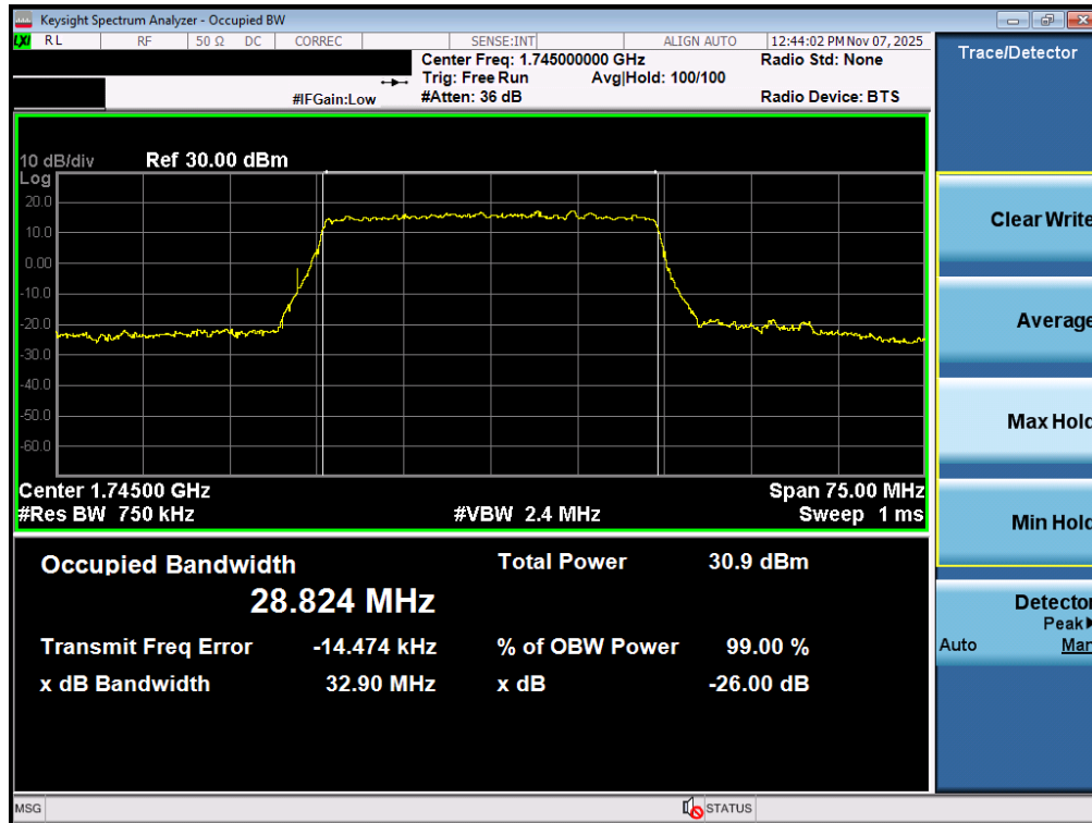
Plot 7-59. Occupied Bandwidth Plot (NR Band n66 - 30.0MHz CP-OFDM QPSK - Full RB – ANT1)
