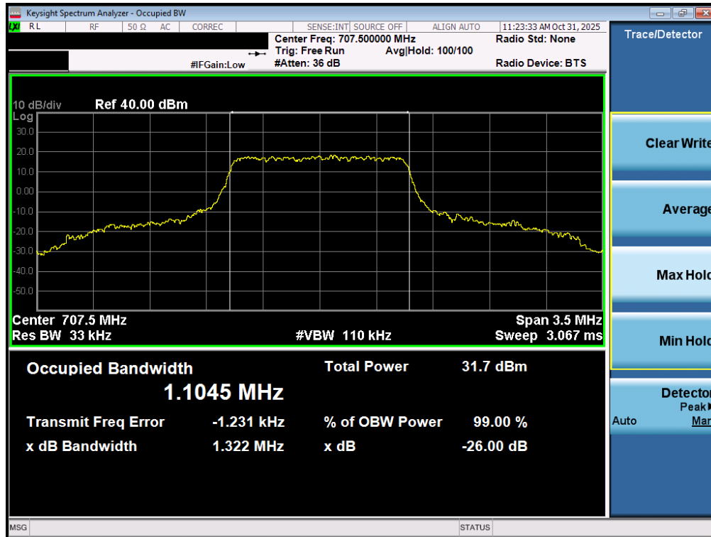
Plot 7-90. Occupied Bandwidth Plot (LTE Band 12 – 1.4MHz QPSK - Full RB – ANT2)
