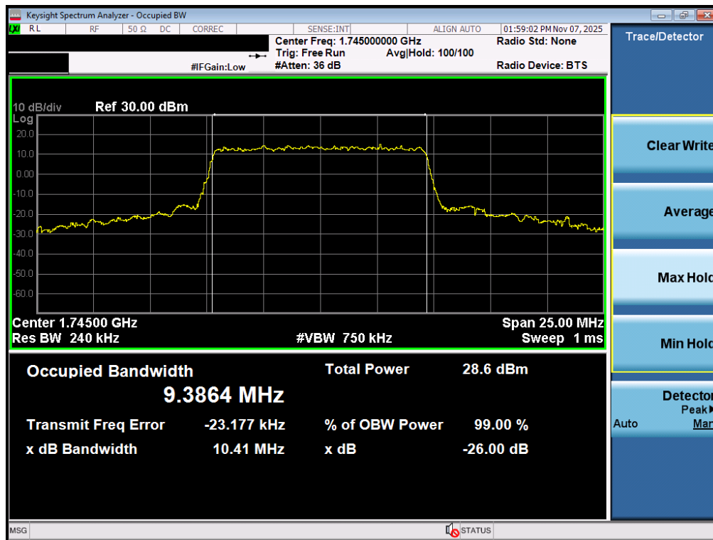
Plot 7-72. Occupied Bandwidth Plot (NR Band n66 - 10.0MHz CP-OFDM 16QAM - Full RB – ANT1)
