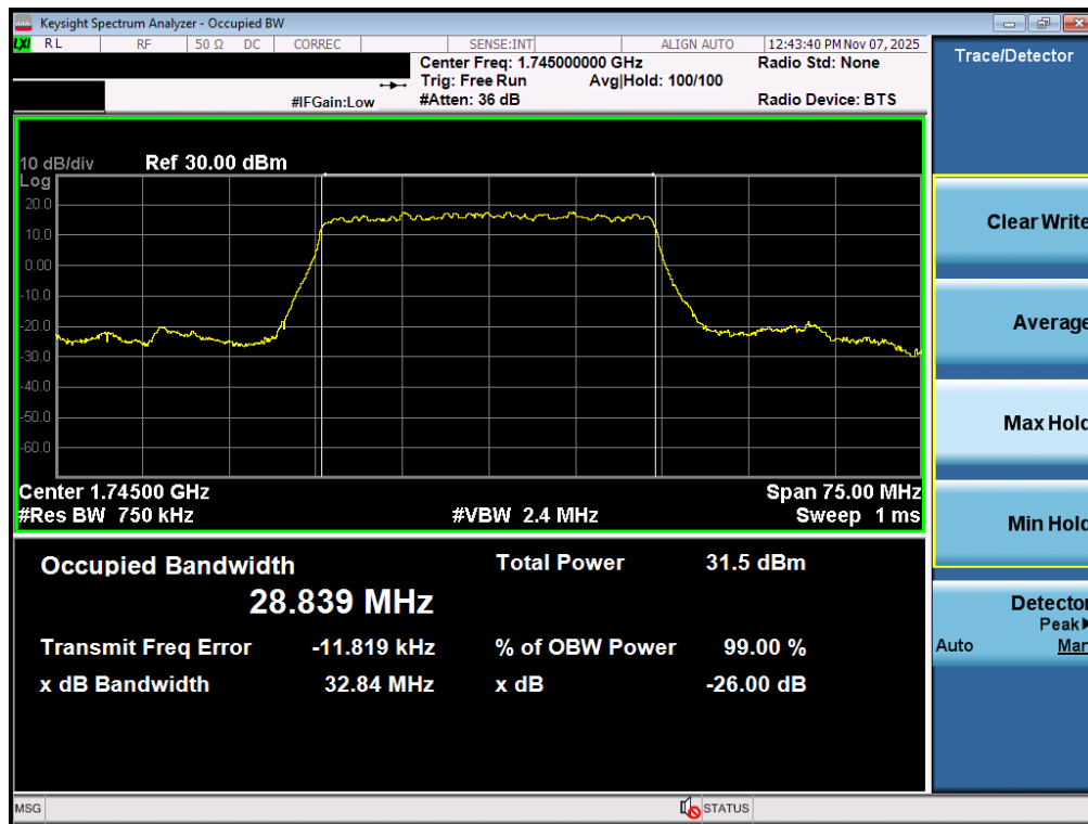
Plot 7-58. Occupied Bandwidth Plot (NR Band n66 - 30.0MHz DFT-s-OFDM BPSK - Full RB - ANT1)
