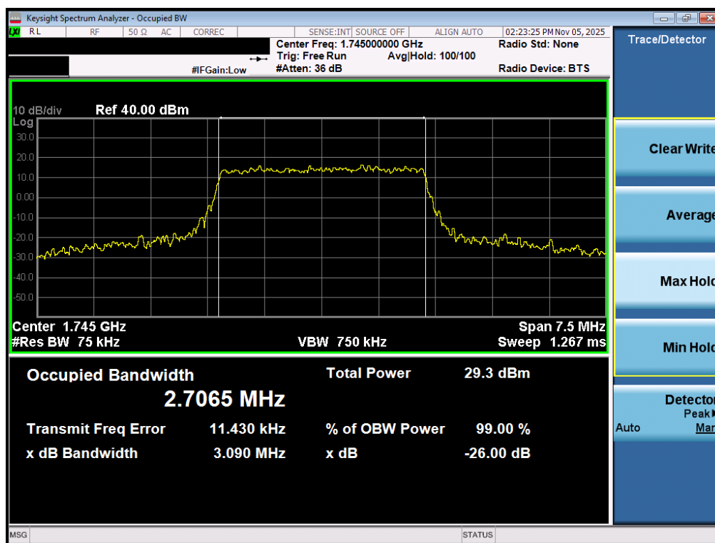
Plot 7-104. Occupied Bandwidth Plot (LTE Band 66/4 - 3MHz QPSK - Full RB - ANT2)
