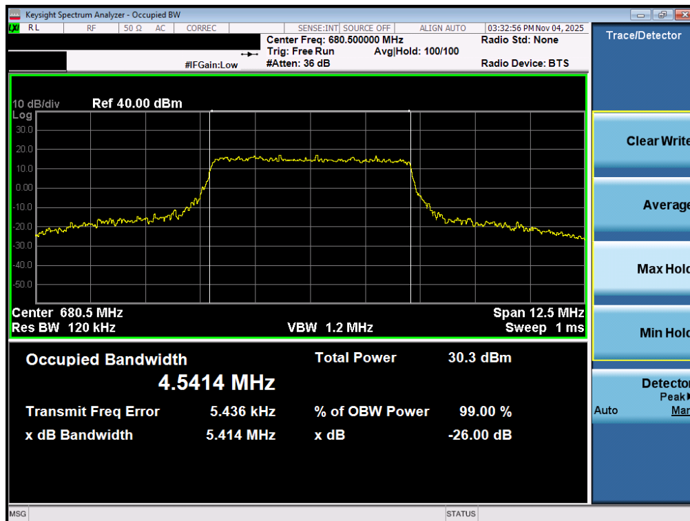
Plot 7-83. Occupied Bandwidth Plot (LTE Band 71 - 5MHz 16-QAM - Full RB – ANT2)
