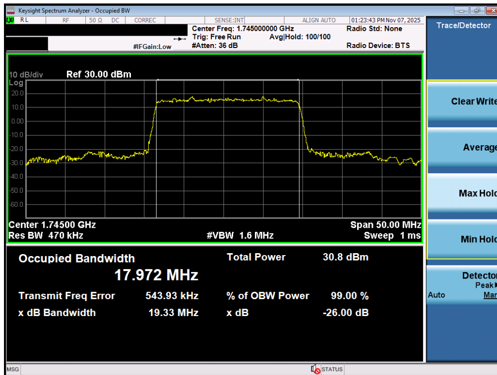
Plot 7-64. Occupied Bandwidth Plot (NR Band n66 - 20.0MHz DFT-s-OFDM BPSK - Full RB – ANT1)
