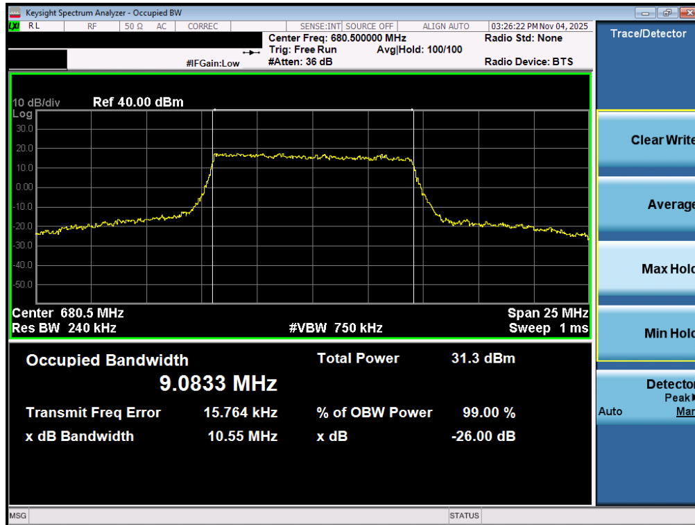
Plot 7-80. Occupied Bandwidth Plot (LTE Band 71 - 10MHz QPSK - Full RB – ANT2)
