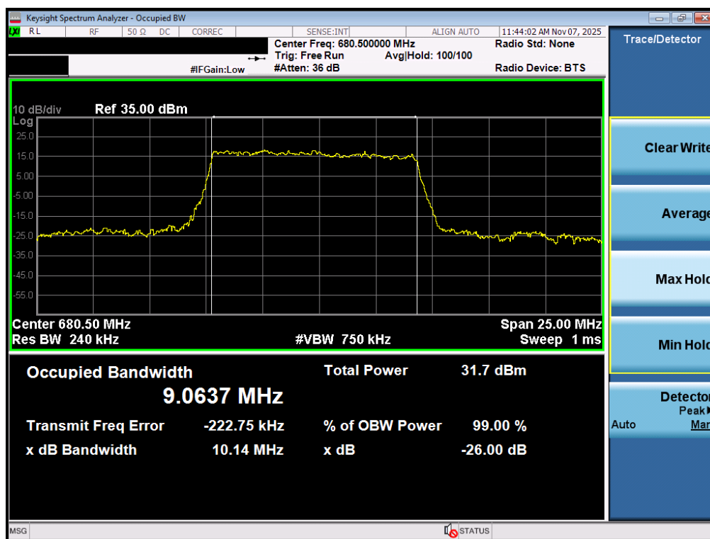
Plot 7-40. Occupied Bandwidth Plot (NR Band n71 - 10MHz DFT-s-OFDM BPSK - Full RB – ANT1)
