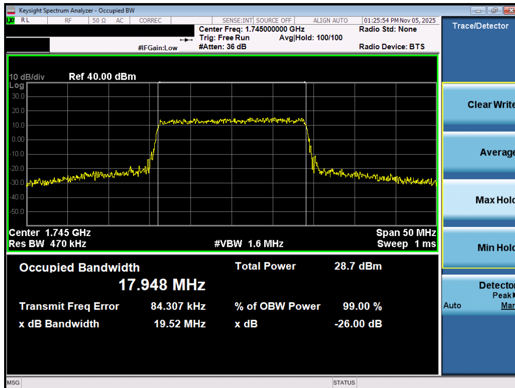
Plot 7-97. Occupied Bandwidth Plot (LTE Band 66/4 - 20MHz 16-QAM - Full RB - ANT2)
