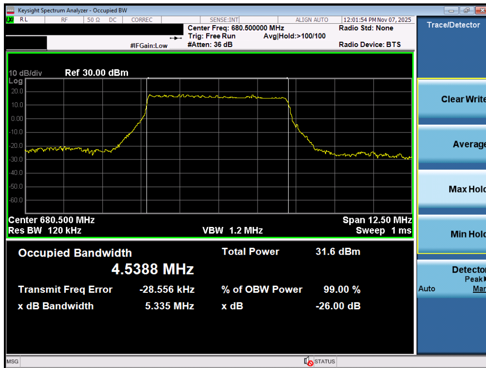
Plot 7-43. Occupied Bandwidth Plot (NR Band n71 - 5MHz DFT-s-OFDM BPSK - Full RB – ANT1)
