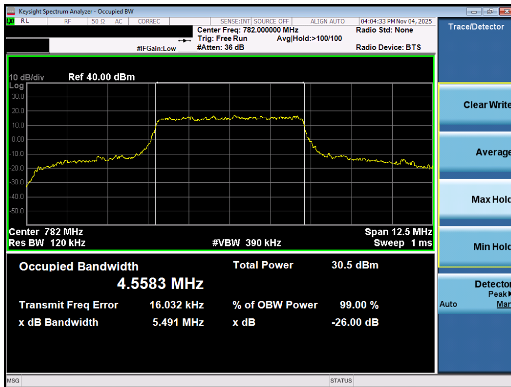
Plot 7-95. Occupied Bandwidth Plot (LTE Band 13 - 5MHz 16-QAM - Full RB – ANT2)
