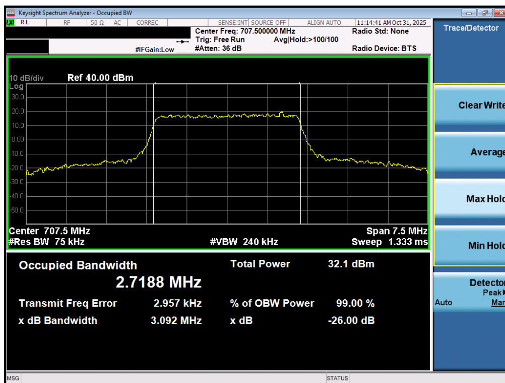
Plot 7-88. Occupied Bandwidth Plot (LTE Band 12 - 3MHz QPSK - Full RB – ANT2)
