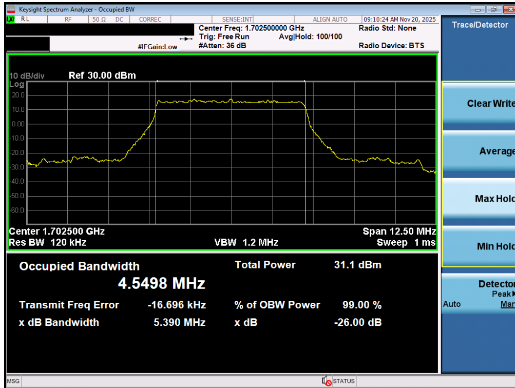
Plot 7-52. Occupied Bandwidth Plot (NR Band n70 - 5.0MHz DFT-s-OFDM BPSK - Full RB – ANT1)
