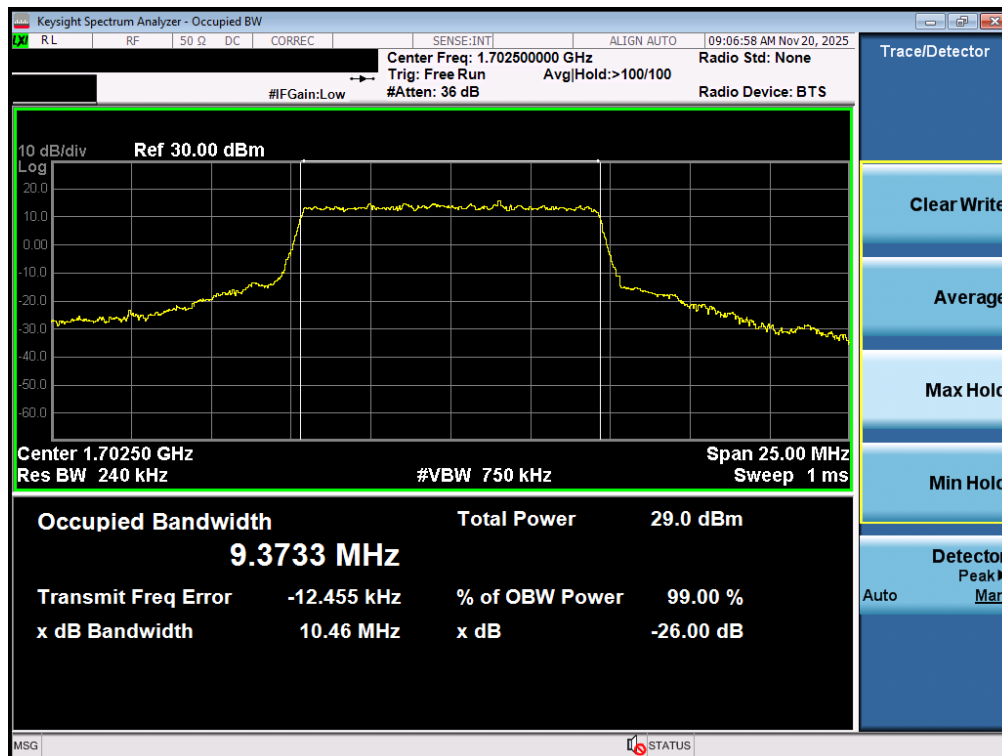
Plot 7-51. Occupied Bandwidth Plot (NR Band n70 - 10.0MHz CP-OFDM 16QAM - Full RB – ANT1)
