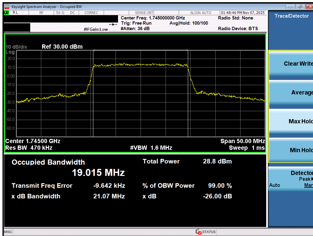
Plot 7-66. Occupied Bandwidth Plot (NR Band n66 - 20.0MHz CP-OFDM 16QAM - Full RB – ANT1)
