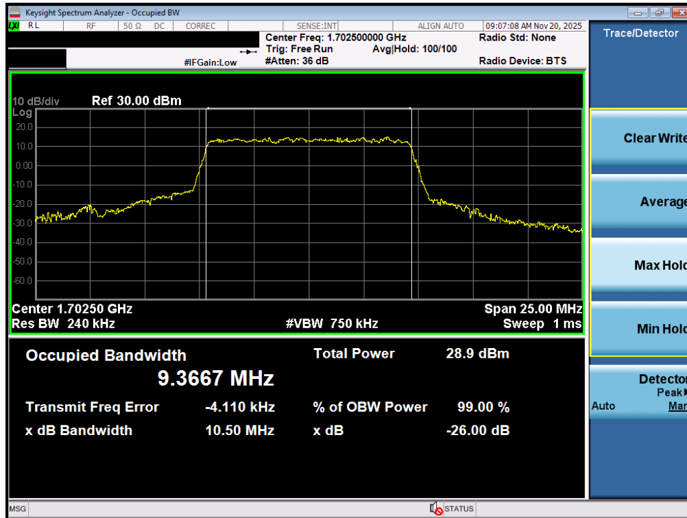
Plot 7-50. Occupied Bandwidth Plot (NR Band n70 - 10.0MHz CP-OFDM QPSK - Full RB – ANT1)
