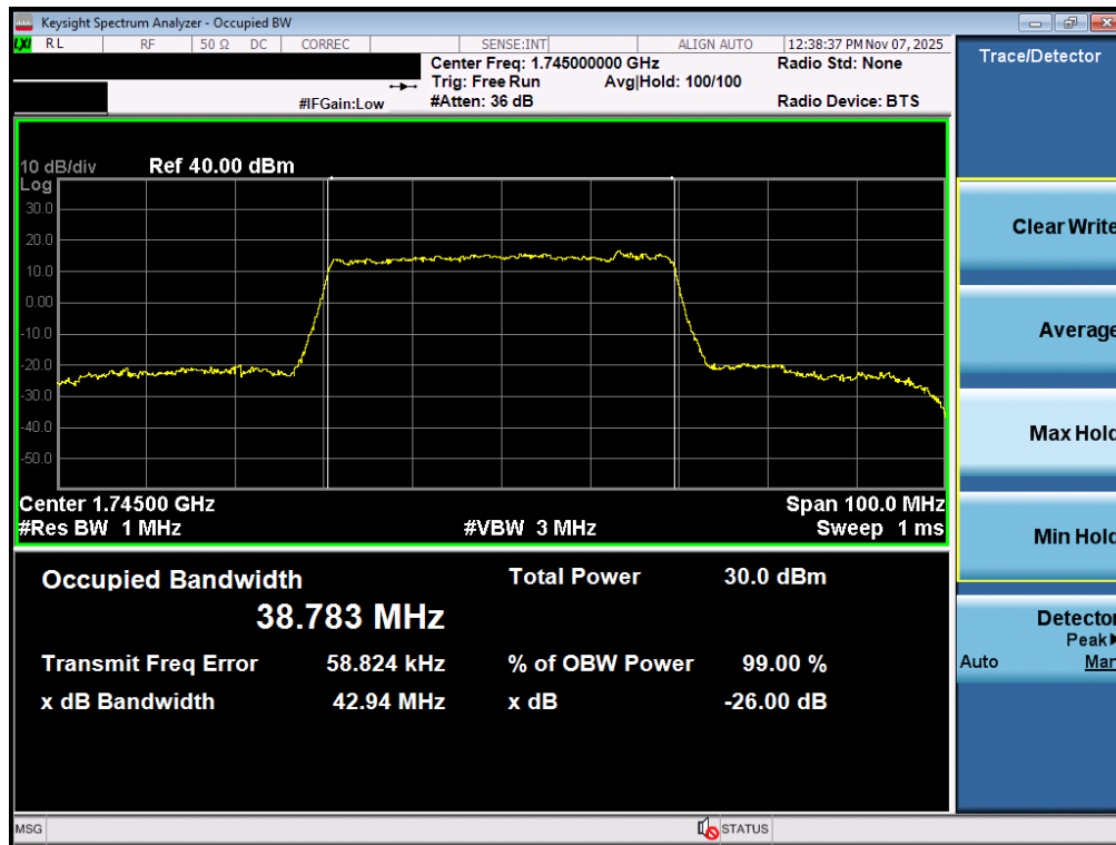
Plot 7-57. Occupied Bandwidth Plot (NR Band n66 - 40.0MHz CP-OFDM 16QAM - Full RB - ANT1)
