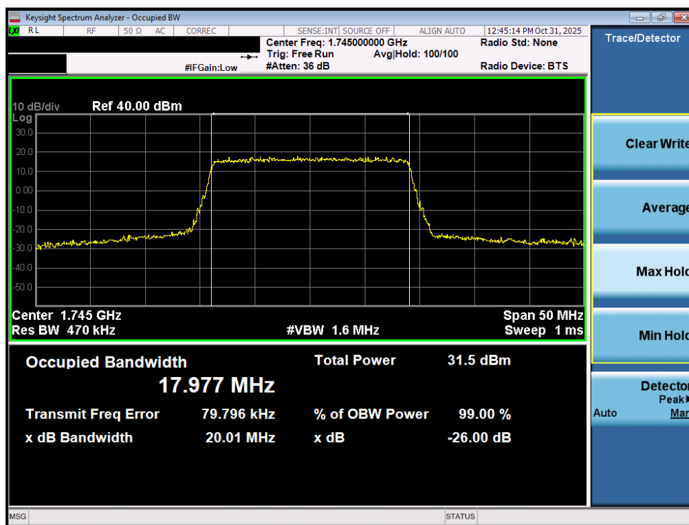
Plot 7-22. Occupied Bandwidth Plot (LTE Band 66/4 - 20MHz QPSK - Full RB - ANT1)
