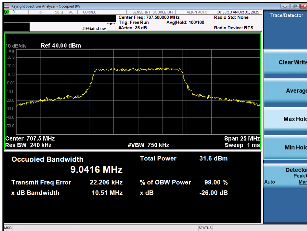
Plot 7-85. Occupied Bandwidth Plot (LTE Band 12 - 10MHz 16-QAM - Full RB – ANT2)
