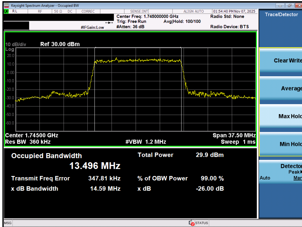
Plot 7-67. Occupied Bandwidth Plot (NR Band n66 - 15.0MHz DFT-s-OFDM BPSK - Full RB – ANT1)
