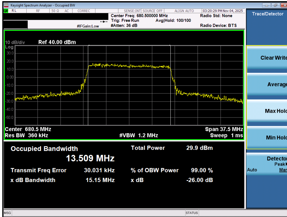
Plot 7-78. Occupied Bandwidth Plot (LTE Band 71 - 15MHz QPSK - Full RB – ANT2)
