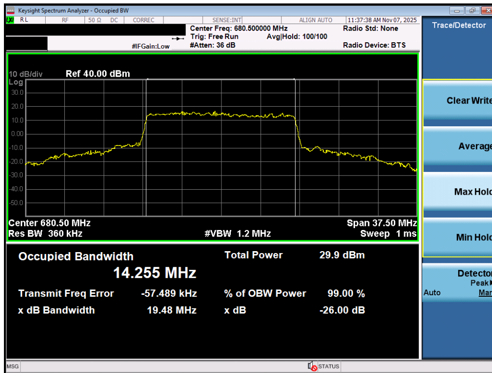
Plot 7-39. Occupied Bandwidth Plot (NR Band n71 - 15MHz CP-OFDM 16-QAM - Full RB – ANT1)
