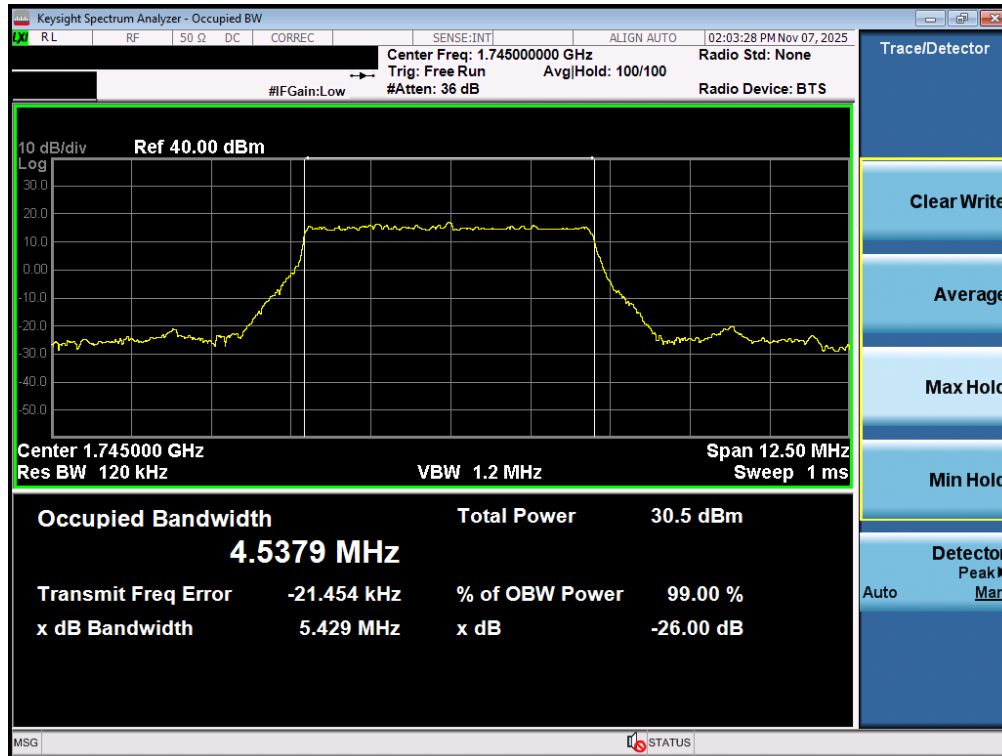
Plot 7-73. Occupied Bandwidth Plot (NR Band n66 - 5.0MHz DFT-s-OFDM BPSK - Full RB – ANT1)
