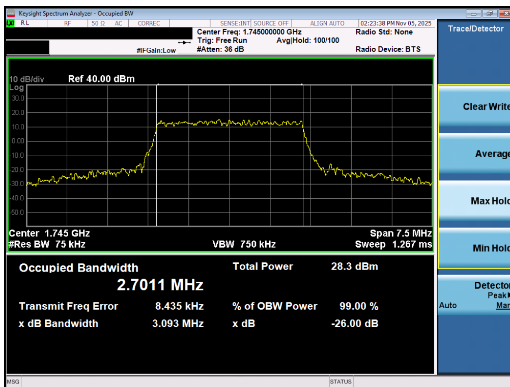
Plot 7-105. Occupied Bandwidth Plot (LTE Band 66/4 - 3MHz 16-QAM - Full RB - ANT2)
