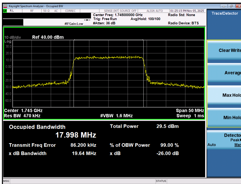
Plot 7-96. Occupied Bandwidth Plot (LTE Band 66/4 - 20MHz QPSK - Full RB - ANT2)
