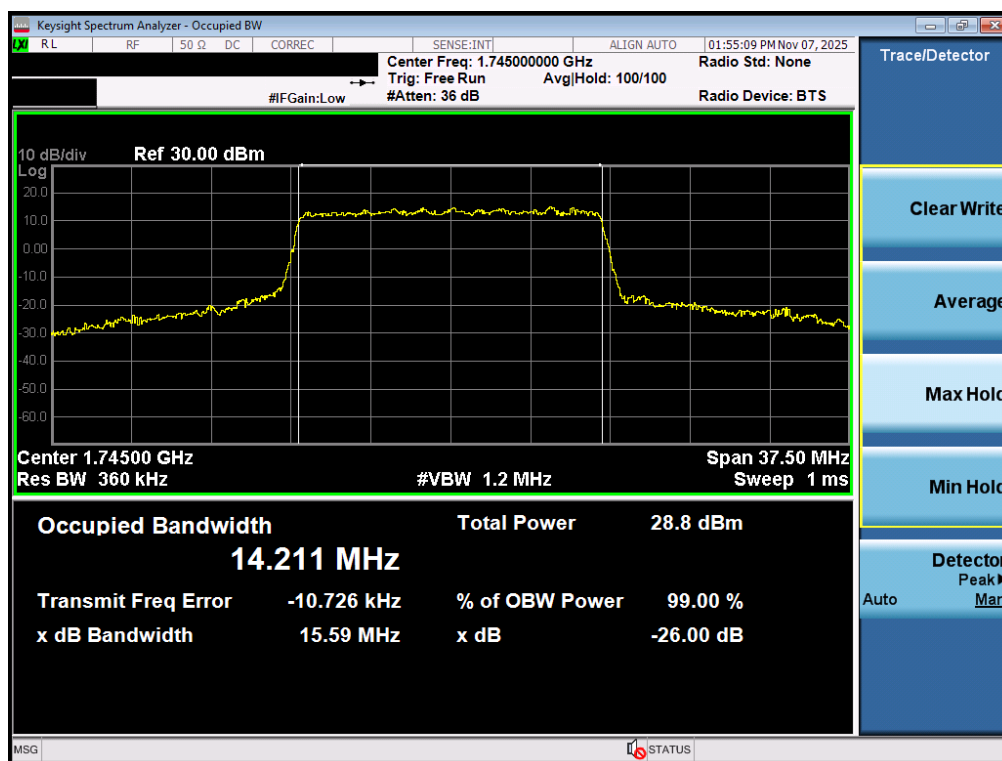
Plot 7-69. Occupied Bandwidth Plot (NR Band n66 - 15.0MHz CP-OFDM 16QAM - Full RB – ANT1)
