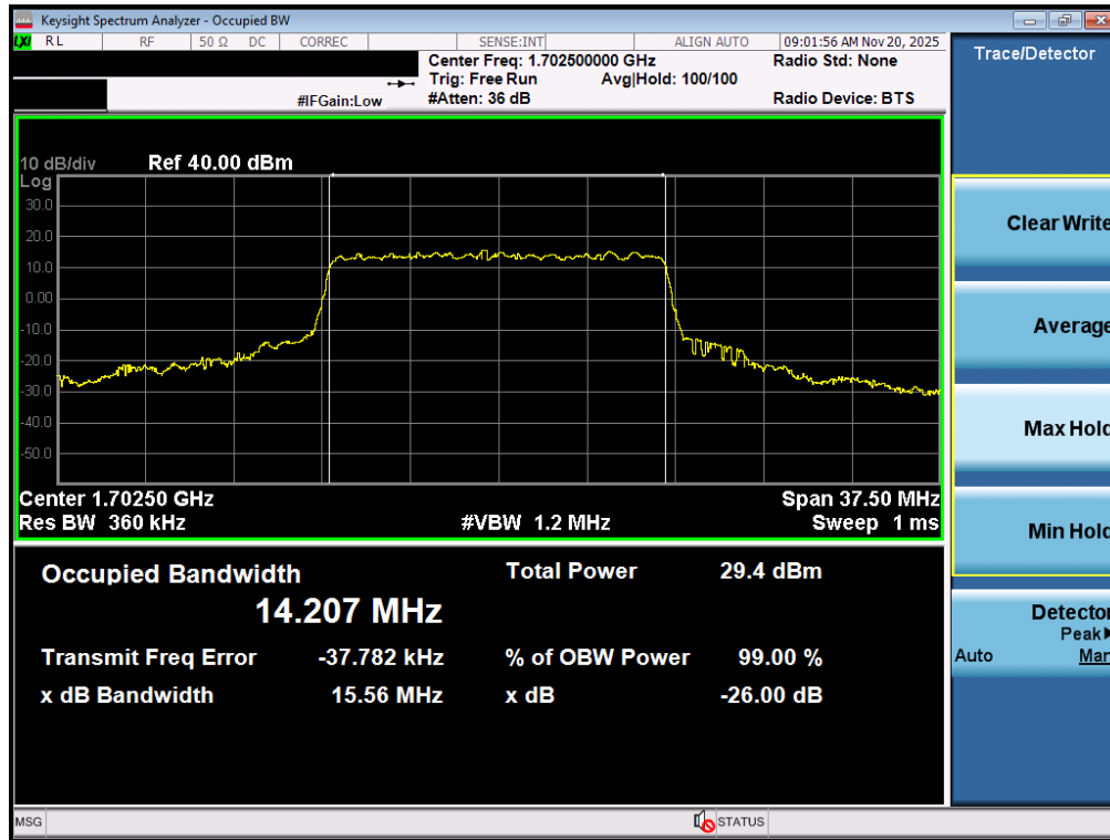
Plot 7-48. Occupied Bandwidth Plot (NR Band n70 - 15.0MHz CP-OFDM 16QAM - Full RB – ANT1)
