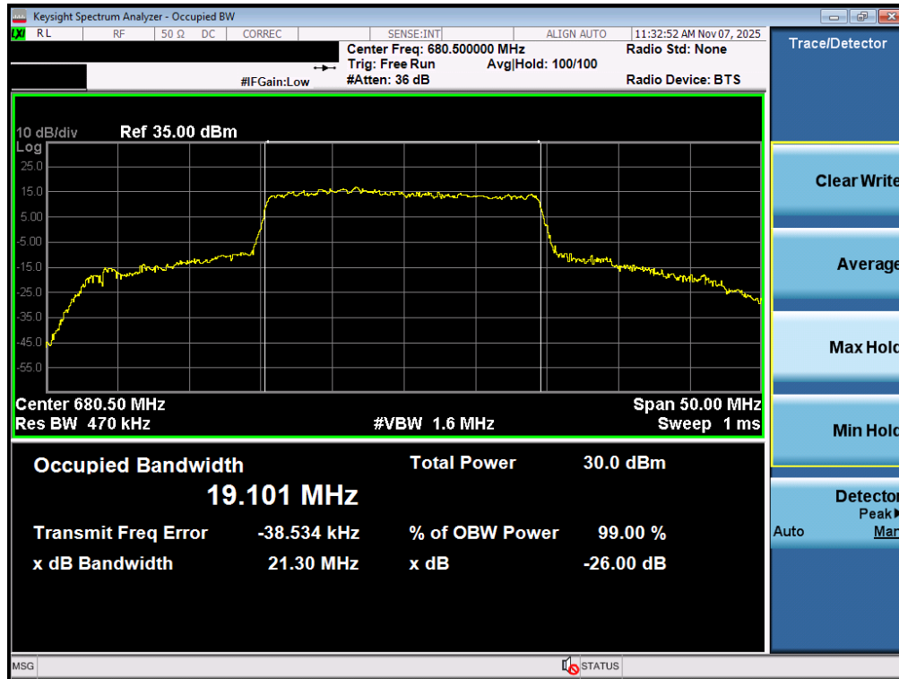
Plot 7-36. Occupied Bandwidth Plot (NR Band n71 - 20MHz CP-OFDM 16-QAM - Full RB – ANT1)
