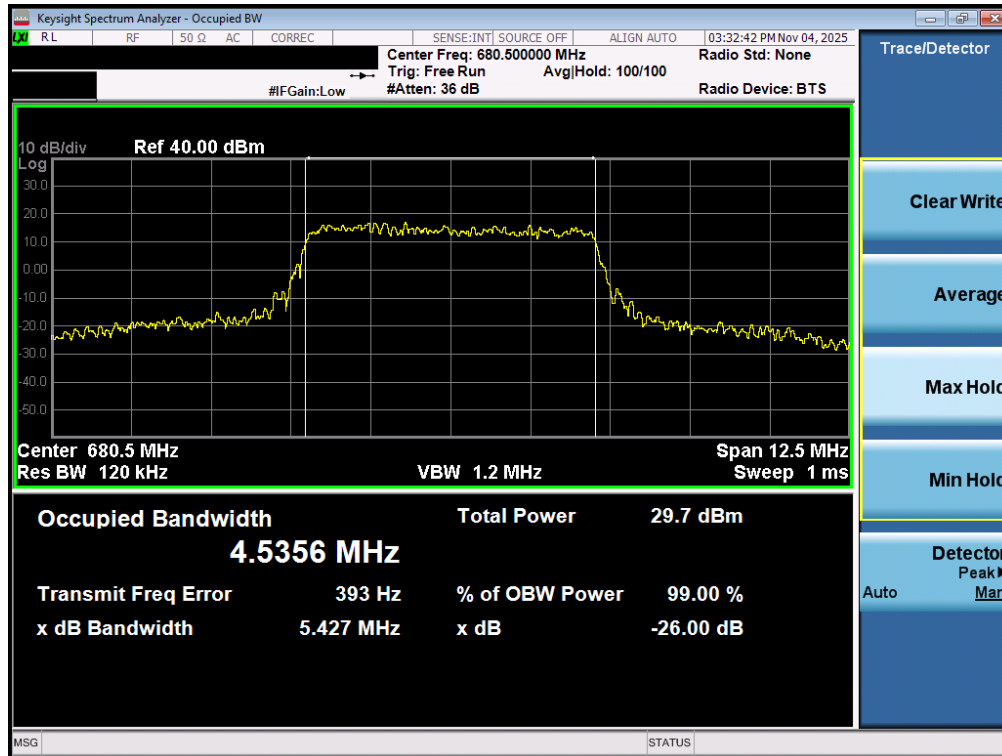
Plot 7-82. Occupied Bandwidth Plot (LTE Band 71 - 5MHz QPSK - Full RB – ANT2)
