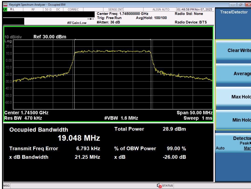
Plot 7-65. Occupied Bandwidth Plot (NR Band n66 - 20.0MHz CP-OFDM QPSK - Full RB – ANT1)
