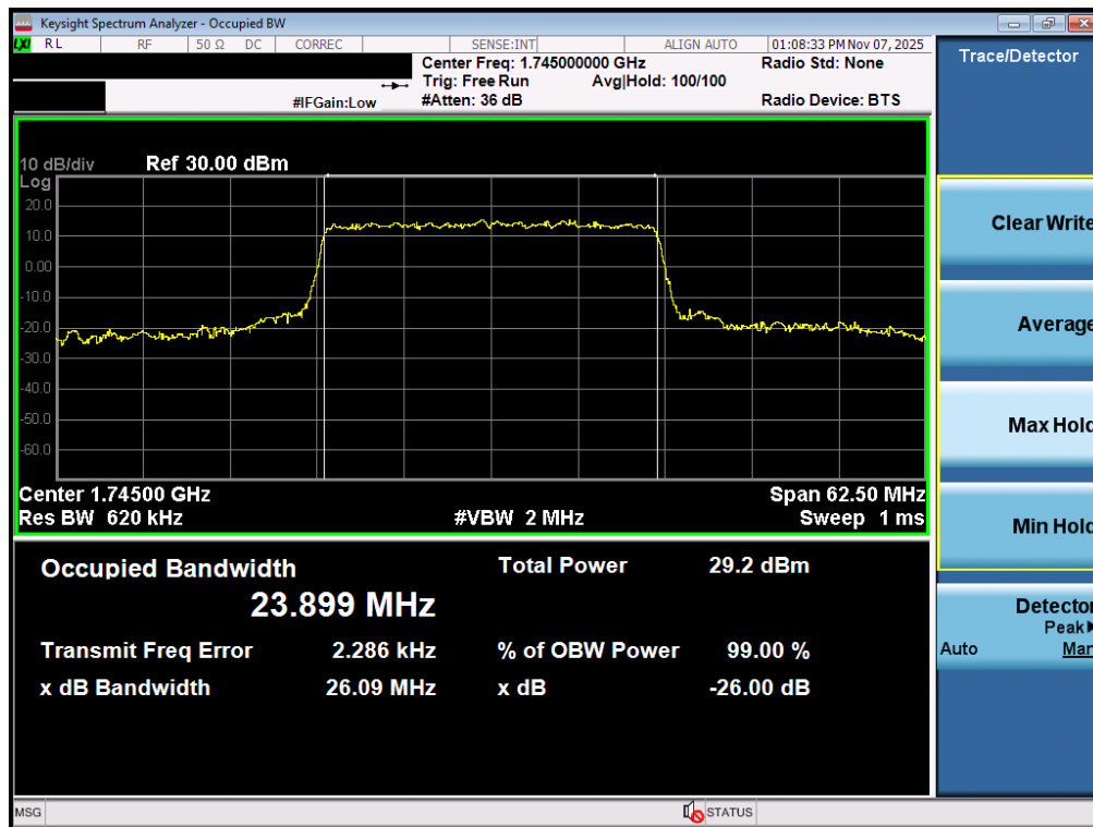
Plot 7-62. Occupied Bandwidth Plot (NR Band n66 - 25.0MHz CP-OFDM QPSK - Full RB – ANT1)
