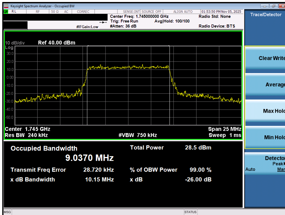
Plot 7-101. Occupied Bandwidth Plot (LTE Band 66/4 - 10MHz 16-QAM - Full RB - ANT2)
