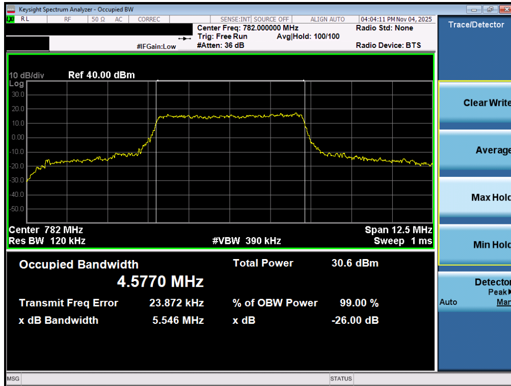
Plot 7-94. Occupied Bandwidth Plot (LTE Band 13 - 5MHz QPSK - Full RB – ANT2)
