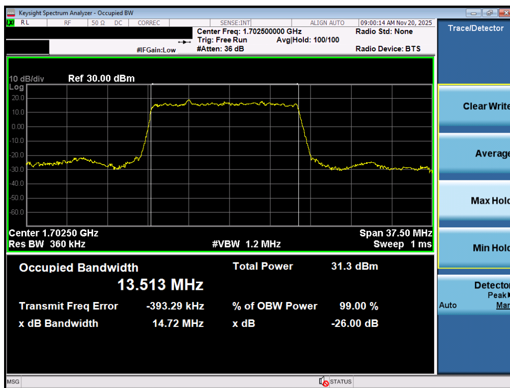
Plot 7-46. Occupied Bandwidth Plot (NR Band n70 - 15.0MHz DFT-s-OFDM BPSK - Full RB – ANT1)
