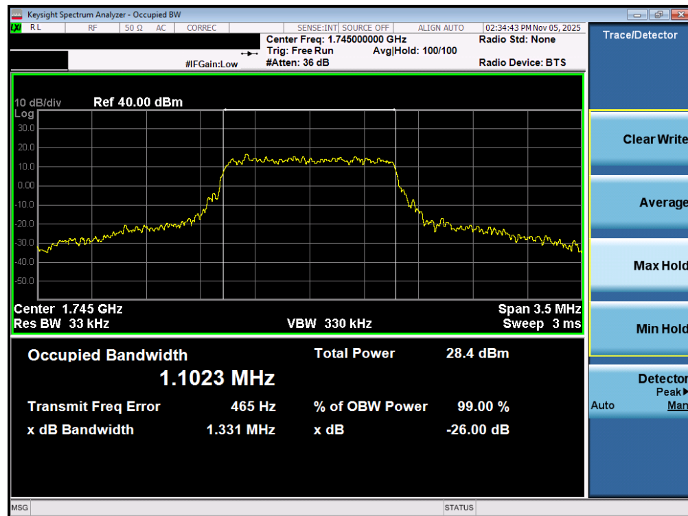
Plot 7-107. Occupied Bandwidth Plot (LTE Band 66/4 - 1.4MHz 16-QAM - Full RB - ANT2)
