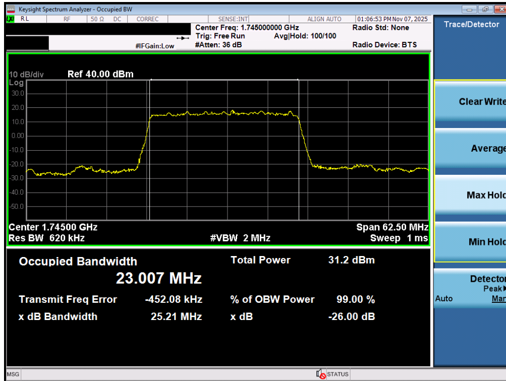
Plot 7-61. Occupied Bandwidth Plot (NR Band n66 - 25.0MHz DFT-s-OFDM BPSK - Full RB – ANT1)
