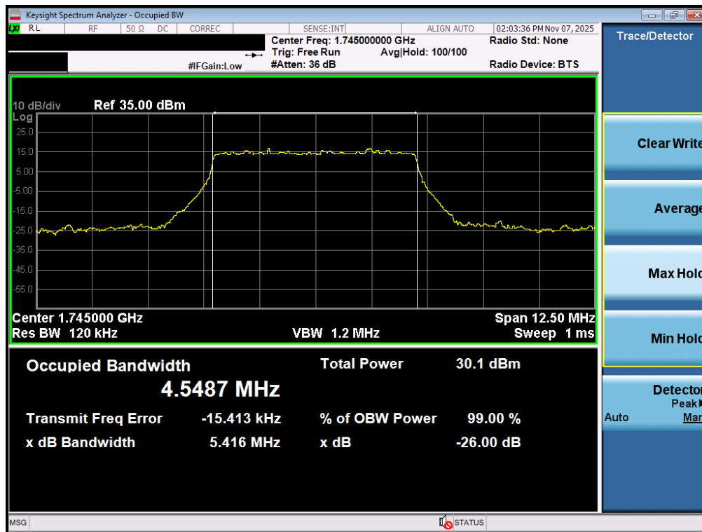
Plot 7-74. Occupied Bandwidth Plot (NR Band n66 - 5.0MHz CP-OFDM QPSK - Full RB – ANT1)
