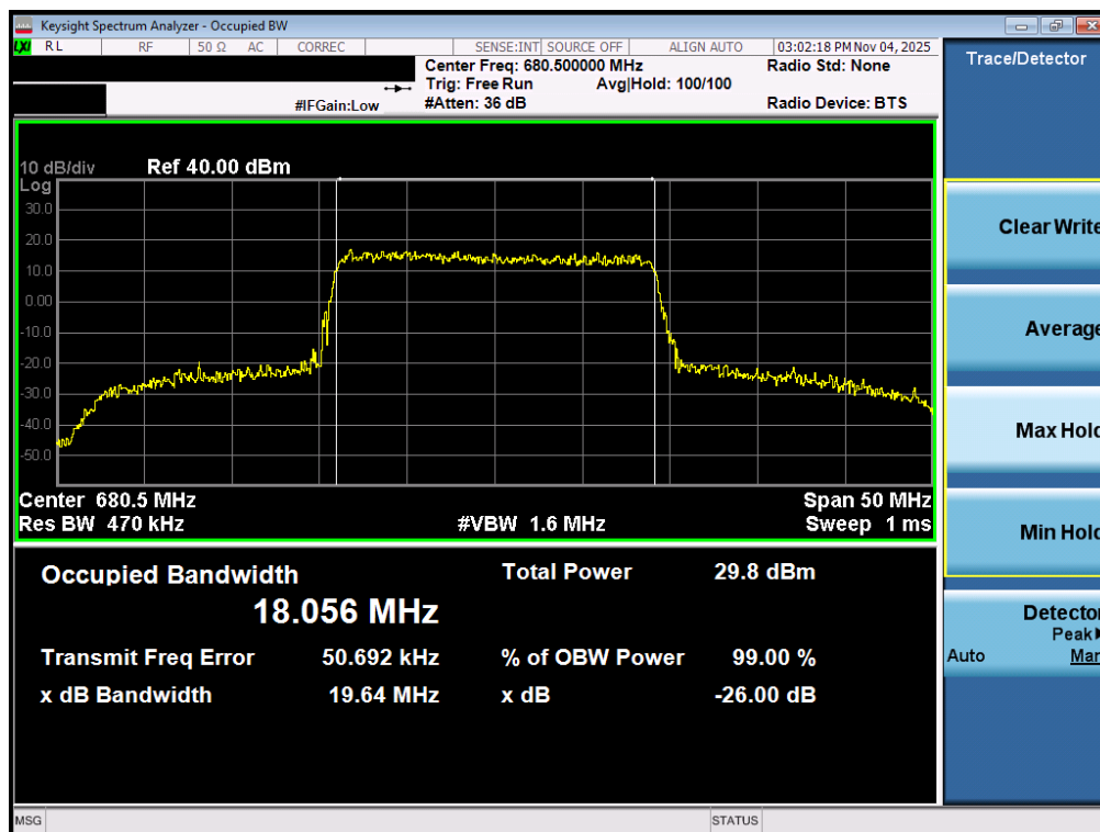
Plot 7-76. Occupied Bandwidth Plot (LTE Band 71 - 20MHz QPSK - Full RB – ANT2)
