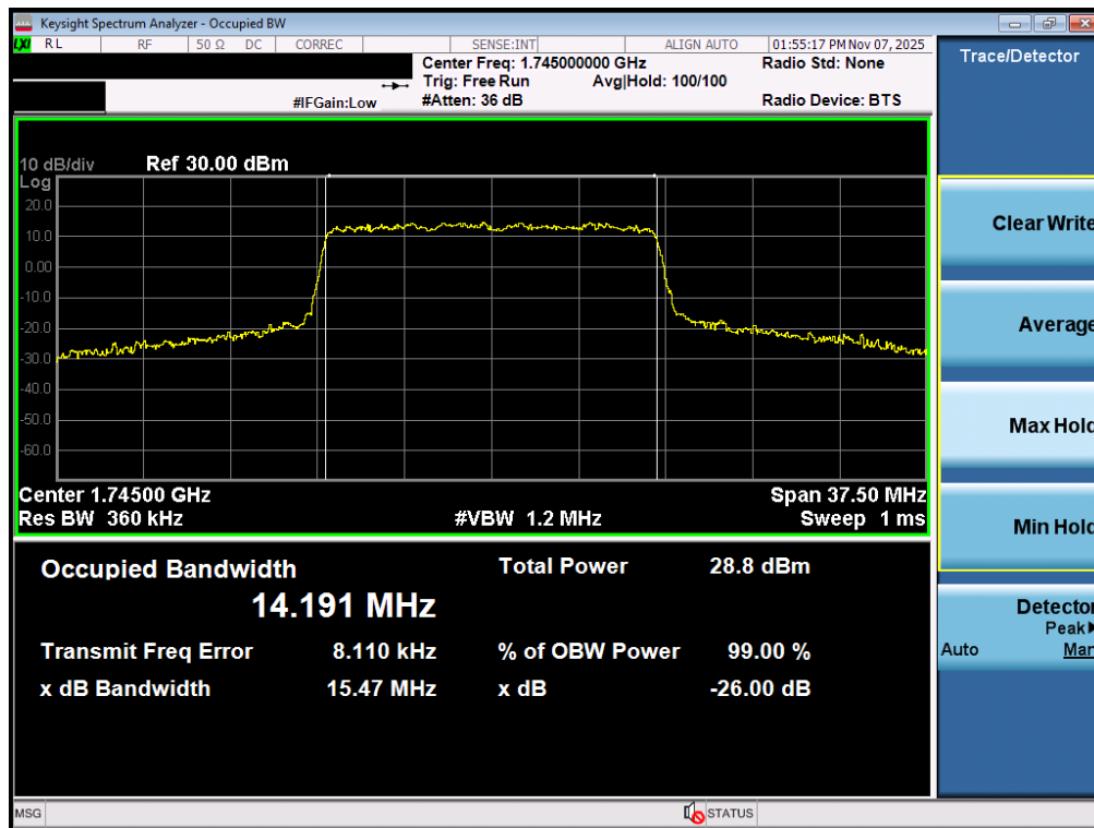
Plot 7-68. Occupied Bandwidth Plot (NR Band n66 - 15.0MHz CP-OFDM QPSK - Full RB – ANT1)
