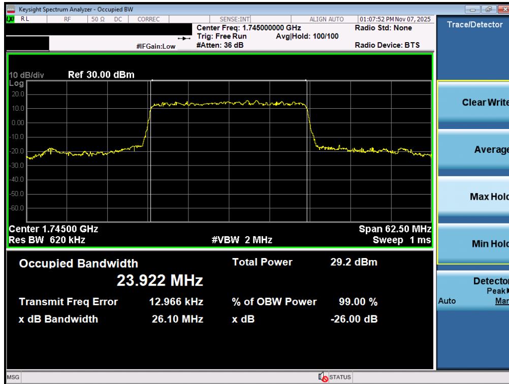
Plot 7-63. Occupied Bandwidth Plot (NR Band n66 - 25.0MHz CP-OFDM 16QAM - Full RB – ANT1)
