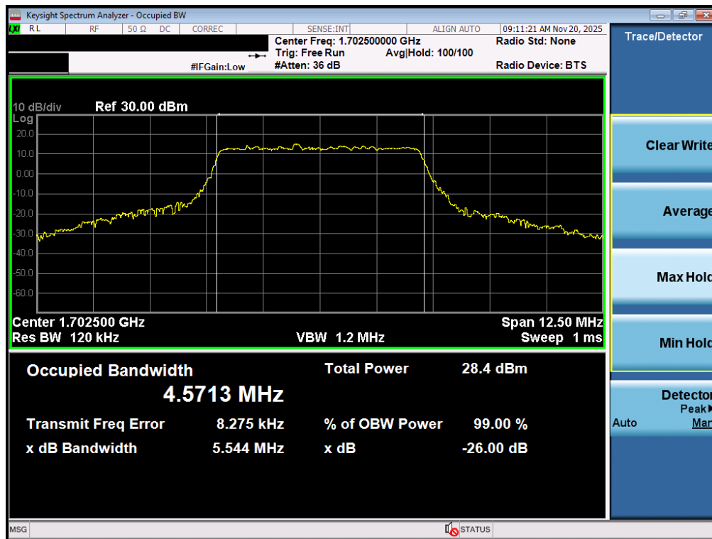
Plot 7-53. Occupied Bandwidth Plot (NR Band n70 - 5.0MHz CP-OFDM QPSK - Full RB – ANT1)
