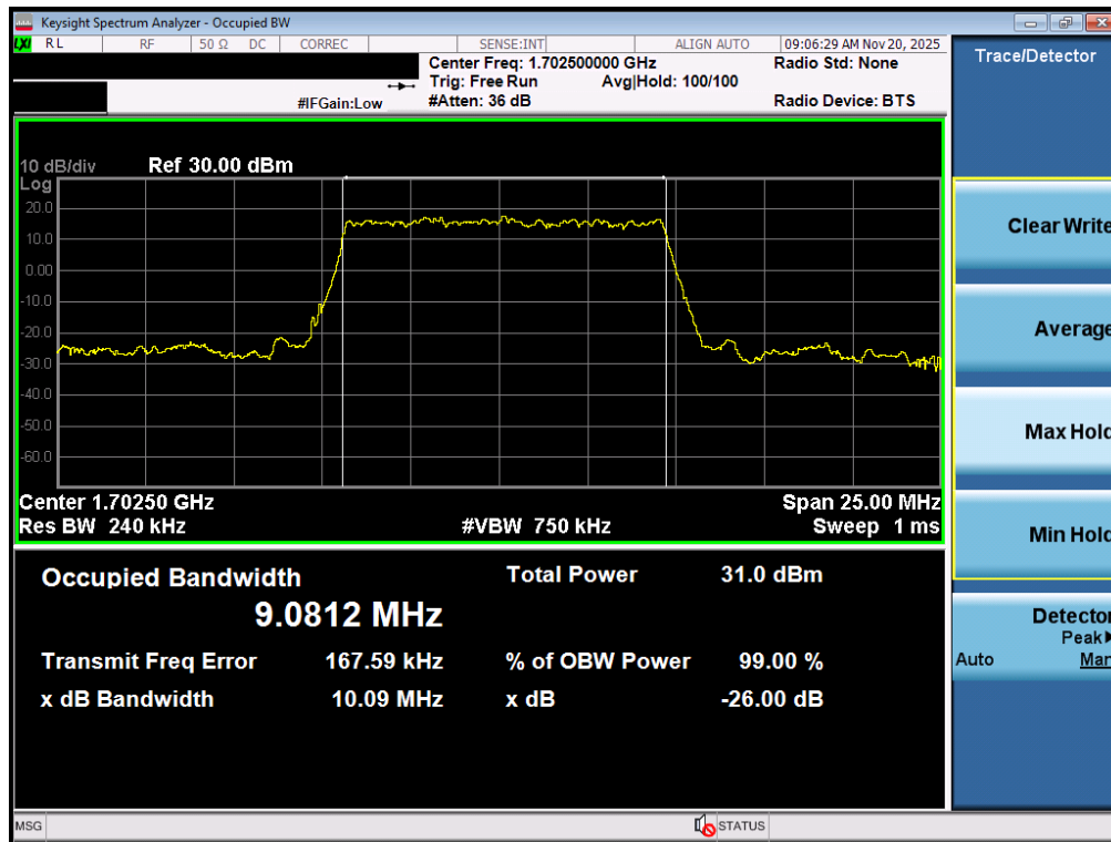
Plot 7-49. Occupied Bandwidth Plot (NR Band n70 - 10.0MHz DFT-s-OFDM BPSK - Full RB – ANT1)
