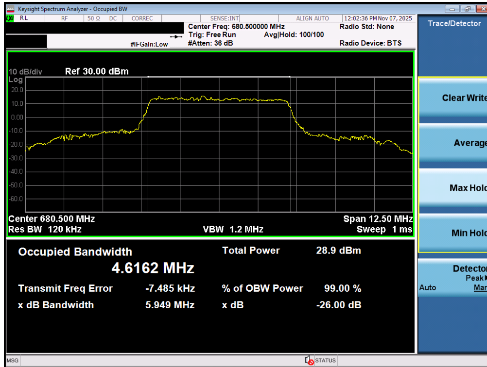
Plot 7-44. Occupied Bandwidth Plot (NR Band n71 - 5MHz CP-OFDM QPSK - Full RB – ANT1)
