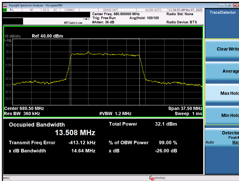
Plot 7-37. Occupied Bandwidth Plot (NR Band n71 - 15MHz DFT-s-OFDM BPSK - Full RB – ANT1)
