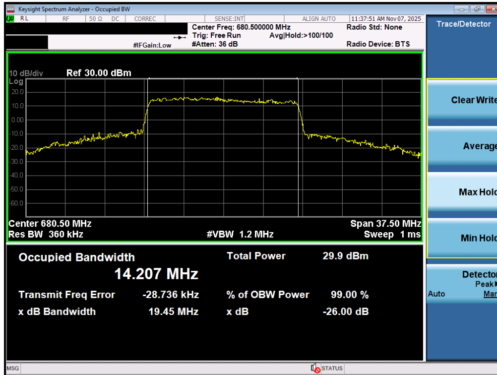
Plot 7-38. Occupied Bandwidth Plot (NR Band n71 - 15MHz QPSK - Full RB – ANT1)
