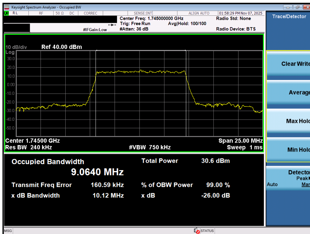
Plot 7-70. Occupied Bandwidth Plot (NR Band n66 - 10.0MHz DFT-s-OFDM BPSK - Full RB – ANT1)
