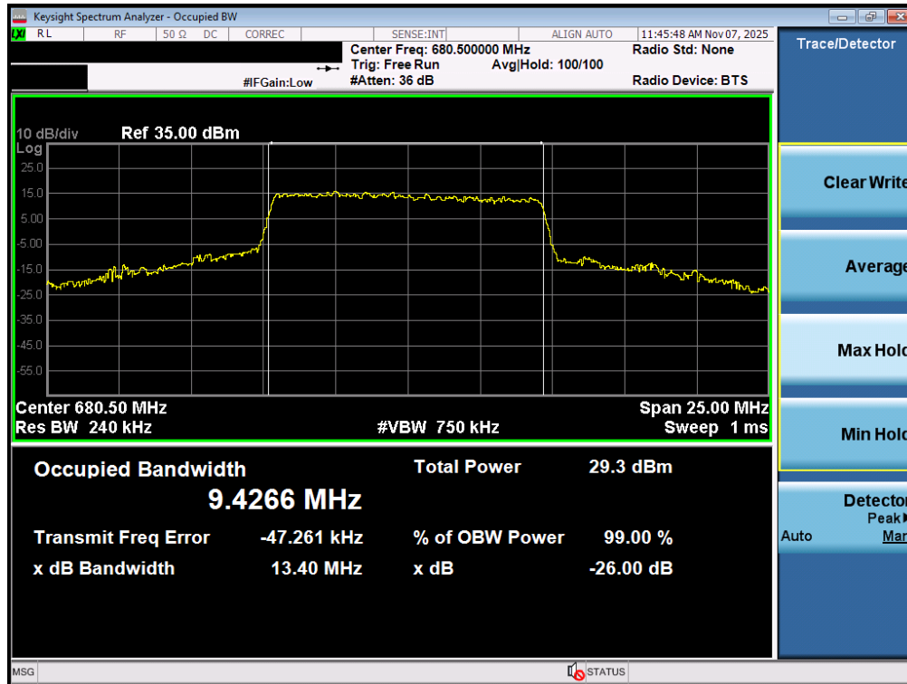
Plot 7-42. Occupied Bandwidth Plot (NR Band n71 - 10MHz CP-OFDM 16-QAM - Full RB – ANT1)
