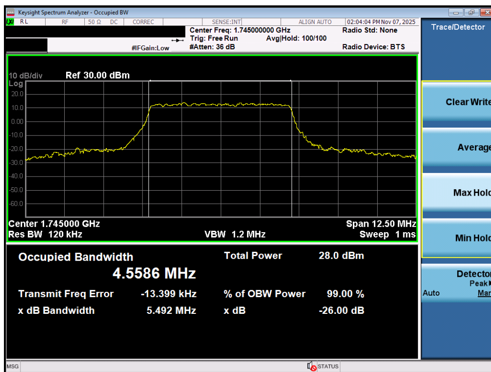
Plot 7-75. Occupied Bandwidth Plot (NR Band n66 - 5.0MHz CP-OFDM 16QAM - Full RB – ANT1)
