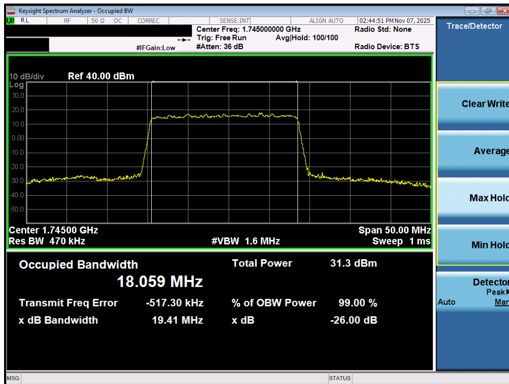
Plot 7-138. Occupied Bandwidth Plot (NR Band n66 - 20.0MHz DFT-s-OFDM BPSK - Full RB – ANT2)
