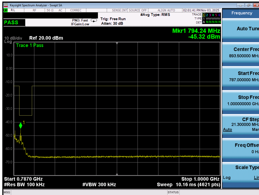
Plot 7-160. Conducted Spurious Plot (LTE Band 13 - 10MHz QPSK - 1 RB)
