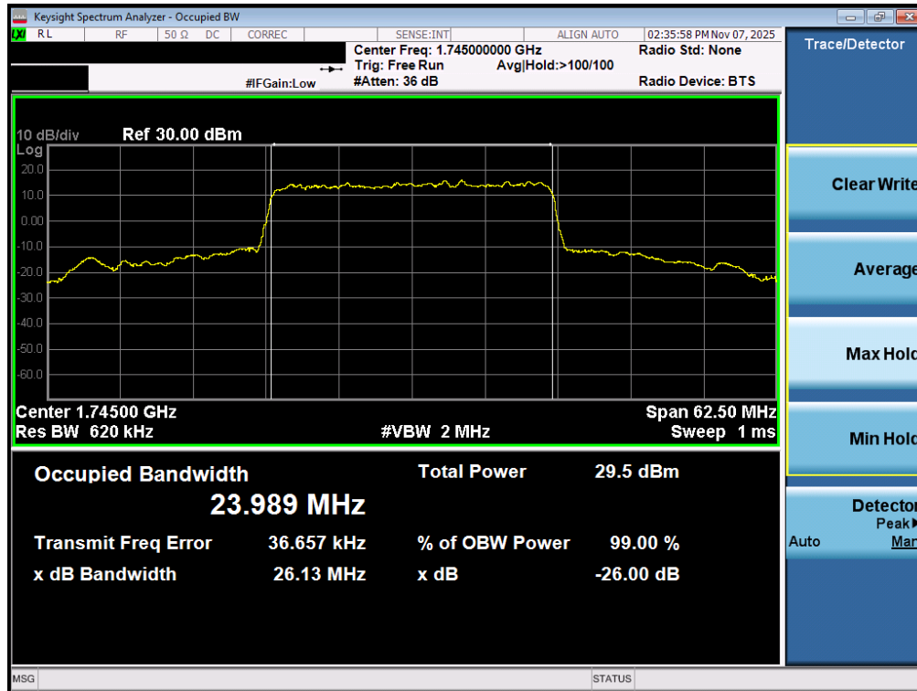
Plot 7-137. Occupied Bandwidth Plot (NR Band n66 - 25.0MHz CP-OFDM 16QAM - Full RB – ANT2)
