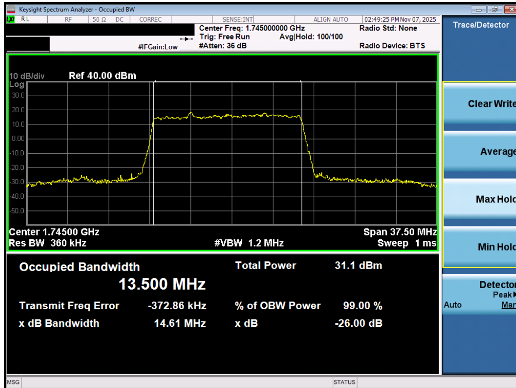
Plot 7-141. Occupied Bandwidth Plot (NR Band n66 - 15.0MHz DFT-s-OFDM BPSK - Full RB – ANT2)
