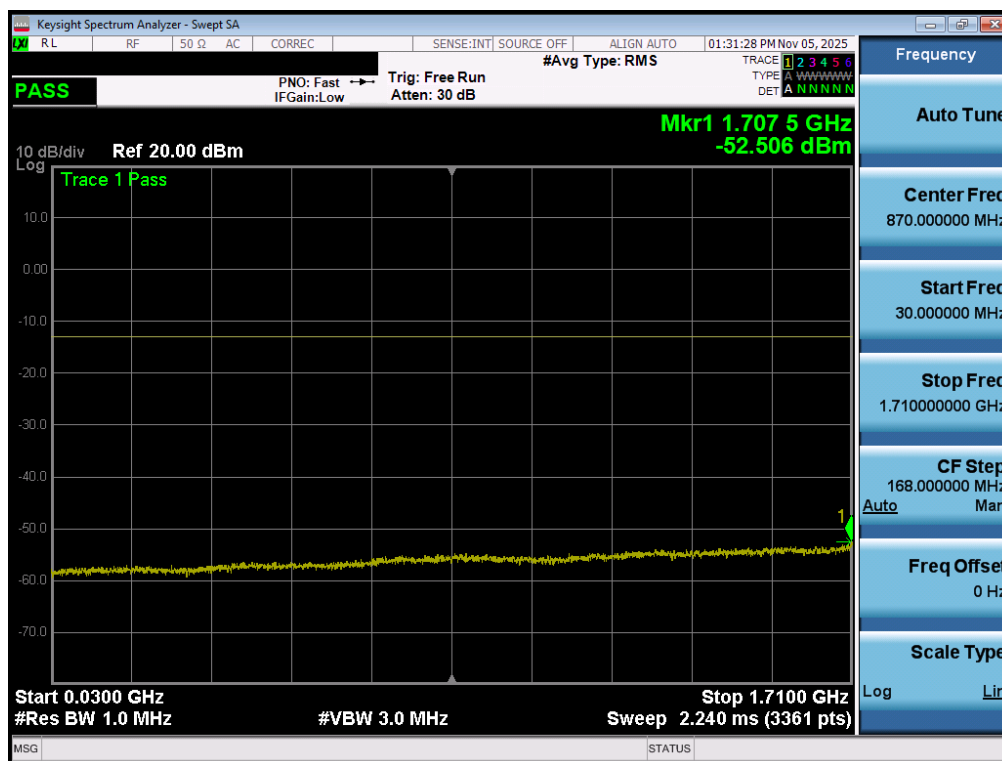
Plot 7-183. Conducted Spurious Plot (LTE Band 66/4 - 20MHz QPSK - 1 RB – Mid Channel)
