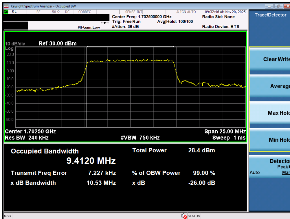
Plot 7-125. Occupied Bandwidth Plot (NR Band n70 - 10.0MHz CP-OFDM 16QAM - Full RB – ANT2)
