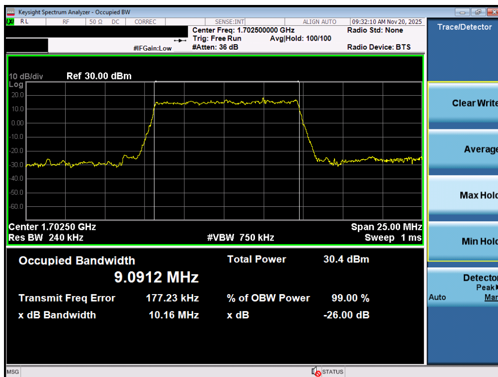
Plot 7-123. Occupied Bandwidth Plot (NR Band n70 - 10.0MHz DFT-s-OFDM BPSK - Full RB – ANT2)
