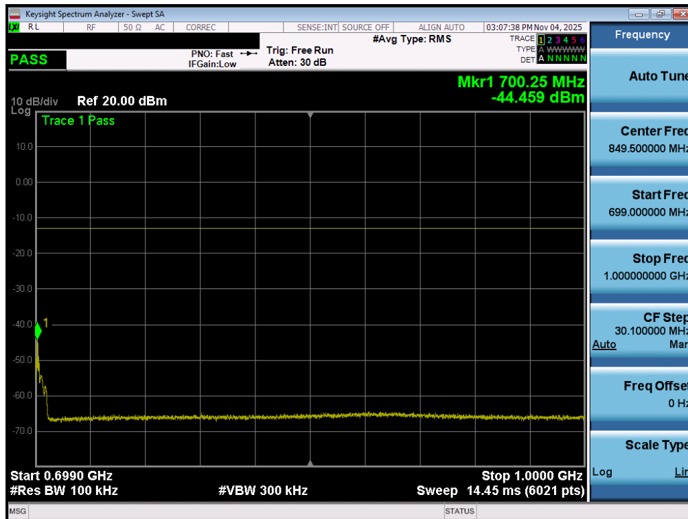
Plot 7-175. Conducted Spurious Plot (LTE Band 71 - 20MHz QPSK - 1 RB - High Channel - ANT2)
