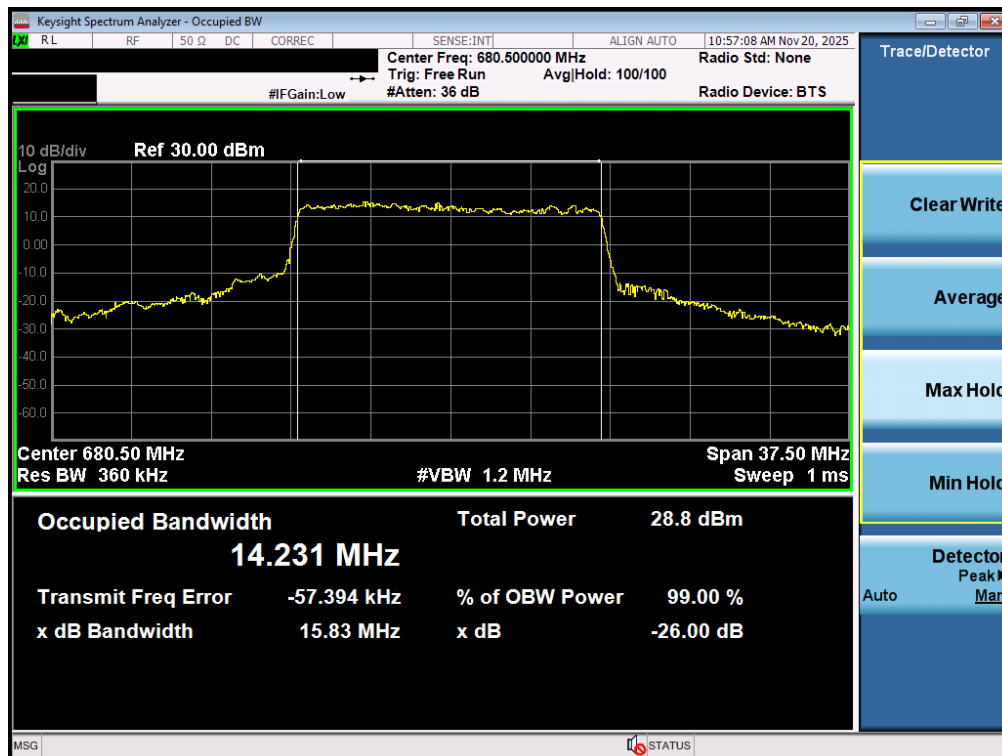
Plot 7-113. Occupied Bandwidth Plot (NR Band n71 - 15MHz CP-OFDM 16-QAM - Full RB – ANT2)
