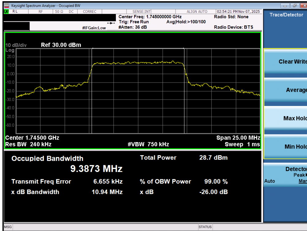
Plot 7-145. Occupied Bandwidth Plot (NR Band n66 - 10.0MHz CP-OFDM QPSK - Full RB – ANT2)
