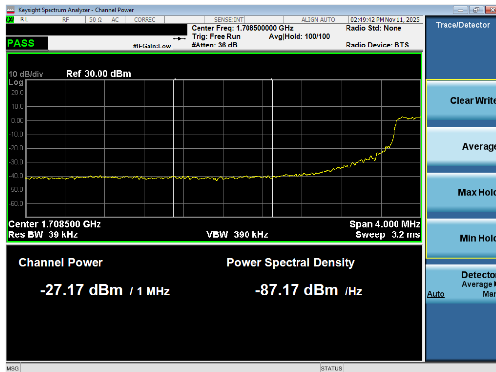
Plot 7-208. Lower Extended Band Edge Plot (LTE Band 66/4 – 5MHz QPSK – Full RB - ANT1)
