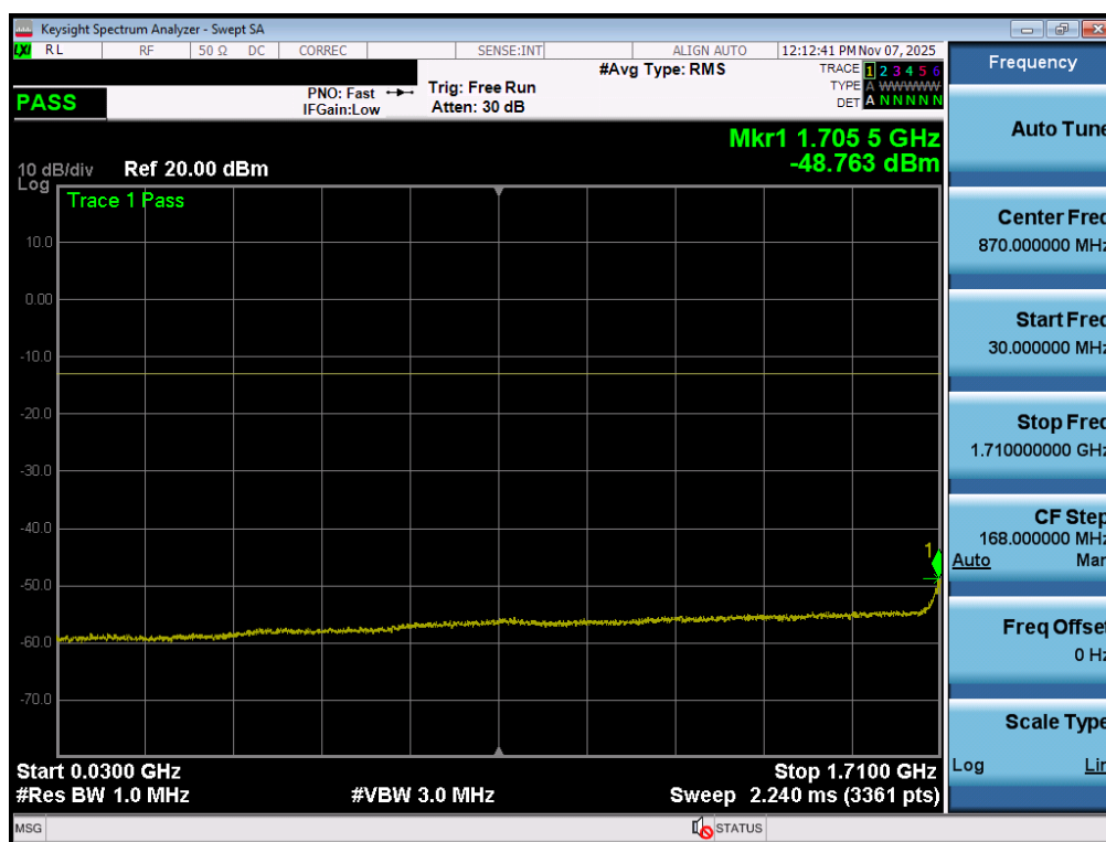
Plot 7-171. Conducted Spurious Plot (NR Band n66 - 40.0MHz - 1 RB - High Channel - ANT1)
