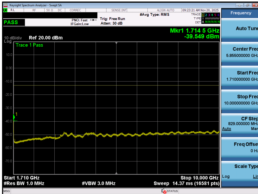
Plot 7-190. Conducted Spurious Plot (NR Band n70 - 15.0MHz - 1 RB - Mid Channel - ANT2)
