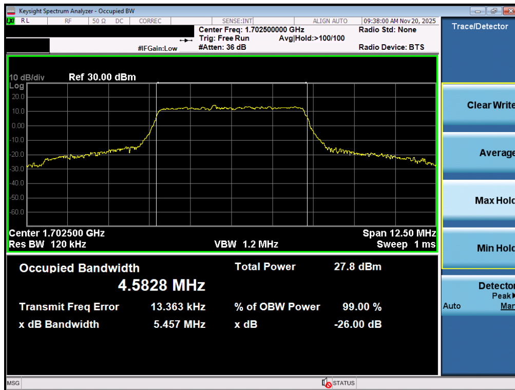
Plot 7-127. Occupied Bandwidth Plot (NR Band n70 - 5.0MHz CP-OFDM QPSK - Full RB – ANT2)
