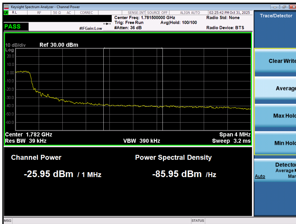
Plot 7-212. Upper Extended Band Edge Plot (LTE Band 66 – 5MHz QPSK – Full RB - ANT1)
