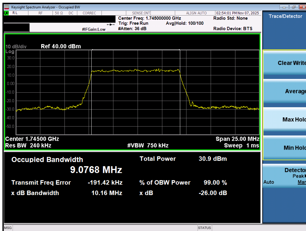
Plot 7-144. Occupied Bandwidth Plot (NR Band n66 - 10.0MHz DFT-s-OFDM BPSK - Full RB – ANT2)
