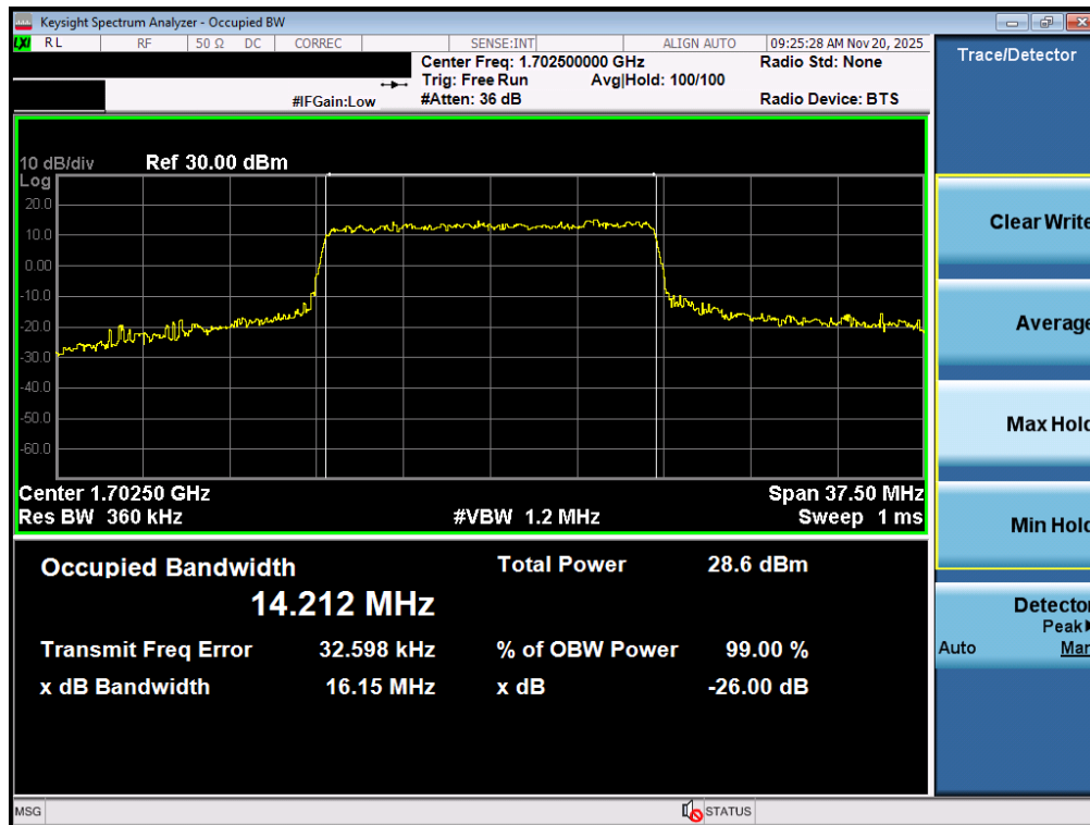
Plot 7-121. Occupied Bandwidth Plot (NR Band n70 - 15.0MHz CP-OFDM QPSK - Full RB – ANT2)
