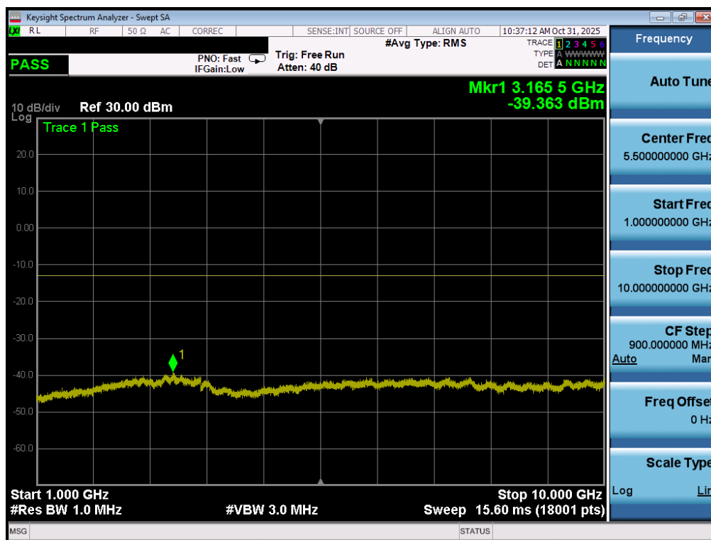
Plot 7-179. Conducted Spurious Plot (LTE Band 12 - 10MHz QPSK - 1 RB - Low Channel - ANT2)
