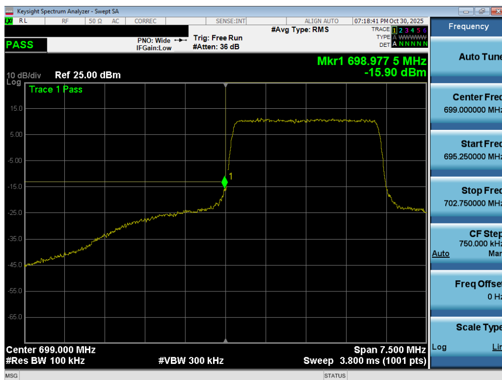
Plot 7-201. Lower Band Edge Plot (LTE Band 12 – 3MHz QPSK – Full RB - ANT1)
