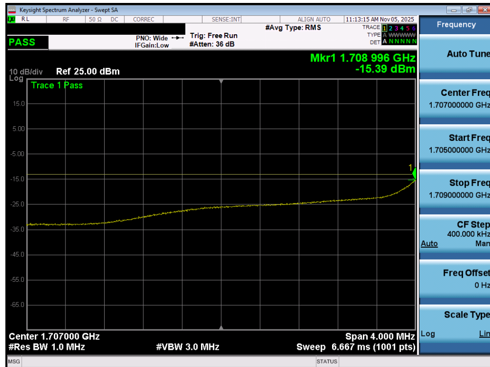
Plot 7-196. Lower Extended Band Edge Plot (WCDMA AWS – Ch. 1312 – ANT1)
