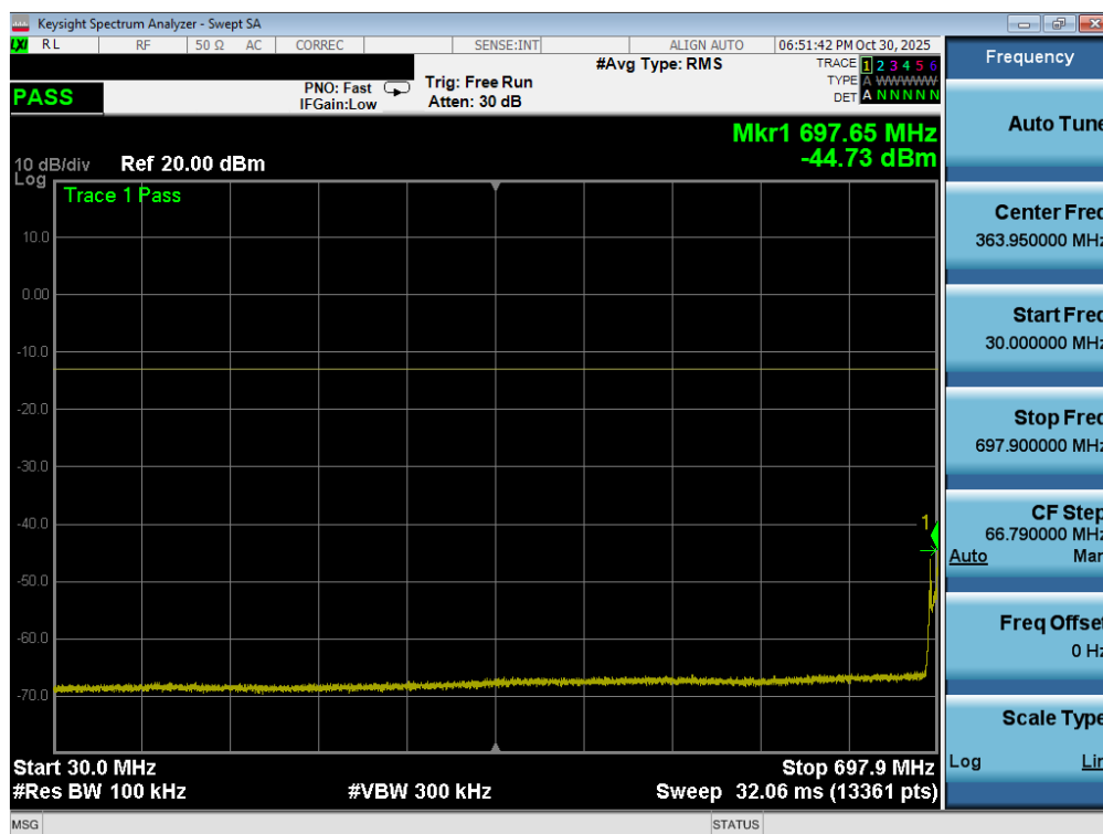
Plot 7-156. Conducted Spurious Plot (LTE Band 12 - 10MHz QPSK - 1 RB - Low Channel - ANT1)
