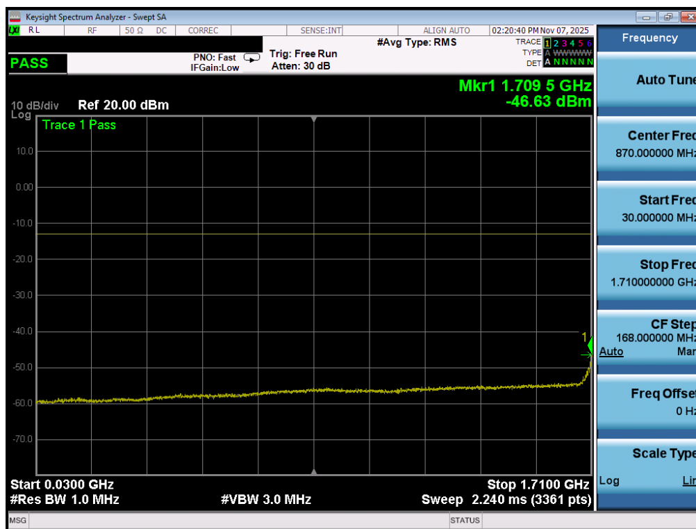
Plot 7-192. Conducted Spurious Plot (NR Band n66 - 40.0MHz - 1 RB - High Channel - ANT2)
