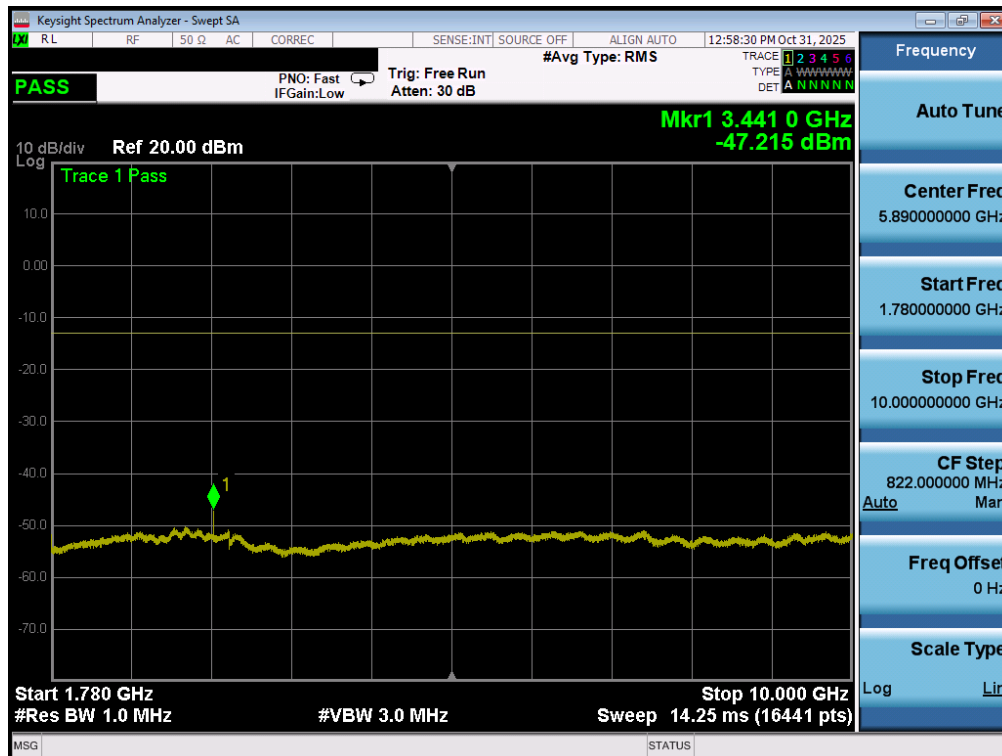
Plot 7-163. Conducted Spurious Plot (LTE Band 66/4 - 20MHz QPSK - 1 RB - Low Channel - ANT1)
