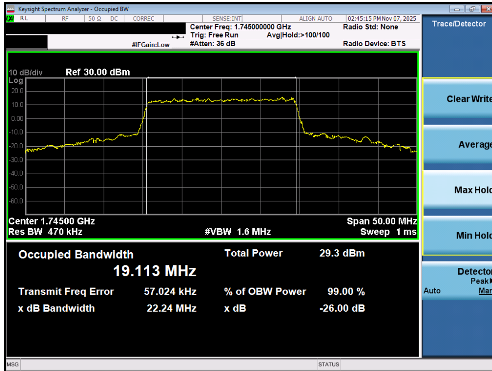
Plot 7-139. Occupied Bandwidth Plot (NR Band n66 - 20.0MHz CP-OFDM QPSK - Full RB – ANT2)
