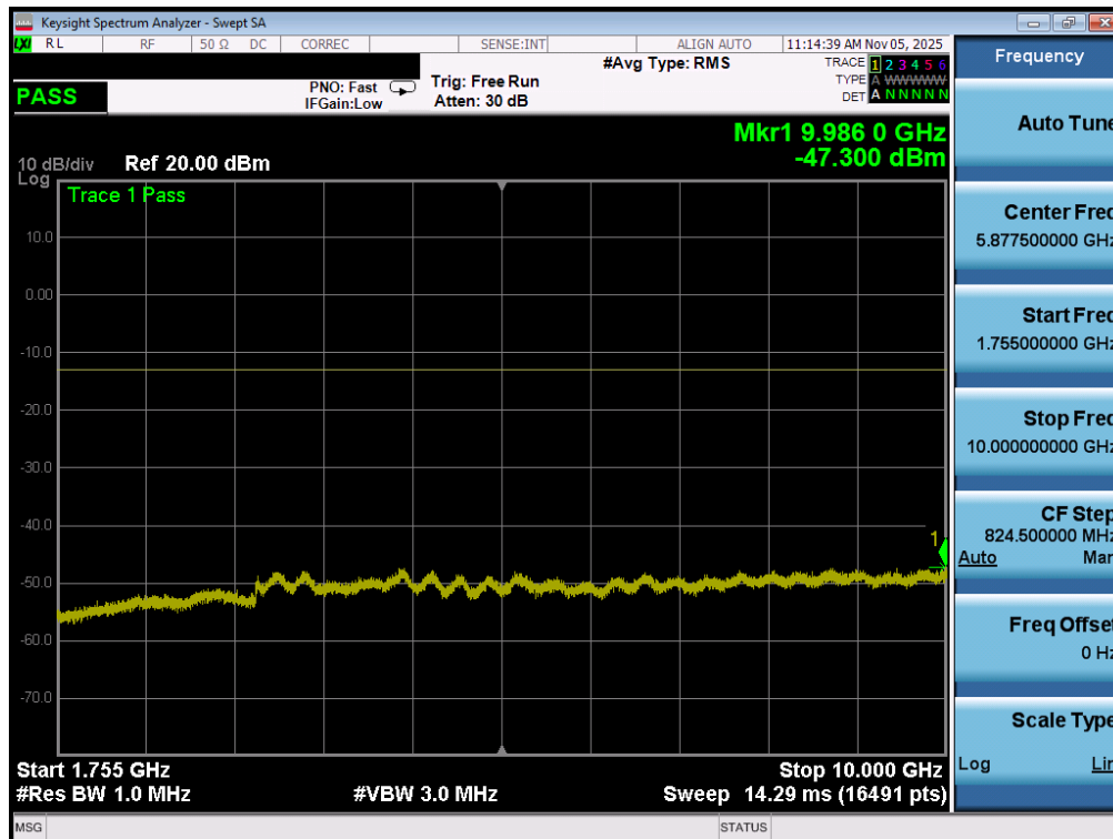
Plot 7-151. Conducted Spurious Plot (WCDMA-AWS - 5MHz QPSK - 1 RB – Low Channel)
