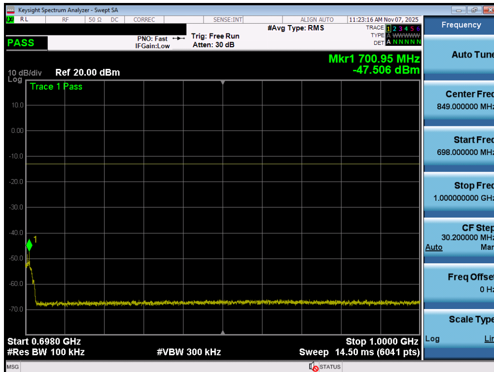
Plot 7-166. Conducted Spurious Plot (NR Band n71 - 20MHz - 1 RB - High Channel - ANT1)
