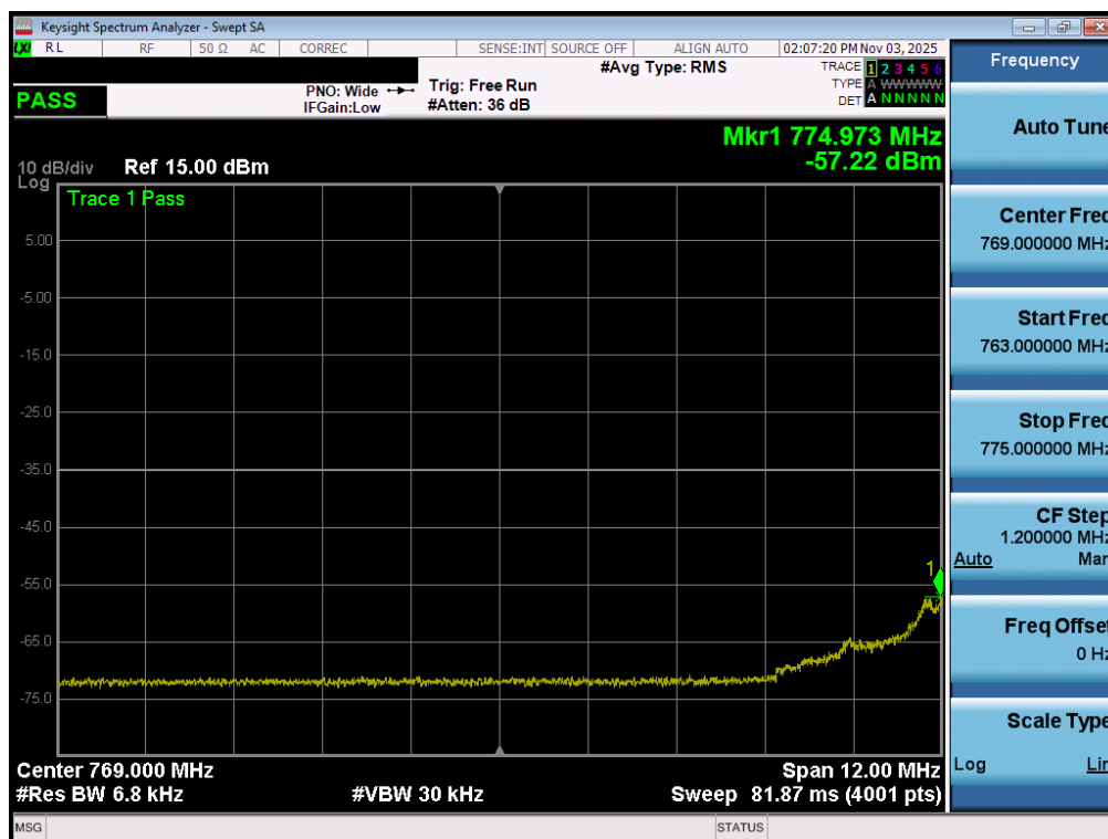
Plot 7-204. Lower Emission Mask Plot (LTE Band 13 - 5MHz QPSK – Full RB - ANT1)
