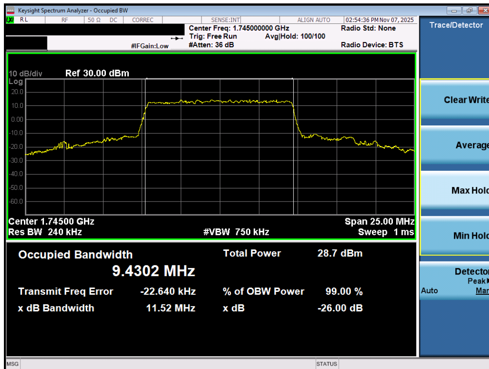
Plot 7-146. Occupied Bandwidth Plot (NR Band n66 - 10.0MHz CP-OFDM 16QAM - Full RB – ANT2)
