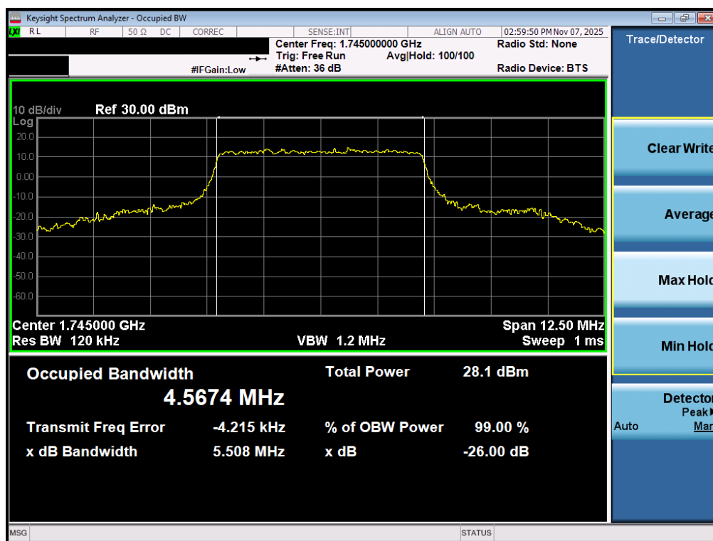
Plot 7-149. Occupied Bandwidth Plot (NR Band n66 - 5.0MHz CP-OFDM 16QAM - Full RB – ANT2)
