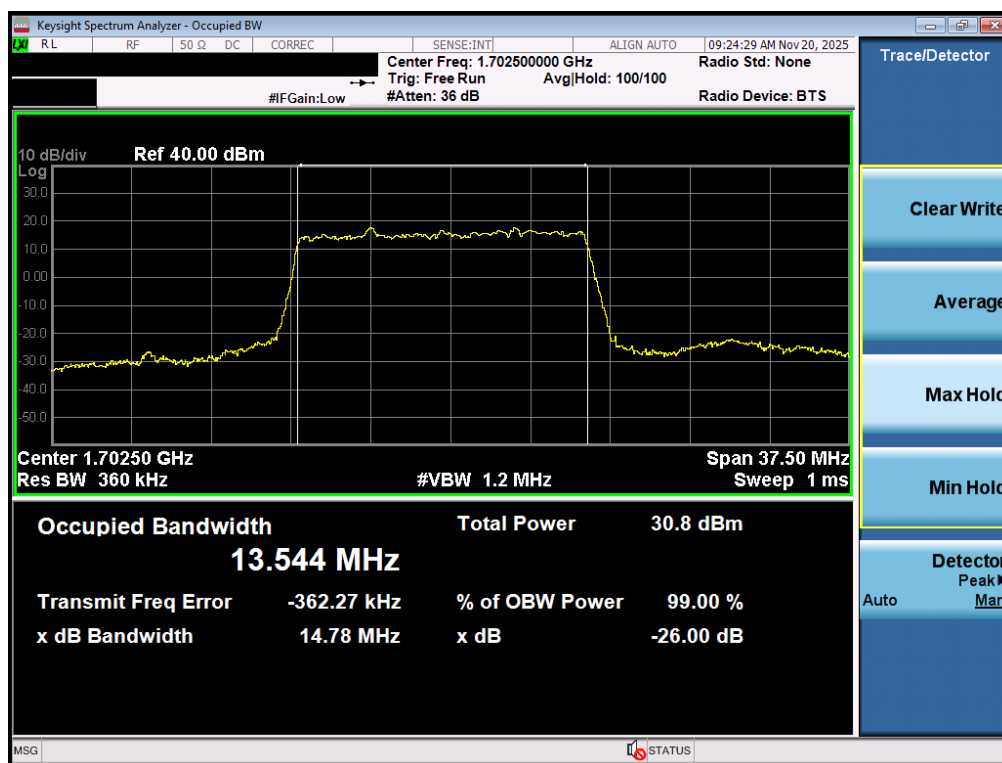
Plot 7-120. Occupied Bandwidth Plot (NR Band n70 - 15.0MHz DFT-s-OFDM BPSK - Full RB – ANT2)
