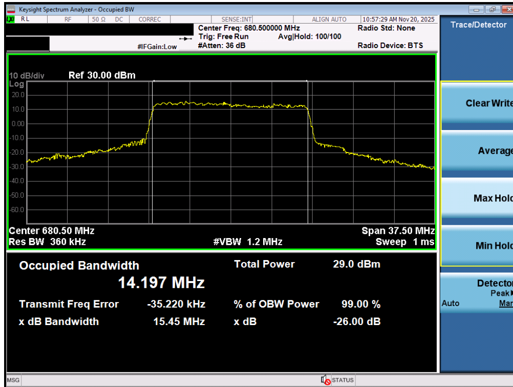
Plot 7-112. Occupied Bandwidth Plot (NR Band n71 - 15MHz QPSK - Full RB – ANT2)
