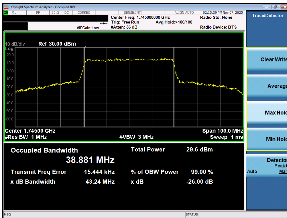
Plot 7-131. Occupied Bandwidth Plot (NR Band n66 - 40.0MHz CP-OFDM 16QAM - Full RB – ANT2)
