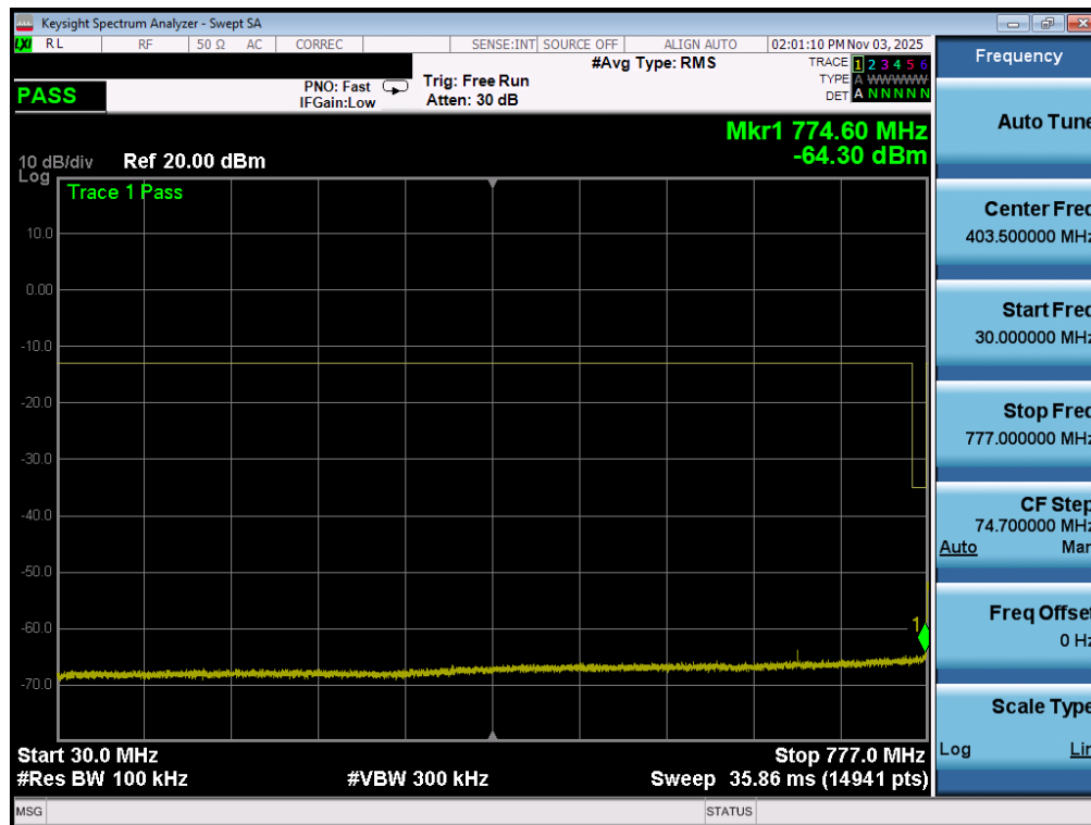
Plot 7-159. Conducted Spurious Plot (LTE Band 13 - 10MHz QPSK - 1 RB)
