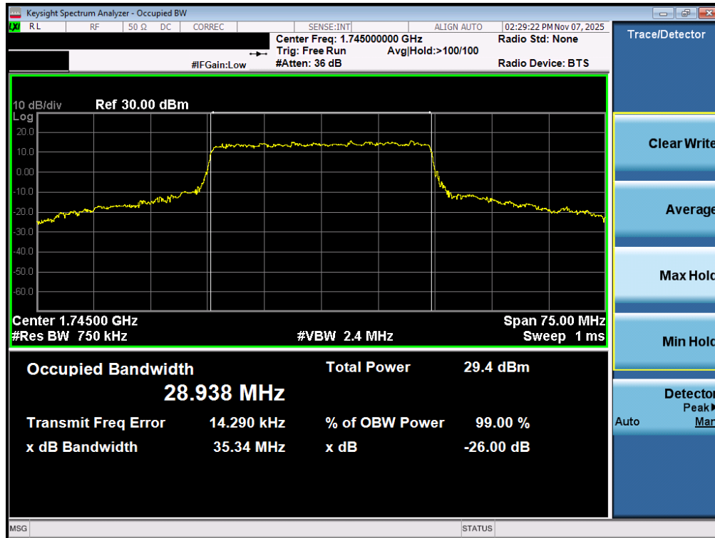
Plot 7-133. Occupied Bandwidth Plot (NR Band n66 - 30.0MHz CP-OFDM QPSK - Full RB – ANT2)
