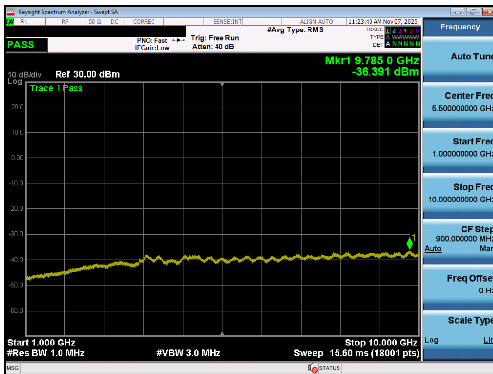
Plot 7-167. Conducted Spurious Plot (NR Band n71 - 20MHz - 1 RB - HighChannel - ANT1)
