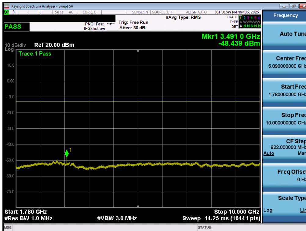
Plot 7-184. Conducted Spurious Plot (LTE Band 66/4 - 20MHz QPSK - 1 RB – Mid Channel)
