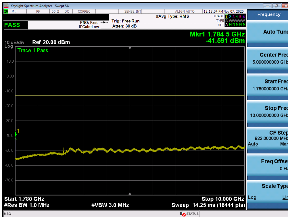
Plot 7-172. Conducted Spurious Plot (NR Band n66 - 40.0MHz - 1 RB - High Channel - ANT1)
