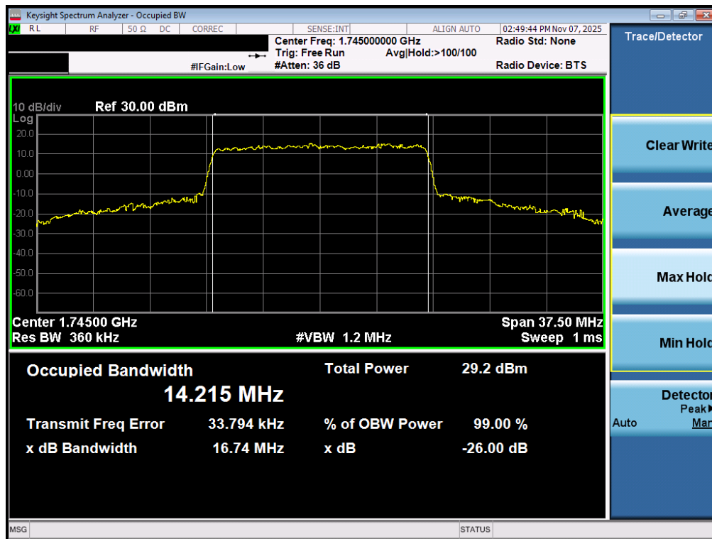
Plot 7-142. Occupied Bandwidth Plot (NR Band n66 - 15.0MHz CP-OFDM QPSK - Full RB – ANT2)
