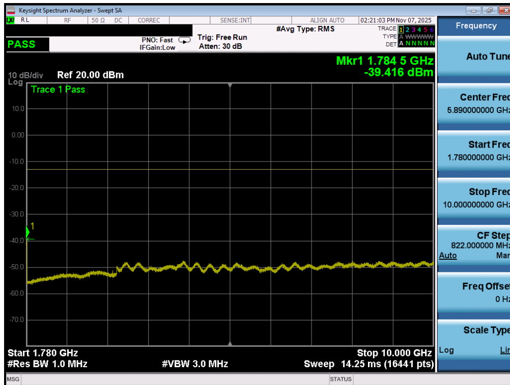
Plot 7-193. Conducted Spurious Plot (NR Band n66 - 40.0MHz - 1 RB - High Channel - ANT2)
