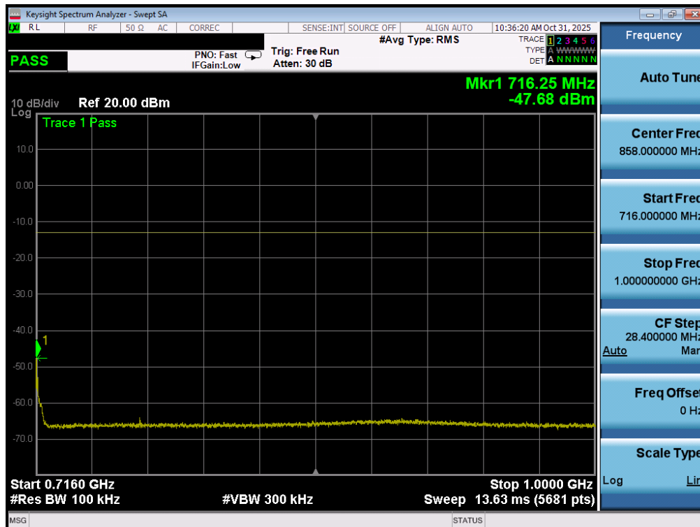
Plot 7-178. Conducted Spurious Plot (LTE Band 12 - 10MHz QPSK - 1 RB - Low Channel - ANT2)
