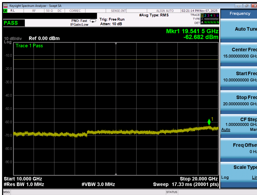
Plot 7-194. Conducted Spurious Plot (NR Band n66 - 40.0MHz - 1 RB - High Channel - ANT2)
