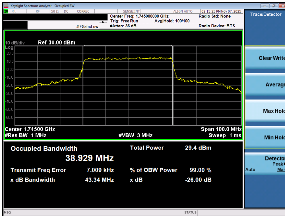
Plot 7-130. Occupied Bandwidth Plot (NR Band n66 - 40.0MHz CP-OFDM QPSK - Full RB – ANT2)
