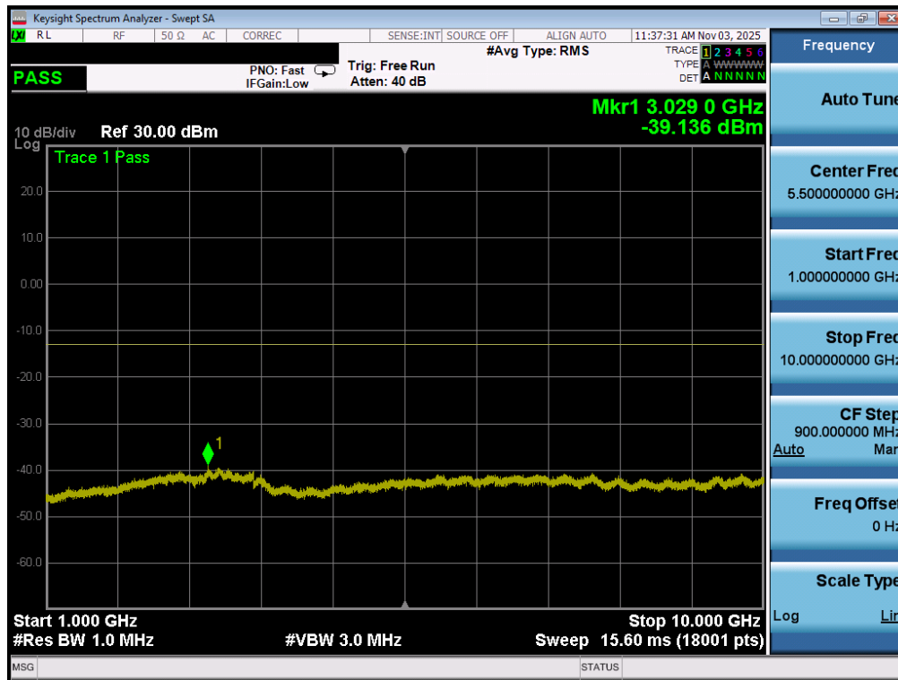
Plot 7-155. Conducted Spurious Plot (LTE Band 71 - 20MHz QPSK - 1 RB - Mid Channel - ANT1)
