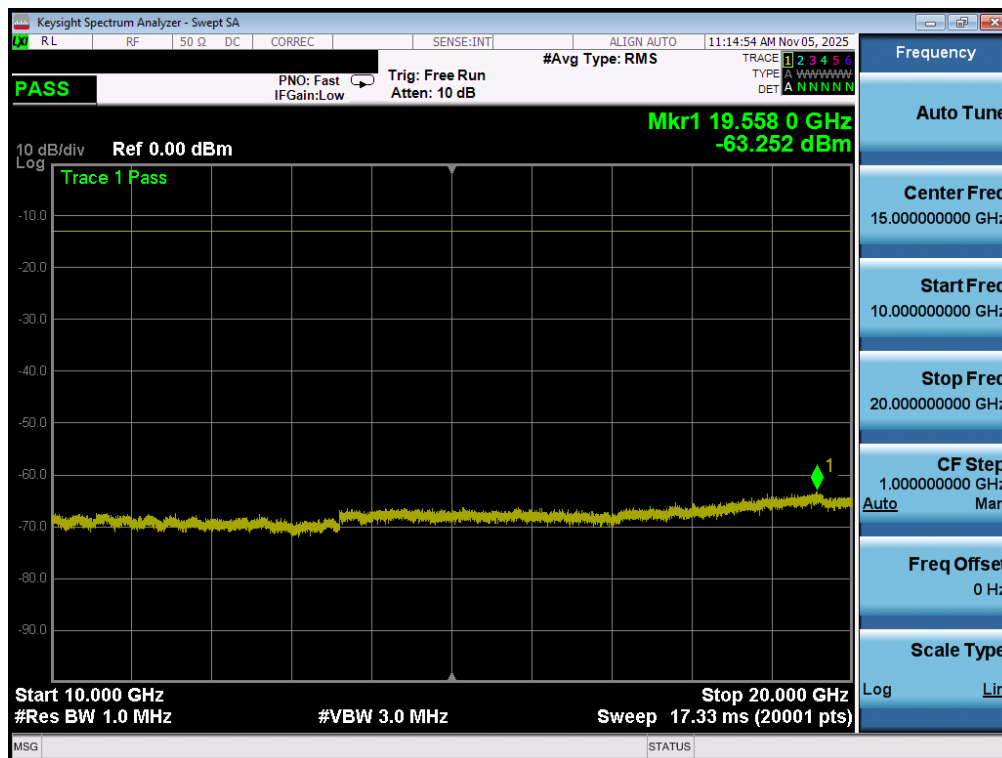
Plot 7-152. Conducted Spurious Plot (WCDMA-AWS - 5MHz QPSK - 1 RB – Low Channel)
