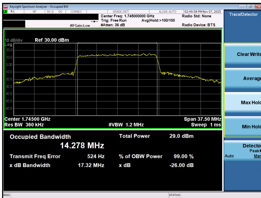
Plot 7-143. Occupied Bandwidth Plot (NR Band n66 - 15.0MHz CP-OFDM 16QAM - Full RB – ANT2)
