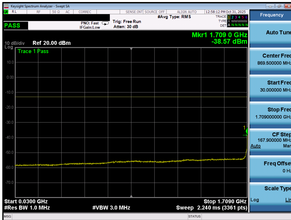
Plot 7-162. Conducted Spurious Plot (LTE Band 66/4 - 20MHz QPSK - 1 RB - Low Channel - ANT1)
