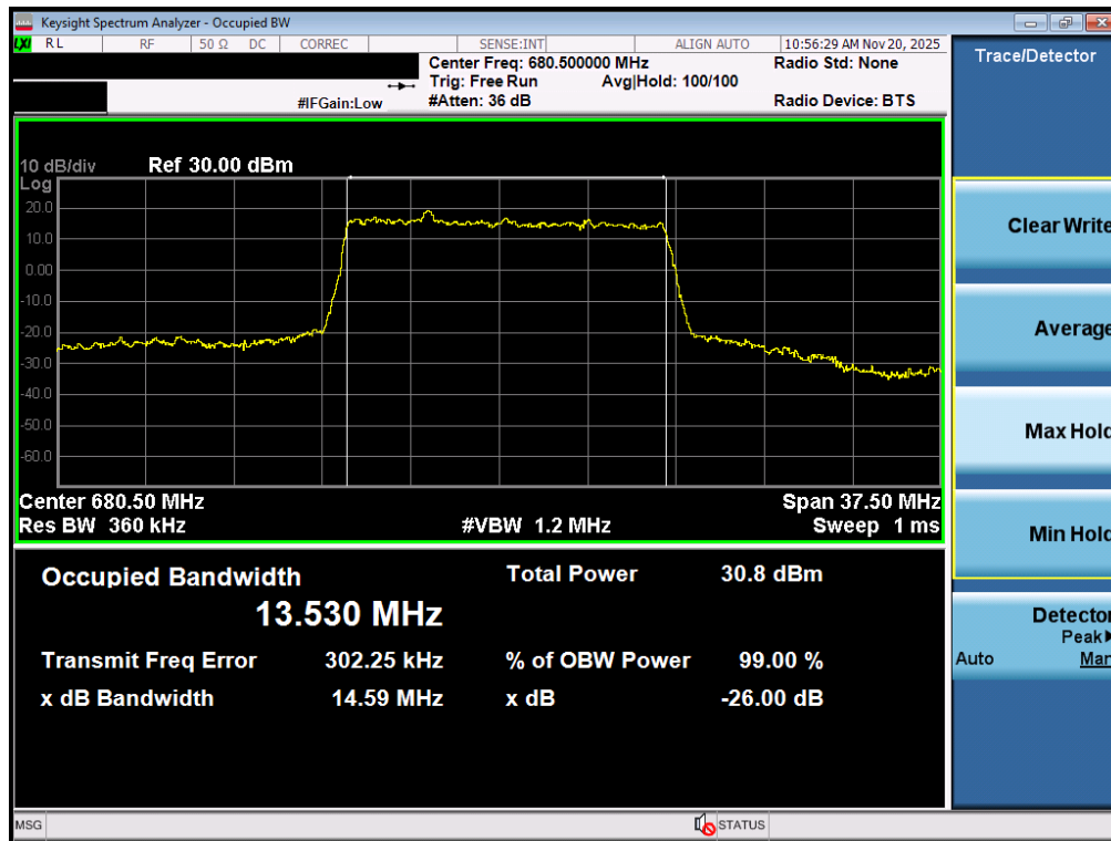
Plot 7-111. Occupied Bandwidth Plot (NR Band n71 - 15MHz DFT-s-OFDM BPSK - Full RB – ANT2)
