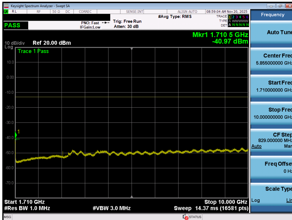
Plot 7-169. Conducted Spurious Plot (NR Band n70 - 15.0MHz - 1 RB - Mid Channel - ANT1)
