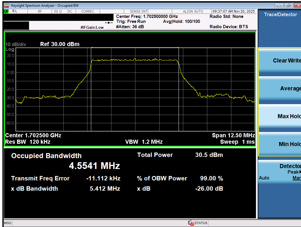
Plot 7-126. Occupied Bandwidth Plot (NR Band n70 - 5.0MHz DFT-s-OFDM BPSK - Full RB – ANT2)
