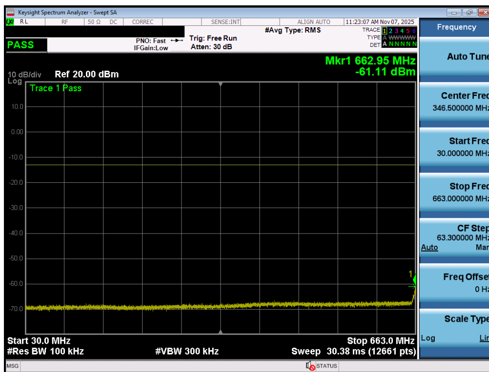
Plot 7-165. Conducted Spurious Plot (NR Band n71 - 20MHz - 1 RB - High Channel - ANT1)
