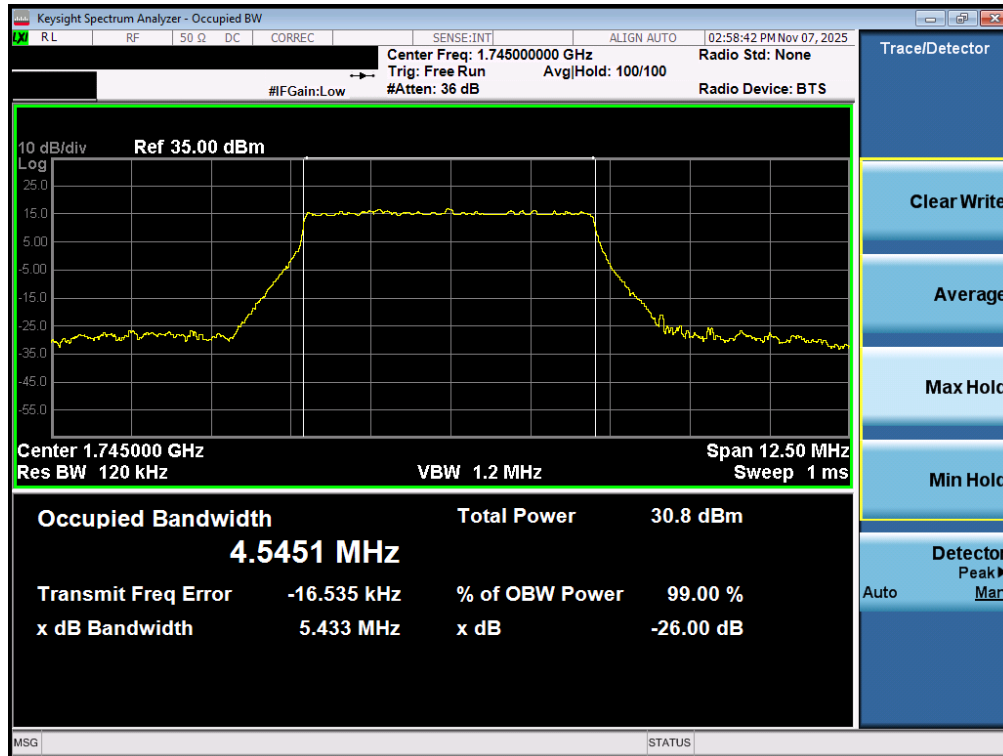
Plot 7-147. Occupied Bandwidth Plot (NR Band n66 - 5.0MHz DFT-s-OFDM BPSK - Full RB – ANT2)
