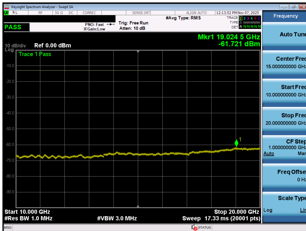
Plot 7-173. Conducted Spurious Plot (NR Band n66 - 40.0MHz - 1 RB - High Channel - ANT1)
