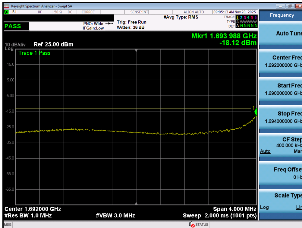
Plot 7-216. Lower Extended Band Edge Plot (NR Band n70 – 10.0MHz - Full RB - ANT1)
