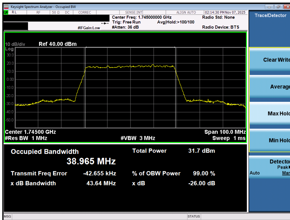
Plot 7-129. Occupied Bandwidth Plot (NR Band n66 - 40.0MHz DFT-s-OFDM BPSK - Full RB – ANT2)
