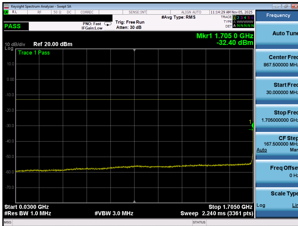
Plot 7-150. Conducted Spurious Plot (WCDMA-AWS - 5MHz QPSK - 1 RB – Low Channel)
