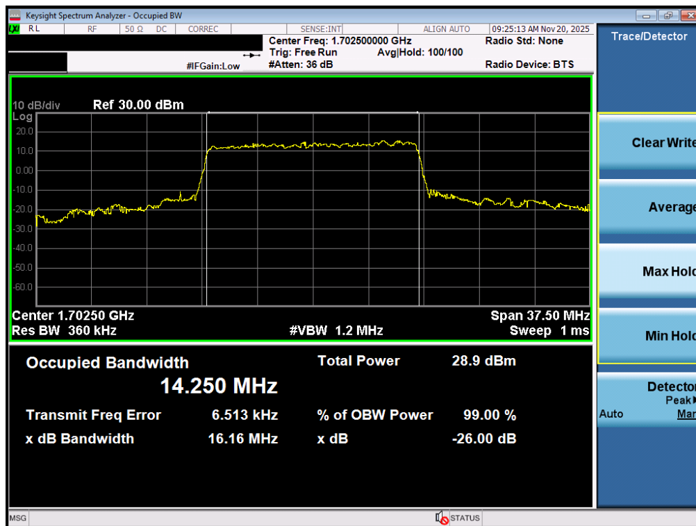
Plot 7-122. Occupied Bandwidth Plot (NR Band n70 - 15.0MHz CP-OFDM 16QAM - Full RB – ANT2)
