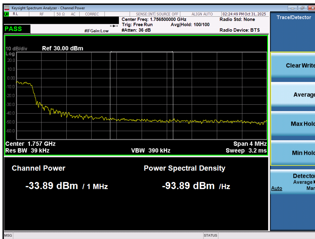
Plot 7-210. Upper Extended Band Edge Plot (LTE Band 4 – 5MHz QPSK – Full RB - ANT1)
