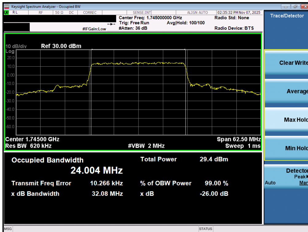
Plot 7-136. Occupied Bandwidth Plot (NR Band n66 - 25.0MHz CP-OFDM QPSK - Full RB – ANT2)
