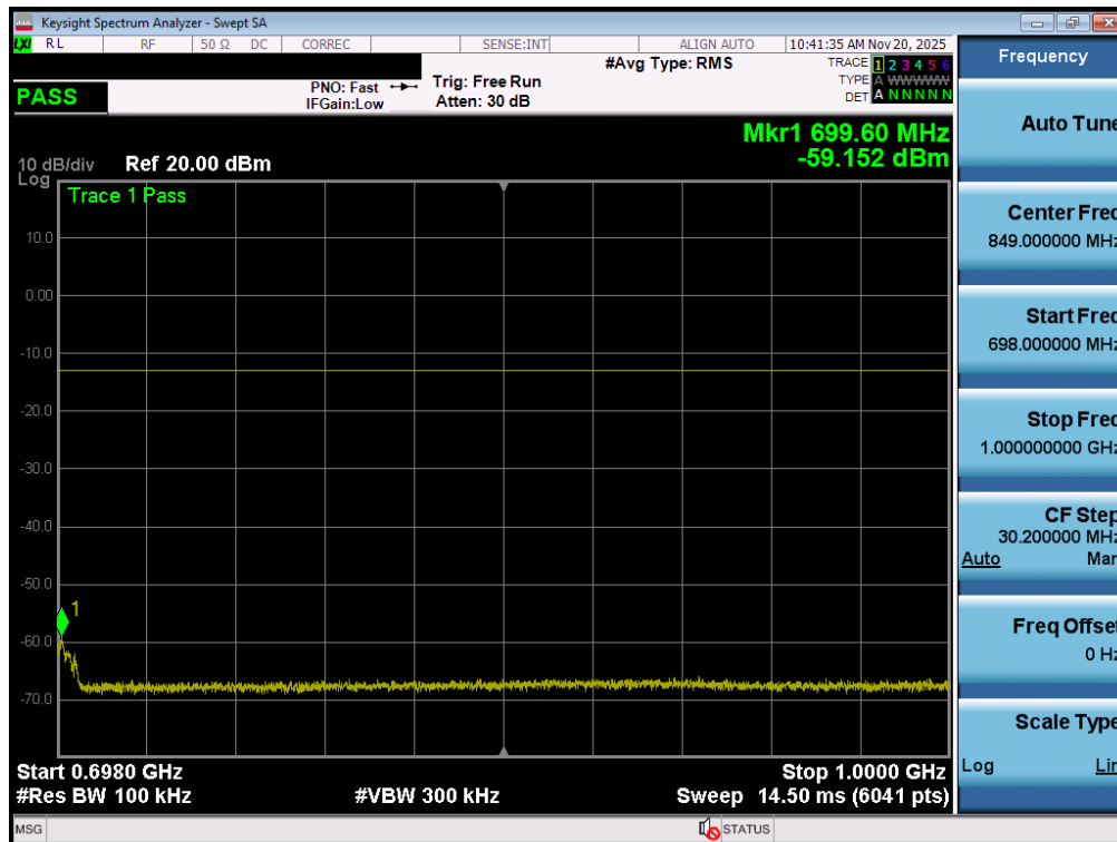
Plot 7-187. Conducted Spurious Plot (NR Band n71 - 20MHz - 1 RB - Low Channel - ANT2)
