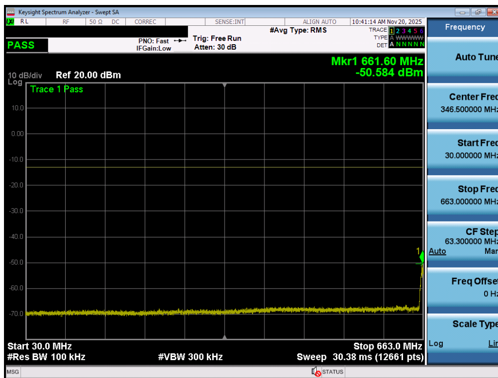
Plot 7-186. Conducted Spurious Plot (NR Band n71 - 20MHz - 1 RB - Low Channel - ANT2)
