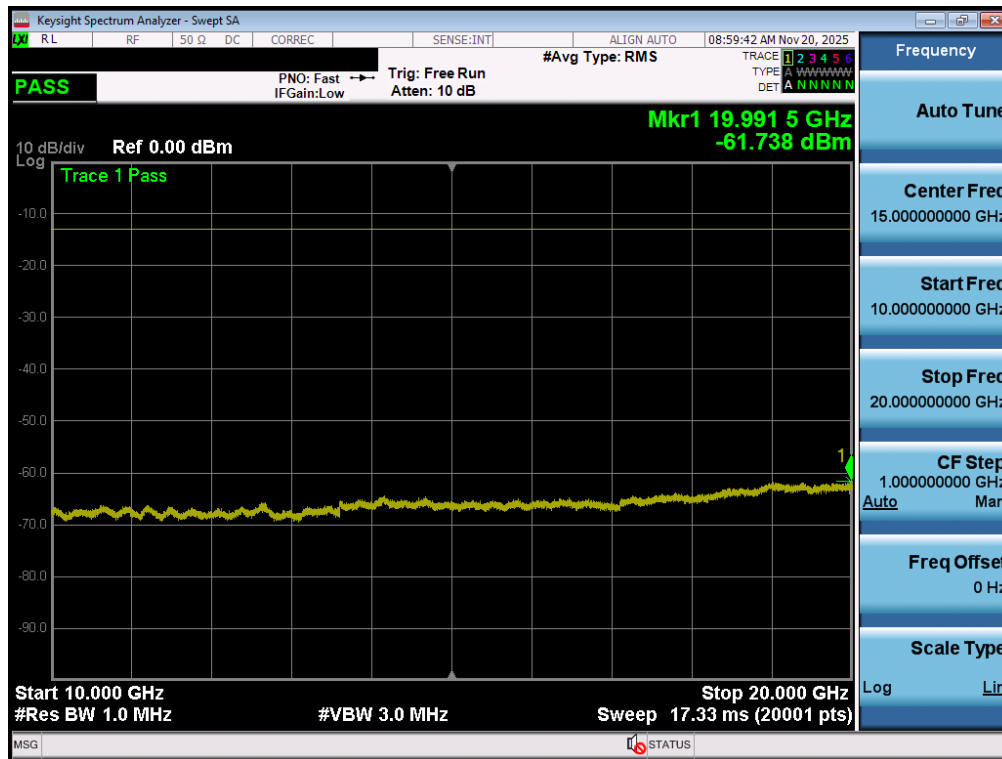
Plot 7-170. Conducted Spurious Plot (NR Band n70 - 15.0MHz - 1 RB - Mid Channel - ANT1)
