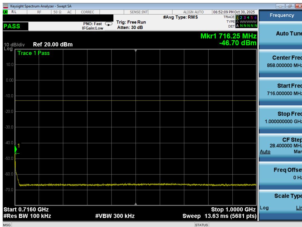
Plot 7-157. Conducted Spurious Plot (LTE Band 12 - 10MHz QPSK - 1 RB - Low Channel - ANT1)
