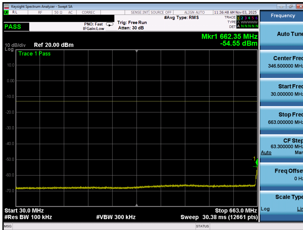
Plot 7-153. Conducted Spurious Plot (LTE Band 71 - 20MHz QPSK - 1 RB - Mid Channel - ANT1)
