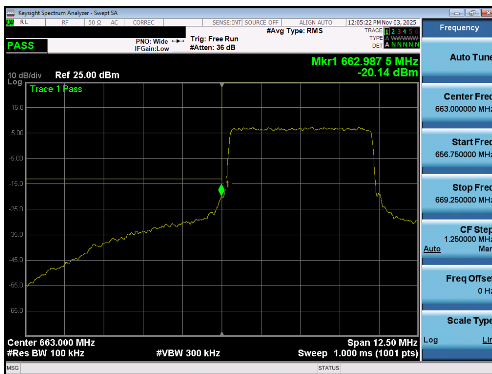
Plot 7-199. Lower Band Edge Plot (LTE Band 71 - 5MHz QPSK – Full RB - ANT1)
