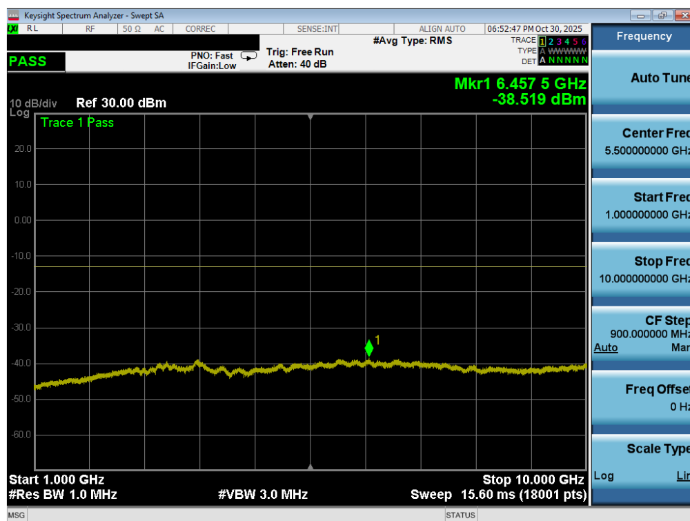
Plot 7-158. Conducted Spurious Plot (LTE Band 12 - 10MHz QPSK - 1 RB - Low Channel - ANT1)
