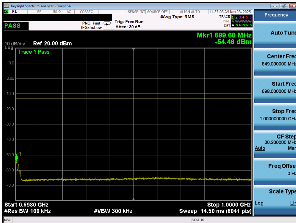
Plot 7-154. Conducted Spurious Plot (LTE Band 71 - 20MHz QPSK - 1 RB - Mid Channel - ANT1)
