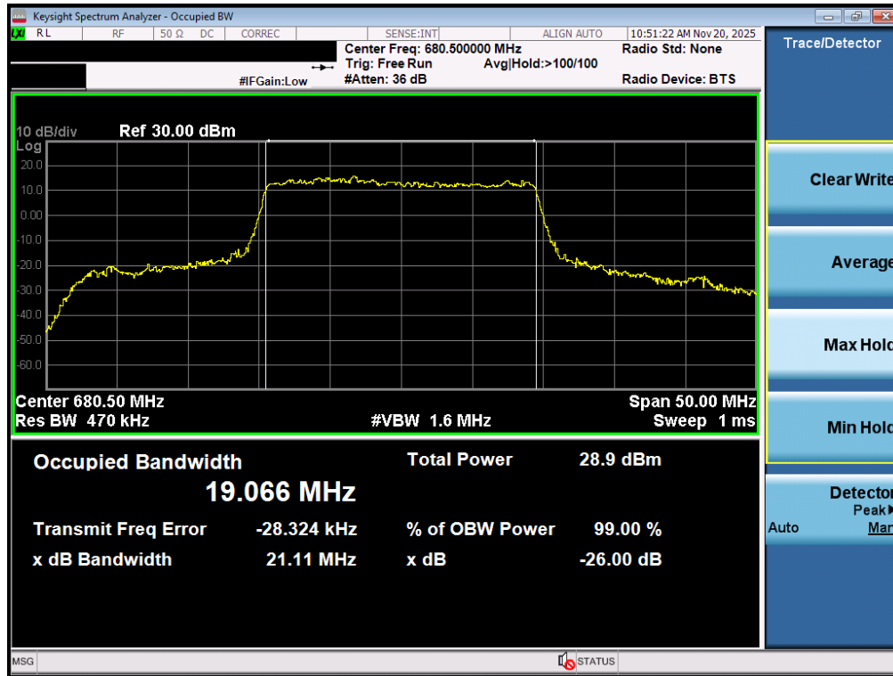
Plot 7-110. Occupied Bandwidth Plot (NR Band n71 - 20MHz CP-OFDM 16-QAM - Full RB – ANT2)
