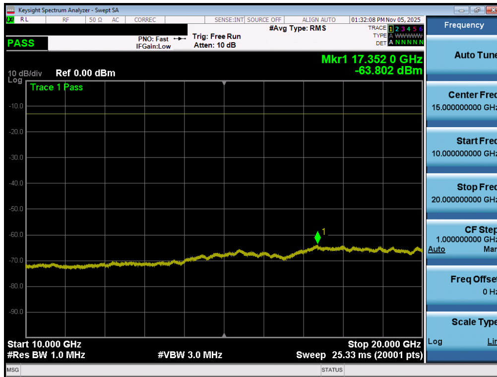
Plot 7-185. Conducted Spurious Plot (LTE Band 66/4 - 20MHz QPSK - 1 RB – High Channel)
