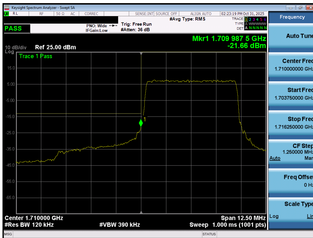
Plot 7-207. Lower Band Edge Plot (LTE Band 66/4 – 5MHz QPSK – Full RB - ANT1)
