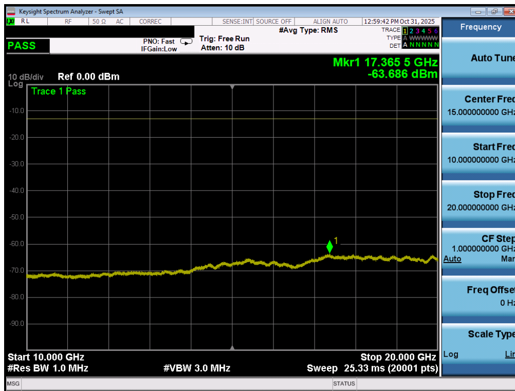
Plot 7-164. Conducted Spurious Plot (LTE Band 66/4 - 20MHz QPSK - 1 RB - Low Channel - ANT1)
