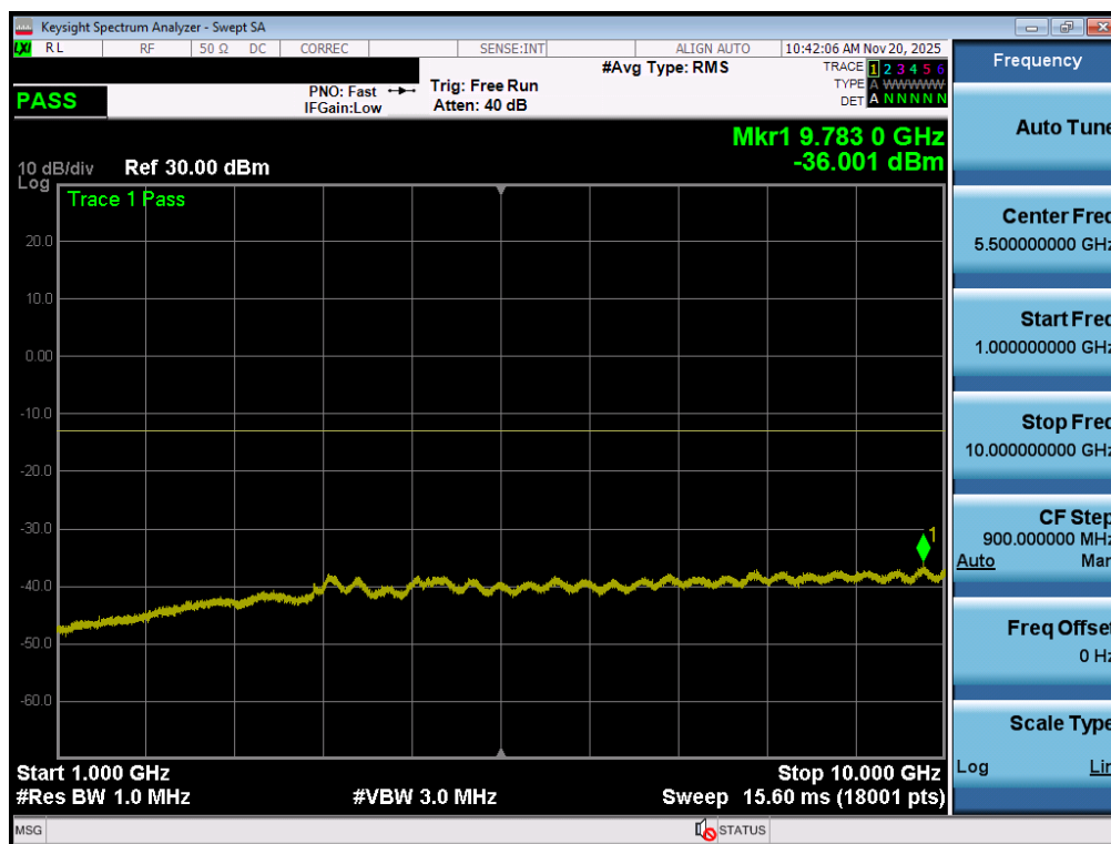
Plot 7-188. Conducted Spurious Plot (NR Band n71 - 20MHz - 1 RB - Low Channel - ANT2)
