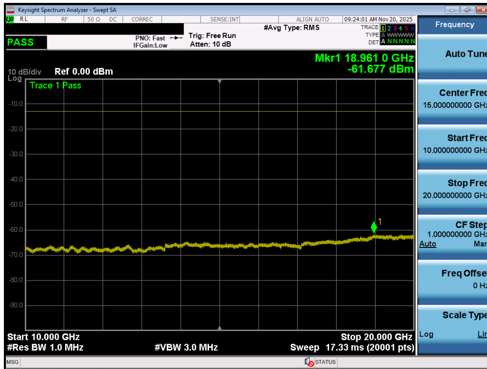
Plot 7-191. Conducted Spurious Plot (NR Band n70 - 15.0MHz - 1 RB - Mid Channel - ANT2)
