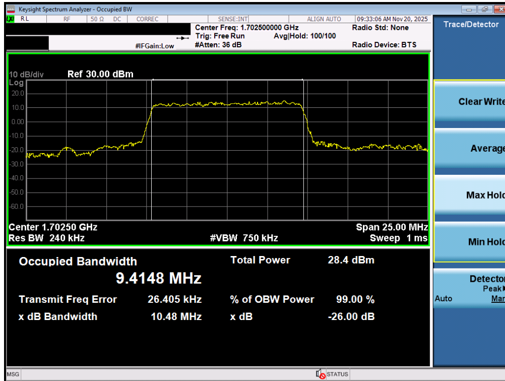
Plot 7-124. Occupied Bandwidth Plot (NR Band n70 - 10.0MHz CP-OFDM QPSK - Full RB – ANT2)
