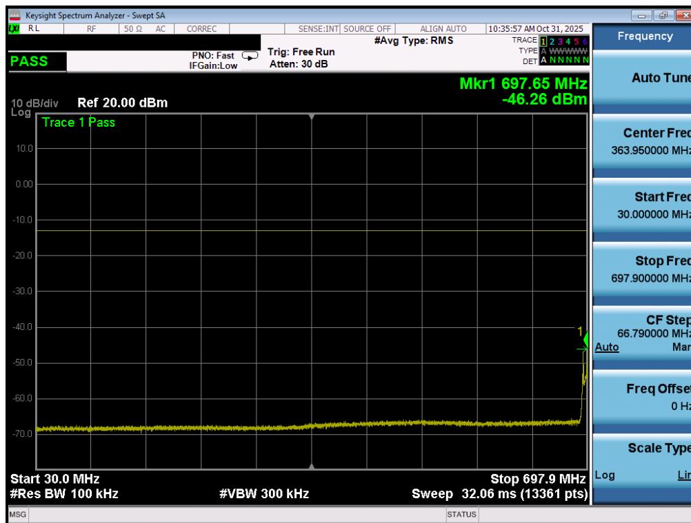
Plot 7-177. Conducted Spurious Plot (LTE Band 12 - 10MHz QPSK - 1 RB - Low Channel - ANT2)
