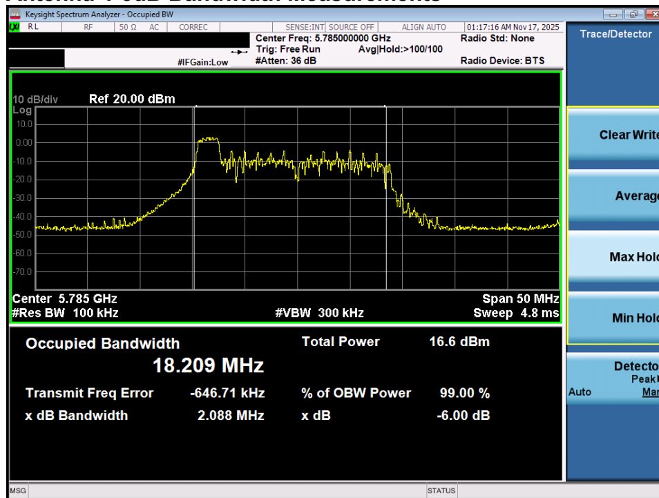
Plot 7-13. 6dB Bandwidth Plot MIMO ANT1 (20MHz BW 802.11ax – 26 Tones (UNII Band 3) – Ch. 157)
