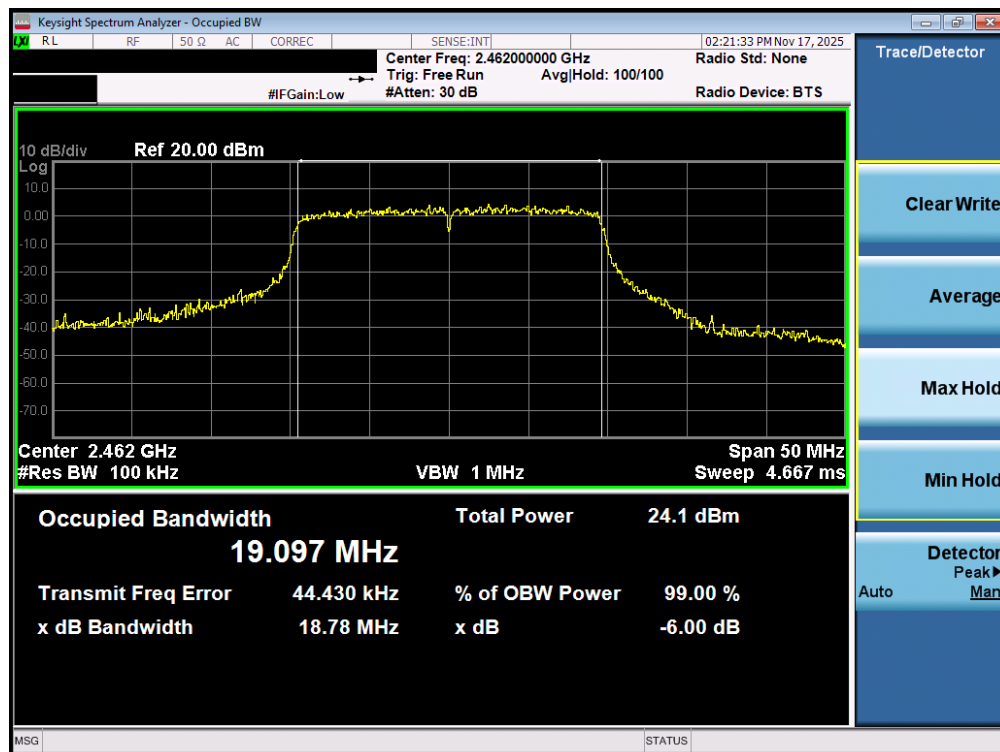
Plot 7-12. 6dB Bandwidth Plot MIMO ANT1 (802.11ax (2.4GHz) – Ch. 11)
