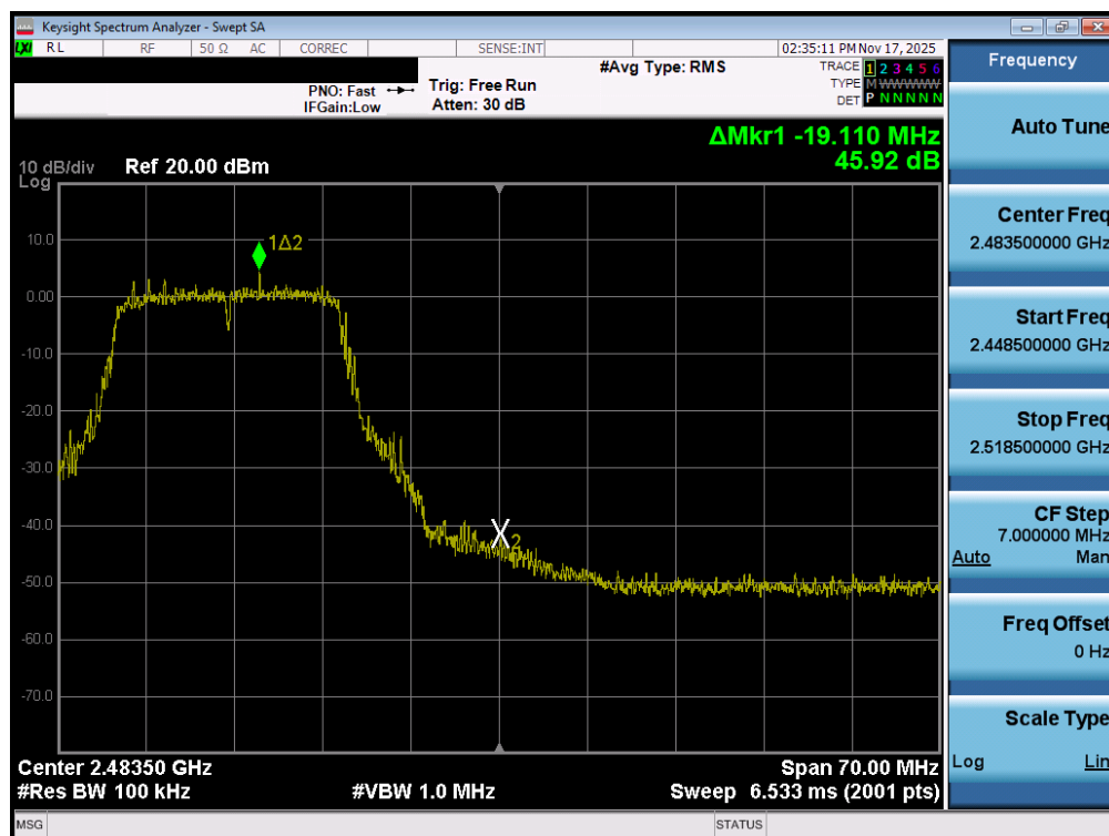
Plot 7-80. Band Edge Plot MIMO ANT1 (802.11n(2.4GHz) – Ch. 11)
