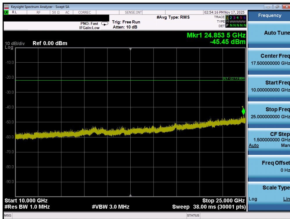
Plot 7-96. Conducted Spurious Plot MIMO ANT1 (802.11b – Ch. 1)
