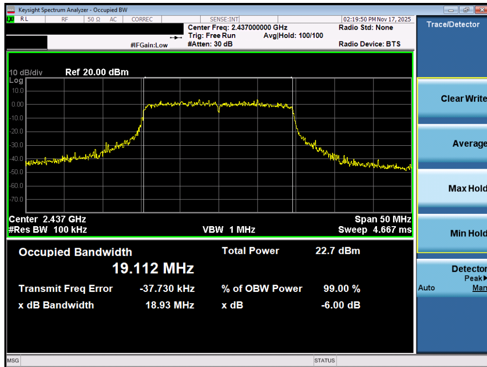
Plot 7-11. 6dB Bandwidth Plot MIMO ANT1 (802.11ax (2.4GHz) – Ch. 6)
