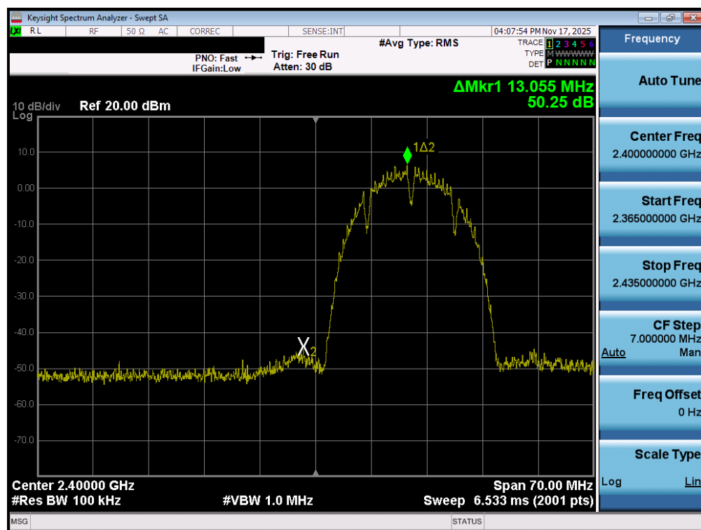
Plot 7-84. Band Edge Plot MIMO ANT2 (802.11b – Ch. 1)
