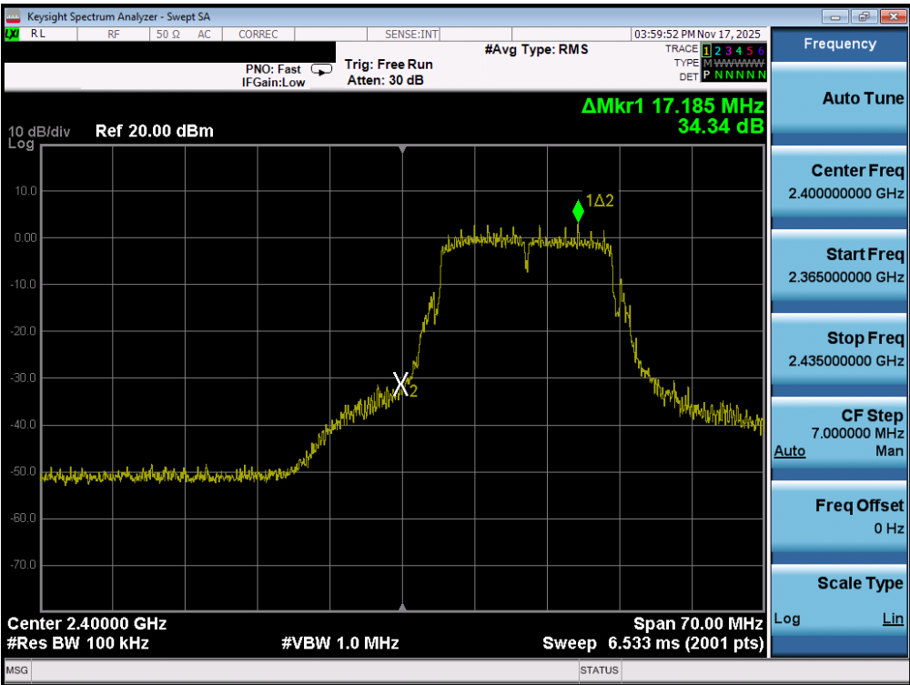
Plot 7-86. Band Edge Plot MIMO ANT2 (802.11g- Ch. 1)
