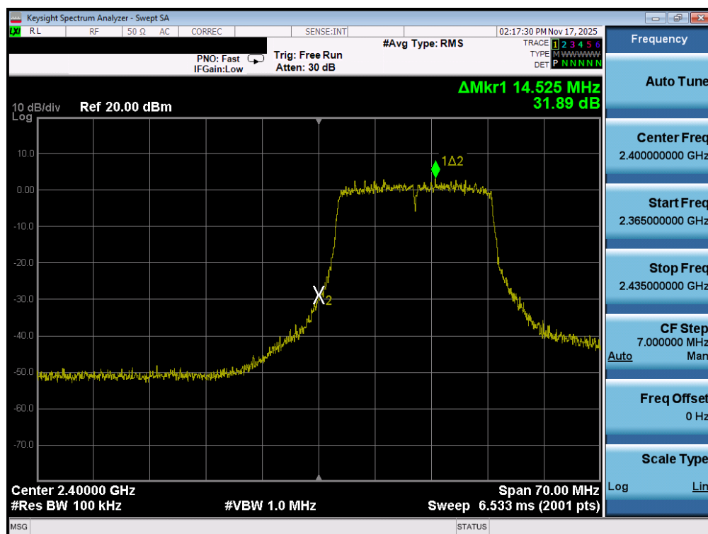
Plot 7-81. Band Edge Plot MIMO ANT1 (802.11ax (2.4GHz) – Ch. 1)
