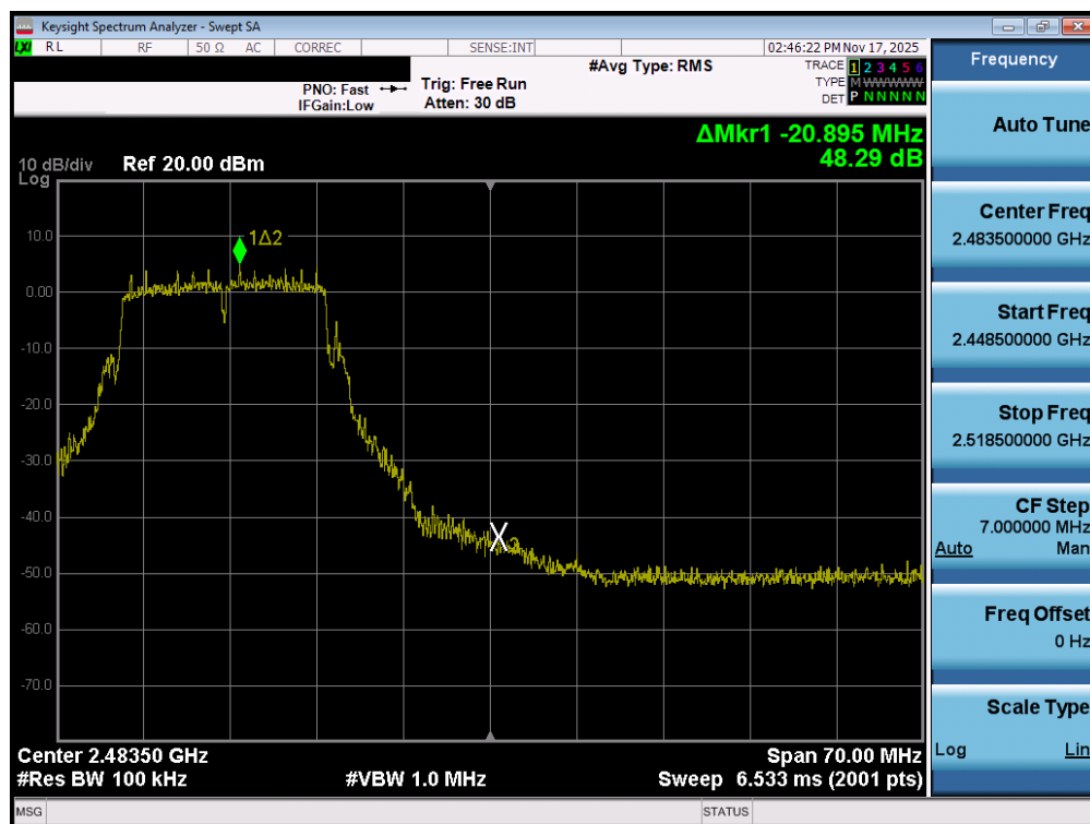
Plot 7-77. Band Edge Plot MIMO ANT1 (802.11g – Ch. 11)
