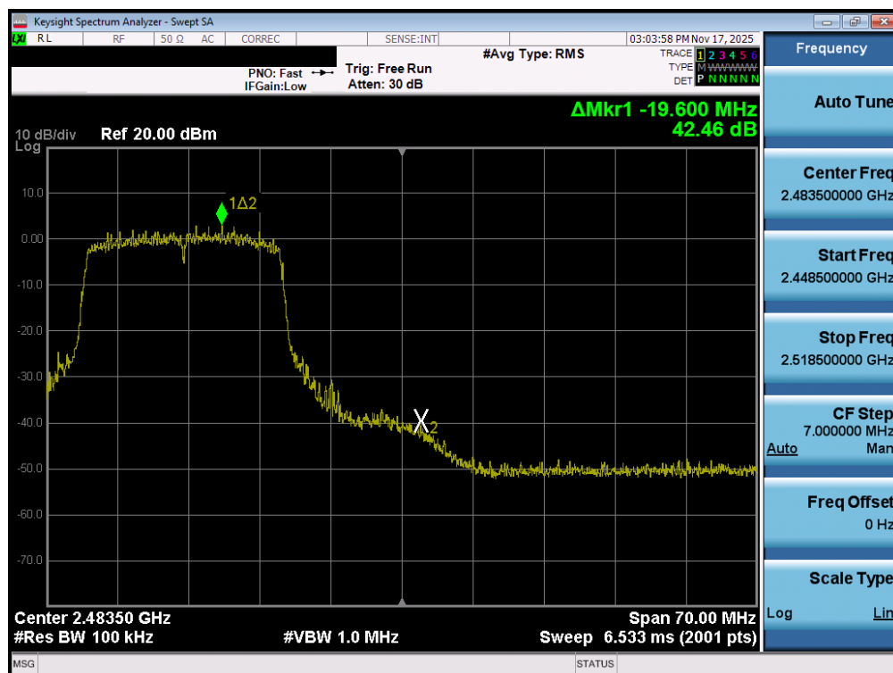
Plot 7-94. Band Edge Plot MIMO ANT2 (802.11ax (2.4GHz) – Ch. 11)
