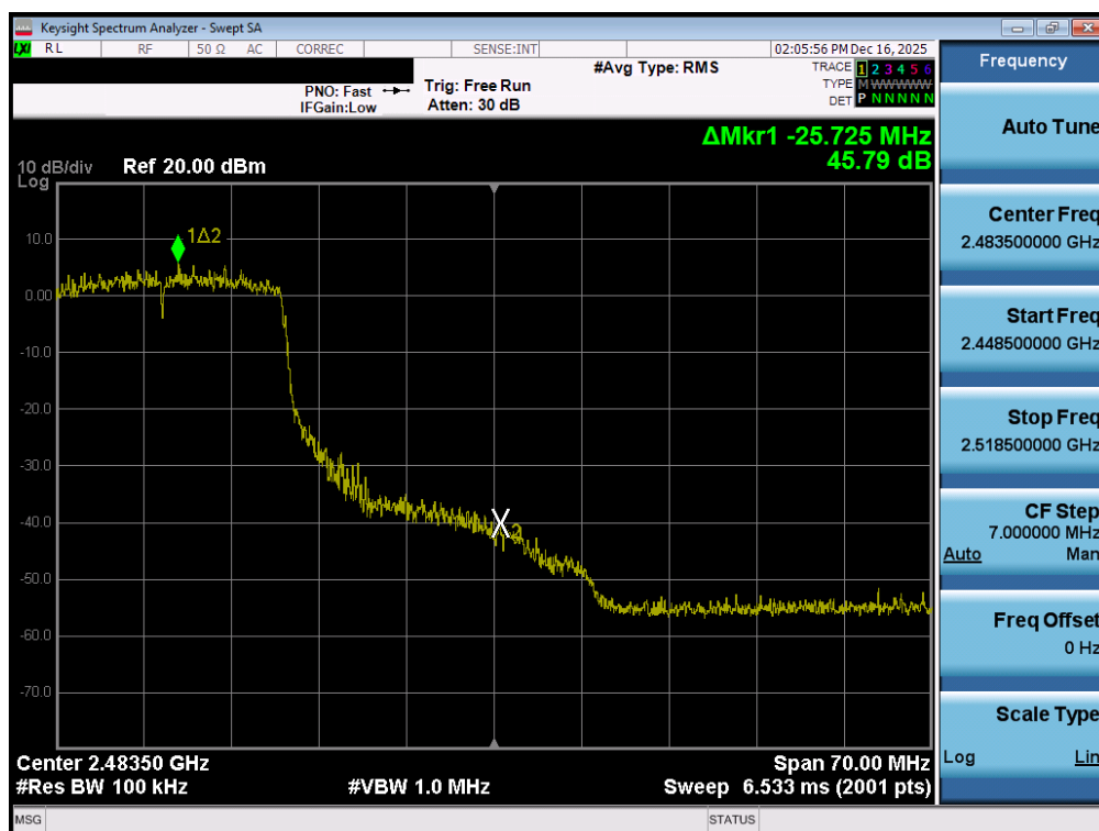
Plot 7-82. Band Edge Plot MIMO ANT1 (802.11ax (2.4GHz) – Ch. 10)
