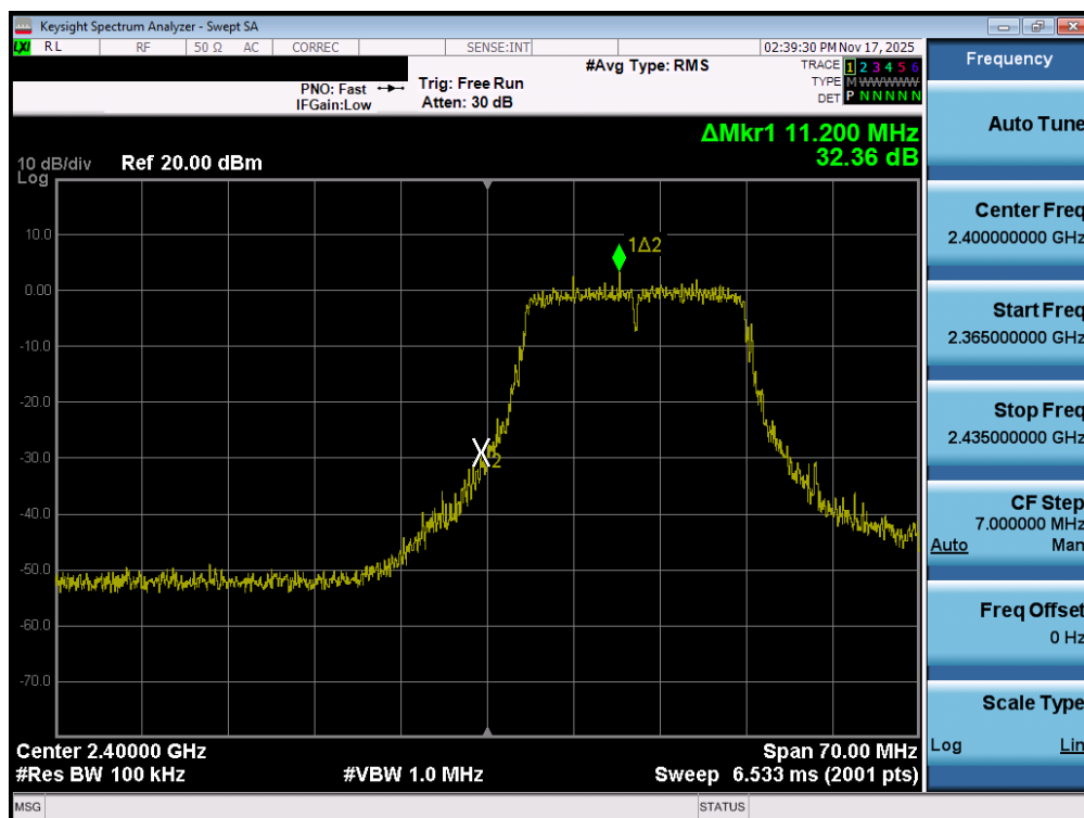
Plot 7-78. Band Edge Plot MIMO ANT1 (802.11n(2.4GHz) – Ch. 1)
