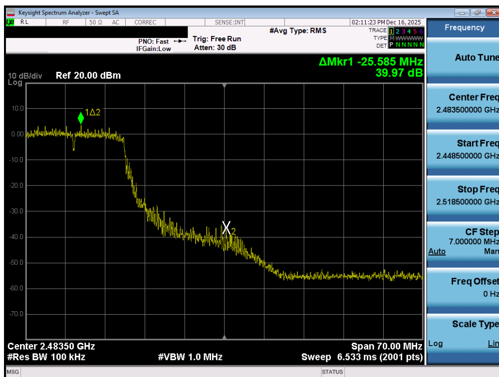
Plot 7-90. Band Edge Plot MIMO ANT2 (802.11n(2.4GHz) – Ch. 10)
