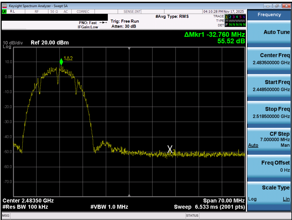
Plot 7-85. Band Edge Plot MIMO ANT2 (802.11b – Ch. 11)
