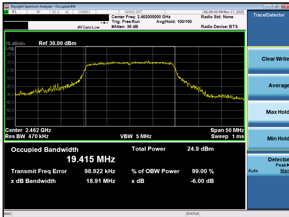
Plot 7-36. OBW Plot MIMO ANT1 (802.11ax (2.4GHz) – Ch. 11)
