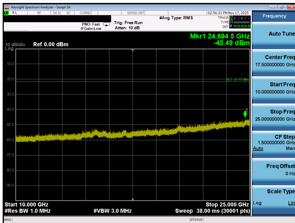
Plot 7-98. Conducted Spurious Plot MIMO ANT1 (802.11b – Ch. 6)
