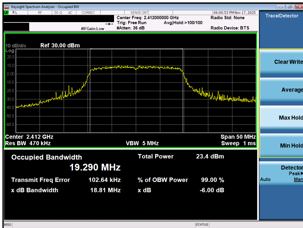
Plot 7-46. OBW Plot MIMO ANT2 (802.11ax (2.4GHz) – Ch. 1)
