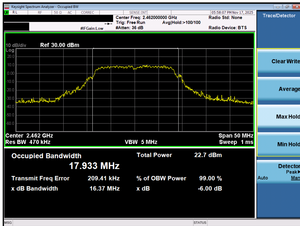
Plot 7-42. OBW Plot MIMO ANT2 (802.11g – Ch. 11)
