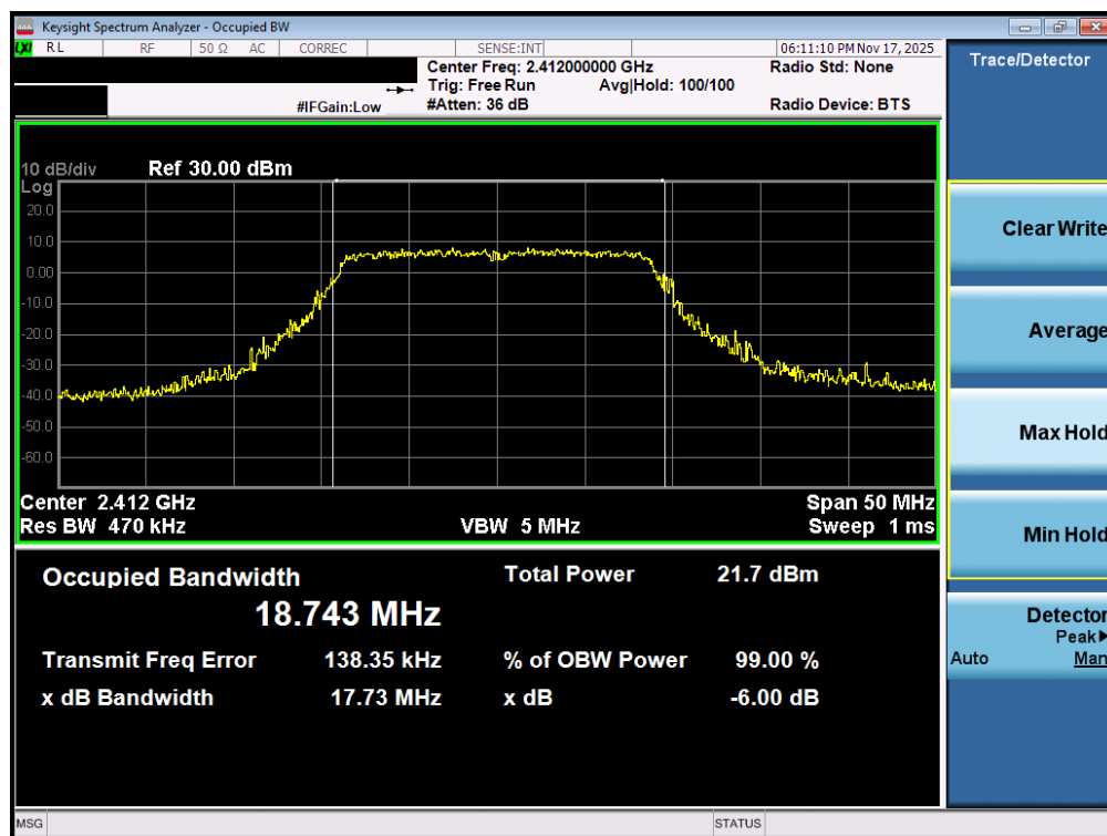
Plot 7-31. OBW Plot MIMO ANT1 (802.11n/ac (2.4GHz) – Ch. 1)
