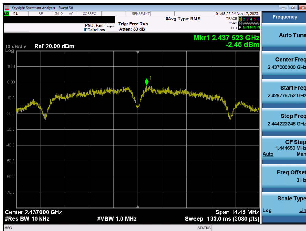
Plot 7-62. Power Spectral Density Plot MIMO ANT1 (802.11b – Ch. 6)
