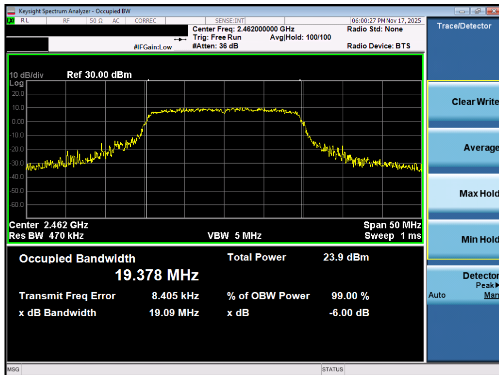
Plot 7-48. OBW Plot MIMO ANT2 (802.11ax (2.4GHz) – Ch. 11)
