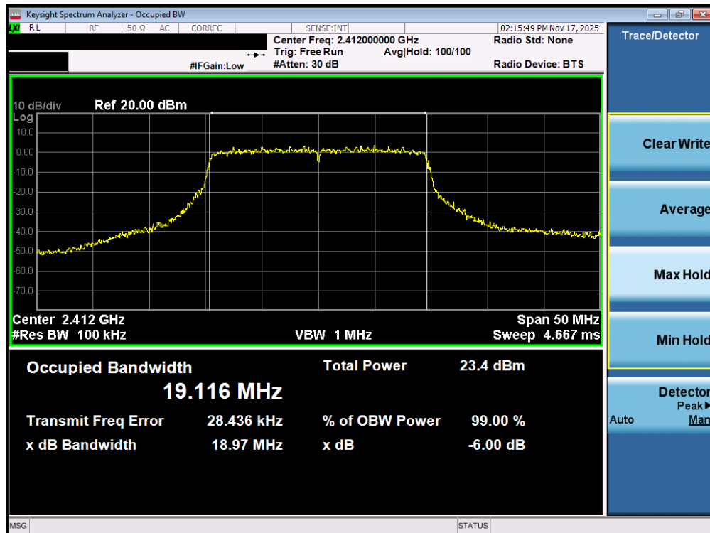
Plot 7-10. 6dB Bandwidth Plot MIMO ANT1 (802.11ax (2.4GHz) – Ch. 1)
