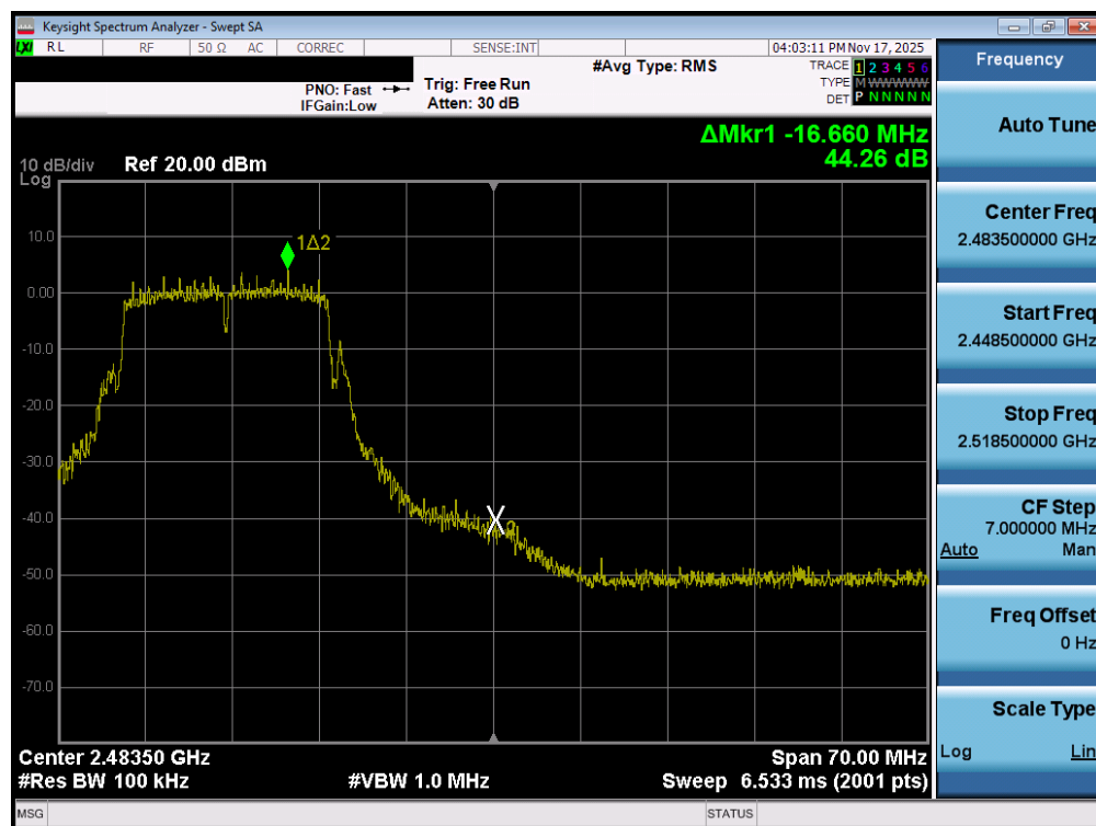
Plot 7-88. Band Edge Plot MIMO ANT2 (802.11g - Ch. 11)
