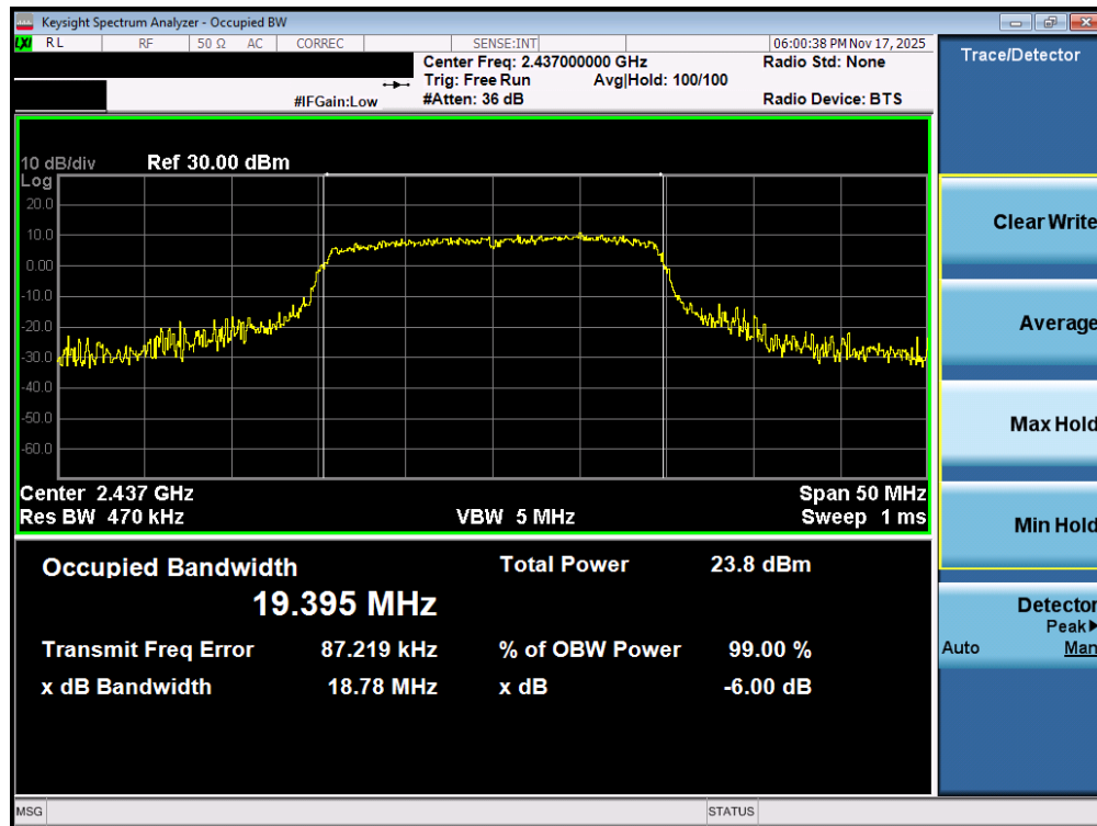
Plot 7-47. OBW Plot MIMO ANT2 (802.11ax (2.4GHz) – Ch. 6)
