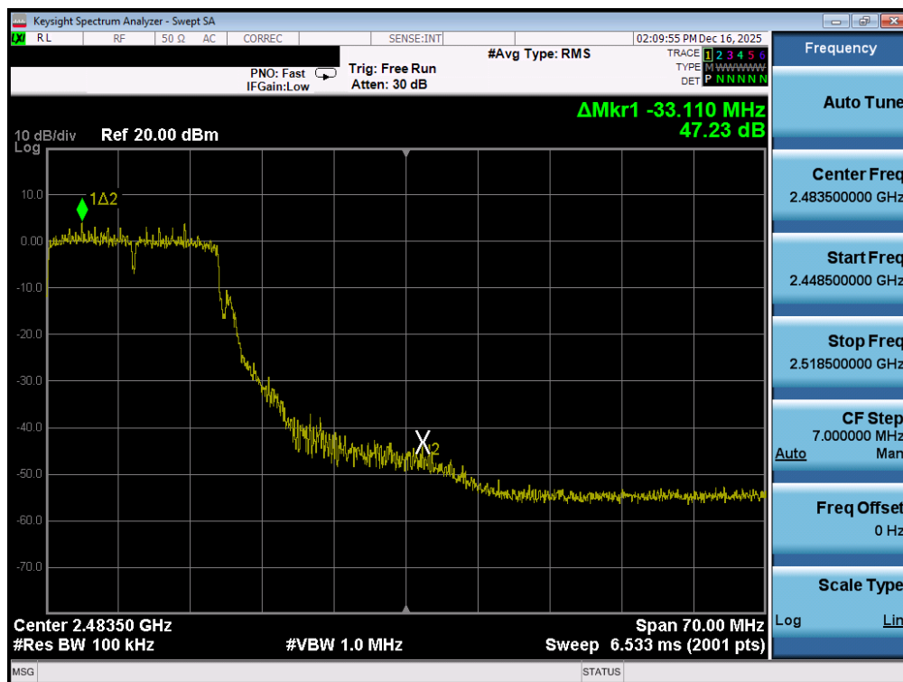
Plot 7-87. Band Edge Plot MIMO ANT2 (802.11g - Ch. 10)
