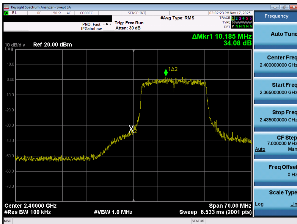
Plot 7-92. Band Edge Plot MIMO ANT2 (802.11ax (2.4GHz) – Ch. 1)
