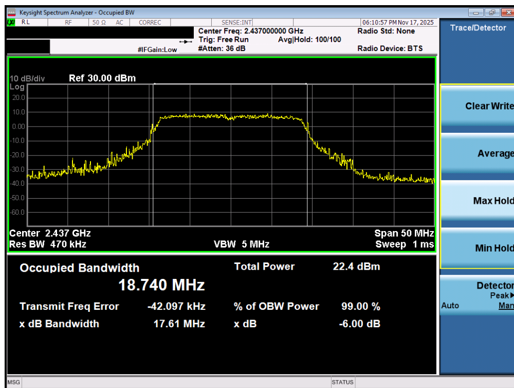
Plot 7-32. OBW Plot MIMO ANT1 (802.11n/ac (2.4GHz) – Ch. 6)
