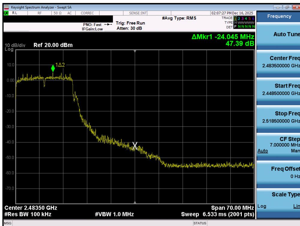
Plot 7-76. Band Edge Plot MIMO ANT1 (802.11g - Ch. 10)
