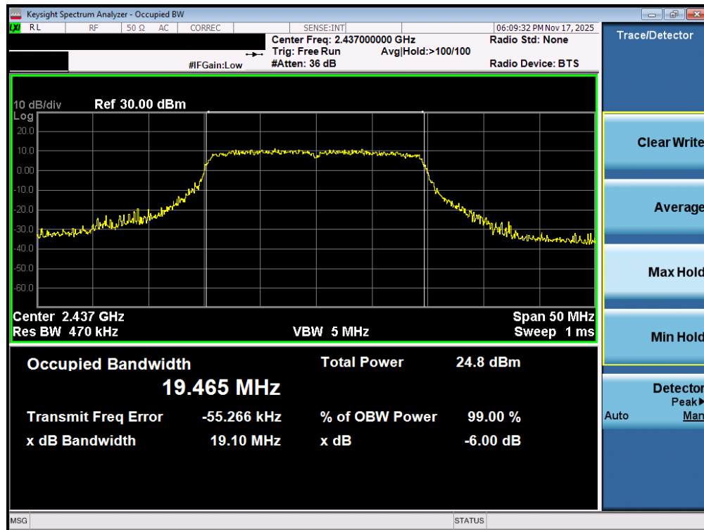
Plot 7-35. OBW Plot MIMO ANT1 (802.11ax (2.4GHz) – Ch. 6)
