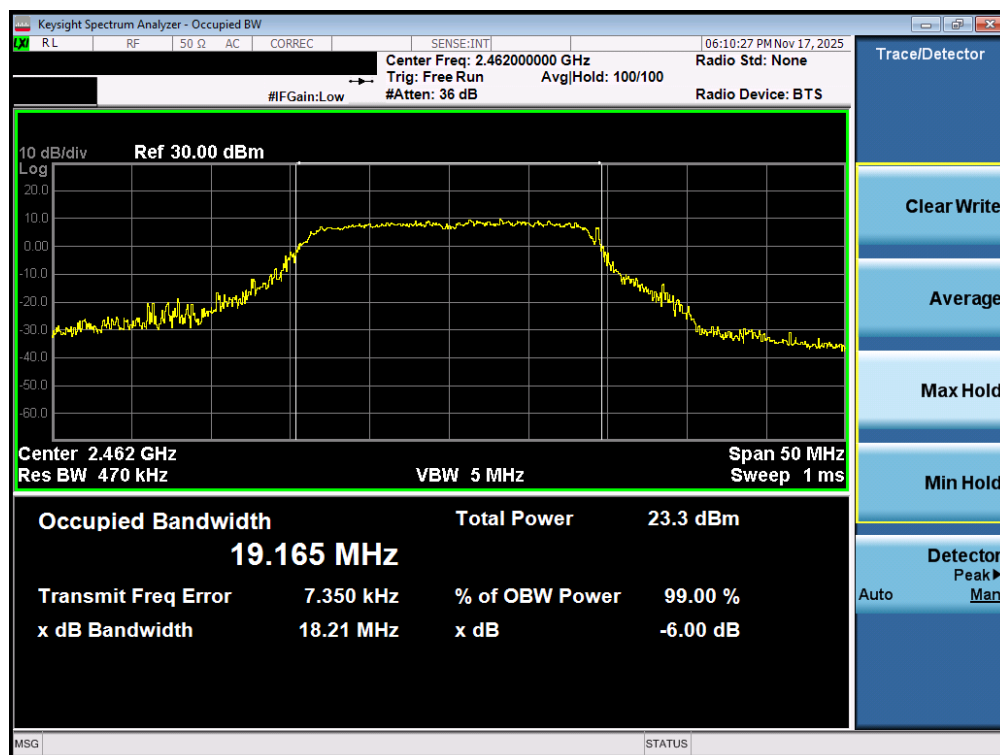
Plot 7-33. OBW Plot MIMO ANT1 (802.11n/ac (2.4GHz) – Ch. 11)
