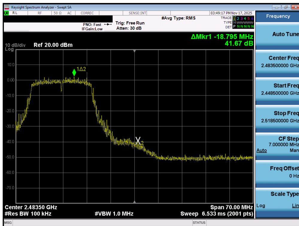
Plot 7-91. Band Edge Plot MIMO ANT2 (802.11n(2.4GHz) – Ch. 11)
