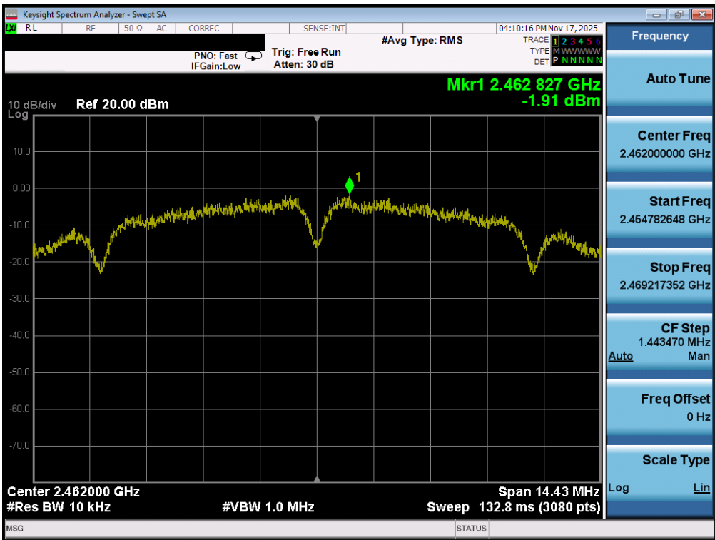
Plot 7-63. Power Spectral Density Plot MIMO ANT1 (802.11b – Ch. 11)
