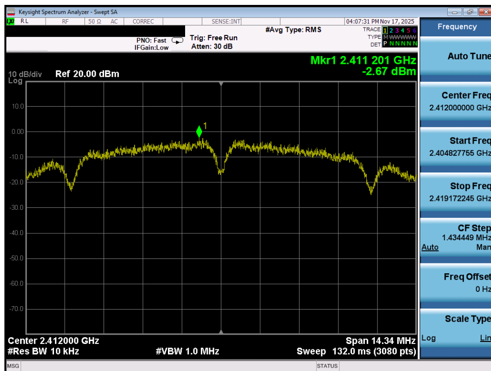
Plot 7-61. Power Spectral Density Plot MIMO ANT1 (802.11b – Ch. 1)
