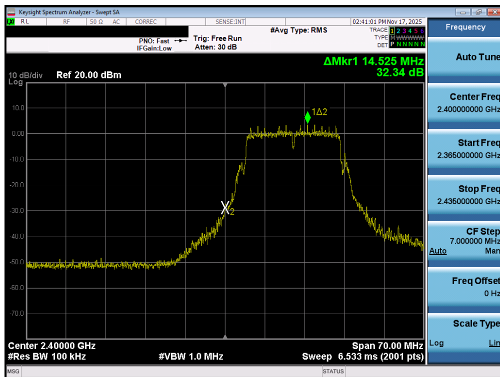
Plot 7-75. Band Edge Plot MIMO ANT1 (802.11g- Ch. 1)
