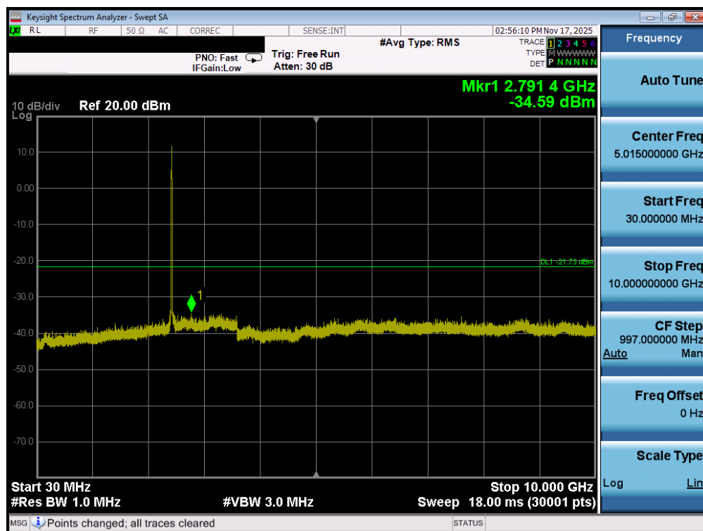
Plot 7-97. Conducted Spurious Plot MIMO ANT1 (802.11b – Ch. 6)
