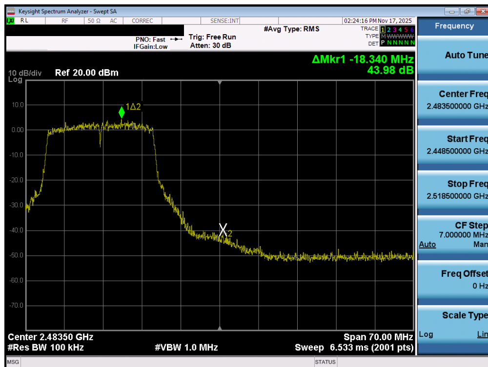
Plot 7-83. Band Edge Plot MIMO ANT1 (802.11ax (2.4GHz) – Ch. 11)
