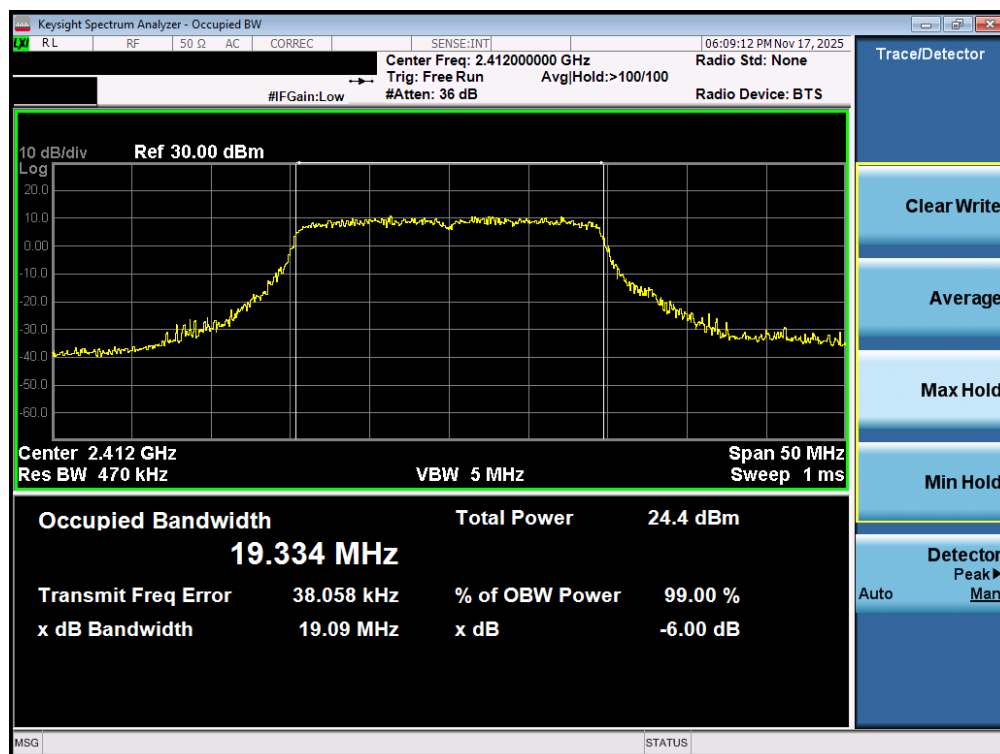
Plot 7-34. OBW Plot MIMO ANT1 (802.11ax (2.4GHz) – Ch. 1)
