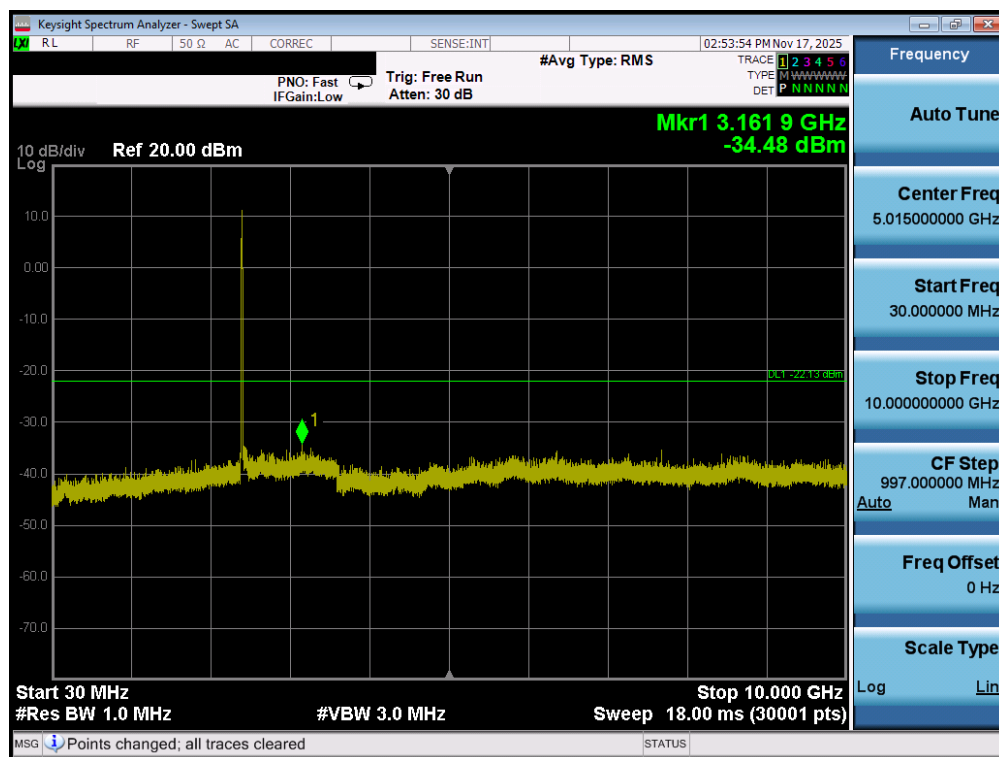
Plot 7-95. Conducted Spurious Plot MIMO ANT1 (802.11b – Ch. 1)
