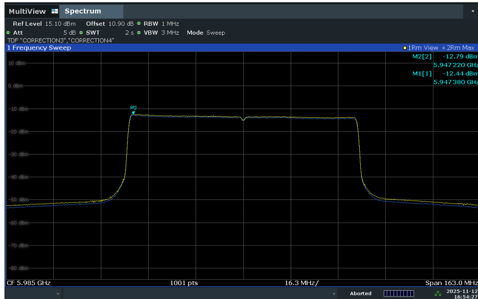
Plot 7-26. Power Spectral Density Plot – ANT2 (80MHz Bandwidth, RSSI level at -42dBm (yellow) and -28dBm (blue))
