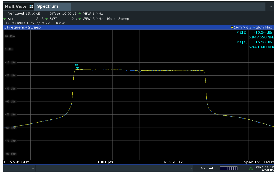
Plot 7-25. Power Spectral Density Plot – ANT1 (80MHz Bandwidth, RSSI level at -42dBm (yellow) and -28dBm (blue))
