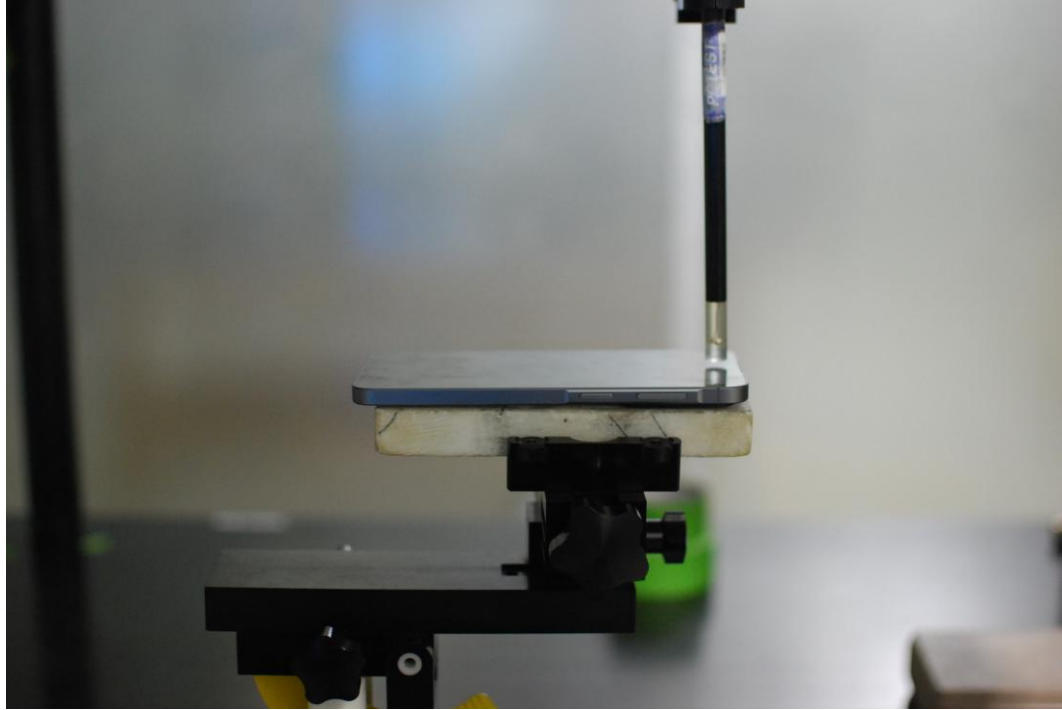
Figure 18-1 Test Setup for Wireless Device – Single Point Measurement
