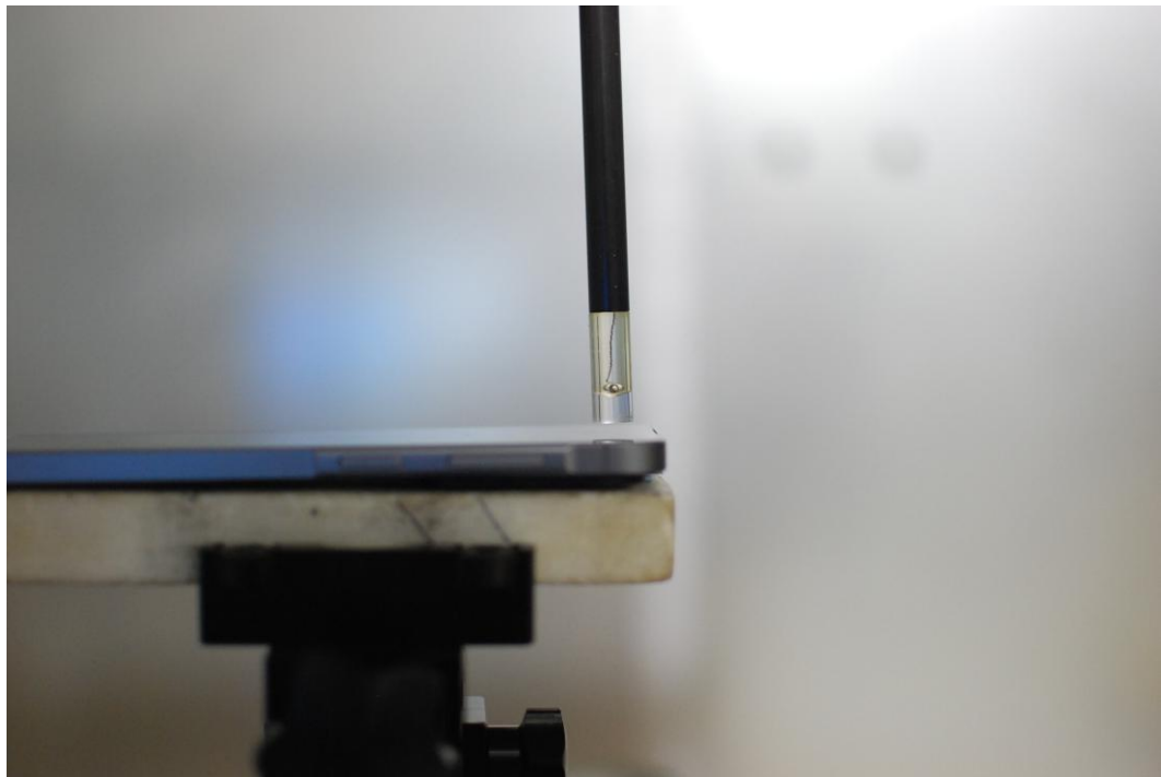
Figure 18-2 Test Setup for Wireless Device – Single Point Measurement
