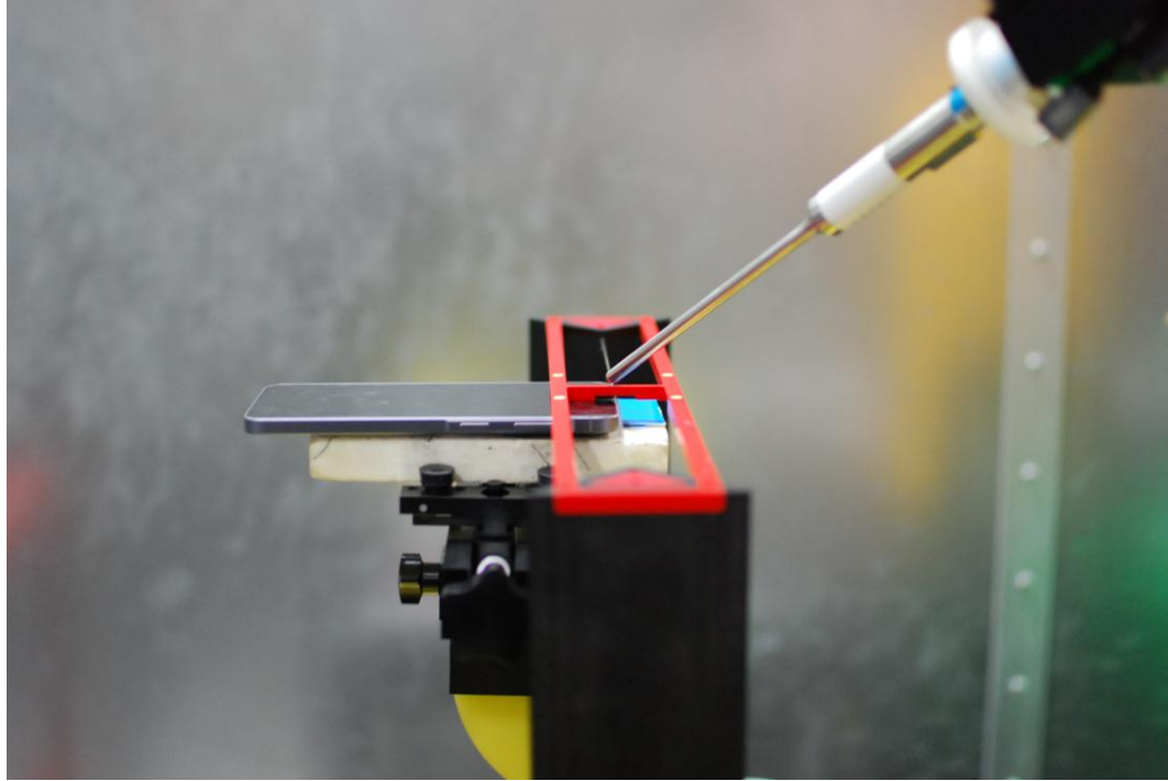
Figure 18-3 Test Setup for Wireless Device – Scan Measurement
