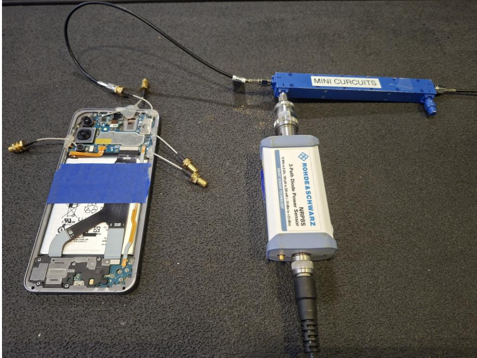
Test Setup Photo 7 – Conducted Test Setup (Figure 7-1a)
