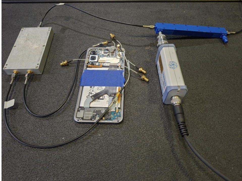
Test Setup Photo 3 – Conducted Test Setup (Figure 7-1b)
