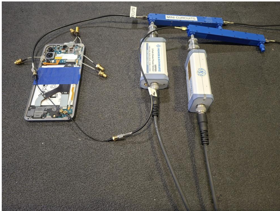
Test Setup Photo 4 – Conducted Test Setup (Figure 7-1c)
