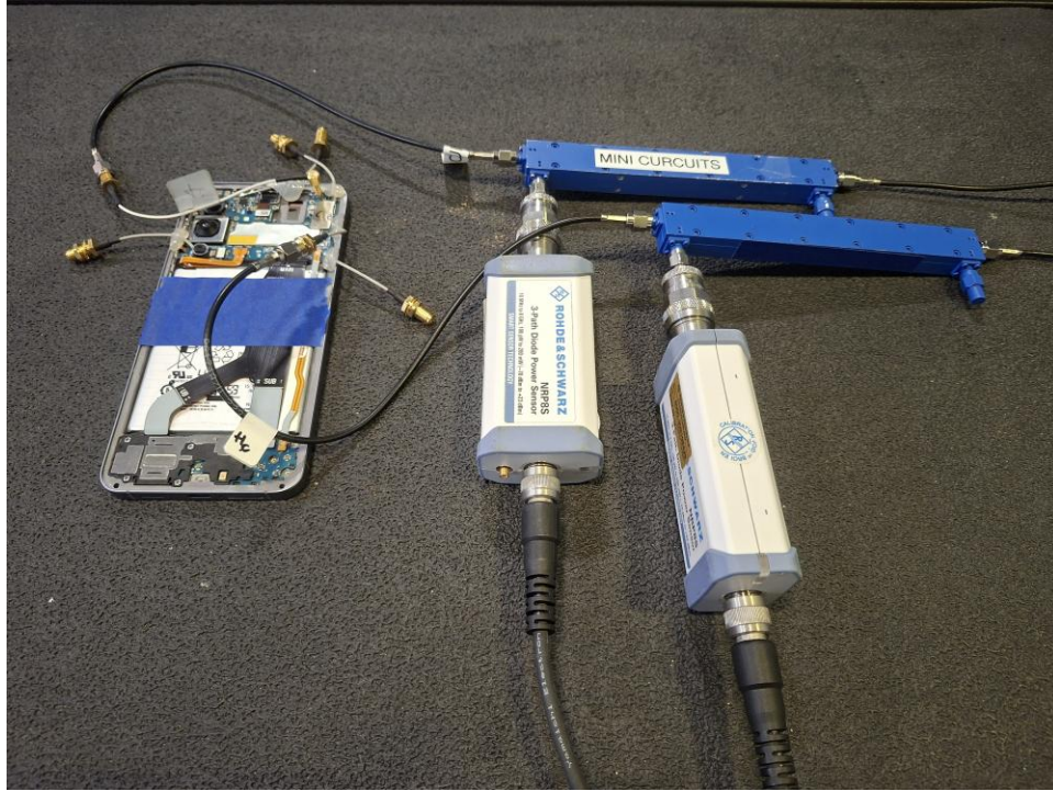
Test Setup Photo 9 – Conducted Test Setup (Figure 7-1f)
