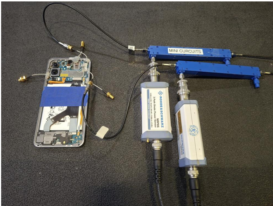
Test Setup Photo 8 – Conducted Test Setup (Figure 7-1e)
