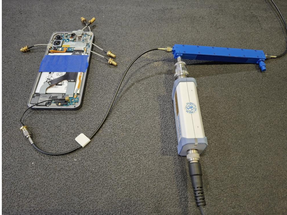
Test Setup Photo 1 – Conducted Test Setup (Figure 7-1a)
