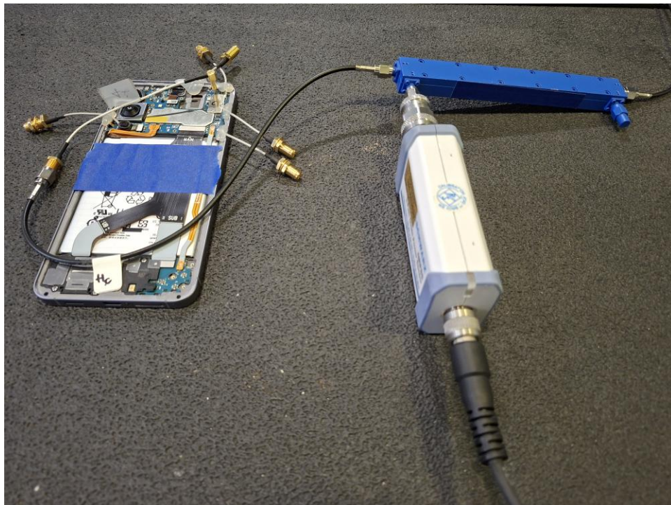
Test Setup Photo 2 – Conducted Test Setup (Figure 7-1a)
