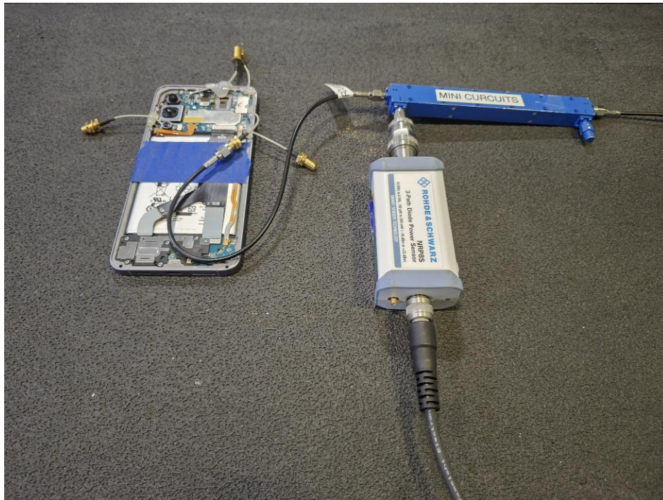
Test Setup Photo 6 – Conducted Test Setup (Figure 7-1a)
