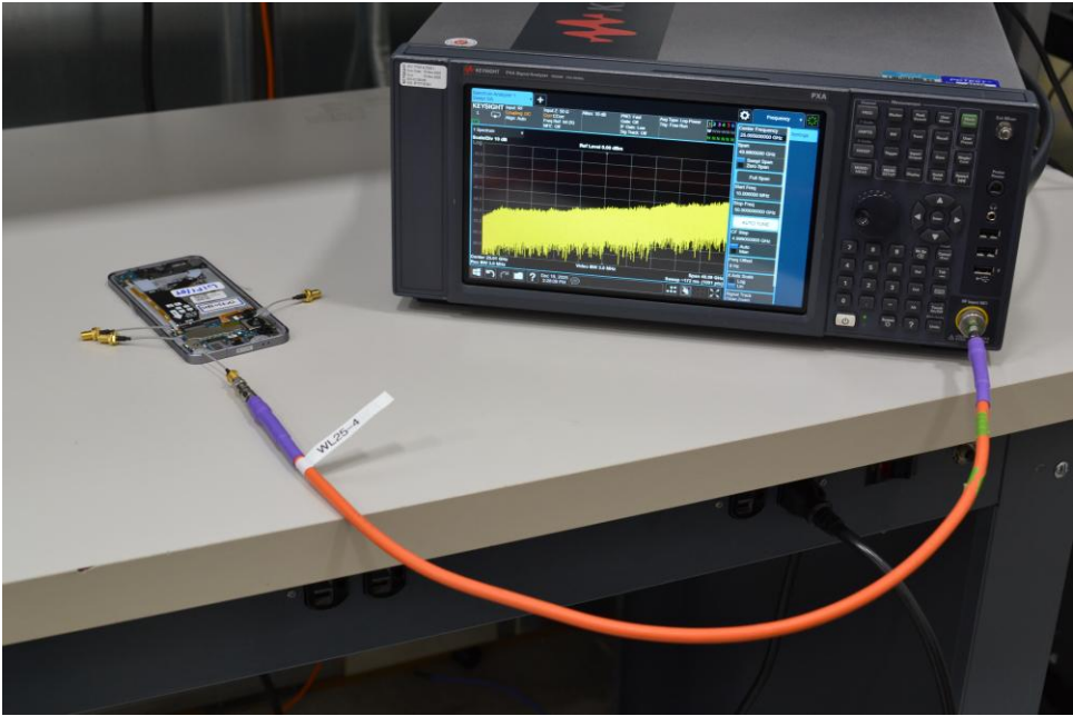
Figure 7. Conducted Test Setup
