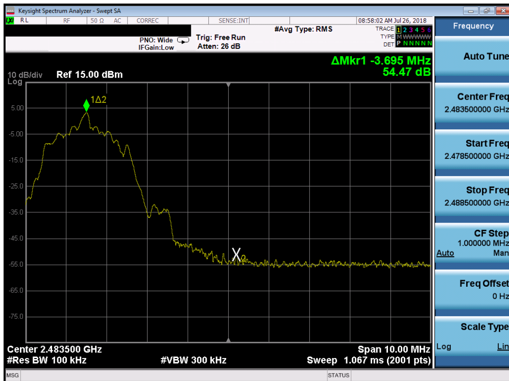
Plot 7-22. Band Edge Plot (Bluetooth (LE), 1Mbps – Ch. 39)
