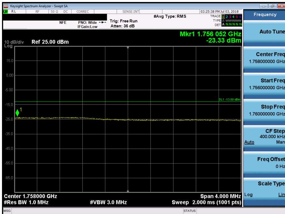
Plot 7-144. Upper Extended Band Edge Plot (Band 4 - 15.0MHz QPSK - Full RB Configuration)
