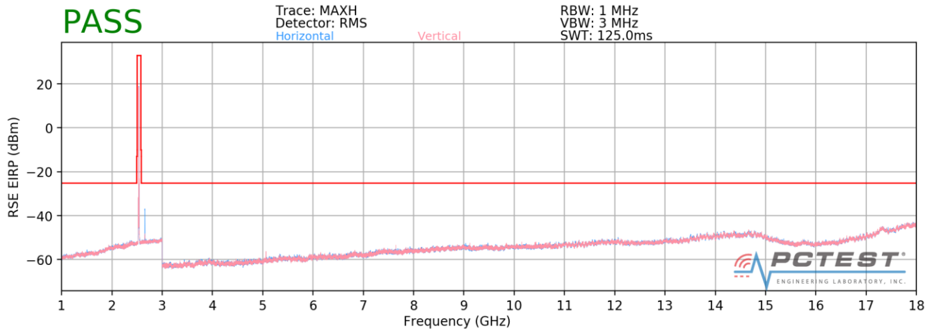
Plot 7-197. Radiated Spurious Plot 1GHz - 18GHz (Band 7)
