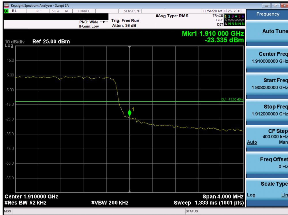
Plot 7-159. Upper Band Edge Plot (Band 2 - 5.0MHz QPSK - Full RB Configuration)
