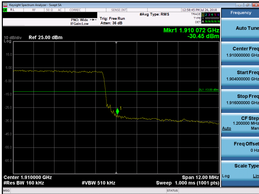
Plot 7-167. Upper Band Edge Plot (Band 2 - 15.0MHz QPSK - Full RB Configuration)
