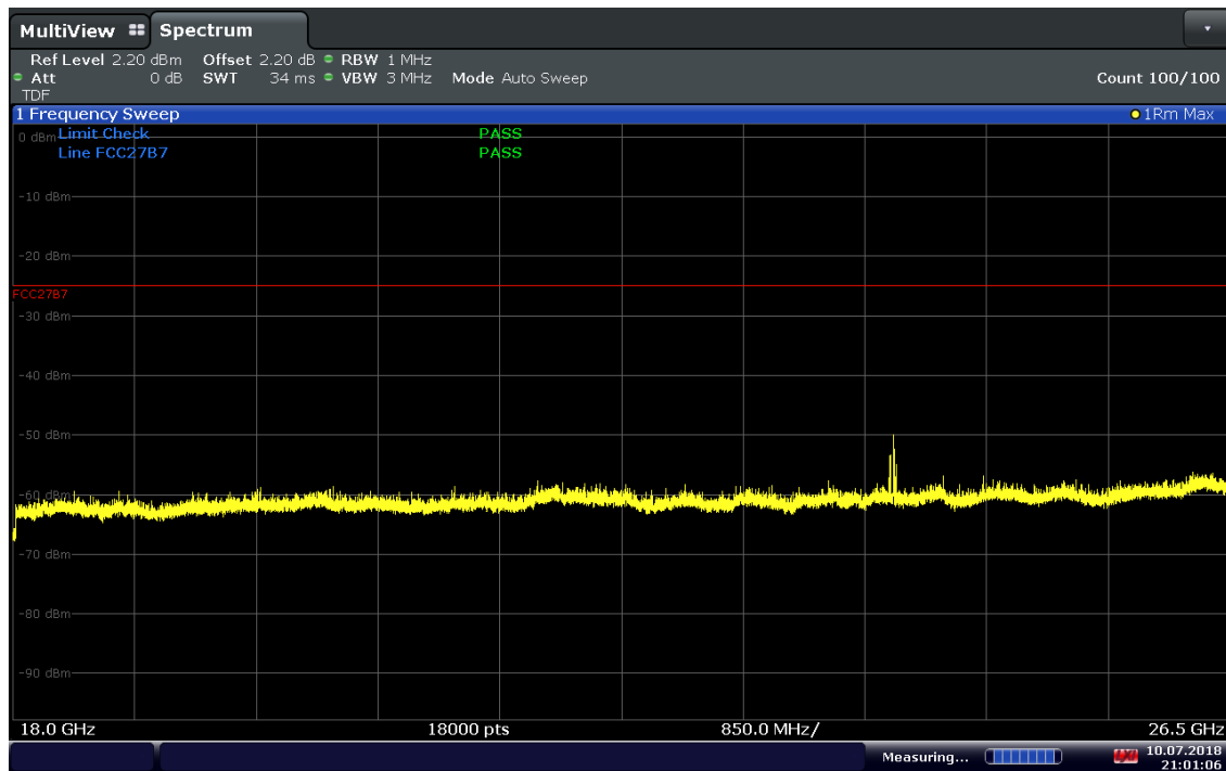
Plot 7-198. Radiated Spurious Plot 18GHz – 26.5GHz (Band 7), H Pol.
