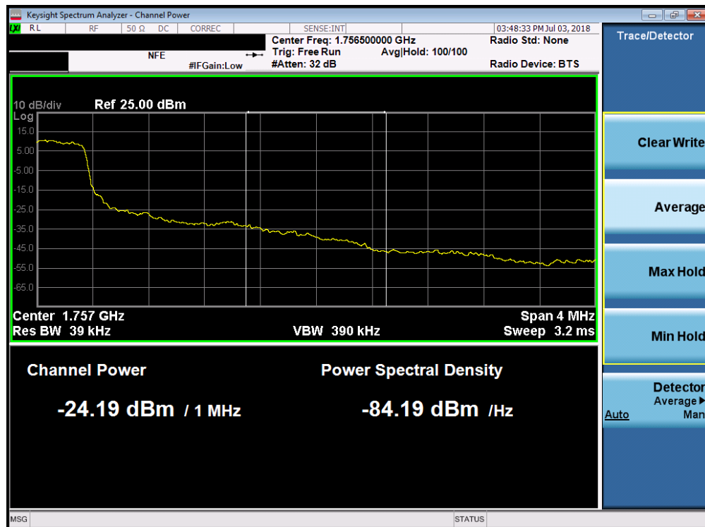
Plot 7-128. Upper Extended Band Edge Plot (Band 4 - 1.4MHz QPSK - Full RB Configuration)
