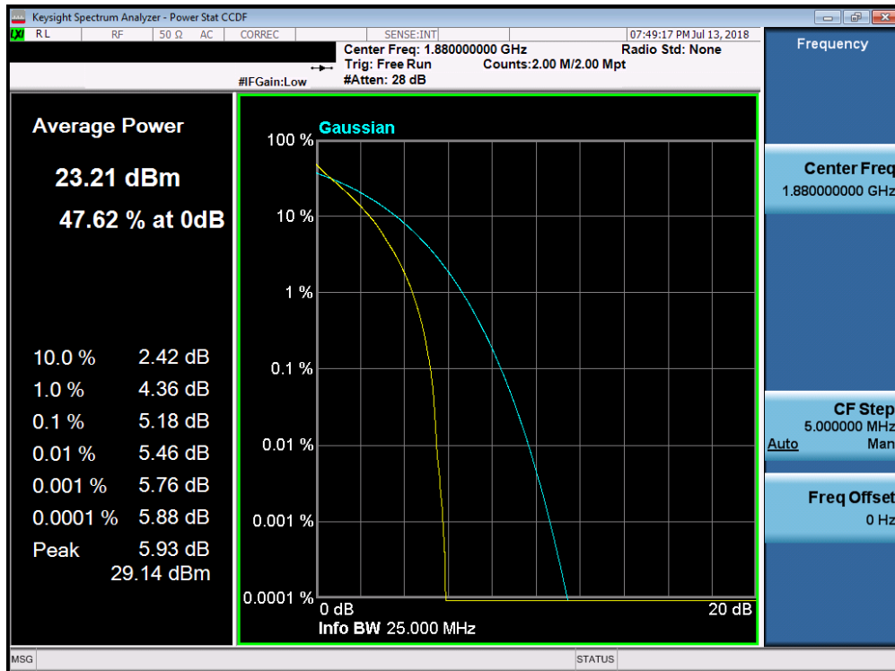
Plot 7-189. PAR Plot (Band 2 - 15.0MHz QPSK - Full RB Configuration)
