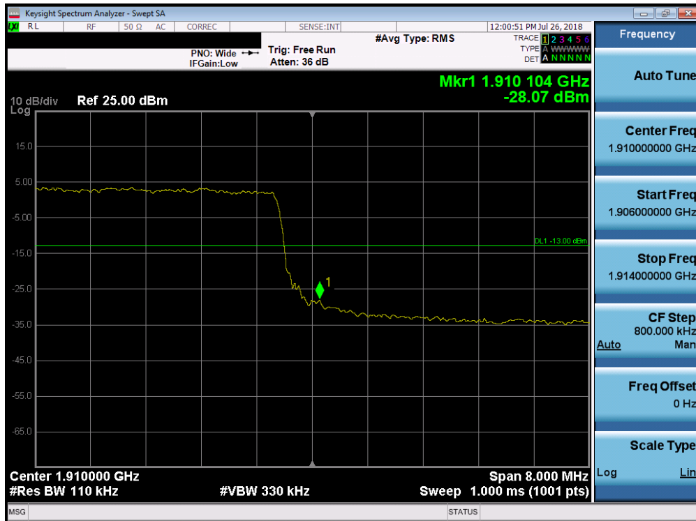
Plot 7-163. Upper Band Edge Plot (Band 2 - 10.0MHz QPSK - Full RB Configuration)
