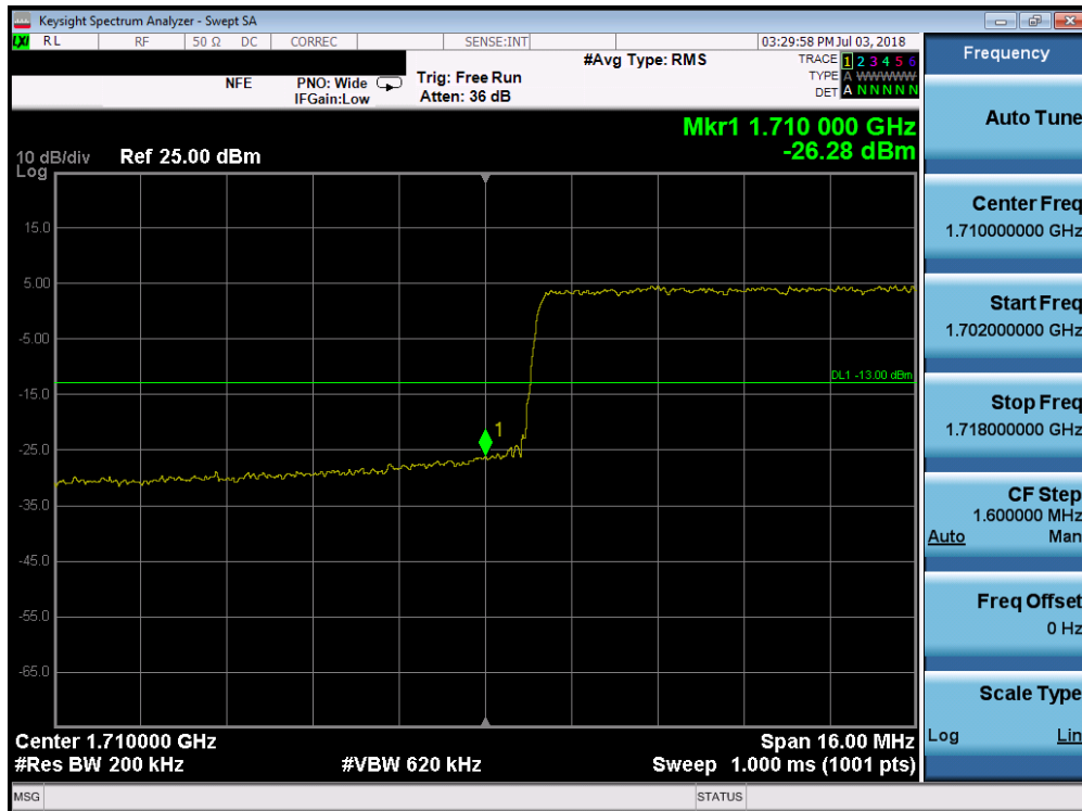
Plot 7-145. Lower Band Edge Plot (Band 4 - 20.0MHz QPSK - Full RB Configuration)
