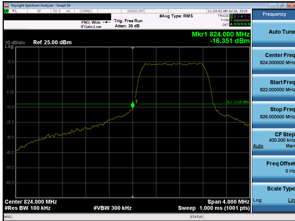
Plot 7-111. Lower Band Edge Plot (Band 5 - 1.4MHz QPSK - Full RB Configuration)
