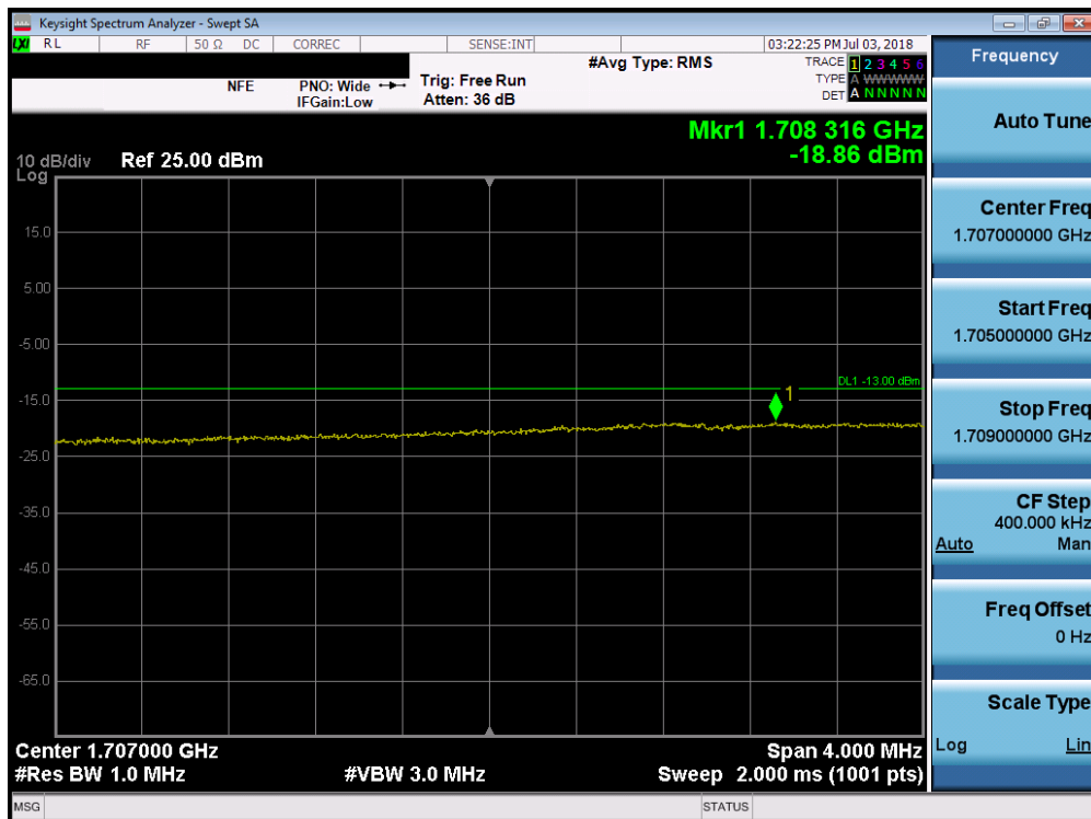
Plot 7-142. Lower Extended Band Edge Plot (Band 4 - 15.0MHz QPSK - Full RB Configuration)
