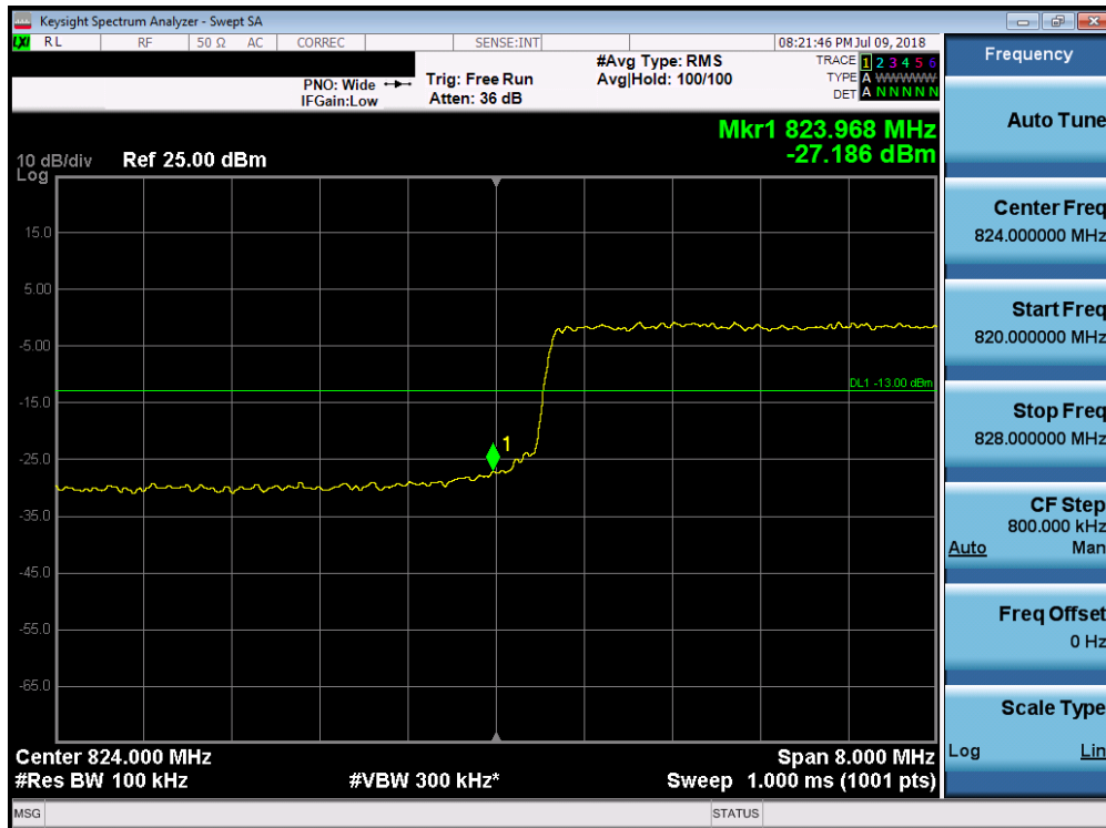
Plot 7-121. Lower Band Edge Plot (Band 5 - 10.0MHz QPSK - Full RB Configuration)
