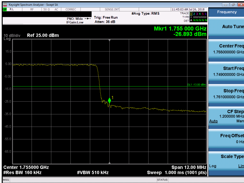
Plot 7-143. Upper Band Edge Plot (Band 4 - 15.0MHz QPSK - Full RB Configuration)
