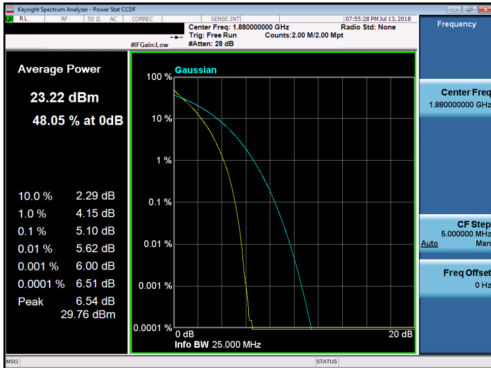
Plot 7-191. PAR Plot (Band 2 - 20.0MHz QPSK - Full RB Configuration)
