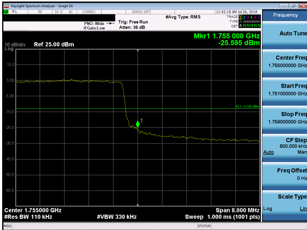
Plot 7-139. Upper Band Edge Plot (Band 4 - 10.0MHz QPSK - Full RB Configuration)
