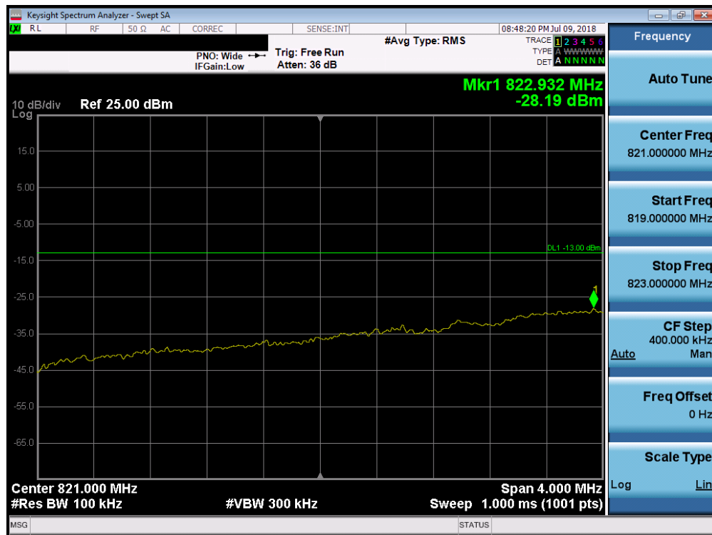
Plot 7-114. Lower Extended Band Edge Plot (Band 5 - 3.0MHz QPSK - Full RB Configuration)
