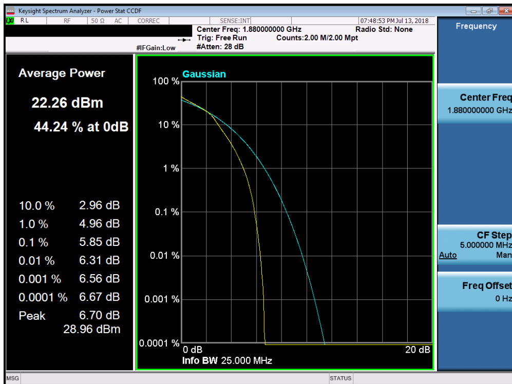
Plot 7-190. PAR Plot (Band 2 - 15.0MHz 16-QAM - Full RB Configuration)
