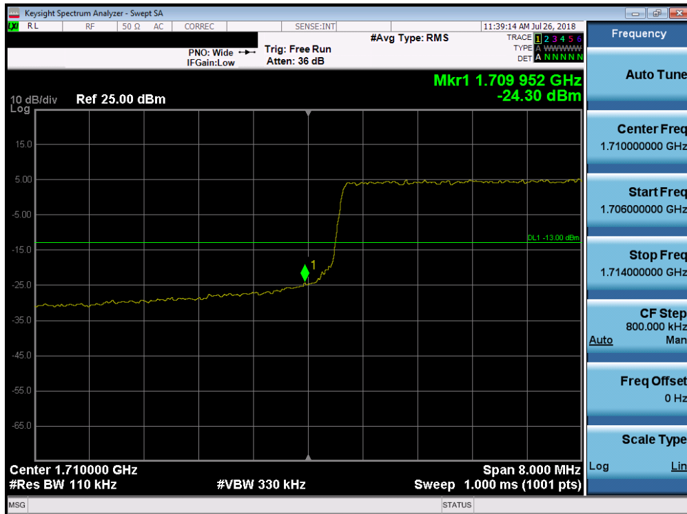
Plot 7-137. Lower Band Edge Plot (Band 4 - 10.0MHz QPSK - Full RB Configuration)
