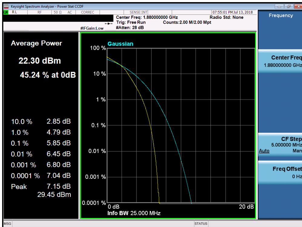
Plot 7-192. PAR Plot (Band 2 - 20.0MHz 16-QAM - Full RB Configuration)
