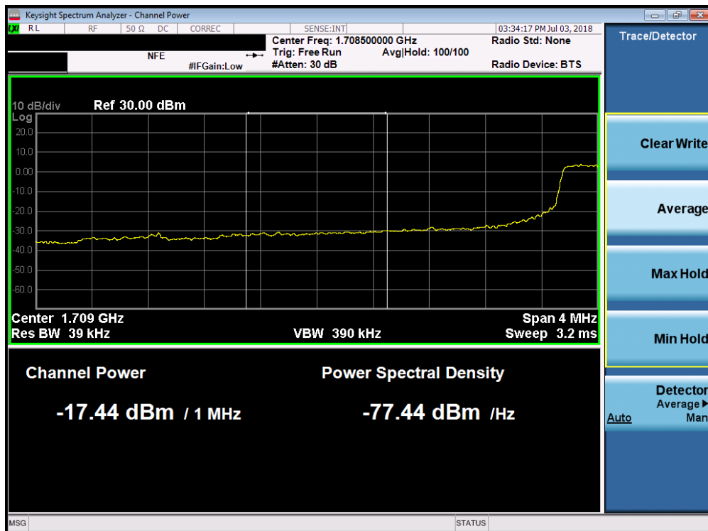
Plot 7-134. Lower Extended Band Edge Plot (Band 4 - 5.0MHz QPSK - Full RB Configuration)
