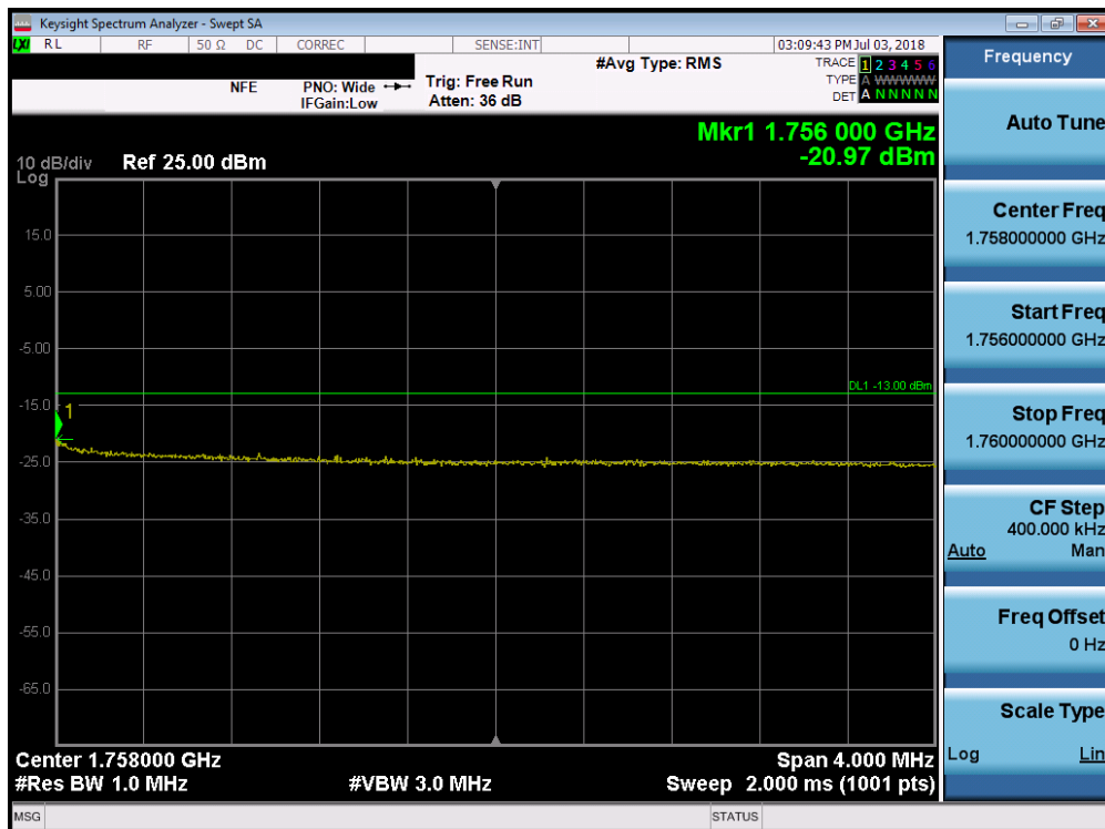
Plot 7-140. Upper Extended Band Edge Plot (Band 4 - 10.0MHz QPSK - Full RB Configuration)
