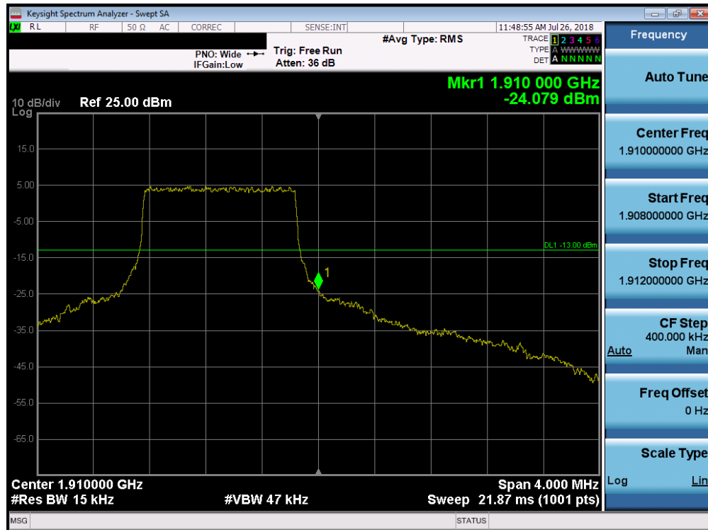
Plot 7-151. Upper Band Edge Plot (Band 2 - 1.4MHz QPSK - Full RB Configuration)
