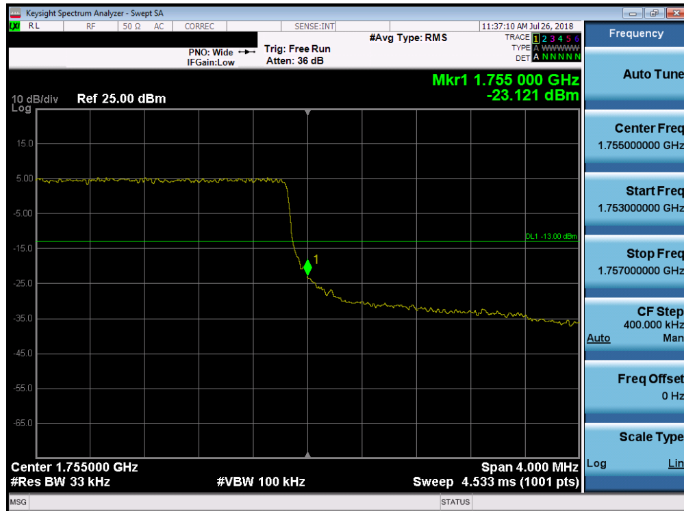
Plot 7-131. Upper Band Edge Plot (Band 4 - 3.0MHz QPSK - Full RB Configuration)
