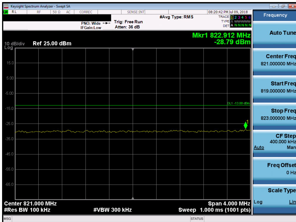
Plot 7-122. Lower Extended Band Edge Plot (Band 5 - 10.0MHz QPSK - Full RB Configuration)
