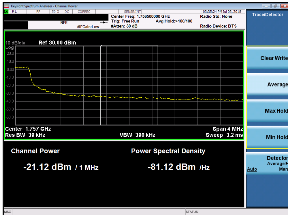
Plot 7-136. Upper Extended Band Edge Plot (Band 4 - 5.0MHz QPSK - Full RB Configuration)
