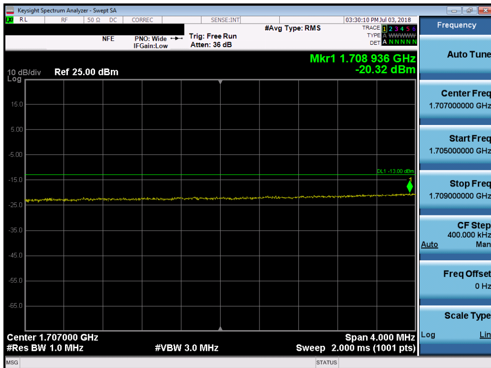
Plot 7-146. Lower Extended Band Edge Plot (Band 4 - 20.0MHz QPSK - Full RB Configuration)
