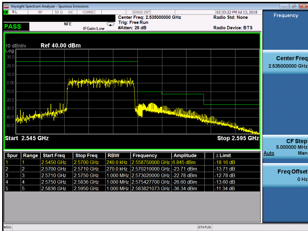
Plot 7-178. Upper ACP Plot (Band 7 – 15.0MHz QPSK – RB Size 75)
