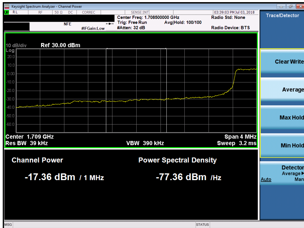
Plot 7-130. Lower Extended Band Edge Plot (Band 4 - 3.0MHz QPSK - Full RB Configuration)
