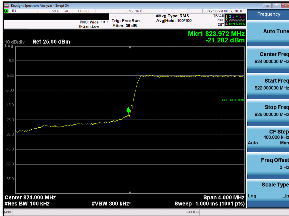
Plot 7-113. Lower Band Edge Plot (Band 5 - 3.0MHz QPSK - Full RB Configuration)
