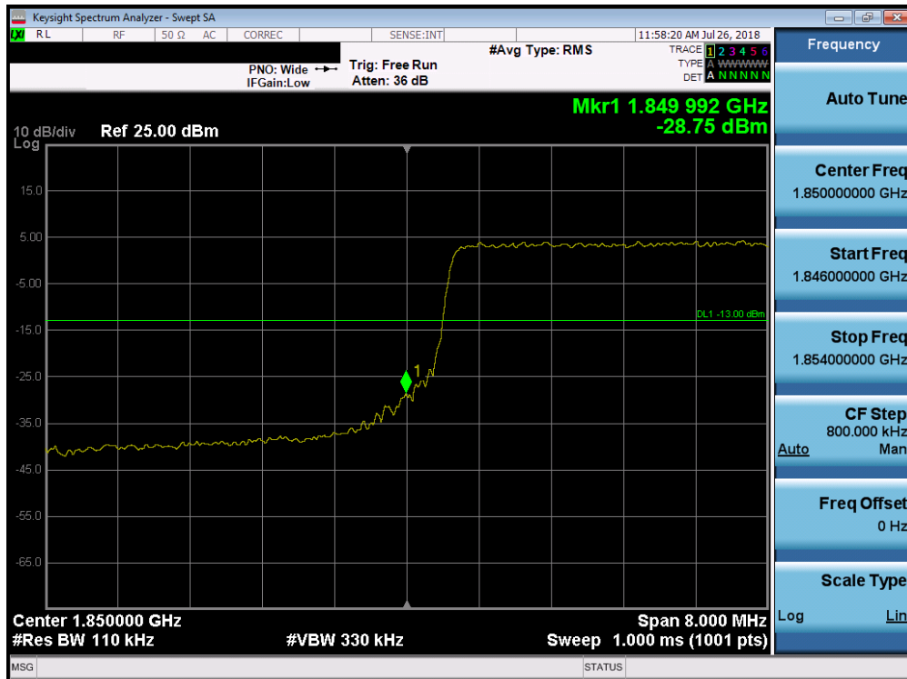
Plot 7-161. Lower Band Edge Plot (Band 2 - 10.0MHz QPSK - Full RB Configuration)
