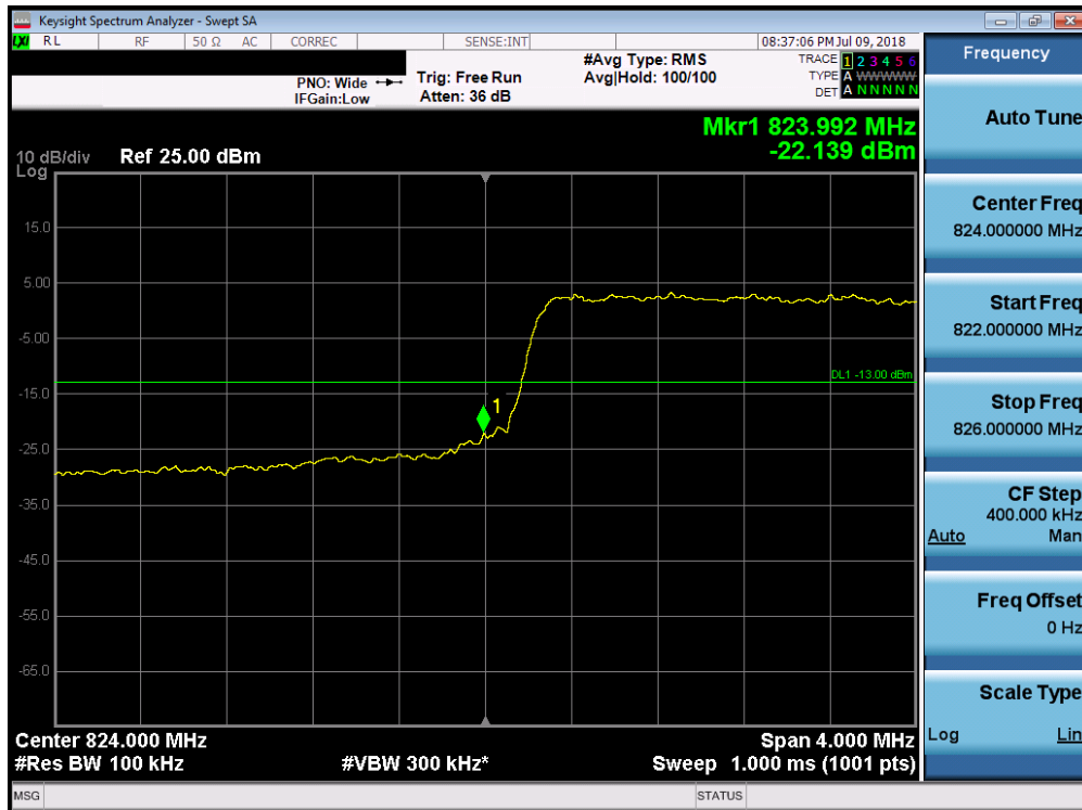
Plot 7-117. Lower Band Edge Plot (Band 5 - 5.0MHz QPSK - Full RB Configuration)
