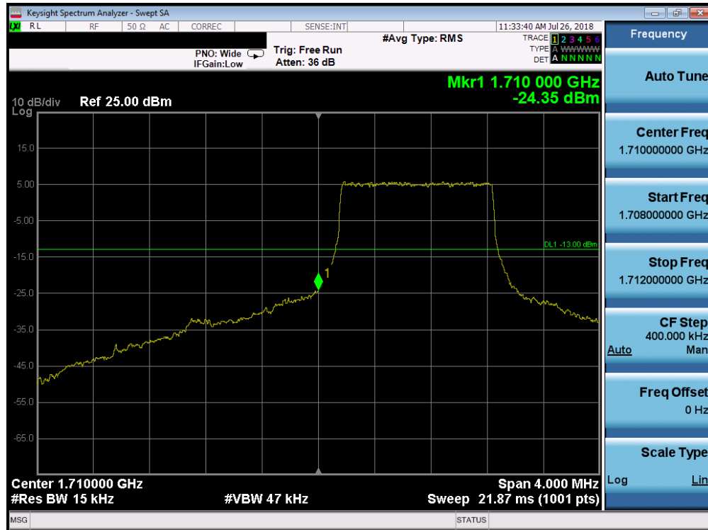
Plot 7-125. Lower Band Edge Plot (Band 4 - 1.4MHz QPSK - Full RB Configuration)
