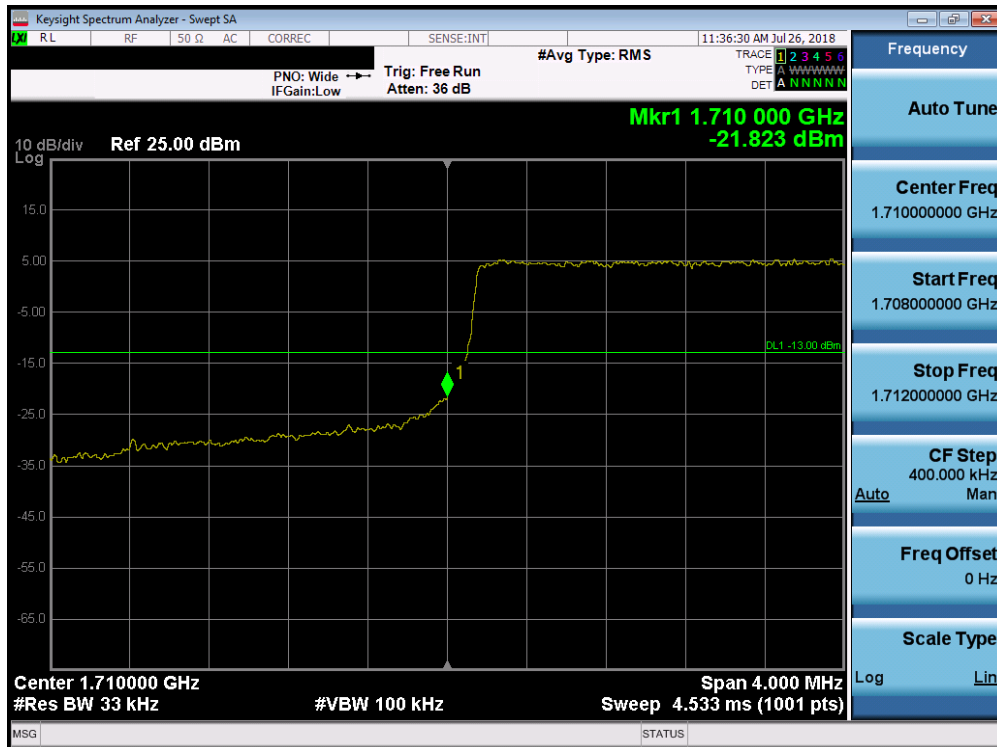
Plot 7-129. Lower Band Edge Plot (Band 4 - 3.0MHz QPSK - Full RB Configuration)
