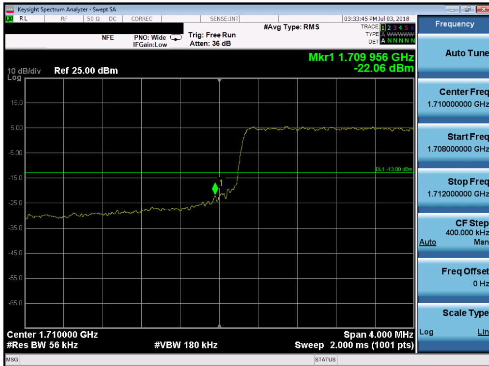
Plot 7-133. Lower Band Edge Plot (Band 4 - 5.0MHz QPSK - Full RB Configuration)
