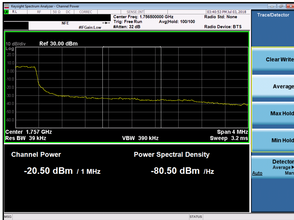
Plot 7-132. Upper Extended Band Edge Plot (Band 4 - 3.0MHz QPSK - Full RB Configuration)
