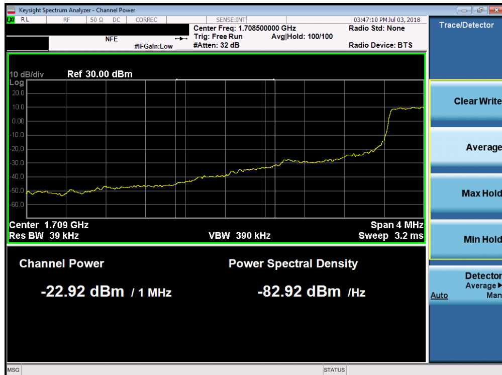
Plot 7-126. Lower Extended Band Edge Plot (Band 4 - 1.4MHz QPSK - Full RB Configuration)
