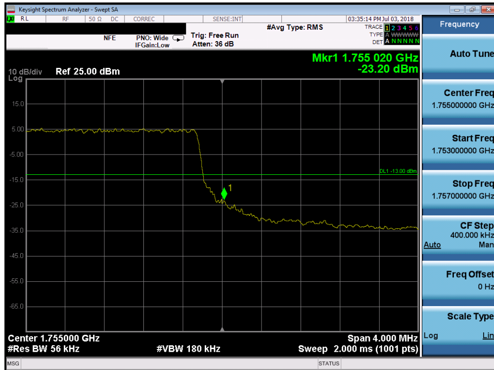
Plot 7-135. Upper Band Edge Plot (Band 4 - 5.0MHz QPSK - Full RB Configuration)
