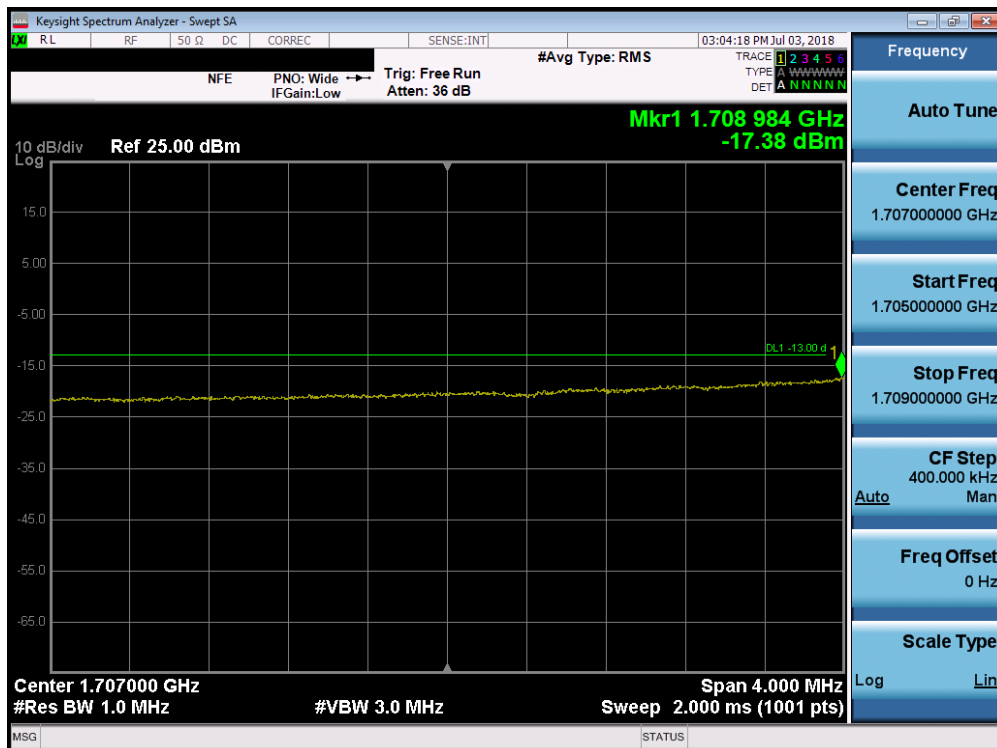
Plot 7-138. Lower Extended Band Edge Plot (Band 4 - 10.0MHz QPSK - Full RB Configuration)
