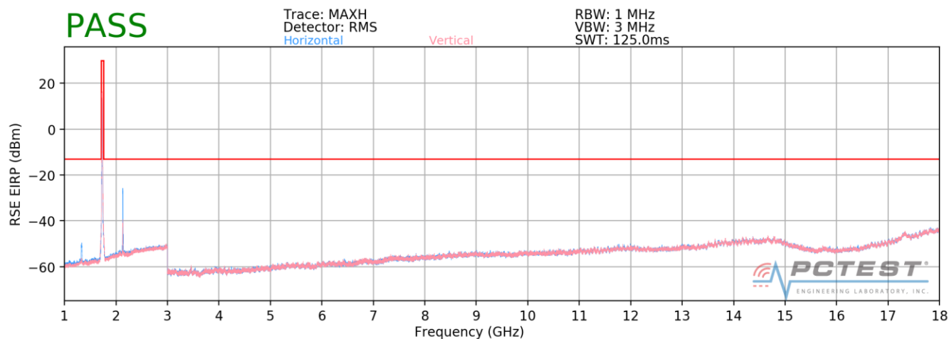
Plot 7-195. Radiated Spurious Plot above 1GHz (Band 4)
