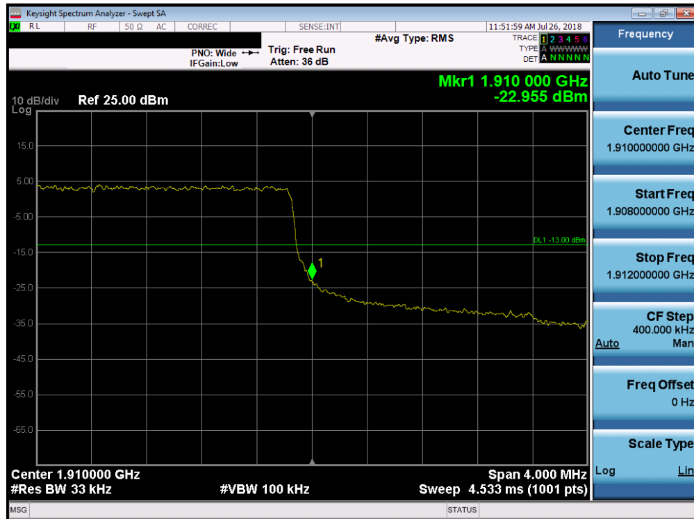
Plot 7-155. Upper Band Edge Plot (Band 2 - 3.0MHz QPSK - Full RB Configuration)
