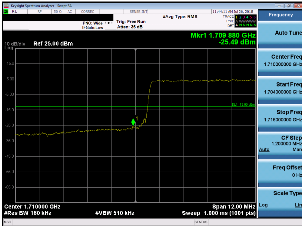
Plot 7-141. Lower Band Edge Plot (Band 4 - 15.0MHz QPSK - Full RB Configuration)
