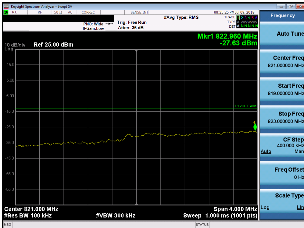
Plot 7-118. Lower Extended Band Edge Plot (Band 5 - 5.0MHz QPSK - Full RB Configuration)
