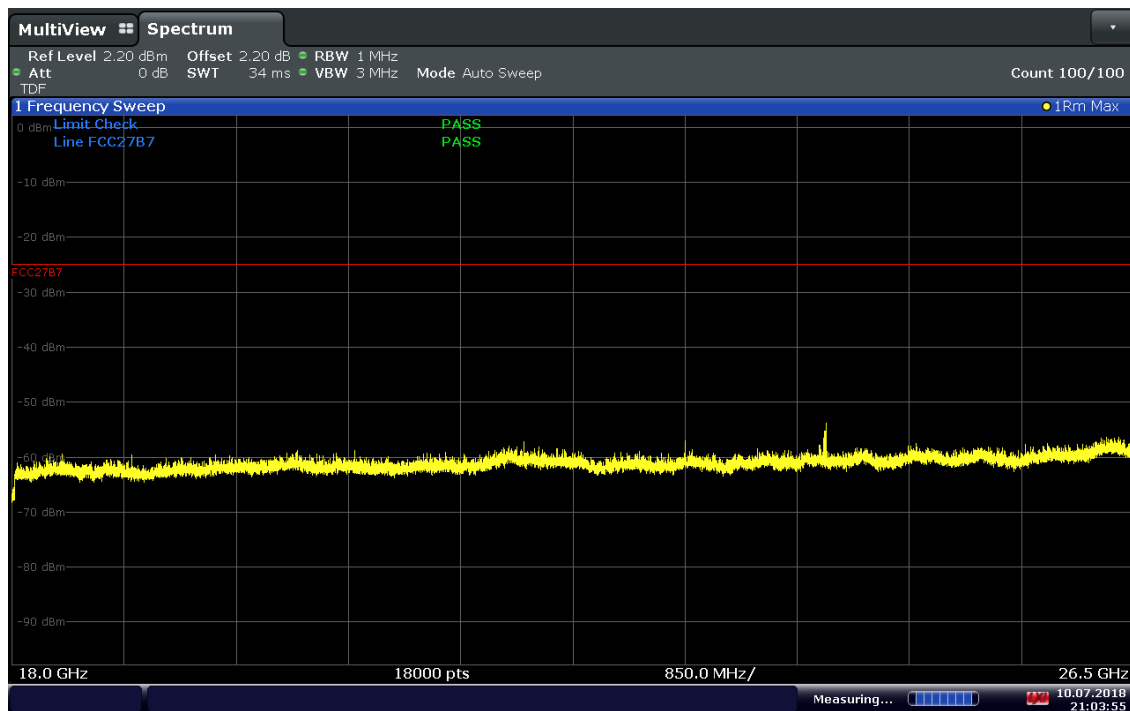
Plot 7-199. Radiated Spurious Plot 18GHz – 26.5GHz (Band 7), V Pol.
