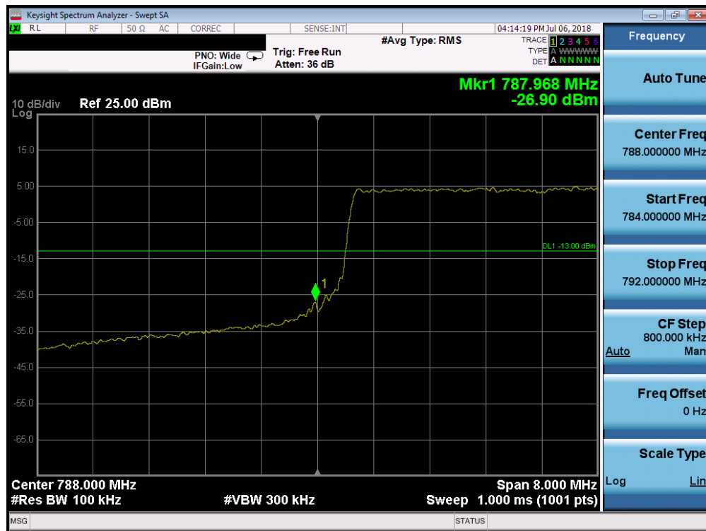
Plot 7-18. Lower Band Edge Plot (LTE Band 14, 10MHz QPSK – RB Size 50)
