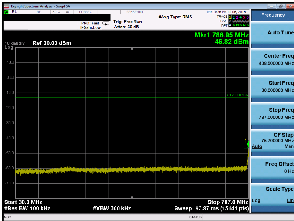
Plot 7-5. Conducted Spurious Plot (LTE Band 14, 10MHz QPSK – RB Size 1, RB Offset 0 – Low Channel)
