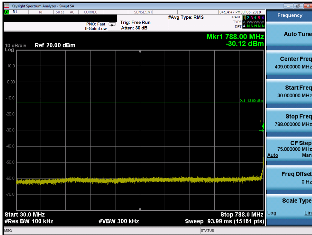
Plot 7-11. Conducted Spurious Plot (LTE Band 14, 10MHz QPSK – RB Size 1, RB Offset 0 – High Channel)
