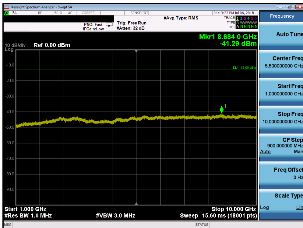
Plot 7-10. Conducted Spurious Plot (LTE Band 14, 10MHz QPSK – RB Size 1, RB Offset 0 – Mid Channel)
