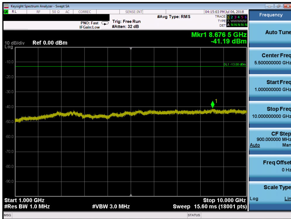
Plot 7-13. Conducted Spurious Plot (LTE Band 14, 10MHz QPSK – RB Size 1, RB Offset 0 – High Channel)
