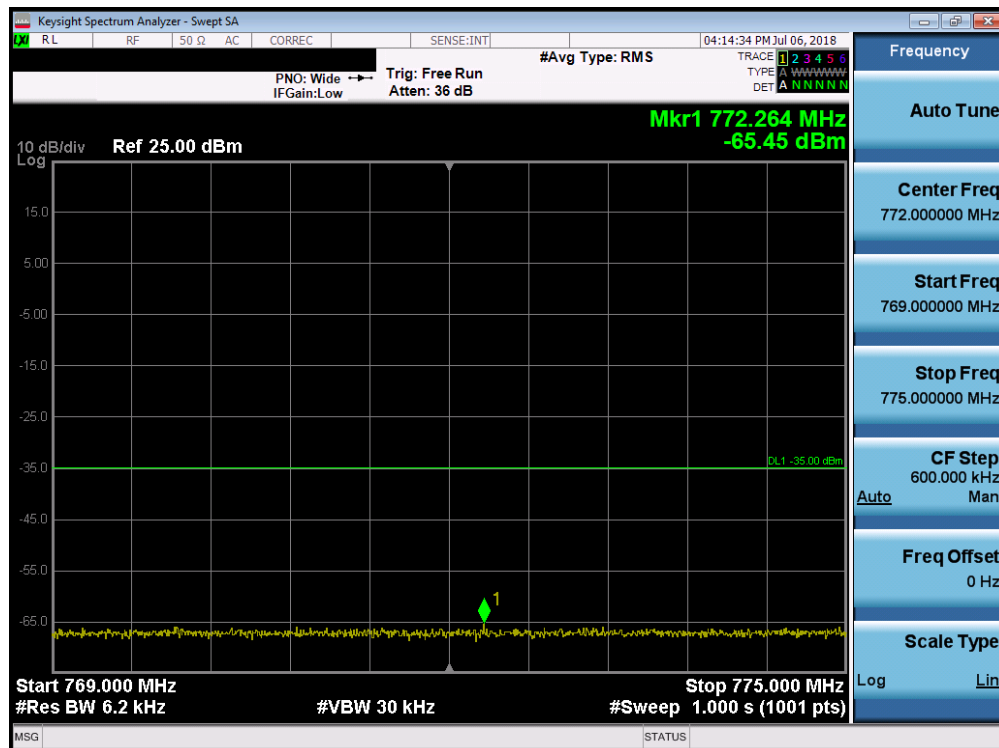
Plot 7-19. Lower Emission Mask Plot (LTE Band 14, 10MHz QPSK – RB Size 50)
