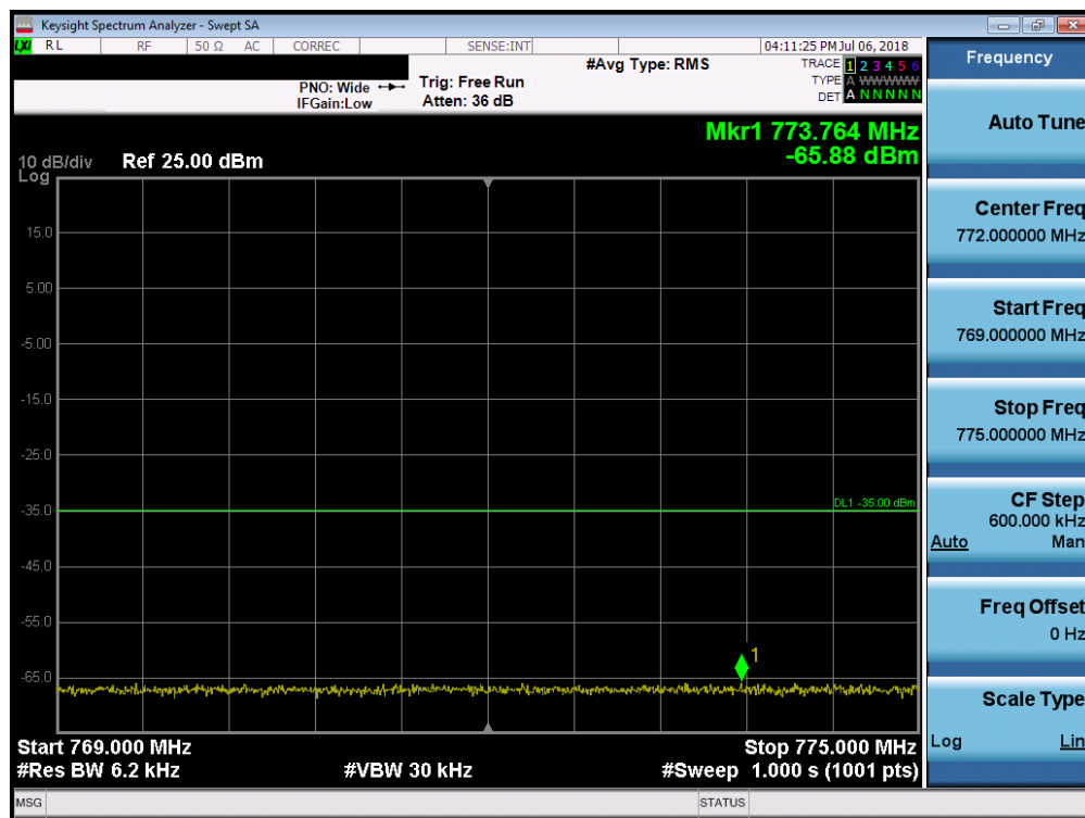
Plot 7-14. Lower Emission Mask Plot (LTE Band 14, 5MHz QPSK – RB Size 25)
