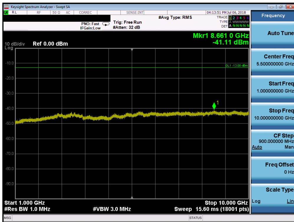
Plot 7-7. Conducted Spurious Plot (LTE Band 14, 10MHz QPSK – RB Size 1, RB Offset 0 – Low Channel)
