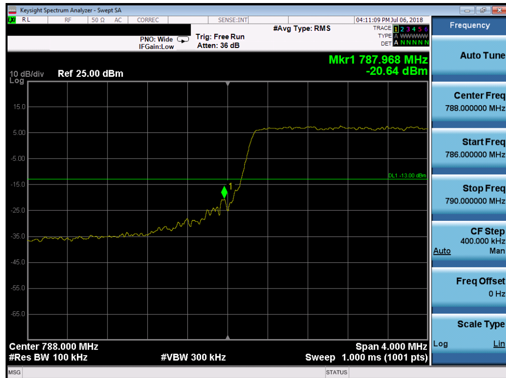
Plot 7-15. Lower Band Edge Plot (LTE Band 14, 5MHz QPSK – RB Size 25)
