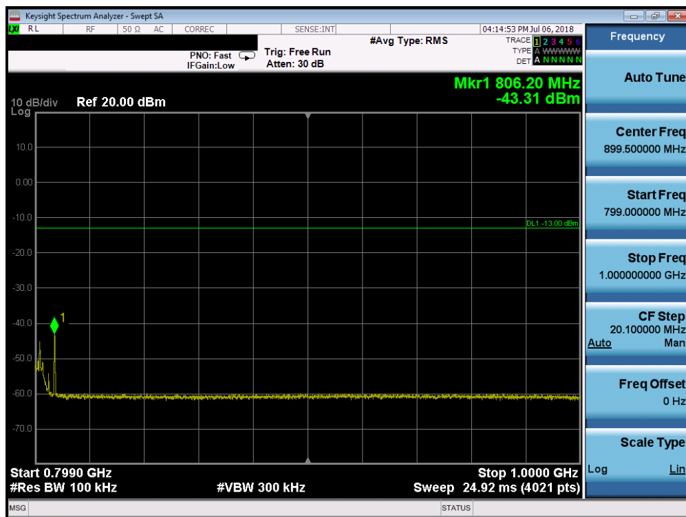
Plot 7-12. Conducted Spurious Plot (LTE Band 14, 10MHz QPSK – RB Size 1, RB Offset 0 – High Channel)
