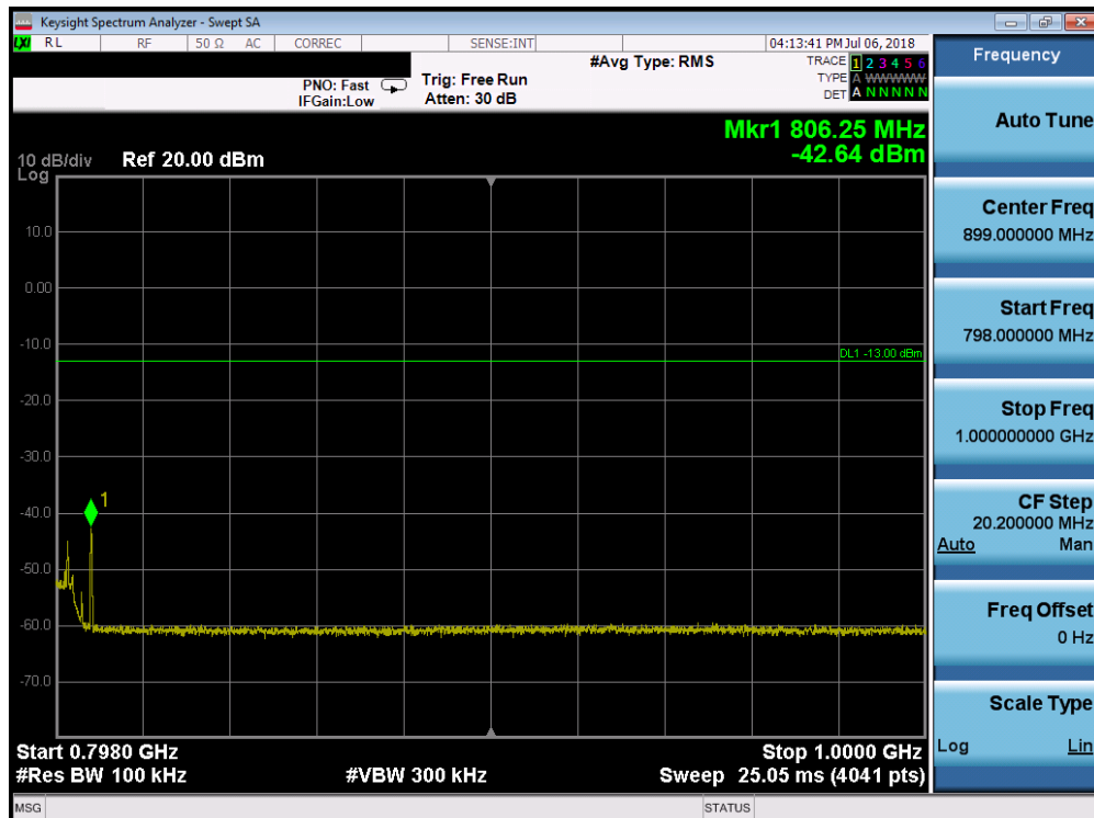
Plot 7-6. Conducted Spurious Plot (LTE Band 14, 10MHz QPSK – RB Size 1, RB Offset 0 – Low Channel)
