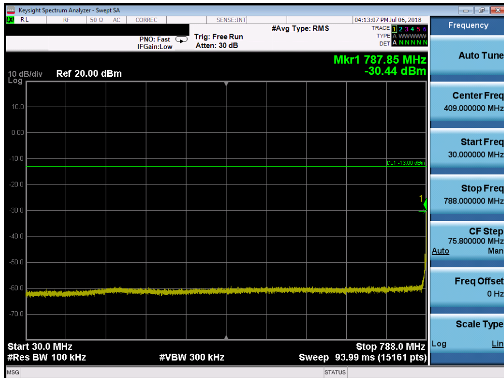
Plot 7-8. Conducted Spurious Plot (LTE Band 14, 10MHz QPSK – RB Size 1, RB Offset 0 – Mid Channel)
