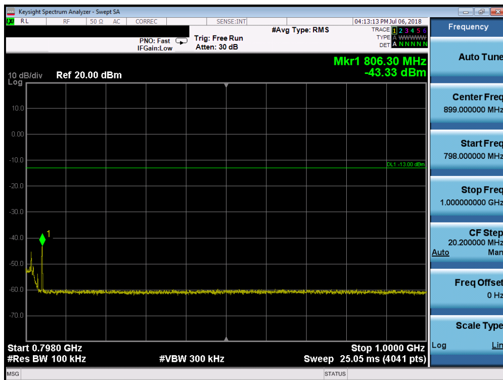
Plot 7-9. Conducted Spurious Plot (LTE Band 14, 10MHz QPSK – RB Size 1, RB Offset 0 – Mid Channel)
