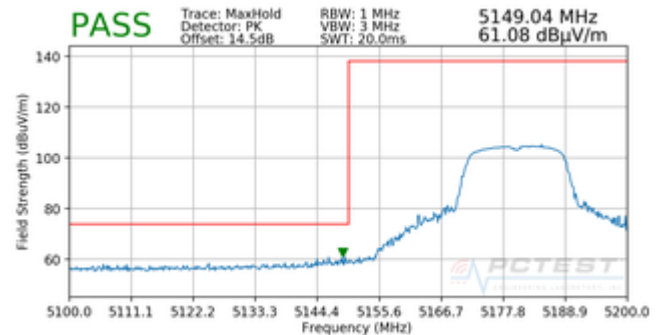
Plot 7-86. Radiated Lower Band Edge Plot (Peak – UNII Band 1)
