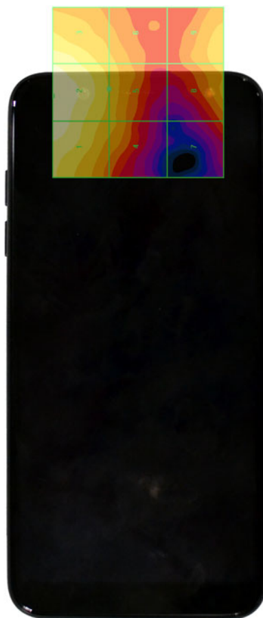
Figure 17-4 E-Field WD Scan overlay
