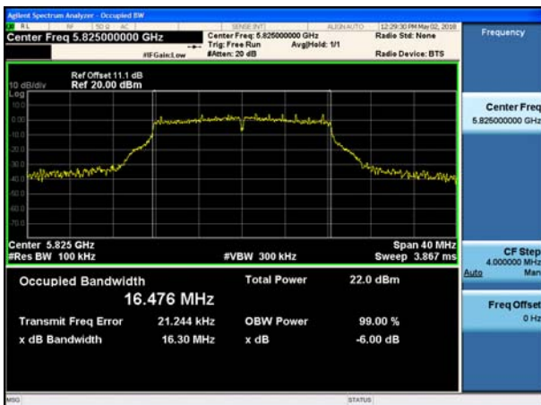
802.11a UNII 3 BAND 6dB Bandwidth (CH.165)
