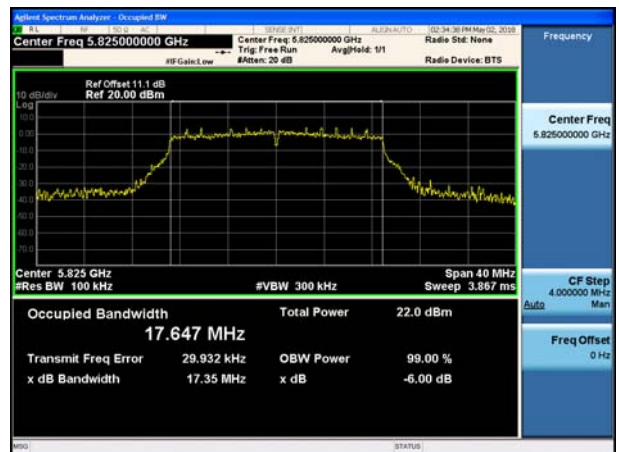
802.11n_HT20 UNII 3 BAND 6dB Bandwidth(CH.165)
