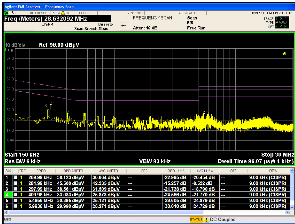
Plot 7-32. Line Conducted Plot with Bluetooth LE (N)
