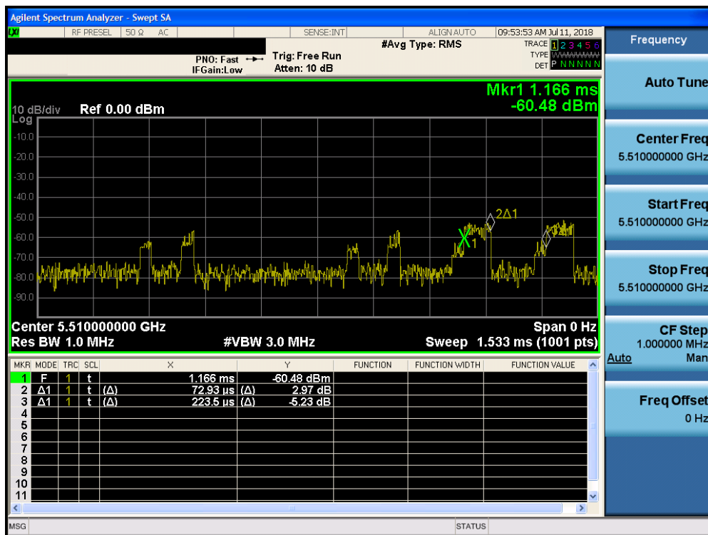
Figure 5-2. Band 2C Pulse Width and Period
