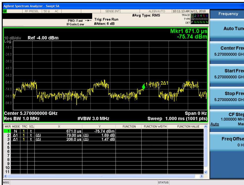
Figure 5-1. Band 2A Pulse Width and Period
