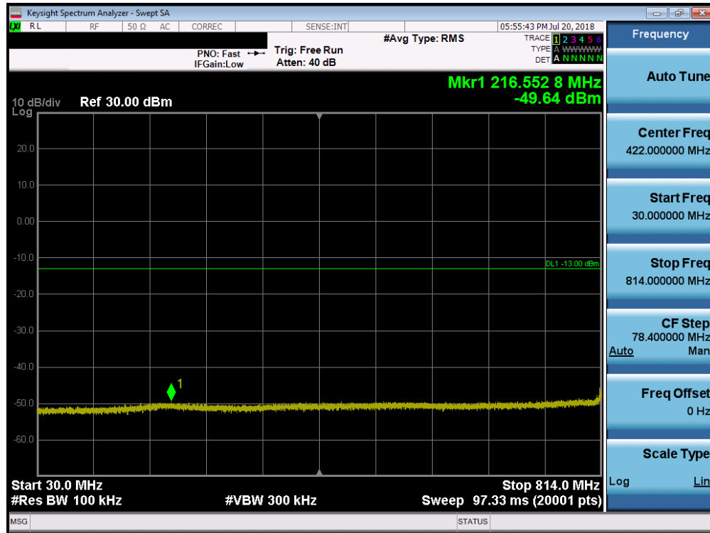
Plot 7-19. Conducted Spurious Plot (LTE B26 – 10MHz QPSK – RB Size 1, RB Offset 0)
