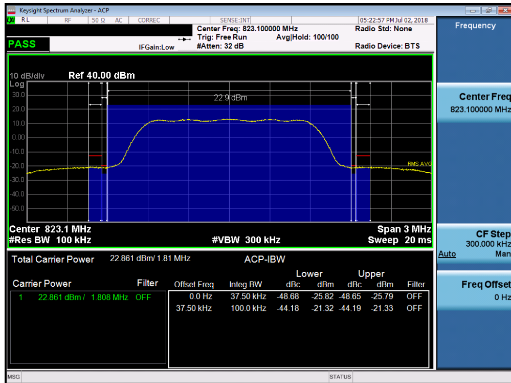
Plot 7-23. Channel Edge Plot (CDMA BC10 - Ch. 684)
