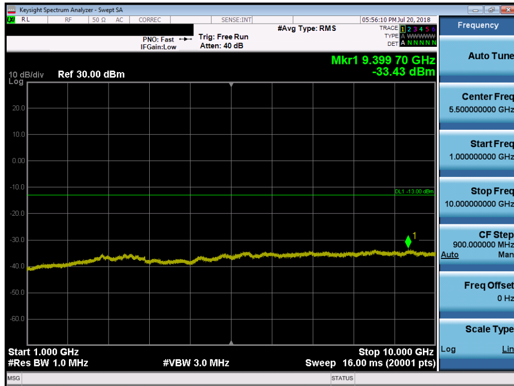
Plot 7-21. Conducted Spurious Plot (LTE B26 – 10MHz QPSK – RB Size 1, RB Offset 0)
