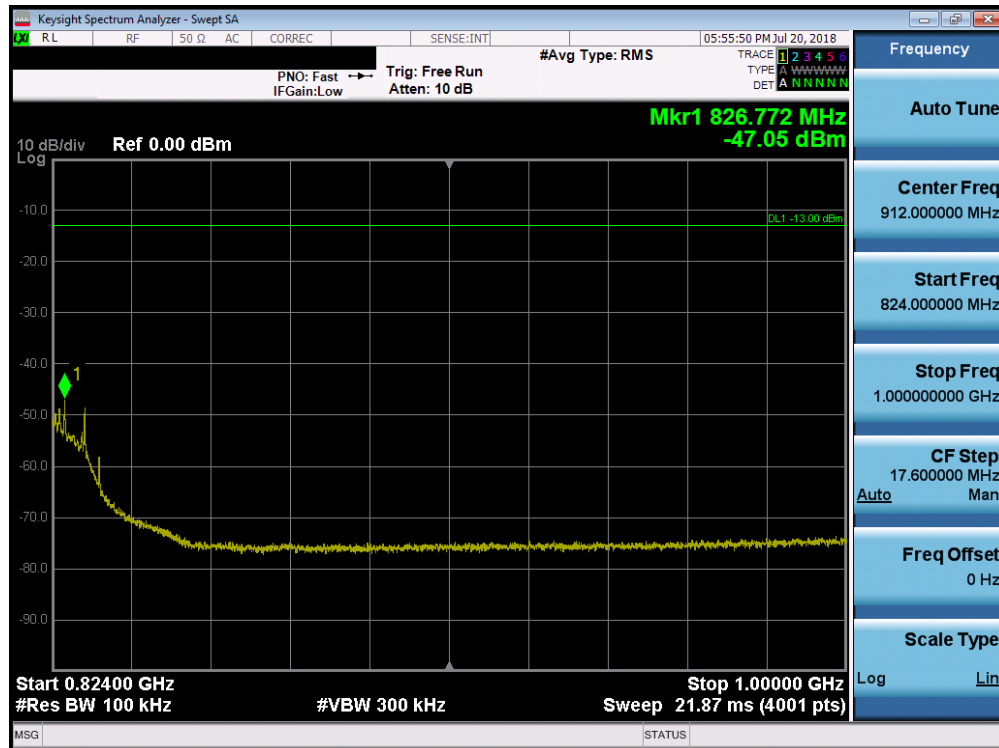
Plot 7-20. Conducted Spurious Plot (LTE B26 – 10MHz QPSK – RB Size 1, RB Offset 0)
